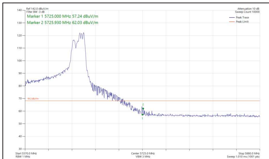
Figure 564 - 802.11ax HE80, RU 106-60, CDD, Core 0 + Core 1 - 5610 MHz Band Edge Frequency 5725 MHz
