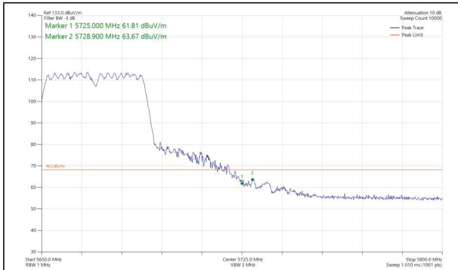
Figure 490 - 802.11n HT40, CDD, Core 0 + Core 1 - 5670 MHz Band Edge Frequency 5725 MHz
