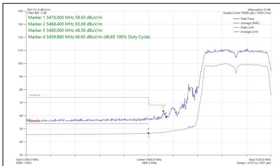
Figure 519 - 802.11ac VHT40, TxBF, Core 0 + Core 1 - 5510 MHz Band Edge Frequency 5470 MHz
