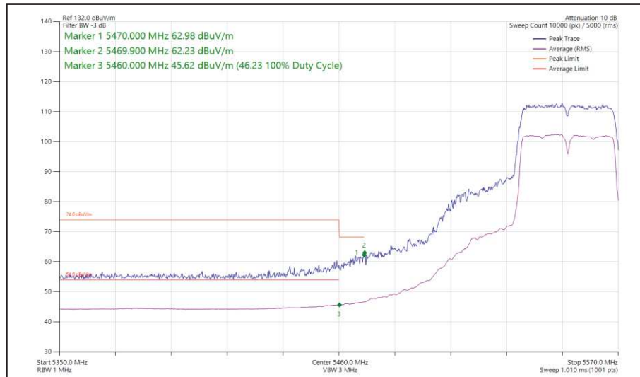
Figure 463 - 802.11n HT40, SISO, Core 1 - 5550 MHz Band Edge Frequency 5470 MHz
