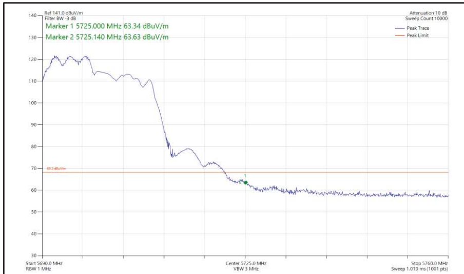
Figure 425 - 802.11ax HE20, RU 106-53, SDM, Core 0 + Core 1 - 5700 MHz Band Edge Frequency 5725 MHz
