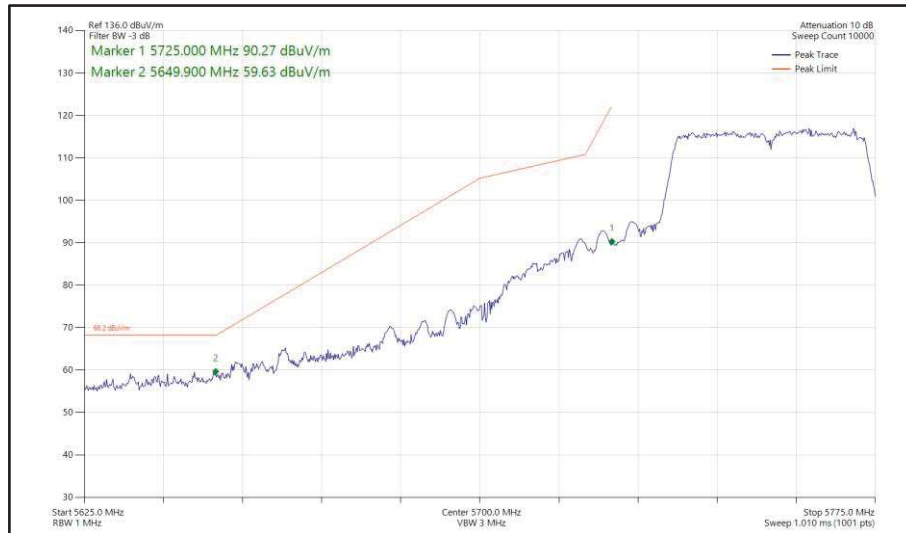
Figure 505 - 802.11n HT40, SDM, Core 0 + Core 1 - 5755 MHz Band Edge Frequency 5725 MHz
