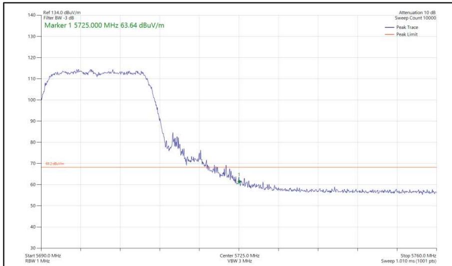
Figure 439 - 802.11ac VHT20, TxBF, Core 0 + Core 1 - 5700 MHz Band Edge Frequency 5725 MHz
