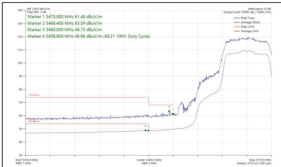
Figure 434 - 802.11ac VHT20, TxBF, Core 0 + Core 1 - 5500 MHz Band Edge Frequency 5470 MHz
