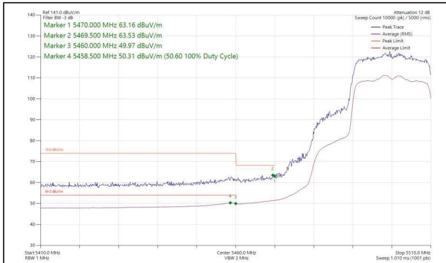
Figure 413 - 802.11ax HE20, SU, SDM, Core 0 + Core 1 - 5500 MHz Band Edge Frequency 5470 MHz
