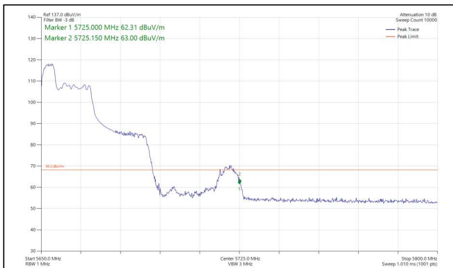
Figure 455 - 802.11ax HE40, RU 52-37, SISO, Core 0 - 5670 MHz Band Edge Frequency 5725 MHz
