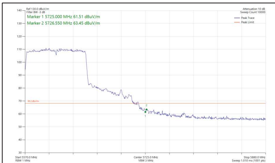
Figure 547 - 802.11ac VHT80, SISO, Core 1 - 5610 MHz Band Edge Frequency 5725 MHz
