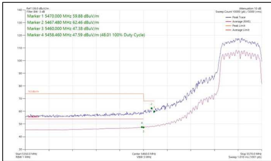
Figure 482 - 802.11n HT40, CDD, Core 0 + Core 1 - 5550 MHz Band Edge Frequency 5470 MHz
