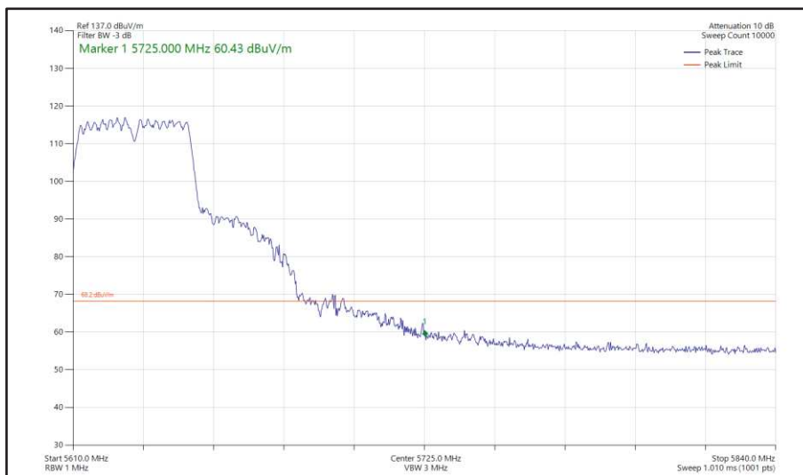
Figure 489 - 802.11n HT40, CDD, Core 0 + Core 1 - 5630 MHz Band Edge Frequency 5725 MHz
