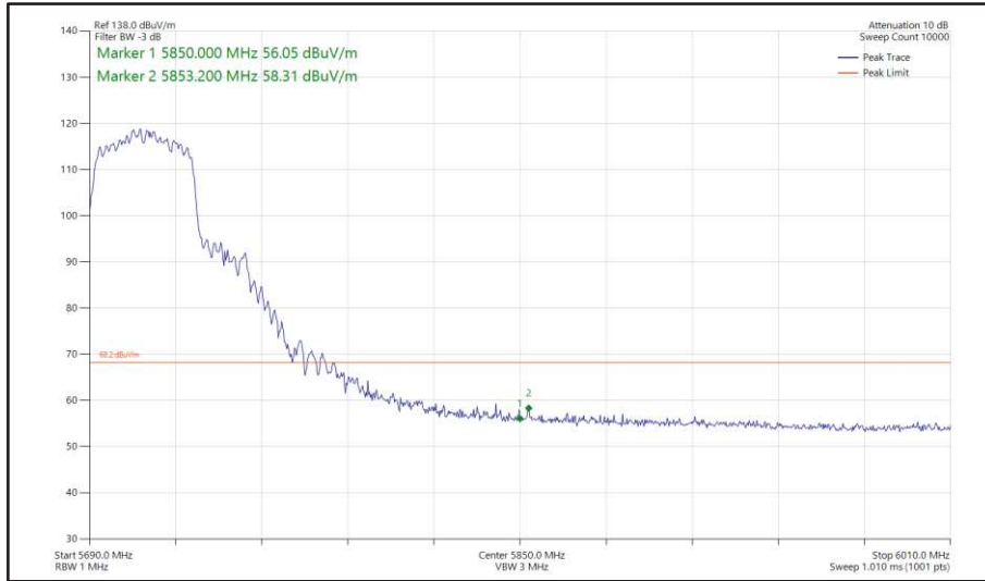
Figure 494 - 802.11n HT40, CDD, Core 0 + Core 1 - 5710 MHz Band Edge Frequency 5850 MHz
