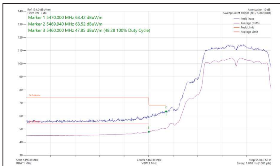
Figure 500 - 802.11n HT40, SDM, Core 0 + Core 1 - 5510 MHz Band Edge Frequency 5470 MHz
