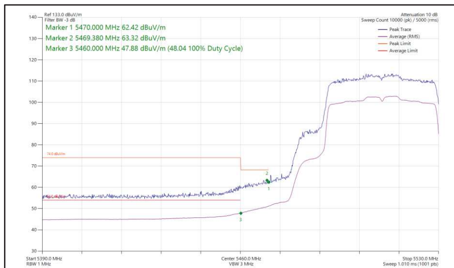
Figure 464 - 802.11ax HE40, SU, SISO, Core 1 - 5510 MHz Band Edge Frequency 5470 MHz
