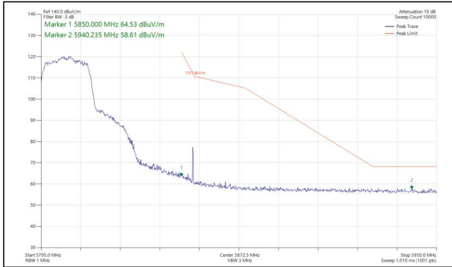
Figure 441 - 802.11ac VHT20, TxBF, Core 0 + Core 1 - 5805 MHz Band Edge Frequency 5850 MHz
