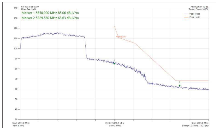
Figure 554 - 802.11ax HE80, SU, SISO, Core 1 - 5775 MHz Band Edge Frequency 5850 MHz
