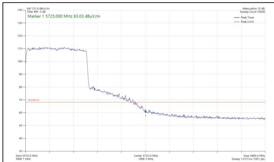
Figure 548 - 802.11ax HE80, SU, SISO, Core 1 - 5610 MHz Band Edge Frequency 5725 MHz
