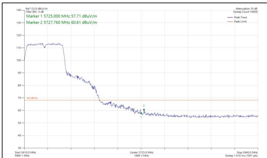
Figure 470 - 802.11n HT40, SISO, Core 1 - 5630 MHz Band Edge Frequency 5725 MHz
