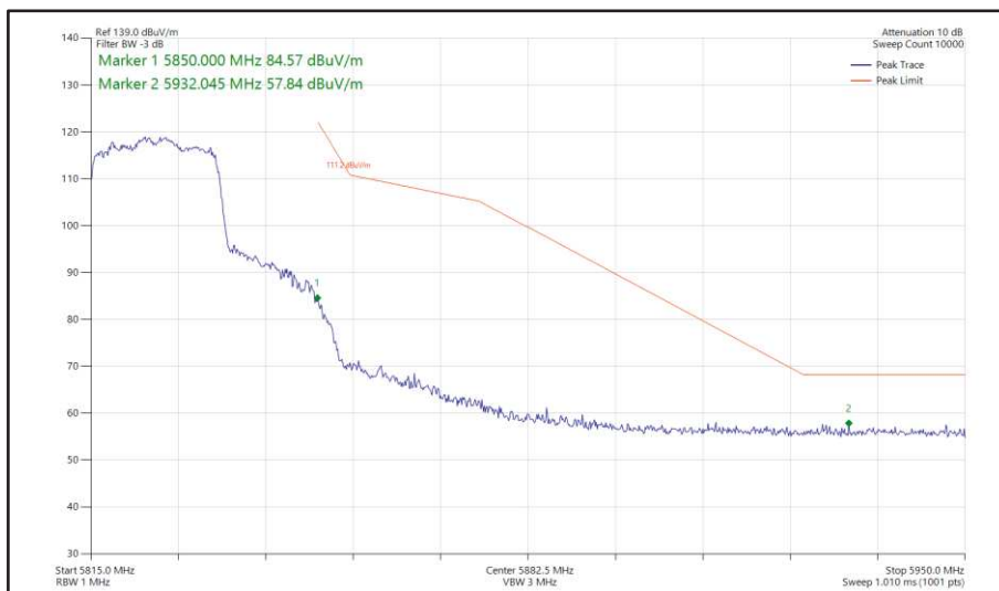
Figure 432 - 802.11ax HE20, SU, SDM, Core 0 + Core 1 - 5825 MHz Band Edge Frequency 5850 MHz
