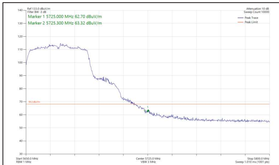
Figure 471 - 802.11n HT40, SISO, Core 1 - 5670 MHz Band Edge Frequency 5725 MHz
