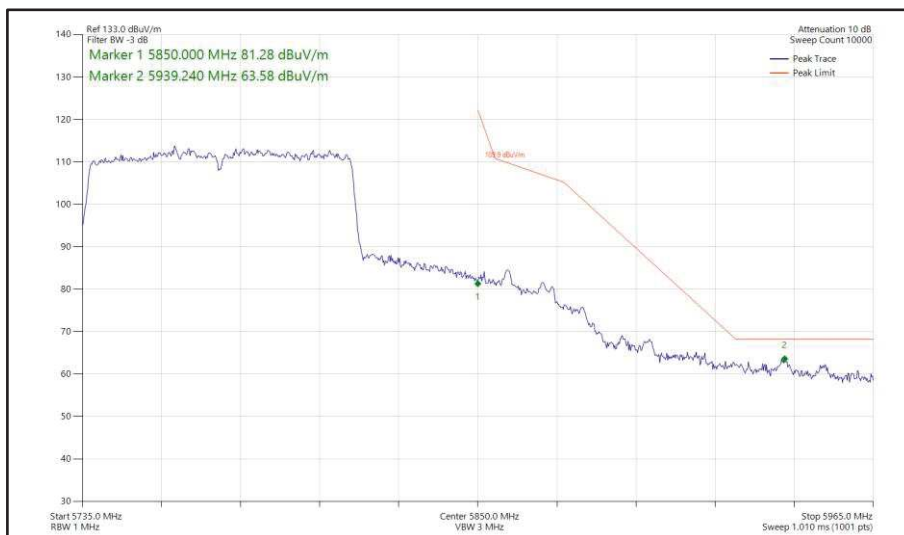
Figure 551 - 802.11ac VHT80, SISO, Core 1 - 5775 MHz Band Edge Frequency 5850 MHz
