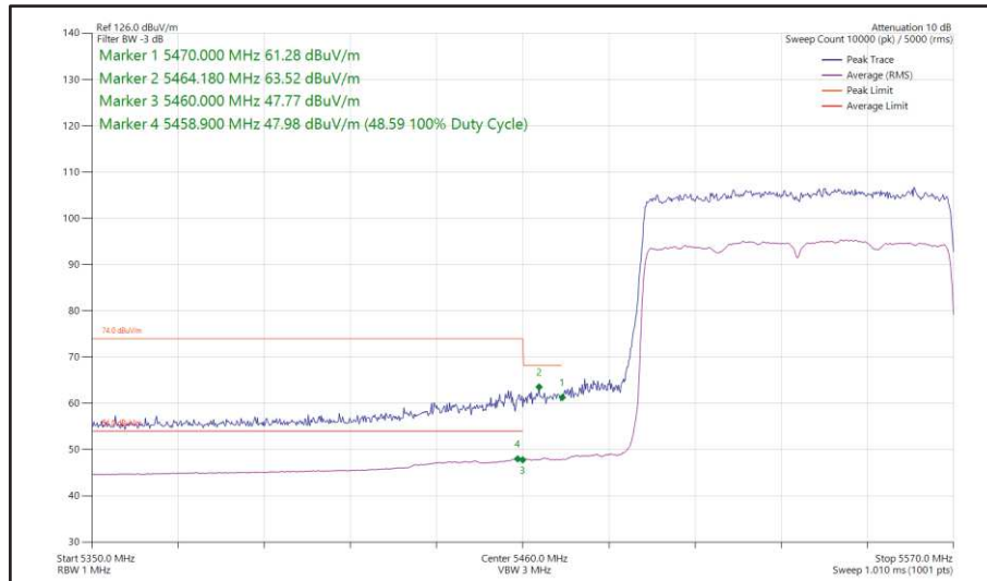
Figure 542 - 802.11ax HE80, SU, SISO, Core 1 - 5530 MHz Band Edge Frequency 5470 MHz
