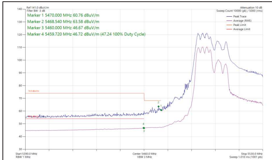
Figure 484 - 802.11ax HE40, RU 106-53, CDD, Core 0 + Core 1 - 5510 MHz Band Edge Frequency 5470 MHz
