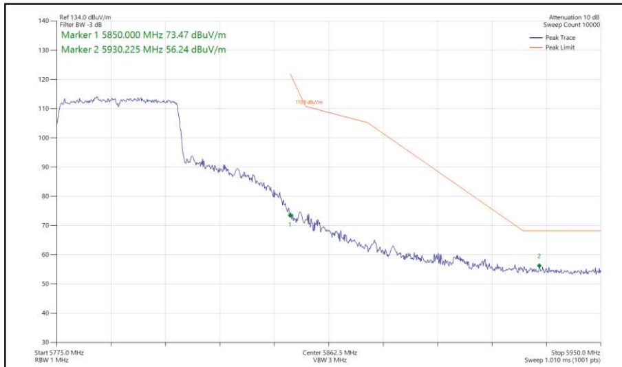
Figure 460 - 802.11ax HE40, SU, SISO, Core 0 - 5795 MHz Band Edge Frequency 5850 MHz
