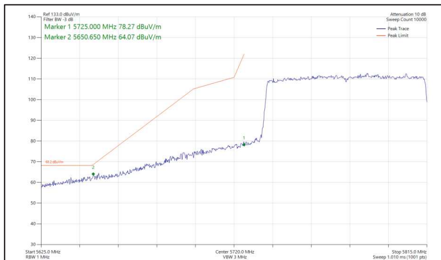
Figure 545 - 802.11ax HE80, SU, SISO, Core 1 - 5775 MHz Band Edge Frequency 5725 MHz
