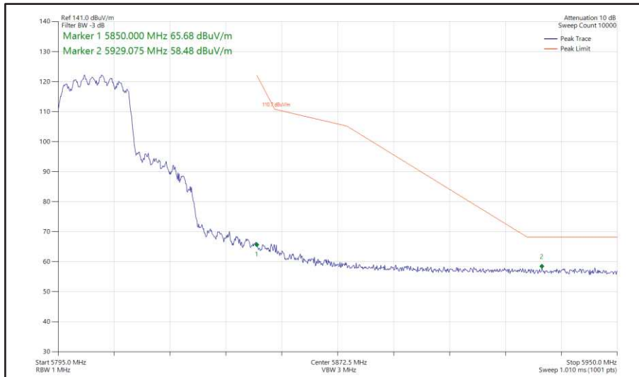
Figure 408 - 802.11ax HE20, SU, CDD, Core 0 + Core 1 - 5805 MHz Band Edge Frequency 5850 MHz
