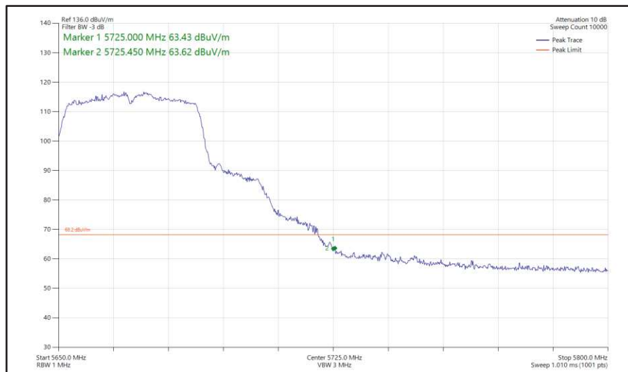
Figure 509 - 802.11n HT40, SDM, Core 0 + Core 1 - 5670 MHz Band Edge Frequency 5725 MHz
