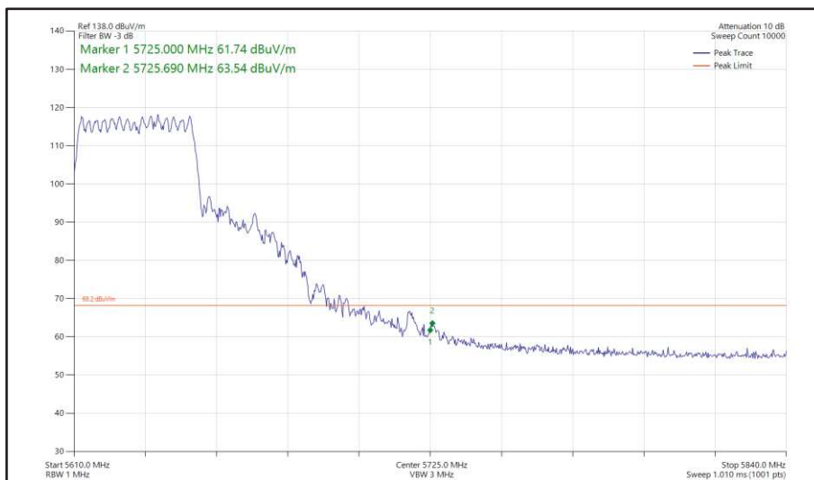
Figure 491 - 802.11ax HE40, SU, CDD, Core 0 + Core 1 - 5630 MHz Band Edge Frequency 5725 MHz
