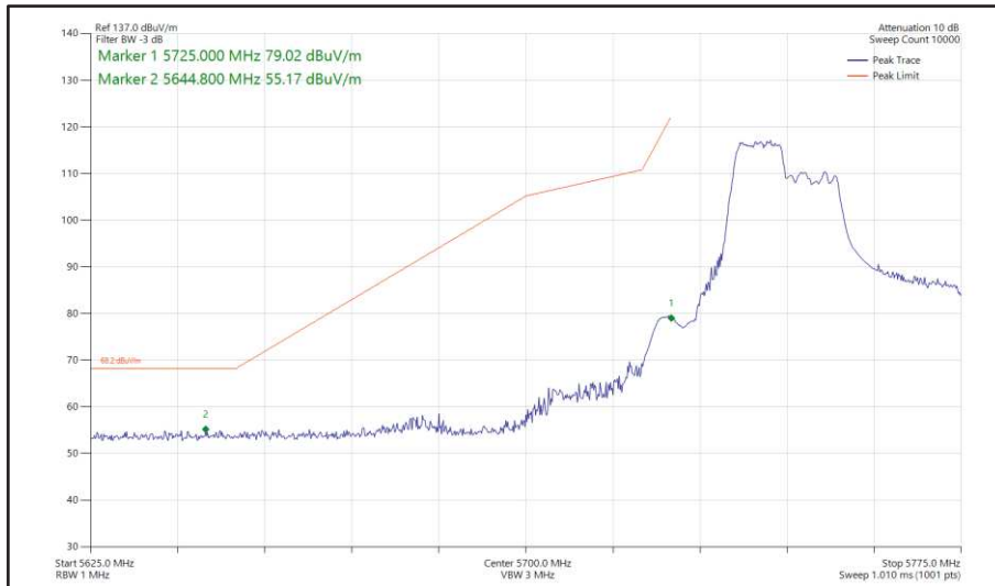
Figure 450 - 802.11ax HE40, RU 106-53, SISO, Core 0 - 5755 MHz Band Edge Frequency 5725 MHz
