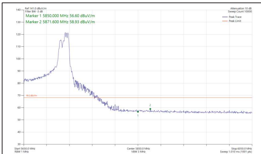
Figure 568 - 802.11ax HE80, RU 106-60, CDD, Core 0 + Core 1 - 5690 MHz Band Edge Frequency 5850 MHz
