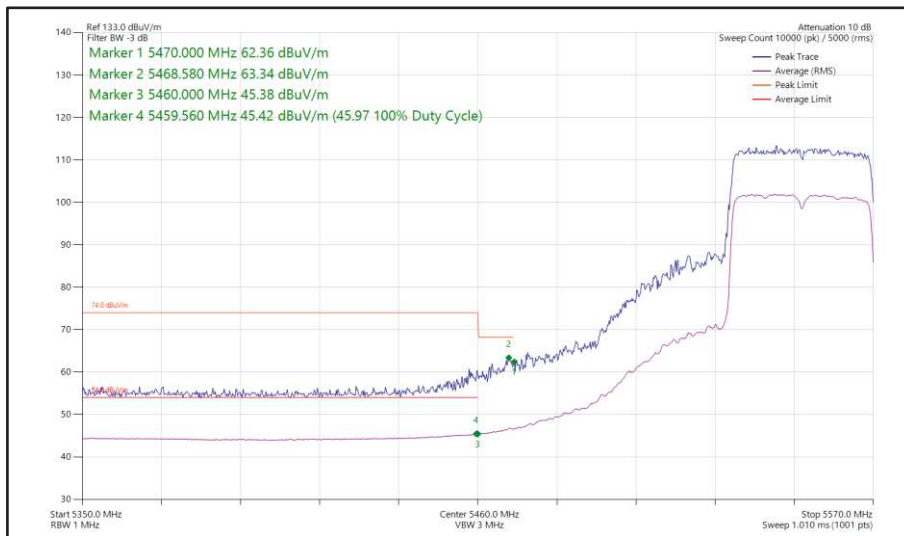
Figure 466 - 802.11ax HE40, SU, SISO, Core 1 - 5550 MHz Band Edge Frequency 5470 MHz
