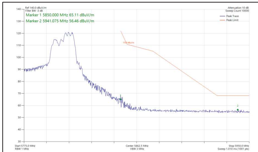
Figure 518 - 802.11ax HE40, RU 106-56, SDM, Core 0 + Core 1 - 5795 MHz Band Edge Frequency 5850 MHz
