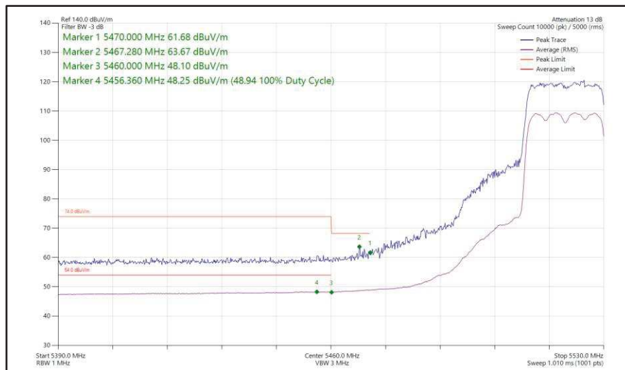
Figure 415 - 802.11ax HE20, SU, SDM, Core 0 + Core 1 - 5520 MHz Band Edge Frequency 5470 MHz
