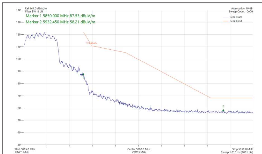
Figure 409 - 802.11ax HE20, SU, CDD, Core 0 + Core 1 - 5825 MHz Band Edge Frequency 5850 MHz
