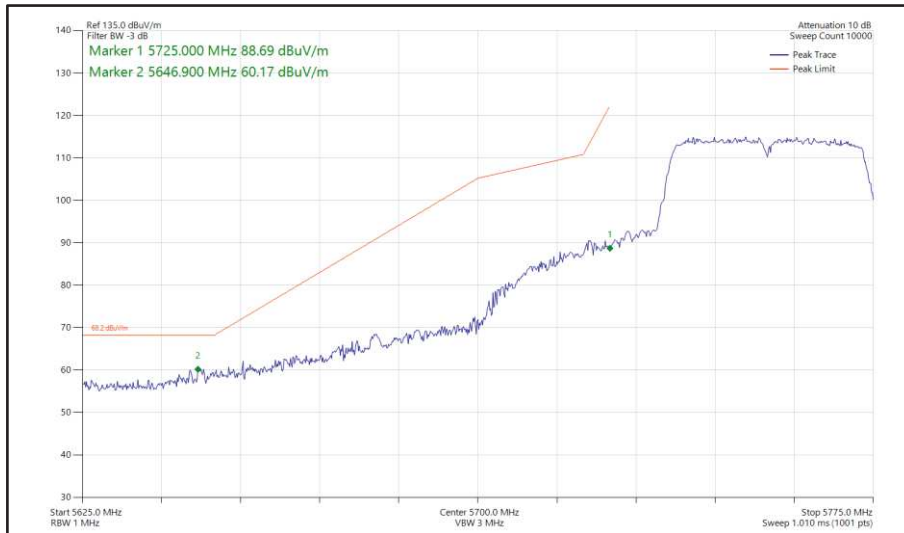
Figure 448 - 802.11n HT40, SISO, Core 0 - 5755 MHz Band Edge Frequency 5725 MHz
