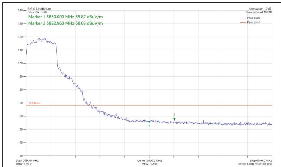
Figure 515 - 802.11ax HE40, SU, SDM, Core 0 + Core 1 - 5710 MHz Band Edge Frequency 5850 MHz
