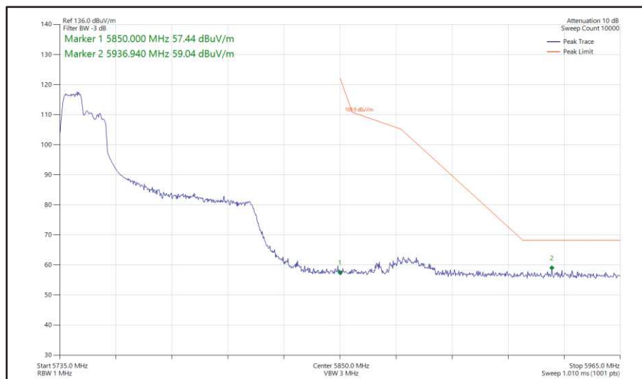
Figure 540 - 802.11ax HE80, RU 106-53, SISO, Core 0 - 5775 MHz Band Edge Frequency 5850 MHz
