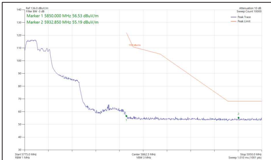
Figure 461 - 802.11ax HE40, RU 106-53, SISO, Core 0 - 5795 MHz Band Edge Frequency 5850 MHz
