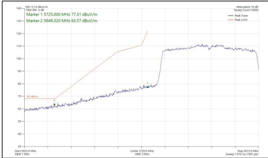
Figure 529 - 802.11ac VHT80, SISO, Core 0 - 5775 MHz Band Edge Frequency 5725 MHz
