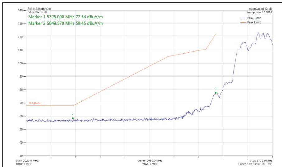
Figure 419 - 802.11ax HE20, RU 106-54, SDM, Core 0 + Core 1 - 5745 MHz Band Edge Frequency 5725 MHz
