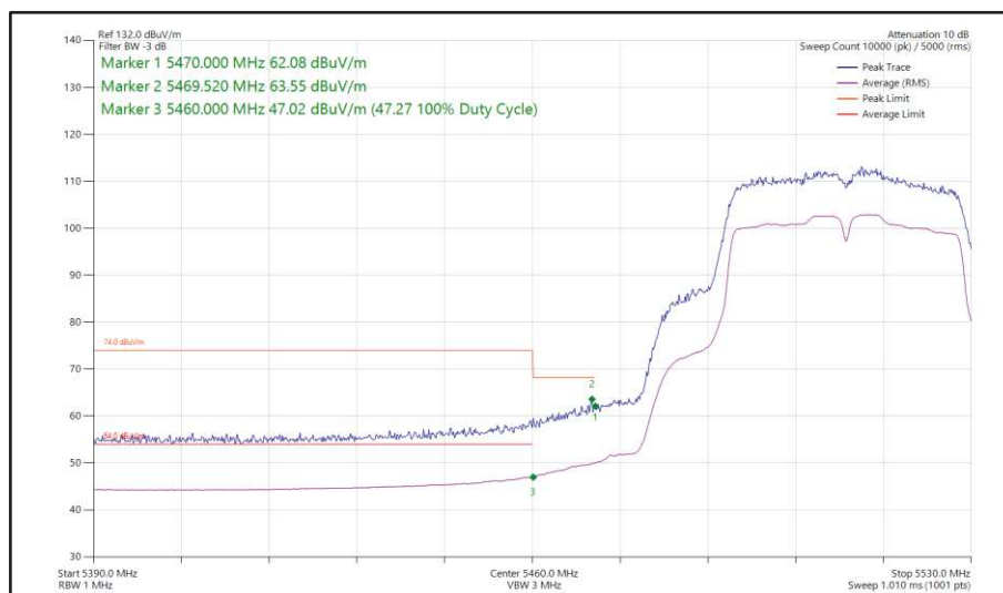
Figure 462 - 802.11n HT40, SISO, Core 1 - 5510 MHz Band Edge Frequency 5470 MHz
