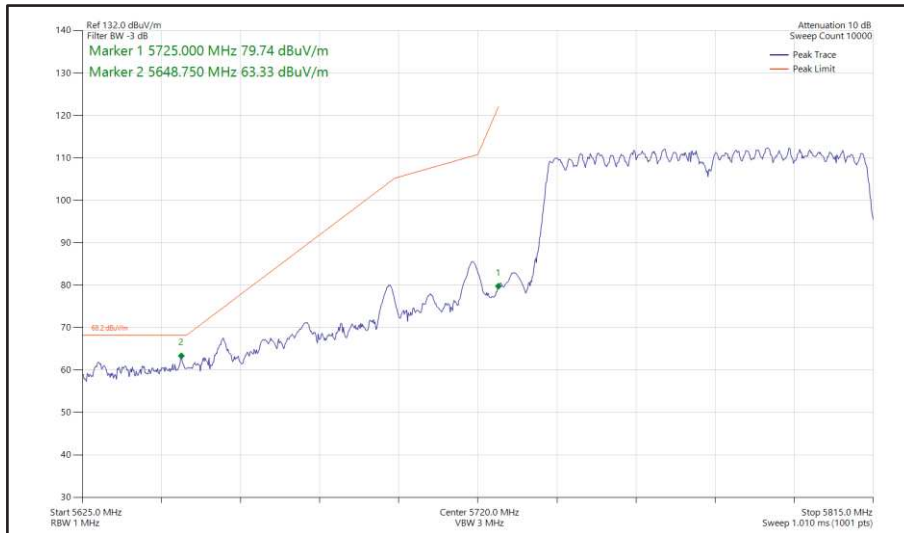
Figure 559 - 802.11ac VHT80, CDD, Core 0 + Core 1 - 5775 MHz Band Edge Frequency 5725 MHz
