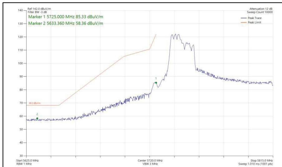
Figure 561 - 802.11ax HE80, RU 106-53, CDD, Core 0 + Core 1 - 5775 MHz Band Edge Frequency 5725 MHz
