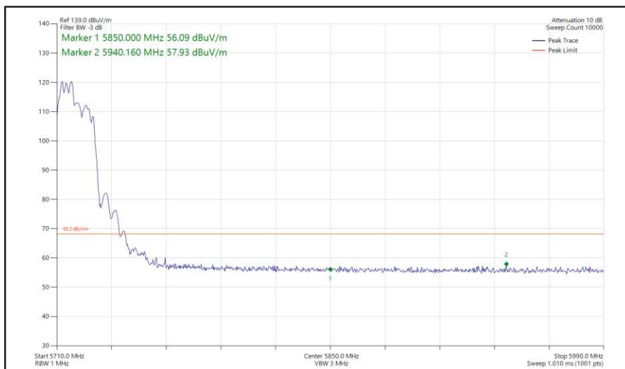
Figure 430 - 802.11ax HE20, RU 106-53, SDM, Core 0 + Core 1 - 5720 MHz Band Edge Frequency 5850 MHz
