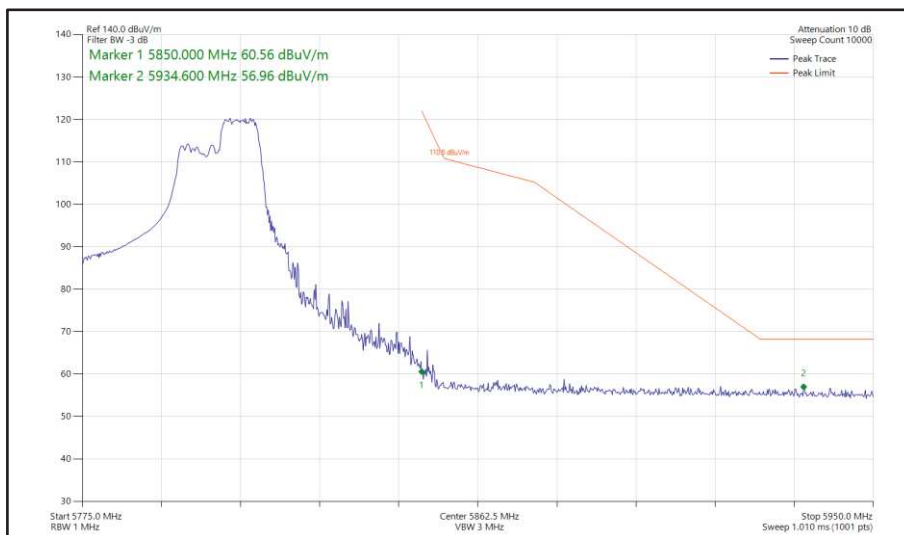
Figure 480 - 802.11ax HE40, RU 106-56, SISO, Core 1 - 5795 MHz Band Edge Frequency 5850 MHz
