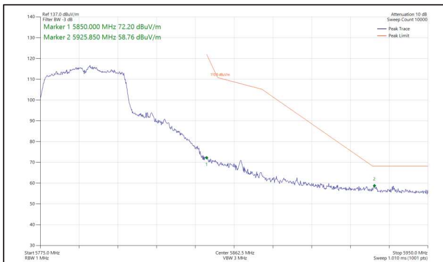
Figure 476 - 802.11n HT40, SISO, Core 1 - 5795 MHz Band Edge Frequency 5850 MHz
