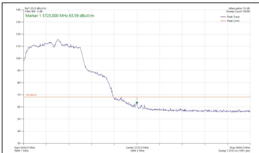
Figure 523 - 802.11ac VHT40, TxBF, Core 0 + Core 1 - 5670 MHz Band Edge Frequency 5725 MHz
