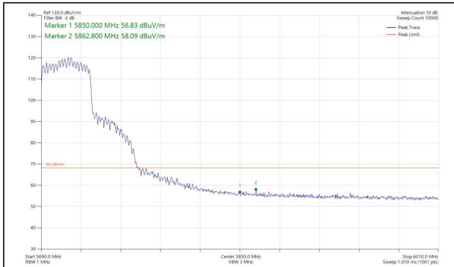
Figure 496 - 802.11ax HE40, SU, CDD, Core 0 + Core 1 - 5710 MHz Band Edge Frequency 5850 MHz
