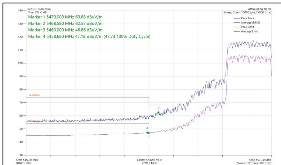
Figure 485 - 802.11ax HE40, SU, CDD, Core 0 + Core 1 - 5550 MHz Band Edge Frequency 5470 MHz
