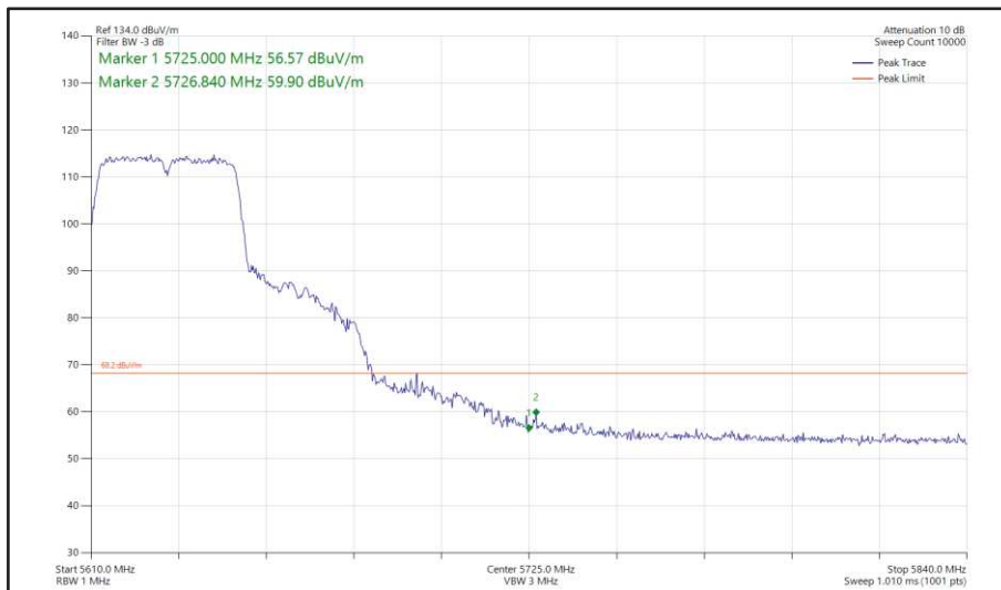
Figure 451 - 802.11n HT40, SISO, Core 0 - 5630 MHz Band Edge Frequency 5725 MHz
