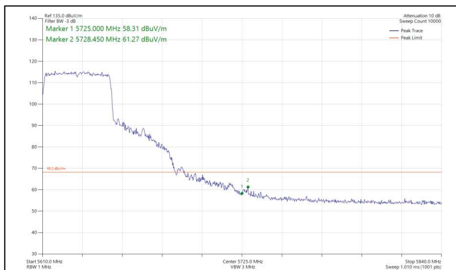
Figure 453 - 802.11ax HE40, SU, SISO, Core 0 - 5630 MHz Band Edge Frequency 5725 MHz
