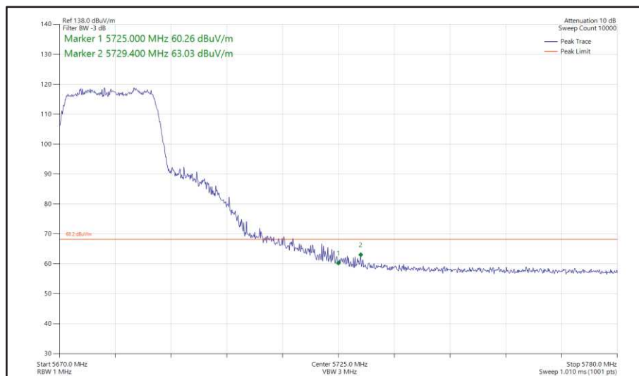
Figure 438 - 802.11ac VHT20, TxBF, Core 0 + Core 1 - 5680 MHz Band Edge Frequency 5725 MHz
