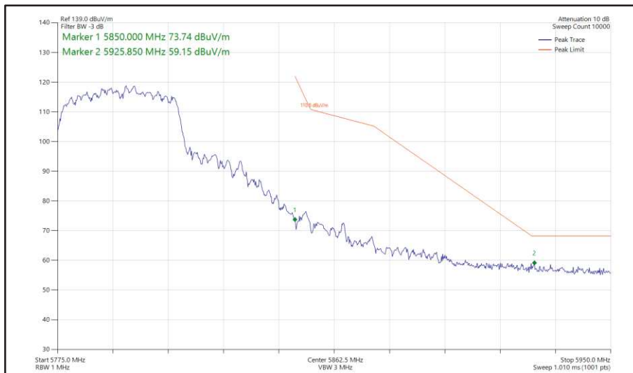
Figure 495 - 802.11n HT40, CDD, Core 0 + Core 1 - 5795 MHz Band Edge Frequency 5850 MHz
