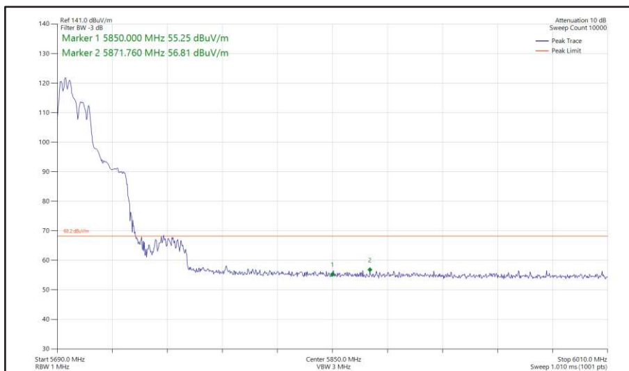
Figure 497 - 802.11ax HE40, RU 106-53, CDD, Core 0 + Core 1 - 5710 MHz Band Edge Frequency 5850 MHz
