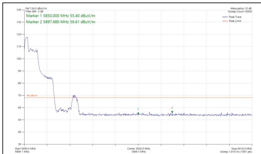
Figure 478 - 802.11ax HE40, RU 52-37, SISO, Core 1 - 5710 MHz Band Edge Frequency 5850 MHz
