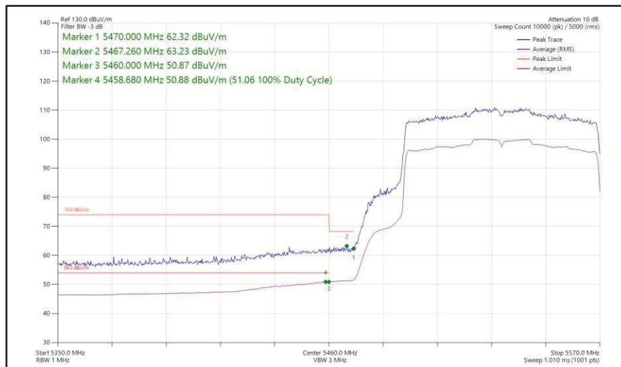
Figure 527 - 802.11ax HE80, SU, SISO, Core 0 - 5530 MHz Band Edge Frequency 5470 MHz
