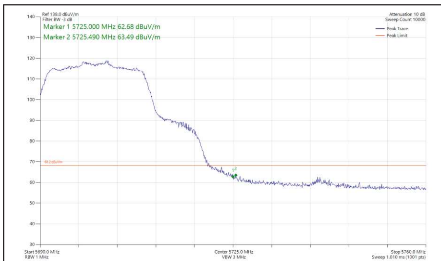
Figure 422 - 802.11n HT20, SDM, Core 0 + Core 1 - 5700 MHz Band Edge Frequency 5725 MHz
