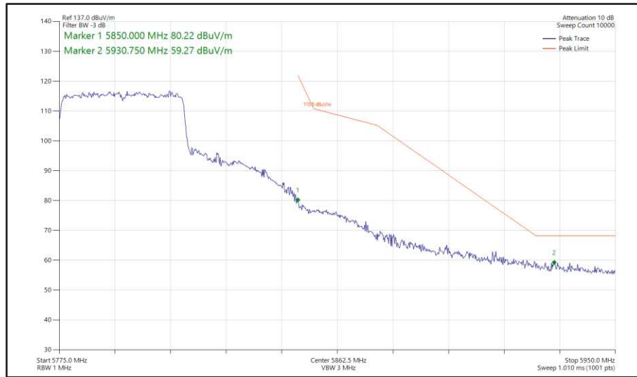
Figure 517 - 802.11ax HE40, SU, SDM, Core 0 + Core 1 - 5795 MHz Band Edge Frequency 5850 MHz
