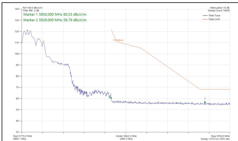
Figure 499 - 802.11ax HE40, RU 106-53, CDD, Core 0 + Core 1 - 5795 MHz Band Edge Frequency 5850 MHz
