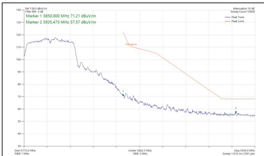
Figure 514 - 802.11n HT40, SDM, Core 0 + Core 1 - 5795 MHz Band Edge Frequency 5850 MHz
