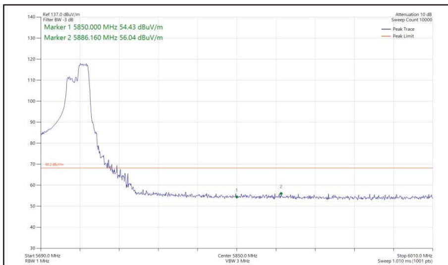
Figure 459 - 802.11ax HE40, RU 106-56, SISO, Core 0 - 5710 MHz Band Edge Frequency 5850 MHz
