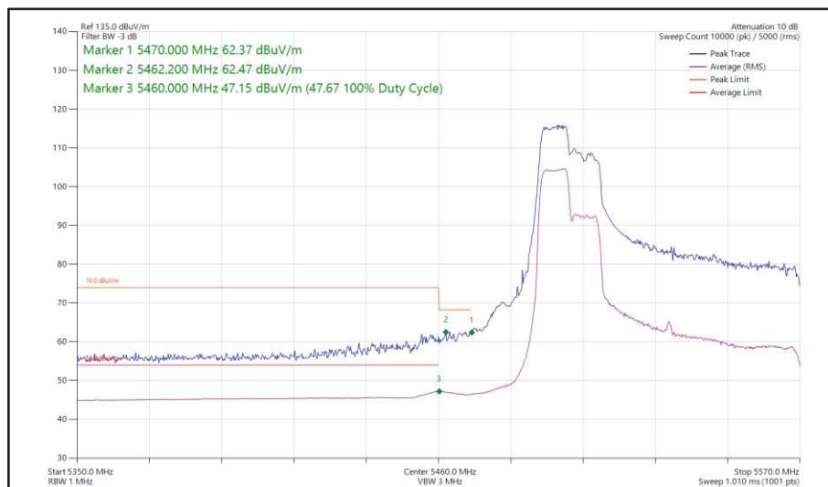
Figure 543 - 802.11ax HE80, RU 106-53, SISO, Core 1 - 5530 MHz Band Edge Frequency 5470 MHz
