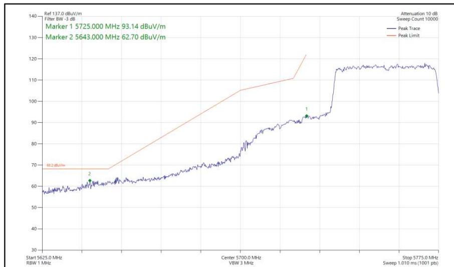
Figure 506 - 802.11ax HE40, SU, SDM, Core 0 + Core 1 - 5755 MHz Band Edge Frequency 5725 MHz
