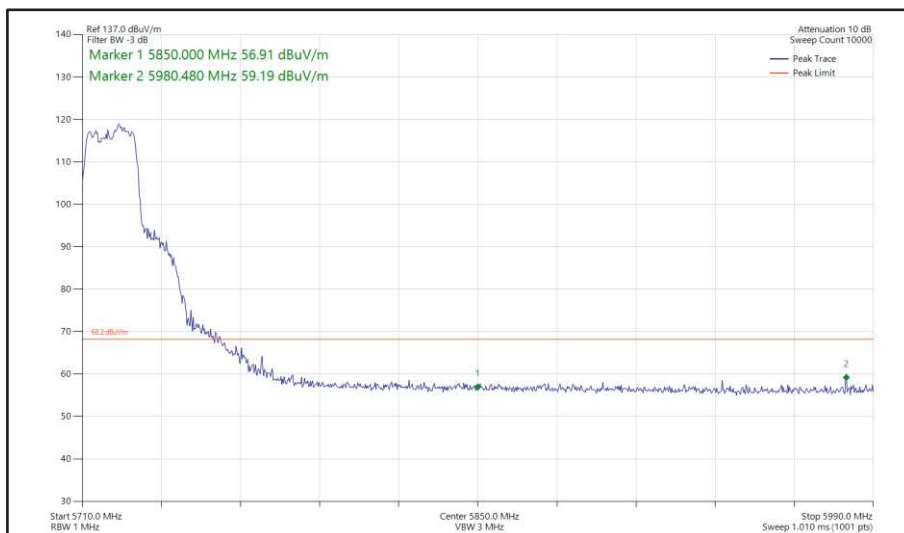
Figure 440 - 802.11ac VHT20, TxBF, Core 0 + Core 1 - 5720 MHz Band Edge Frequency 5850 MHz
