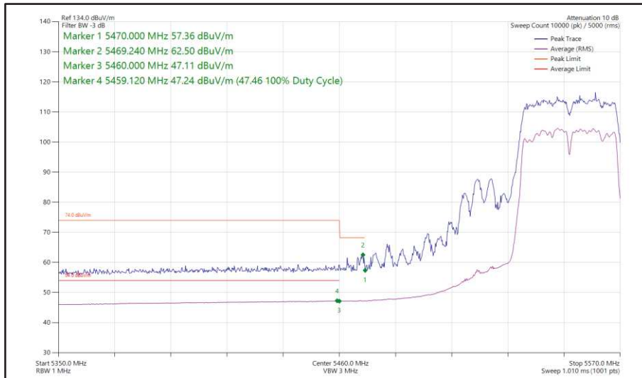
Figure 520 - 802.11ac VHT40, TxBF, Core 0 + Core 1 - 5550 MHz Band Edge Frequency 5470 MHz
