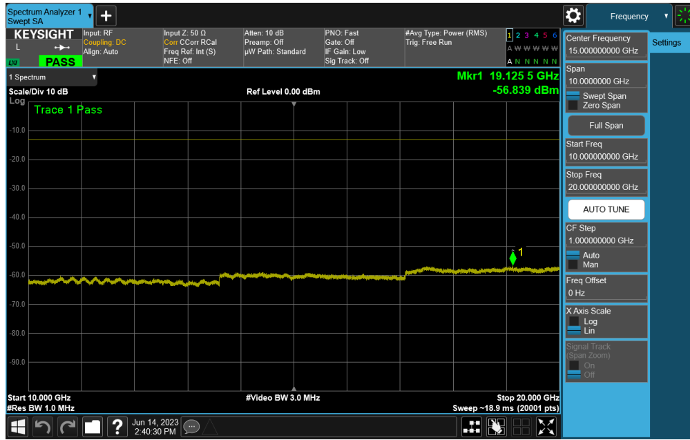
Plot 7-22. Conducted Spurious Plot (LTE Band 25/2 - 20MHz QPSK - RB Size 1, RB Offset 0 - High Channel)
