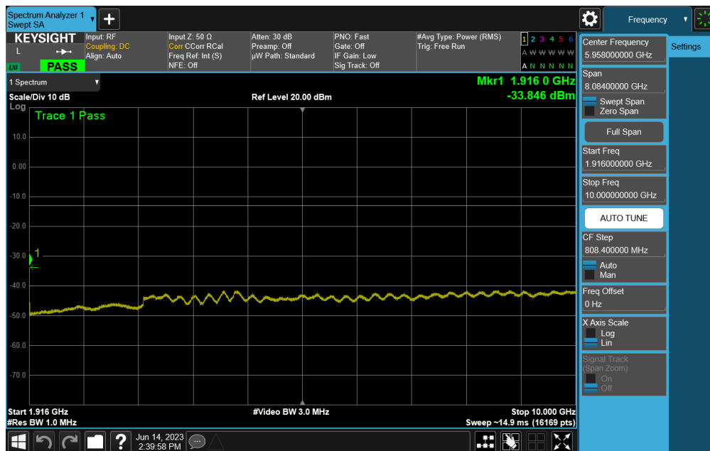
Plot 7-21. Conducted Spurious Plot (LTE Band 25/2 - 20MHz QPSK - RB Size 1, RB Offset 0 - High Channel)
