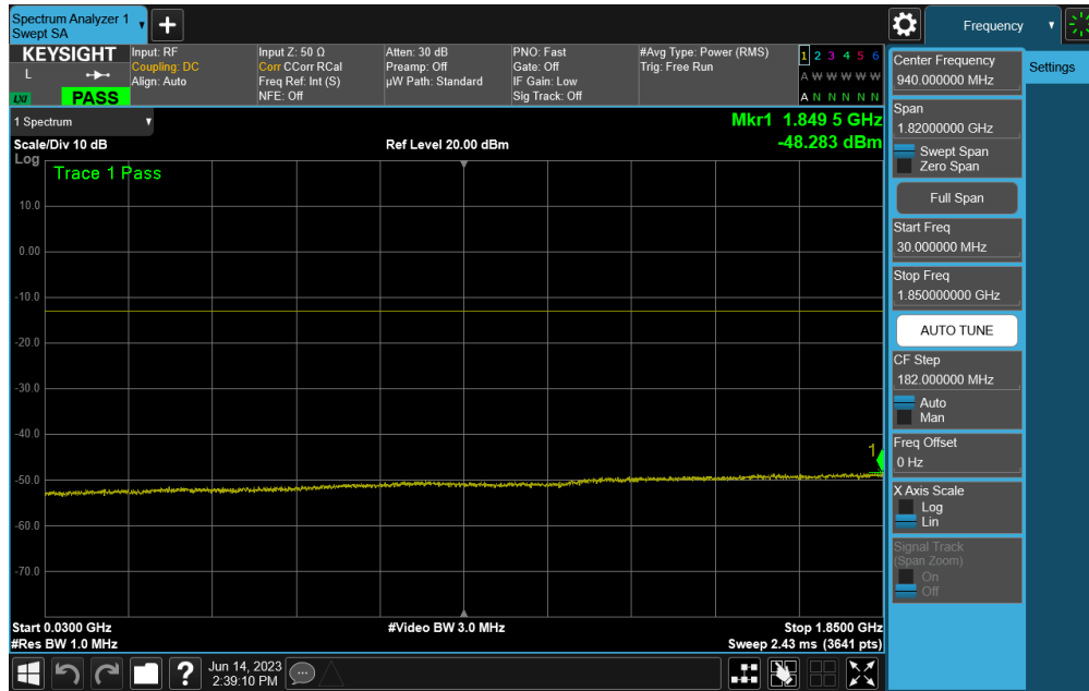
Plot 7-20. Conducted Spurious Plot (LTE Band 25/2 - 20MHz QPSK - RB Size 1, RB Offset 0 - High Channel)
