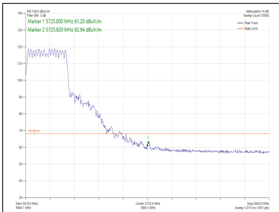
Figure 421 - 802.11ax, HE40, SU, CDD, Core 0-1 - 5630 MHz, Band Edge Frequency 5725 MHz
