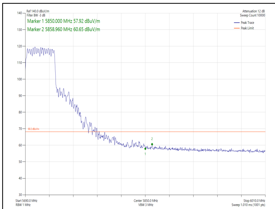
Figure 427 - 802.11ax, HE40, SU, CDD, Core 0-1 - 5710 MHz, Band Edge Frequency 5850 MHz
