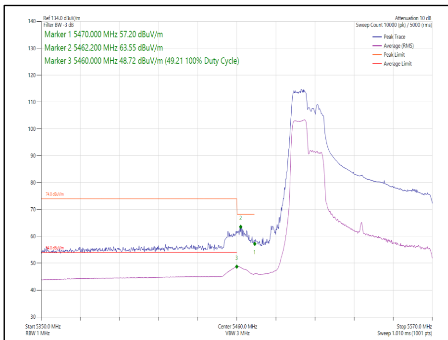
Figure 473 - 802.11ax, HE80, RU 106-53, SISO, Core 1 - 5530 MHz, Band Edge Frequency 5470 MHz
