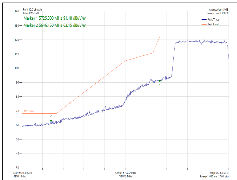
Figure 438 - 802.11ax, HE40, SU, SDM, Core 0-1 - 5755 MHz, Band Edge Frequency 5725 MHz
