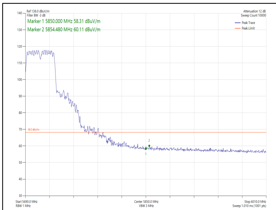
Figure 425 - 802.11n, HT40, CDD, Core 0-1 - 5710 MHz, Band Edge Frequency 5850 MHz
