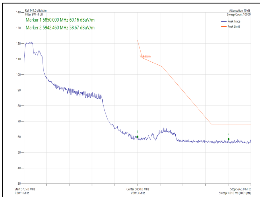
Figure 470 - 802.11ax, HE80, RU 106-53, SISO, Core 0 - 5775 MHz, Band Edge Frequency 5850 MHz
