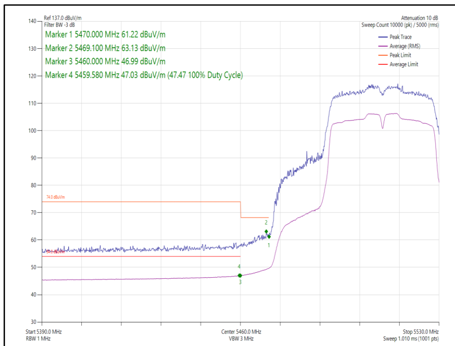
Figure 451 - 802.11ac, VHT40, TxBF, Core 0-1 - 5510 MHz, Band Edge Frequency 5470 MHz
