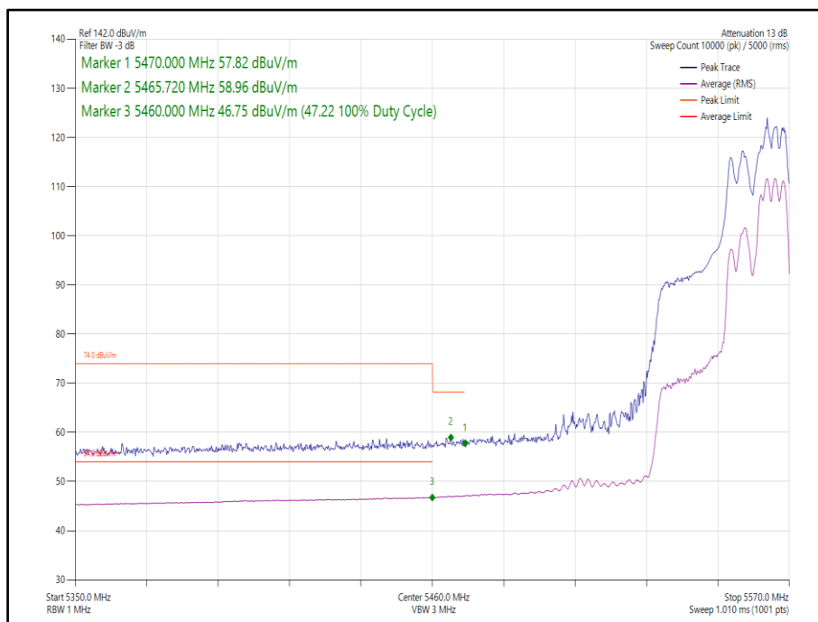
Figure 415 - 802.11ax, HE40, RU 106-56, CDD, Core 0-1 - 5550 MHz, Band Edge Frequency 5470 MHz
