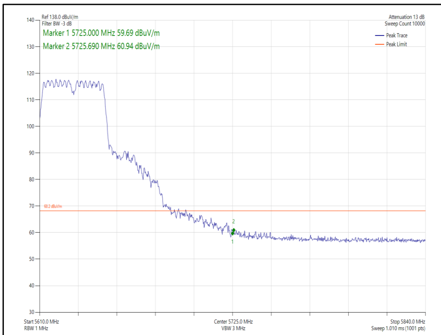
Figure 419 - 802.11n, HT40, CDD, Core 0-1 - 5630 MHz, Band Edge Frequency 5725 MHz
