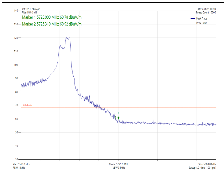
Figure 464 - 802.11ax, HE80, RU 106-60, SISO, Core 0 - 5610 MHz, Band Edge Frequency 5725 MHz
