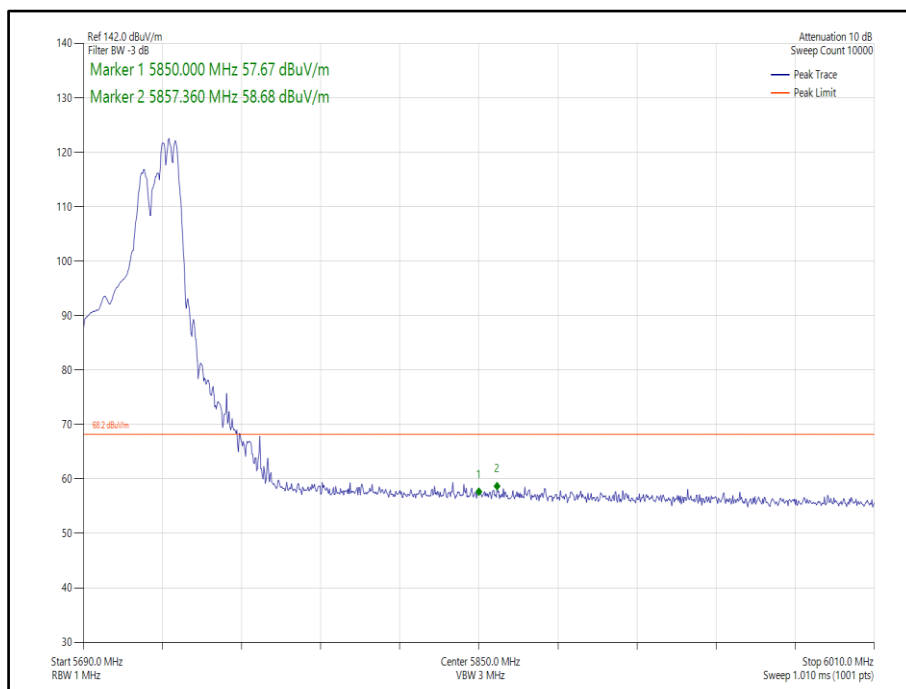
Figure 448 - 802.11ax, HE40, RU 106-56, SDM, Core 0-1 - 5710 MHz, Band Edge Frequency 5850 MHz
