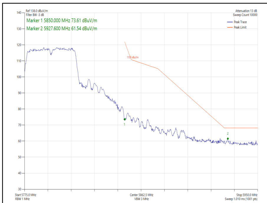
Figure 446 - 802.11n, HT40, SDM, Core 0-1 - 5795 MHz, Band Edge Frequency 5850 MHz
