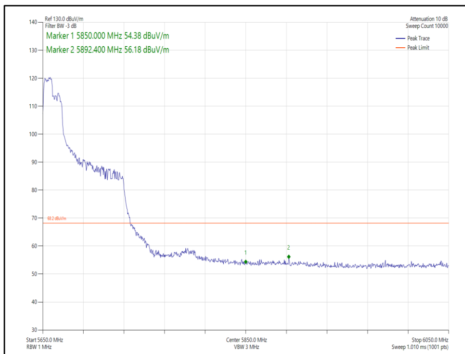
Figure 468 - 802.11ax, HE80, RU 106-53, SISO, Core 0 - 5690 MHz, Band Edge Frequency 5850 MHz
