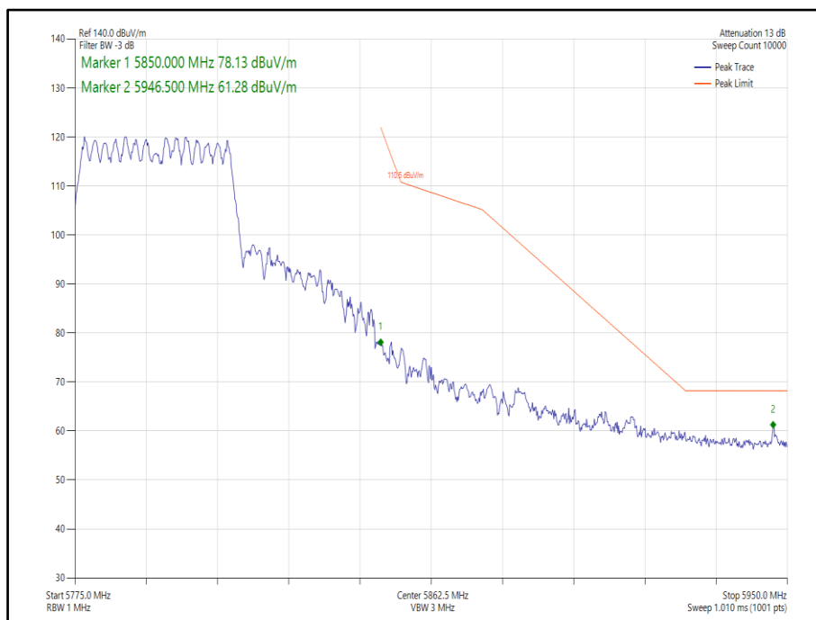
Figure 429 - 802.11ax, HE40, SU, CDD, Core 0-1 - 5795 MHz, Band Edge Frequency 5850 MHz
