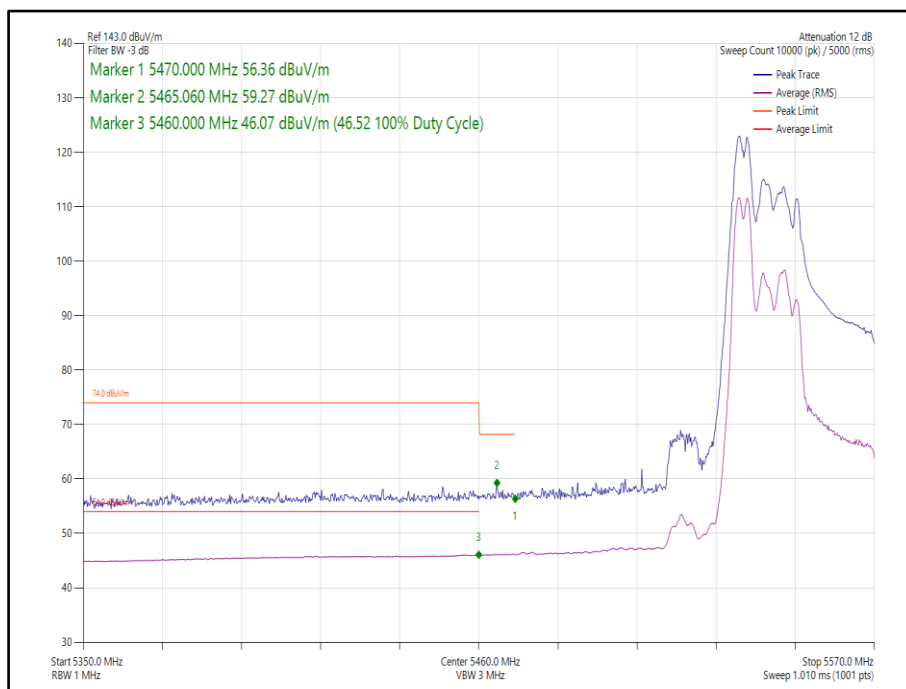
Figure 436 - 802.11ax, HE40, RU 52-37, SDM, Core 0-1 - 5550 MHz, Band Edge Frequency 5470 MHz
