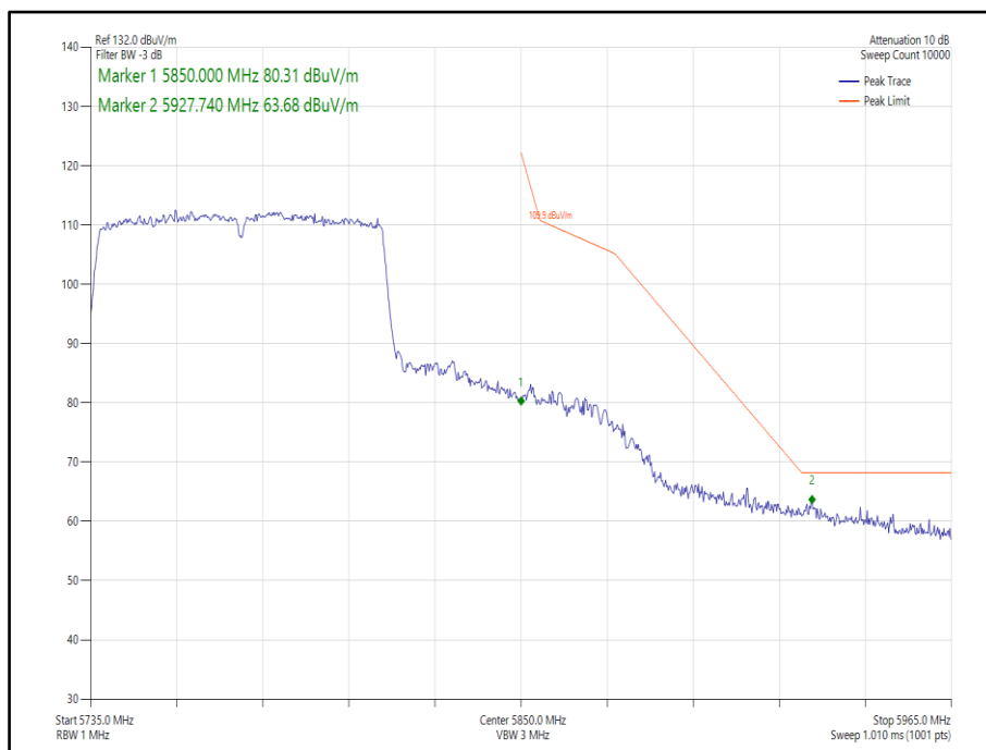
Figure 466 - 802.11ac, VHT80, SISO, Core 0 - 5775 MHz, Band Edge Frequency 5850 MHz
