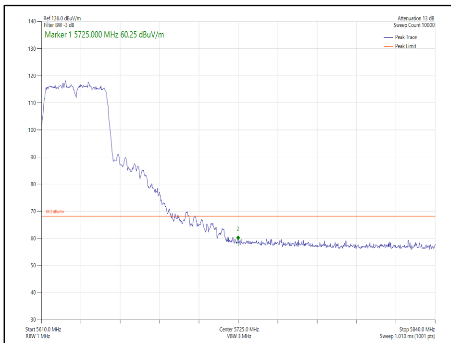
Figure 440 - 802.11n, HT40, SDM, Core 0-1 - 5630 MHz, Band Edge Frequency 5725 MHz
