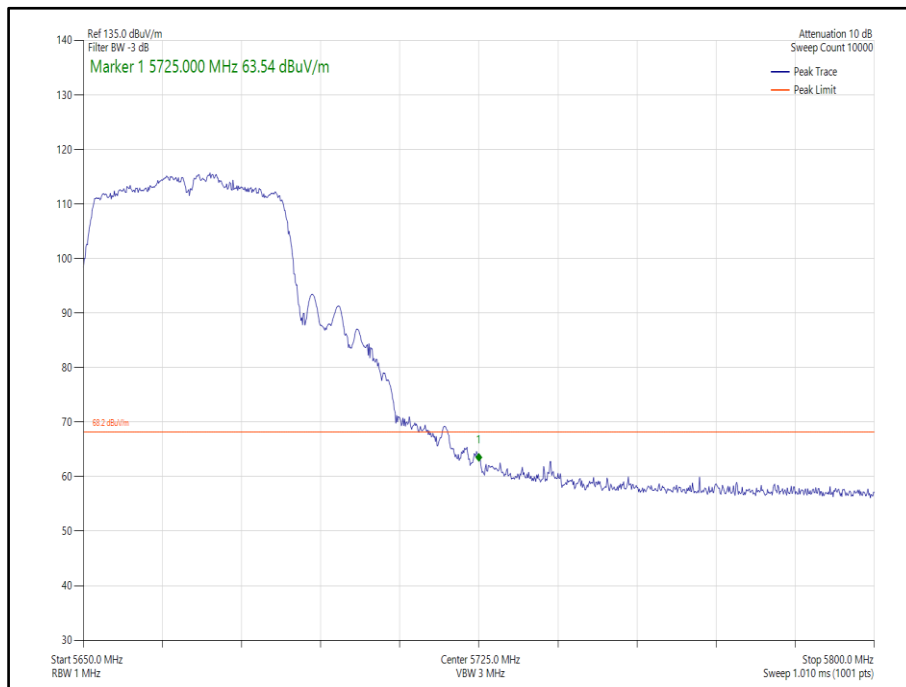
Figure 441 - 802.11n HT40, SDM, Core 0-1 - 5670 MHz, Band Edge Frequency 5725 MHz
