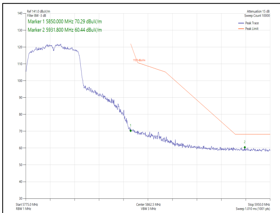
Figure 455 - 802.11ac, VHT40, TxBF, Core 0-1 - 5795 MHz, Band Edge Frequency 5850 MHz
