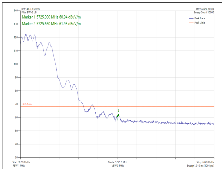
Figure 358 - 802.11ax, HE20, RU 106-53, SDM, Core 0-1 - 5680 MHz, Band Edge Frequency 5725 MHz
