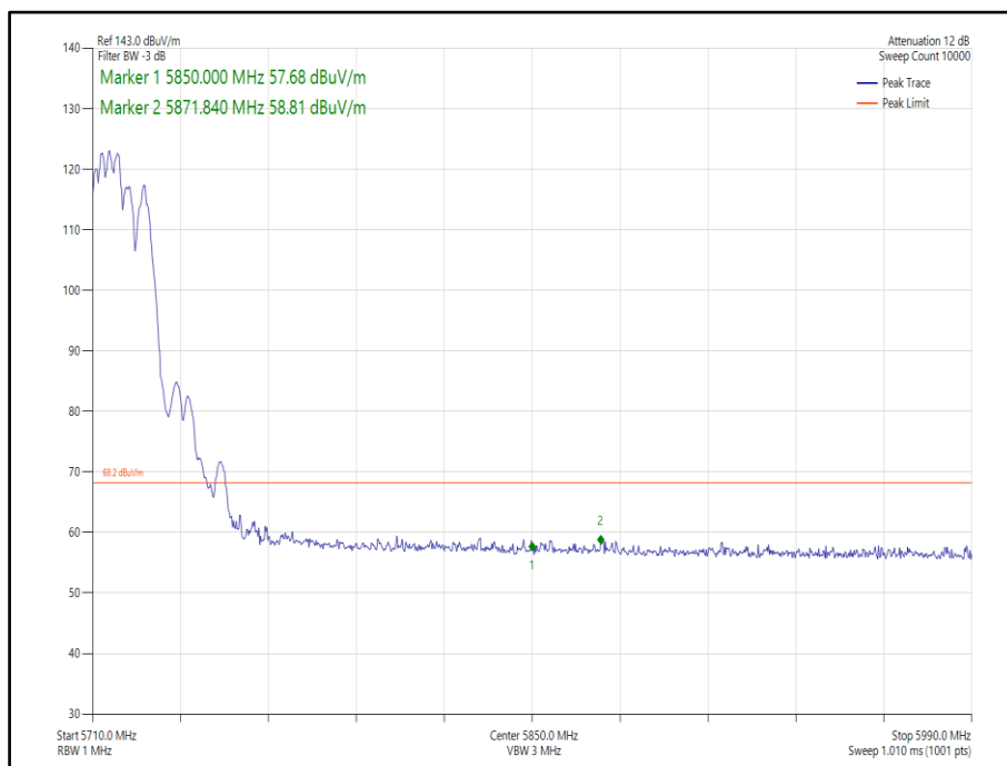
Figure 364 - 802.11ax, HE20, RU 106-53, SDM, Core 0-1 - 5720 MHz, Band Edge Frequency 5850 MHz
