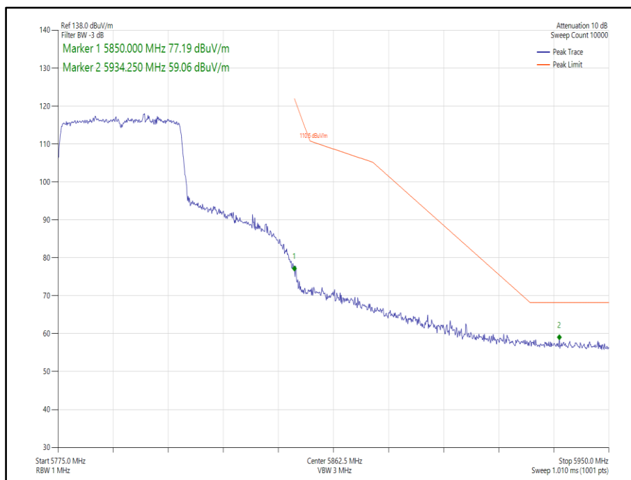
Figure 389 - 802.11ax, HE40, SU, SISO, Core 0 - 5795 MHz, Band Edge Frequency 5850 MHz
