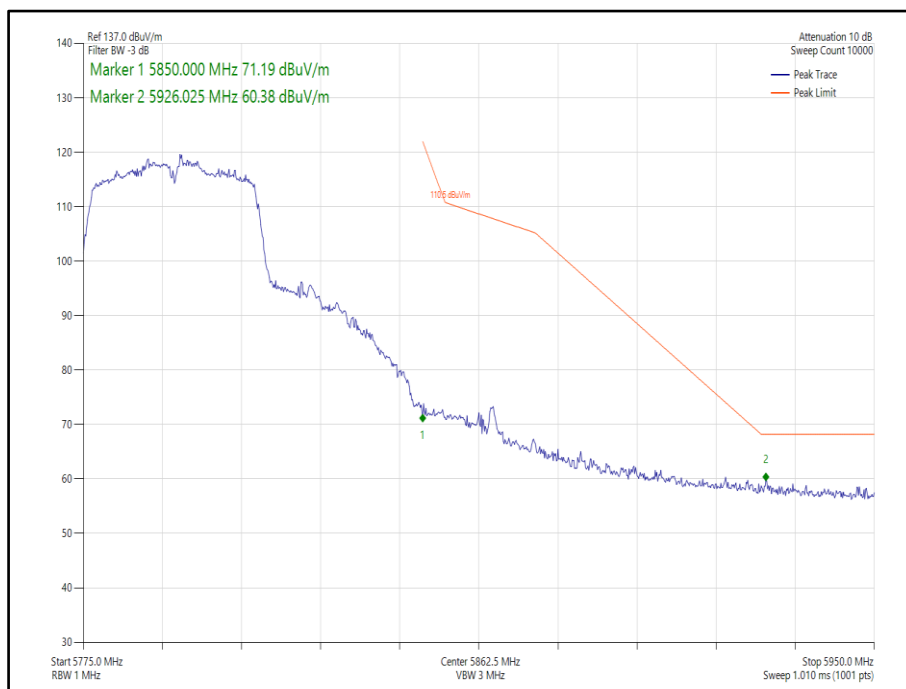
Figure 406 - 802.11n, HT40, SISO, Core 1 - 5795 MHz, Band Edge Frequency 5850 MHz
