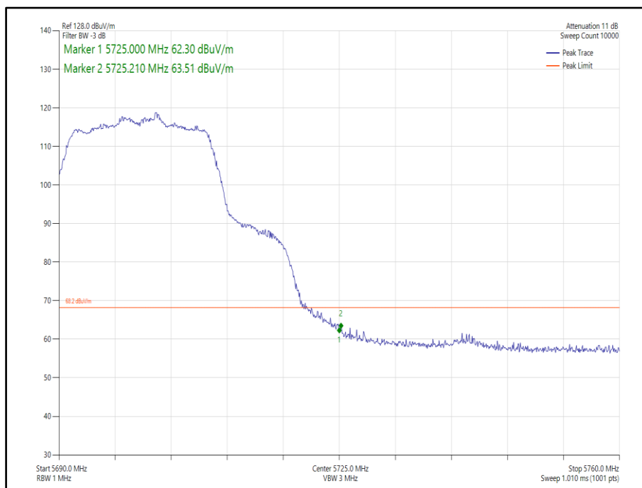
Figure 356 - 802.11n, HT20, SDM, Core 0-1 - 5700 MHz, Band Edge Frequency 5725 MHz
