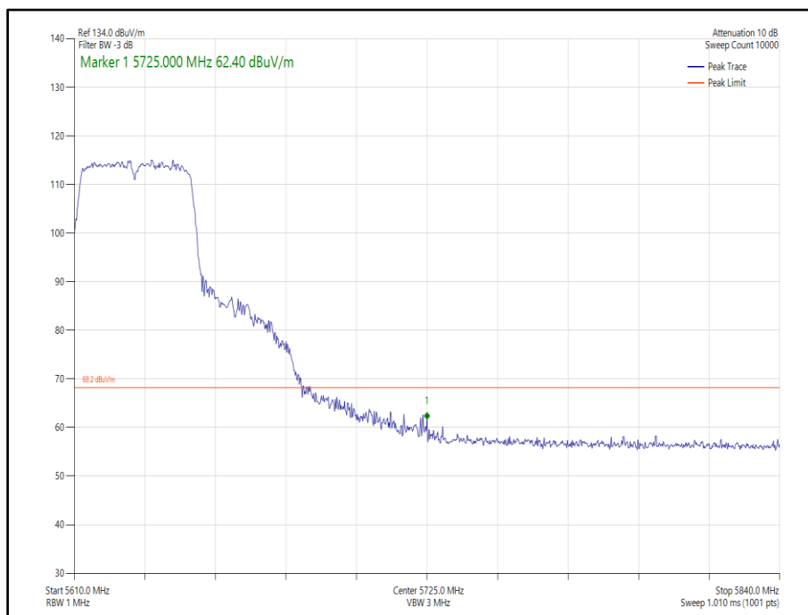
Figure 400 - 802.11n, HT40, SISO, Core 1 - 5630 MHz, Band Edge Frequency 5725 MHz
