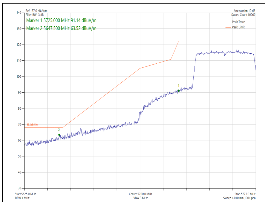
Figure 379 - 802.11ax, HE40, SU, SISO, Core 0 - 5755 MHz, Band Edge Frequency 5725 MHz
