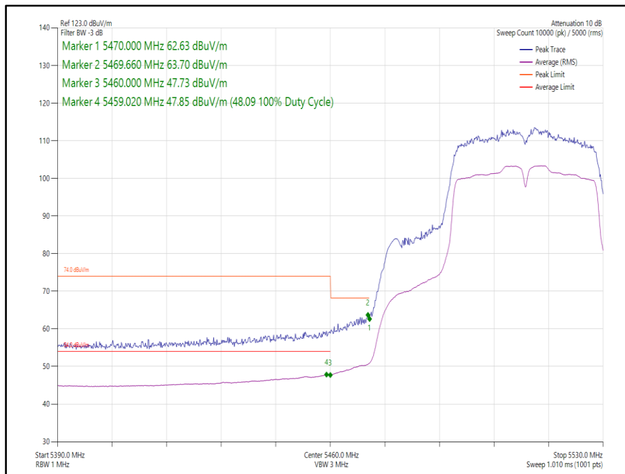
Figure 372 - 802.11n, HT40, SISO, Core 0 - 5510 MHz, Band Edge Frequency 5470 MHz
