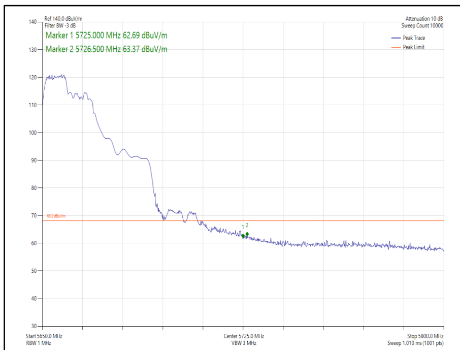
Figure 385 - 802.11ax, HE40, RU 106-53, SISO, Core 0 - 5670 MHz, Band Edge Frequency 5725 MHz
