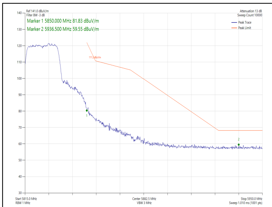
Figure 362 - 802.11n, HT20, SDM, Core 0-1 - 5825 MHz, Band Edge Frequency 5850 MHz
