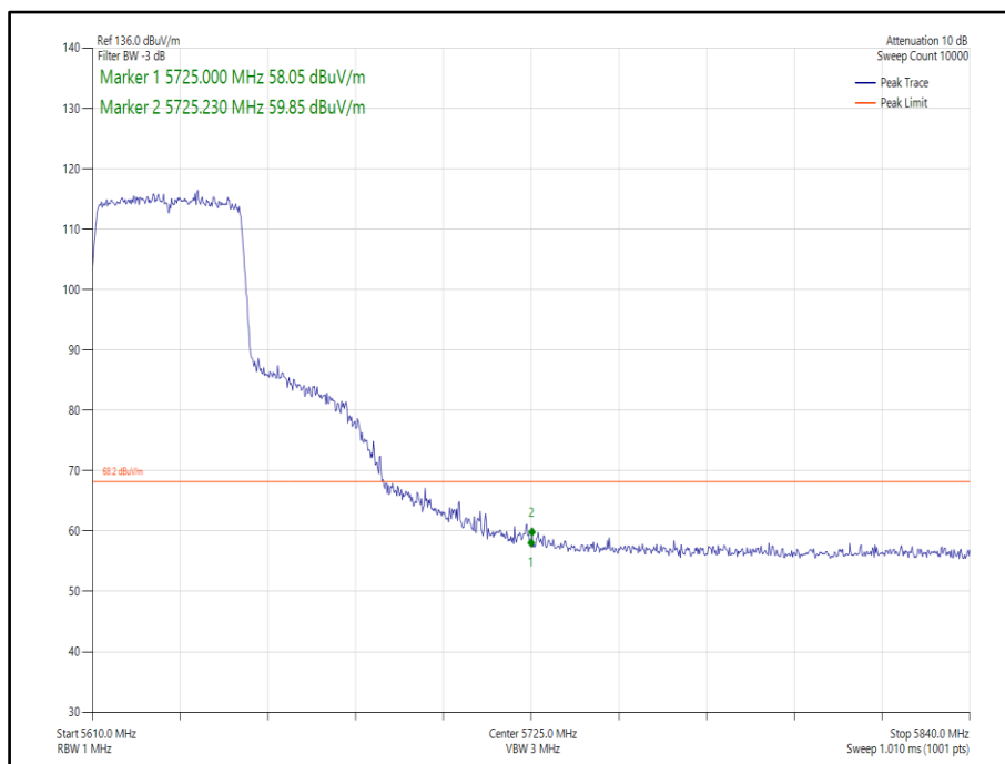
Figure 402 - 802.11ax, HE40, SU, SISO, Core 1 - 5630 MHz, Band Edge Frequency 5725 MHz
