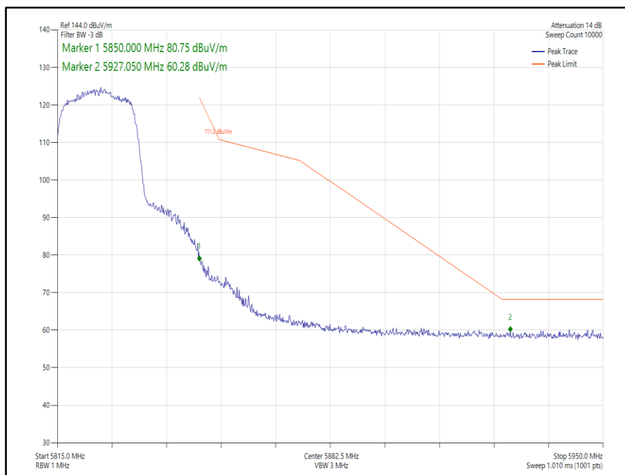
Figure 371 - 802.11ac, VHT20, TxBF, Core 0-1 - 5825 MHz, Band Edge Frequency 5850 MHz
