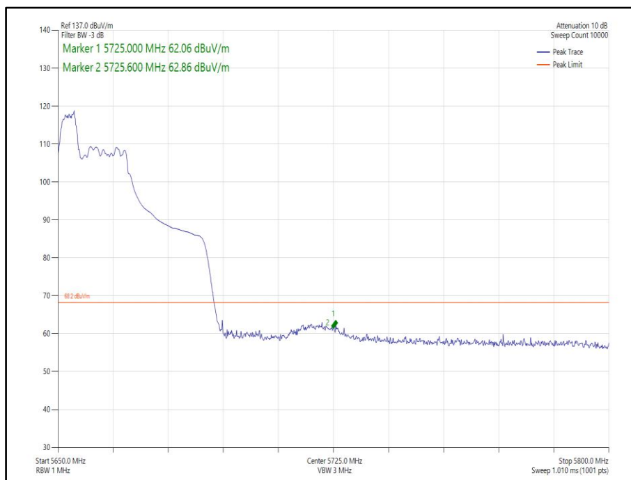
Figure 404 - 802.11ax, HE40, RU 52-37, SISO, Core 1 - 5670 MHz, Band Edge Frequency 5725 MHz
