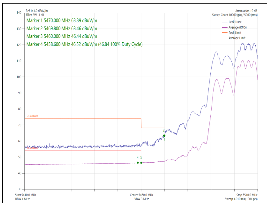
Figure 350 - 802.11ax, HE20, RU 106-54, SDM, Core 0-1 - 5500 MHz, Band Edge Frequency 5470 MHz
