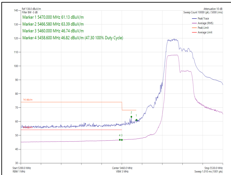
Figure 375 - 802.11ax, HE40, RU 106-53, SISO, Core 0 - 5510 MHz, Band Edge Frequency 5470 MHz
