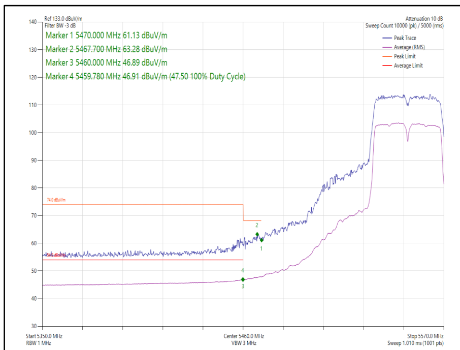
Figure 392 - 802.11n, HT40, SISO, Core 1 - 5550 MHz, Band Edge Frequency 5470 MHz
