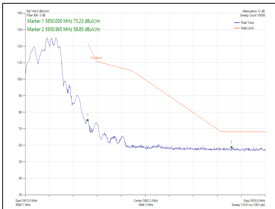
Figure 366 - 802.11ax, HE20, RU 106-54, SDM, Core 0-1 - 5825 MHz, Band Edge Frequency 5850 MHz
