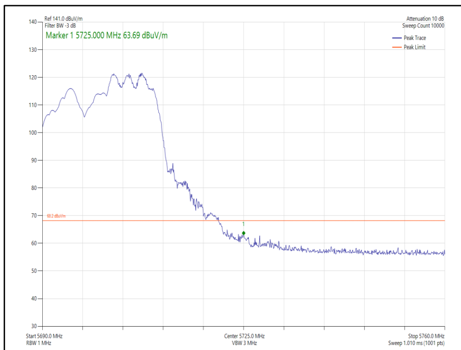
Figure 360 - 802.11ax, HE20, RU 106-54, SDM, Core 0-1 - 5700 MHz, Band Edge Frequency 5725 MHz
