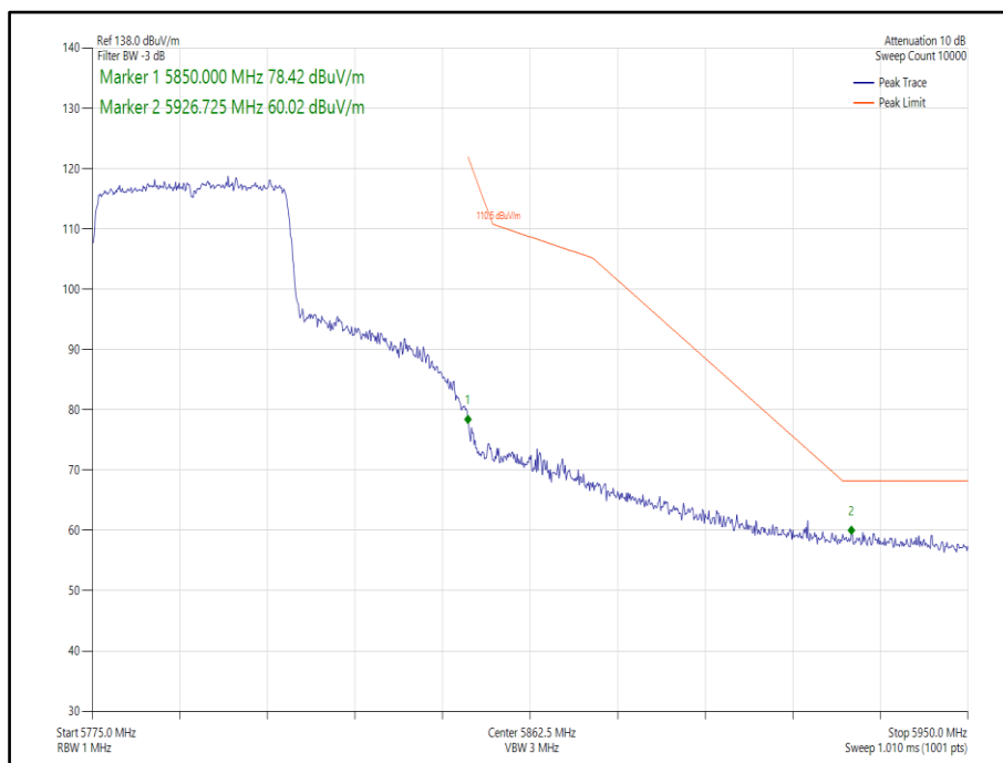
Figure 408 - 802.11ax, HE40, SU, SISO, Core 1 - 5795 MHz, Band Edge Frequency 5850 MHz
