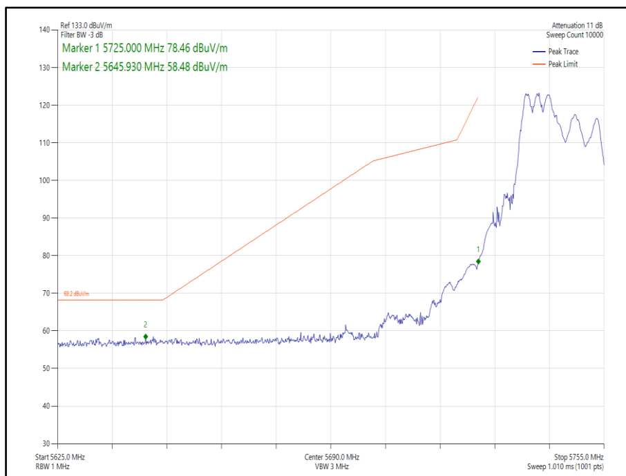
Figure 354 - 802.11ax, HE20, RU 106-53, SDM, Core 0-1 - 5745 MHz, Band Edge Frequency 5725 MHz
