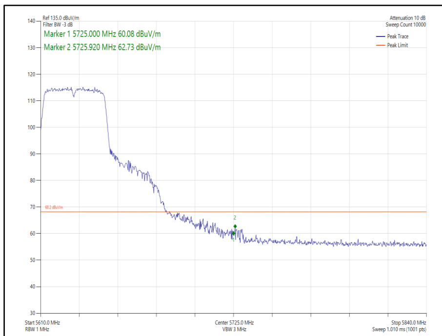
Figure 381 - 802.11n, HT40, SISO, Core 0 - 5630 MHz, Band Edge Frequency 5725 MHz
