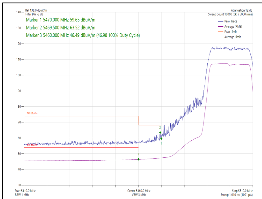
Figure 367 - 802.11ac, VHT20, TxBF, Core 0-1 - 5500 MHz, Band Edge Frequency 5470 MHz
