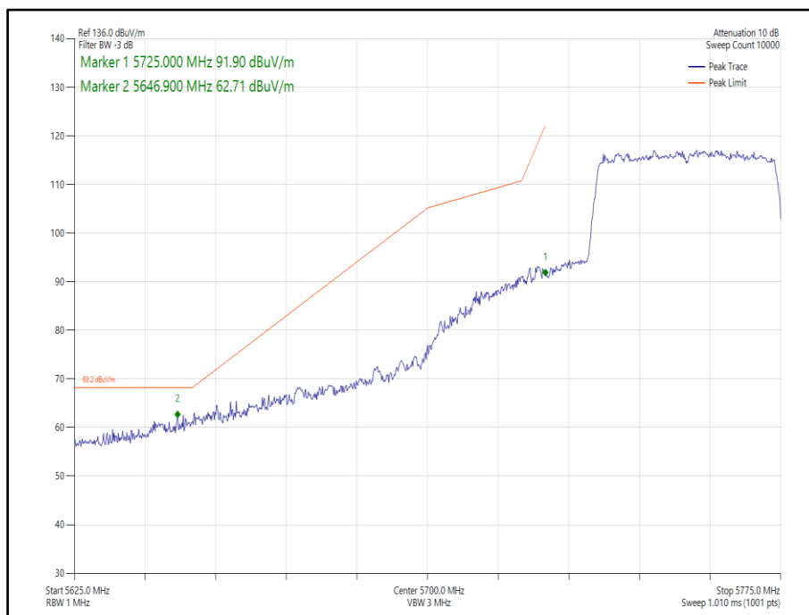
Figure 398 - 802.11ax, HE40, SU, SISO, Core 1 - 5755 MHz, Band Edge Frequency 5725 MHz
