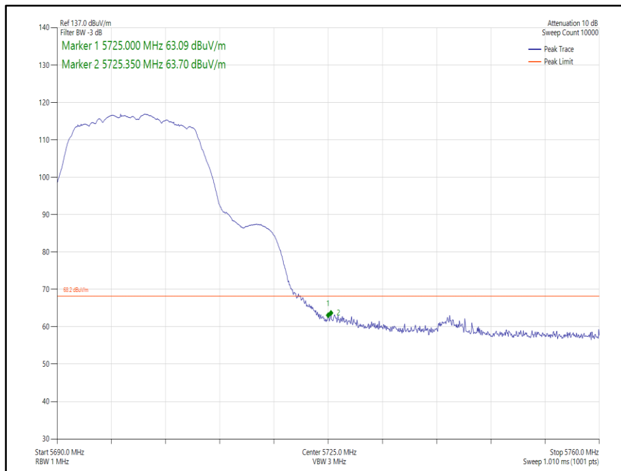
Figure 314 - 802.11a, SISO, Core 1 - 5700 MHz, Band Edge Frequency 5725 MHz
