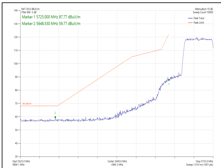
Figure 311 - 802.11ax, HE20, SU, SISO, Core 1 - 5745 MHz, Band Edge Frequency 5725 MHz
