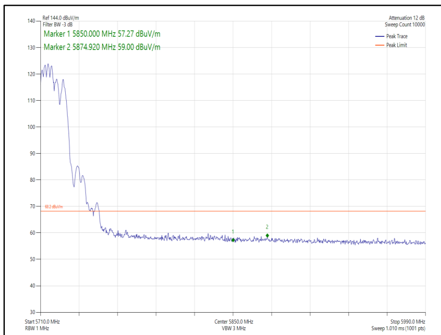
Figure 344 - 802.11ax, HE20, RU 106-53, CDD, Core 0-1 - 5720 MHz, Band Edge Frequency 5850 MHz
