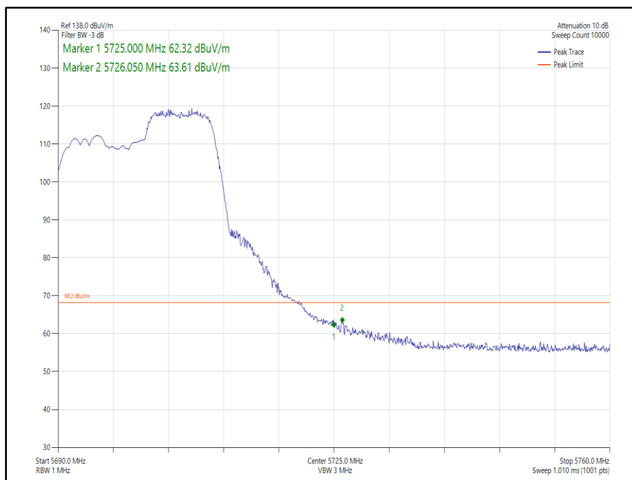
Figure 294 - 802.11ax, HE20, RU 106-54, SISO, Core 0 - 5700 MHz, Band Edge Frequency 5725 MHz
