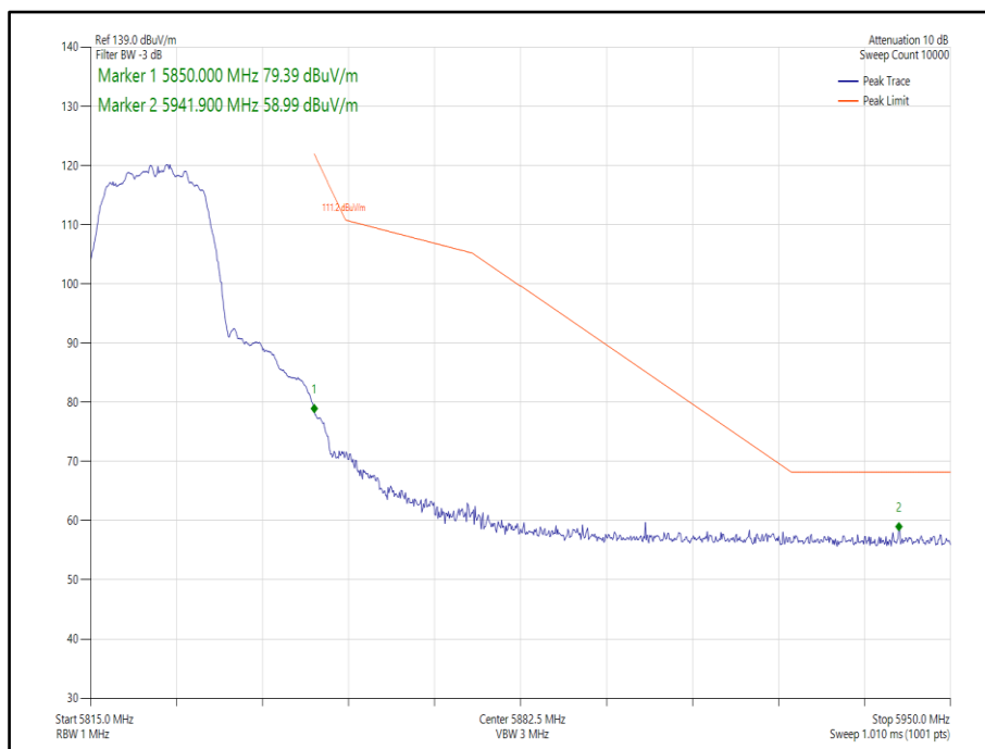
Figure 296 - 802.11a, SISO, Core 0 - 5825 MHz, Band Edge Frequency 5850 MHz
