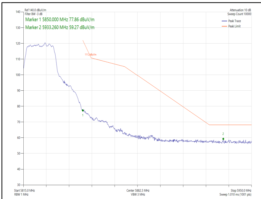
Figure 321 - 802.11a, SISO, Core 1 - 5825 MHz, Band Edge Frequency 5850 MHz
