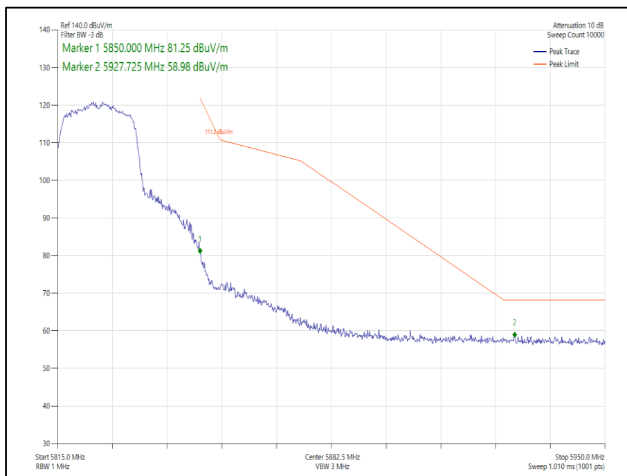
Figure 323 - 802.11n, HT20, SISO, Core 1 - 5825 MHz, Band Edge Frequency 5850 MHz
