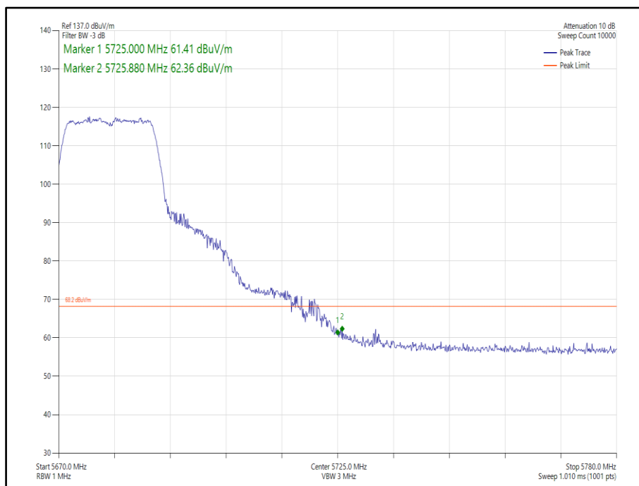
Figure 290 - 802.11n, HT20, SISO, Core 0 - 5680 MHz, Band Edge Frequency 5725 MHz
