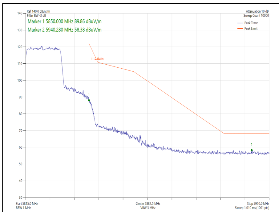
Figure 300 - 802.11ax, HE20, SU, SISO, Core 0 - 5825 MHz, Band Edge Frequency 5850 MHz
