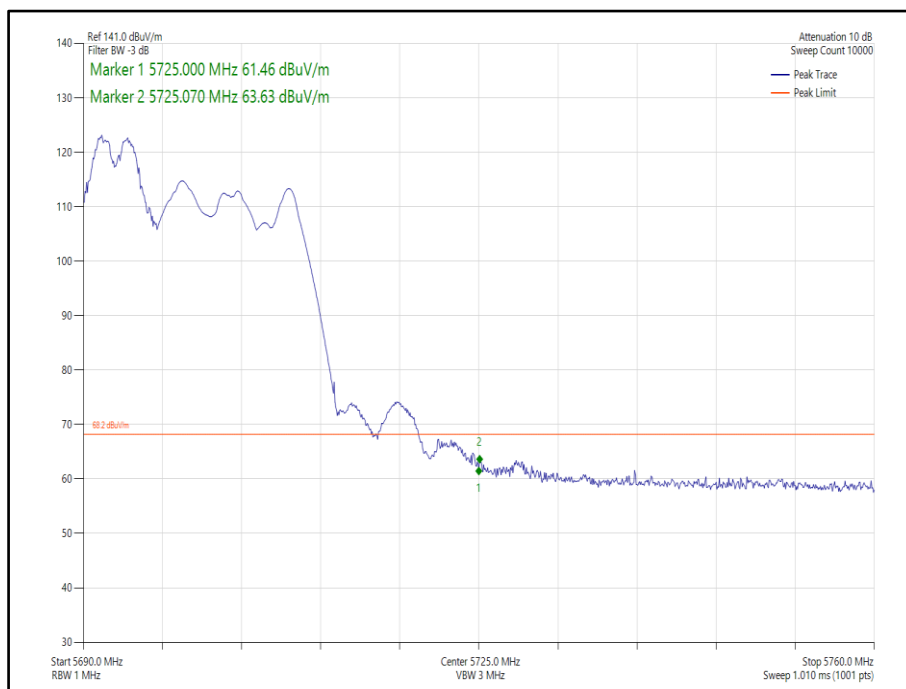
Figure 340 - 802.11ax, HE20, RU 52-37, CDD, Core 0-1 - 5700 MHz, Band Edge Frequency 5725 MHz
