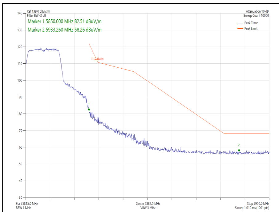
Figure 298 - 802.11n, HT20, SISO, Core 0 - 5825 MHz, Band Edge Frequency 5850 MHz
