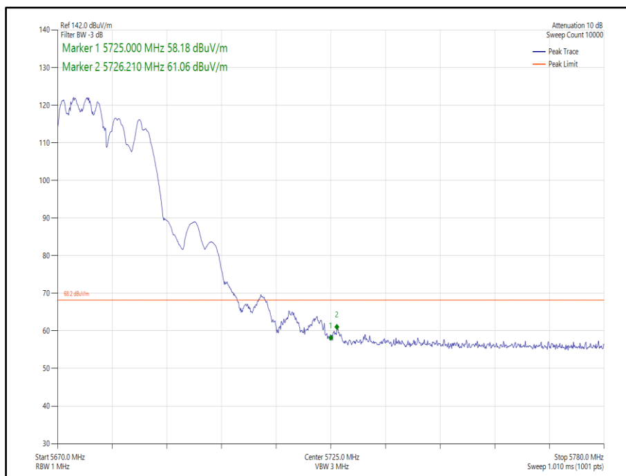
Figure 338 - 802.11ax, HE20, RU 106-53, CDD, Core 0-1 - 5680 MHz, Band Edge Frequency 5725 MHz
