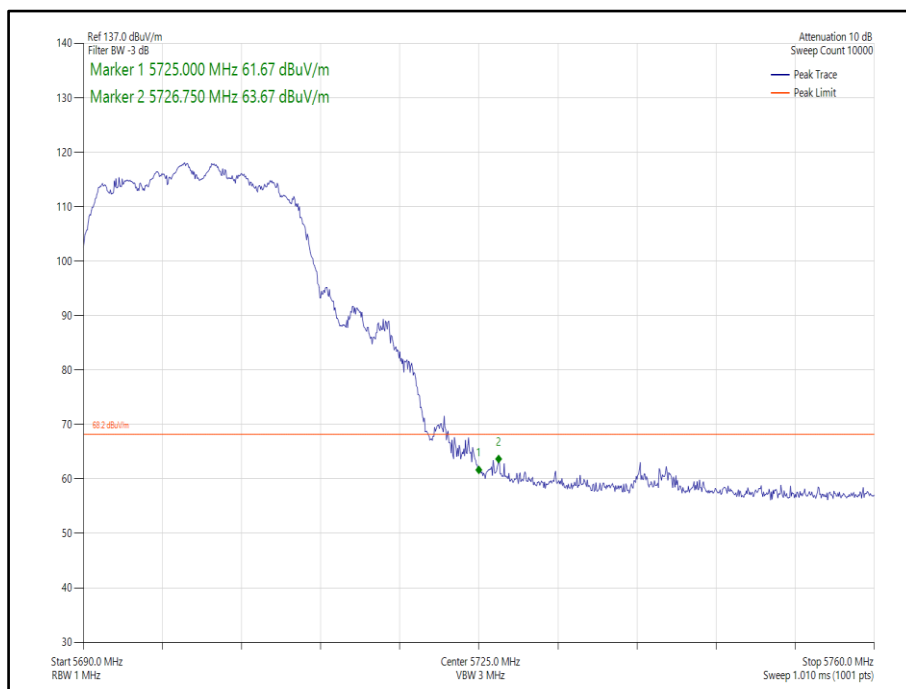
Figure 336 - 802.11n, HT20, CDD, Core 0-1 - 5700 MHz, Band Edge Frequency 5725 MHz
