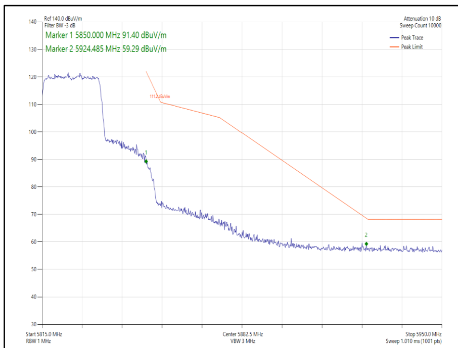
Figure 325 - 802.11ax, HE20, SU, SISO, Core 1 - 5825 MHz, Band Edge Frequency 5850 MHz
