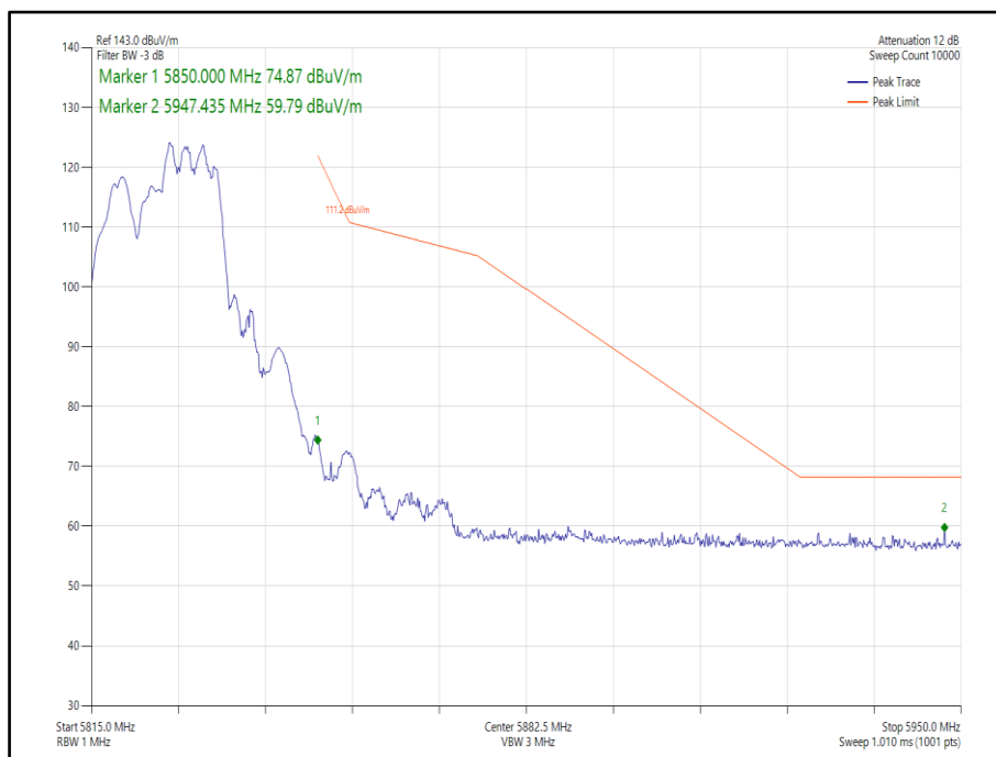
Figure 346 - 802.11ax, HE20, RU 106-54, CDD, Core 0-1 - 5825 MHz, Band Edge Frequency 5850 MHz
