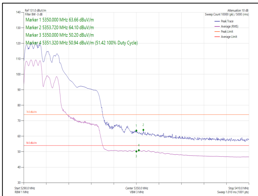
Figure 140 - 802.11ax, HE40, RU 106-53, SDM, Core 0-1 - 5310 MHz, Band Edge Frequency 5350 MHz
