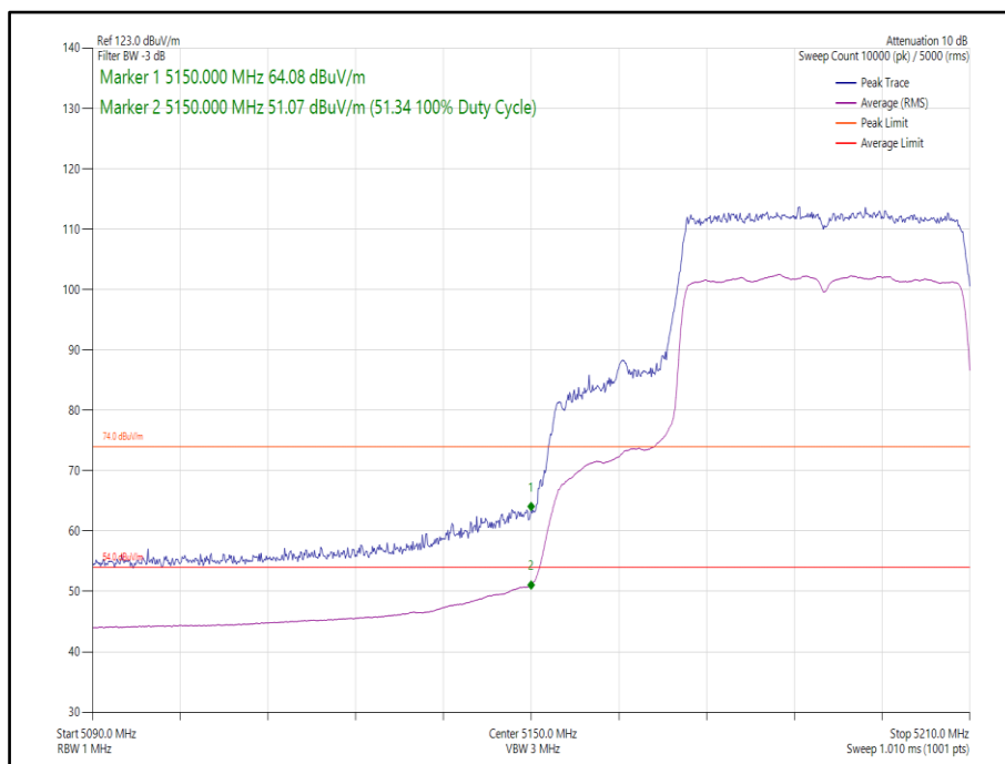
Figure 132 - 802.11ax, HE40, SU, SDM, Core 0-1 - 5190 MHz, Band Edge Frequency 5150 MHz
