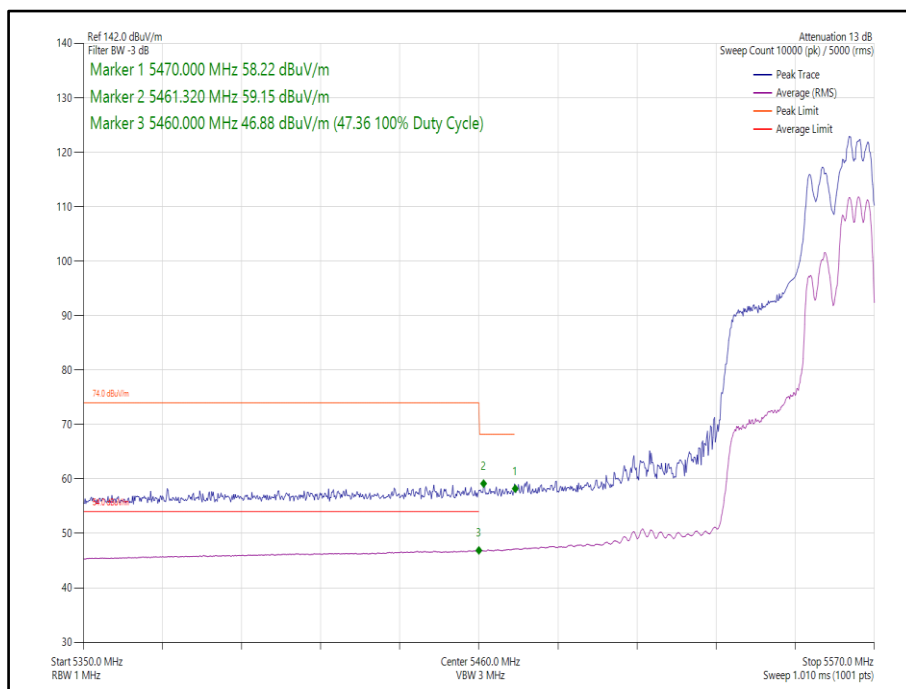
Figure 146 - 802.11ax, HE40, RU 106-56, SDM, Core 0-1 - 5550 MHz, Band Edge Frequency 5460 MHz
