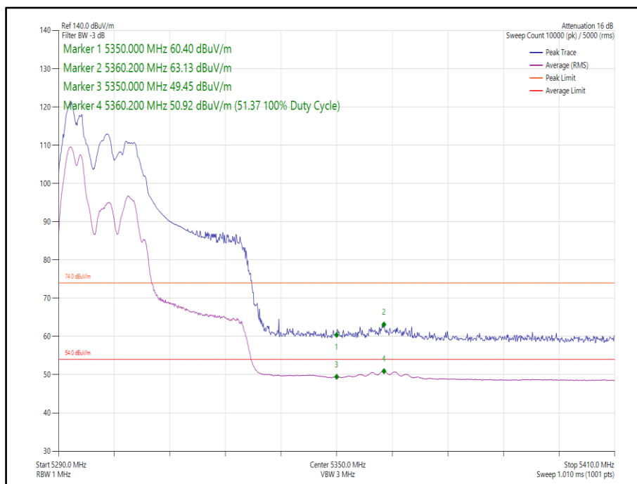
Figure 123 - 802.11ax, HE40, RU 52-37, CDD, Core 0-1 - 5310 MHz, Band Edge Frequency 5350 MHz
