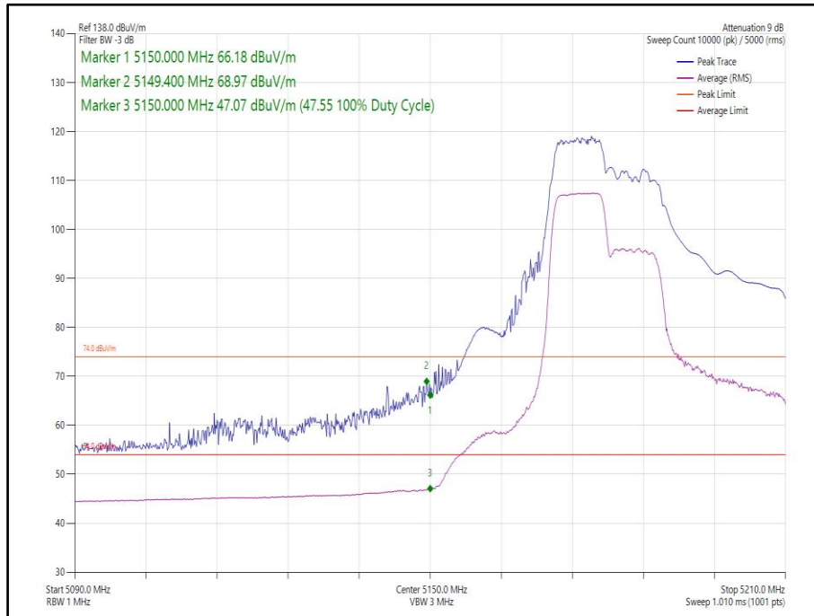
Figure 98 - 802.11ax, HE40, RU 106-53, SISO, Core 1 - 5190 MHz, Band Edge Frequency 5150 MHz
