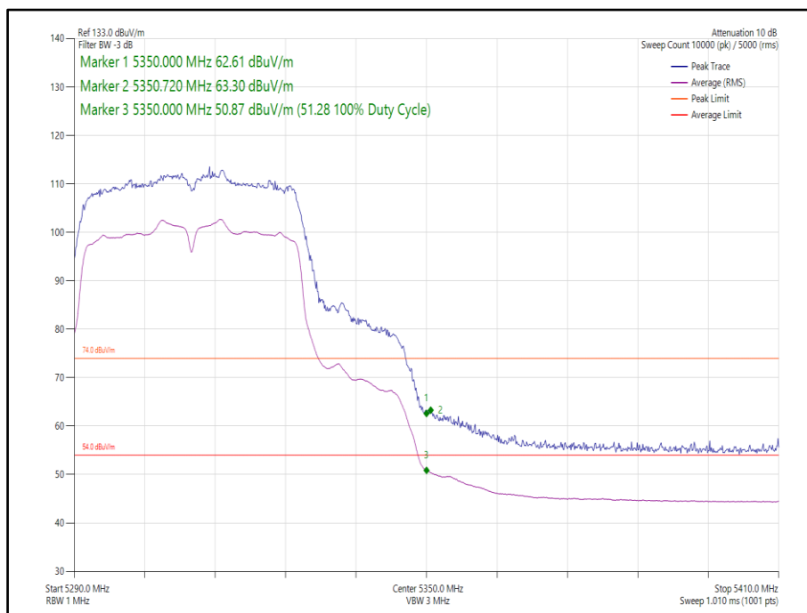
Figure 136 - 802.11n, HT40, SDM, Core 0-1 - 5310 MHz, Band Edge Frequency 5350 MHz
