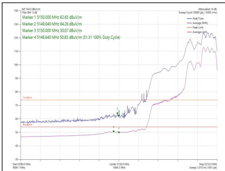
Figure 115 - 802.11ax, HE40, RU 106-56, CDD, Core 0-1 - 5190 MHz, Band Edge Frequency 5150 MHz
