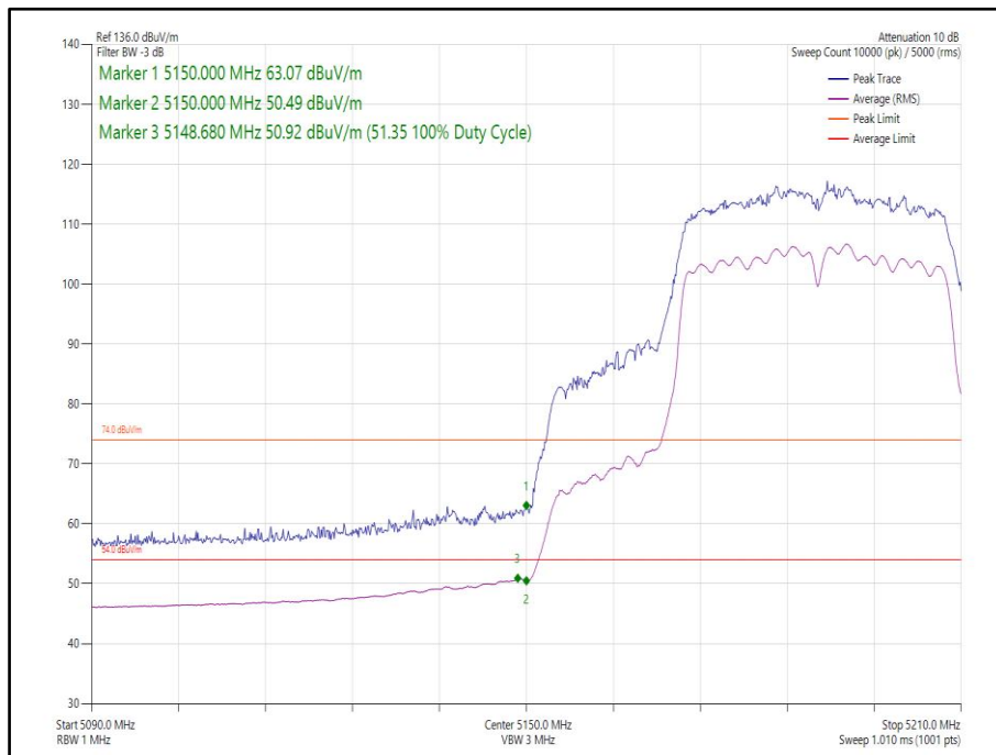
Figure 112 - 802.11n, HT40, CDD, Core 0-1 - 5190 MHz, Band Edge Frequency 5150 MHz
