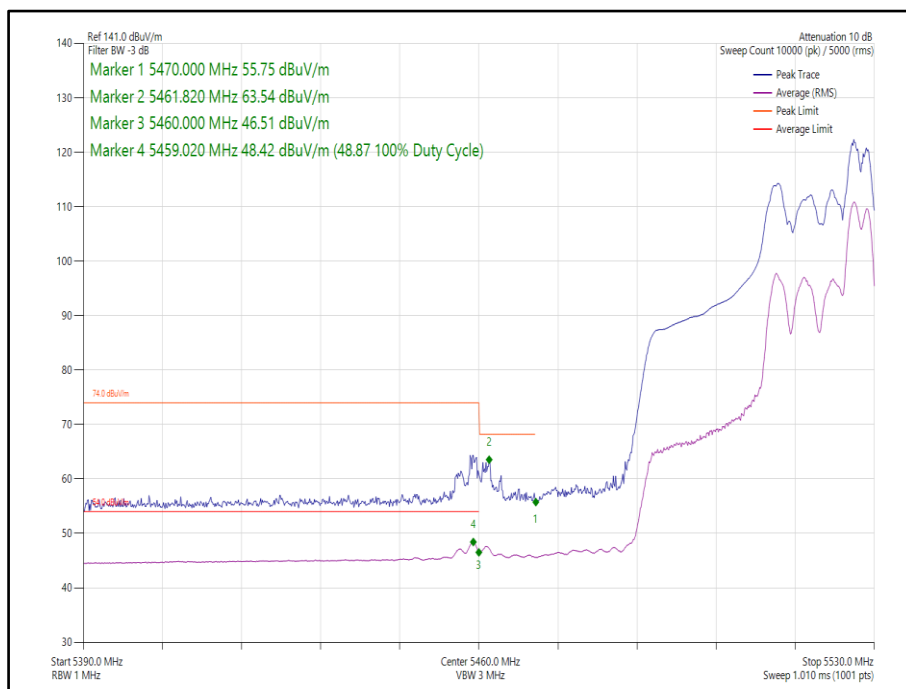
Figure 127 - 802.11ax, HE40, RU 52-44, CDD, Core 0-1 - 5510 MHz, Band Edge Frequency 5460 MHz
