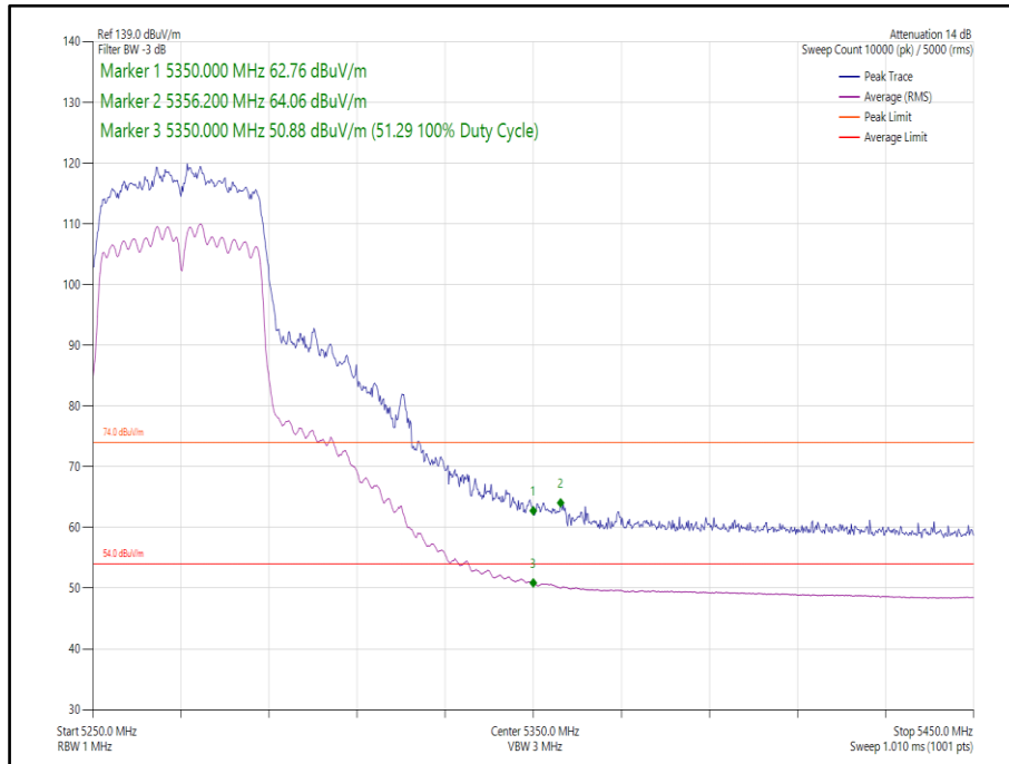
Figure 118 - 802.11n, HT40, CDD, Core 0-1 - 5270 MHz, Band Edge Frequency 5350 MHz
