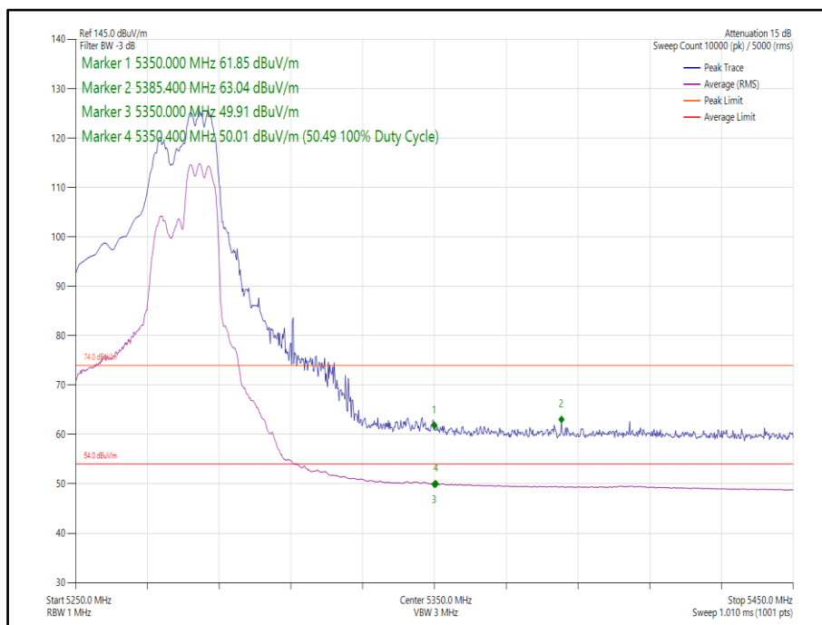
Figure 121 - 802.11ax, HE40, RU 106-56, CDD, Core 0-1 - 5270 MHz, Band Edge Frequency 5350 MHz
