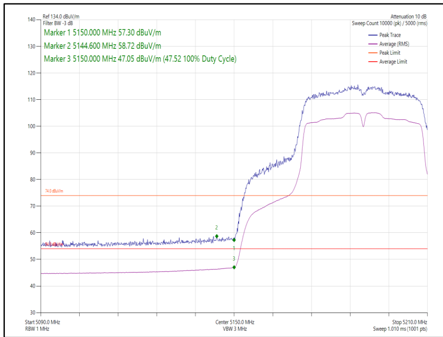
Figure 147 - 802.11ac, VHT40, TxBF, Core 0-1 - 5190 MHz, Band Edge Frequency 5150 MHz
