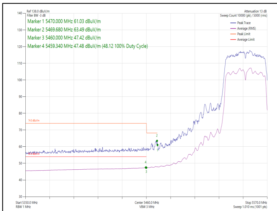
Figure 142 - 802.11n, HT40, SDM, Core 0-1 - 5550 MHz, Band Edge Frequency 5460 MHz
