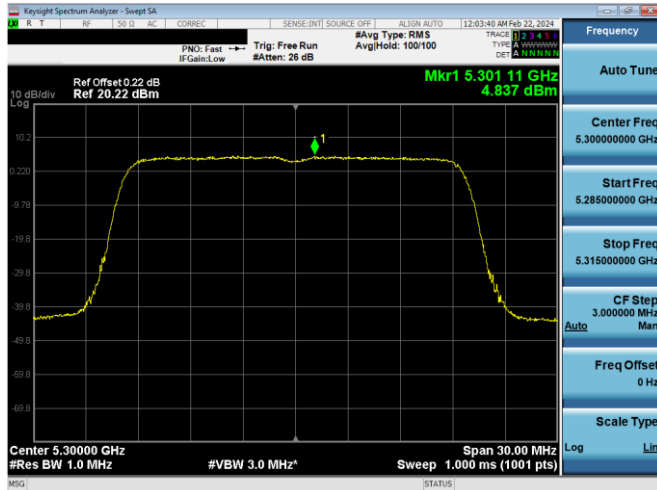
Plot 7-638. PSD CDD Primary Antenna 4a (20MHz BW 802.11n – Ch. 60, MCS12)
