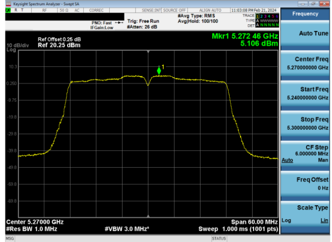
Plot 7-598. PSD CDD Primary Antenna 4a (40MHz BW 802.11n – Ch. 54, MCS10)
