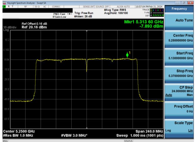
Plot 7-592. PSD CDD Primary Antenna 4a (160MHz BW 802.11ax(SU) – Ch. 50, MCS2)
