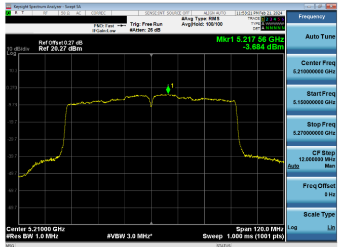
Plot 7-630. PSD CDD Primary Antenna 4a (80MHz BW 802.11ac – Ch. 42, MCS4)
