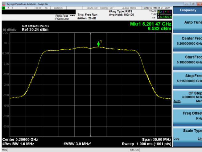
Plot 7-578. PSD CDD Primary Antenna 4a (20MHz BW 802.11n – Ch. 40, MCS10)
