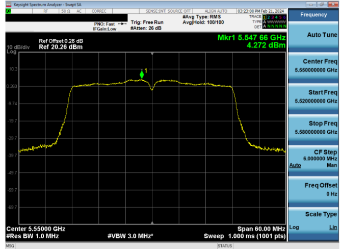
Plot 7-653. PSD CDD Primary Antenna WF5b (40MHz BW 802.11n – Ch. 110, MCS12)
