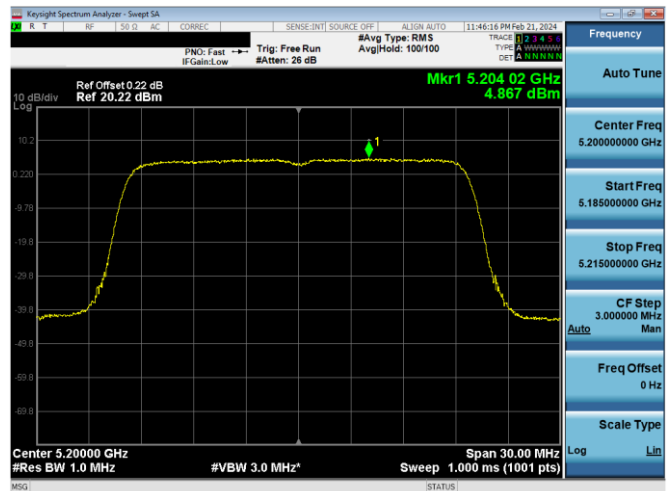
Plot 7-624. PSD CDD Primary Antenna 4a (20MHz BW 802.11ax(SU) – Ch. 40, MCS4)
