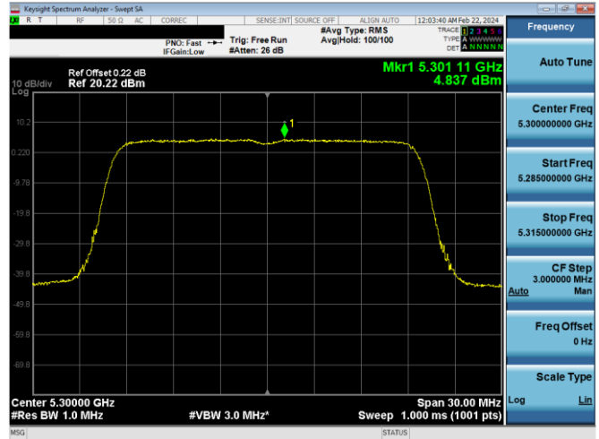
Plot 7-640. PSD CDD Primary Antenna 4a (20MHz BW 802.11ax(SU) – Ch. 60, MCS4)
