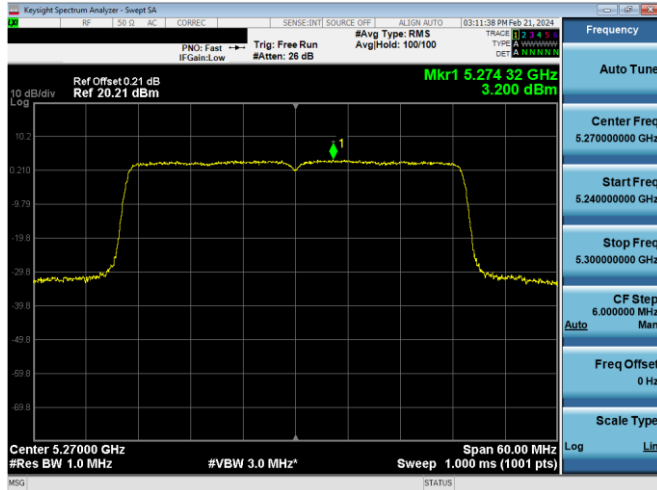
Plot 7-643. PSD CDD Primary Antenna WF5b (40MHz BW 802.11ax(SU) - Ch. 54, MCS4)
