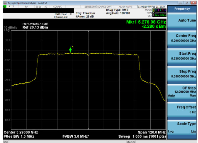
Plot 7-604. PSD CDD Primary Antenna 4a (80MHz BW 802.11ax(SU) – Ch. 58, MCS2)
