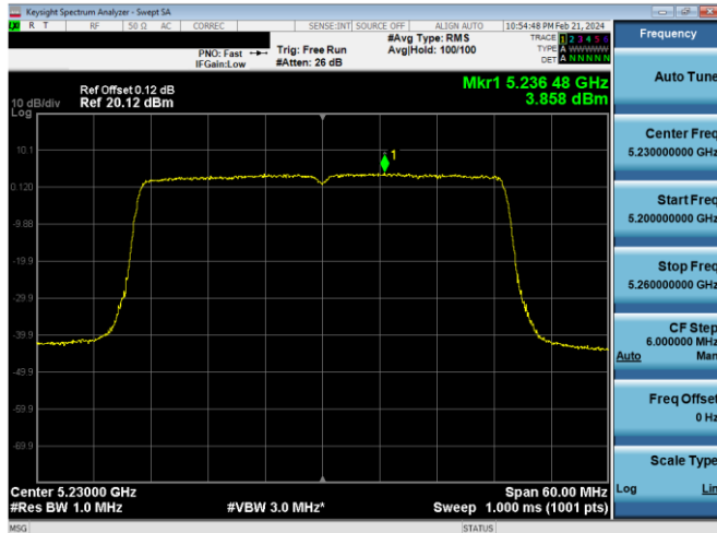
Plot 7-584. PSD CDD Primary Antenna 4a (40MHz BW 802.11ax(SU) – Ch. 46, MCS2)
