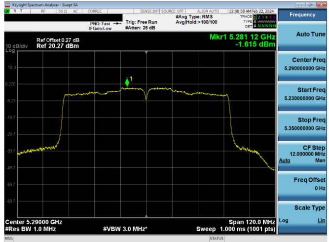
Plot 7-646. PSD CDD Primary Antenna 4a (80MHz BW 802.11ac - Ch. 58, MCS4)
