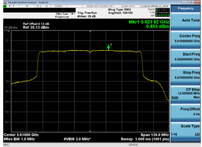
Plot 7-616. PSD CDD Primary Antenna 4a (80MHz BW 802.11ax(SU) – Ch. 122, MCS2)
