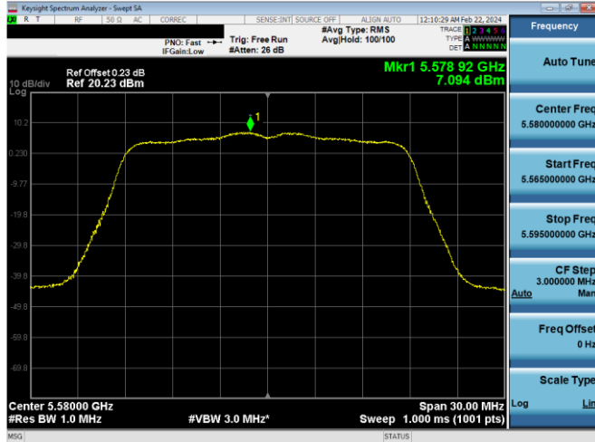
Plot 7-650. PSD CDD Primary Antenna 4a (20MHz BW 802.11n – Ch. 116, MCS12)
