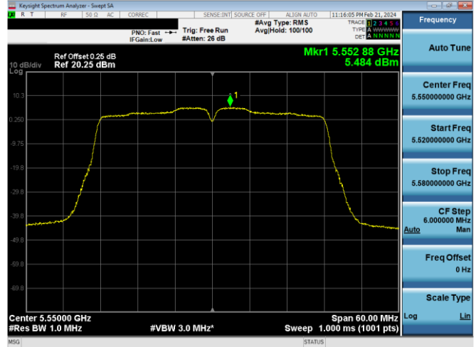
Plot 7-610. PSD CDD Primary Antenna 4a (40MHz BW 802.11n – Ch. 110, MCS10)
