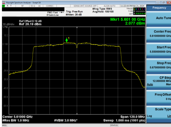
Plot 7-614. PSD CDD Primary Antenna 4a (80MHz BW 802.11ac – Ch. 122, MCS2)
