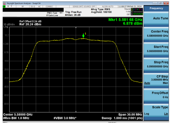
Plot 7-606. PSD CDD Primary Antenna 4a (20MHz BW 802.11n – Ch. 116, MCS10)
