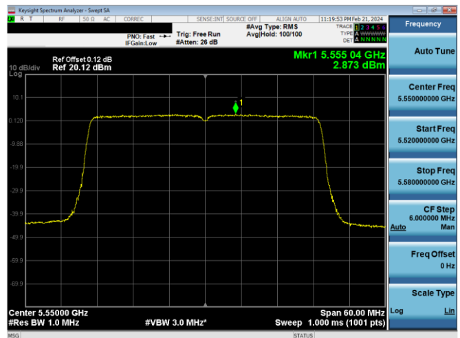
Plot 7-612. PSD CDD Primary Antenna 4a (40MHz BW 802.11ax(SU) – Ch. 110, MCS2)
