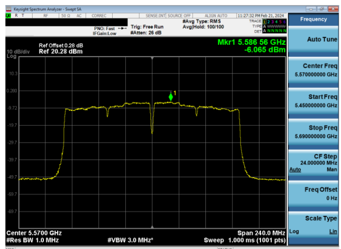
Plot 7-618. PSD CDD Primary Antenna 4a (160MHz BW 802.11ac – Ch. 114, MCS2)
