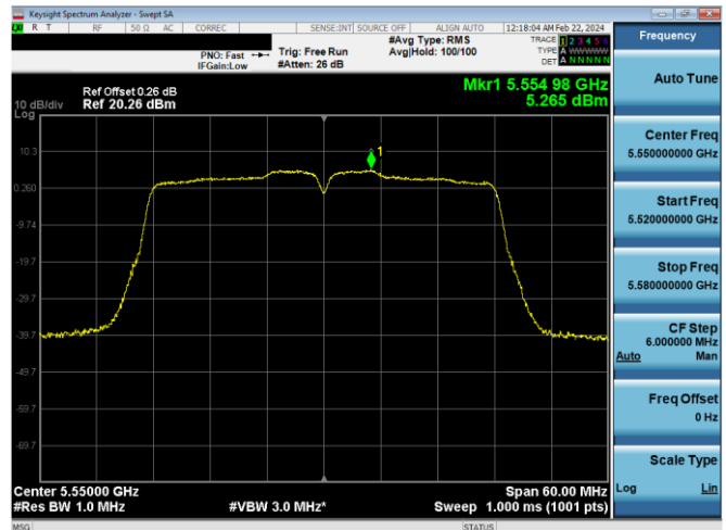
Plot 7-654. PSD CDD Primary Antenna 4a (40MHz BW 802.11n – Ch. 110, MCS12)
