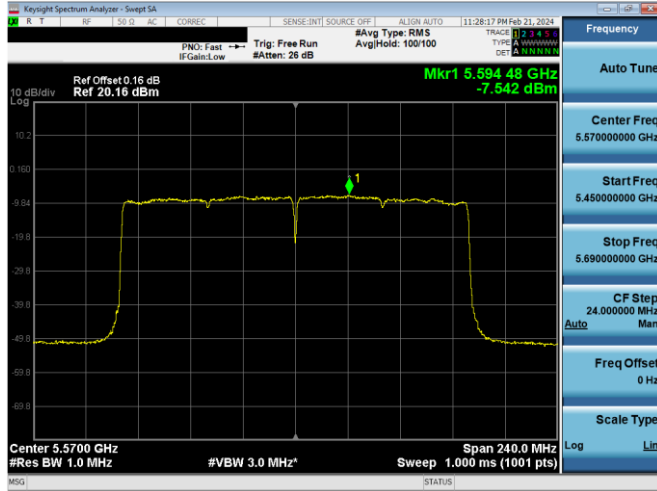
Plot 7-620. PSD CDD Primary Antenna 4a (160MHz BW 802.11ax(SU) – Ch. 114, MCS2)
