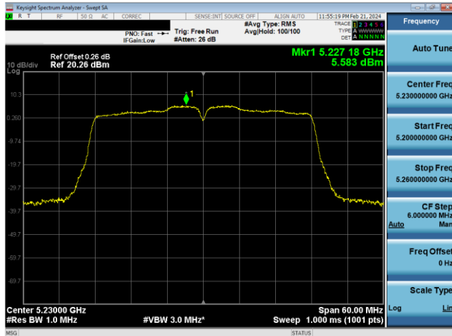
Plot 7-626. PSD CDD Primary Antenna 4a (40MHz BW 802.11n – Ch. 46, MCS12)
