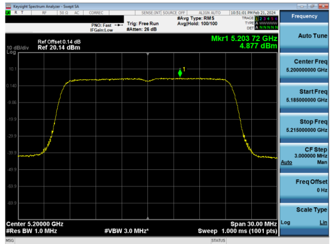
Plot 7-580. PSD CDD Primary Antenna 4a (20MHz BW 802.11ax(SU) – Ch. 40, MCS2)
