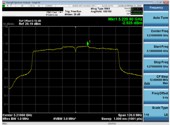
Plot 7-586. PSD CDD Primary Antenna 4a (80MHz BW 802.11ac – Ch. 42, MCS2)
