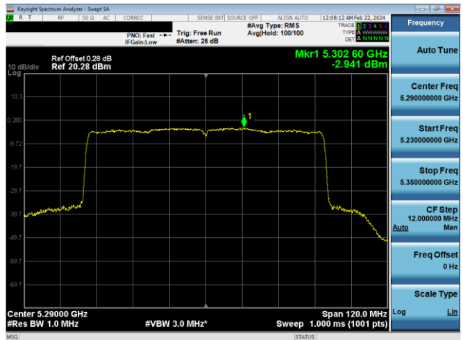
Plot 7-648. PSD CDD Primary Antenna 4a (80MHz BW 802.11ax(SU) - Ch. 58, MCS4)
