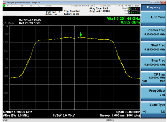
Plot 7-622. PSD CDD Primary Antenna 4a (20MHz BW 802.11n – Ch. 40, MCS12)
