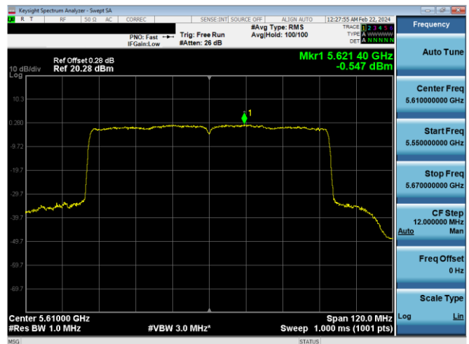
Plot 7-660. PSD CDD Primary Antenna 4a (80MHz BW 802.11ax(SU) – Ch. 122, MCS4)
