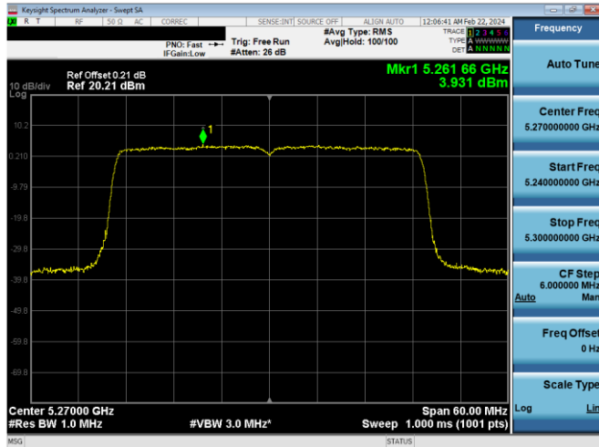
Plot 7-644. PSD CDD Primary Antenna 4a (40MHz BW 802.11ax(SU) - Ch. 54, MCS4)
