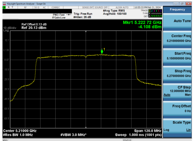
Plot 7-588. PSD CDD Primary Antenna 4a (80MHz BW 802.11ax(SU) – Ch. 42, MCS2)
