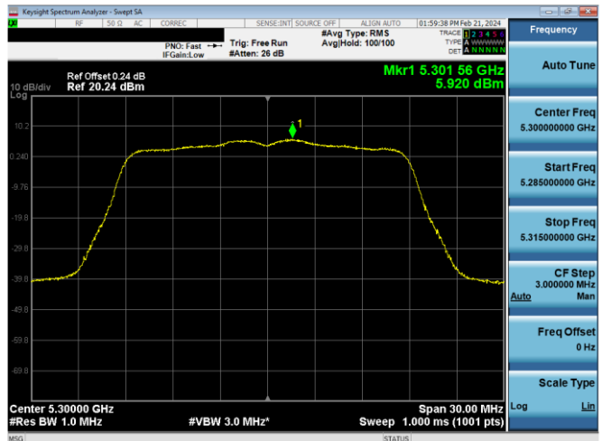
Plot 7-593. PSD CDD Primary Antenna WF5b (20MHz BW 802.11n – Ch. 60, MCS10)
