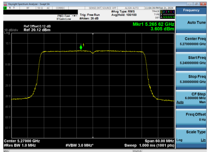
Plot 7-600. PSD CDD Primary Antenna 4a (40MHz BW 802.11ax(SU) – Ch. 54, MCS2)
