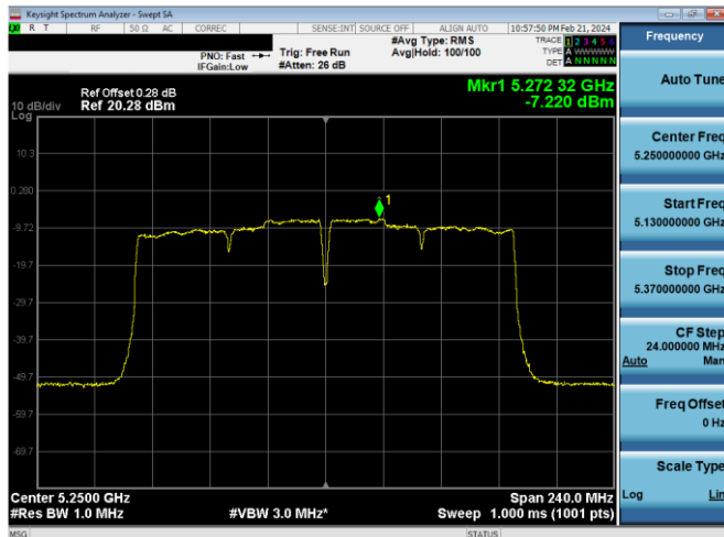
Plot 7-590. PSD CDD Primary Antenna 4a (160MHz BW 802.11ac – Ch. 50, MCS2)
