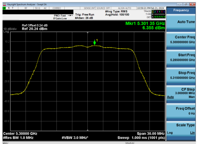
Plot 7-594. PSD CDD Primary Antenna 4a (20MHz BW 802.11n – Ch. 60, MCS10)
