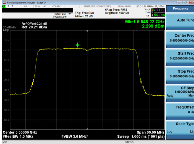
Plot 7-656. PSD CDD Primary Antenna 4a (40MHz BW 802.11ax(SU) – Ch. 110, MCS4)
