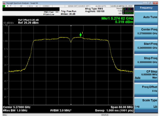
Plot 7-642. PSD CDD Primary Antenna 4a (40MHz BW 802.11n – Ch. 54, MCS12)
