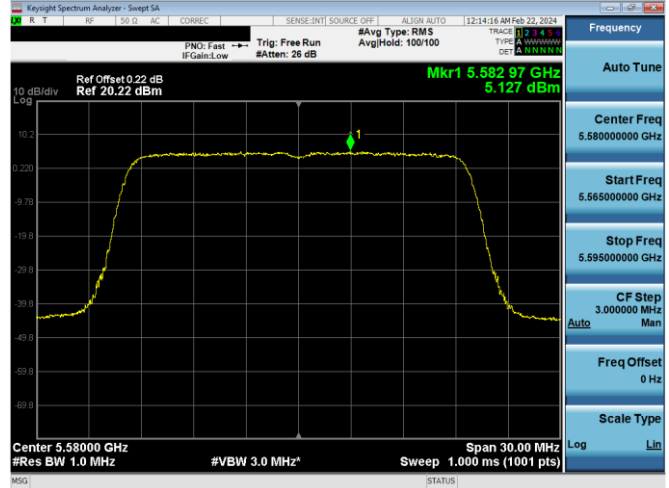
Plot 7-652. PSD CDD Primary Antenna 4a (20MHz BW 802.11ax(SU) – Ch. 116, MCS4)
