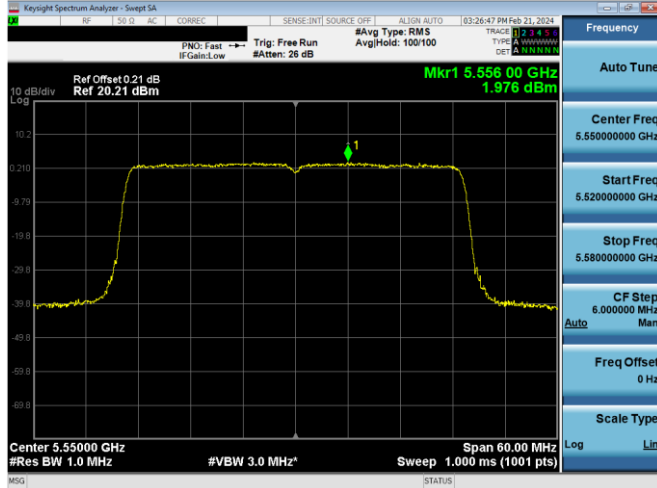
Plot 7-655. PSD CDD Primary Antenna WF5b (40MHz BW 802.11ax(SU) – Ch. 110, MCS4)
