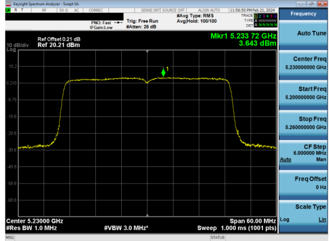
Plot 7-628. PSD CDD Primary Antenna 4a (40MHz BW 802.11ax(SU) – Ch. 46, MCS4)
