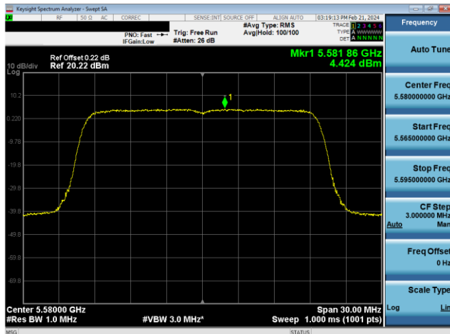
Plot 7-651. PSD CDD Primary Antenna WF5b (20MHz BW 802.11ax(SU) – Ch. 116, MCS4)
