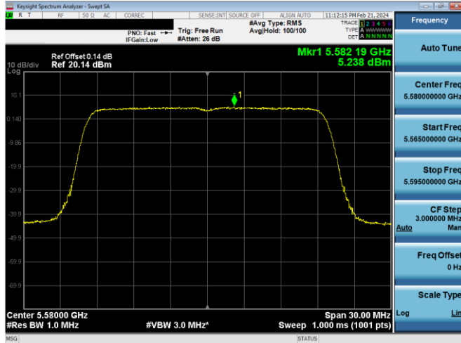
Plot 7-608. PSD CDD Primary Antenna 4a (20MHz BW 802.11ax(SU) – Ch. 116, MCS2)
