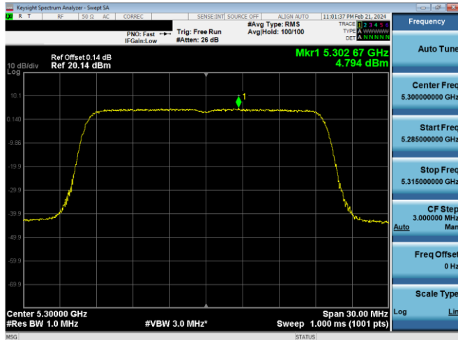
Plot 7-596. PSD CDD Primary Antenna 4a (20MHz BW 802.11ax(SU) – Ch. 60, MCS2)
