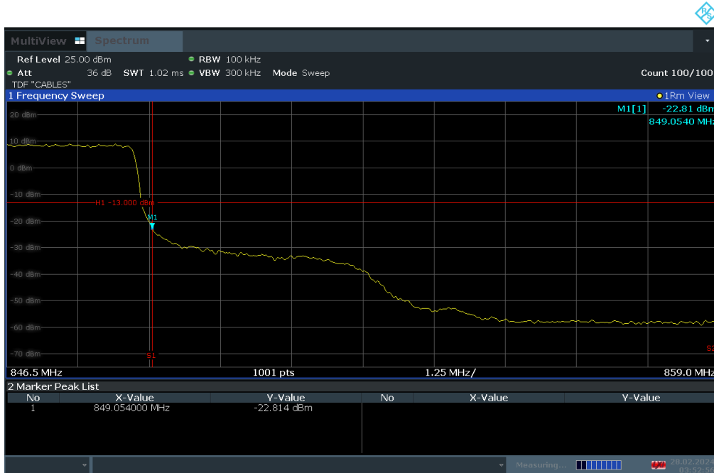
Plot 7-83. Upper BE Plot (LTE Band 26 - 5MHz QPSK – Full RB Configuration)
