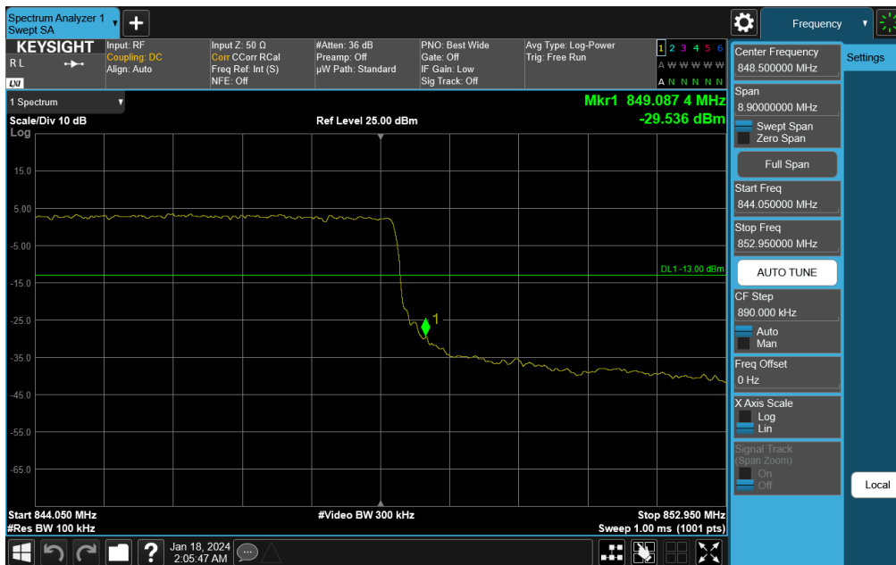
Plot 7-99. Upper BE Plot (NR Band n26 CP-OFDM QPSK – 10.0MHz - Full RB)
