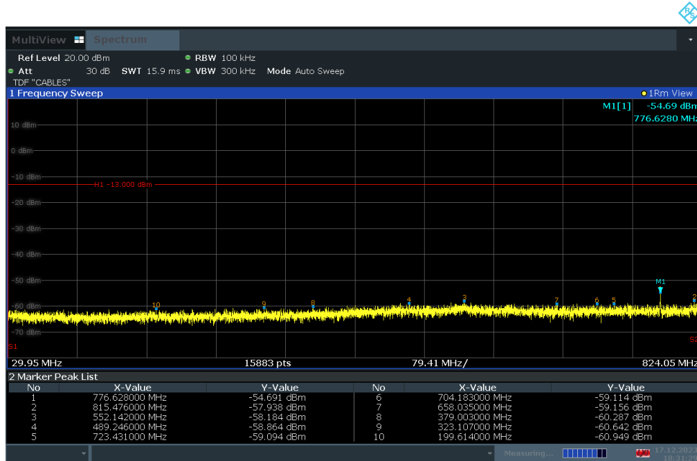
Plot 7-45. Conducted Spurious Plot (LTE Band 26/5 - 10MHz QPSK - RB Size 1, RB Offset 0 - Mid Channel)
