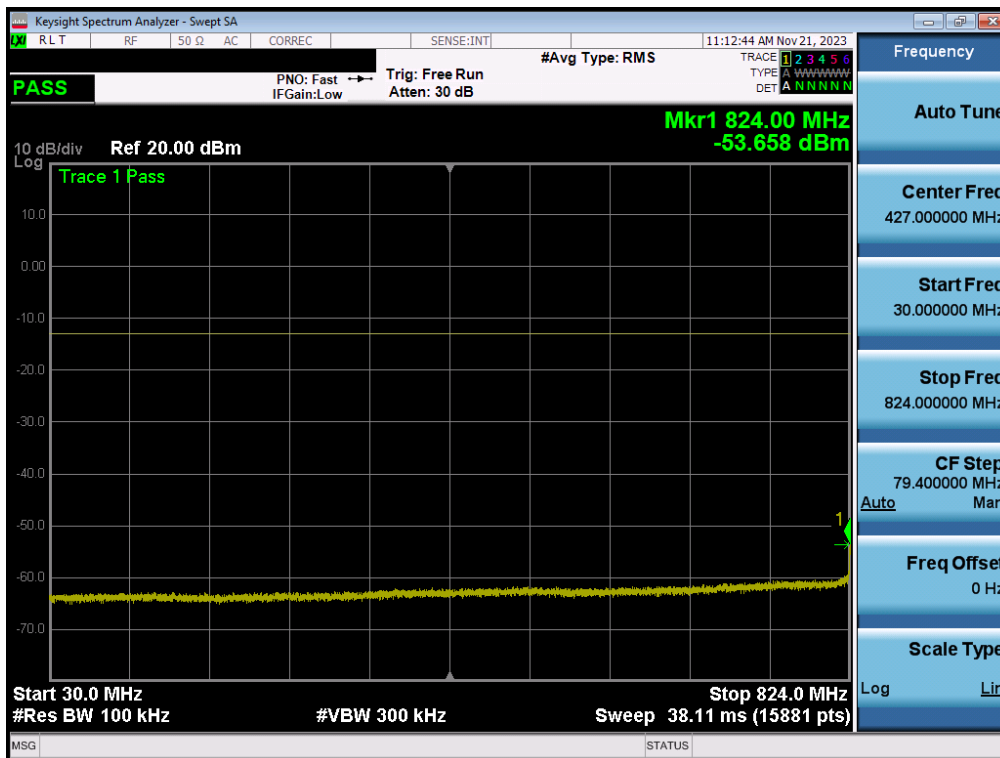
Plot 7-72. Conducted Spurious Plot (WCDMA Ch. 4183)
