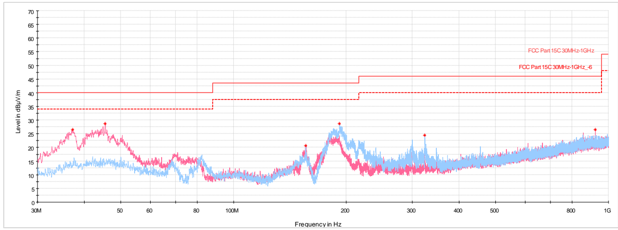
Plot 7-222. Radiated Spurious Emissions Below 1GHz TxBF (HDR4, ePA – 5245MHz), with AC/DC Adapter
