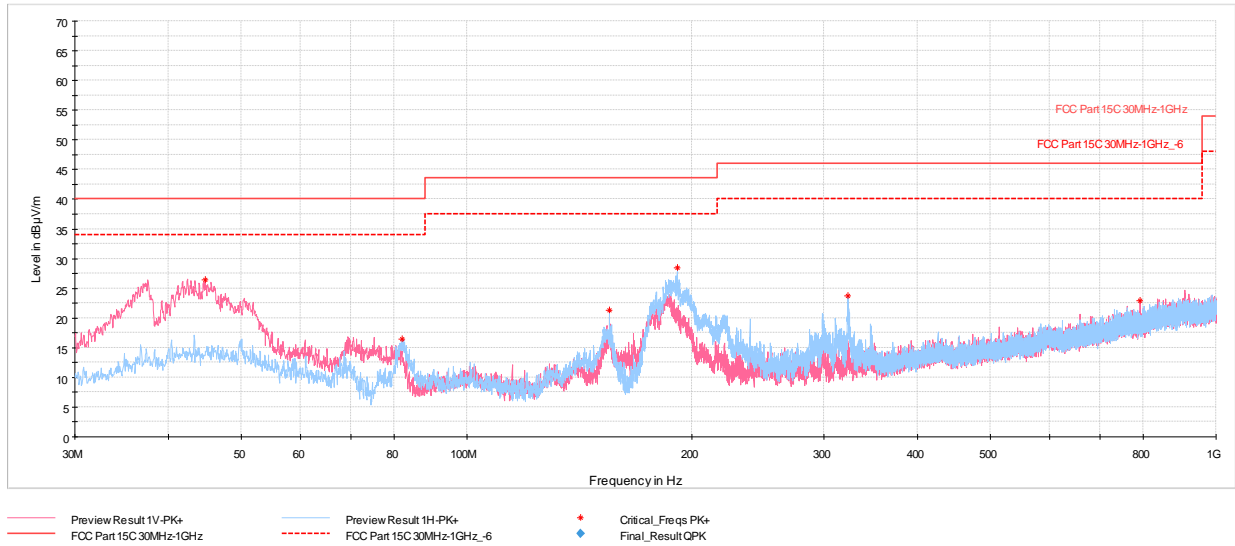
Plot 7-223. Radiated Spurious Emissions Below 1GHz TxBF (HDR4, ePA – 5844MHz), with AC/DC Adapter
