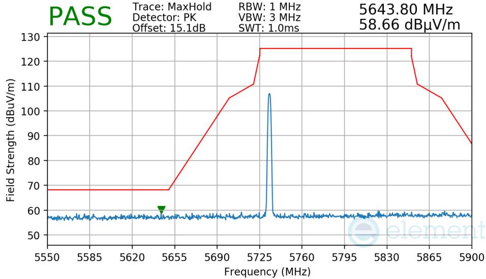
Plot 7-212. Radiated Lower Band Edge Measurement Antenna 2a
