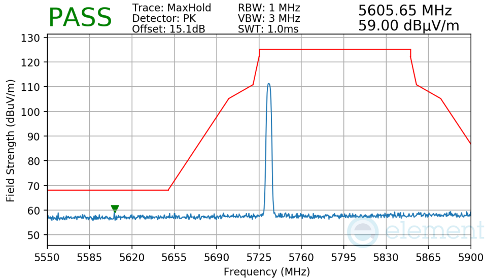
Plot 7-218. Radiated Lower Band Edge Measurement TxBF
