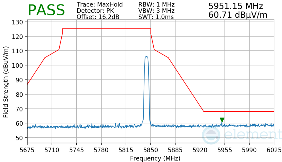
Plot 7-215. Radiated Upper Band Edge Measurement Antenna 2a
