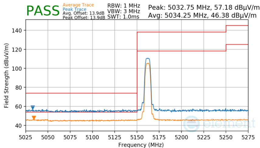
Plot 7-217. Radiated Lower Band Edge Measurement TxBF
