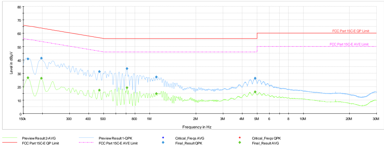
Plot 7-227. AC Line Conducted Plot TxBF (HDR4, ePA – 5844MHz) (N) with AC/DC Adapter
