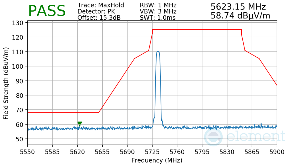
Plot 7-219. Radiated Lower Band Edge Measurement TxBF
