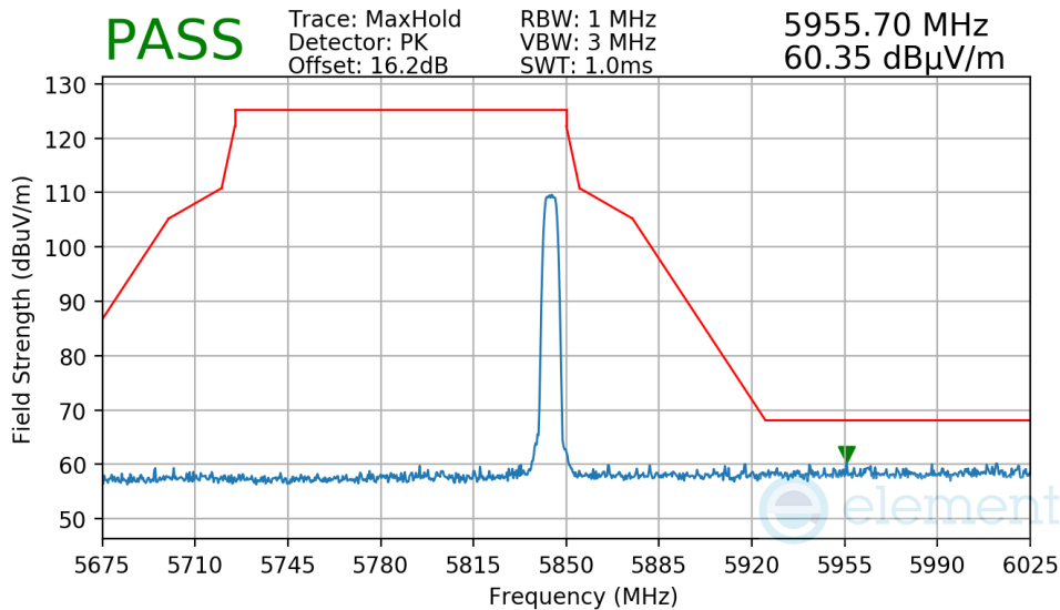
Plot 7-221. Radiated Upper Band Edge Measurement TxBF
