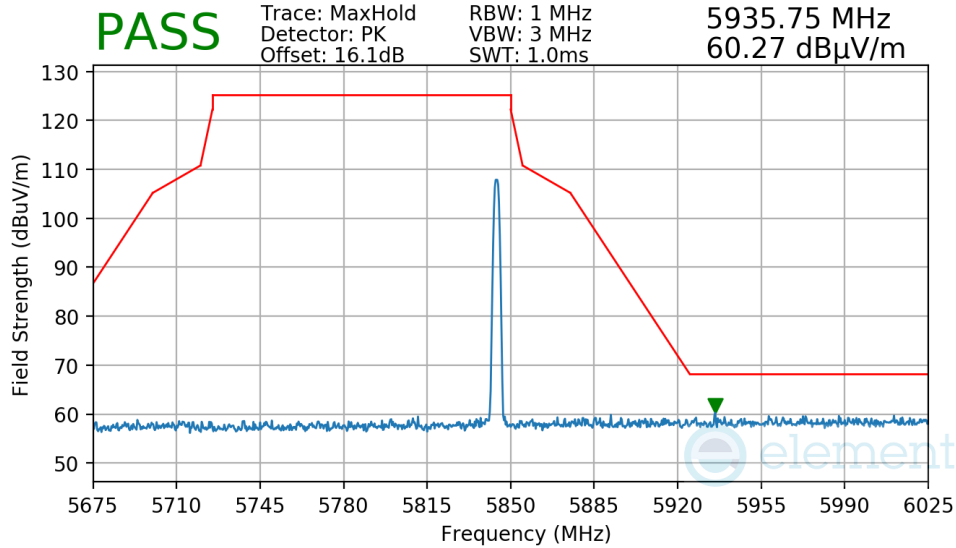
Plot 7-214. Radiated Upper Band Edge Measurement Antenna 2a
