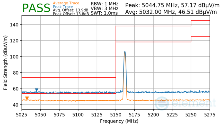
Plot 7-210. Radiated Lower Band Edge Measurement Antenna 2a
