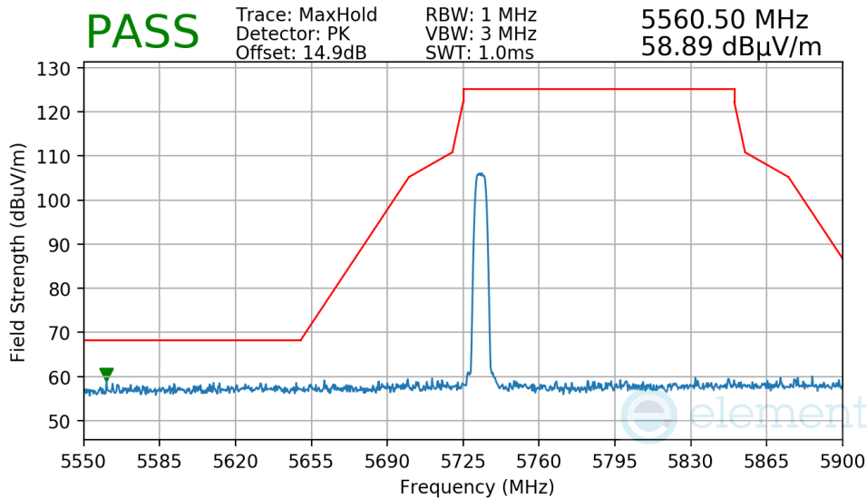
Plot 7-213. Radiated Lower Band Edge Measurement Antenna 2a
