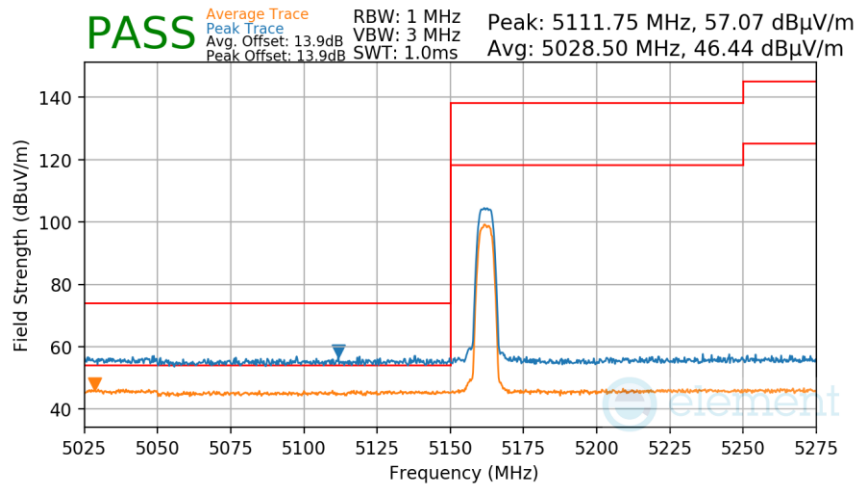
Plot 7-211. Radiated Lower Band Edge Measurement Antenna 2a
