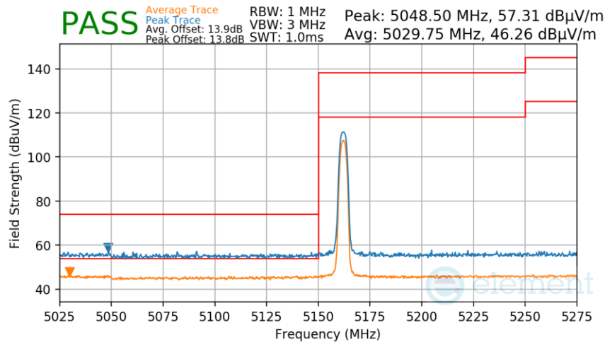
Plot 7-216. Radiated Lower Band Edge Measurement TxBF
