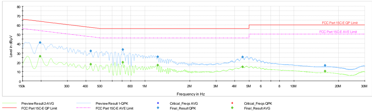
Plot 7-225. AC Line Conducted Plot TxBF (HDR4, ePA – 5245MHz) (N) with AC/DC Adapter
