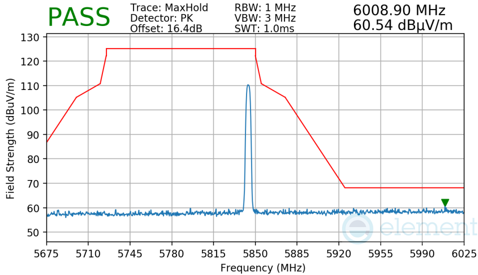
Plot 7-220. Radiated Upper Band Edge Measurement TxBF
