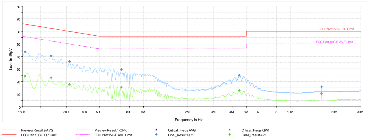
Plot 7-224. AC Line Conducted Plot TxBF (HDR4, ePA – 5245MHz) (L1) with AC/DC Adapter
