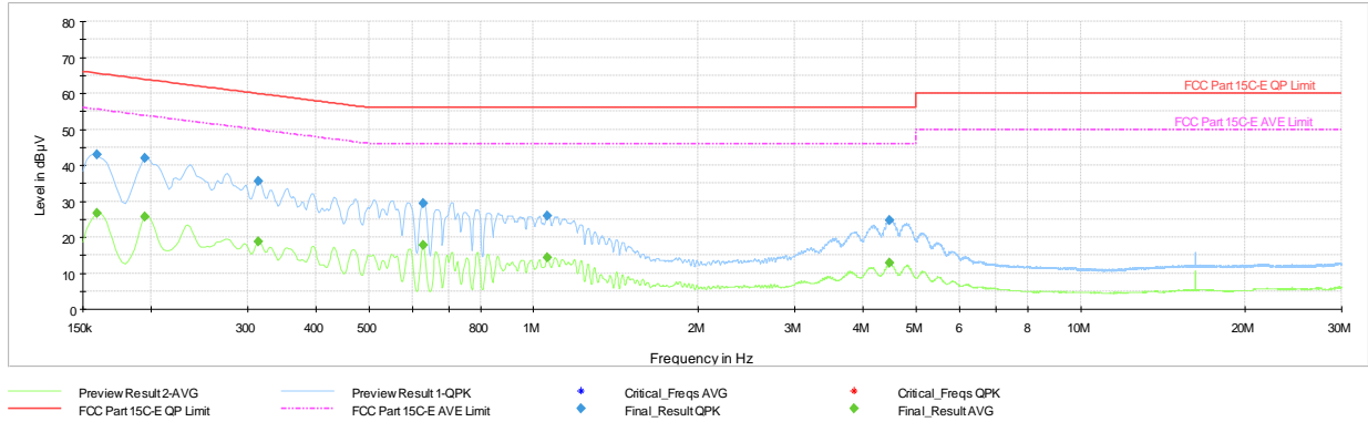
Plot 7-226. AC Line Conducted Plot TxBF (HDR4, ePA – 5844MHz) (L1) with AC/DC Adapter
