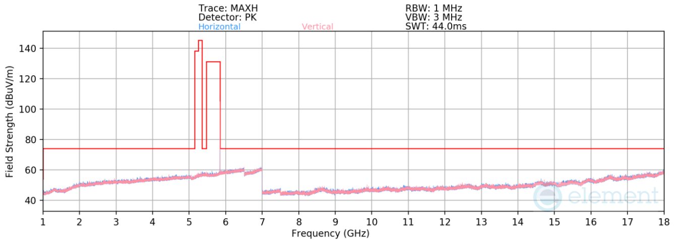
Plot 7-196. Radiated Spurious Emissions 1-18GHz TxBF (HDR4, ePA – 5844MHz)
