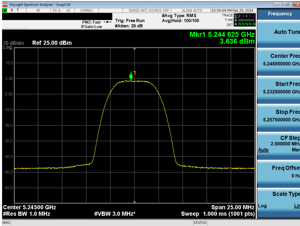
Plot 7-129. FCC PSD Tx BF Antenna 4a (HDR8, ePA- 5245MHz)
