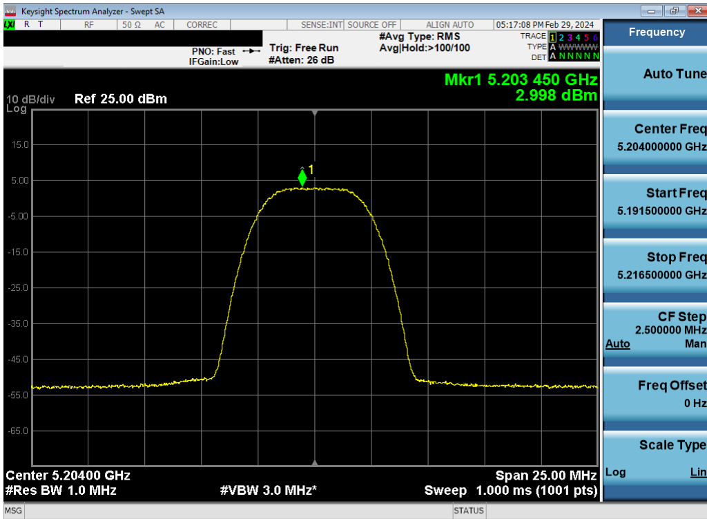
Plot 7-145. ISED PSD TxBF Antenna 4a (HDR8, ePA – 5204MHz)
