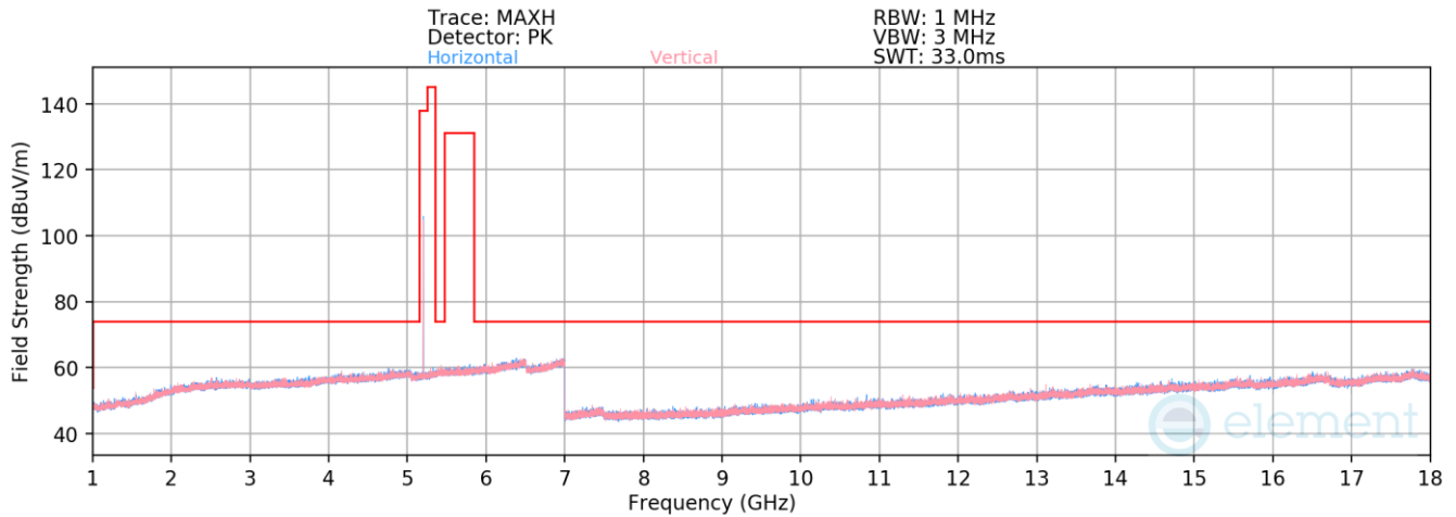
Plot 7-179. Radiated Spurious Emissions 1-18GHz Antenna 4a (HDR4, ePA – 5204MHz)
