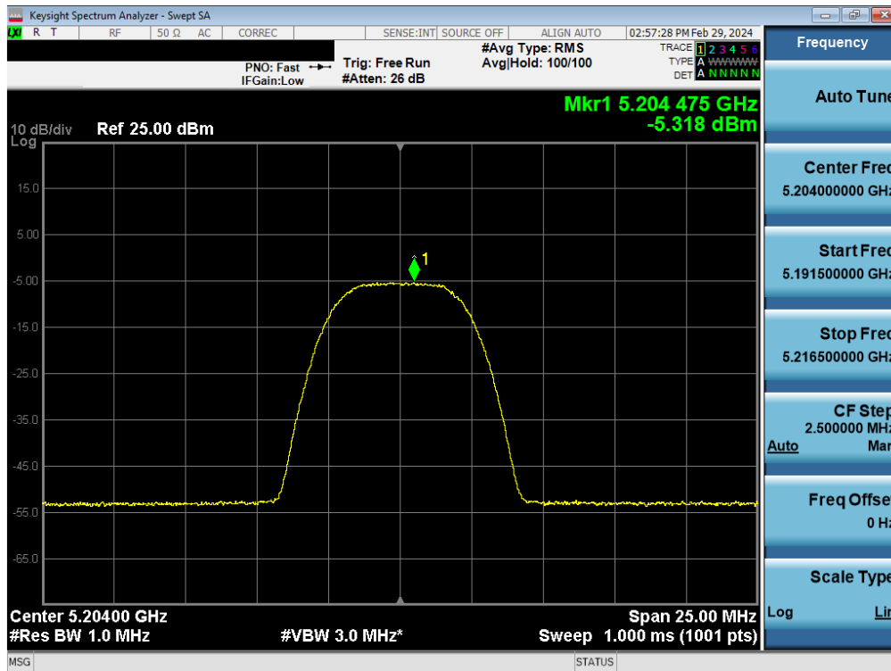
Plot 7-133. FCC/ISED PSD TxBF Antenna 4a (HDR8, iPA – 5204MHz)
