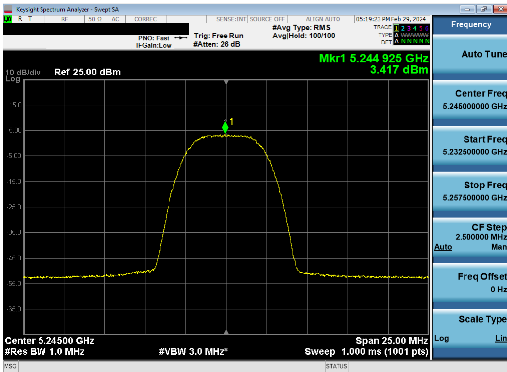
Plot 7-147. ISED PSD TxBF Antenna 4a (HDR8, ePA- 5245MHz)
