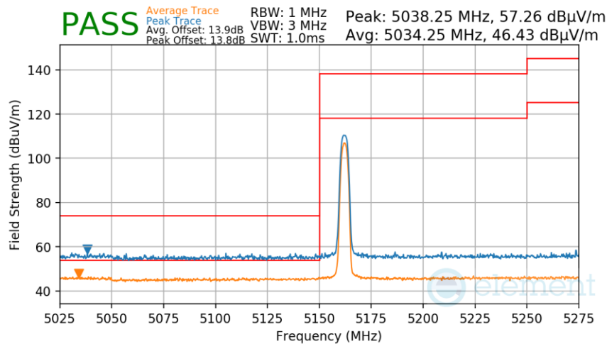
Plot 7-198. Radiated Lower Band Edge Measurement Antenna WF5B
