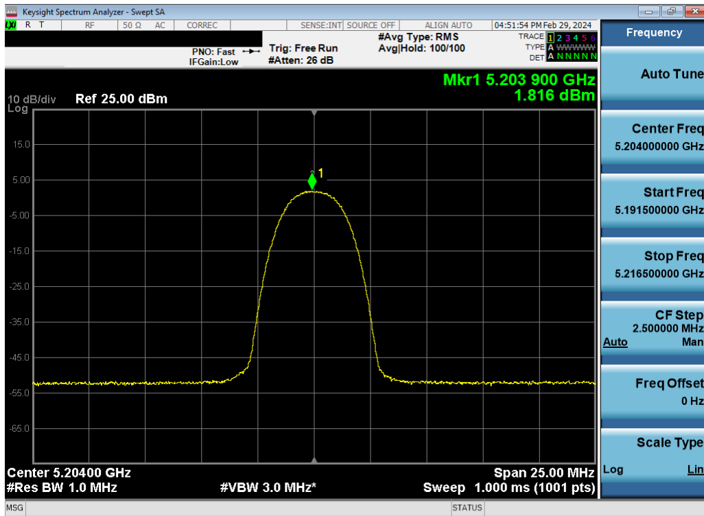
Plot 7-138. ISED PSD TxBF Antenna WF5B (HDR4, ePA – 5204MHz)
