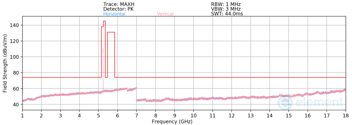
Plot 7-192. Radiated Spurious Emissions 1-18GHz TxBF (HDR4, ePA – 5245MHz)
