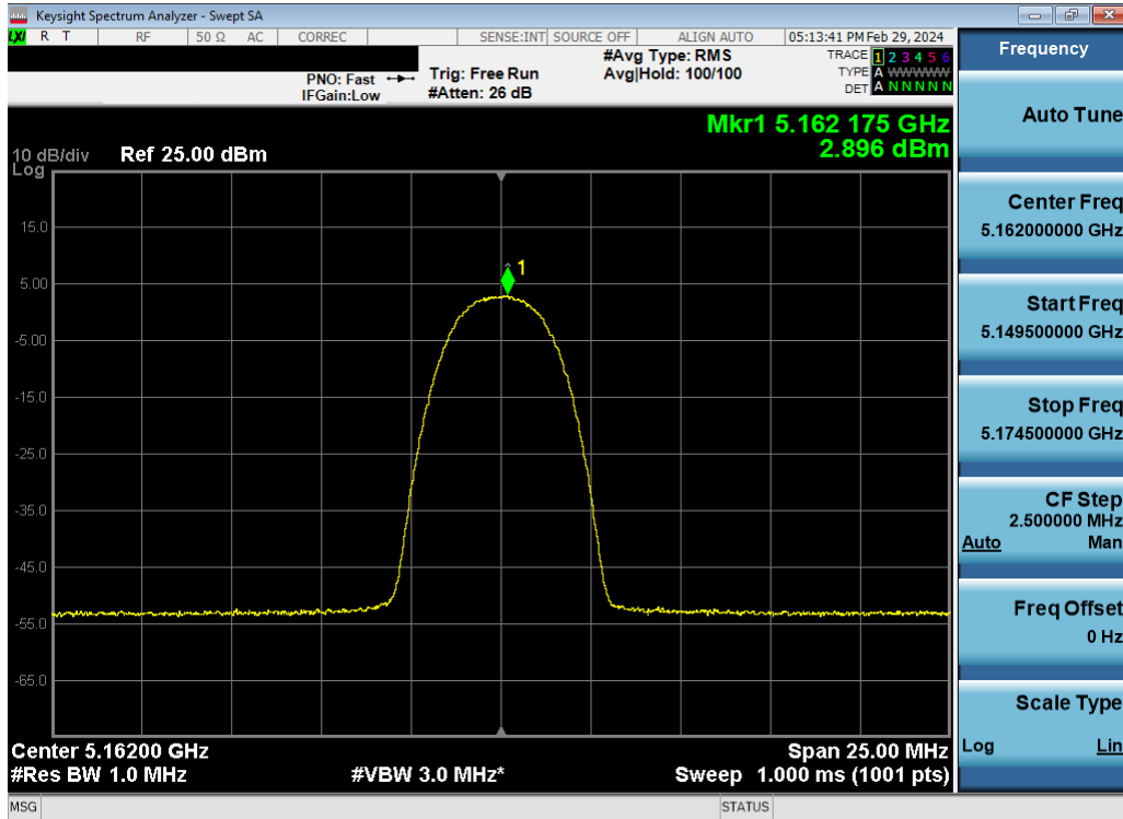
Plot 7-137. ISED PSD TxBF Antenna 4a (HDR4, ePA – 5162MHz)
