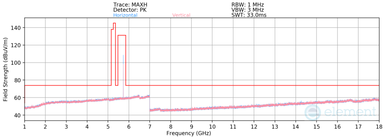
Plot 7-175. Radiated Spurious Emissions 1-18GHz Antenna WF5B (HDR4, ePA – 5733MHz)
