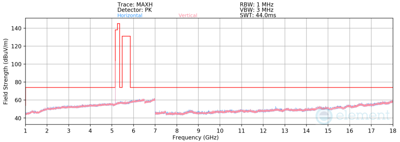
Plot 7-184. Radiated Spurious Emissions 1-18GHz Antenna 2a (HDR4, ePA – 5162MHz)
