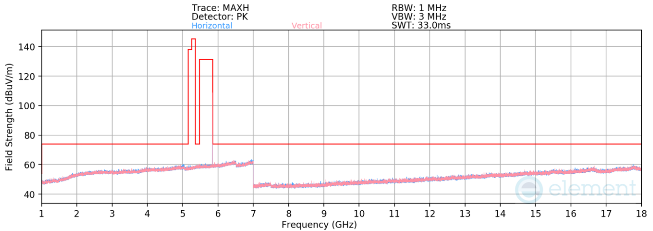
Plot 7-183. Radiated Spurious Emissions 1-18GHz Antenna 4a (HDR4, ePA – 5844MHz)
