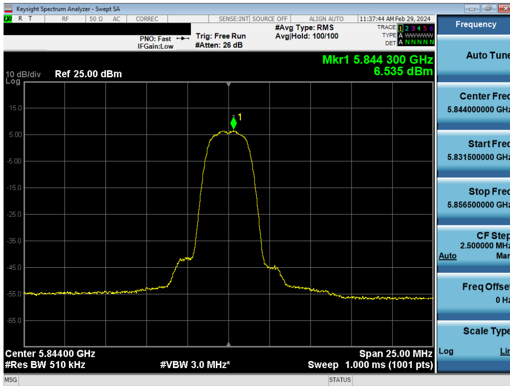
Plot 7-152. PSD TxBF Antenna WF5B (HDR4, ePA 5844MHz)
