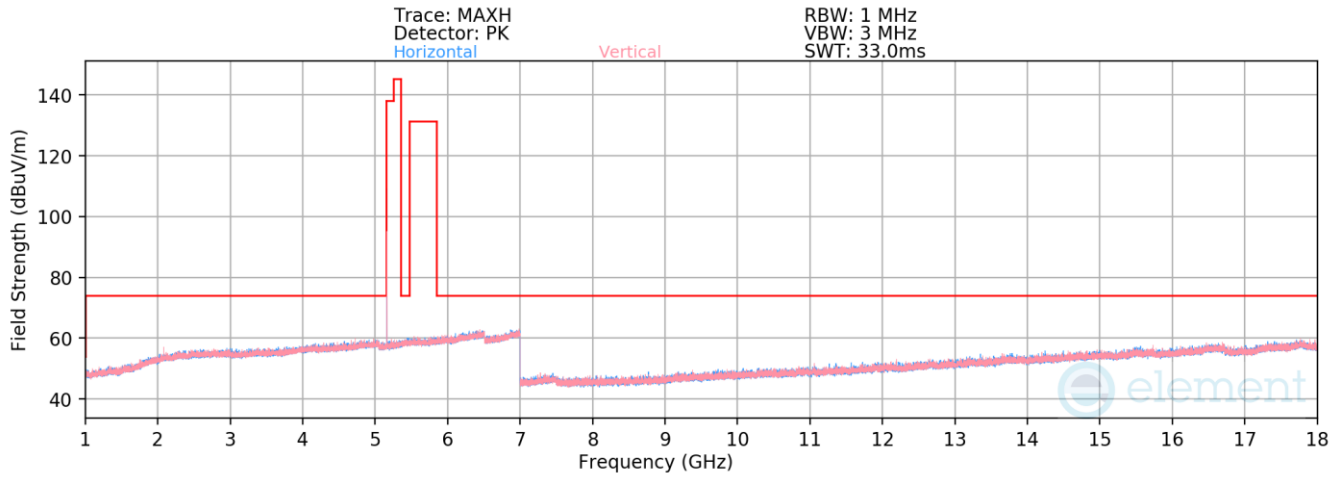
Plot 7-172. Radiated Spurious Emissions 1-18GHz Antenna WF5B (HDR4, ePA – 5162MHz)
