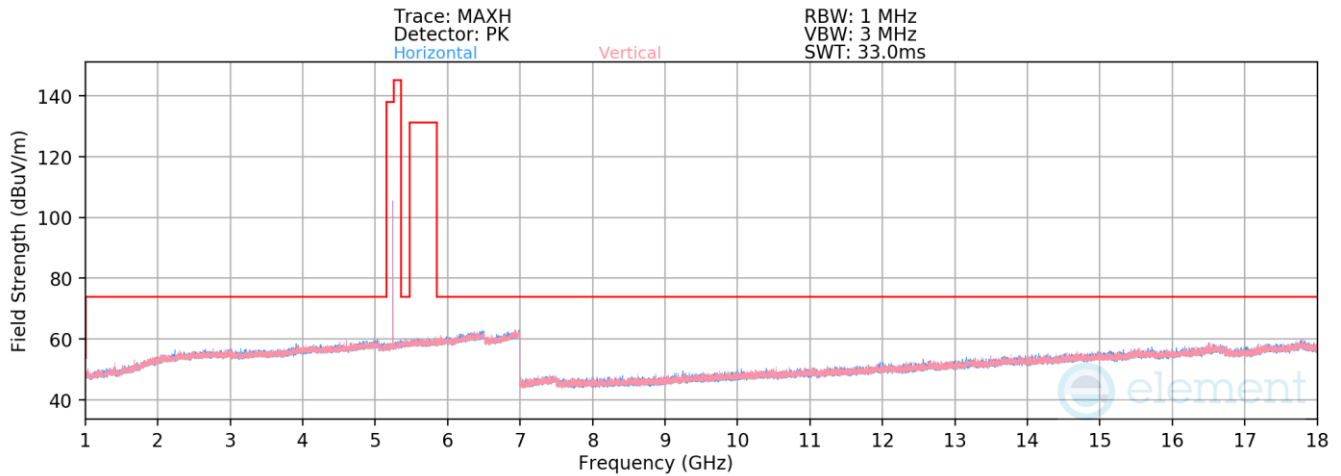
Plot 7-180. Radiated Spurious Emissions 1-18GHz Antenna 4a (HDR4, ePA – 5245MHz)
