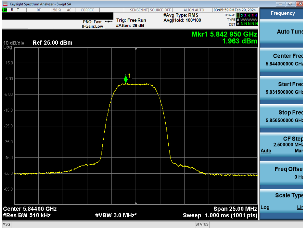
Plot 7-165. PSD TxBF Antenna 4a (HDR8, ePA 5844MHz)
