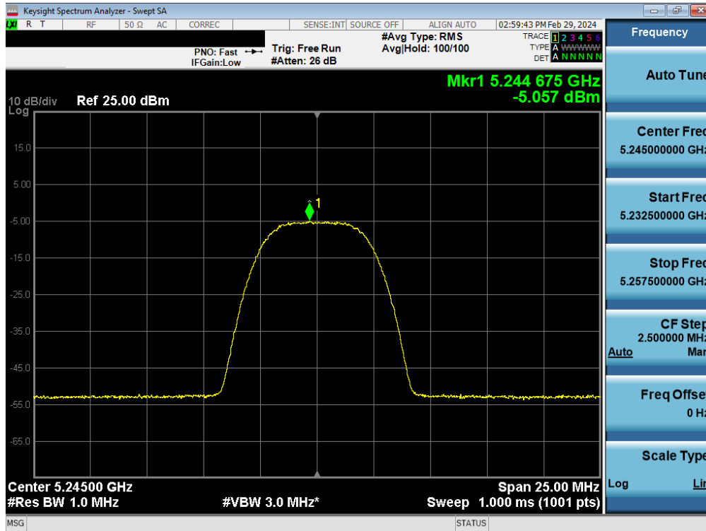
Plot 7-135. FCC/ISED PSD TxBF Antenna 4a (HDR8, iPA- 5245MHz)
