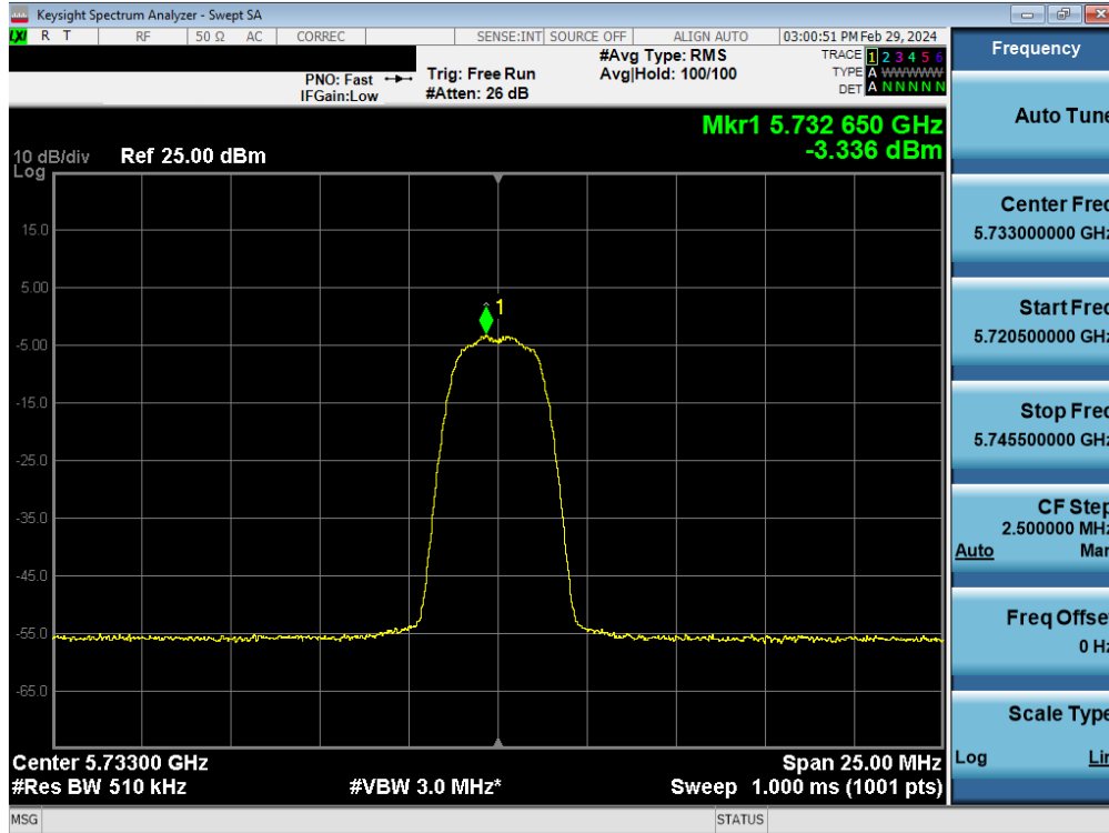
Plot 7-155. PSD TxBF Antenna 4a (HDR4, iPA 5733MHz)
