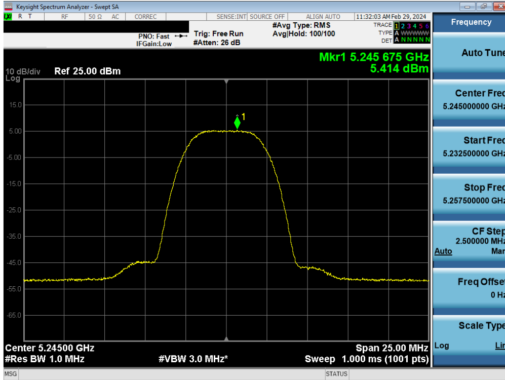
Plot 7-128. FCC PSD Tx BF Antenna WF5B (HDR8, ePA- 5245MHz)
