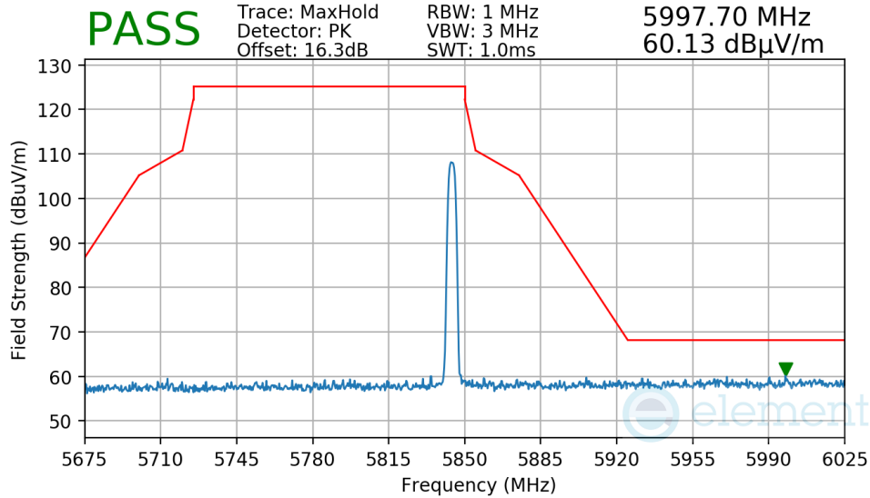
Plot 7-202. Radiated Upper Band Edge Measurement Antenna WF5B
