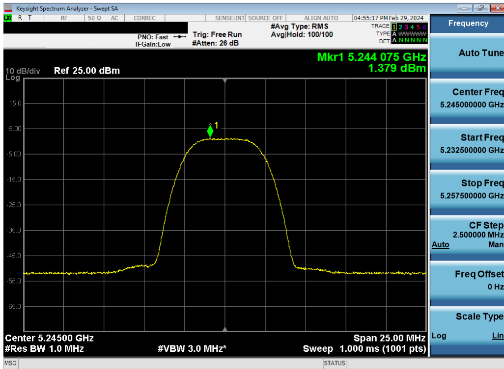
Plot 7-146. ISED PSD TxBF Antenna WF5B (HDR8, ePA- 5245MHz)
