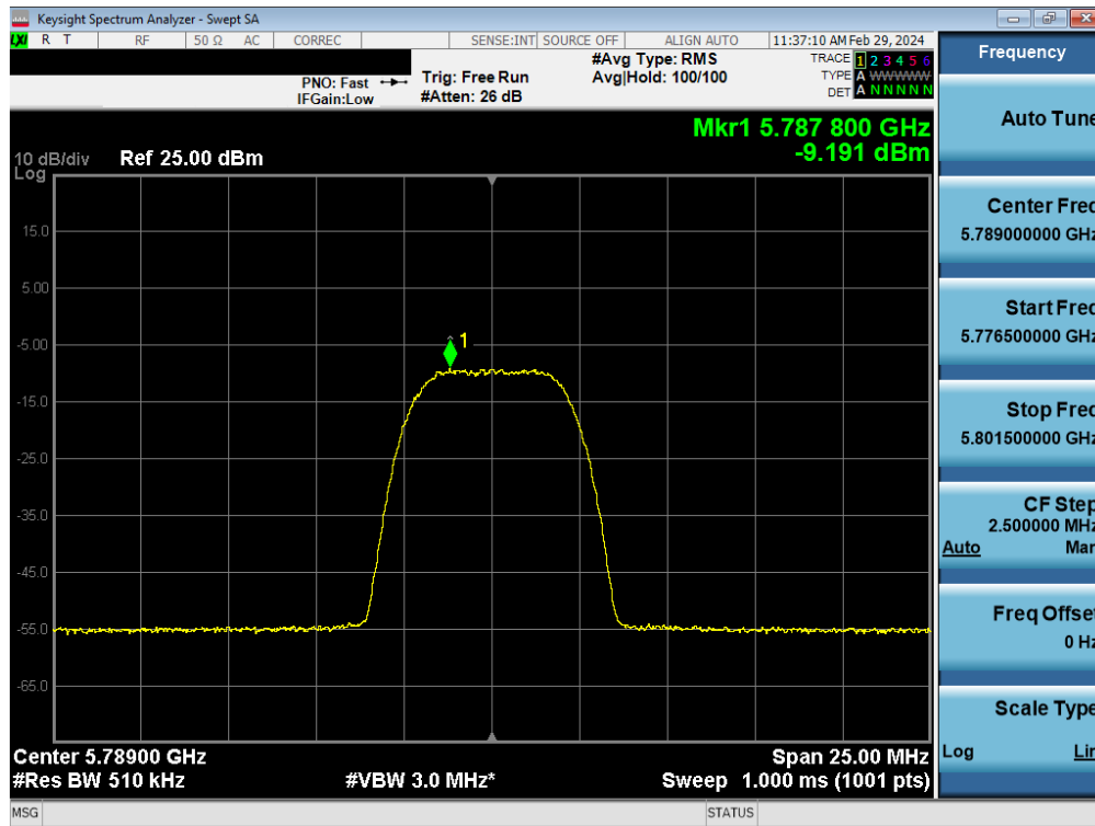
Plot 7-168. PSD TxBF Antenna WF5B (HDR8, iPA 5789MHz)
