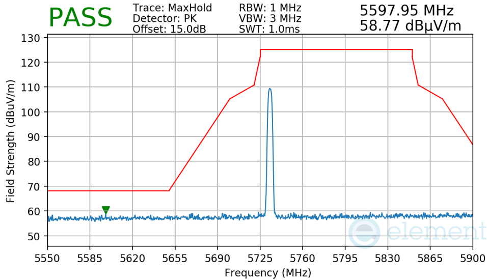
Plot 7-200. Radiated Lower Band Edge Measurement Antenna WF5B
