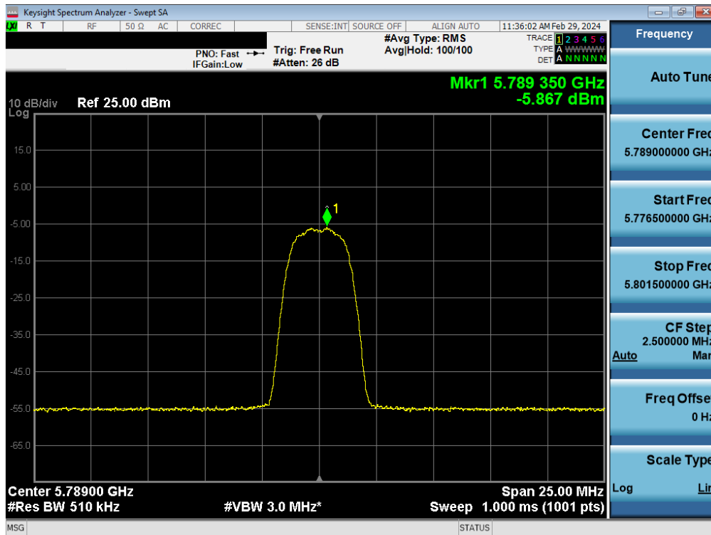
Plot 7-156. PSD TxBF Antenna WF5B (HDR4, iPA 5789MHz)
