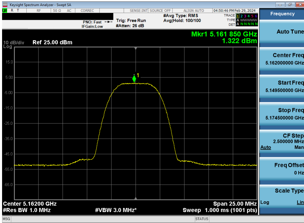
Plot 7-142. ISED PSD Tx BF Antenna WF5B (HDR8, ePA – 5162MHz)
