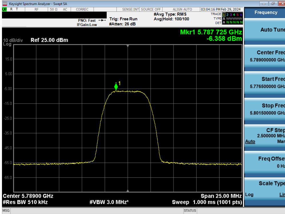
Plot 7-169. PSD TxBF Antenna 4a (HDR8, iPA 5789MHz)
