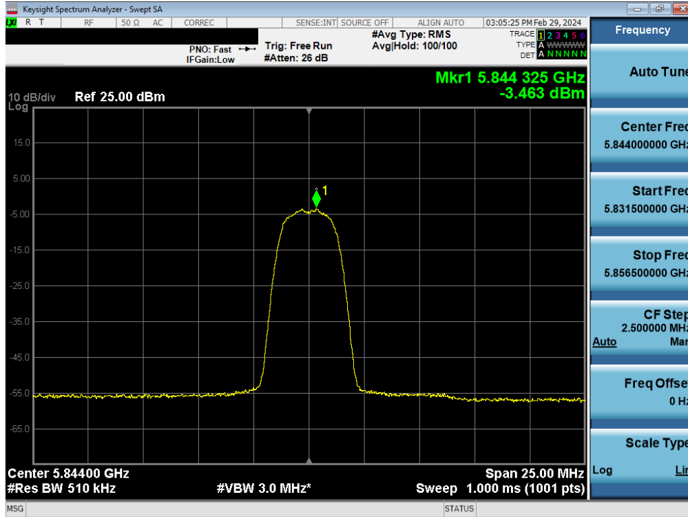
Plot 7-159. PSD TxBF Antenna 4a (HDR4, iPA 5844MHz)
