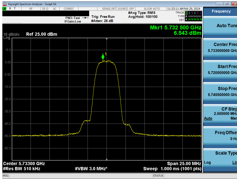
Plot 7-148. PSD TxBF Antenna WF5B (HDR4, ePA 5733MHz)
