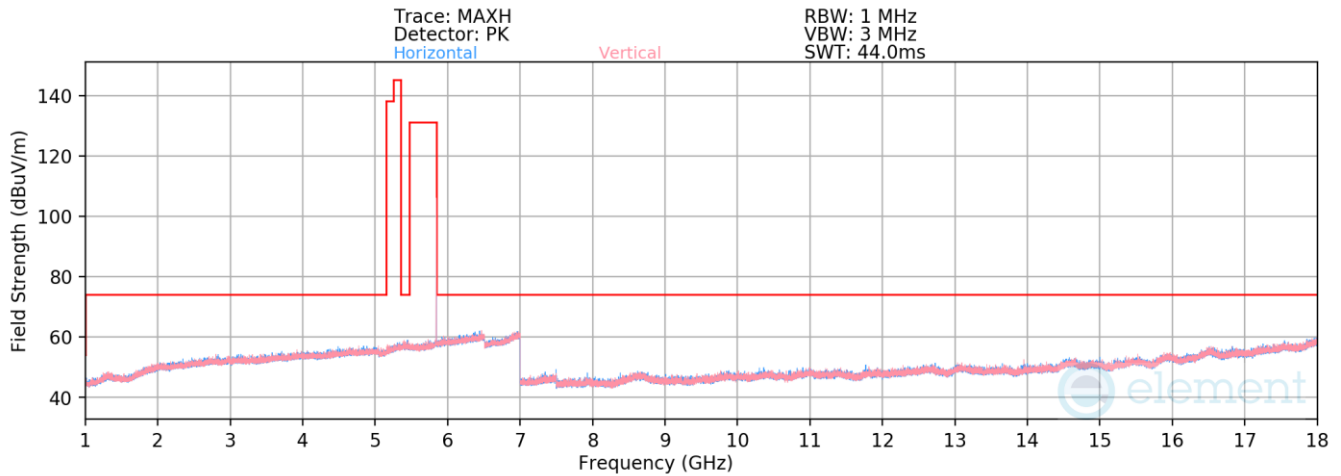
Plot 7-189. Radiated Spurious Emissions 1-18GHz Antenna 2a (HDR4, ePA – 5844MHz)
