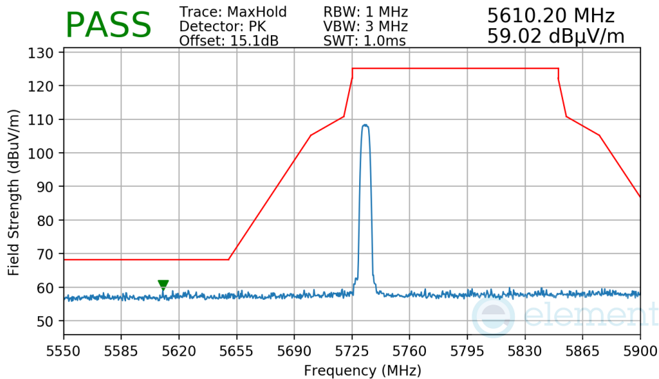
Plot 7-201. Radiated Lower Band Edge Measurement Antenna WF5B
