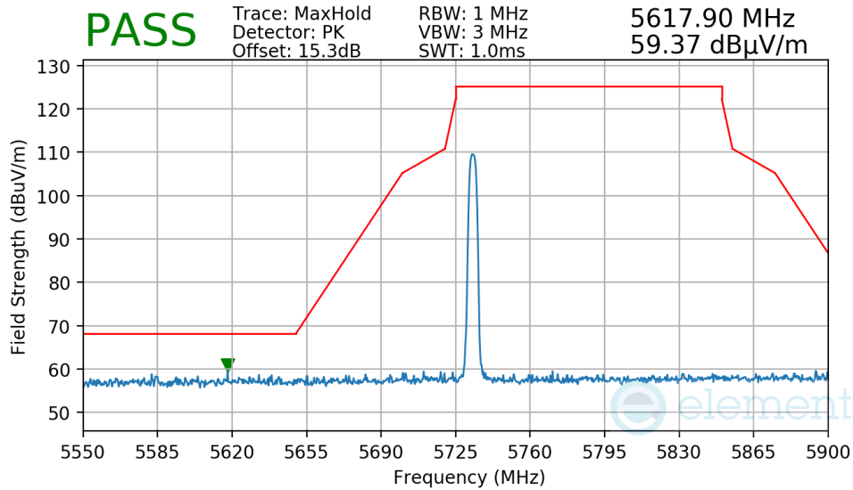
Plot 7-206. Radiated Lower Band Edge Measurement Antenna 4a
