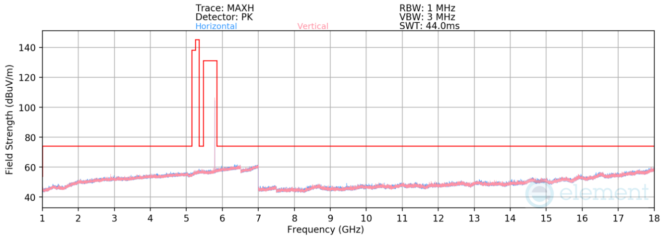
Plot 7-188. Radiated Spurious Emissions 1-18GHz Antenna 2a (HDR4, ePA – 5789MHz)
