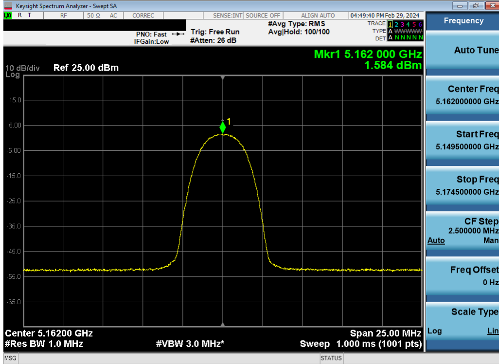
Plot 7-136. ISED PSD TxBF Antenna WF5B (HDR4, ePA – 5162MHz)
