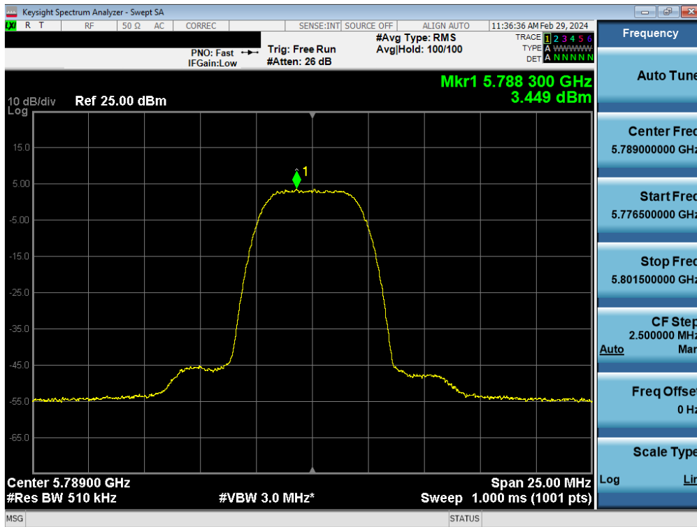
Plot 7-162. PSD TxBF Antenna WF5B (HDR8, ePA 5789MHz)
