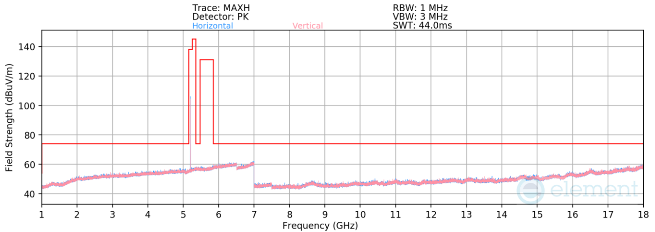
Plot 7-185. Radiated Spurious Emissions 1-18GHz Antenna 2a (HDR4, ePA – 5204MHz)
