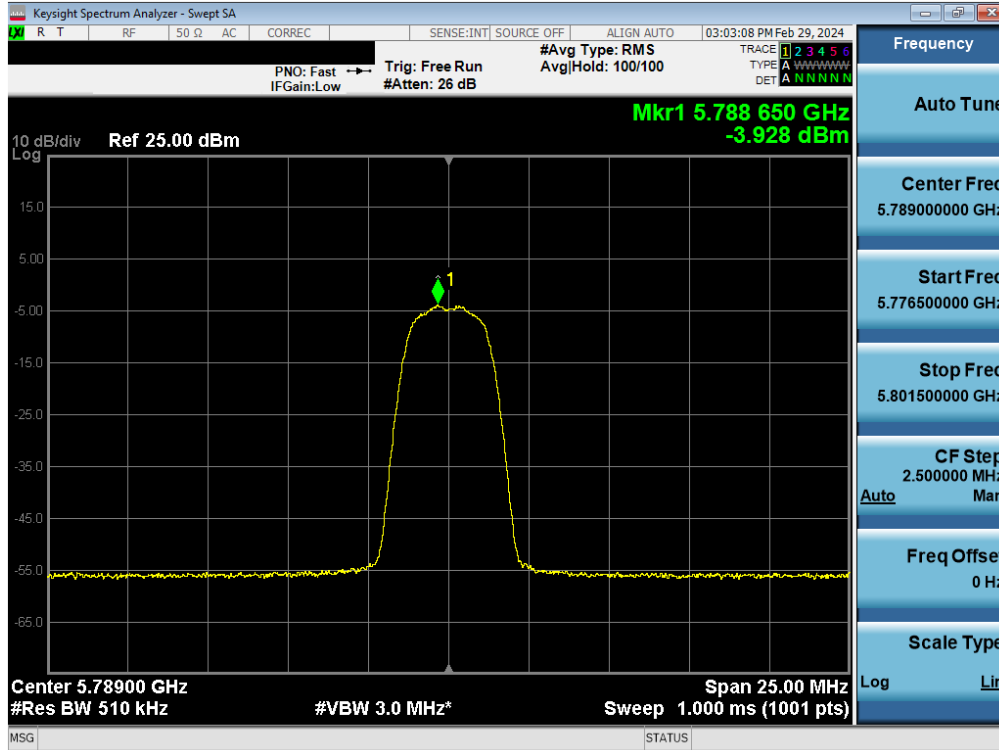
Plot 7-157. PSD TxBF Antenna 4a (HDR4, iPA 5789MHz)
