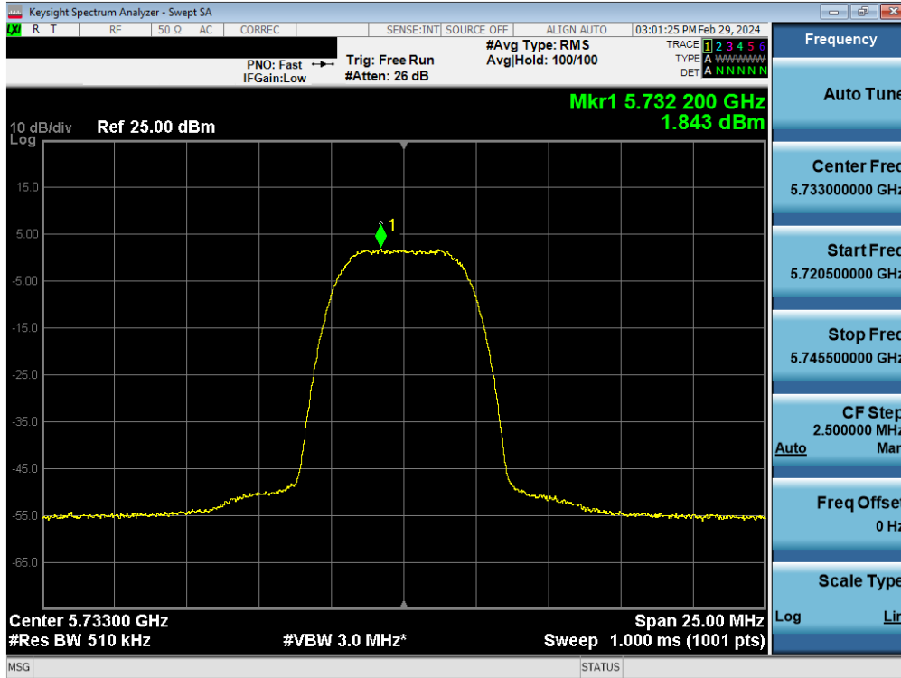
Plot 7-161. PSD TxBF Antenna 4a (HDR8, ePA 5733MHz)
