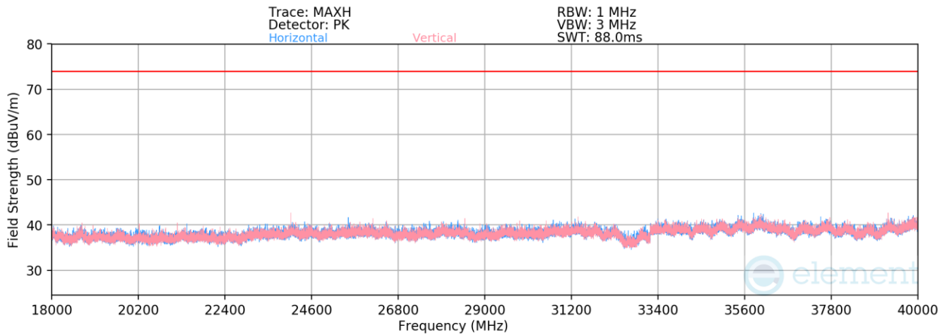
Plot 7-193. Radiated Spurious Emissions Above 18GHz TxBF (HDR4, ePA – 5245MHz)
