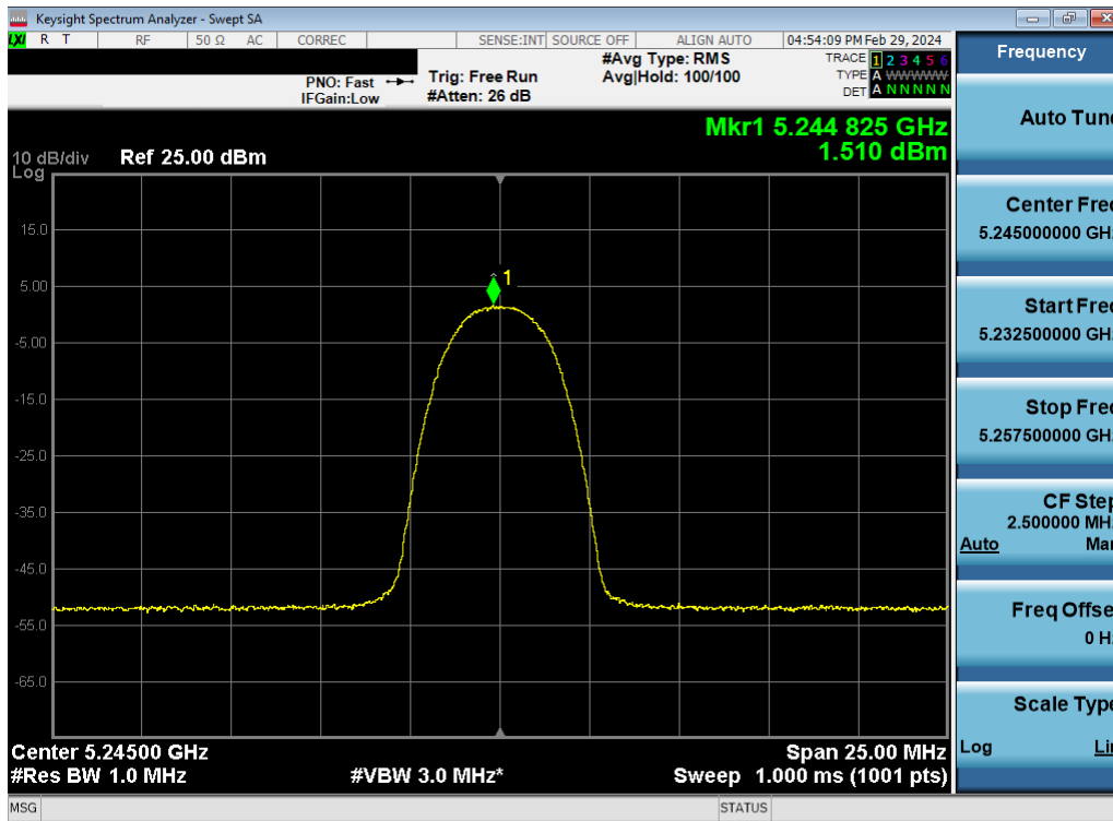
Plot 7-140. ISED PSD TxBF Antenna WF5B (HDR4, ePA- 5245MHz)
