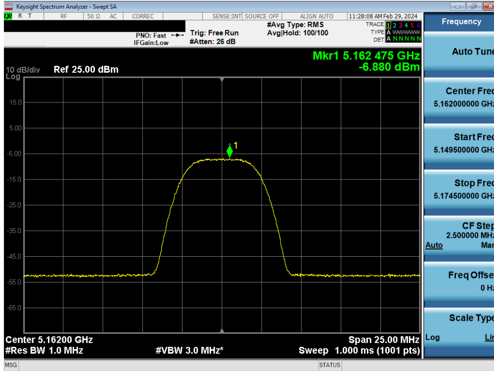
Plot 7-130. FCC/ISED PSD Tx BF Antenna WF5B (HDR8, iPA – 5162MHz)
