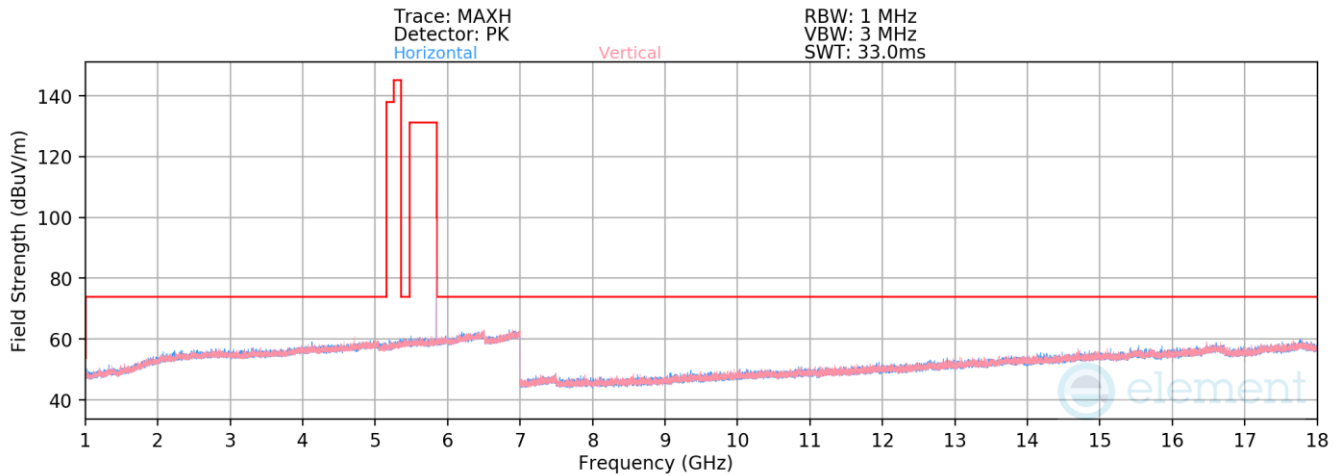
Plot 7-177. Radiated Spurious Emissions 1-18GHz Antenna WF5B (HDR4, ePA – 5844MHz)
