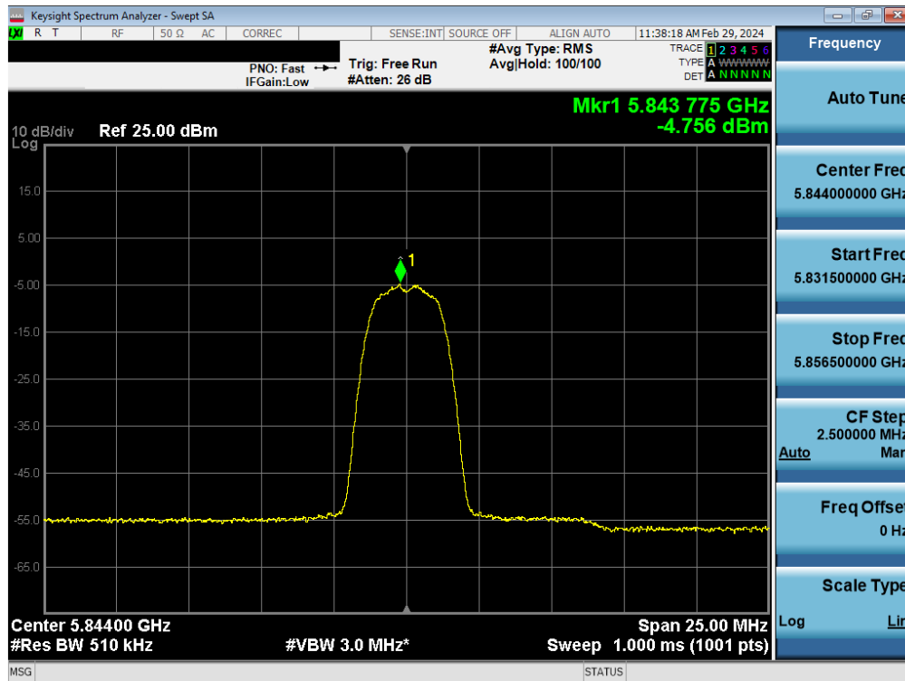
Plot 7-158. PSD TxBF Antenna WF5B (HDR4, iPA 5844MHz)
