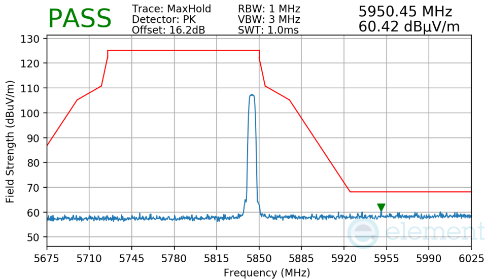
Plot 7-209. Radiated Upper Band Edge Measurement Antenna 4a
