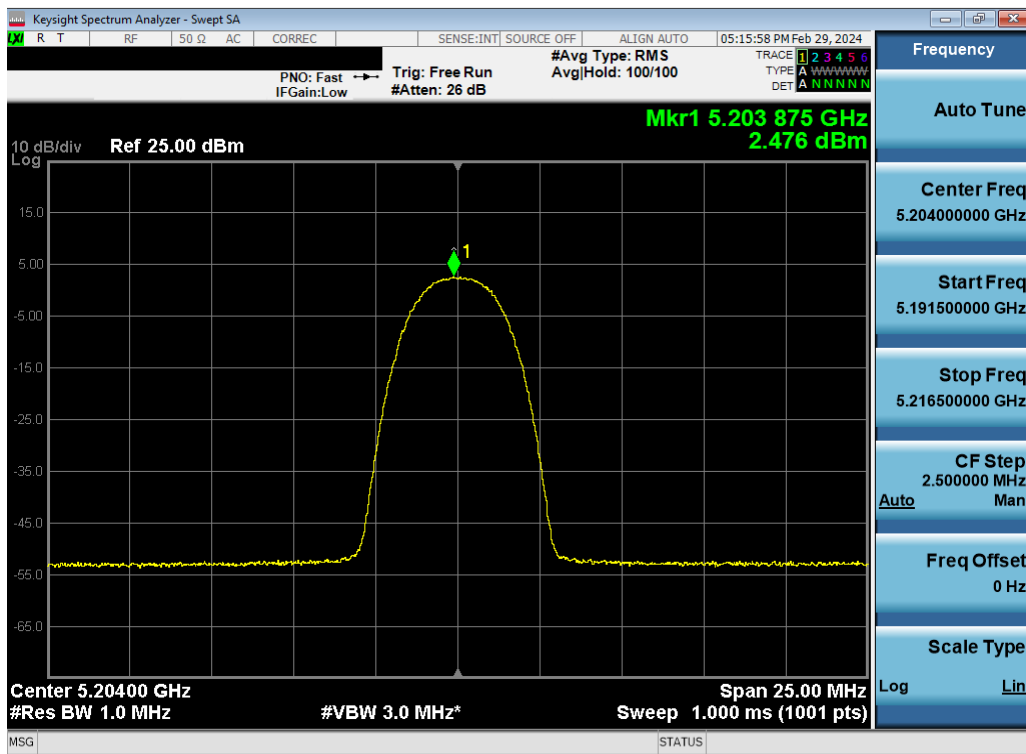
Plot 7-139. ISED PSD TxBF Antenna 4a (HDR4, ePA – 5204MHz)
