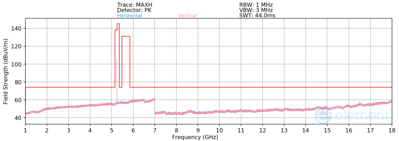
Plot 7-186. Radiated Spurious Emissions 1-18GHz Antenna 2a (HDR4, ePA – 5245MHz)
