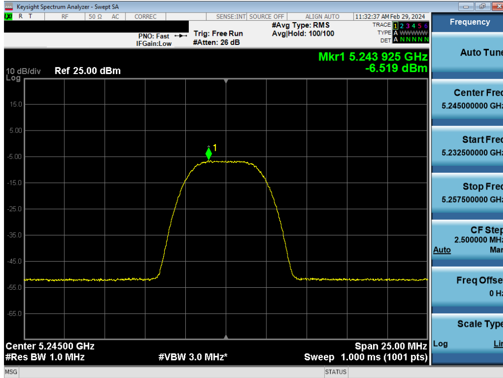
Plot 7-134. FCC/ISED PSD TxBF Antenna WF5B (HDR8, iPA- 5245MHz)
