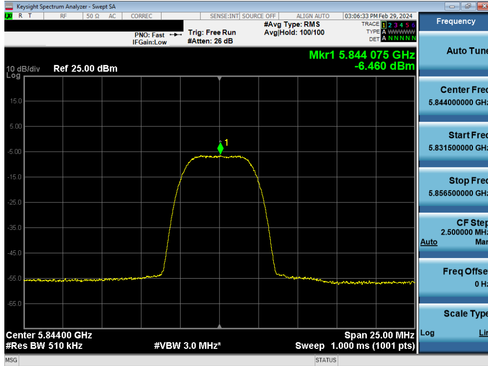
Plot 7-171. PSD TxBF Antenna 4a (HDR8, iPA 5844MHz)
