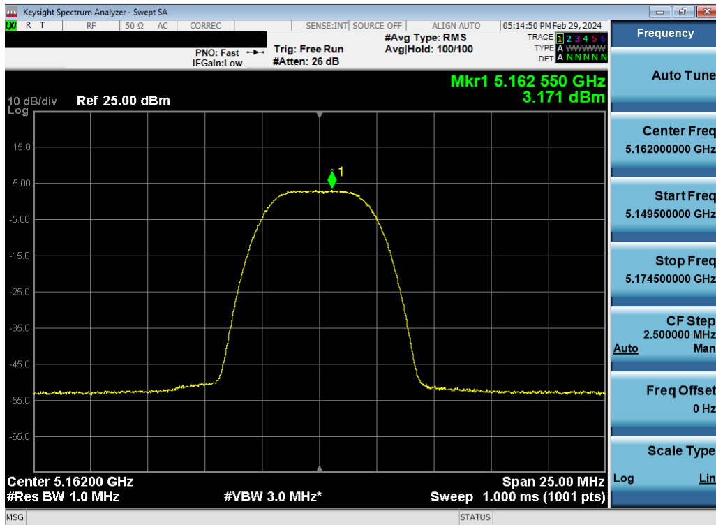
Plot 7-143. ISED PSD Tx BF Antenna 4a (HDR8, ePA – 5162MHz)
