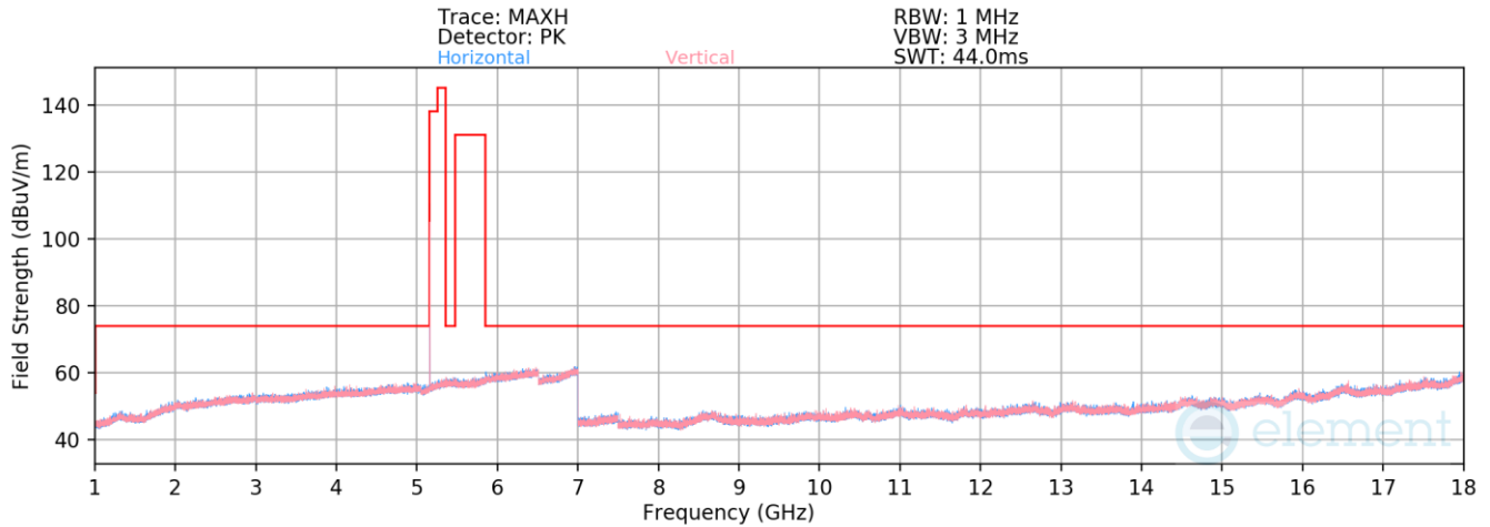
Plot 7-190. Radiated Spurious Emissions 1-18GHz TxBF (HDR4, ePA – 5162MHz)
