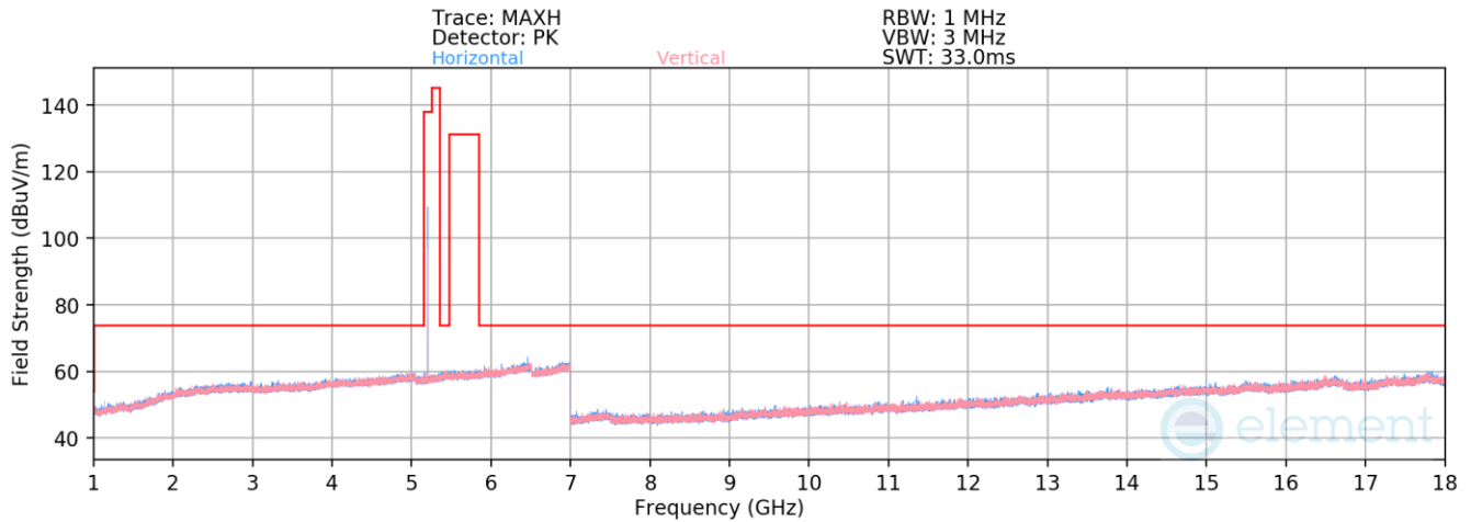
Plot 7-173. Radiated Spurious Emissions 1-18GHz Antenna WF5B (HDR4, ePA – 5204MHz)
