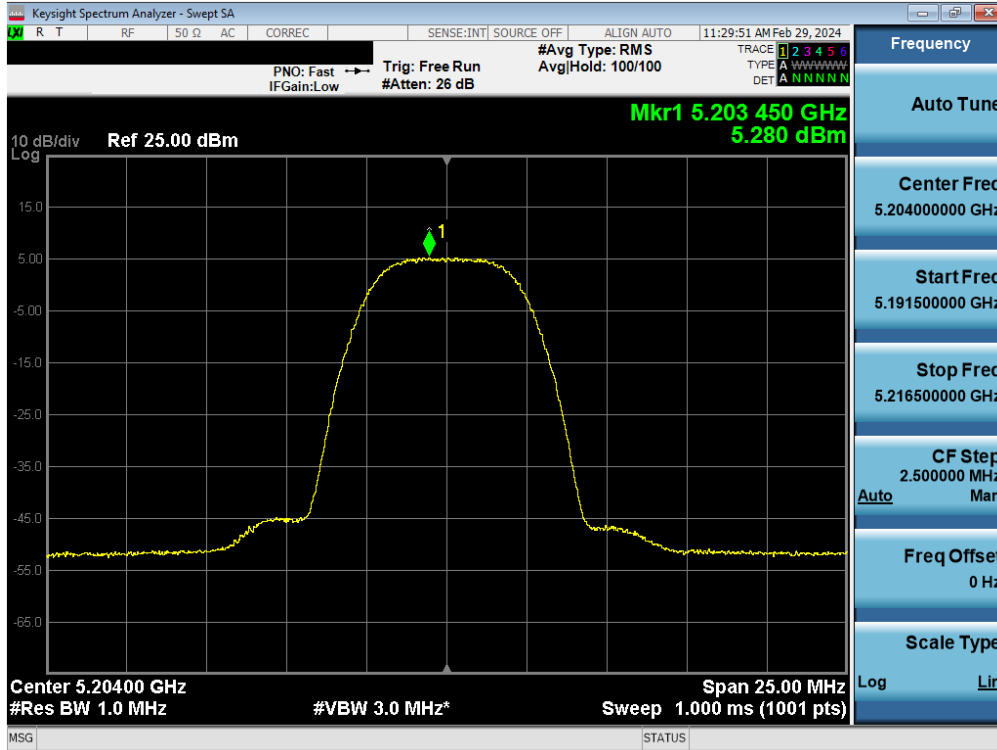
Plot 7-126. FCC PSD Tx BF Antenna WF5B (HDR8, ePA – 5204MHz)
