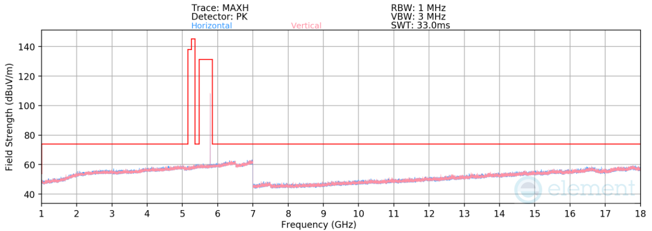
Plot 7-182. Radiated Spurious Emissions 1-18GHz Antenna 4a (HDR4, ePA – 5789MHz)
