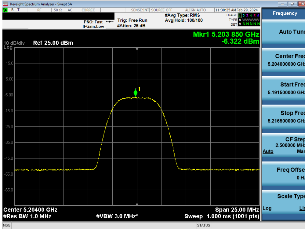
Plot 7-132. FCC/ISED PSD TxBF Antenna WF5B (HDR8, iPA – 5204MHz)
