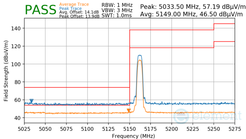
Plot 7-199. Radiated Lower Band Edge Measurement Antenna WF5B
