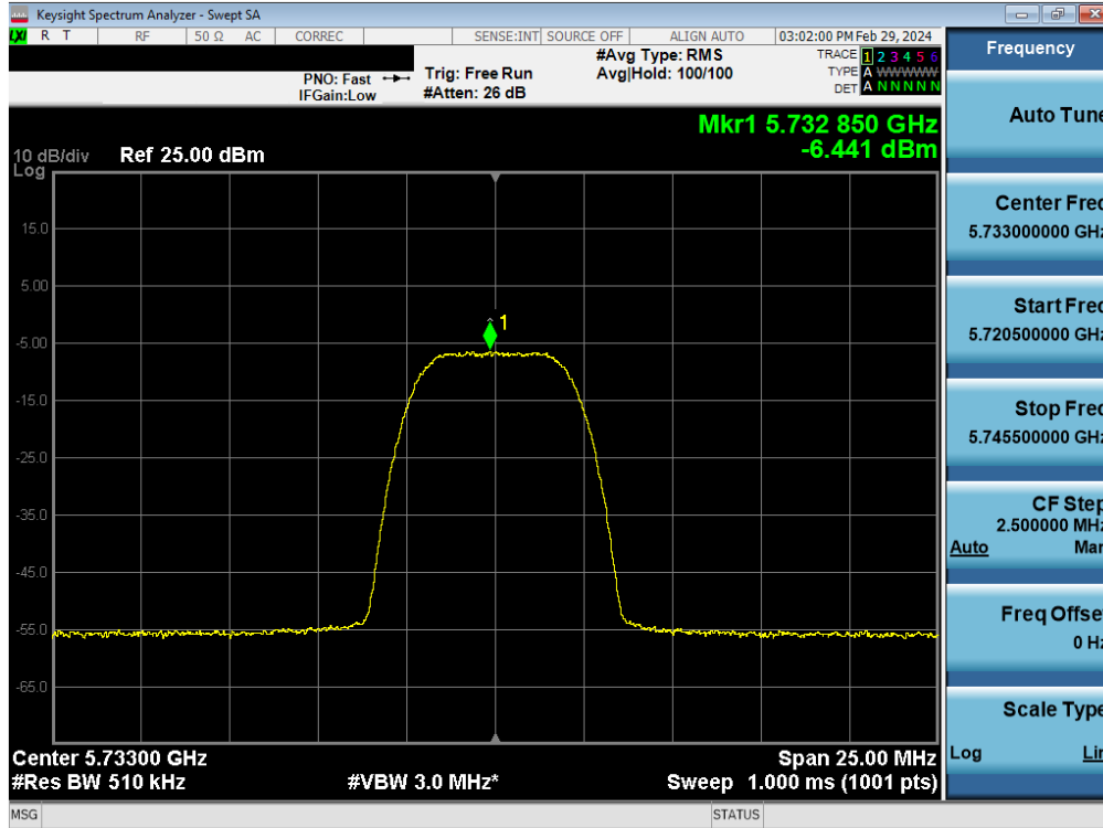
Plot 7-167. PSD TxBF Antenna 4a (HDR8, iPA 5733MHz)
