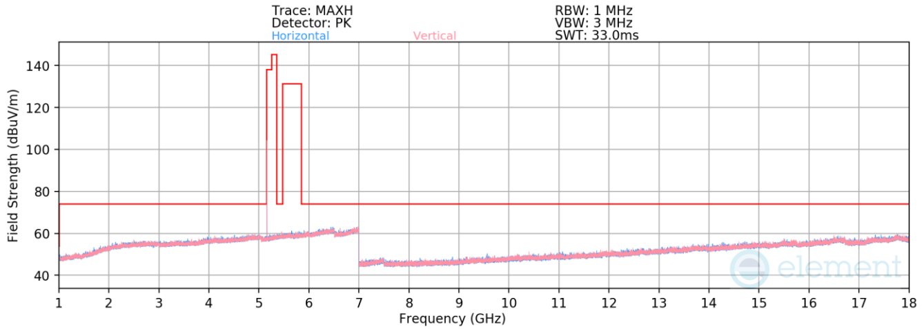
Plot 7-178. Radiated Spurious Emissions 1-18GHz Antenna 4a (HDR4, ePA - 5162MHz)
