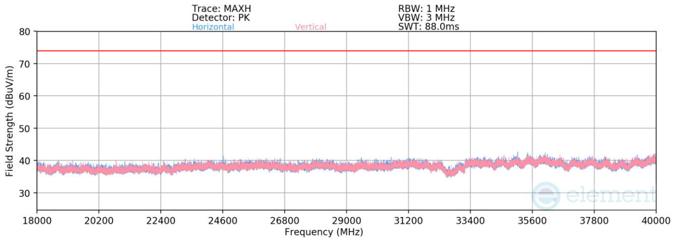
Plot 7-197. Radiated Spurious Emissions Above 18GHz TxBF (HDR4, ePA – 5844MHz)
