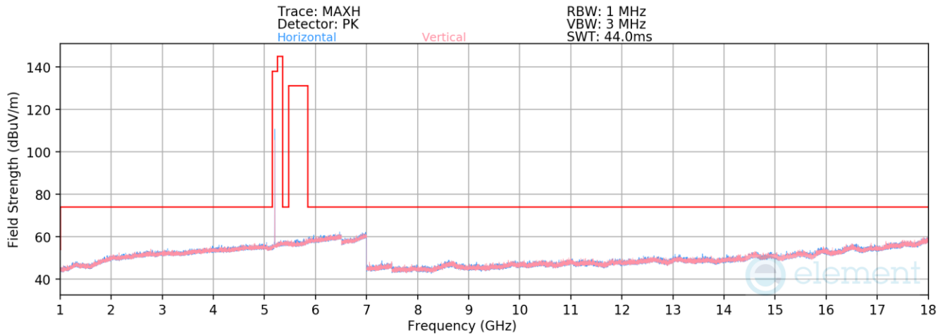
Plot 7-191. Radiated Spurious Emissions 1-18GHz TxBF (HDR4, ePA – 5204MHz)
