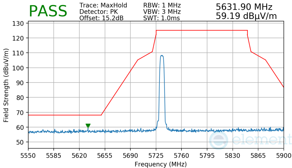
Plot 7-207. Radiated Lower Band Edge Measurement Antenna 4a
