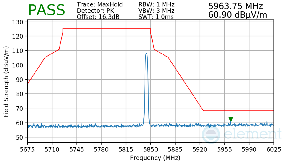
Plot 7-208. Radiated Upper Band Edge Measurement Antenna 4a
