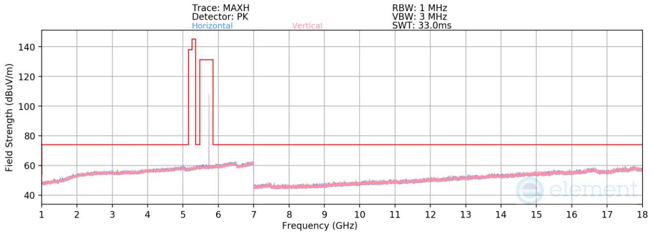
Plot 7-181. Radiated Spurious Emissions 1-18GHz Antenna 4a (HDR4, ePA – 5733MHz)
