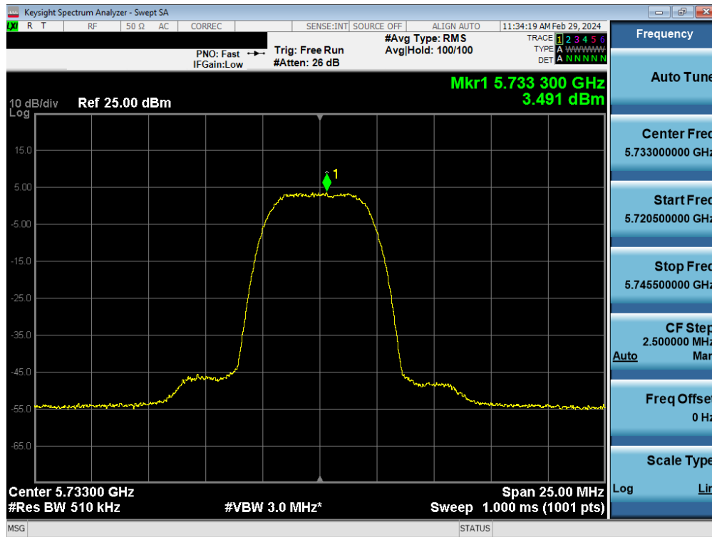
Plot 7-160. PSD TxBF Antenna WF5B (HDR8, ePA 5733MHz)
