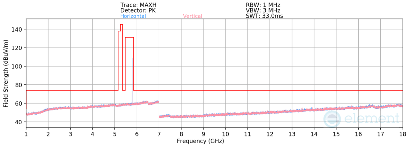
Plot 7-176. Radiated Spurious Emissions 1-18GHz Antenna WF5B (HDR4, ePA – 5789MHz)
