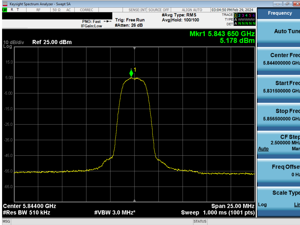
Plot 7-153. PSD TxBF Antenna 4a (HDR4, ePA 5844MHz)
