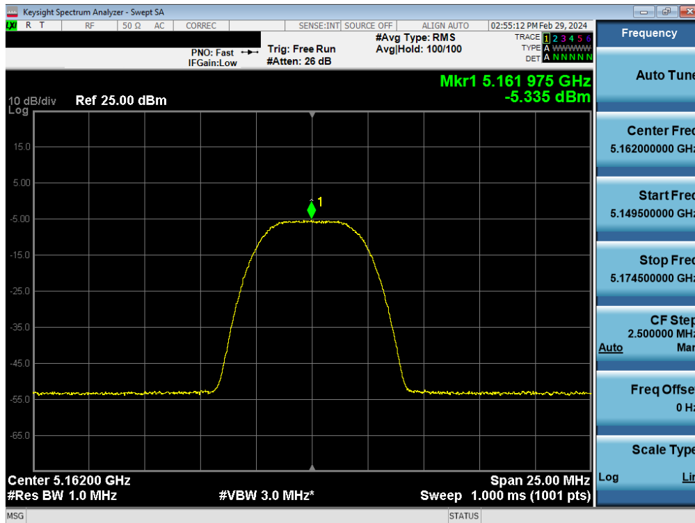
Plot 7-131. FCC/ISED PSD Tx BF Antenna 4a (HDR8, iPA – 5162MHz)
