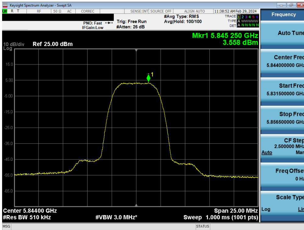
Plot 7-164. PSD TxBF Antenna WF5B (HDR8, ePA 5844MHz)
