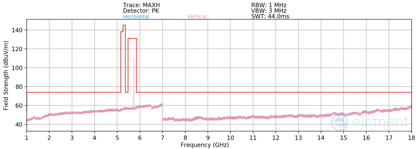
Plot 7-194. Radiated Spurious Emissions 1-18GHz TxBF (HDR4, ePA – 5733MHz)
