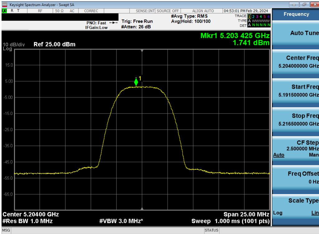
Plot 7-144. ISED PSD TxBF Antenna WF5B (HDR8, ePA – 5204MHz)
