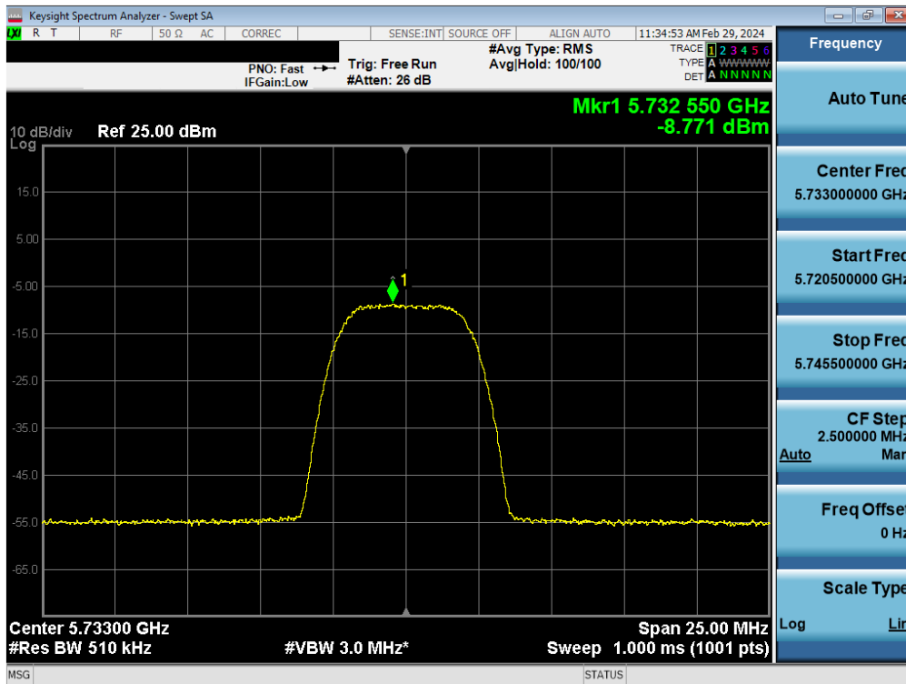
Plot 7-166. PSD TxBF Antenna WF5B (HDR8, iPA 5733MHz)
