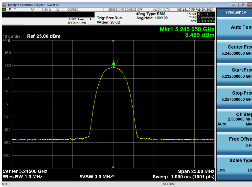
Plot 7-141. ISED PSD TxBF Antenna 4a (HDR4, ePA - 5245MHz)
