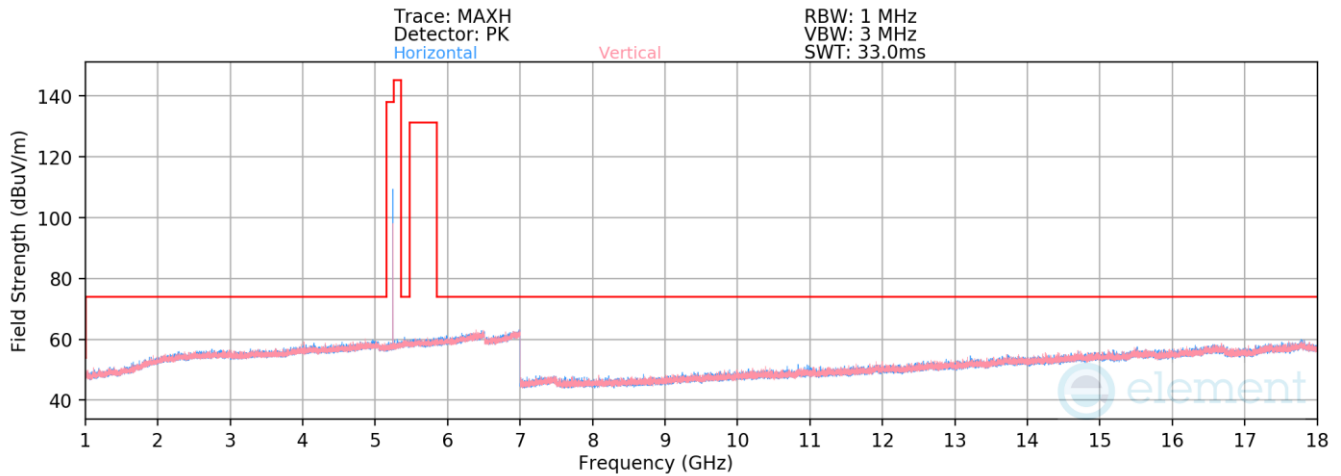
Plot 7-174. Radiated Spurious Emissions 1-18GHz Antenna WF5B (HDR4, ePA – 5245MHz)
