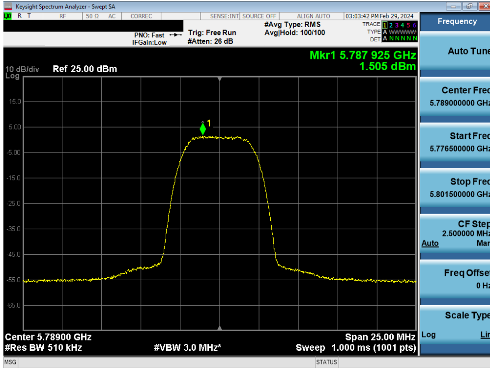
Plot 7-163. PSD TxBF Antenna 4a (HDR8, ePA 5789MHz)
