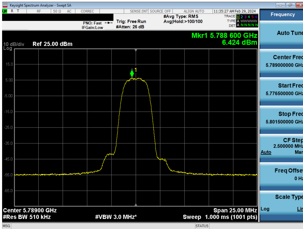
Plot 7-150. PSD TxBF Antenna WF5B (HDR4, ePA 5789MHz)
