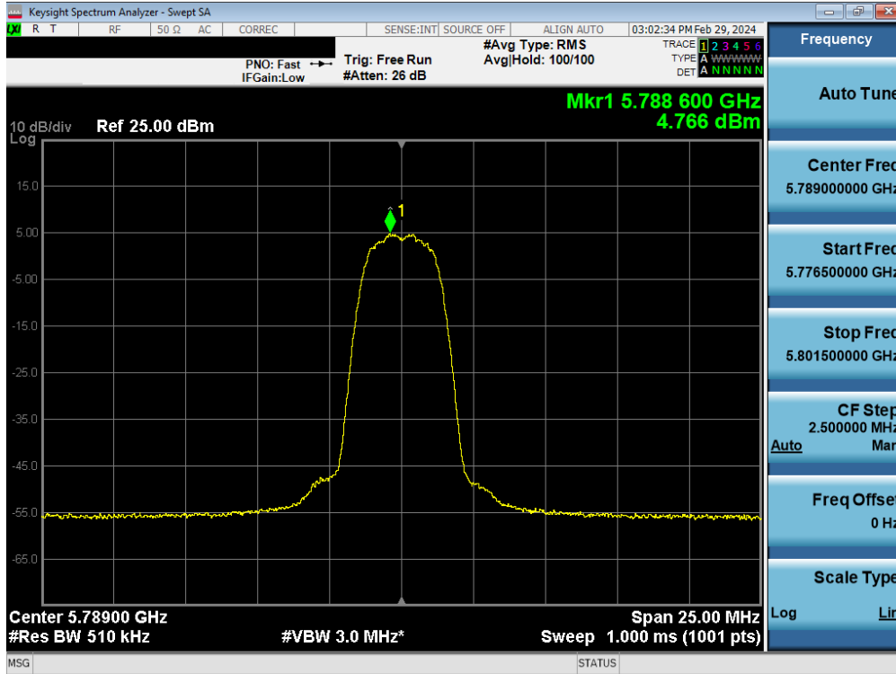
Plot 7-151. PSD TxBF Antenna 4a (HDR4, ePA 5789MHz)
