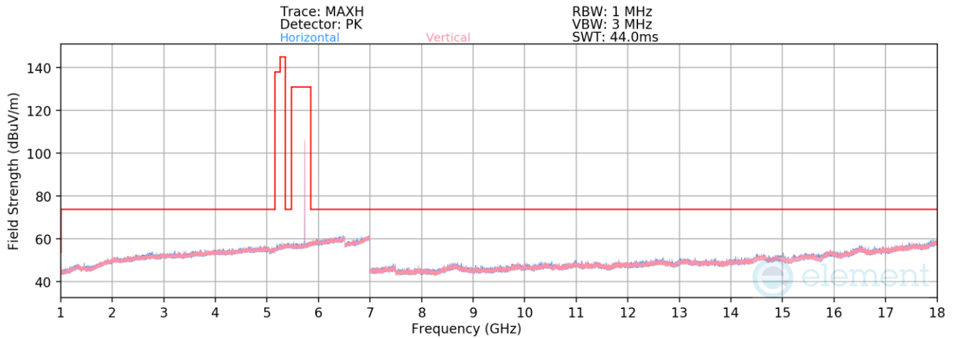
Plot 7-187. Radiated Spurious Emissions 1-18GHz Antenna 2a (HDR4, ePA – 5733MHz)
