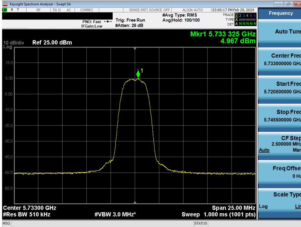
Plot 7-149. PSD TxBF Antenna 4a (HDR4, ePA 5733MHz)
