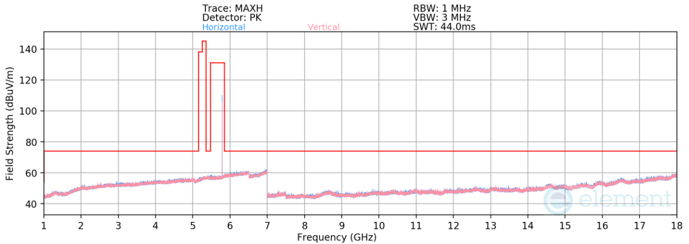
Plot 7-195. Radiated Spurious Emissions 1-18GHz TxBF (HDR4, ePA – 5789MHz)
