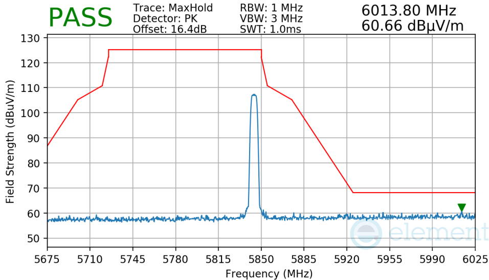
Plot 7-203. Radiated Upper Band Edge Measurement Antenna WF5B
