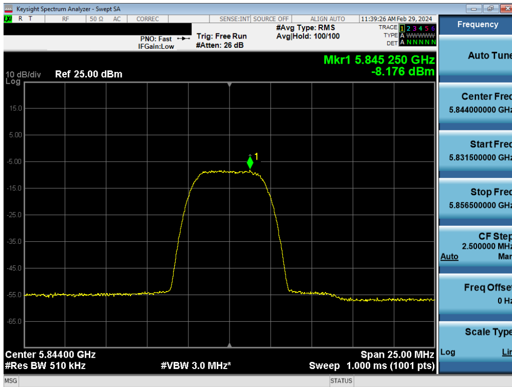
Plot 7-170. PSD TxBF Antenna WF5B (HDR8, iPA 5844MHz)
