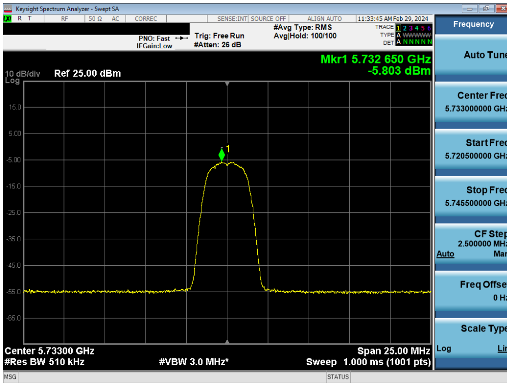
Plot 7-154. PSD TxBF Antenna WF5B (HDR4, iPA 5733MHz)
