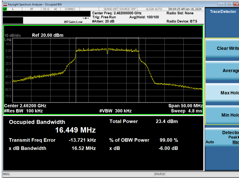
Plot 7-12. 6 dB BW and 99% OBW Plot Antenna 4a (802.11g - Ch. 11) - 24Mbps
