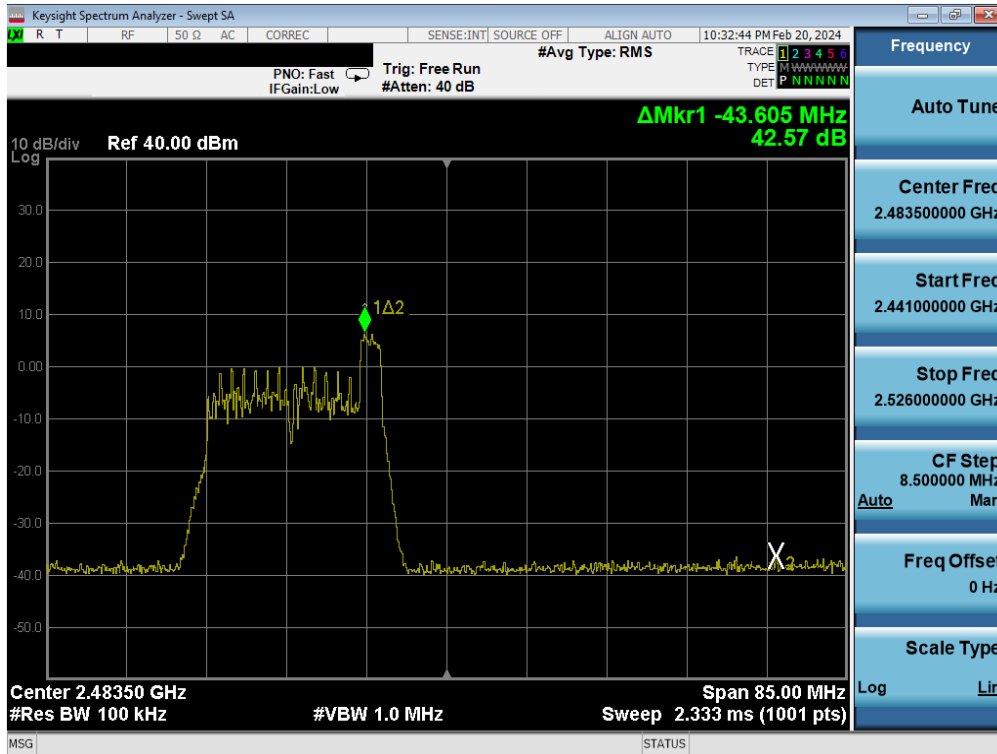
Plot 7-91. Band Edge Antenna 2a (802.11ax OFDMA – RU26 Index 8 – Ch. 12)
