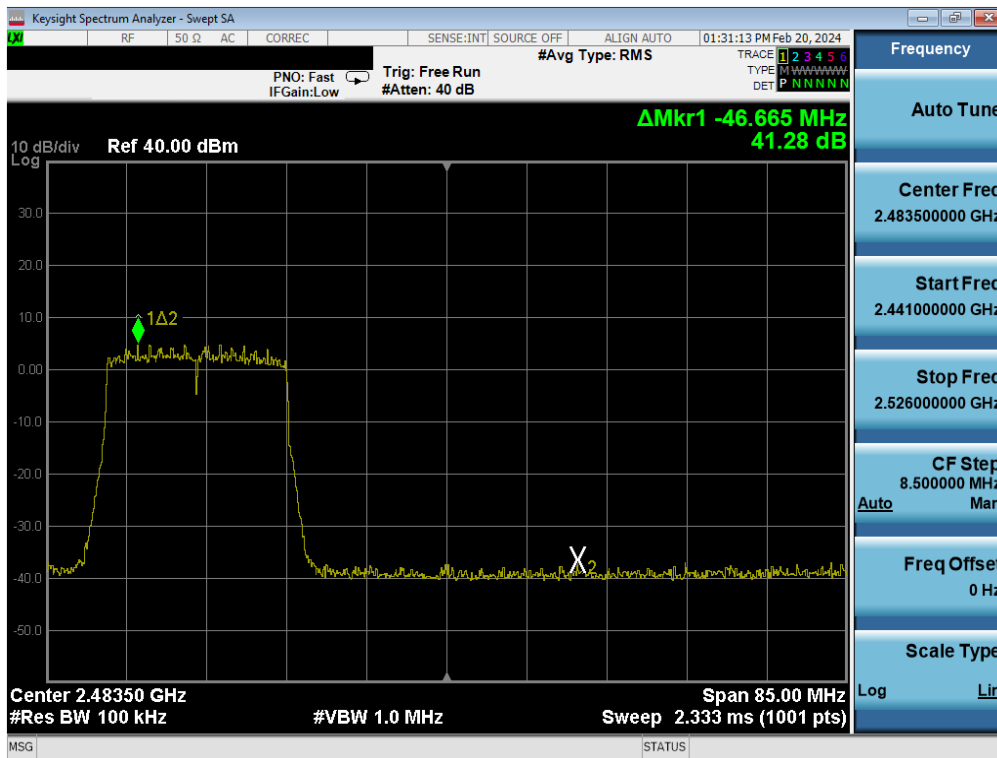
Plot 7-86. Band Edge Antenna 4a (802.11ax OFDMA – RU242 – Ch. 10)
