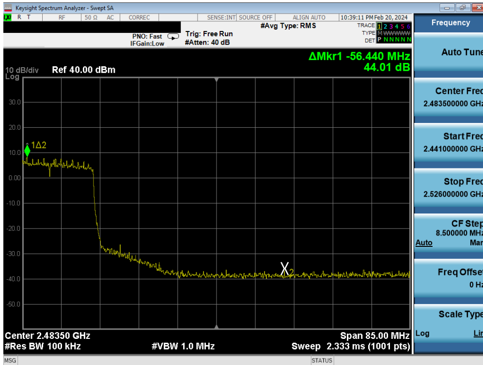
Plot 7-100. Band Edge Antenna 2a (802.11ax OFDMA – RU242 – Ch. 8)
