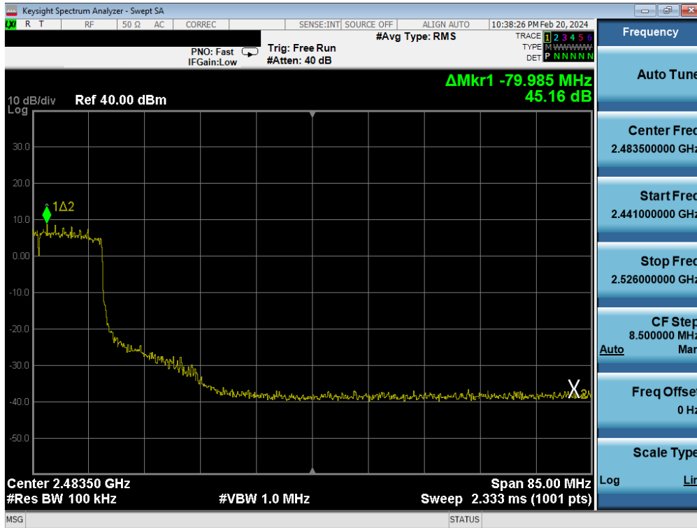
Plot 7-99. Band Edge Antenna 2a (802.11ax OFDMA – RU242 – Ch. 7)
