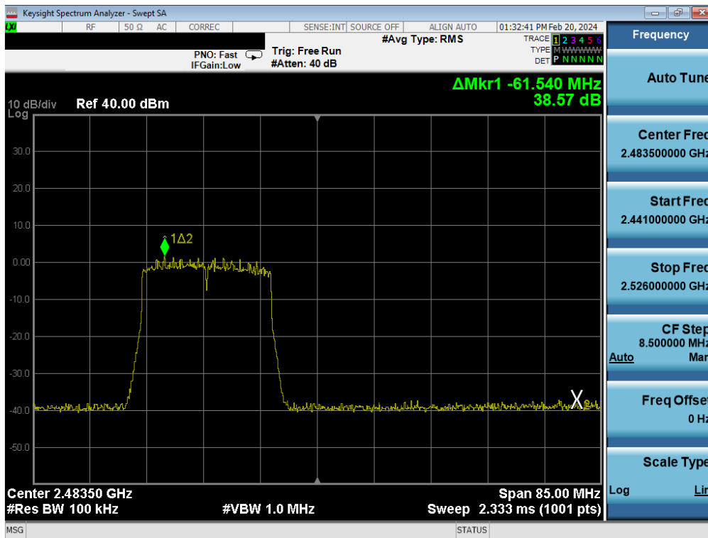
Plot 7-88. Band Edge Antenna 4a (802.11ax OFDMA – RU242 – Ch. 12)
