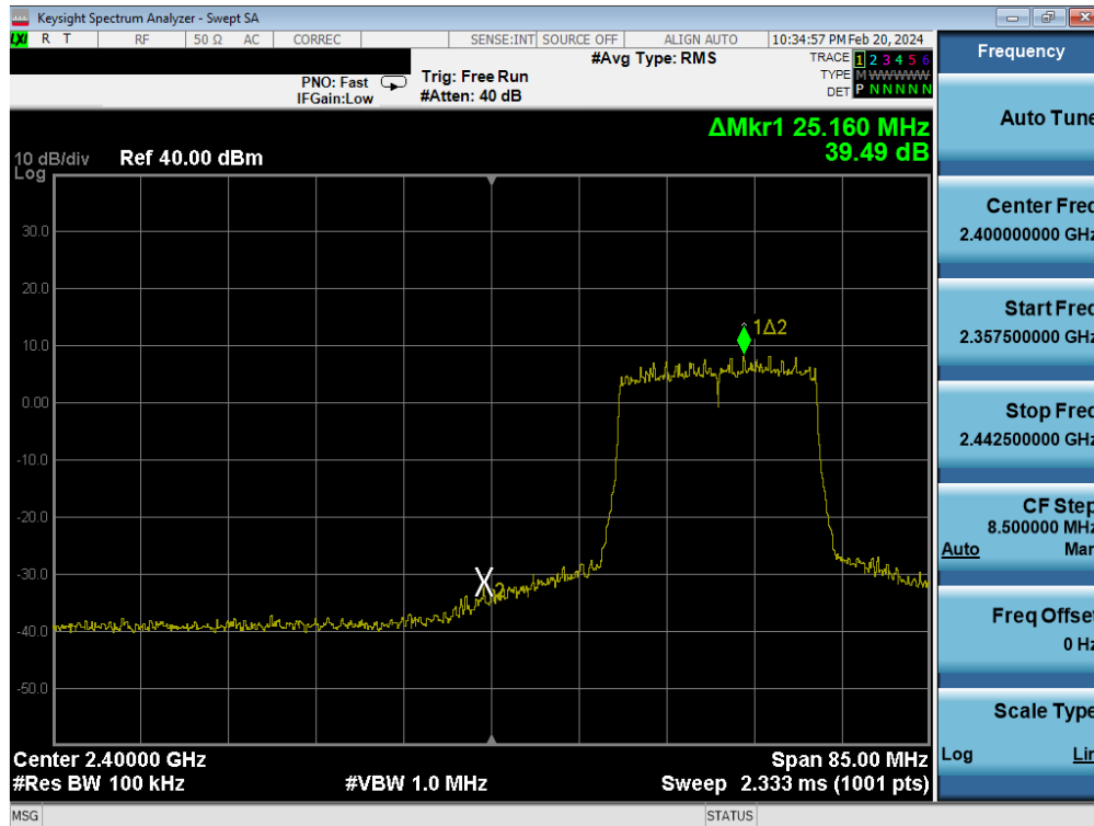
Plot 7-94. Band Edge Antenna 2a (802.11ax OFDMA – RU242 – Ch. 3)
