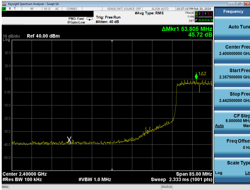
Plot 7-97. Band Edge Antenna 2a (802.11ax OFDMA – RU242 – Ch. 6(low))
