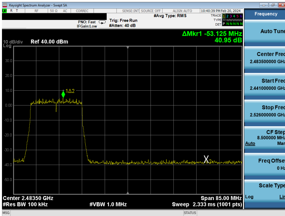
Plot 7-102. Band Edge Antenna 2a (802.11ax OFDMA – RU242 – Ch. 10)
