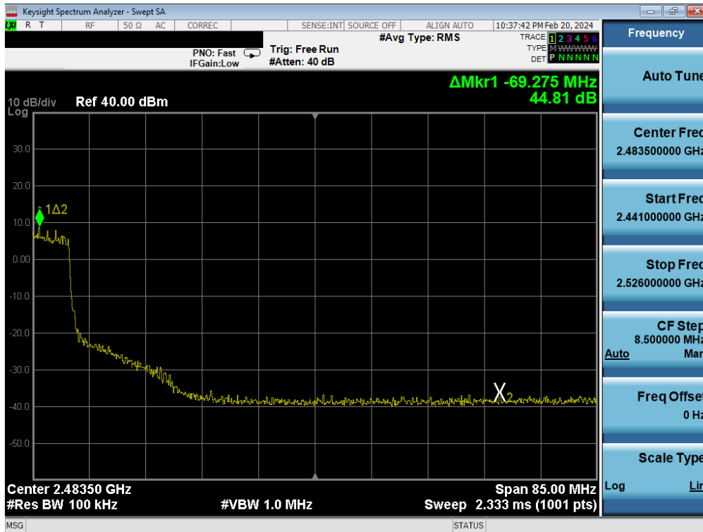
Plot 7-98. Band Edge Antenna 2a (802.11ax OFDMA – RU242 – Ch. 6(high))
