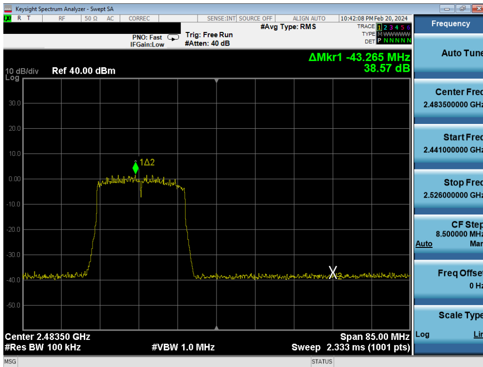
Plot 7-104. Band Edge Antenna 2a (802.11ax OFDMA – RU242 – Ch. 12)
