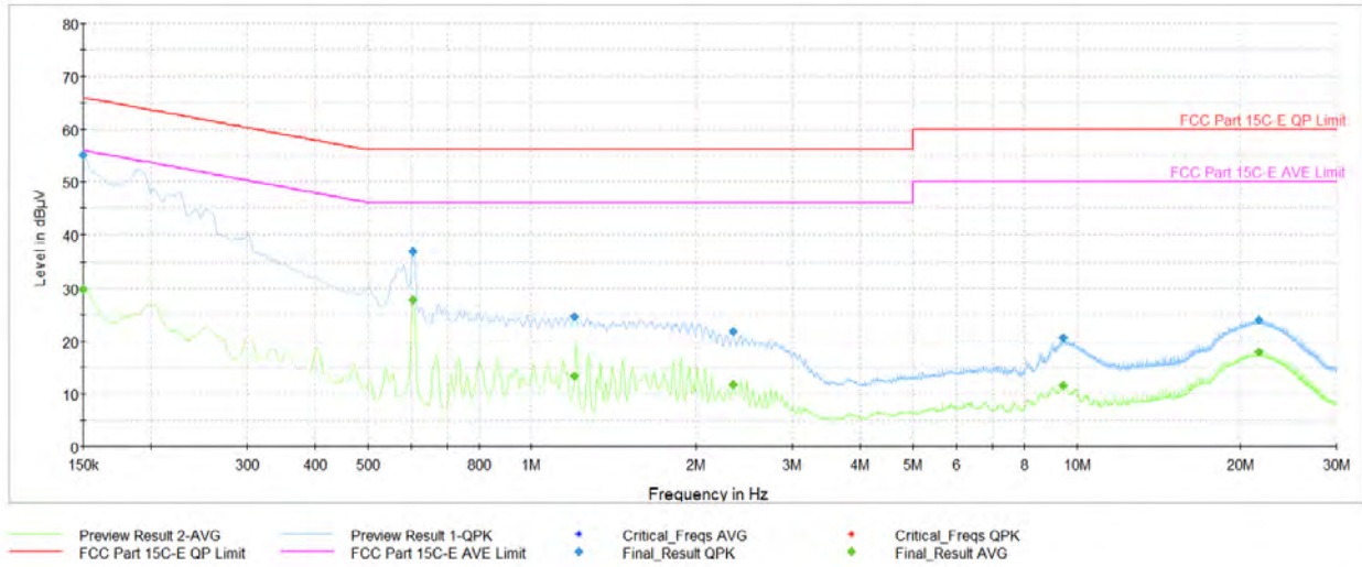
Plot 7-104. AC Line Conducted Plot with Bluetooth LE TxBF (L1, 1Mbps ePA – Ch.19 with Laptop)
