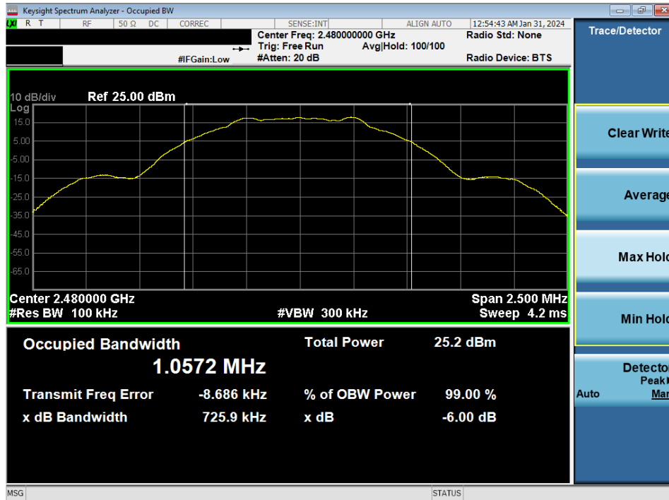
Plot 7-9. 6dB BW & 99% OBW Plot Antenna 2a (Bluetooth (LE), 1Mbps, ePA – Ch. 39)
