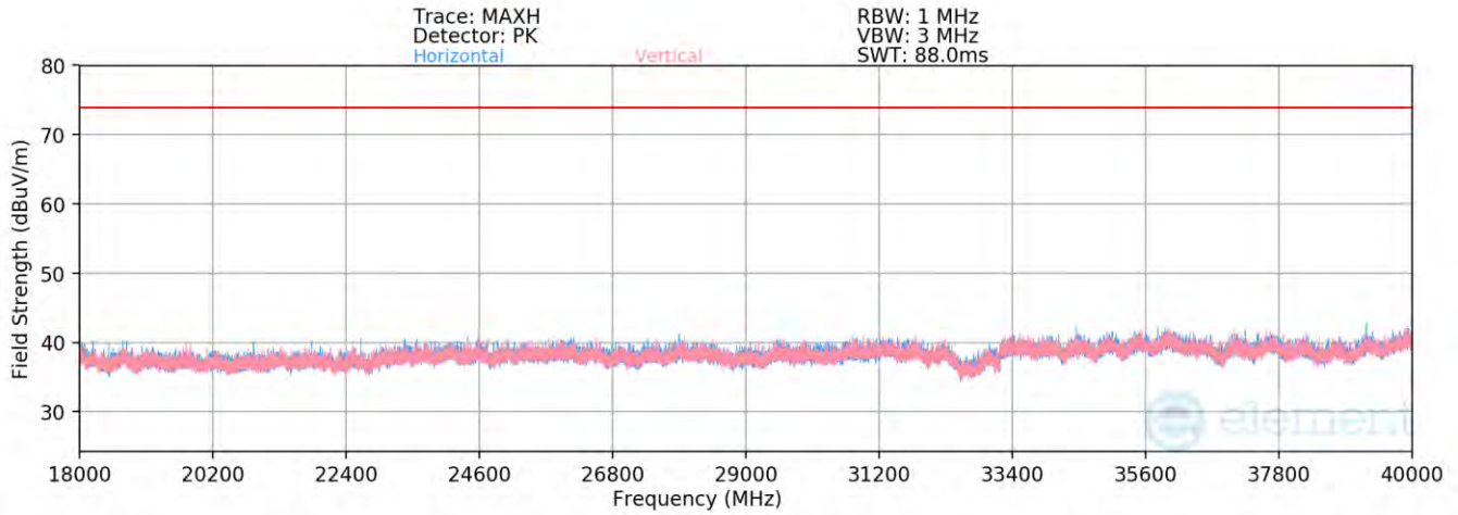
Plot 7-90. Radiated Spurious Emissions Above 18GHz TxBF (1Mbps, ePA – Ch. 39)
