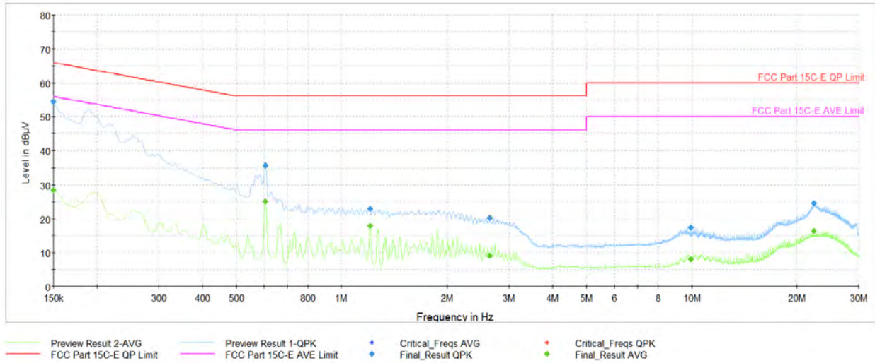
Plot 7-105. AC Line Conducted Plot with Bluetooth LE Tx BF (N, 1Mbps ePA – Ch.19, with Laptop)
