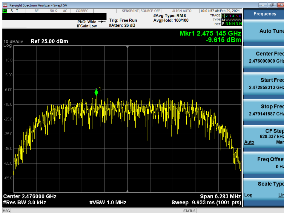
Plot 7-54. Power Spectral Density Plot TxBF Antenna 2a (Bluetooth (HDR), 8Mbps, ePA – Ch. 73)
