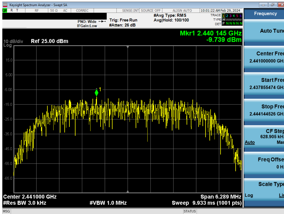
Plot 7-52. Power Spectral Density Plot TxBF Antenna 2a (Bluetooth (HDR), 8Mbps, ePA – Ch. 38)
