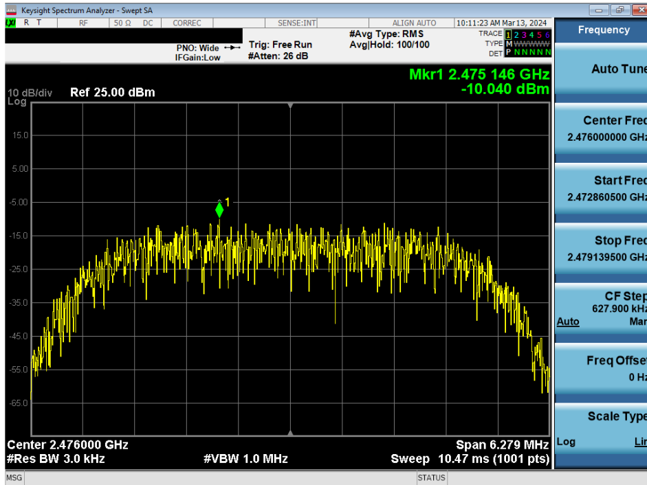
Plot 7-53. Power Spectral Density Plot TxBF Antenna 4a (Bluetooth (HDR), 8Mbps, ePA – Ch. 73)
