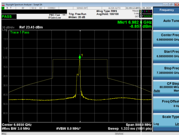
Plot 7-1531. LPI In-Band Emission Plot SDM Diversity Antenna 4a (160MHz 802.11ax RU26 (UNII Band 8) – Ch. 207)
