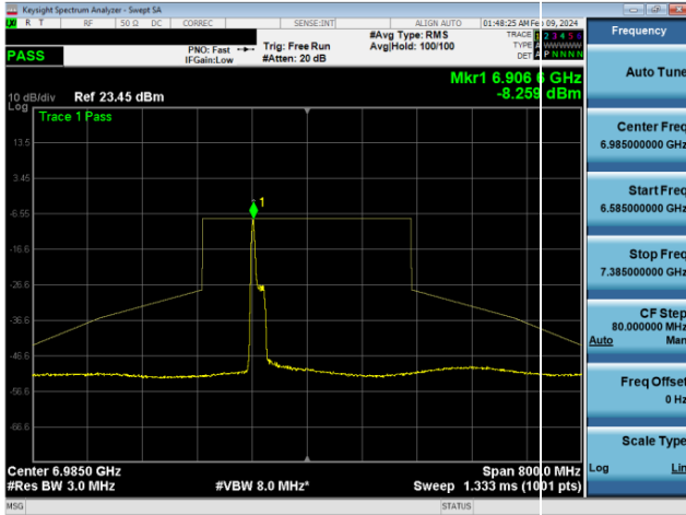
Plot 7-1529. LPI In-Band Emission Plot SDM Diversity Antenna 4a (160MHz 802.11ax RU26 (UNII Band 8) – Ch. 207)
