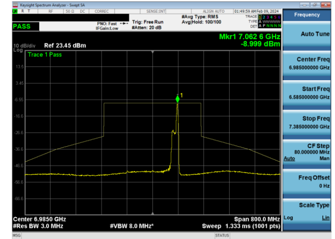
Plot 7-1533. LPI In-Band Emission Plot SDM Diversity Antenna 4a (160MHz 802.11ax RU26 (UNII Band 8) – Ch. 207)
