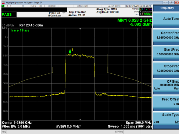
Plot 7-1535. LPI In-Band Emission Plot SDM Diversity Antenna 4a (160MHz 802.11ax RU996x2 (UNII Band 8) – Ch. 207)
