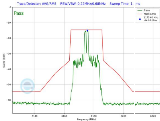
Plot 7-1283. LPI In-Band Emission Plot SDM Primary Antenna WF5B (20MHz 802.11ax RU26 (UNII Band 5) – Ch. 45)
