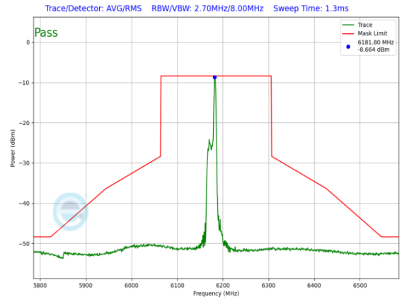
Plot 7-1308. LPI In-Band Emission Plot SDM Primary Antenna 4a (160MHz 802.11ax RU26 (UNII Band 5) – Ch. 47)
