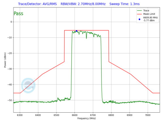
Plot 7-1376. LPI In-Band Emission Plot SDM Primary Antenna 4a (160MHz 802.11ax RU996x2 (UNII Band 7) – Ch. 143)
