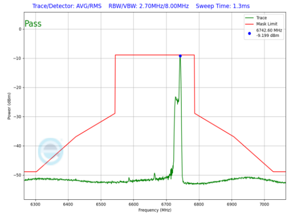
Plot 7-1374. LPI In-Band Emission Plot SDM Primary Antenna 4a (160MHz 802.11ax RU26 (UNII Band 7) – Ch. 143)
