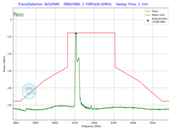
Plot 7-1306. LPI In-Band Emission Plot SDM Primary Antenna 4a (160MHz 802.11ax RU26 (UNII Band 5) – Ch. 47)
