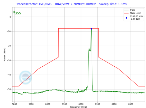
Plot 7-1310. LPI In-Band Emission Plot SDM Primary Antenna 4a (160MHz 802.11ax RU26 (UNII Band 5) – Ch. 47)
