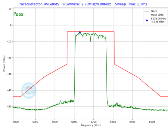
Plot 7-1312. LPI In-Band Emission Plot SDM Primary Antenna 4a (160MHz 802.11ax RU996x2 (UNII Band 5) – Ch. 47)
