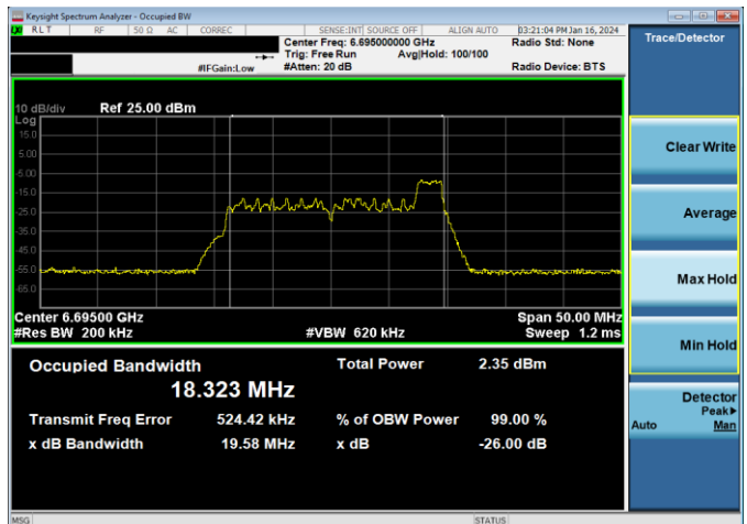
Plot 7-35. 26dB & 99% Bandwidth Plot Antenna WF5B (20MHz 802.11ax RU26 (UNII Band 7) – Ch. 149)
