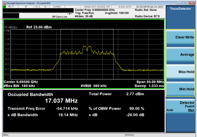
Plot 7-34. 26dB & 99% Bandwidth Plot Antenna WF5B (20MHz 802.11ax RU26 (UNII Band 7) – Ch. 149)
