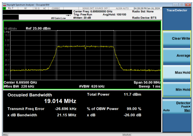
Plot 7-36. 26dB & 99% Bandwidth Plot Antenna WF5B (20MHz 802.11ax RU242 (UNII Band 7) – Ch. 149)
