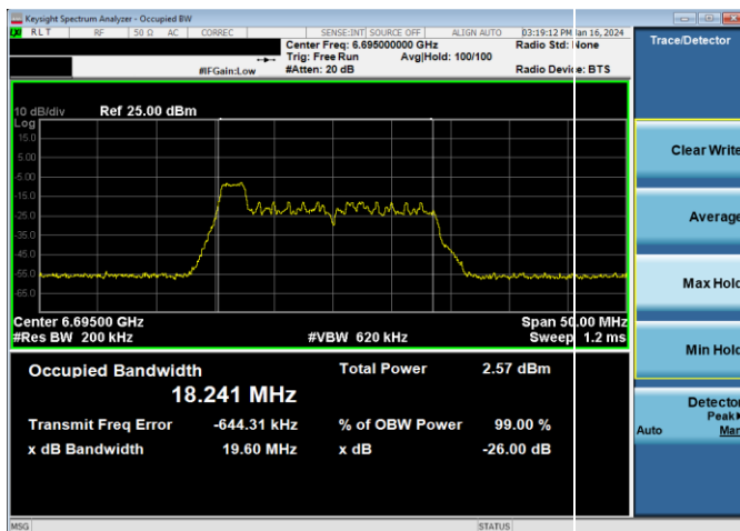
Plot 7-33. 26dB & 99% Bandwidth Plot Antenna WF5B (20MHz 802.11ax RU26 (UNII Band 7) – Ch. 149)
