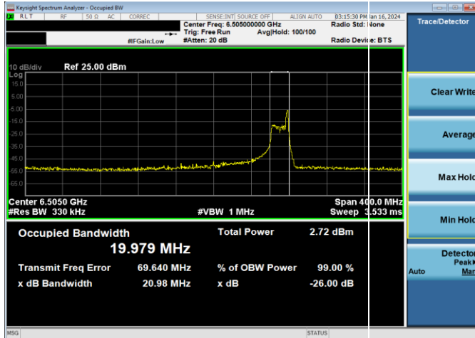
Plot 7-31. 26dB & 99% Bandwidth Plot Antenna WF5B (160MHz 802.11ax RU26 (UNII Band 6) – Ch. 111)
