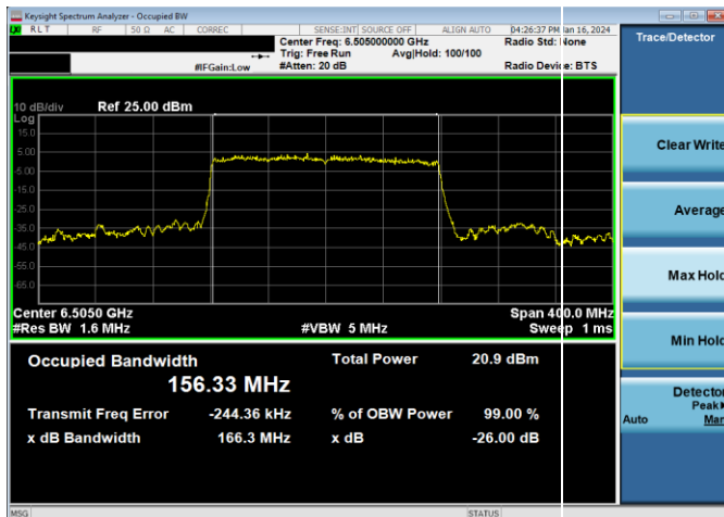
Plot 7-32. 26dB & 99% Bandwidth Plot Antenna WF5B (160MHz 802.11ax RU996x2 (UNII Band 6) – Ch. 111)
