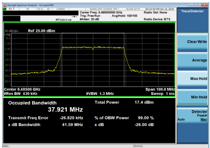
Plot 7-24. 26dB & 99% Bandwidth Plot Antenna WF5B (40MHz 802.11ax RU484 (UNII Band 6) – Ch. 107)
