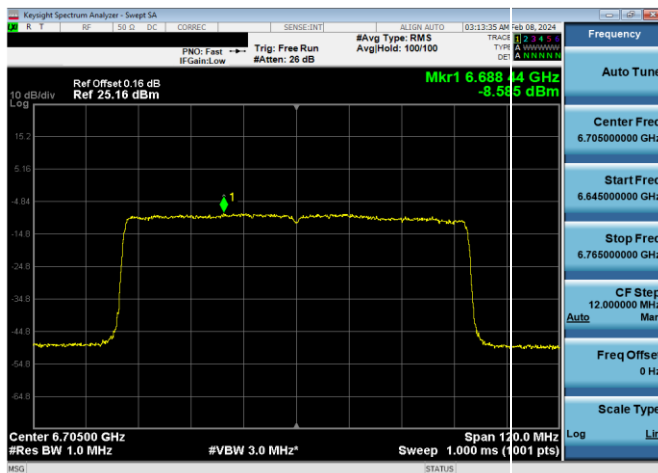
Plot 7-471. Power Spectral Density Plot SDM Primary Antenna WF5B LPI (80MHz 802.11ax (UNII Band 7) – Ch. 151, MCS2)
