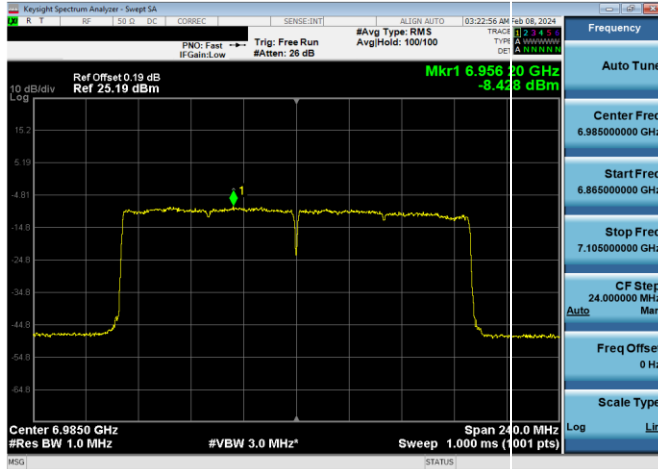
Plot 7-481. Power Spectral Density Plot SDM Primary Antenna WF5B LPI (160MHz 802.11ax (UNII Band 8) – Ch. 207, MCS2)
