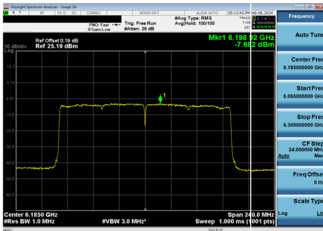
Plot 7-458. Power Spectral Density Plot SDM Primary Antenna 4a LPI (160MHz 802.11ax (UNII Band 5) – Ch. 47, MCS2)
