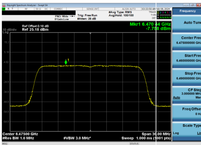
Plot 7-491. Power Spectral Density Plot SDM Primary Antenna WF5B LPI (20MHz 802.11ax (UNII Band 6) – Ch. 105, MCS4)
