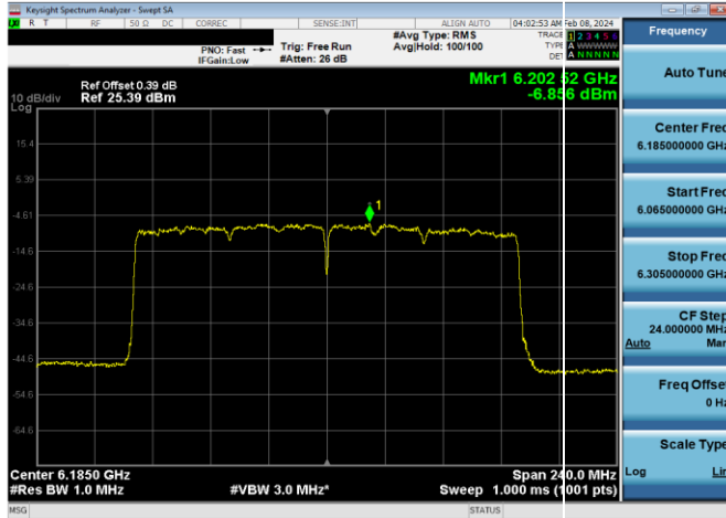
Plot 7-521. Power Spectral Density Plot SDM Primary Antenna WF5B LPI (160MHz 802.11ax (UNII Band 5) – Ch. 47, MCS11)
