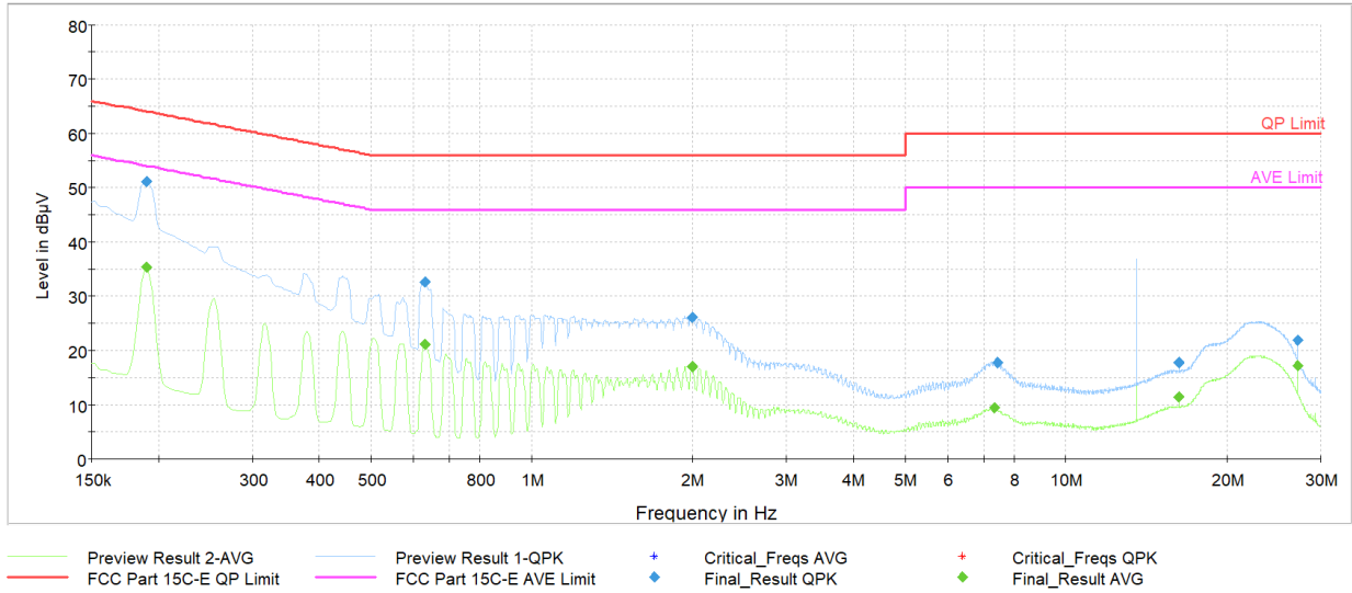
Plot 7-4. AC Line-Conducted Plot (L1, Charging Rate 2.6C, with Laptop)
