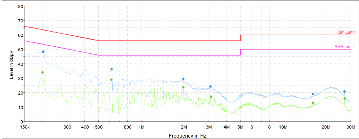
Plot 7-5. AC Line-Conducted Plot (N, Charging Rate 2.6C, with Laptop)
