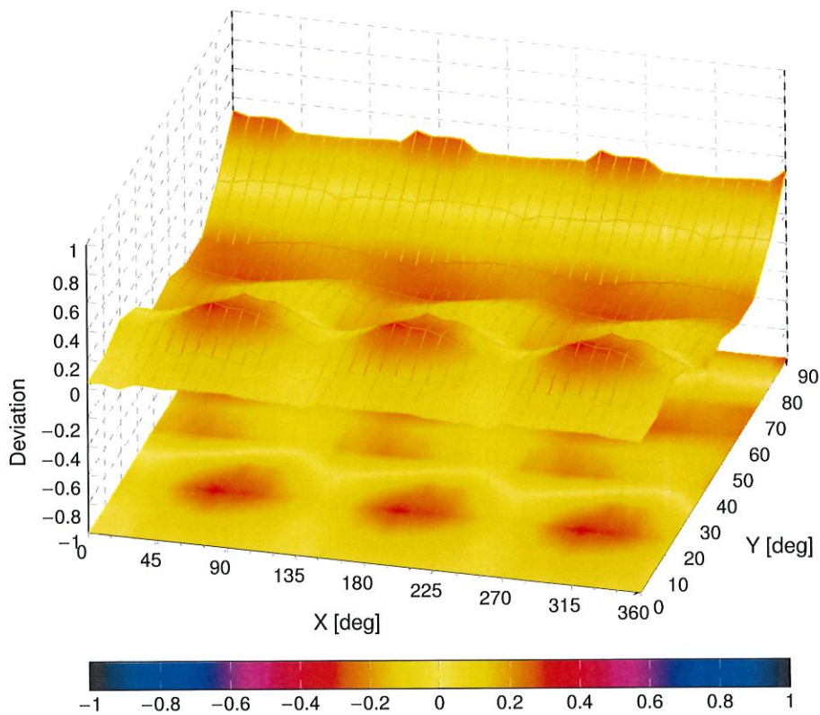
60GHz: 3D isotropy, E-field parallel to probe axis
