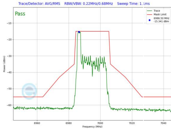
Plot 7-1506. LPI In-Band Emission Plot SDM Diversity Antenna WF7 (20MHz 802.11ax RU26 (UNII Band 8) – Ch. 209)
