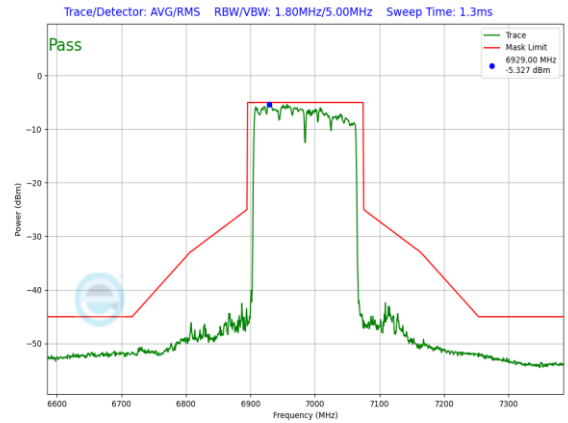
Plot 7-1536. LPI In-Band Emission Plot SDM Diversity Antenna WF7 (160MHz 802.11ax RU996x2 (UNII Band 8) – Ch. 207)
