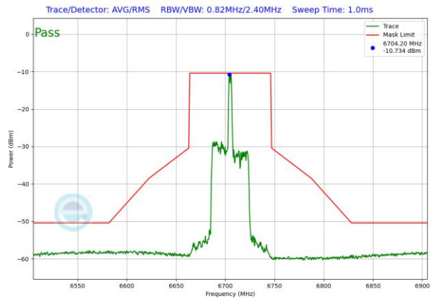
Plot 7-1491. LPI In-Band Emission Plot SDM Diversity Antenna WF8 (80MHz 802.11ax RU26 (UNII Band 7) – Ch. 151)
