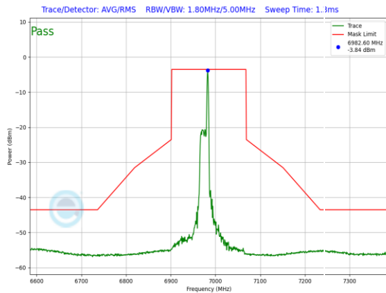
Plot 7-1214. LPI In-Band Emission Plot Antenna WF8 (160MHz 802.11ax RU26 (UNII Band 8) – Ch. 207)
