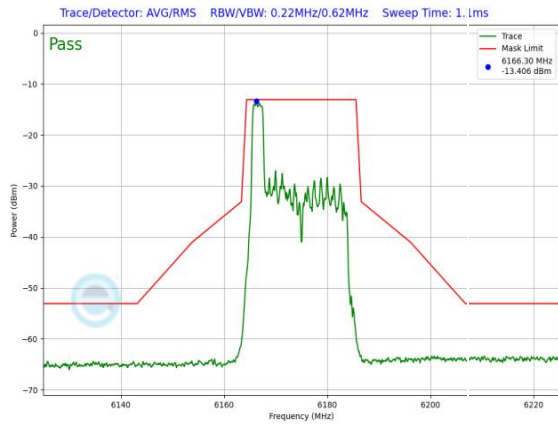
Plot 7-1282. LPI In-Band Emission Plot SDM Primary Antenna WF8 (20MHz 802.11ax RU26 (UNII Band 5) – Ch. 45)
