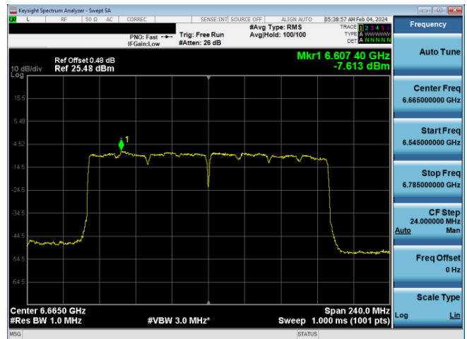
Plot 7-831. LPI Power Spectral Density Plot SDM Diversity Antenna WF8 (160MHz 802.11ax RU996x2 (UNII Band 7) – Ch. 143)
