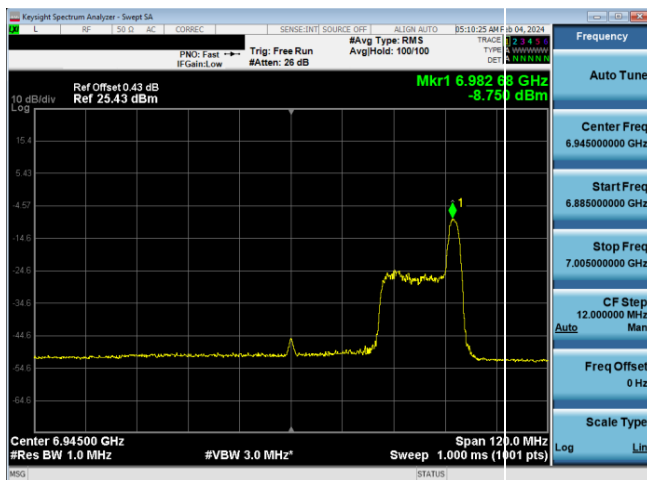
Plot 7-853. LPI Power Spectral Density Plot SDM Diversity Antenna WF8 (80MHz 802.11ax RU26 (UNII Band 8) – Ch. 199)
