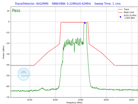
Plot 7-899. SP In-Band Emission Plot Antenna WF8 (20MHz 802.11ax RU26 (UNII Band 5) – Ch. 45)
