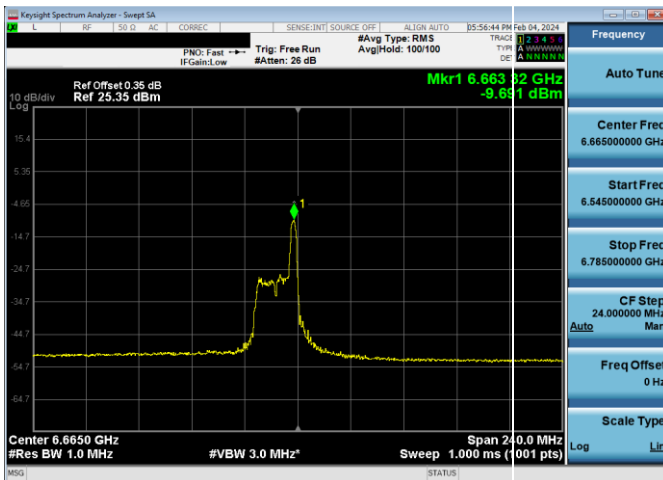
Plot 7-828. LPI Power Spectral Density Plot SDM Diversity Antenna WF7 (160MHz 802.11ax RU26 (UNII Band 7) – Ch. 143)
