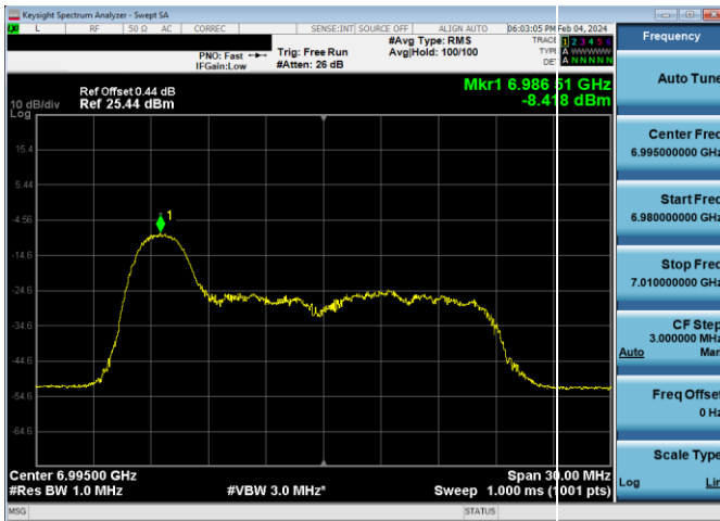
Plot 7-834. LPI Power Spectral Density Plot SDM Diversity Antenna WF7 (20MHz 802.11ax RU26 (UNII Band 8) – Ch. 209)
