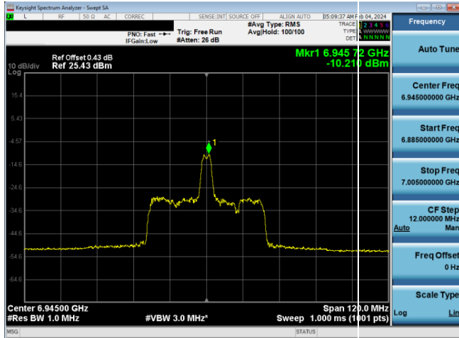
Plot 7-851. LPI Power Spectral Density Plot SDM Diversity Antenna WF8 (80MHz 802.11ax RU26 (UNII Band 8) – Ch. 199)
