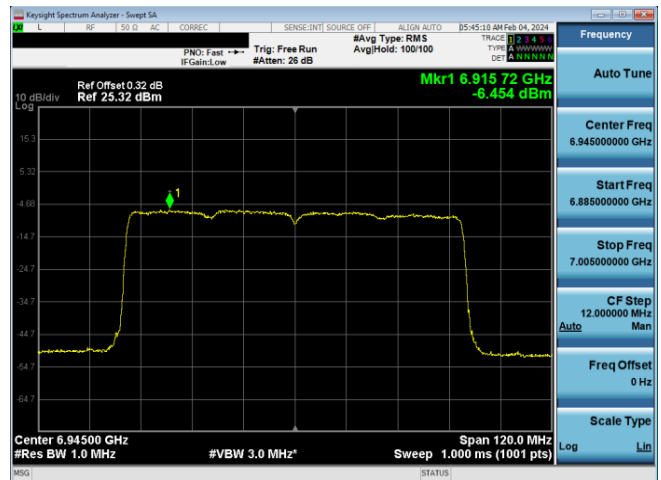
Plot 7-855. LPI Power Spectral Density Plot SDM Diversity Antenna WF8 (80MHz 802.11ax RU996 (UNII Band 8) – Ch. 199)
