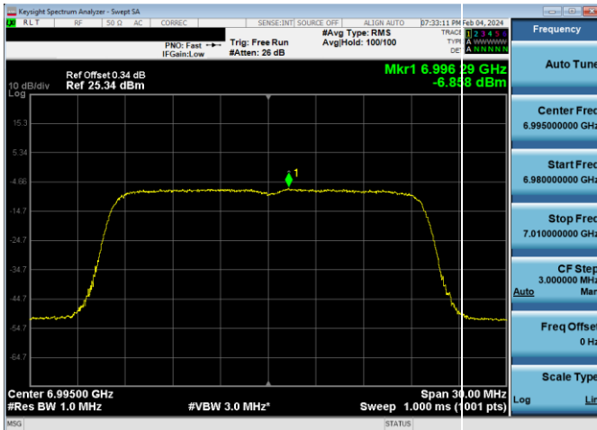
Plot 7-840. LPI Power Spectral Density Plot SDM Diversity Antenna WF7 (20MHz 802.11ax RU242 (UNII Band 8) – Ch. 209)
