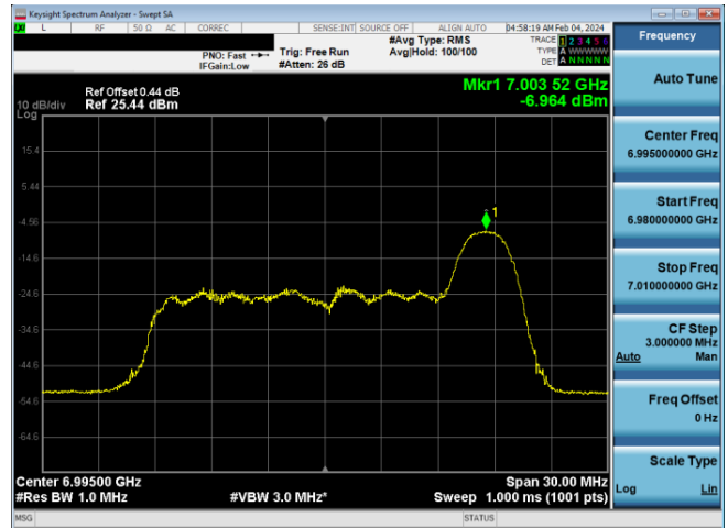
Plot 7-837. LPI Power Spectral Density Plot SDM Diversity Antenna WF8 (20MHz 802.11ax RU26 (UNII Band 8) – Ch. 209)
