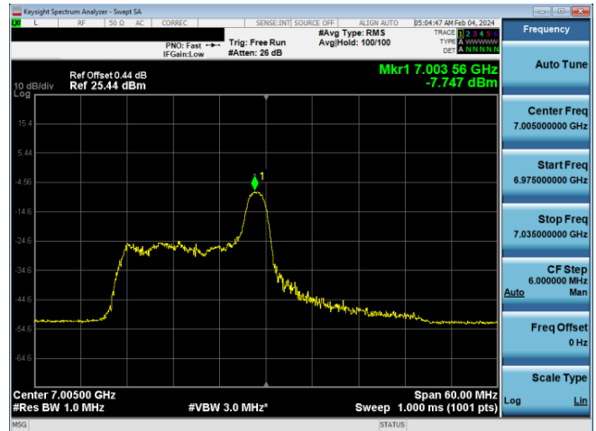
Plot 7-843. LPI Power Spectral Density Plot SDM Diversity Antenna WF8 (40MHz 802.11ax RU26 (UNII Band 8) – Ch. 211)
