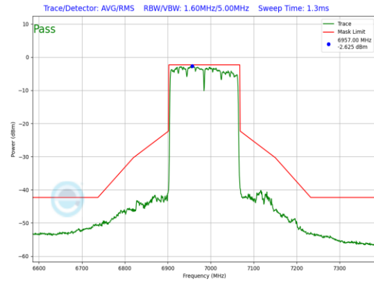
Plot 7-751. LPI In-Band Emission Plot Antenna WF5B (160MHz 802.11ax (UNII Band 8) – Ch. 207, MCS11)
