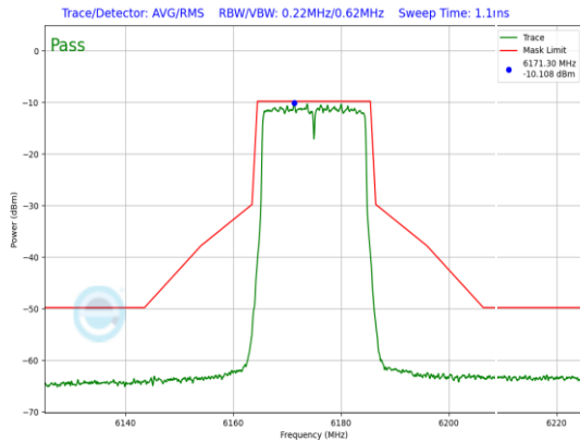
Plot 7-713. LPI In-Band Emission Plot Antenna WF5B (20MHz 802.11ax (UNII Band 5) – Ch. 45, MCS4)
