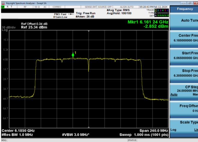
Plot 7-624. Power Spectral Density Plot SDM Diversity Antenna W7 Standard Power (160MHz 802.11ax (UNII Band 5) – Ch. 47, MCS4)
