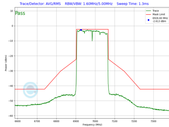
Plot 7-711. LPI In-Band Emission Plot Antenna WF5B (160MHz 802.11ax (UNII Band 8) – Ch. 207, MCS2)
