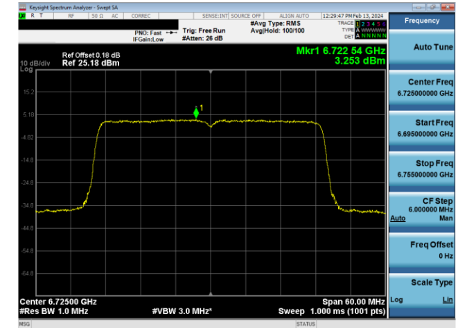
Plot 7-627. Power Spectral Density Plot SDM Diversity Antenna W8 Standard Power (40MHz 802.11ax (UNII Band 7) – Ch. 155, MCS4)
