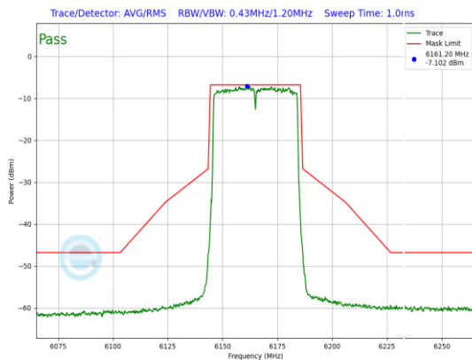
Plot 7-714. LPI In-Band Emission Plot Antenna WF5B (40MHz 802.11ax (UNII Band 5) – Ch. 43, MCS4)
