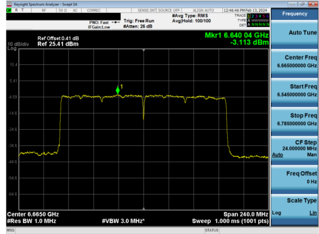
Plot 7-647. Power Spectral Density Plot SDM Diversity Antenna W8 Standard Power (160MHz 802.11ax (UNII Band 7) – Ch. 143, MCS11)
