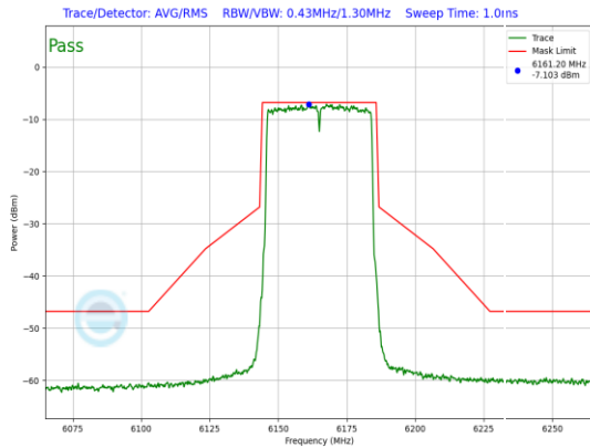
Plot 7-694. LPI In-Band Emission Plot Antenna WF5B (40MHz 802.11ax (UNII Band 5) – Ch. 43, MCS2)
