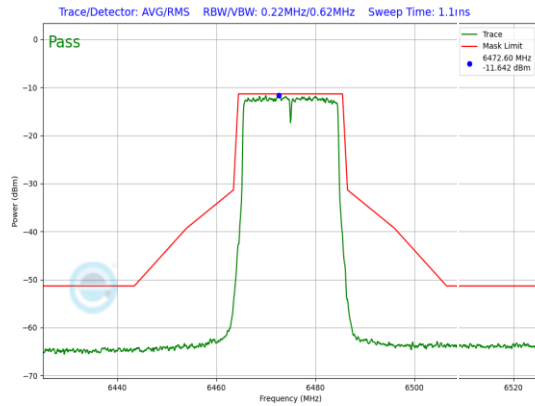
Plot 7-698. LPI In-Band Emission Plot Antenna WF5B (20MHz 802.11ax (UNII Band 6) – Ch. 105, MCS2)
