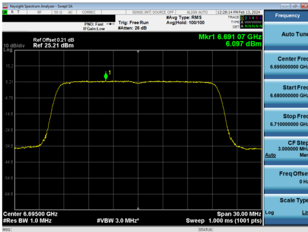
Plot 7-625. Power Spectral Density Plot SDM Diversity Antenna W7 Standard Power (20MHz 802.11ax (UNII Band 7) – Ch. 149, MCS4)
