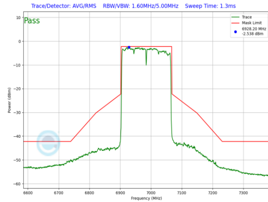
Plot 7-731. LPI In-Band Emission Plot Antenna WF5B (160MHz 802.11ax (UNII Band 8) – Ch. 207, MCS4)
