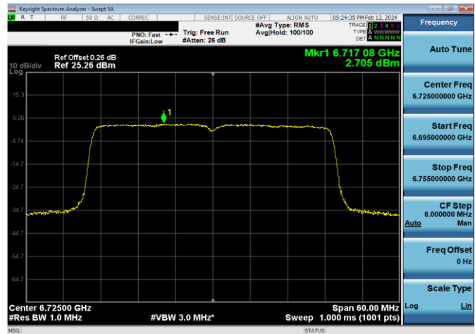
Plot 7-628. Power Spectral Density Plot SDM Diversity Antenna W7 Standard Power (40MHz 802.11ax (UNII Band 7) – Ch. 155, MCS4)
