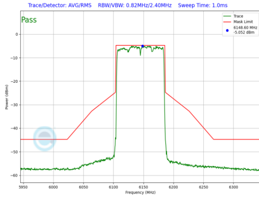
Plot 7-735. LPI In-Band Emission Plot Antenna WF5B (80MHz 802.11ax (UNII Band 5) – Ch. 39, MCS11)
