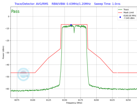
Plot 7-734. LPI In-Band Emission Plot Antenna WF5B (40MHz 802.11ax (UNII Band 5) – Ch. 43, MCS11)
