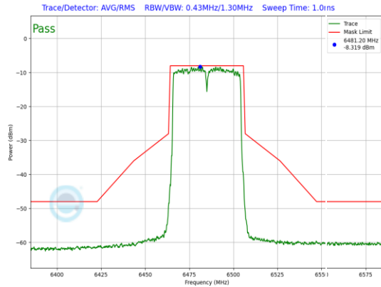
Plot 7-739. LPI In-Band Emission Plot Antenna WF5B (40MHz 802.11ax (UNII Band 6) – Ch. 107, MCS11)
