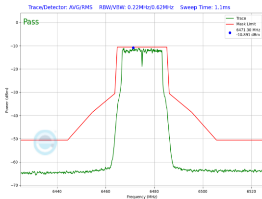
Plot 7-737. LPI In-Band Emission Plot Antenna WF5B (20MHz 802.11a (UNII Band 6) – Ch. 105, 54Mbps)
