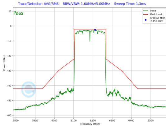
Plot 7-736. LPI In-Band Emission Plot Antenna WF5B (160MHz 802.11ax (UNII Band 5) – Ch. 47, MCS11)
