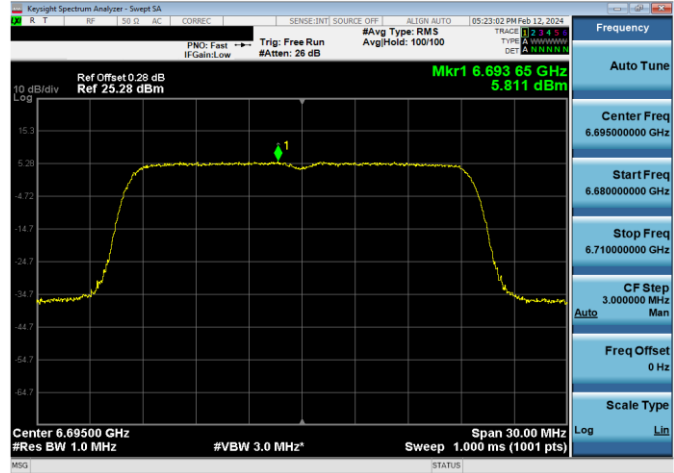
Plot 7-626. Power Spectral Density Plot SDM Diversity Antenna W7 Standard Power (20MHz 802.11ax (UNII Band 7) – Ch. 149, MCS4)
