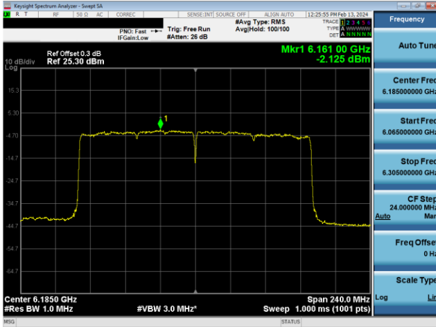
Plot 7-623. Power Spectral Density Plot SDM Diversity Antenna W8 Standard Power (160MHz 802.11ax (UNII Band 5) – Ch. 47, MCS4)
