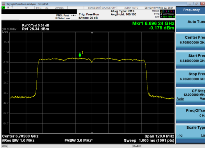
Plot 7-646. Power Spectral Density Plot SDM Diversity Antenna W7 Standard Power (80MHz 802.11ax (UNII Band 7) – Ch. 151, MCS11)
