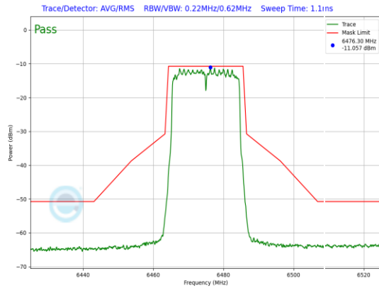
Plot 7-738. LPI In-Band Emission Plot Antenna WF5B (20MHz 802.11ax (UNII Band 6) – Ch. 105, MCS11)
