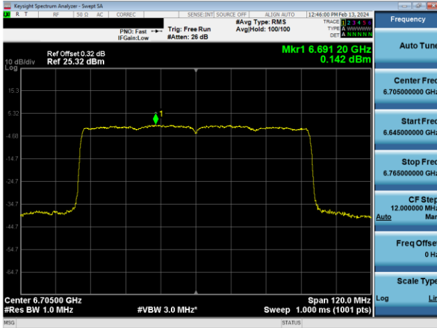
Plot 7-645. Power Spectral Density Plot SDM Diversity Antenna W8 Standard Power (80MHz 802.11ax (UNII Band 7) – Ch. 151, MCS11)
