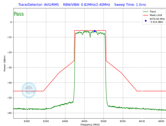
Plot 7-740. LPI In-Band Emission Plot Antenna WF5B (80MHz 802.11ax (UNII Band 6) – Ch. 103, MCS11)
