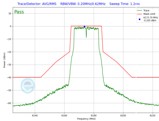
Plot 7-772. SP In-Band Emission Plot Antenna WF5B (20MHz 802.11a (UNII Band 5) – Ch. 45, 54Mbps)
