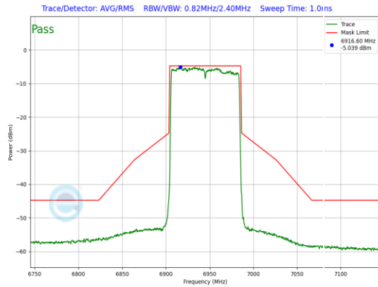
Plot 7-710. LPI In-Band Emission Plot Antenna WF5B (80MHz 802.11ax (UNII Band 8) – Ch. 199, MCS2)
