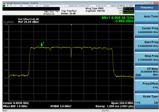
Plot 7-648. Power Spectral Density Plot SDM Diversity Antenna W7 Standard Power (160MHz 802.11ax (UNII Band 7) – Ch. 143, MCS11)
