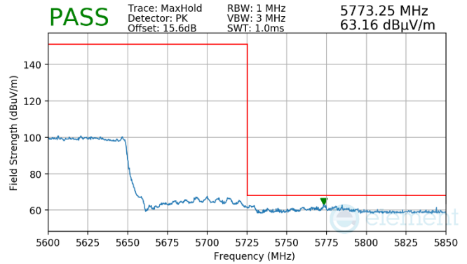
Plot 7-978. (FCC Only) Antenna WF7 (Pk, RU996x2, Index 68, Ch.114, MCS11)
