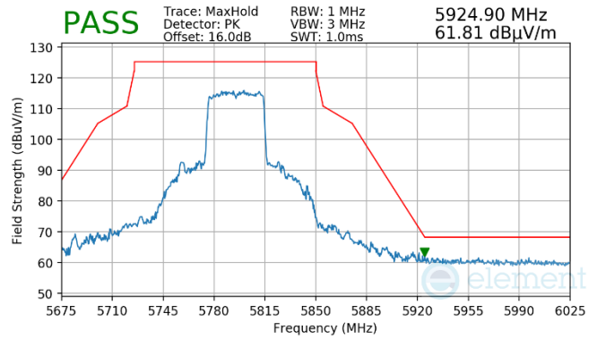
Plot 7-897. Antenna WF8 (Pk, RU484, Index 65, Ch.159, MCS11)
