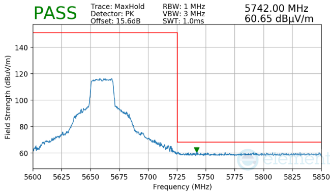
Plot 7-933. Antenna WF7 (Pk, RU242, Index 61, Ch.132, MCS11)
