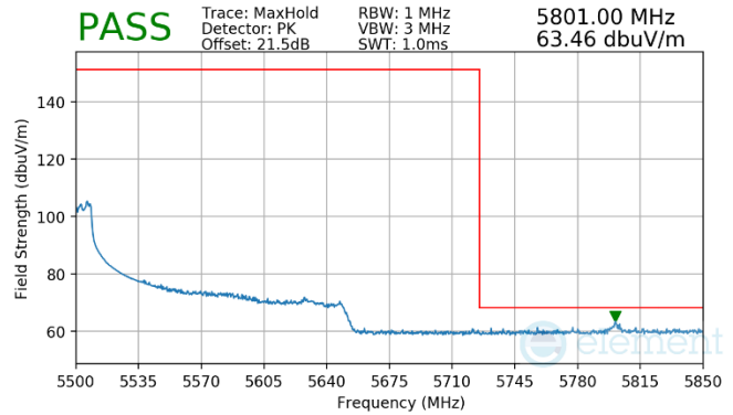
Plot 7-915. (FCC Only) Antenna WF8 (Pk, RU52, Index 37, Ch.114 (U), MCS11)
