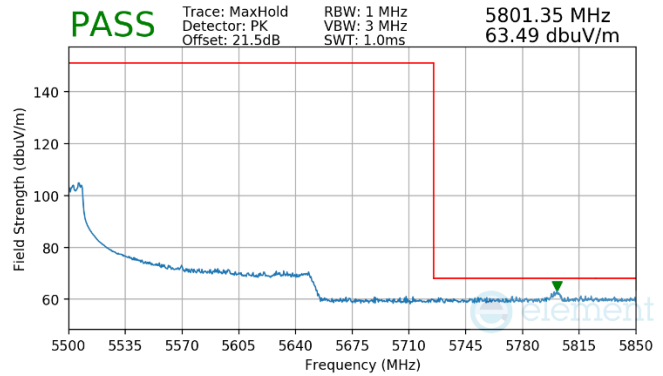
Plot 7-974. Antenna WF7 (Pk, RU52, Index 37, Ch.114 (U), MCS11) (FCC Only)
