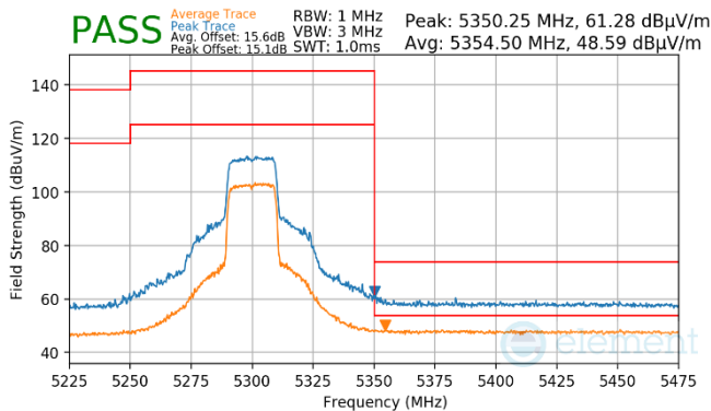
Plot 7-928. Antenna WF7 (Pk & Avg, RU242, Index 61, Ch.60, MCS11)
