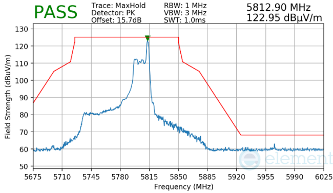
Plot 7-963. Antenna WF7 (Pk, RU26, Index 36, Ch.155, MCS11)
