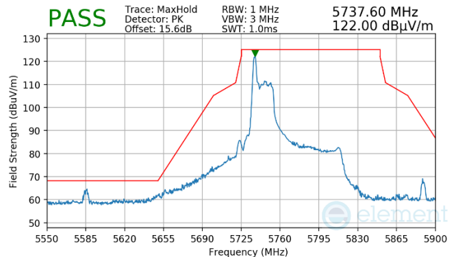
Plot 7-962. Antenna WF7 (Pk, RU26, Index 0, Ch.155, MCS11)
