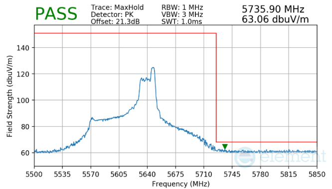
Plot 7-902. (FCC Only) Antenna WF8 (Pk, RU52, Index 52, Ch.122, MCS11)
