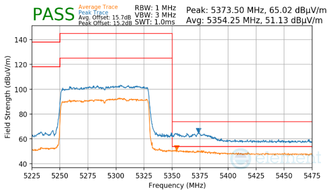
Plot 7-965. Antenna WF7 (Pk & Avg, RU996, Index 67, Ch.58, MCS11)
