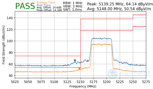
Plot 7-945. Antenna WF7 (Pk & Avg, RU484, Index 65, Ch.38, MCS11)
