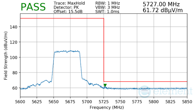
Plot 7-954. Antenna WF7 (Pk, RU484, Index 65, Ch.134, MCS11)
