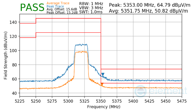
Plot 7-929. Antenna WF7 (Pk & Avg, RU242, Index 61, Ch.64, MCS11)
