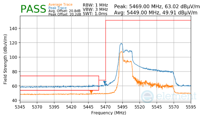
Plot 7-900. Antenna WF8 (Pk & Avg, RU52, Index 37, Ch.106, MCS11)
