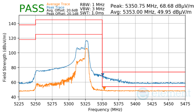
Plot 7-958. Antenna WF7 (Pk & Avg, RU52, Index 52, Ch.58, MCS11)
