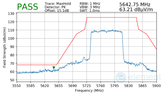
Plot 7-910. Antenna WF8 (Pk, RU996, Index 67, Ch.155, MCS11)
