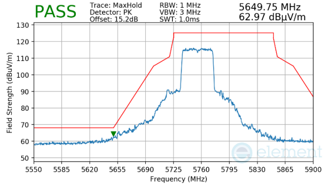
Plot 7-896. Antenna WF8 (Pk, RU484, Index 65, Ch.151, MCS11)
