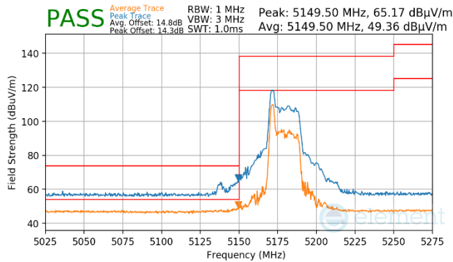
Plot 7-920. Antenna WF7 (Pk & Avg, RU26, Index 0, Ch.36, MCS11)
