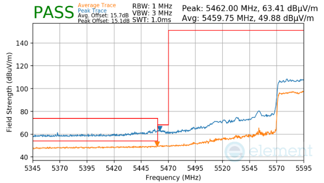
Plot 7-967. (FCC Only) Antenna WF7 (Pk & Avg, RU996, Index 67, Ch.122, MCS11)
