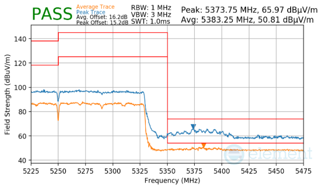
Plot 7-976. Antenna WF7 (Pk & Avg, RU996x2, Index 68, Ch.50, MCS11)
