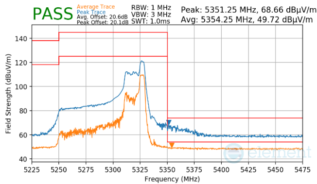
Plot 7-899. Antenna WF8 (Pk & Avg, RU52, Index 52, Ch.58, MCS11)
