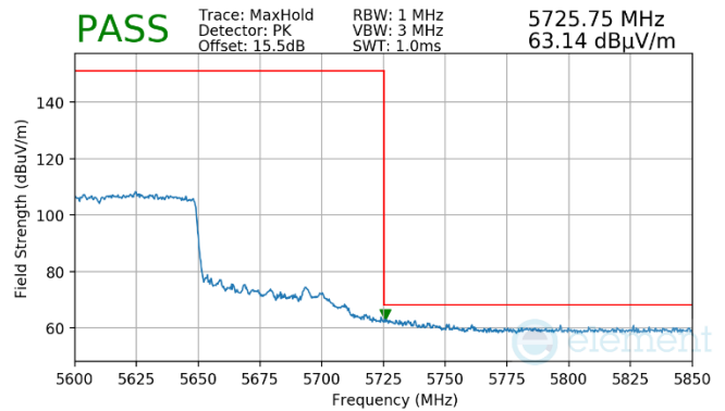
Plot 7-968. (FCC Only) Antenna WF7 (Pk, RU996, Index 67, Ch.122, MCS11)
