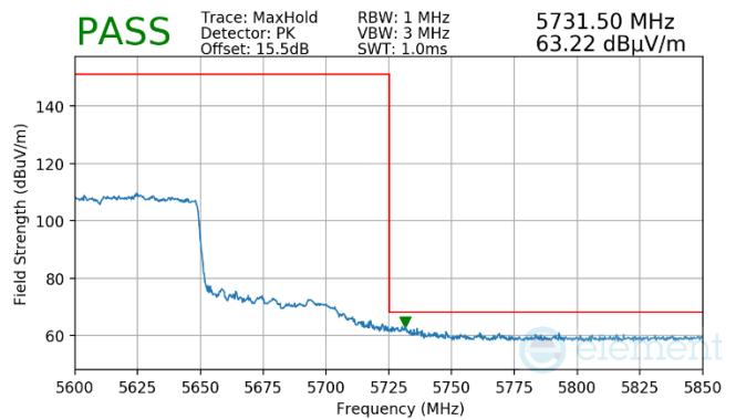
Plot 7-909. (FCC Only) Antenna WF8 (Pk, RU996, Index 67, Ch.122, MCS11)
