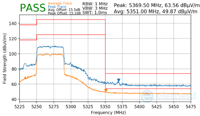
Plot 7-947. Antenna WF7 (Pk & Avg, RU484, Index 65, Ch.54, MCS11)
