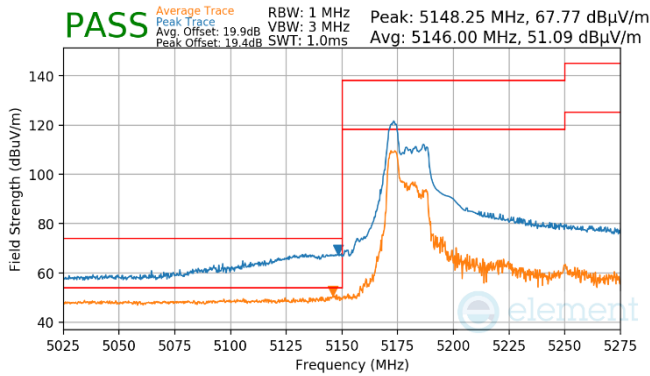
Plot 7-912. Antenna WF8 (Pk & Avg, RU52, Index 37, Ch.50 (L), MCS11)
