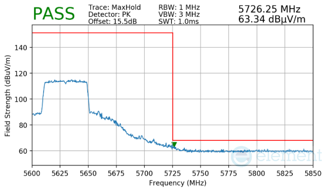
Plot 7-894. (FCC Only) Antenna WF8 (Pk, RU484, Index 65, Ch.126, MCS11)
