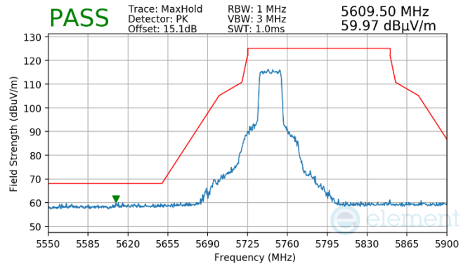
Plot 7-936. Antenna WF7 (Pk, RU242, Index 61, Ch.149, MCS11)
