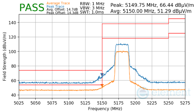
Plot 7-926. Antenna WF7 (Pk & Avg, RU242, Index 61, Ch.36, MCS11)
