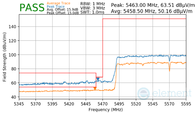
Plot 7-918. (FCC Only) Antenna WF8 (Pk & Avg, RU996x2, Index 68, Ch.114, MCS11)
