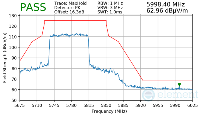
Plot 7-911. Antenna WF8 (Pk, RU996, Index 67, Ch.155, MCS11)
