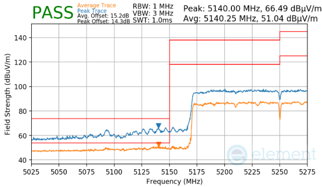
Plot 7-975. Antenna WF7 (Pk & Avg, RU996x2, Index 68, Ch.50, MCS11)
