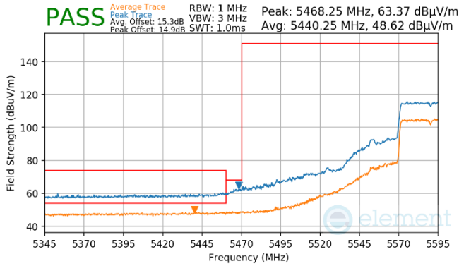
Plot 7-892. (FCC Only) Antenna WF8 (Pk & Avg, RU484, Index 65, Ch.118, MCS11)
