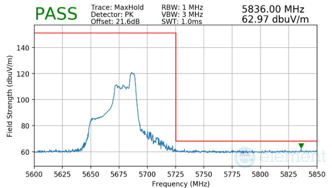
Plot 7-942. Antenna WF7 (Pk, RU52, Index 44, Ch.134, MCS11)
