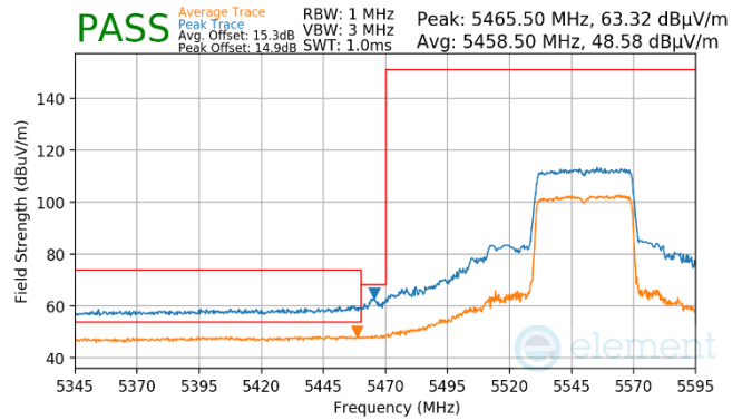
Plot 7-891. Antenna WF8 (Pk & Avg, RU484, Index 65, Ch.110, MCS11)
