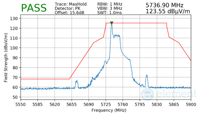
Plot 7-943. Antenna WF7 (Pk, RU26, Index 0, Ch.151, MCS11)
