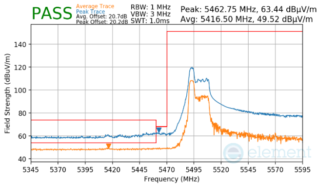
Plot 7-914. (FCC Only) Antenna WF8 (Pk & Avg, RU52, Index 37, Ch.114 (L), MCS11)
