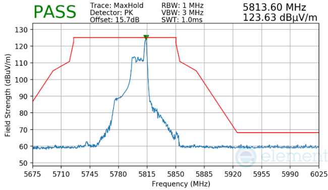
Plot 7-944. Antenna WF7 (Pk, RU26, Index 17, Ch.159, MCS11)
