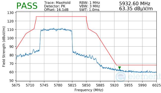
Plot 7-970. Antenna WF7 (Pk, RU996, Index 67, Ch.155, MCS11)
