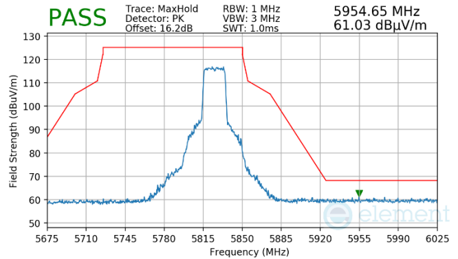
Plot 7-937. Antenna WF7 (Pk, RU242, Index 61, Ch.165, MCS11)
