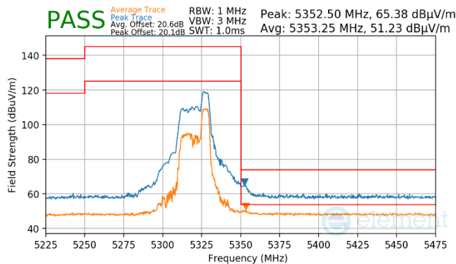
Plot 7-921. Antenna WF7 (Pk & Avg, RU52, Index 40, Ch.64, MCS11)
