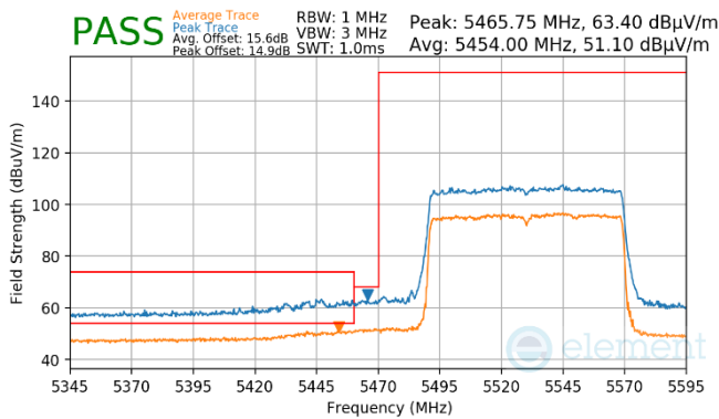
Plot 7-907. Antenna WF8 (Pk & Avg, RU996, Index 67, Ch.106, MCS11)
