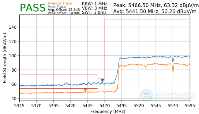
Plot 7-977. (FCC Only) Antenna WF7 (Pk & Avg, RU996x2, Index 68, Ch.114, MCS11)
