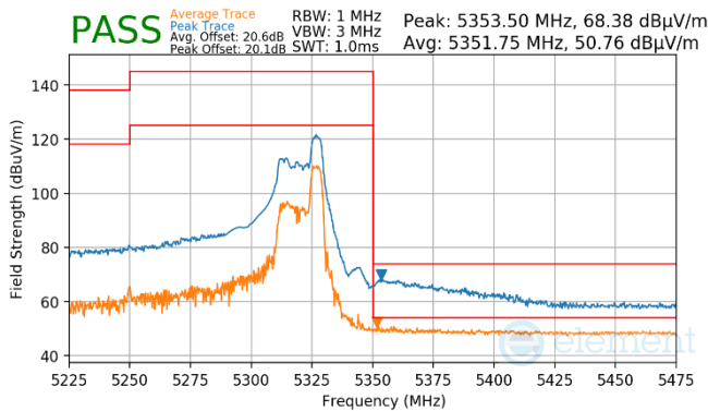
Plot 7-913. Antenna WF8 (Pk & Avg, RU52, Index 52, Ch.50 (U), MCS11)
