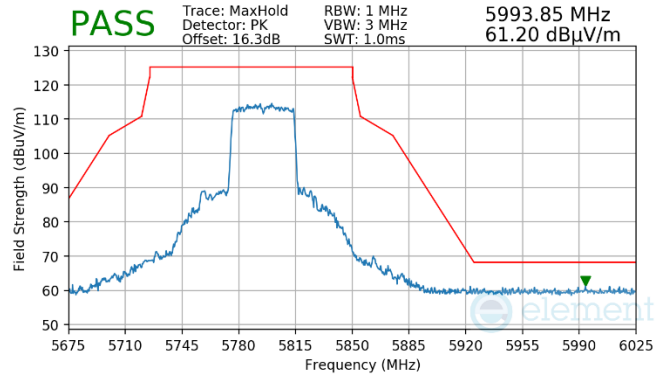
Plot 7-956. Antenna WF7 (Pk, RU484, Index 65, Ch.159, MCS11)
