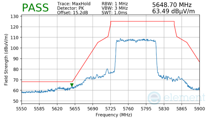
Plot 7-969. Antenna WF7 (Pk, RU996, Index 67, Ch.155, MCS11)
