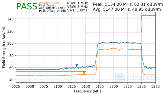
Plot 7-964. Antenna WF7 (Pk & Avg, RU996, Index 67, Ch.42, MCS11)
