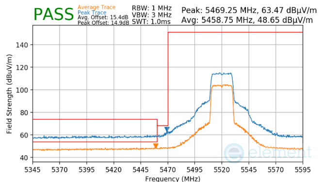
Plot 7-931. Antenna WF7 (Pk & Avg, RU242, Index 61, Ch.104, MCS11)
