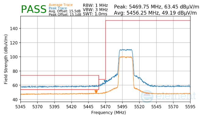
Plot 7-930. Antenna WF7 (Pk & Avg, RU242, Index 61, Ch.100, MCS11)
