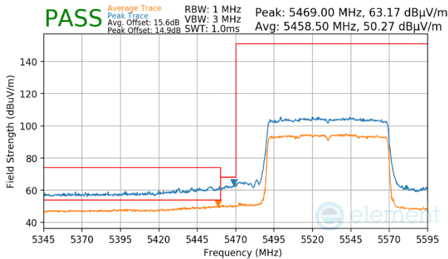
Plot 7-966. Antenna WF7 (Pk & Avg, RU996, Index 67, Ch.106, MCS11)
