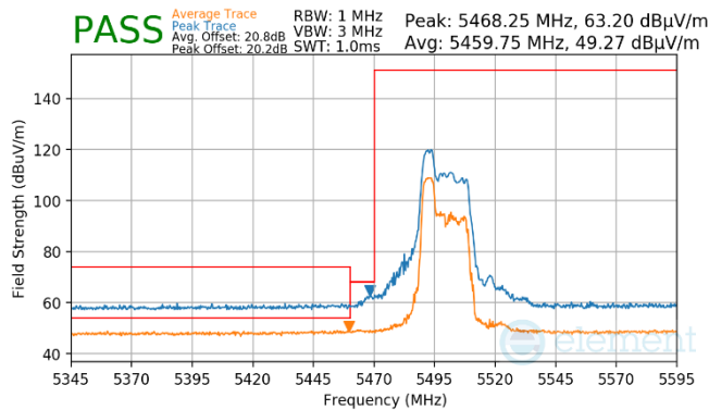
Plot 7-922. Antenna WF7 (Pk & Avg, RU52, Index 37, Ch.100, MCS11)
