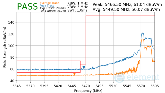
Plot 7-960. (FCC Only) Antenna WF7 (Pk & Avg, RU52, Index 37, Ch.122, MCS11)
