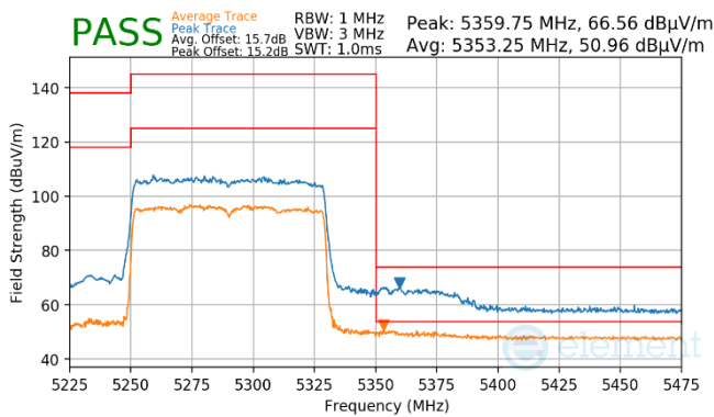
Plot 7-906. Antenna WF8 (Pk & Avg, RU996, Index 67, Ch.58, MCS11)
