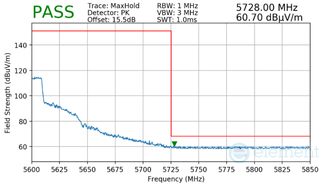
Plot 7-893. (FCC Only) Antenna WF8 (Pk, RU484, Index 65, Ch.118, MCS11)
