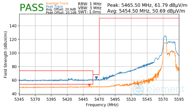
Plot 7-901. (FCC Only) Antenna WF8 (Pk & Avg, RU52, Index 37, Ch.122, MCS11)
