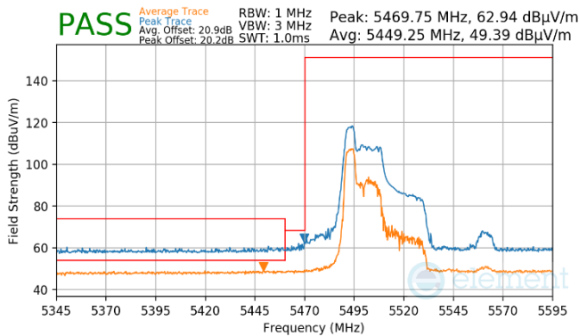
Plot 7-940. Antenna WF7 (Pk & Avg, RU52, Index 37, Ch.102, MCS11)
