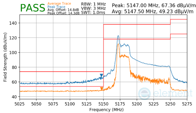
Plot 7-898. Antenna WF8 (Pk & Avg, RU26, Index 0, Ch.42, MCS11)
