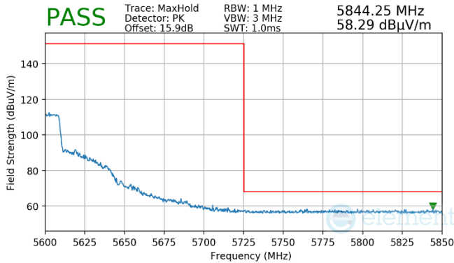
Plot 7-952. (FCC Only) Antenna WF7 (Pk, RU484, Index 65, Ch.118, MCS11)
