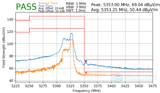
Plot 7-972. Antenna WF7 (Pk & Avg, RU52, Index 52, Ch.50 (U), MCS11)
