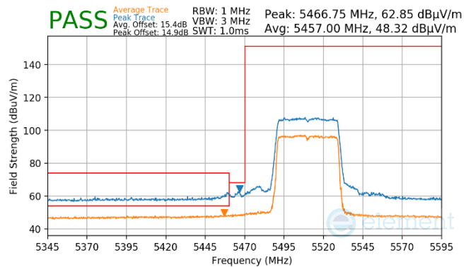
Plot 7-949. Antenna WF7 (Pk & Avg, RU484, Index 65, Ch.102, MCS11)
