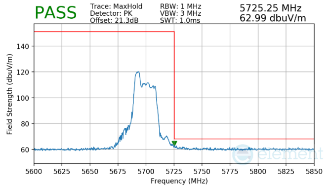
Plot 7-923. Antenna WF7 (Pk, RU52, Index 37, Ch.140, MCS11)
