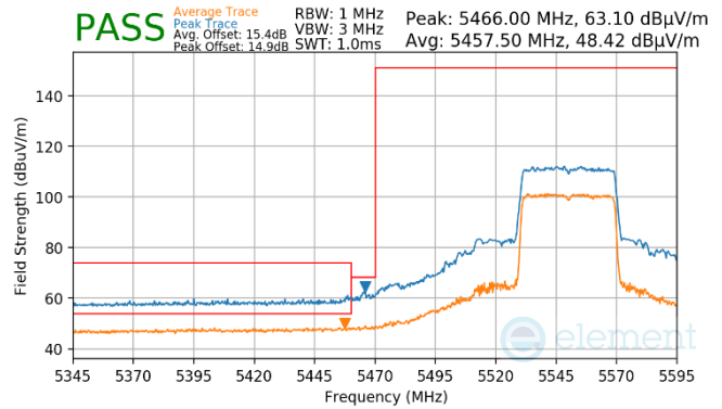
Plot 7-950. Antenna WF7 (Pk & Avg, RU484, Index 65, Ch.110, MCS11)
