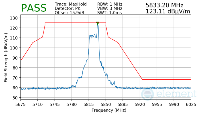
Plot 7-925. Antenna WF7 (Pk, RU26, Index 8, Ch.165, MCS11)
