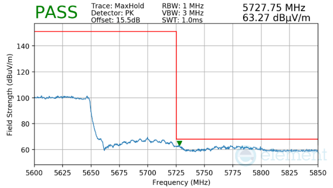
Plot 7-919. (FCC Only) Antenna WF8 (Pk, RU996x2, Index 68, Ch.114, MCS11)
