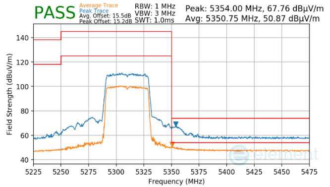
Plot 7-889. Antenna WF8 (Pk & Avg, RU484, Index 65, Ch.62, MCS11)
