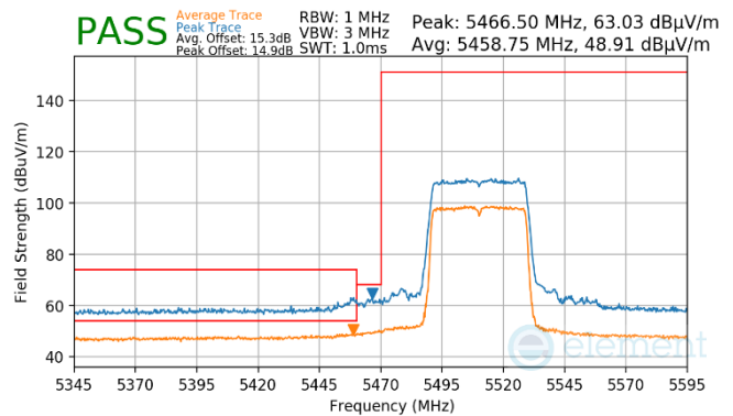
Plot 7-890. Antenna WF8 (Pk & Avg, RU484, Index 65, Ch.102, MCS11)
