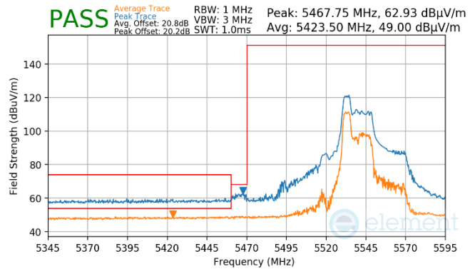
Plot 7-941. Antenna WF7 (Pk & Avg, RU52, Index 37, Ch.110, MCS11)
