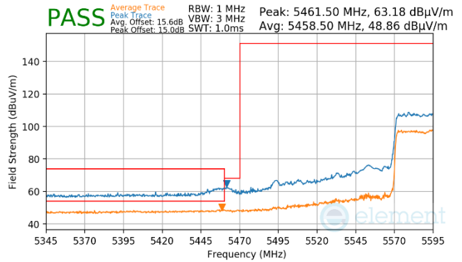
Plot 7-908. (FCC Only) Antenna WF8 (Pk & Avg, RU996, Index 67, Ch.122, MCS11)
