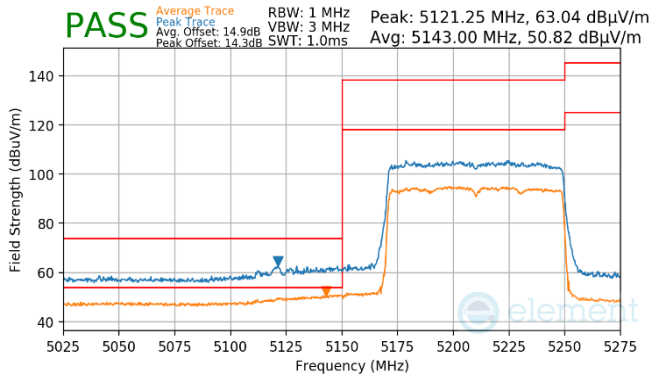
Plot 7-905. Antenna WF8 (Pk & Avg, RU996, Index 67, Ch.42, MCS11)
