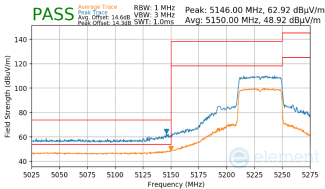
Plot 7-946. Antenna WF7 (Pk & Avg, RU484, Index 65, Ch.46, MCS11)
