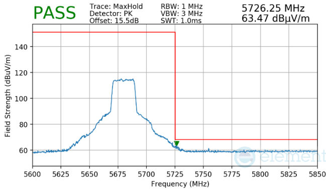
Plot 7-934. Antenna WF7 (Pk, RU242, Index 61, Ch.136, MCS11)
