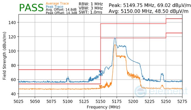
Plot 7-938. Antenna WF7 (Pk & Avg, RU26, Index 0, Ch.38, MCS11)
