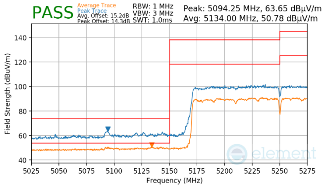
Plot 7-916. Antenna WF8 (Pk & Avg, RU996x2, Index 68, Ch.50, MCS11)
