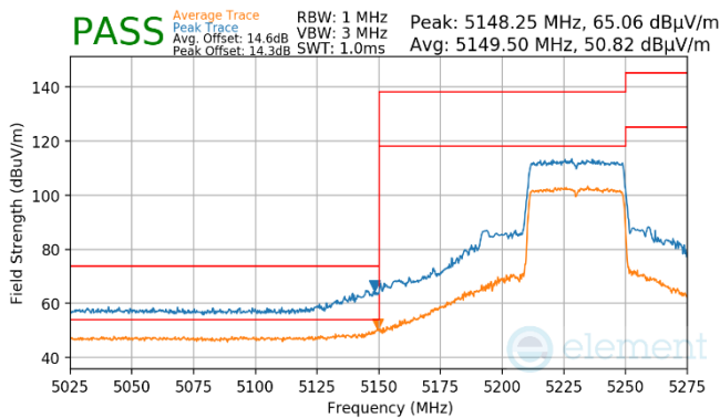
Plot 7-887. Antenna WF8 (Pk & Avg, RU484, Index 65, Ch.46, MCS11)
