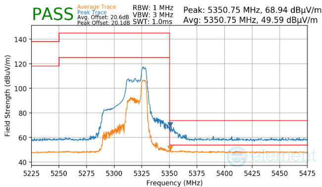
Plot 7-939. Antenna WF7 (Pk & Avg, RU52, Index 44, Ch.62, MCS11)
