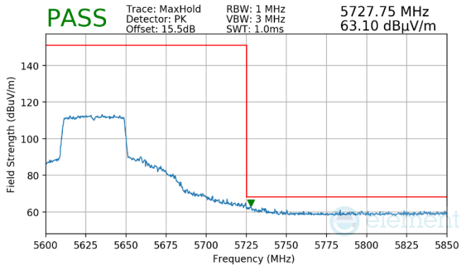
Plot 7-953. (FCC Only) Antenna WF7 (Pk, RU484, Index 65, Ch.126, MCS11)
