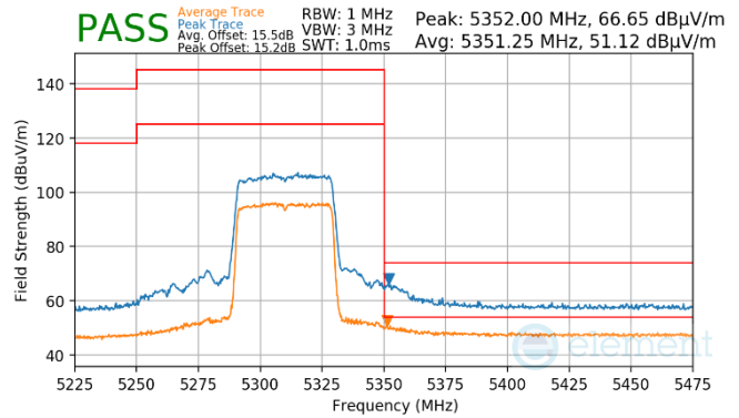
Plot 7-948. Antenna WF7 (Pk & Avg, RU484, Index 65, Ch.62, MCS11)
