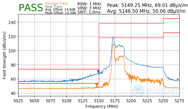
Plot 7-957. Antenna WF7 (Pk & Avg, RU26, Index 0, Ch.42, MCS11)
