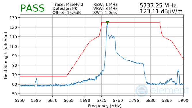
Plot 7-903. Antenna WF8 (Pk, RU26, Index 0, Ch.155, MCS11)
