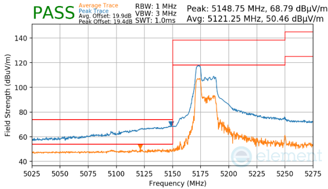
Plot 7-971. Antenna WF7 (Pk & Avg, RU52, Index 37, Ch.50 (L), MCS11)
