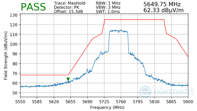
Plot 7-955. Antenna WF7 (Pk, RU484, Index 65, Ch.151, MCS11)
