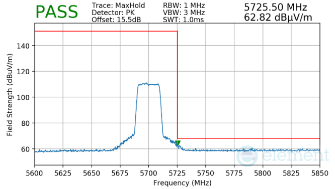
Plot 7-935. Antenna WF7 (Pk, RU242, Index 61, Ch.140, MCS11)
