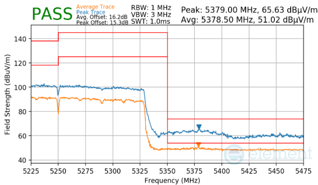
Plot 7-917. Antenna WF8 (Pk & Avg, RU996x2, Index 68, Ch.50, MCS11)
