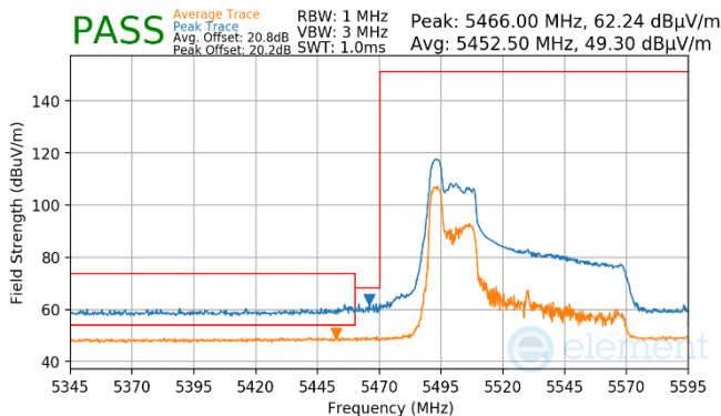
Plot 7-959. Antenna WF7 (Pk & Avg, RU52, Index 37, Ch.106, MCS11)
