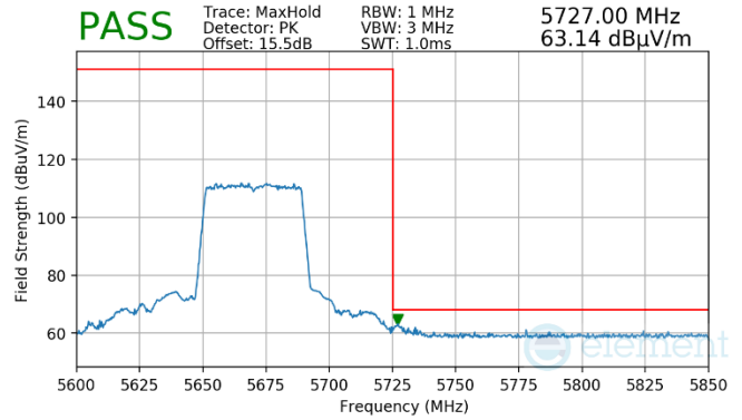
Plot 7-895. Antenna WF8 (Pk, RU484, Index 65, Ch.134, MCS11)
