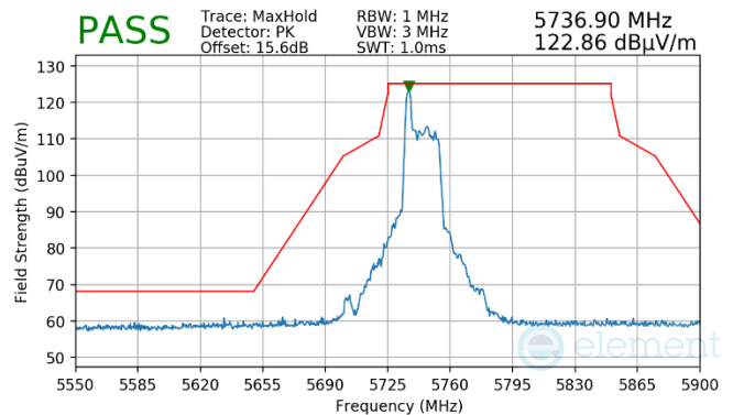
Plot 7-924. Antenna WF7 (Pk, RU26, Index 0, Ch.149, MCS11)
