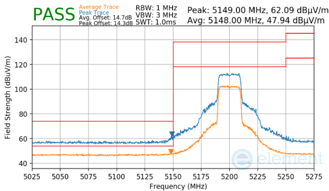
Plot 7-927. Antenna WF7 (Pk & Avg, RU242, Index 61, Ch.40, MCS11)
