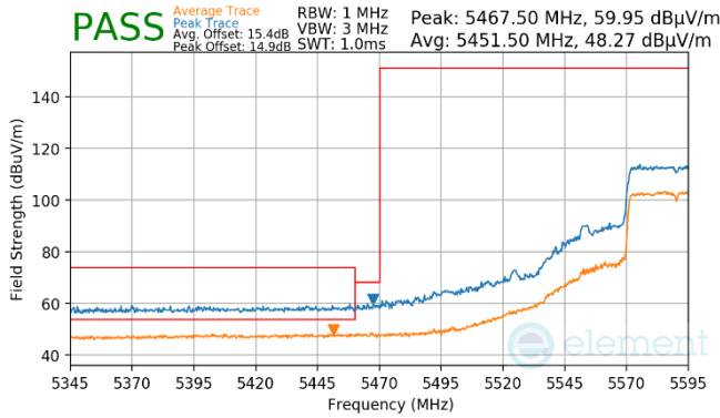
Plot 7-951. (FCC Only) Antenna WF7 (Pk & Avg, RU484, Index 65, Ch.118, MCS11)
