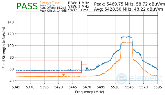
Plot 7-932. Antenna WF7 (Pk & Avg, RU242, Index 61, Ch.108, MCS11)
