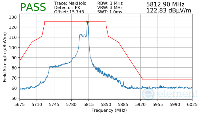
Plot 7-904. Antenna WF8 (Pk, RU26, Index 36, Ch.155, MCS11)
