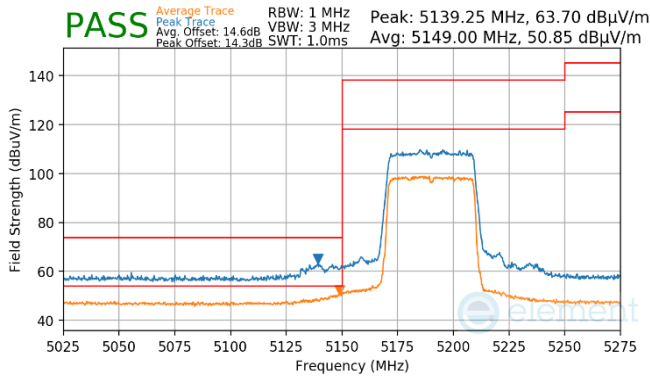
Plot 7-886. Antenna WF8 (Pk & Avg, RU484, Index 65, Ch.38, MCS11)
