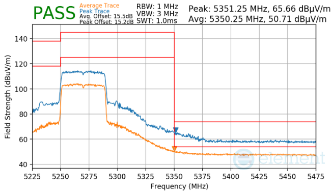
Plot 7-888. Antenna WF8 (Pk & Avg, RU484, Index 65, Ch.54, MCS11)
