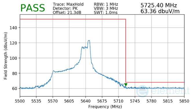
Plot 7-961. (FCC Only) Antenna WF7 (Pk, RU52, Index 52, Ch.122, MCS11)
