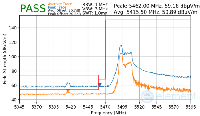
Plot 7-973. Antenna WF7 (Pk & Avg, RU52, Index 37, Ch.114 (L), MCS11) (FCC Only)
