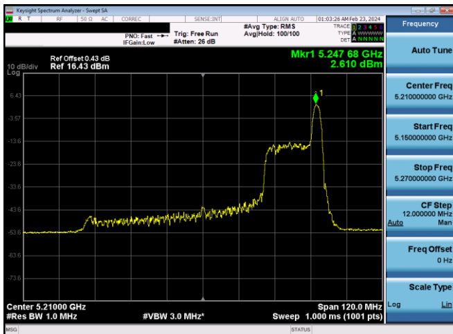
Plot 7-656. ISSED PSD SDM Diversity Antenna WF8 (80MHz BW 11ax Index 36 - RU26 - Ch.42)
