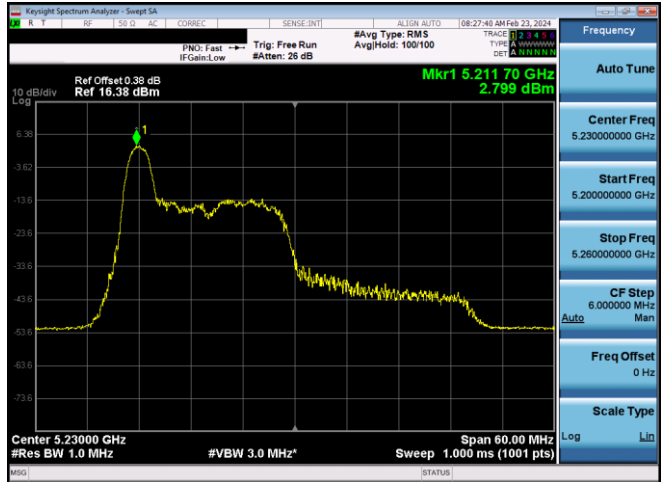
Plot 7-645. ISSED PSD SDM Diversity Antenna WF7 (40MHz BW 11ax Index 0 - RU26 - Ch.46)
