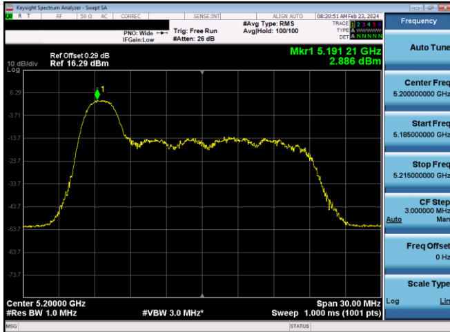
Plot 7-637. ISED PSD SDM Diversity Antenna WF7 (20MHz BW 11ax Index 0 – RU26 – Ch.40)
