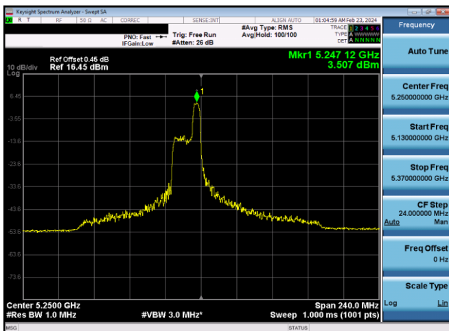
Plot 7-662. ISED PSD SDM Diversity Antenna WF8 (160MHz BW 11ax Index 52 – RU52 – Ch.50(L))
