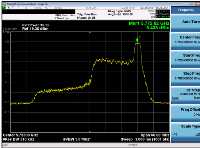
Plot 7-624. PSD CDD Diversity Antenna WF8 (40MHz BW 11ax Index 17 - RU26 - Ch.151)
