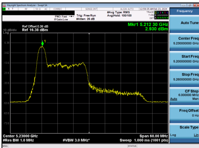
Plot 7-644. ISSED PSD SDM Diversity Antenna WF8 (40MHz BW 11ax Index 0 - RU26 - Ch.46)
