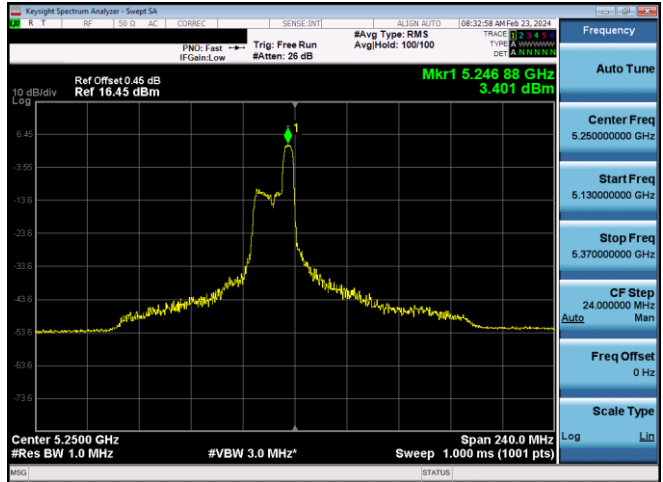
Plot 7-663. ISED PSD SDM Diversity Antenna WF7 (160MHz BW 11ax Index 52 – RU52 – Ch.50(L))
