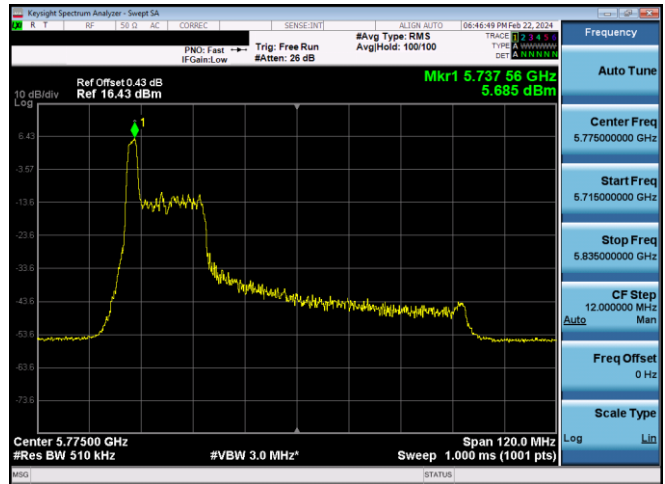
Plot 7-629. PSD CDD Diversity Antenna WF7 (80MHz BW 11ax Index 0 - RU26 - Ch.155)
