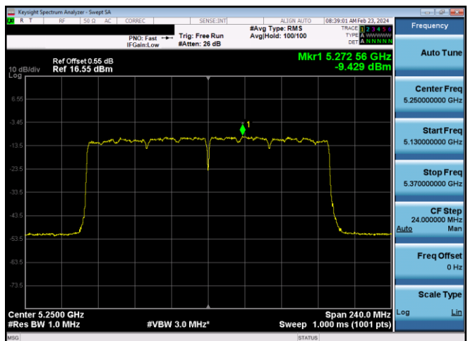
Plot 7-665. ISED PSD CDD Diversity Antenna WF7 (160MHz BW 11ax – RU996x2 – Ch.50)
