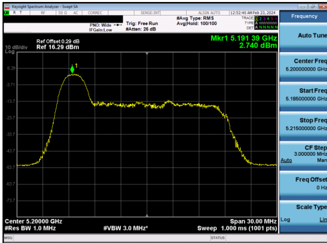
Plot 7-636. ISED PSD SDM Diversity Antenna WF8 (20MHz BW 11ax Index 0 – RU26 – Ch.40)
