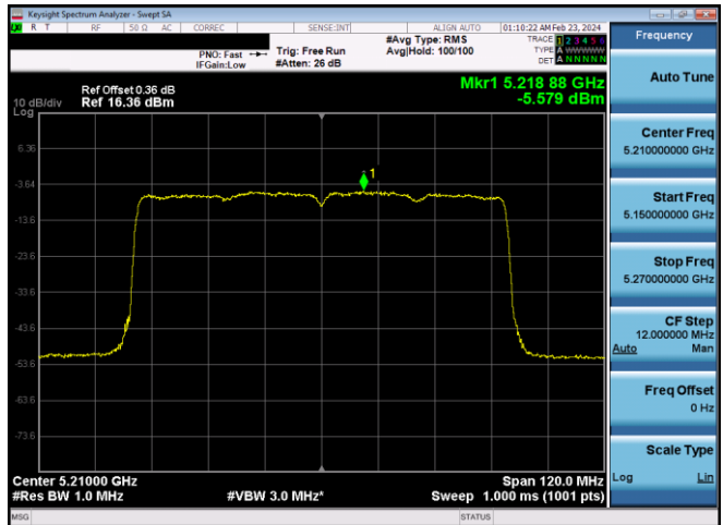
Plot 7-658. ISSED PSD CDD Diversity Antenna WF8 (80MHz BW 11ax - RU996 - Ch.42)
