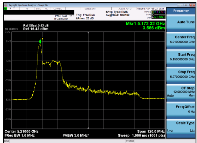
Plot 7-653. ISED PSD SDM Diversity Antenna WF7 (80MHz BW 11ax Index 0 - RU26 - Ch.42)
