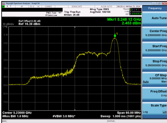
Plot 7-649. ISED PSD SDM Diversity Antenna WF7 (40MHz BW 11ax Index 17 - RU26 - Ch.46)
