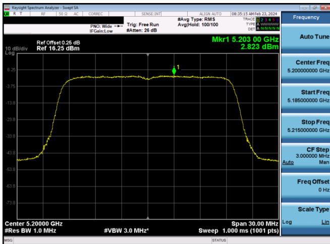
Plot 7-643. ISSED PSD SDM Diversity Antenna WF8 (20MHz BW 11ax- RU242 - Ch.40)
