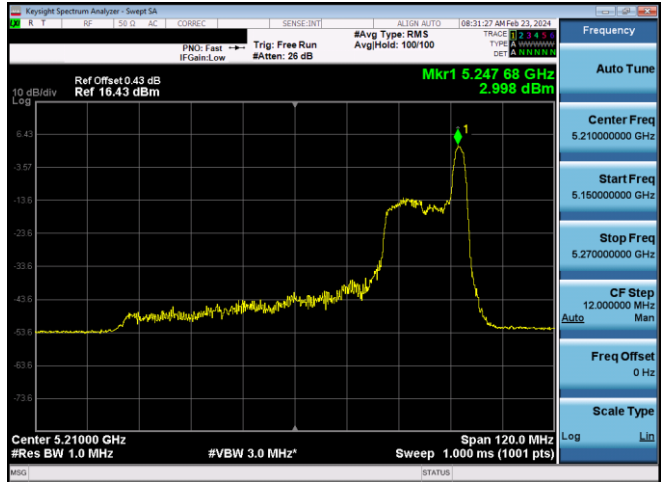
Plot 7-657. ISSED PSD SDM Diversity Antenna WF7 (80MHz BW 11ax Index 36 - RU26 - Ch.42)
