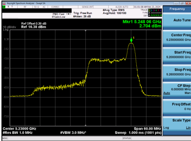
Plot 7-648. ISED PSD SDM Diversity Antenna WF8 (40MHz BW 11ax Index 17 - RU26 - Ch.46)
