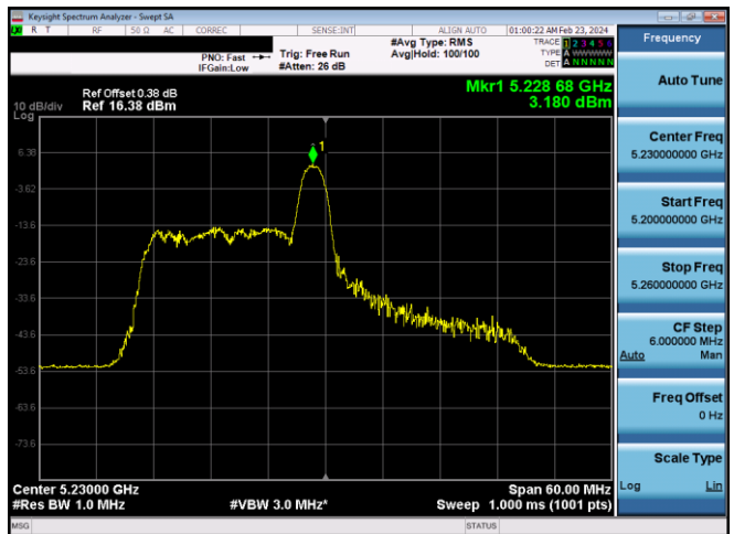
Plot 7-646. ISSED PSD SDM Diversity Antenna WF8 (40MHz BW 11ax Index 8 - RU26 - Ch.46)
