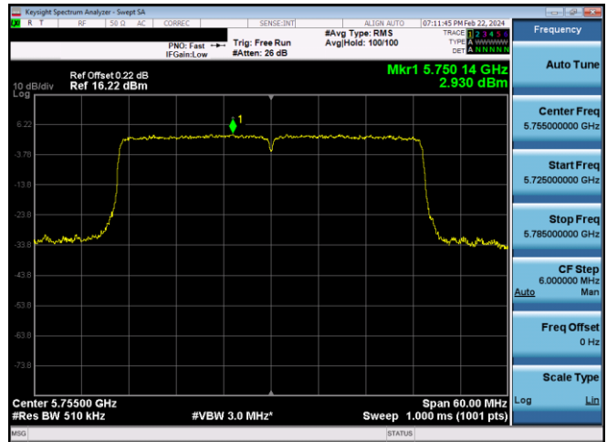
Plot 7-627. PSD CDD Diversity Antenna WF7 (40MHz BW 11ax - RU484 - Ch.151)
