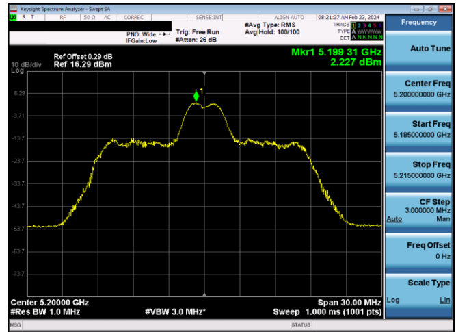
Plot 7-639. ISED PSD SDM Diversity Antenna WF7 (20MHz BW 11ax Index 4 – RU26 – Ch.40)
