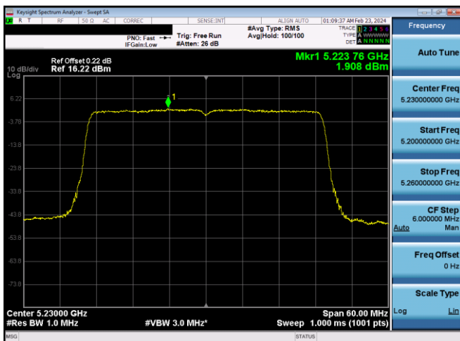
Plot 7-650. ISED PSD CDD Diversity Antenna WF8 (40MHz BW 11ax - RU484 - Ch.46)
