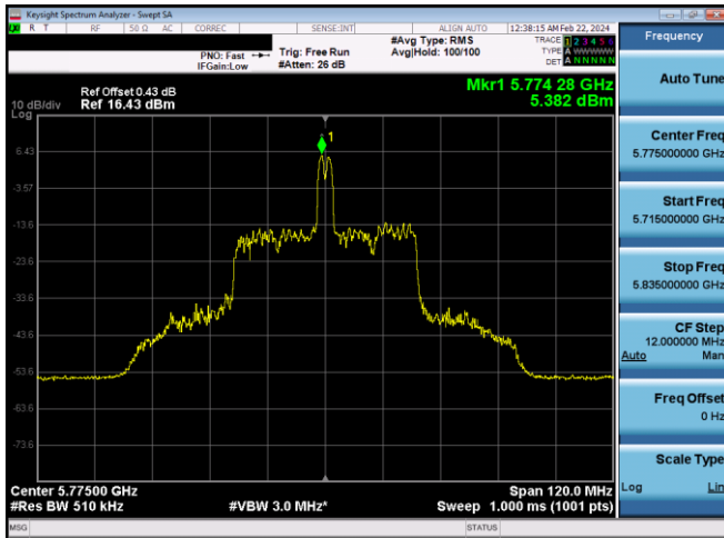
Plot 7-630. PSD CDD Diversity Antenna WF8 (80MHz BW 11ax Index 18 – RU26 – Ch.155)
