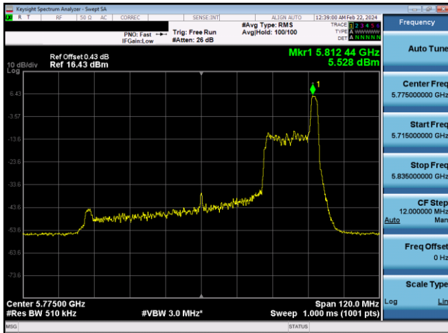
Plot 7-632. PSD CDD Diversity Antenna WF8 (80MHz BW 11ax Index 36 – RU26 – Ch.155)
