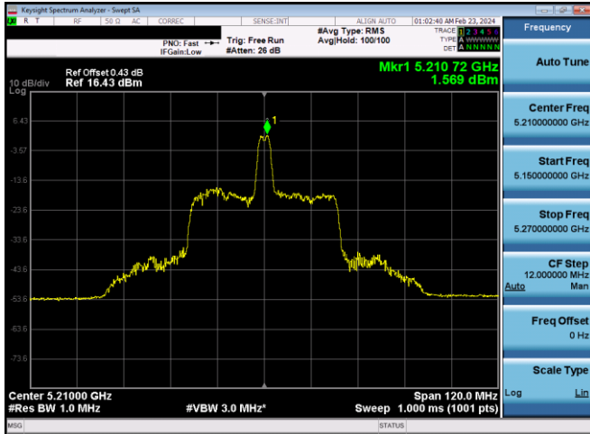
Plot 7-654. ISSED PSD SDM Diversity Antenna WF8 (80MHz BW 11ax Index 18 - RU26 - Ch.42)
