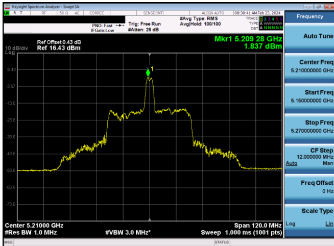
Plot 7-655. ISSED PSD SDM Diversity Antenna WF7 (80MHz BW 11ax Index 18 - RU26 - Ch.42)
