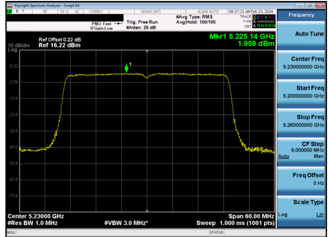
Plot 7-651. ISED PSD CDD Diversity Antenna WF7 (40MHz BW 11ax - RU484 - Ch.46)
