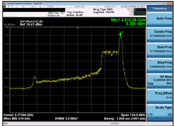
Plot 7-633. PSD CDD Diversity Antenna WF7 (80MHz BW 11ax Index 36 – RU26 – Ch.155)
