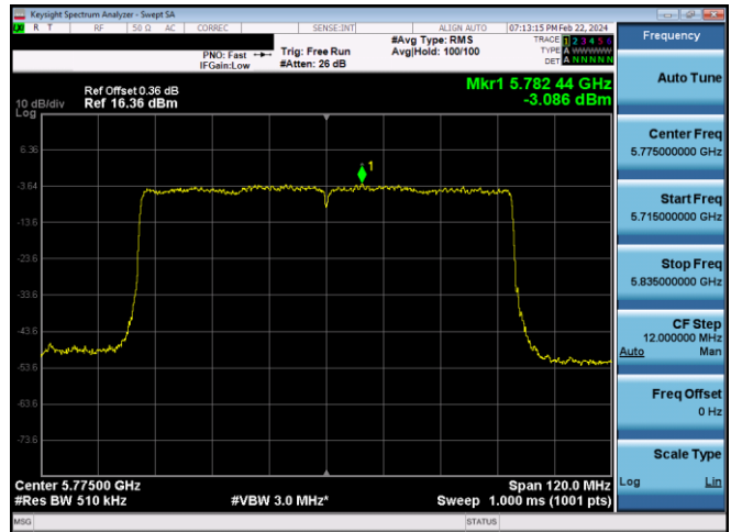
Plot 7-635. PSD CDD Diversity Antenna WF7 (80MHz BW 11ax – RU996 – Ch.155)
