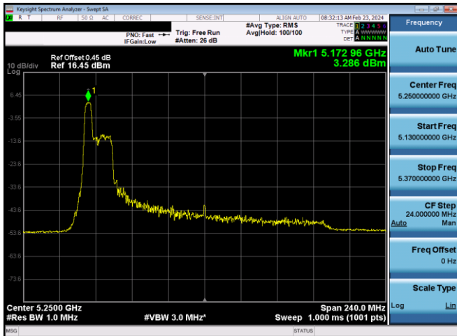
Plot 7-661. ISED PSD SDM Diversity Antenna WF7 (160MHz BW 11ax Index 37 – RU52 – Ch.50(L))
