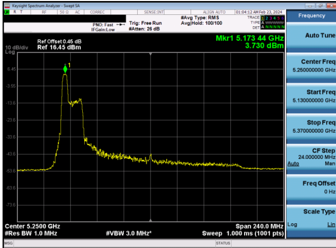
Plot 7-660. ISED PSD SDM Diversity Antenna WF8 (160MHz BW 11ax Index 37 – RU52 – Ch.50(L))
