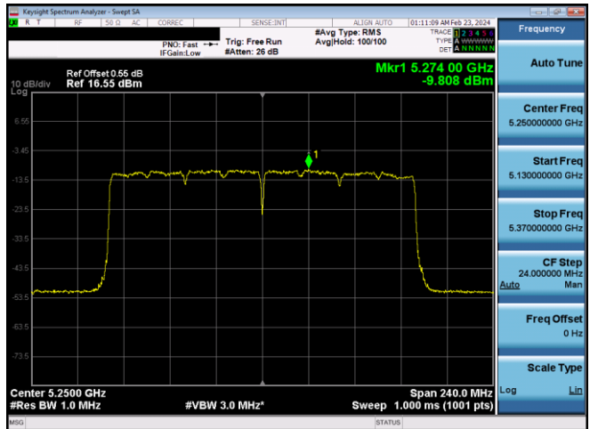
Plot 7-664. ISED PSD CDD Diversity Antenna WF8 (160MHz BW 11ax – RU996x – Ch.50)
