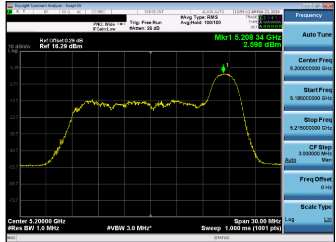
Plot 7-640. ISED PSD SDM Diversity Antenna WF8 (20MHz BW 11ax Index 8– RU26 – Ch.40)
