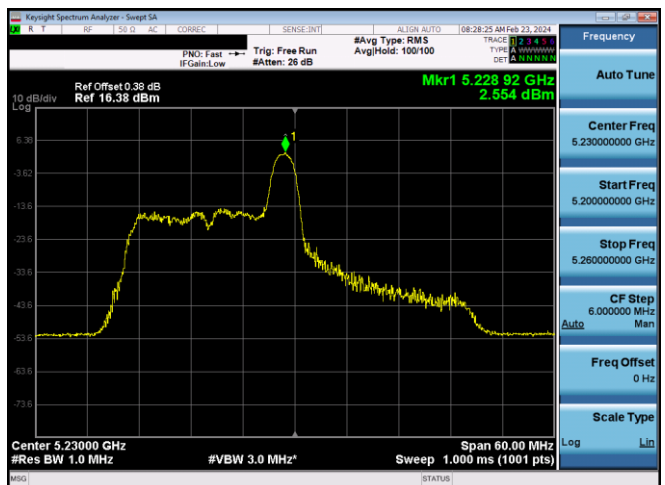
Plot 7-647. ISSED PSD SDM Diversity Antenna WF7 (40MHz BW 11ax Index 8 - RU26 - Ch.46)
