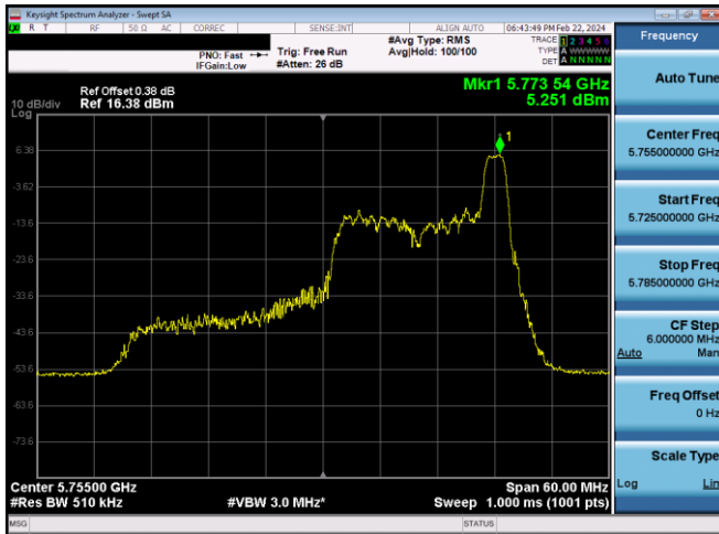
Plot 7-625. PSD CDD Diversity Antenna WF7 (40MHz BW 11ax Index 17 - RU26 - Ch.151)
