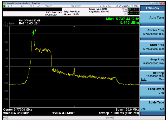
Plot 7-628. PSD CDD Diversity Antenna WF8 (80MHz BW 11ax Index 0 - RU26 - Ch.155)
