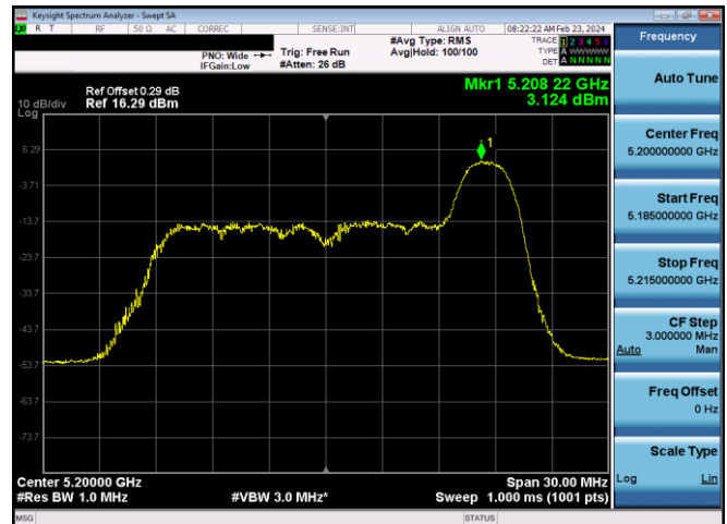
Plot 7-641. ISED PSD SDM Diversity Antenna WF7 (20MHz BW 11ax Index 8– RU26 – Ch.40)
