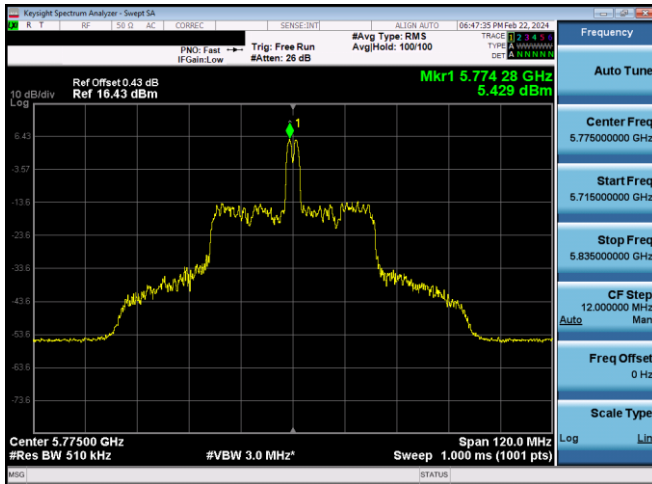
Plot 7-631. PSD CDD Diversity Antenna WF7 (80MHz BW 11ax Index 18 – RU26 – Ch.155)
