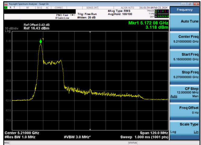
Plot 7-652. ISED PSD SDM Diversity Antenna WF8 (80MHz BW 11ax Index 0 - RU26 - Ch.42)
