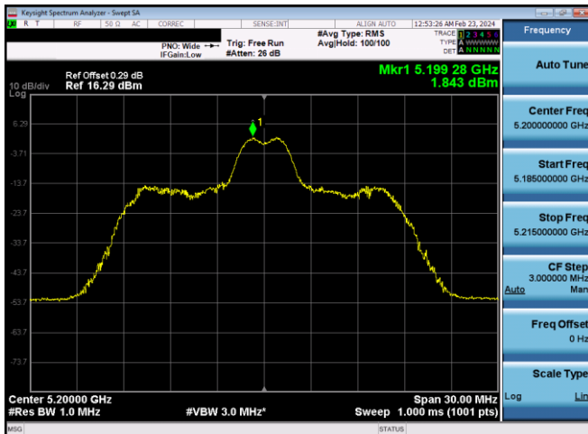
Plot 7-638. ISED PSD SDM Diversity Antenna WF8 (20MHz BW 11ax Index 4 – RU26 – Ch.40)
