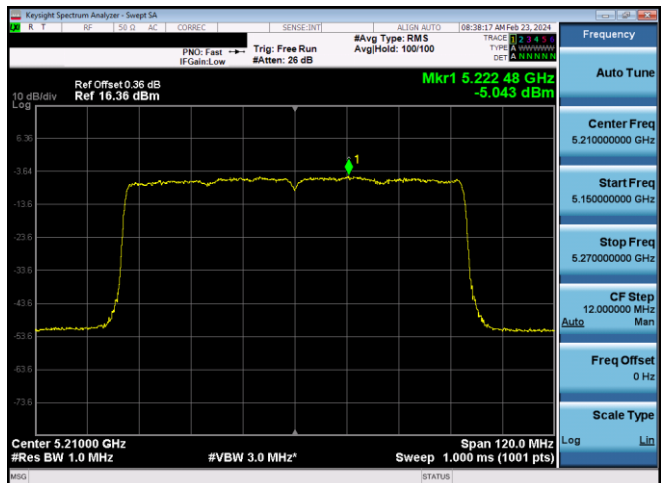
Plot 7-659. ISSED PSD CDD Diversity Antenna WF7 (80MHz BW 11ax - RU996 - Ch.42)
