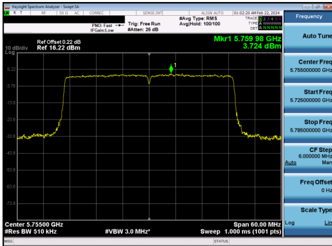
Plot 7-626. PSD CDD Diversity Antenna WF8 (40MHz BW 11ax - RU484 - Ch.151)
