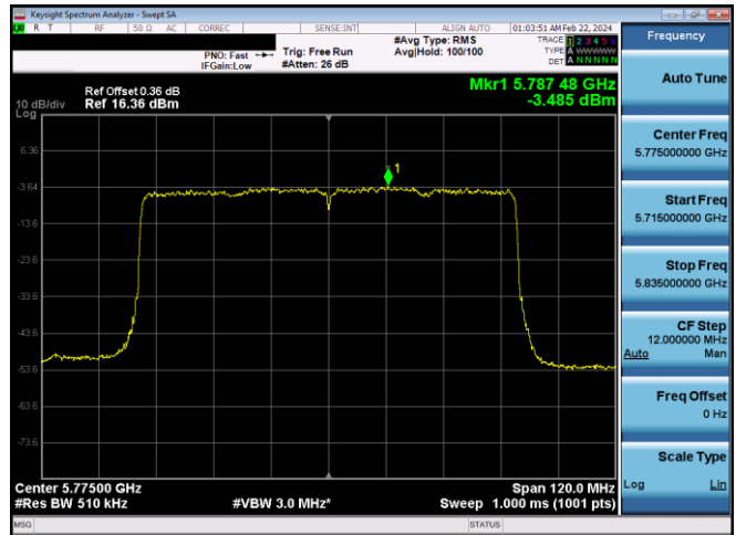
Plot 7-634. PSD CDD Diversity Antenna WF8 (80MHz BW 11ax – RU996 – Ch.155)
