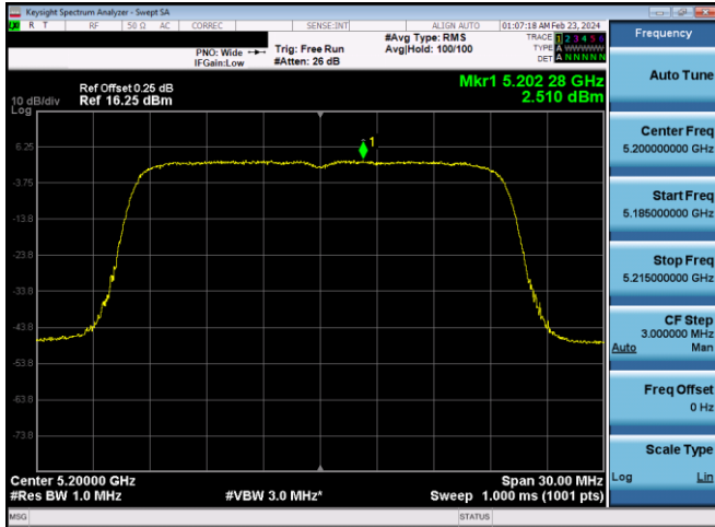
Plot 7-642. ISSED PSD SDM Diversity Antenna WF8 (20MHz BW 11ax- RU242 - Ch.40)
