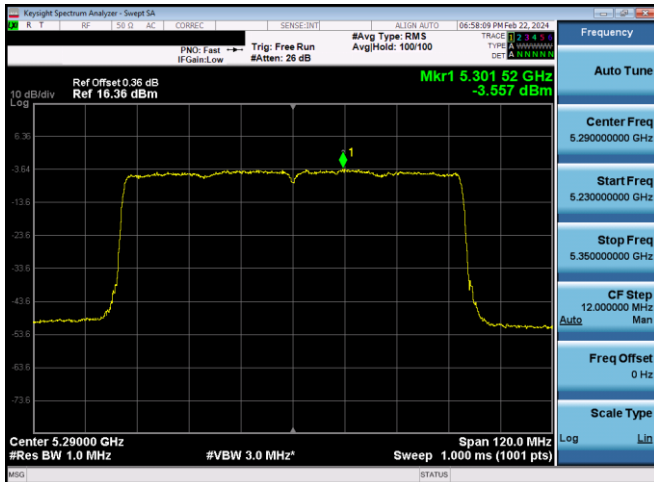
Plot 7-579. PSD CDD Diversity Antenna WF7 (80MHz BW 11ax - RU96 - Ch.58)
