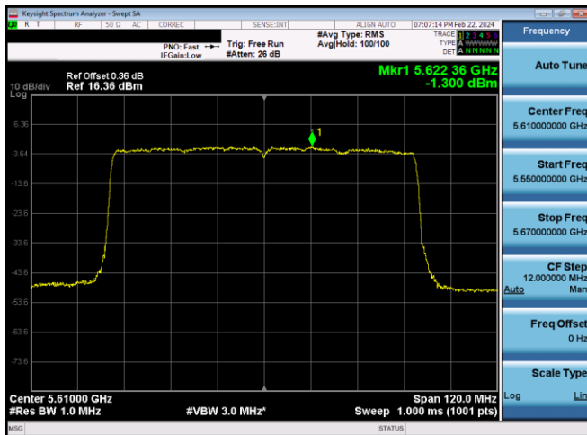
Plot 7-603. PSD CDD Diversity Antenna WF7 (80MHz BW 11ax - RU996 - Ch.122)
