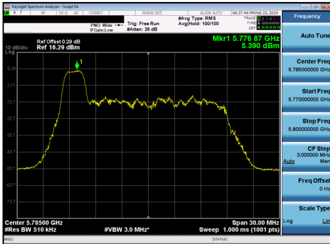
Plot 7-613. PSD CDD Diversity Antenna WF7 (20MHz BW 11ax Index 0 – RU26 – Ch.157)
