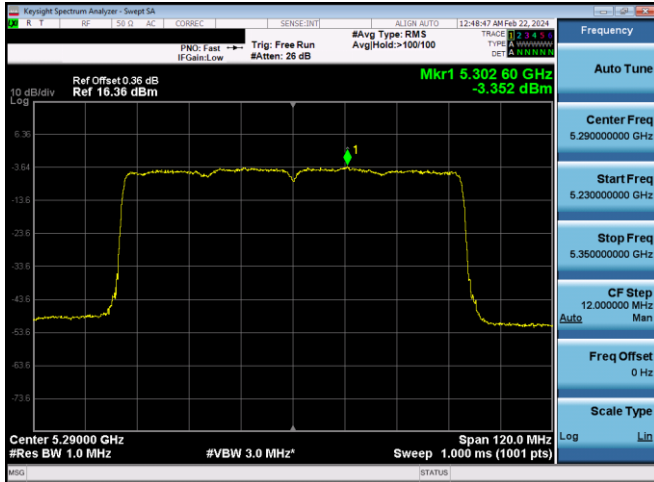
Plot 7-578. PSD CDD Diversity Antenna WF8 (80MHz BW 11ax - RU96 - Ch.58)
