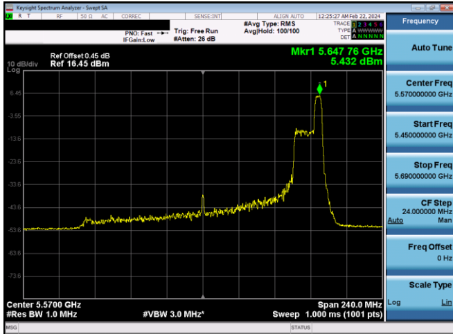
Plot 7-608. PSD CDD Diversity Antenna WF8 (160MHz BW 11ax Index 52 - RU52 - Ch.114 (U))
