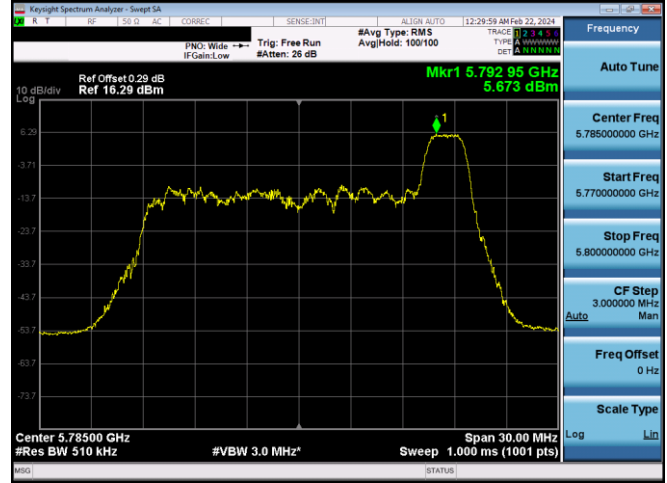
Plot 7-616. PSD CDD Diversity Antenna WF8 (20MHz BW 11ax Index 8 – RU26 – Ch.157)
