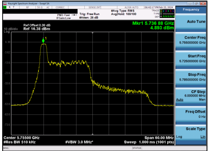
Plot 7-621. PSD CDD Diversity Antenna WF7 (40MHz BW 11ax Index 0 – RU26 – Ch.151)
