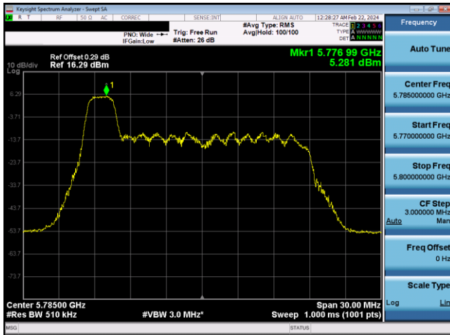
Plot 7-612. PSD CDD Diversity Antenna WF8 (20MHz BW 11ax Index 0 – RU26 – Ch.157)
