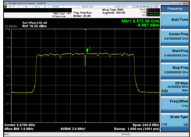
Plot 7-610. PSD CDD Diversity Antenna WF8 (160MHz BW 11ax - RU996x2 - Ch.114)
