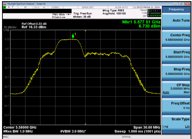
Plot 7-582. PSD CDD Diversity Antenna WF8 (20MHz BW 11ax Index 38 - RU52 - Ch.116)
