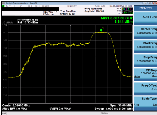
Plot 7-585. PSD CDD Diversity Antenna WF7 (20MHz BW 11ax Index 40 - RU52 - Ch.116)
