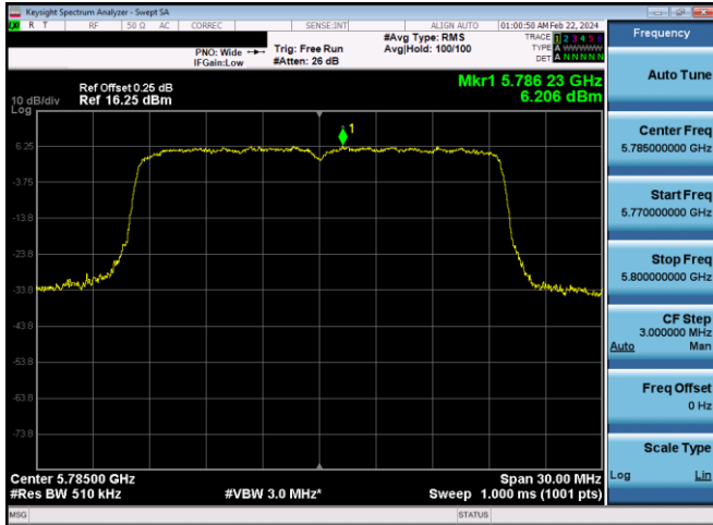
Plot 7-618. PSD CDD Diversity Antenna WF8 (20MHz BW 11ax – RU242 – Ch.157)
