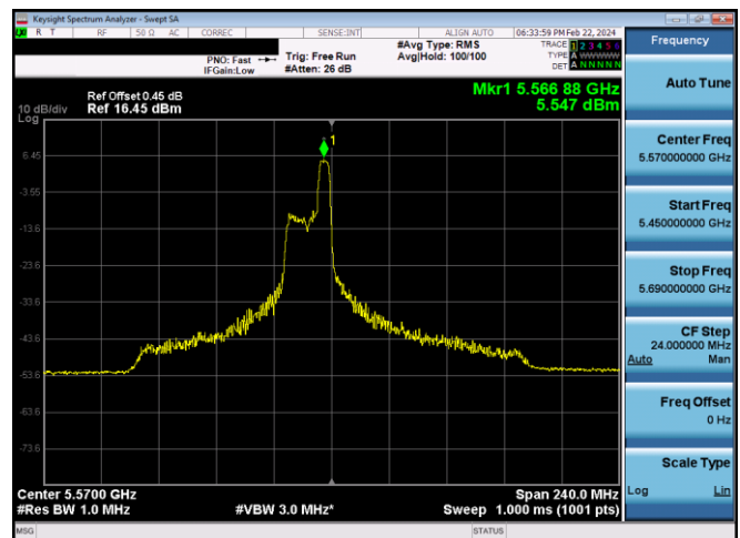
Plot 7-607. PSD CDD Diversity Antenna WF7 (160MHz BW 11ax Index 52 - RU52 - Ch.114 (L))
