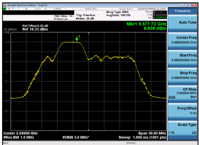
Plot 7-583. PSD CDD Diversity Antenna WF7 (20MHz BW 11ax Index 38 - RU52 - Ch.116)
