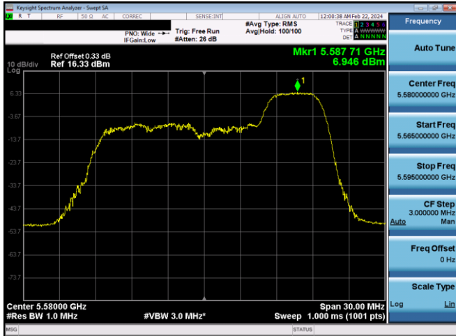
Plot 7-584. PSD CDD Diversity Antenna WF8 (20MHz BW 11ax Index 40 - RU52 - Ch.116)
