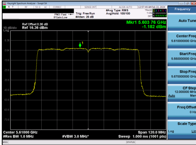
Plot 7-602. PSD CDD Diversity Antenna WF8 (80MHz BW 11ax - RU996 - Ch.122)
