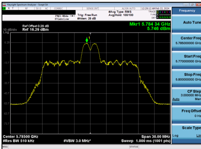
Plot 7-614. PSD CDD Diversity Antenna WF8 (20MHz BW 11ax Index 4 – RU26 – Ch.157)
