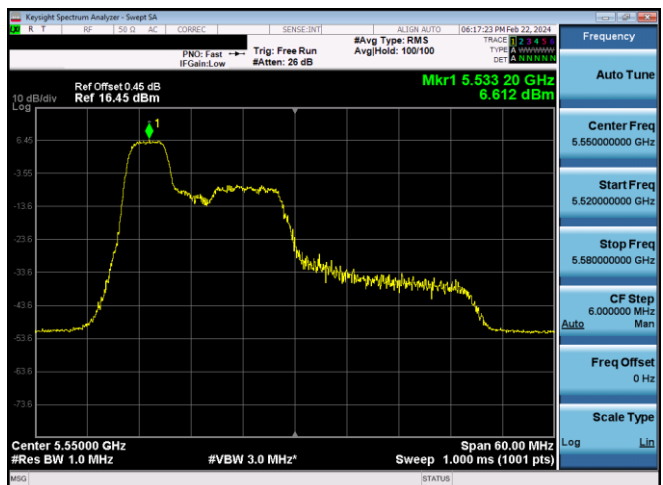
Plot 7-589. PSD CDD Diversity Antenna WF7 (40MHz BW 11ax Index 37 - RU52 - Ch.110)
