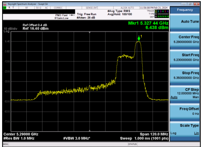
Plot 7-576. PSD CDD Diversity Antenna WF8 (80MHz BW 11ax Index 52 – RU52 – Ch.58)
