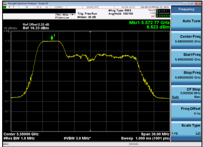
Plot 7-581. PSD CDD Diversity Antenna WF7 (20MHz BW 11ax Index 37 - RU52 - Ch.116)
