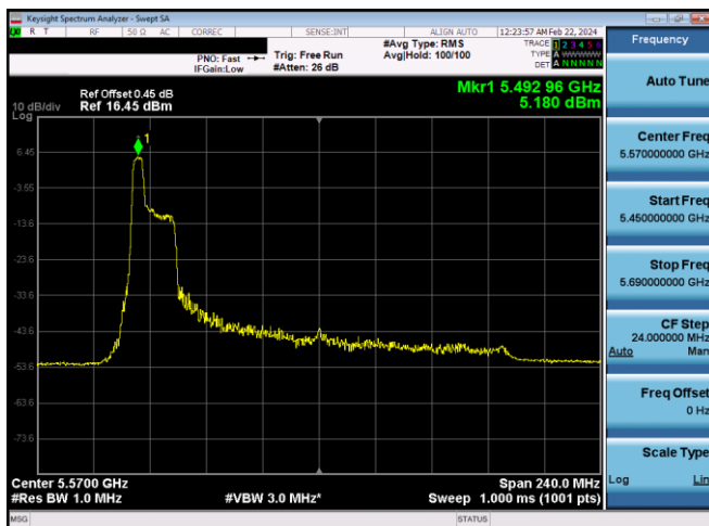
Plot 7-604. PSD CDD Diversity Antenna WF8 (160MHz BW 11ax Index 37 - RU52 - Ch.114 (L))
