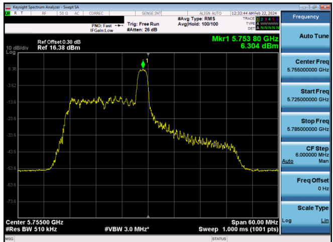
Plot 7-622. PSD CDD Diversity Antenna WF8 (40MHz BW 11ax Index 8 – RU26 – Ch.151)
