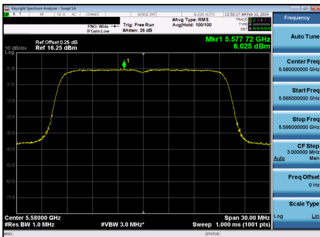
Plot 7-586. PSD CDD Diversity Antenna WF8 (20MHz BW 11ax- RU242 - Ch.116)
