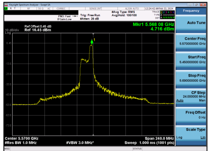
Plot 7-606. PSD CDD Diversity Antenna WF8 (160MHz BW 11ax Index 52 - RU52 - Ch.114 (L))
