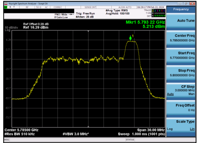
Plot 7-617. PSD CDD Diversity Antenna WF7 (20MHz BW 11ax Index 8 – RU26 – Ch.157)
