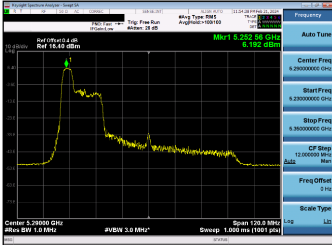
Plot 7-572. PSD CDD Diversity Antenna WF8 (80MHz BW 11ax Index 37 – RU52 – Ch.58)
