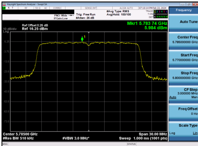
Plot 7-619. PSD CDD Diversity Antenna WF7 (20MHz BW 11ax – RU242 – Ch.157)
