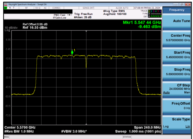
Plot 7-611. PSD CDD Diversity Antenna WF7 (160MHz BW 11ax - RU996x2 - Ch.114)
