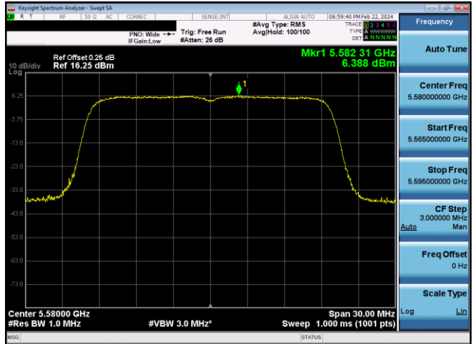
Plot 7-587. PSD CDD Diversity Antenna WF7 (20MHz BW 11ax- RU242 - Ch.116)
