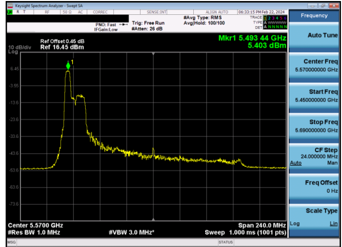
Plot 7-605. PSD CDD Diversity Antenna WF7 (160MHz BW 11ax Index 37 - RU52 - Ch.114 (L))
