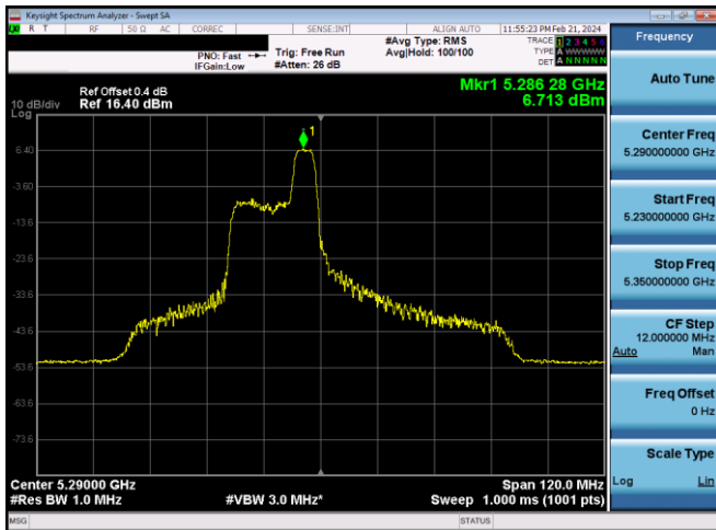
Plot 7-574. PSD CDD Diversity Antenna WF8 (80MHz BW 11ax Index 44 – RU52 – Ch.58)
