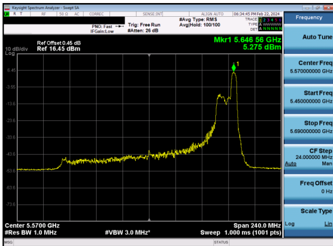
Plot 7-609. PSD CDD Diversity Antenna WF7 (160MHz BW 11ax Index 52 - RU52 - Ch.114 (U))
