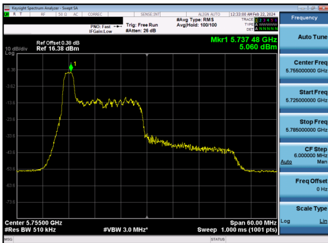
Plot 7-620. PSD CDD Diversity Antenna WF8 (40MHz BW 11ax Index 0 – RU26 – Ch.151)
