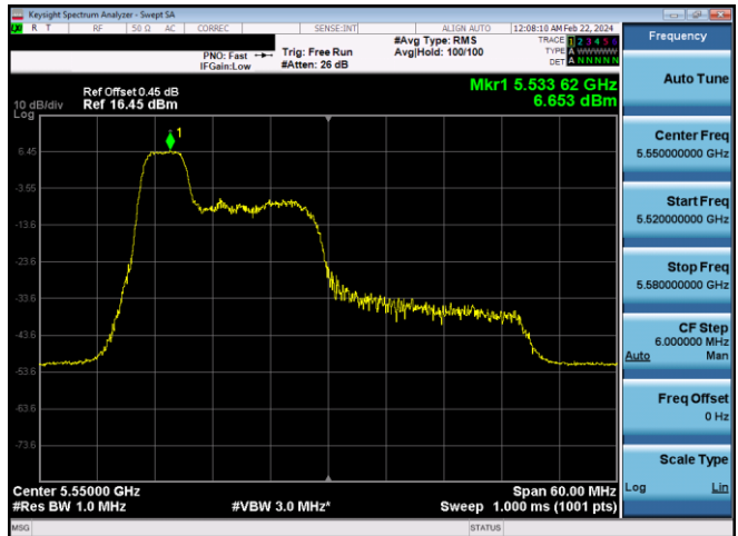
Plot 7-588. PSD CDD Diversity Antenna WF8 (40MHz BW 11ax Index 37 - RU52 - Ch.110)
