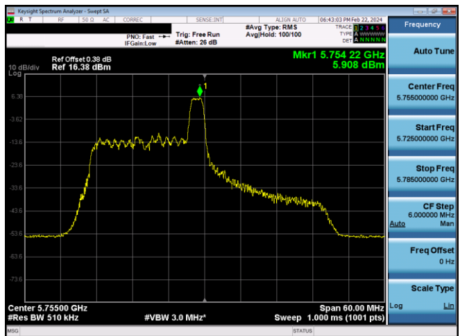
Plot 7-623. PSD CDD Diversity Antenna WF7 (40MHz BW 11ax Index 8 – RU26 – Ch.151)
