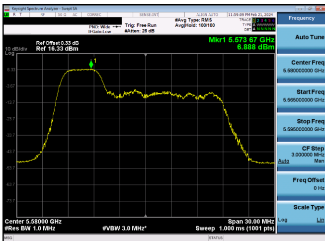
Plot 7-580. PSD CDD Diversity Antenna WF8 (20MHz BW 11ax Index 37 - RU52 - Ch.116)
