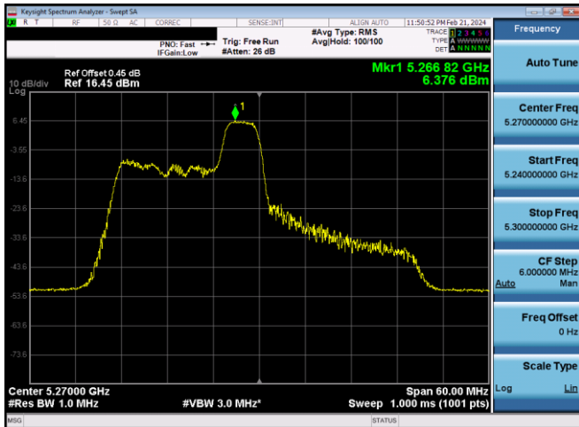
Plot 7-425. PSD CDD Primary Antenna WF8 (40MHz BW 11ax Index 40 - RU52 - Ch.54)
