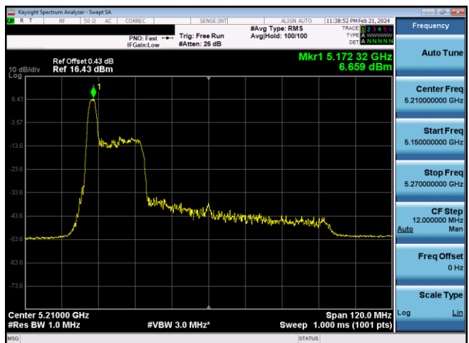
Plot 7-399. PSD CDD Primary Antenna WF8 (80MHz BW 11ax Index 0 - RU26 - Ch.42)
