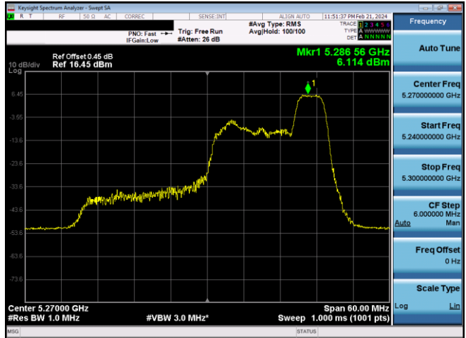
Plot 7-427. PSD CDD Primary Antenna WF8 (40MHz BW 11ax Index 44 - RU52 - Ch.54)
