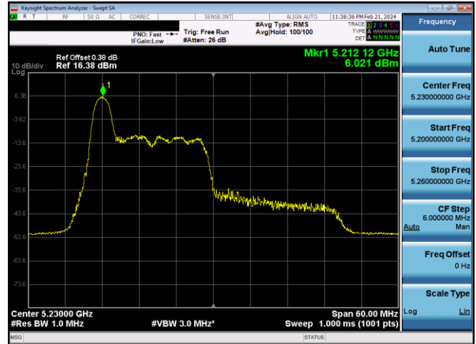
Plot 7-391. PSD CDD Primary Antenna WF8 (40MHz BW 11ax Index 0 - RU26 - Ch.46)
