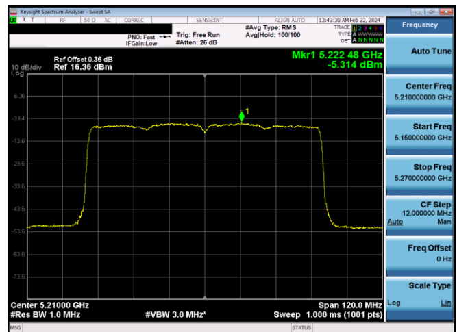
Plot 7-405. PSD CDD Primary Antenna WF8 (80MHz BW 11ax - RU996 - Ch.42)
