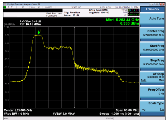
Plot 7-423. PSD CDD Primary Antenna WF8 (40MHz BW 11ax Index 37 - RU52 - Ch.54)
