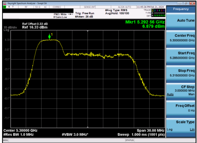
Plot 7-415. PSD CDD Primary Antenna WF8 (20MHz BW 11ax Index 37 - RU52 - Ch.60)
