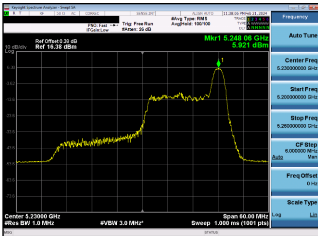
Plot 7-395. PSD CDD Primary Antenna WF8 (40MHz BW 11ax Index 17 - RU26 - Ch.46)
