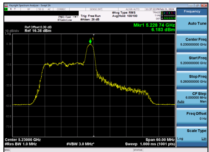
Plot 7-393. PSD CDD Primary Antenna WF8 (40MHz BW 11ax Index 8 - RU26 - Ch.46)
