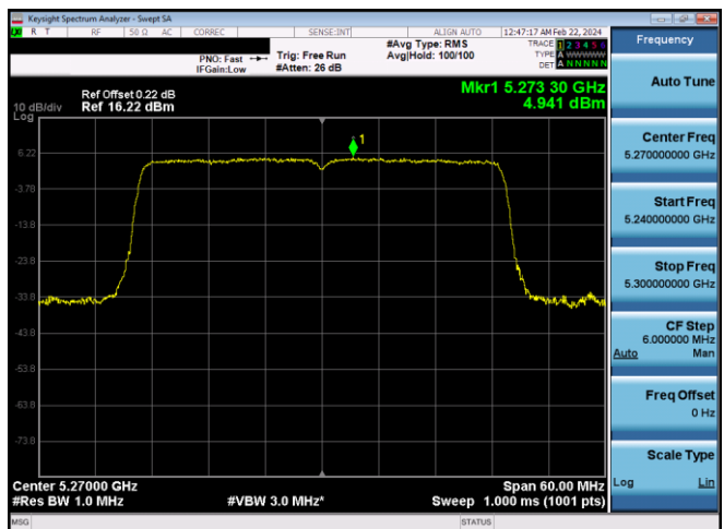
Plot 7-429. PSD CDD Primary Antenna WF8 (40MHz BW 11ax - RU484 - Ch.54)
