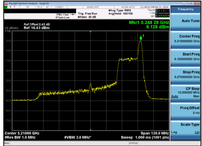
Plot 7-403. PSD CDD Primary Antenna WF8 (80MHz BW 11ax Index 36 - RU26 - Ch.42)
