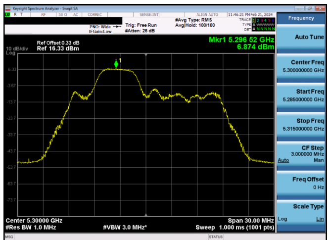
Plot 7-417. PSD CDD Primary Antenna WF8 (20MHz BW 11ax Index 38 - RU52 - Ch.60)
