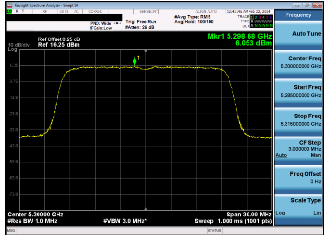
Plot 7-421. PSD CDD Primary Antenna WF8 (20MHz BW 11ax- RU242 - Ch.60)
