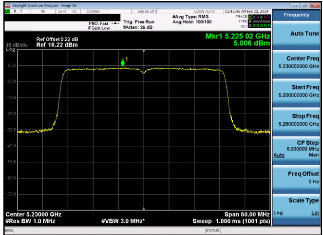
Plot 7-397. PSD CDD Primary Antenna WF8 (40MHz BW 11ax - RU484 - Ch.46)
