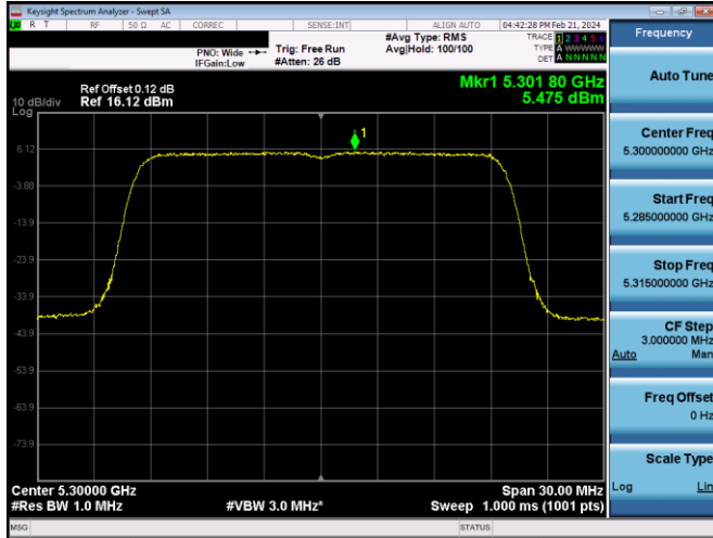
Plot 7-595. PSD CDD PRIMARY Antenna WF5b (20MHz BW 802.11ax(SU) – Ch. 60, MCS2)
