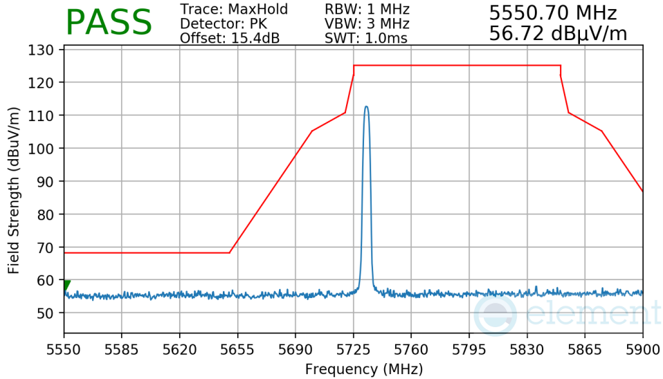
Plot 7-224. Radiated Lower Band Edge Measurement TxBF
