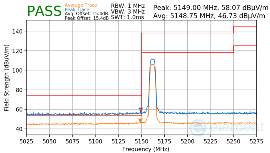
Plot 7-223. Radiated Lower Band Edge Measurement TxBF
