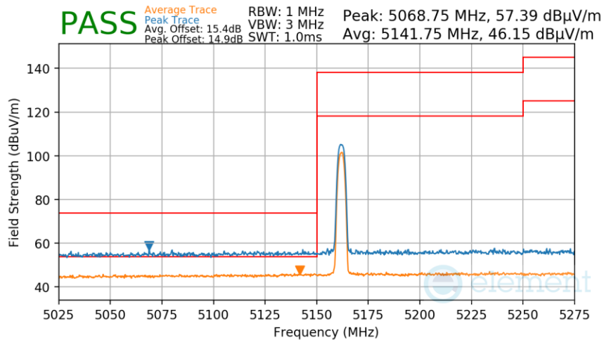
Plot 7-216. Radiated Lower Band Edge Measurement Antenna WF7
