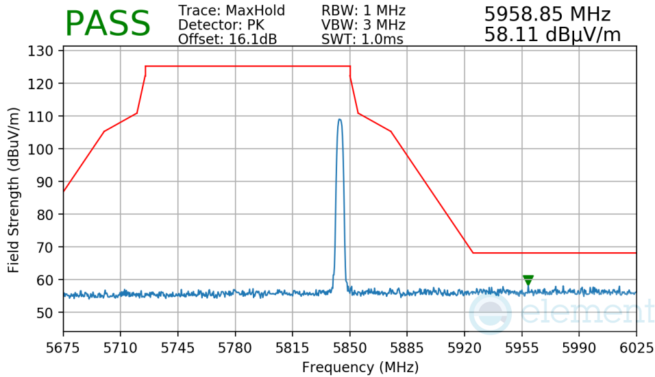
Plot 7-220. Radiated Upper Band Edge Measurement Antenna WF7
