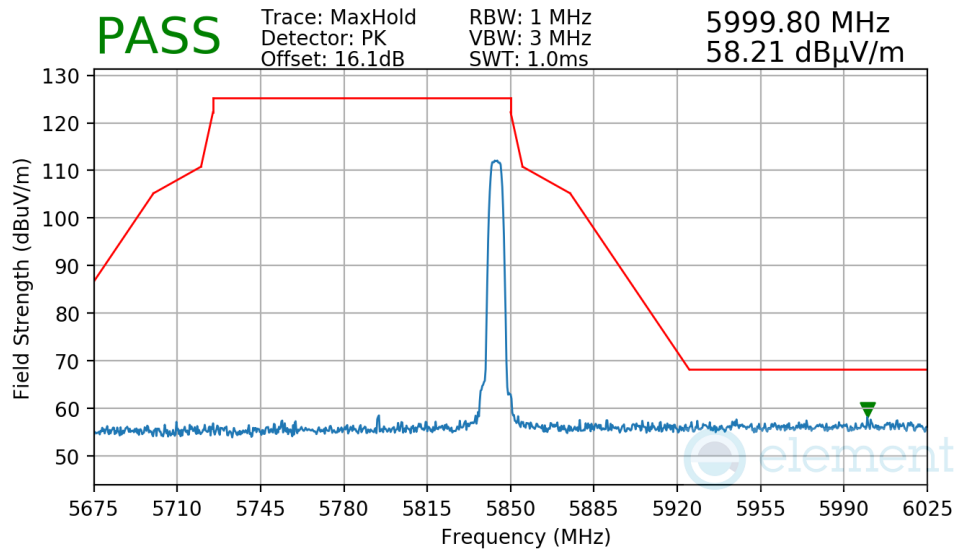
Plot 7-227. Radiated Upper Band Edge Measurement TxBF
