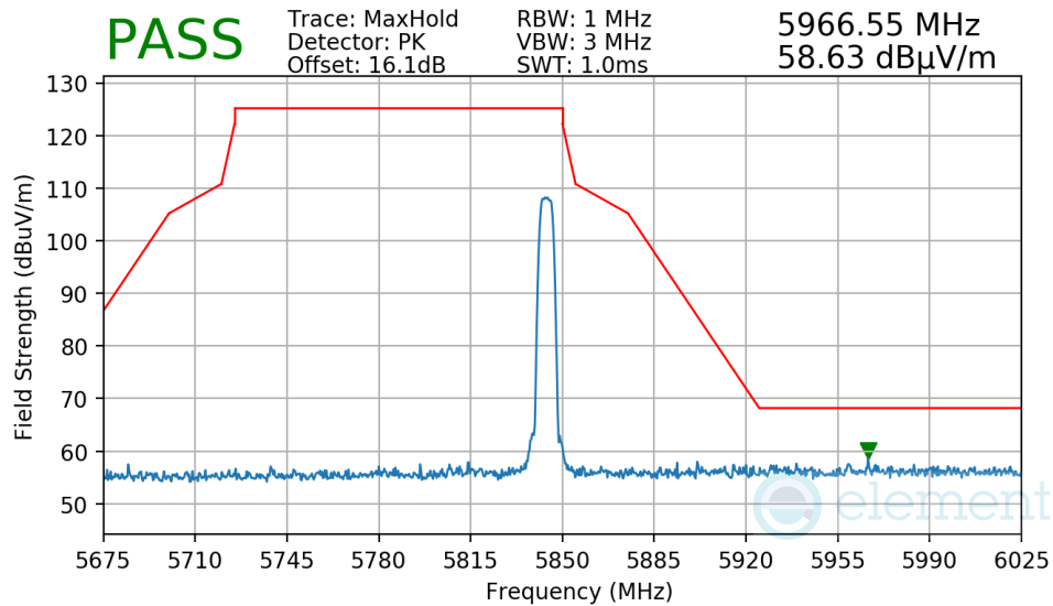
Plot 7-221. Radiated Upper Band Edge Measurement Antenna WF7
