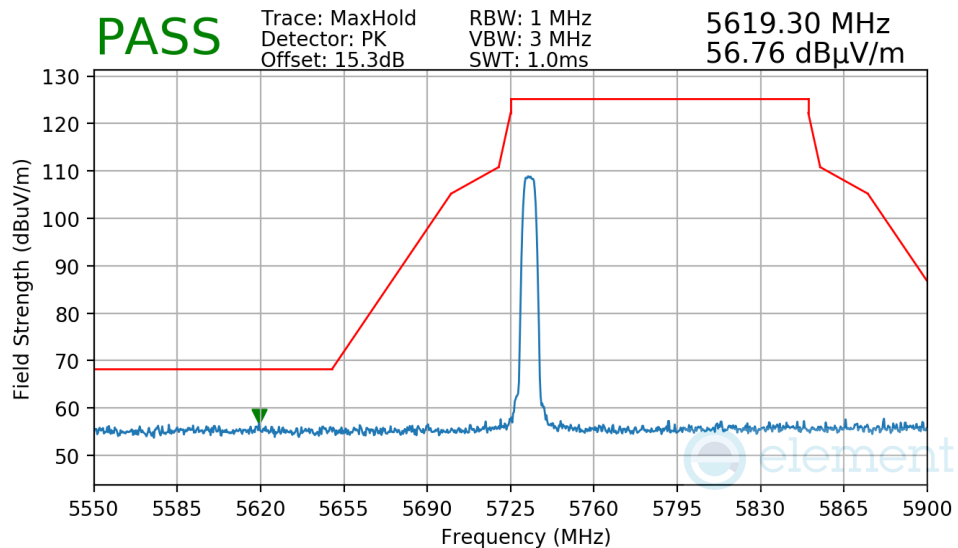
Plot 7-219. Radiated Lower Band Edge Measurement Antenna WF7
