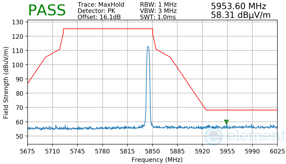
Plot 7-226. Radiated Upper Band Edge Measurement TxBF
