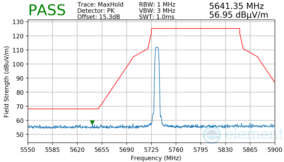
Plot 7-225. Radiated Lower Band Edge Measurement TxBF
