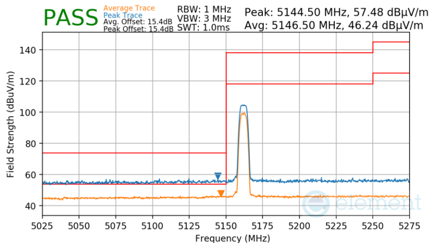
Plot 7-217. Radiated Lower Band Edge Measurement Antenna WF7
