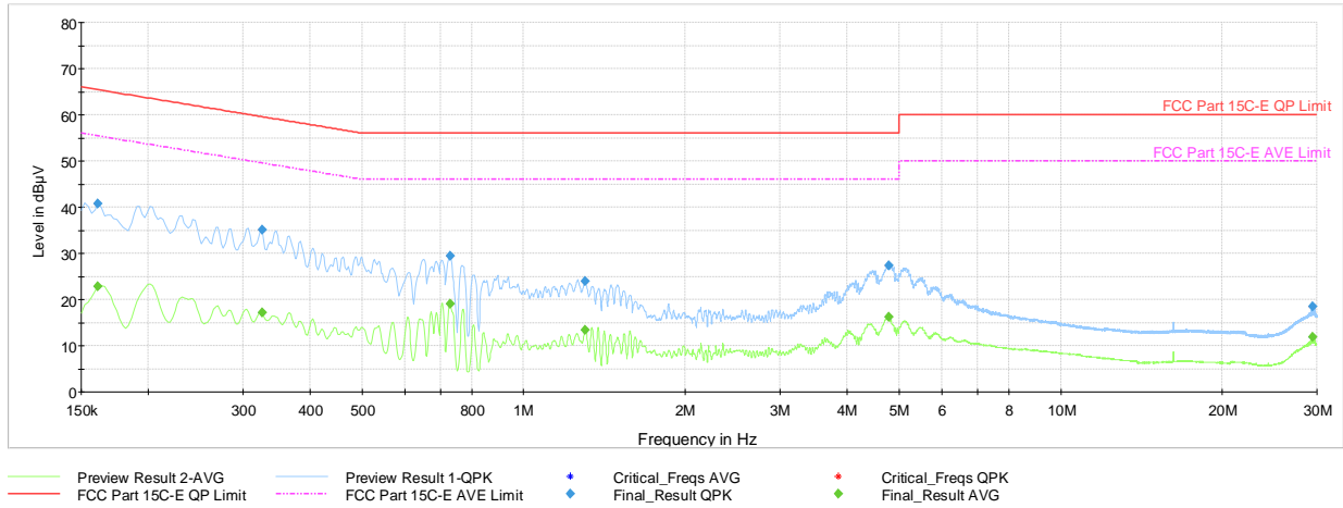
Plot 7-230. AC Line Conducted Plot TxBF (HDR4, ePA – 5245MHz) (N) with AC/DC Adapter
