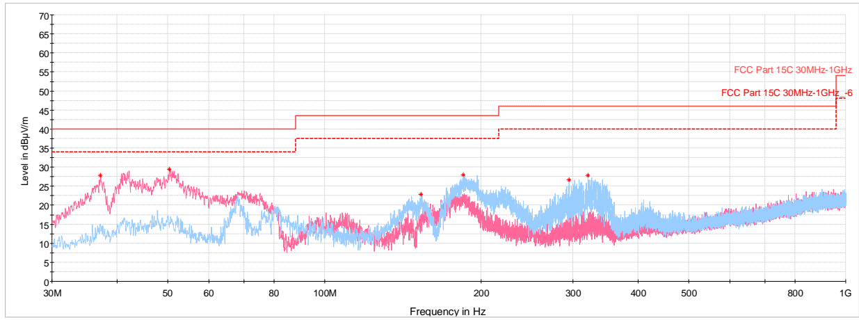
Plot 7-228. Radiated Spurious Emissions Below 1GHz TxBF (HDR4, ePA – 5245MHz), with AC/DC Adapter
