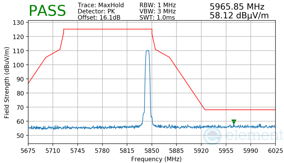
Plot 7-215. Radiated Upper Band Edge Measurement Antenna WF8
