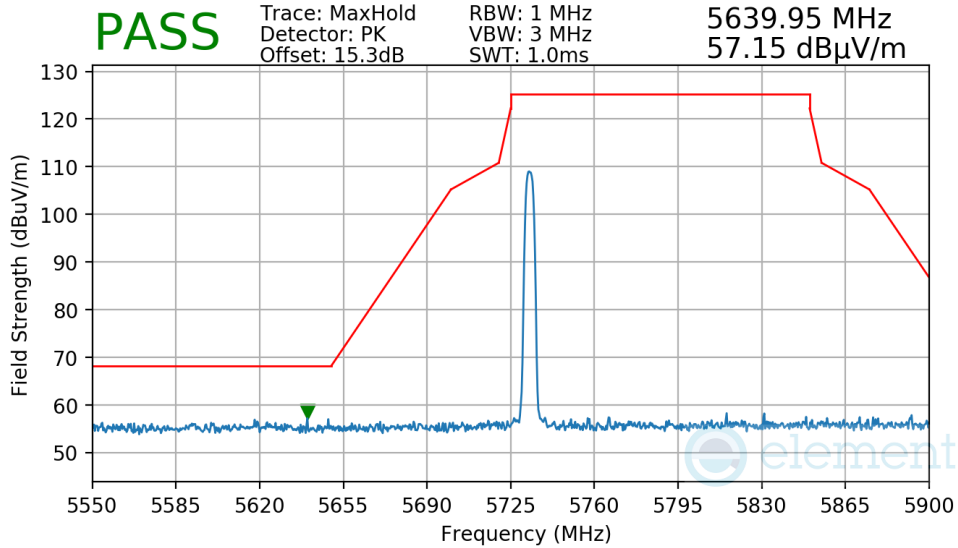
Plot 7-218. Radiated Lower Band Edge Measurement Antenna WF7
