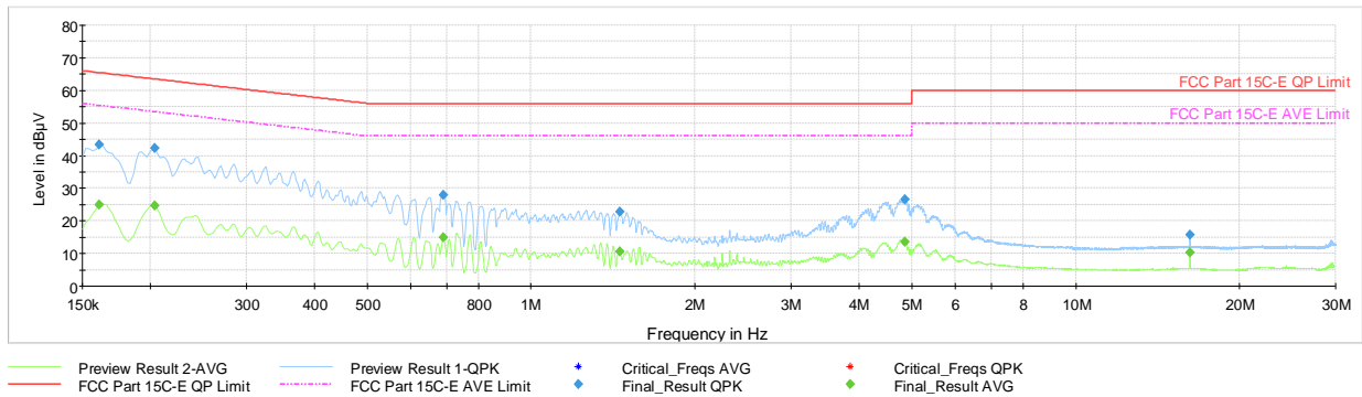
Plot 7-229. AC Line Conducted Plot TxBF (HDR4, ePA – 5245MHz) (L1) with AC/DC Adapter
