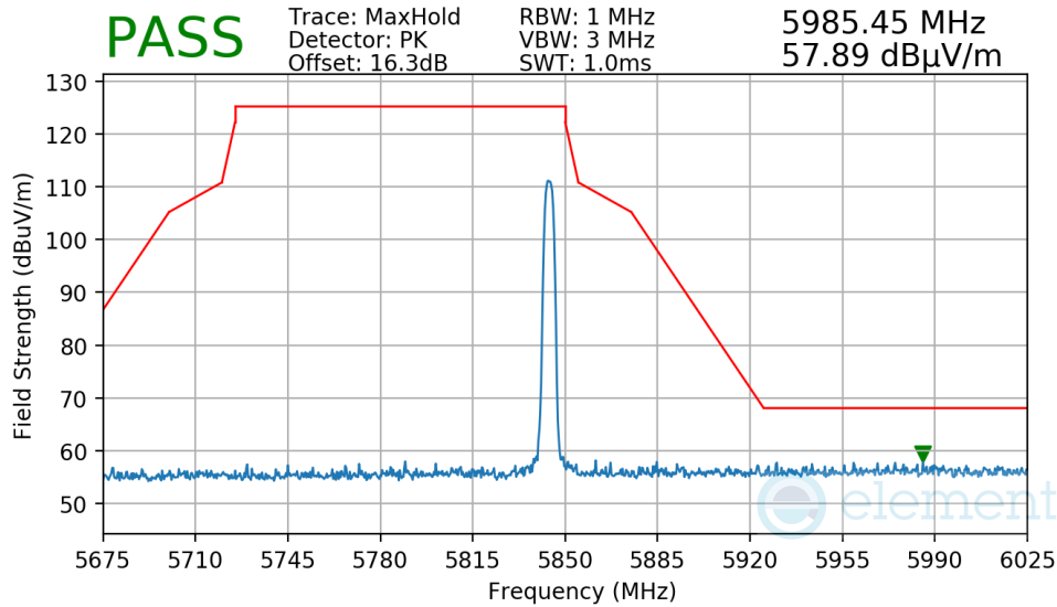
Plot 7-214. Radiated Upper Band Edge Measurement Antenna WF8
