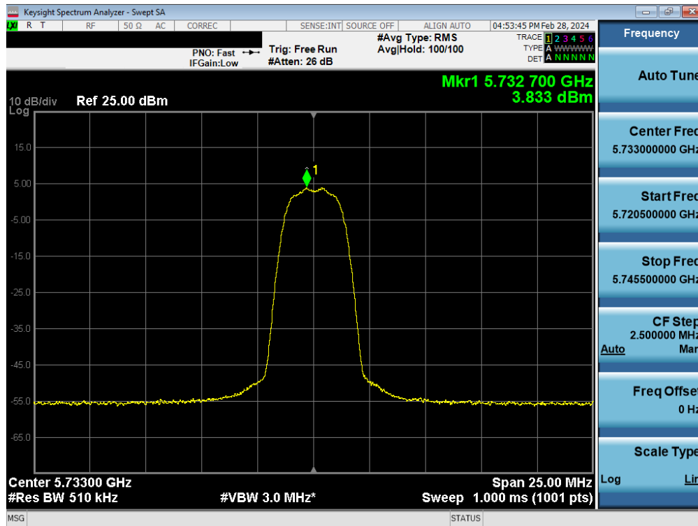
Plot 7-106. PSD Antenna WF7 (HDR4, ePA 5733MHz)
