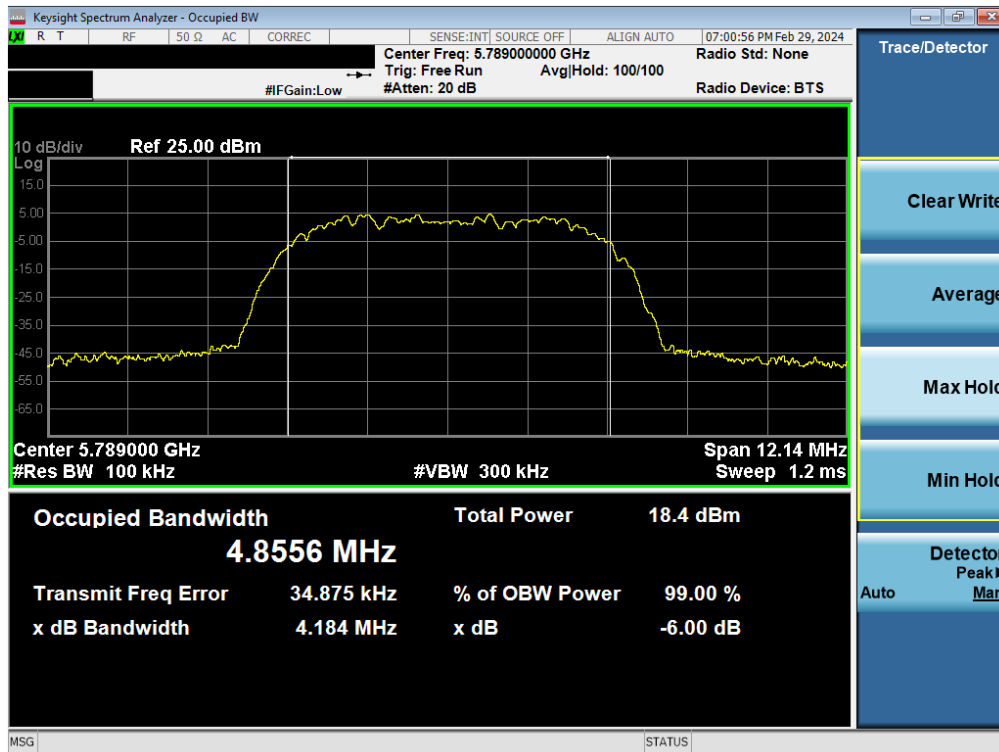
Plot 7-35. 6dB BW & 99% OBW Antenna WF7 (HDR8, ePA, 5789MHz)
