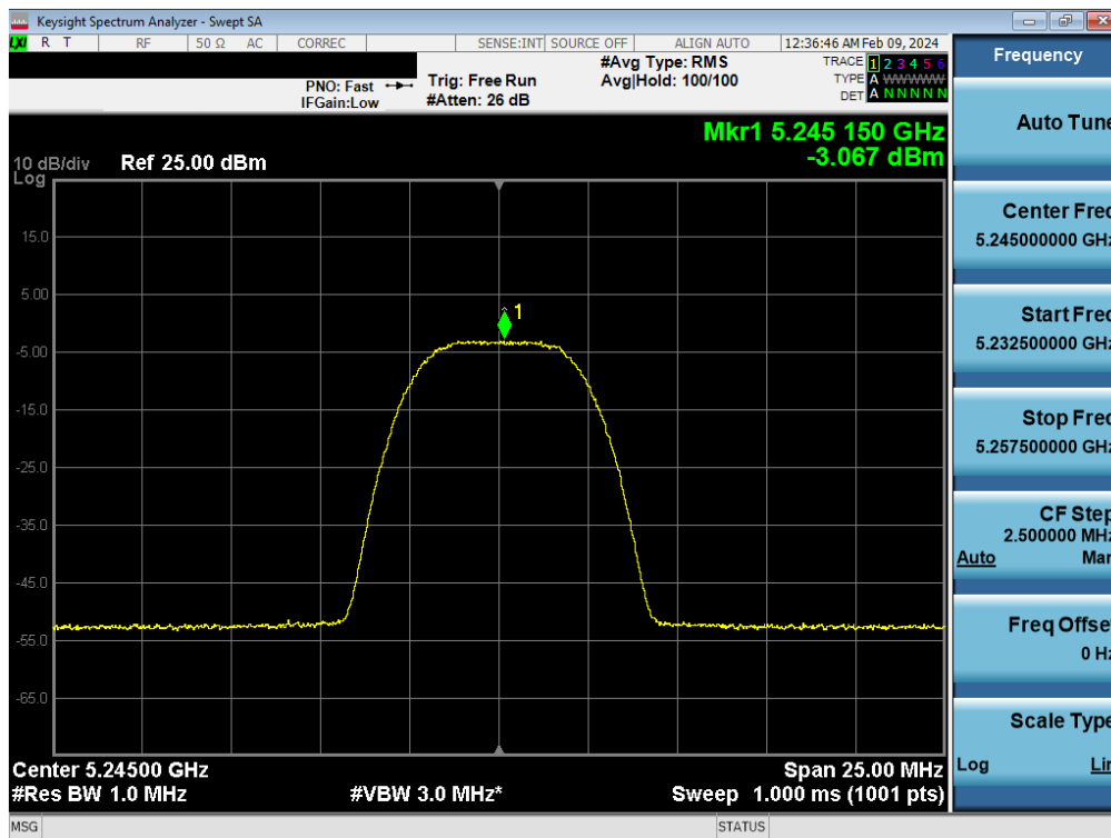
Plot 7-105. PSD Antenna WF7 (HNR8, iPA– 5245MHz)
