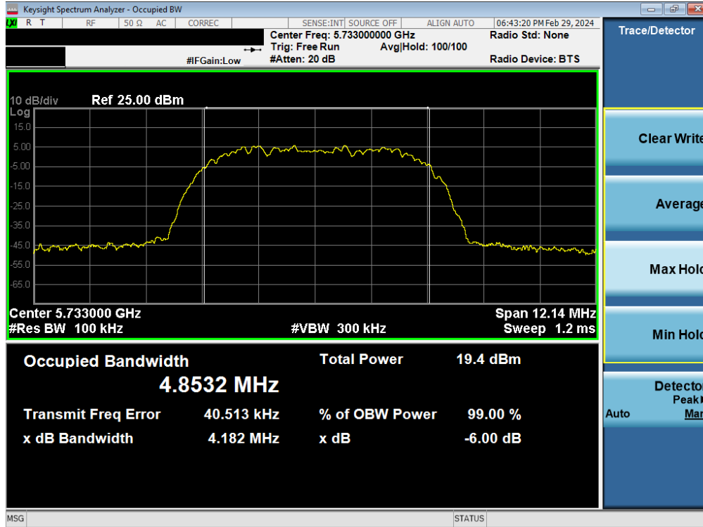
Plot 7-28. 6dB BW & 99% OBW Antenna WF8 (HDR8, ePA, 5733MHz)
