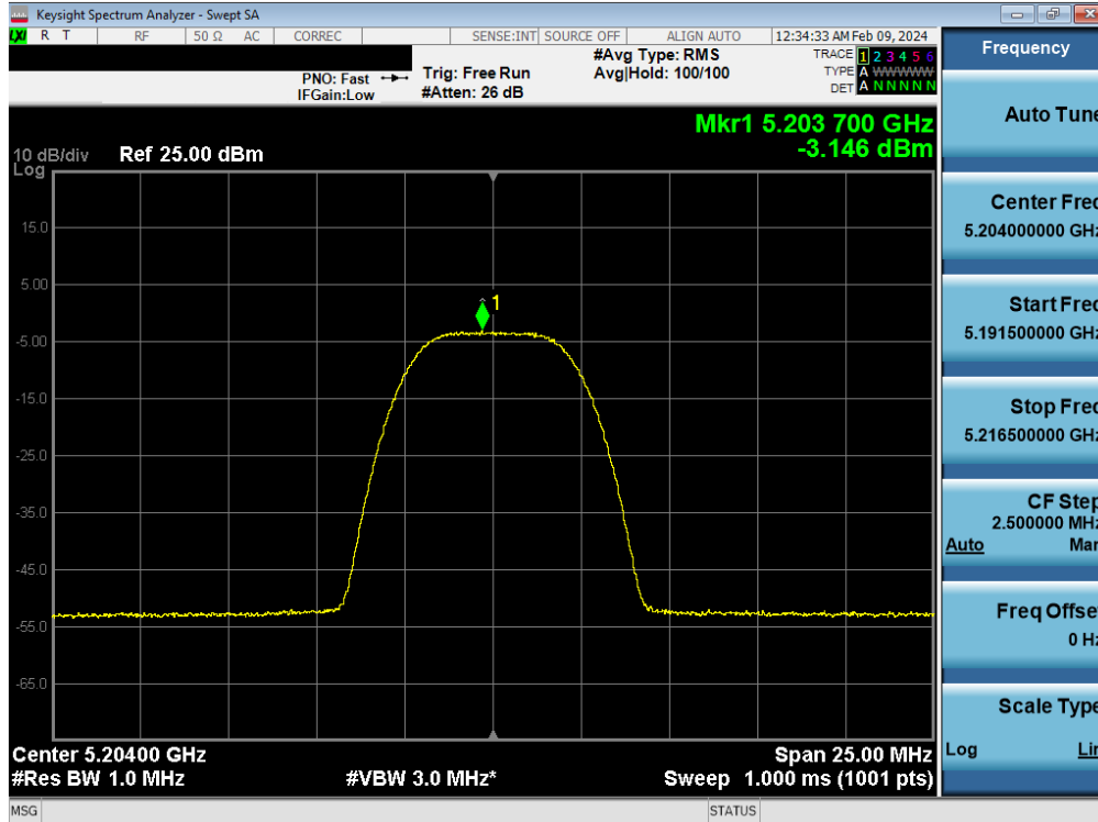
Plot 7-104. PSD Antenna WF7 (HNR8, iPA – 5204MHz)
