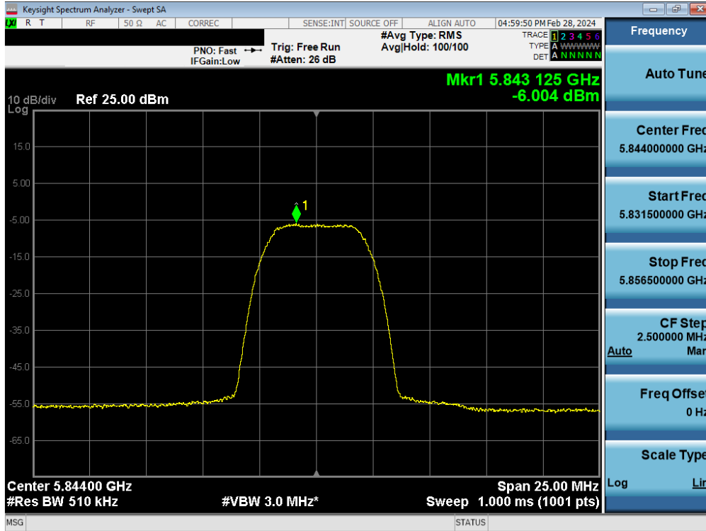
Plot 7-117. PSD Antenna WF7 (HDR8, iPA 5844MHz)
