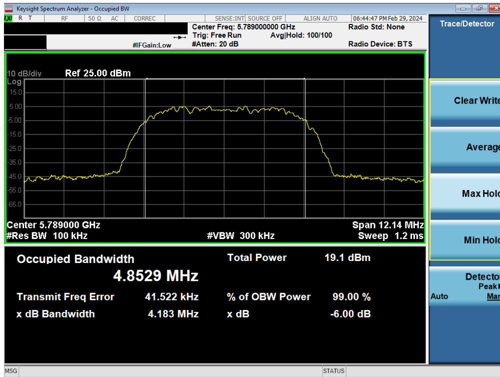
Plot 7-29. 6dB BW & 99% OBW Antenna WF8 (HDR8, ePA, 5789MHz)
