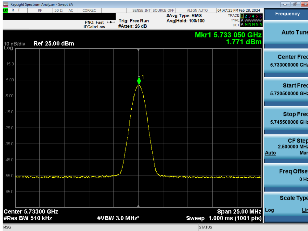
Plot 7-58. PSD Antenna WF7 (BDR, iPA 5733MHz)
