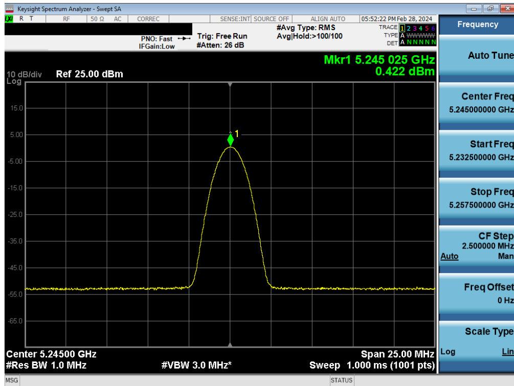
Plot 7-84. ISED PSD TxBF Antenna WF8 (BDR, iPA- 5245MHz)
