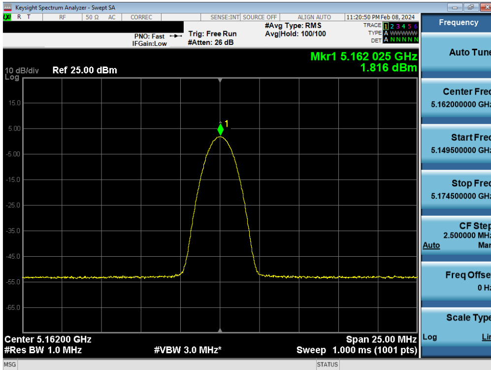
Plot 7-37. FCC/ISED PSD Antenna WF8 (BDR, iPA – 5162MHz)
