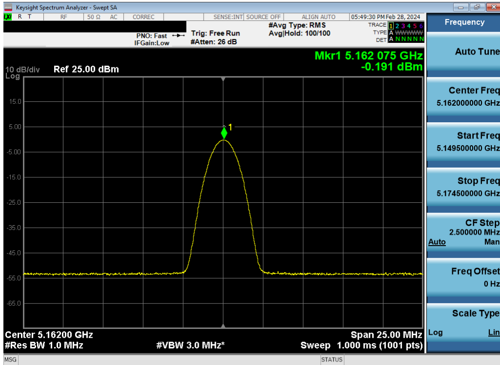
Plot 7-74. ISED PSD TxBF Antenna WF8 (BDR, ePA – 5162MHz)
