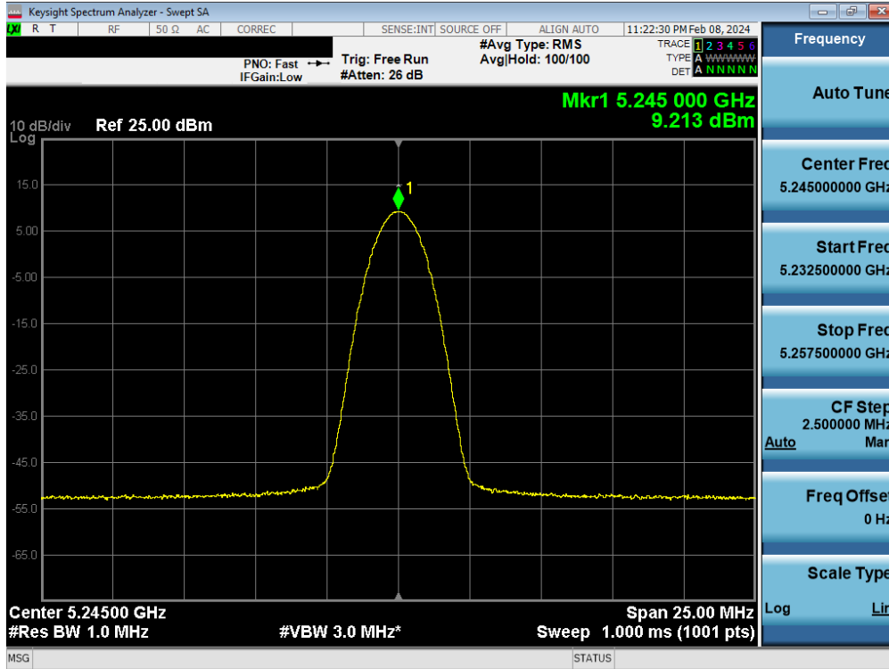
Plot 7-36. FCC PSD Antenna WF8 (BDR, ePA– 5245MHz)
