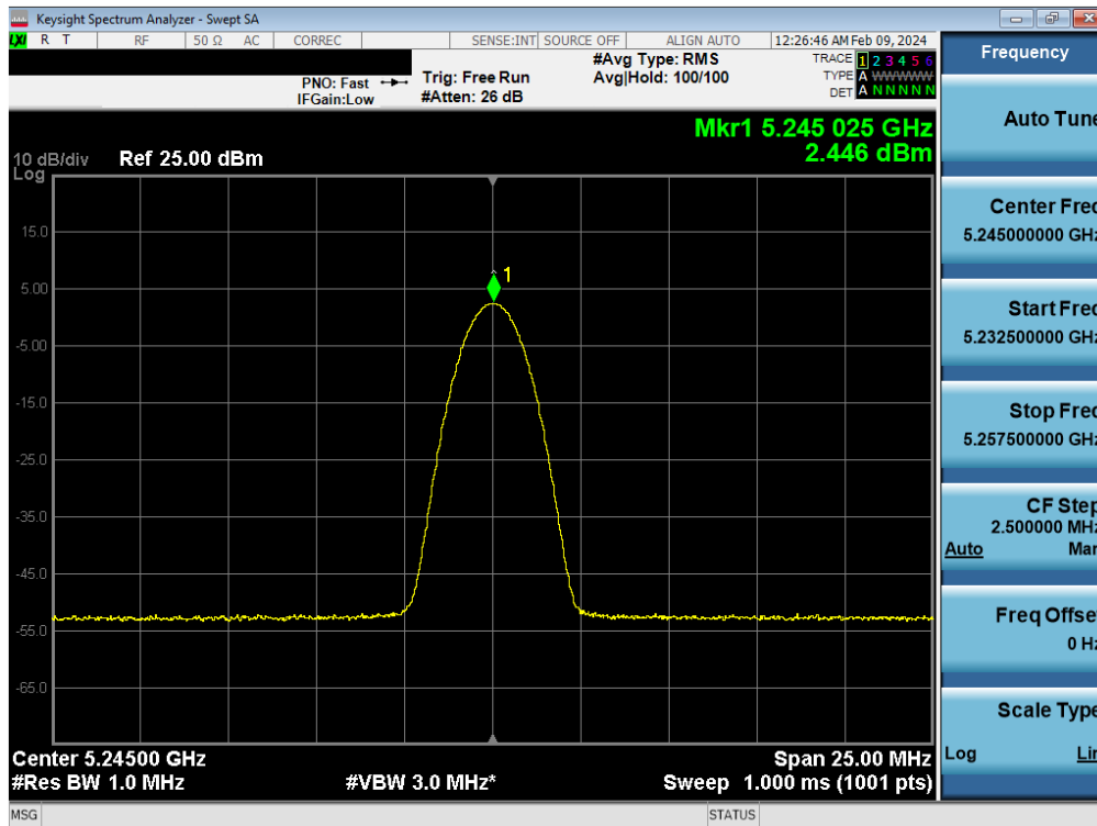
Plot 7-54. FCC/ISED PSD Antenna WF7 (BDR, iPA– 5245MHz)
