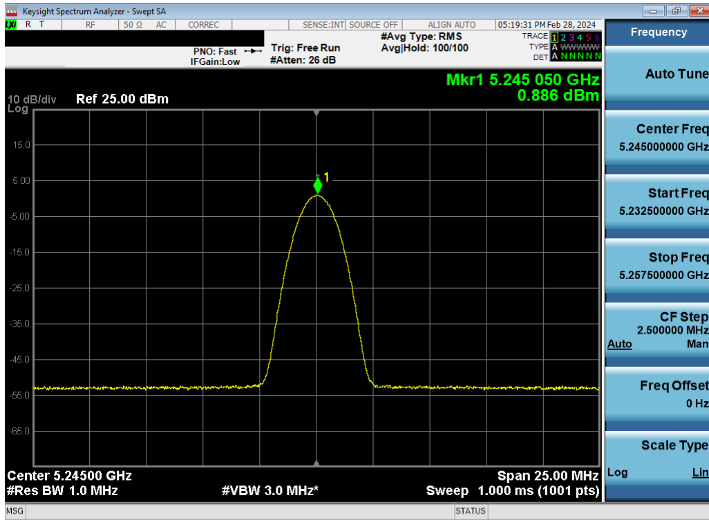
Plot 7-83. ISED PSD TxBF Antenna WF5B (BDR, iPA- 5245MHz)
