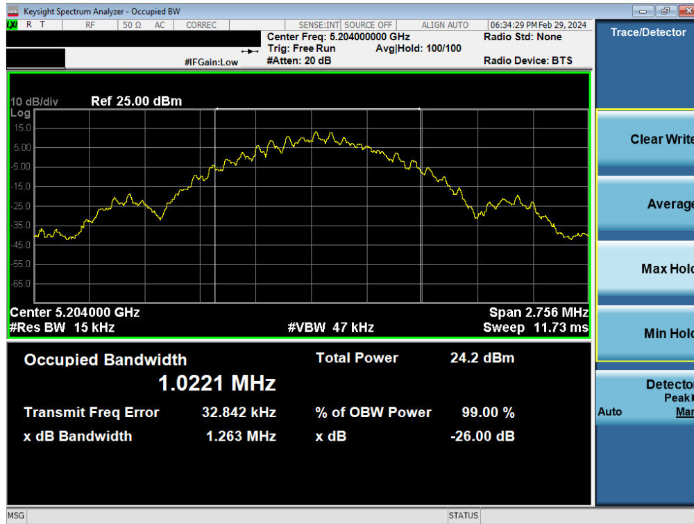
Plot 7-5. 26dB BW & 99% OBW Antenna WF8 (BDR GFSK, ePA- 5204MHz)
