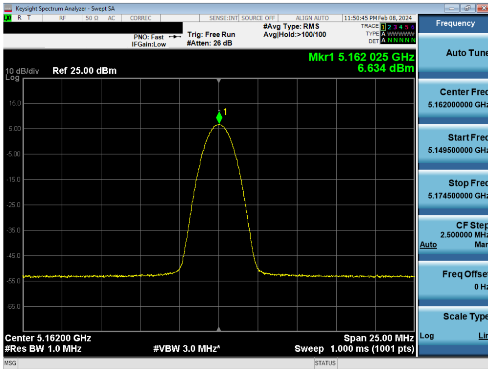
Plot 7-62. FCC PSD TxBF Antenna WF8 (BDR, ePA – 5162MHz)
