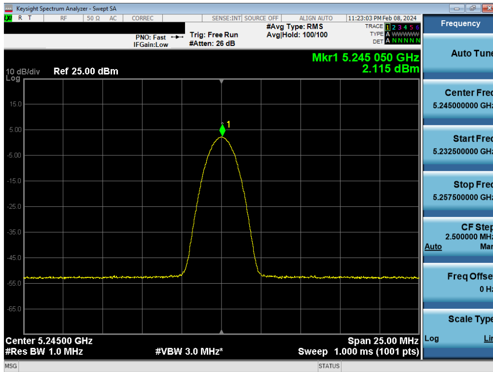
Plot 7-39. FCC/ISED PSD Antenna WF8 (BDR, iPA– 5245MHz)
