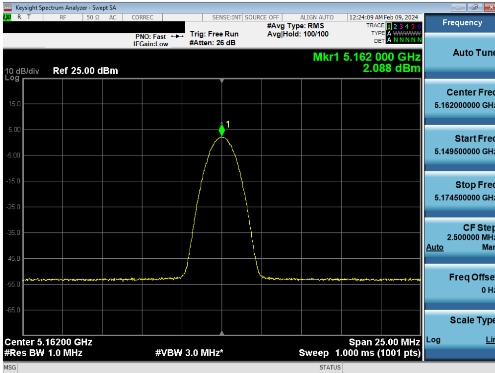
Plot 7-52. FCC/ISED PSD Antenna WF7 (BDR, iPA - 5162MHz)
