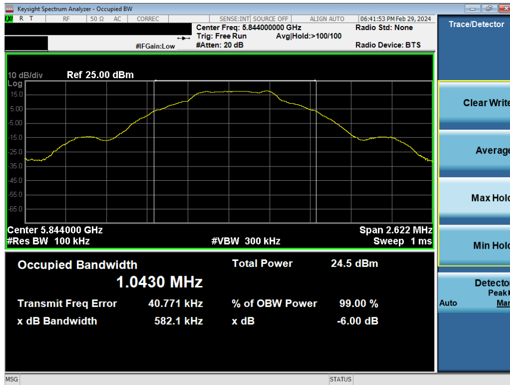
Plot 7-15. 6dB BW & 99% OBW Antenna WF8 (BDR GFSK, 5844MHz)
