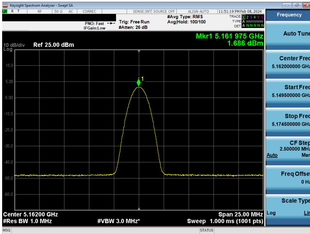
Plot 7-68. FCC PSD TxBF Antenna WF8 (BDR, iPA – 5162MHz)
