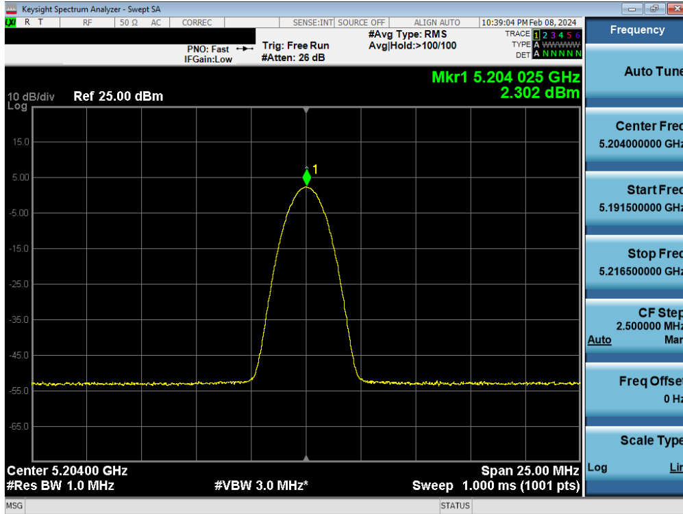
Plot 7-69. FCC PSD TxBF Antenna WF5B (BDR, iPA – 5204MHz)
