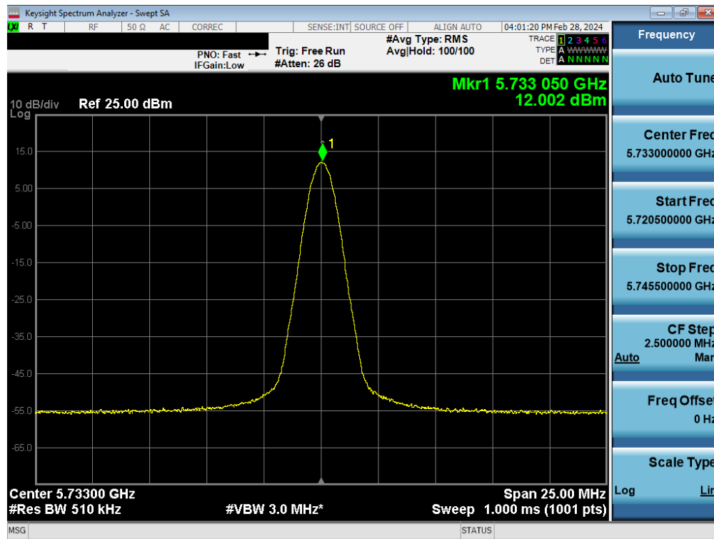
Plot 7-85. PSD TxBF Antenna WF5B (BDR, ePA 5733MHz)
