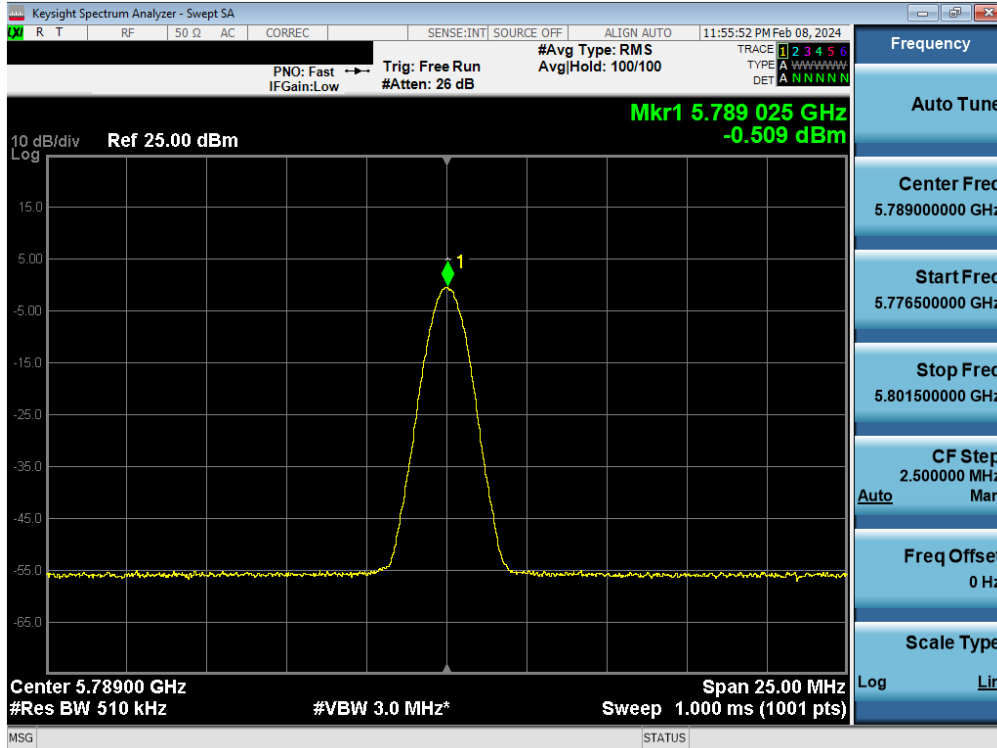
Plot 7-94. PSD TxBF Antenna WF8 (BDR, iPA 5789MHz)
