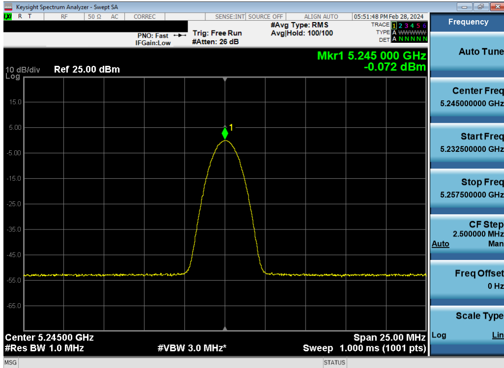
Plot 7-78. ISED PSD TxBF Antenna WF8 (BDR, ePA- 5245MHz)
