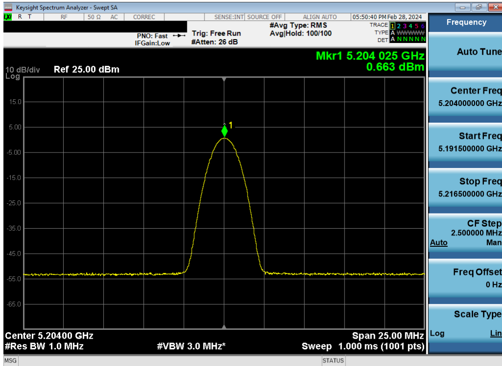
Plot 7-76. ISED PSD TxBF Antenna WF8 (BDR, ePA – 5204MHz)
