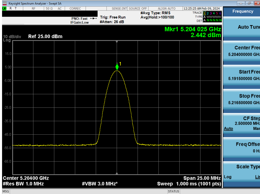
Plot 7-53. FCC/ISED PSD Antenna WF7 (BDR, iPA – 5204MHz)
