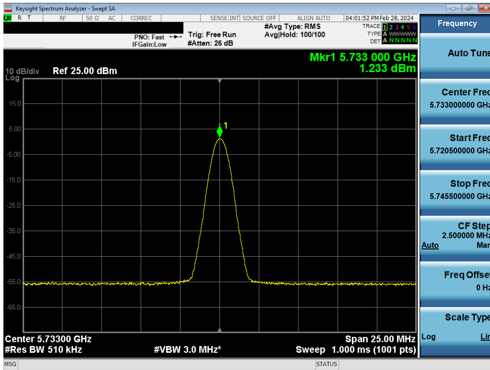
Plot 7-91. PSD TxBF Antenna WF5B (BDR, iPA 5733MHz)
