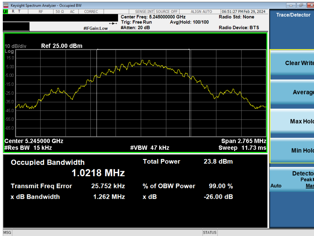
Plot 7-9. 26dB BW & 99% OBW Antenna WF8 (BDR GFSK, ePA - 5245MHz)
