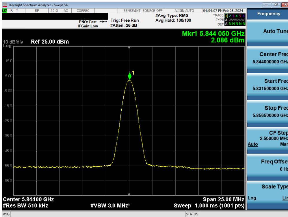
Plot 7-95. PSD TxBF Antenna WF5B (BDR, iPA 5844MHz)
