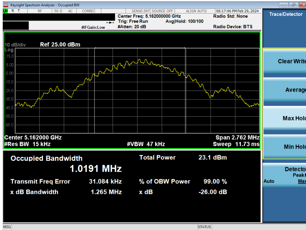
Plot 7-1. 26dB BW & 99% OBW Antenna WF5B (BDR GFSK, ePA– 5162MHz)
