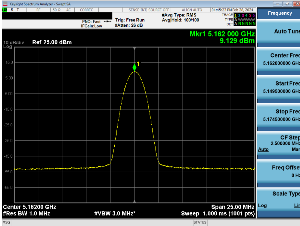
Plot 7-49. FCC/ISED PSD Antenna WF7 (BDR, ePA – 5162MHz)
