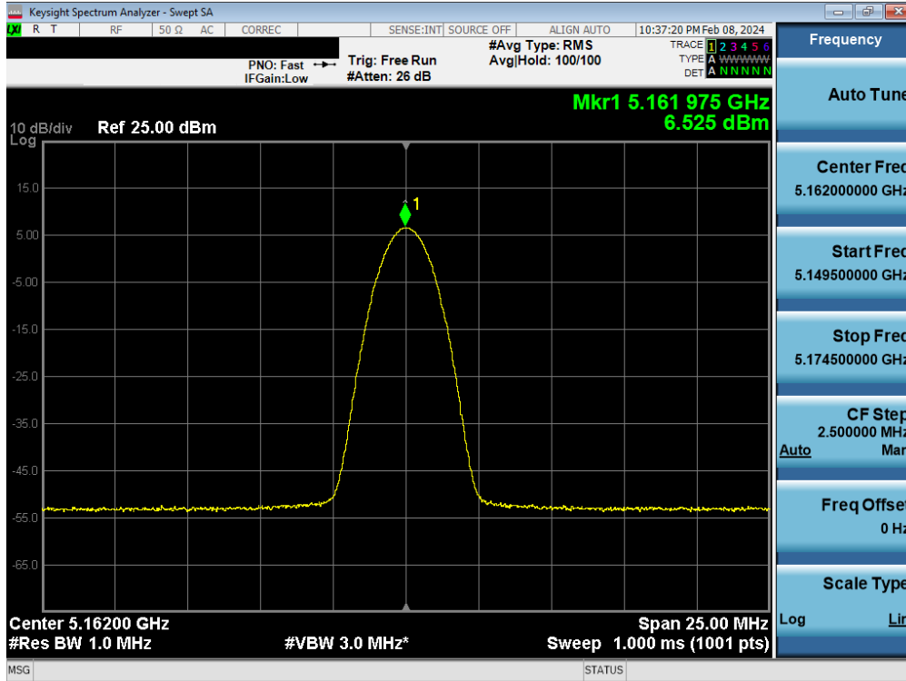
Plot 7-61. FCC PSD TxBF Antenna WF5B (BDR, ePA – 5162MHz)
