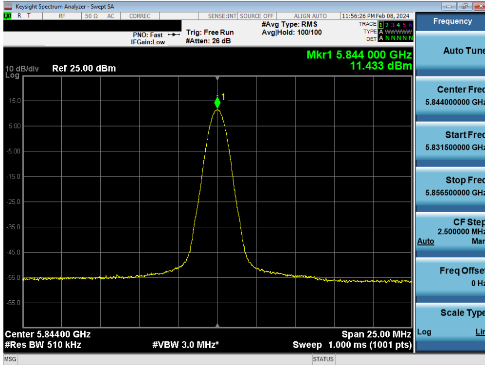
Plot 7-90. PSD TxBF Antenna WF8 (BDR, ePA 5844MHz)
