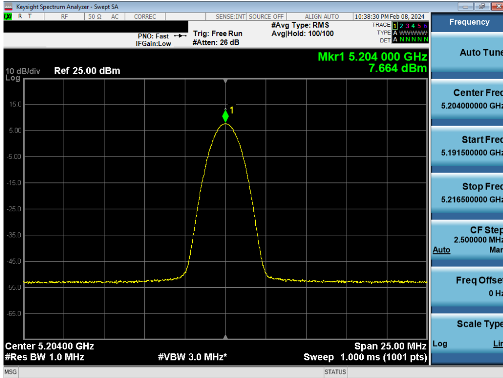
Plot 7-63. FCC PSD TxBF Antenna WF5B (BDR, ePA – 5204MHz)
