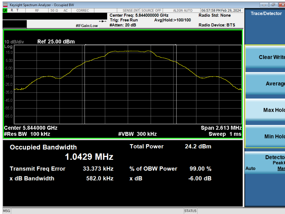
Plot 7-18. 6dB BW & 99% OBW Antenna WF7 (BDR GFSK, 5844MHz)
