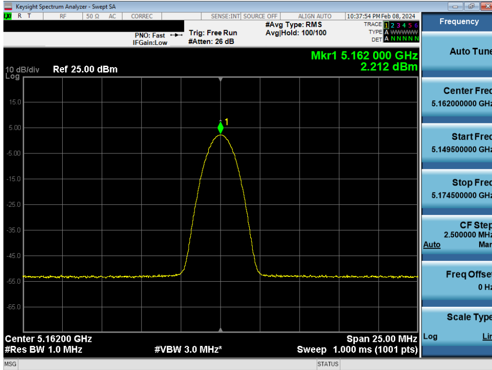
Plot 7-67. FCC PSD TxBF Antenna WF5B (BDR, iPA – 5162MHz)
