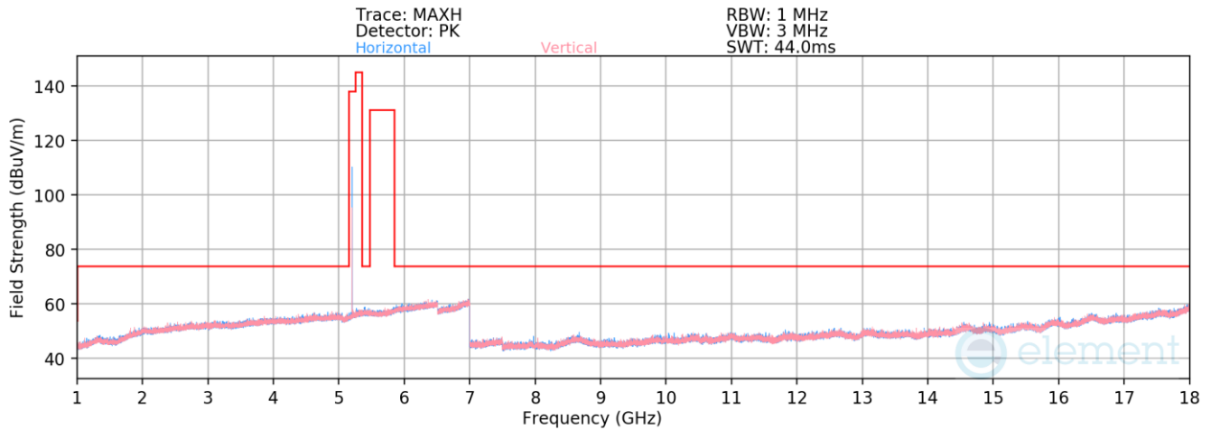
Plot 7-98. Radiated Spurious Emissions 1-18GHz Antenna WF5B (BDR GFSK ePA – 5204MHz)
