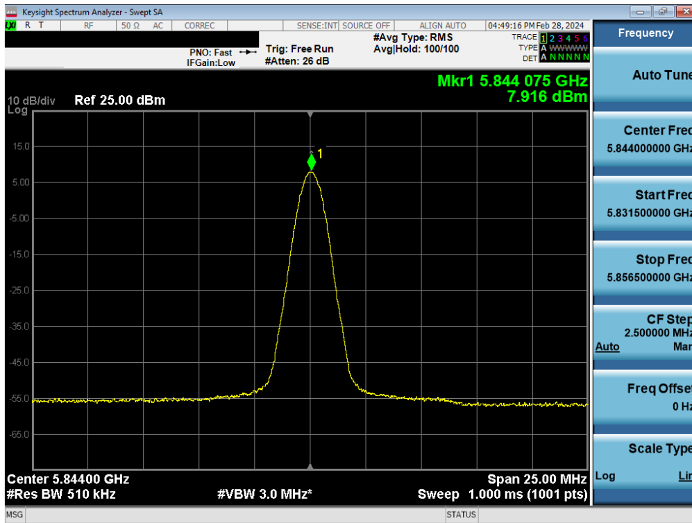
Plot 7-57. PSD Antenna WF7 (BDR, ePA 5844MHz)
