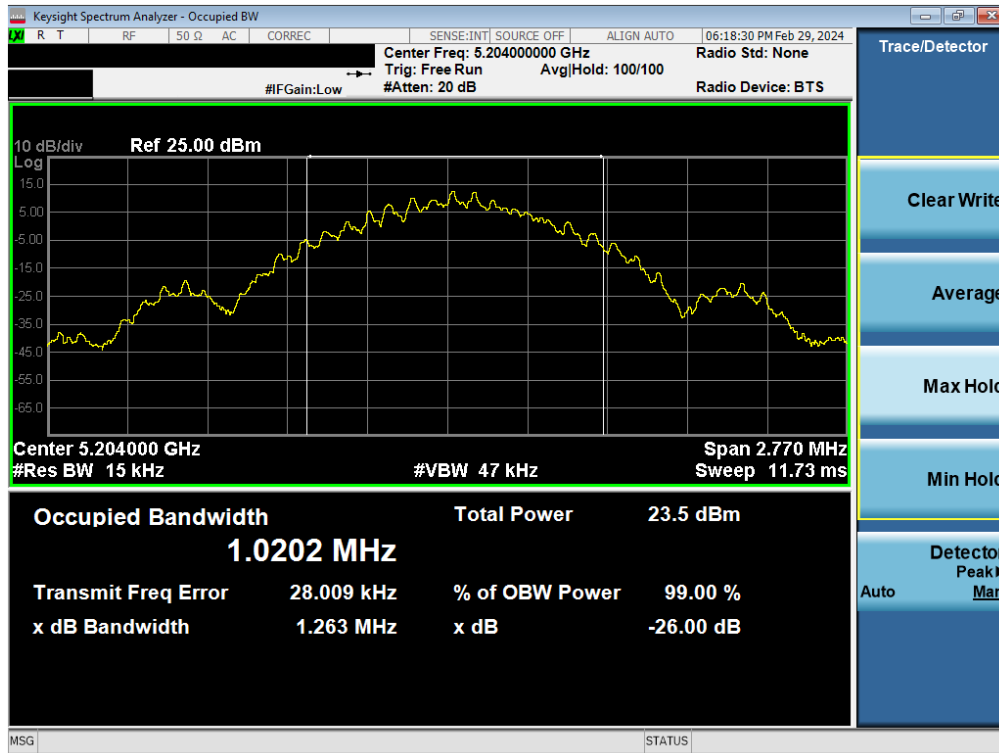
Plot 7-2. 26dB BW & 99% OBW Antenna WF5B (BDR GFSK, ePA- 5204MHz)
