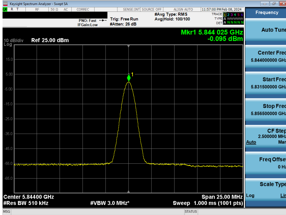
Plot 7-96. PSD TxBF Antenna WF8 (BDR, iPA 5844MHz)
