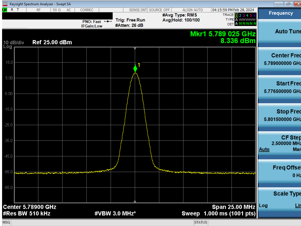
Plot 7-44. PSD Antenna WF8 (BDR, ePA 5789MHz)
