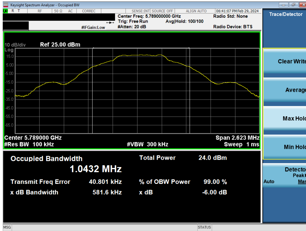
Plot 7-14. 6dB BW & 99% OBW Antenna WF8 (BDR GFSK, 5789MHz)
