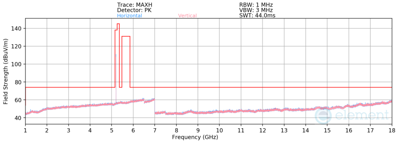
Plot 7-104. Radiated Spurious Emissions 1-18GHz Antenna WF8 (BDR GFSK ePA – 5204MHz)
