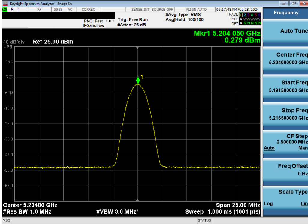
Plot 7-75. ISED PSD TxBF Antenna WF5B (BDR, ePA – 5204MHz)
