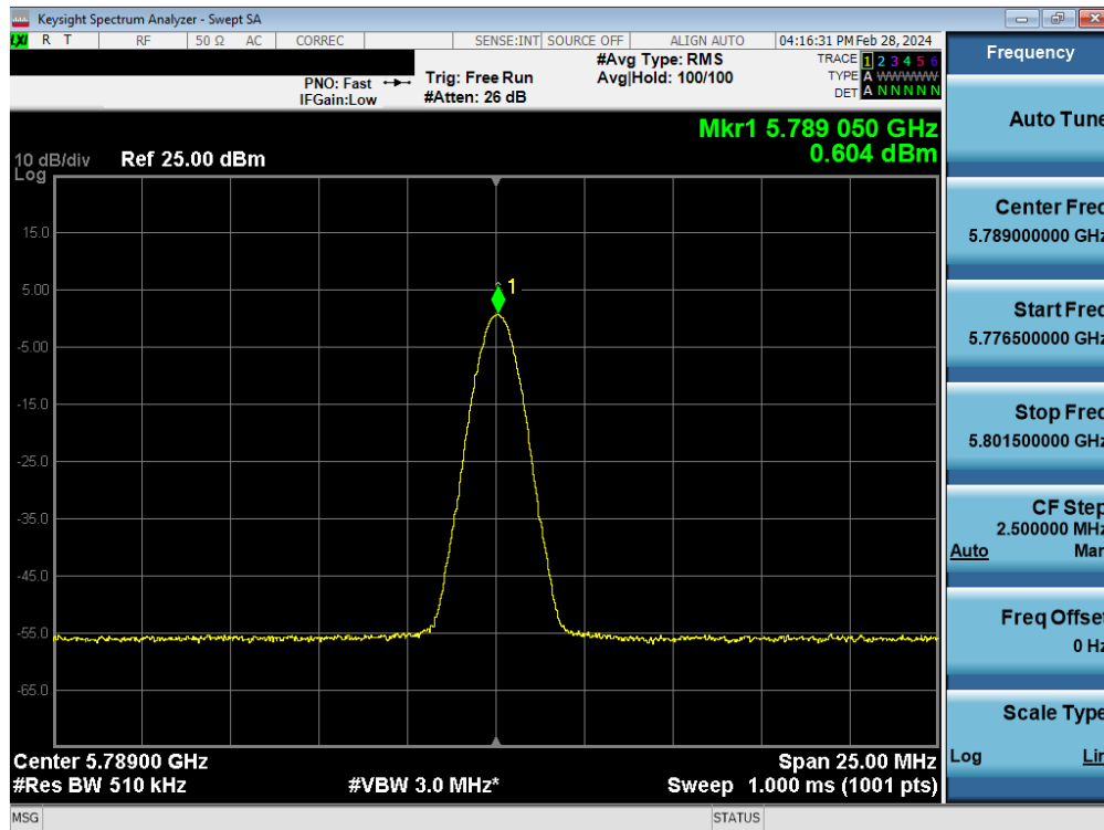
Plot 7-47. PSD Antenna WF8 (BDR, iPA 5789MHz)
