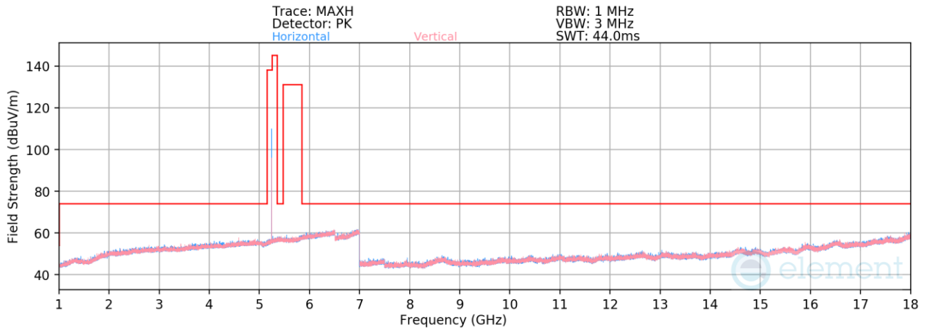
Plot 7-99. Radiated Spurious Emissions 1-18GHz Antenna WF5B (BDR GFSK ePA – 5245MHz)
