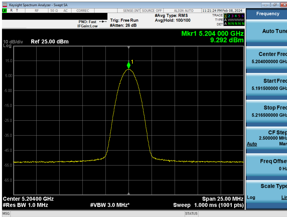
Plot 7-35. FCC PSD Antenna WF8 (BDR, ePA – 5204MHz)
