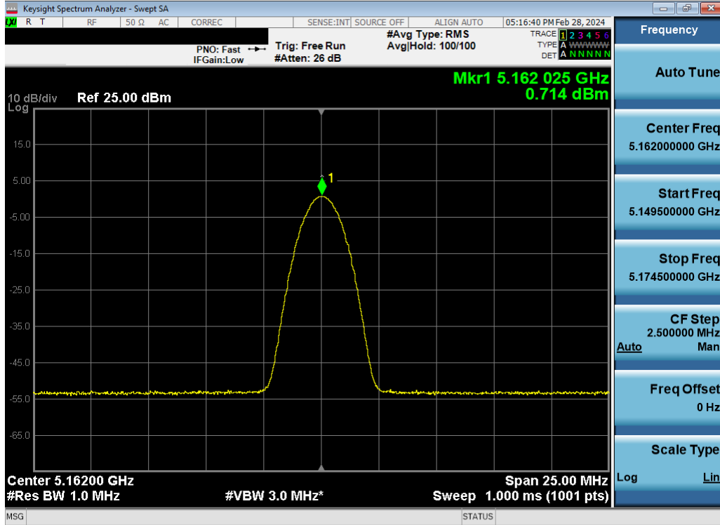
Plot 7-73. ISED PSD TxBF Antenna WF5B (BDR, ePA – 5162MHz)
