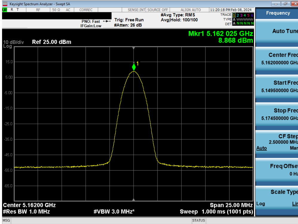
Plot 7-34. FCC PSD Antenna WF8 (BDR, ePA – 5162MHz)
