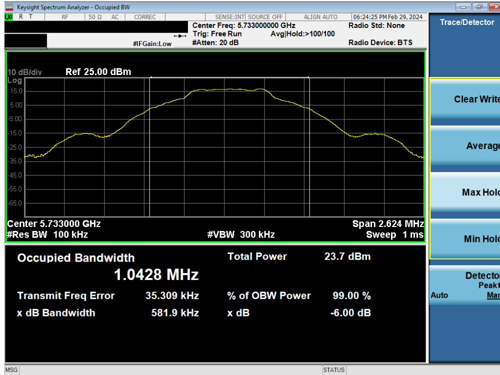
Plot 7-10. 6dB BW & 99% OBW Antenna WF5B (BDR GFSK, 5733MHz)
