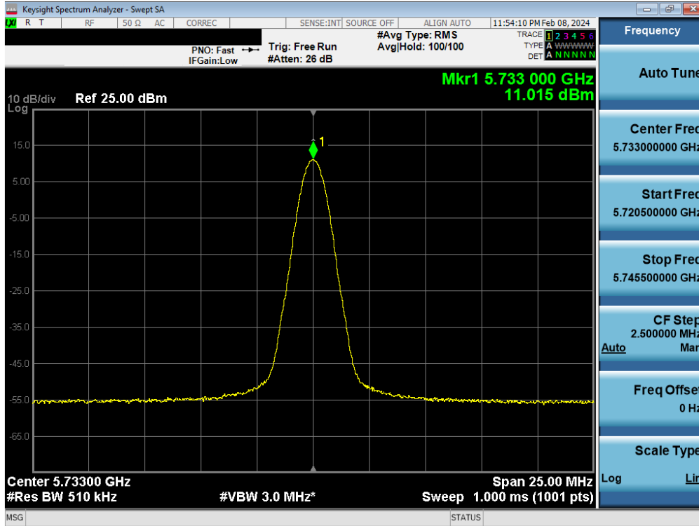
Plot 7-86. PSD TxBF Antenna WF8 (BDR, ePA 5733MHz)
