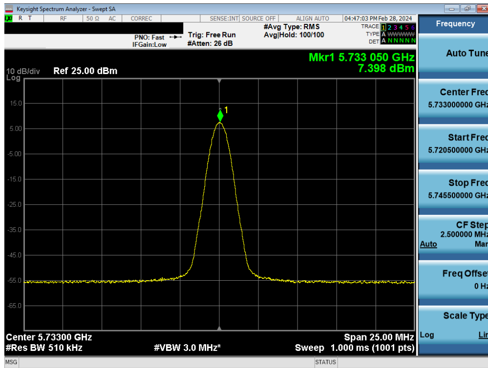
Plot 7-55. PSD Antenna WF7 (BDR, ePA 5733MHz)
