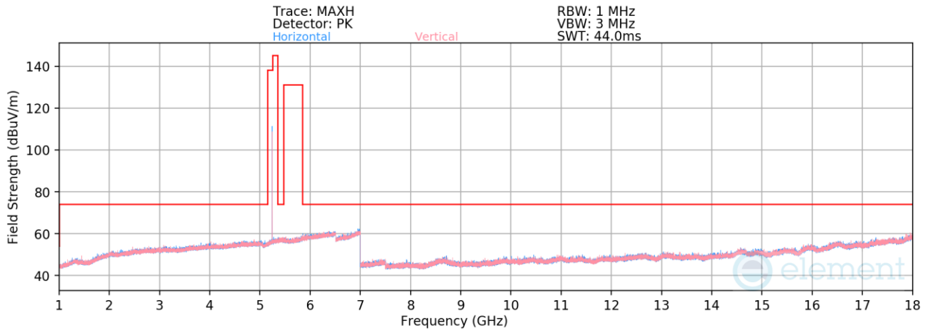
Plot 7-105. Radiated Spurious Emissions 1-18GHz Antenna WF8 (BDR GFSK ePA – 5245MHz)
