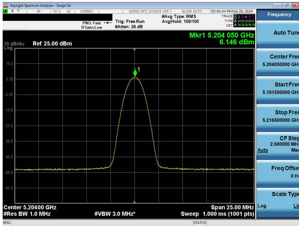
Plot 7-41. ISED PSD Antenna WF8 (BDR, ePA – 5204MHz)
