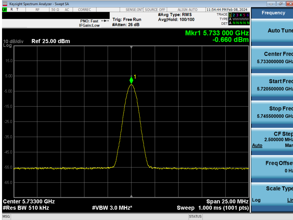
Plot 7-92. PSD TxBF Antenna WF8 (BDR, iPA 5733MHz)
