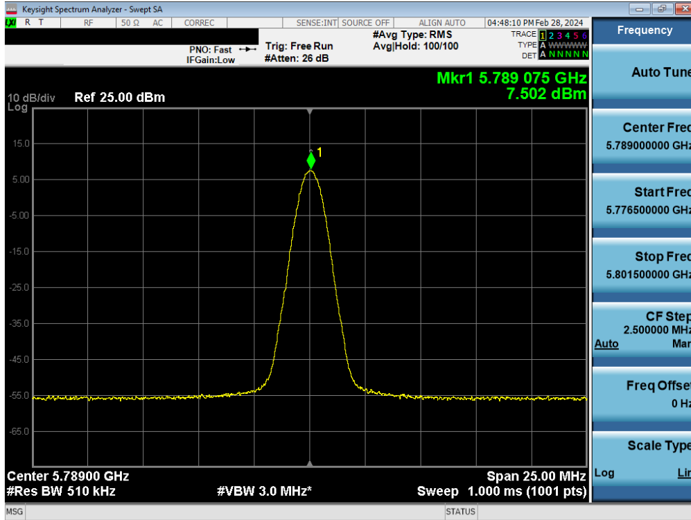
Plot 7-56. PSD Antenna WF7 (BDR, ePA 5789MHz)
