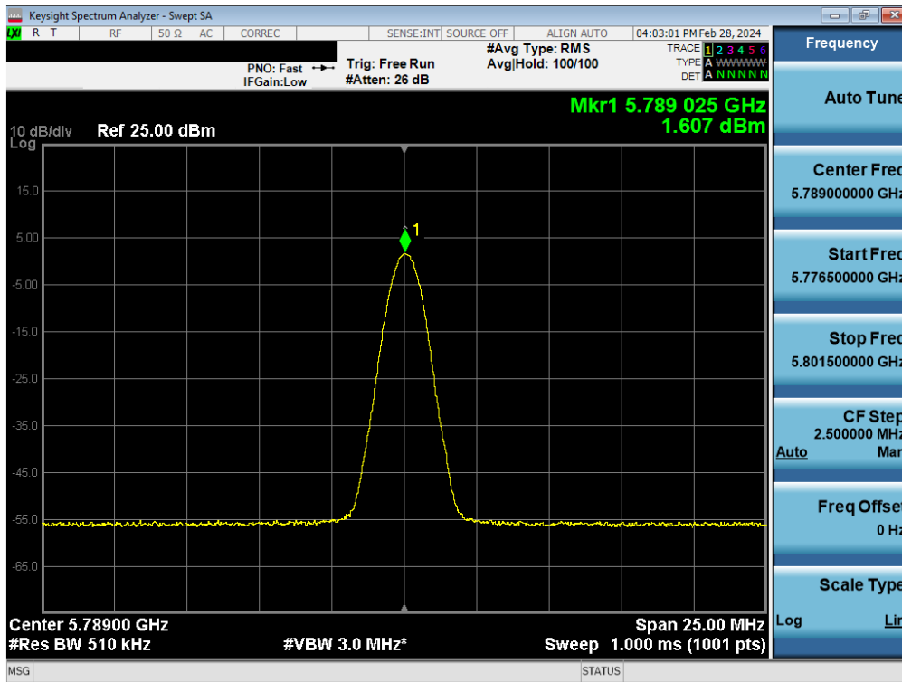
Plot 7-93. PSD TxBF Antenna WF5B (BDR, iPA 5789MHz)
