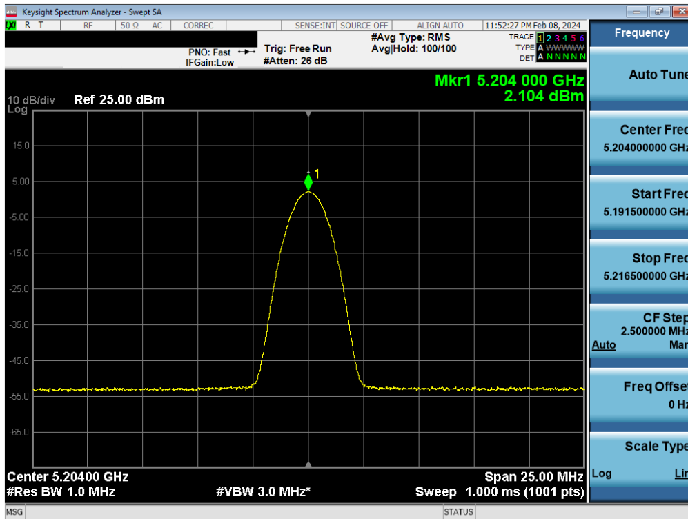
Plot 7-70. FCC PSD TxBF Antenna WF8 (BDR, iPA – 5204MHz)
