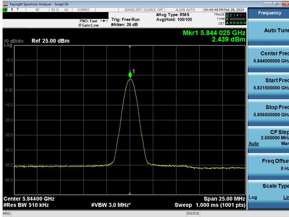
Plot 7-60. PSD Antenna WF7 (BDR, iPA 5844MHz)
