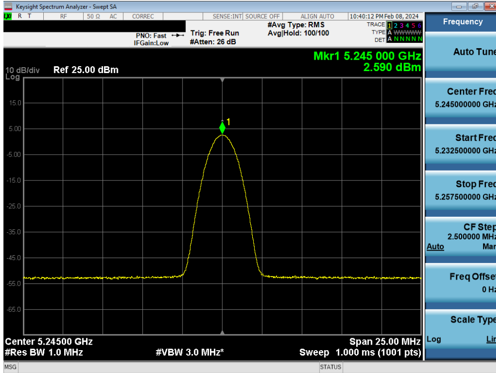
Plot 7-71. FCC PSD TxBF Antenna WF5B (BDR, iPA- 5245MHz)
