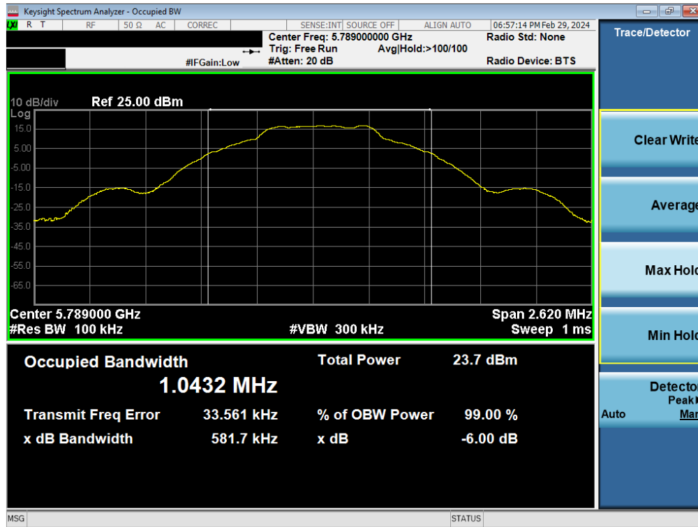
Plot 7-17. 6dB BW & 99% OBW Antenna WF7 (BDR GFSK, 5789MHz)
