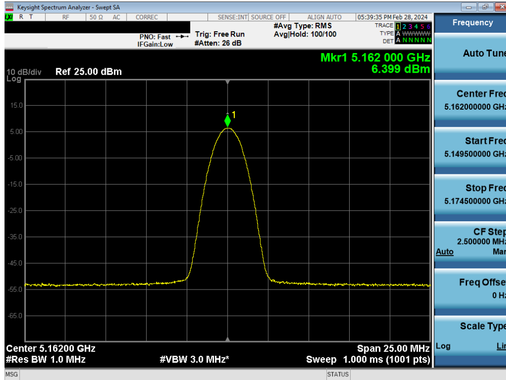
Plot 7-40. ISED PSD Antenna WF8 (BDR, ePA – 5162MHz)
