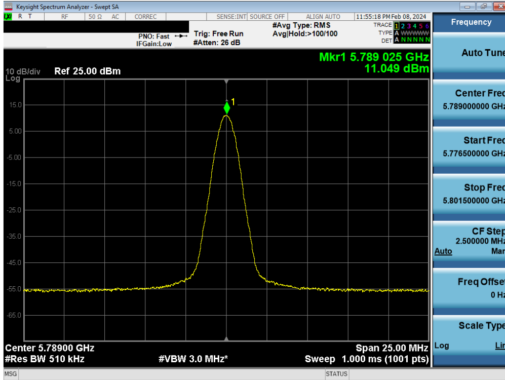
Plot 7-88. PSD TxBF Antenna WF8 (BDR, ePA 5789MHz)
