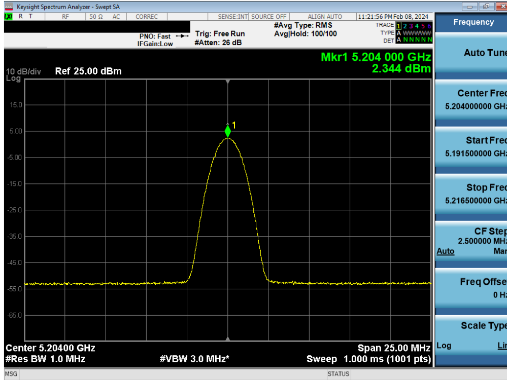
Plot 7-38. FCC/ISED PSD Antenna WF8 (BDR, iPA – 5204MHz)
