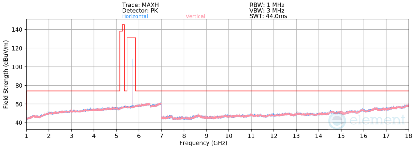
Plot 7-100. Radiated Spurious Emissions 1-18GHz Antenna WF5B (BDR GFSK ePA – 5733MHz)
