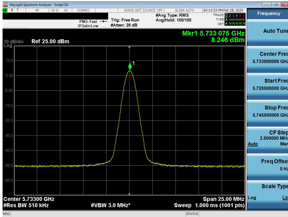
Plot 7-43. PSD Antenna WF8 (BDR, ePA 5733MHz)
