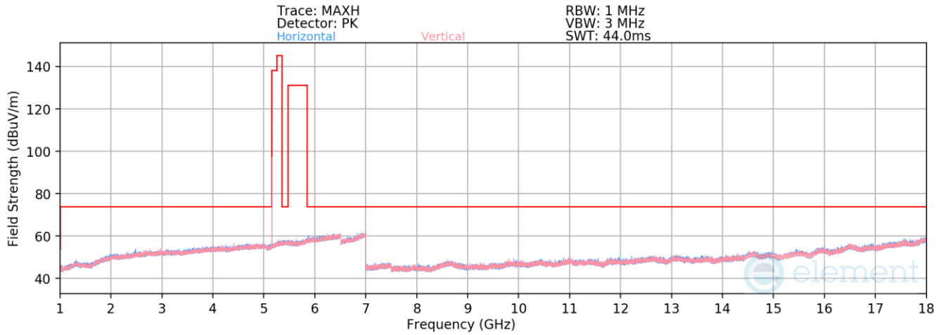
Plot 7-97. Radiated Spurious Emissions 1-18GHz Antenna WF5B (BDR GFSK ePA – 5162MHz)
