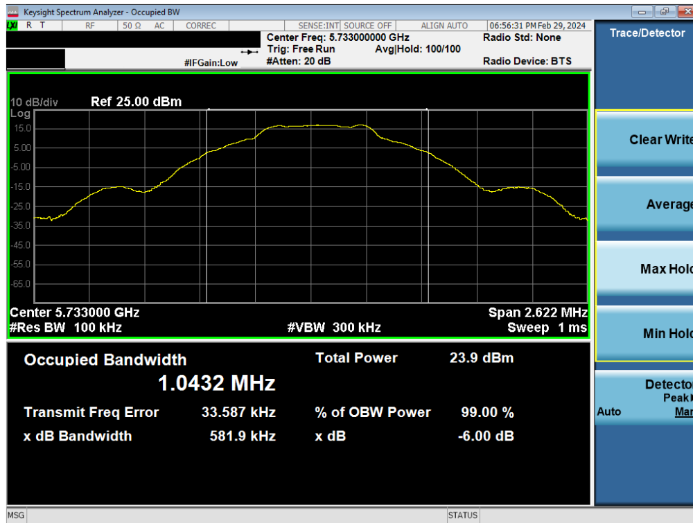
Plot 7-16. 6dB BW & 99% OBW Antenna WF7 (BDR GFSK, 5733MHz)
