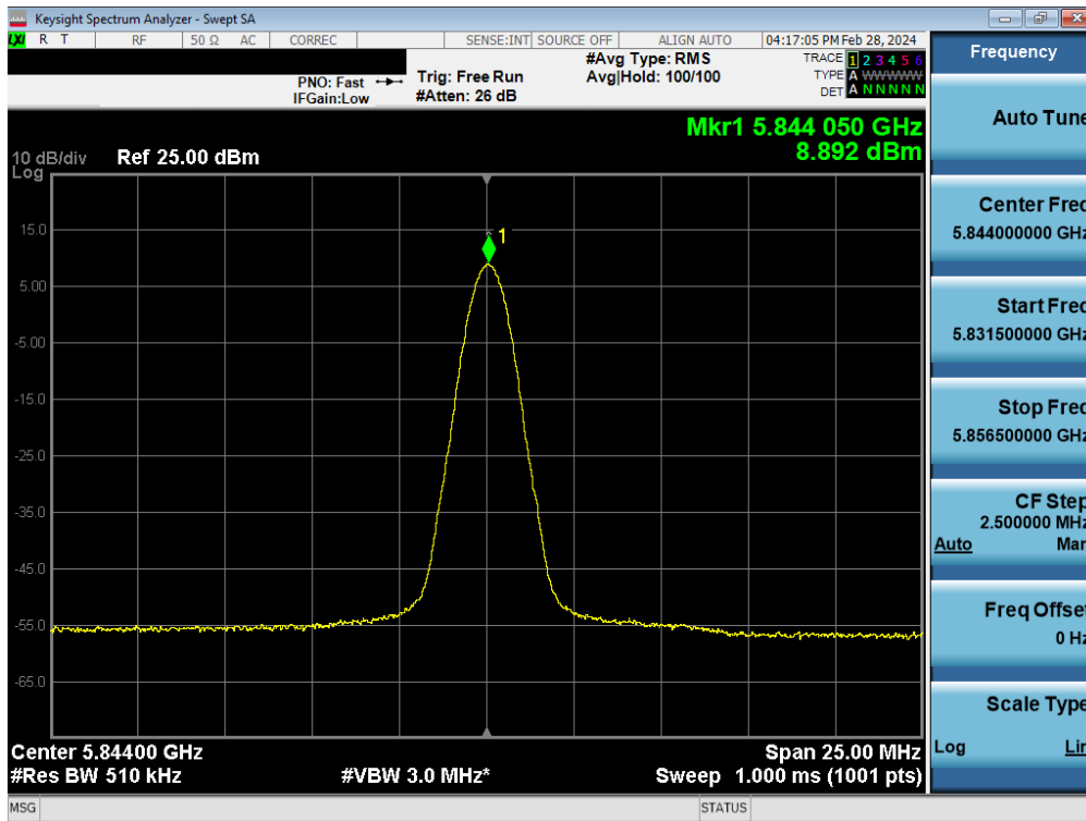
Plot 7-45. PSD Antenna WF8 (BDR, ePA 5844MHz)
