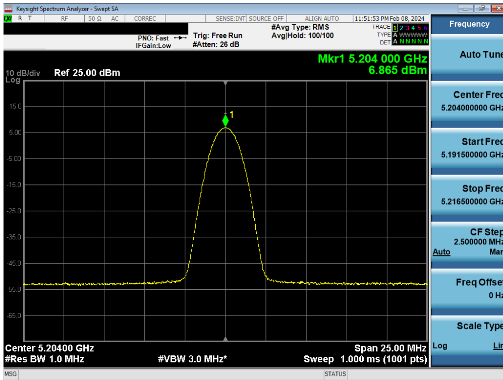
Plot 7-64. FCC PSD TxBF Antenna WF8 (BDR, ePA – 5204MHz)
