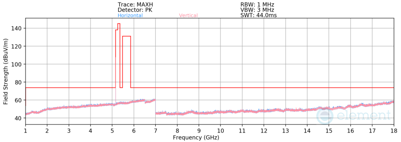
Plot 7-103. Radiated Spurious Emissions 1-18GHz Antenna WF8 (BDR GFSK ePA – 5162MHz)
