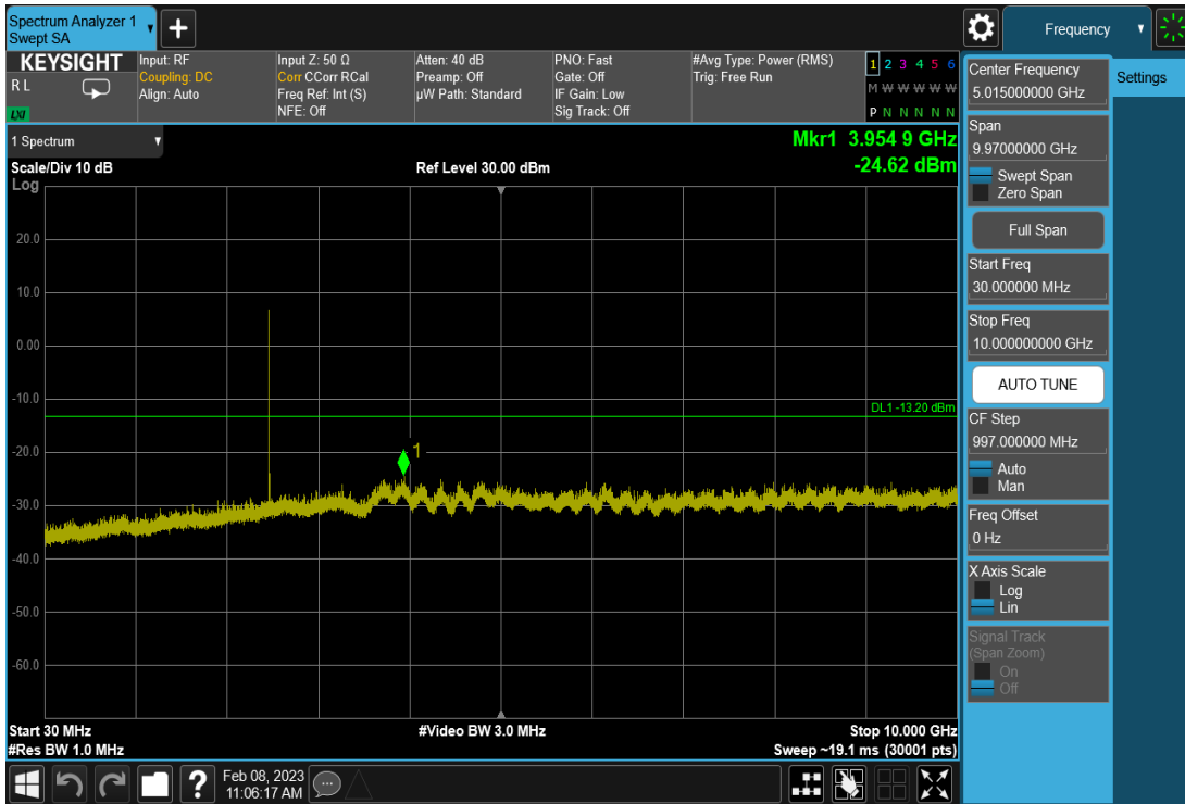
Plot 7-21. Conducted Spurious Plot (Bluetooth (LE), 1Mbps – Ch. 39)
