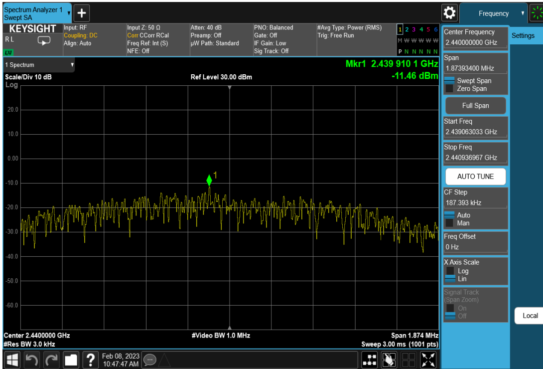
Plot 7-11. Power Spectral Density Plot (Bluetooth (LE), 2Mbps – Ch. 19)
