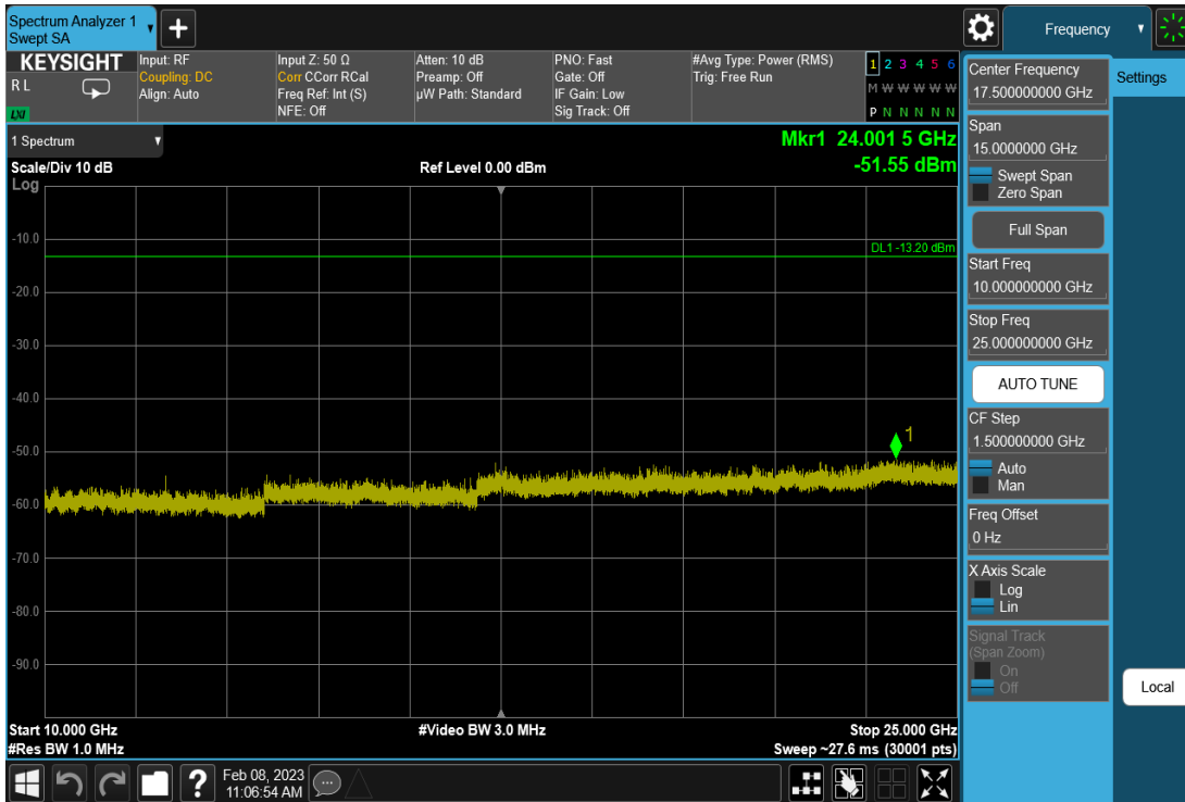
Plot 7-22. Conducted Spurious Plot (Bluetooth (LE), 1Mbps – Ch. 39)
