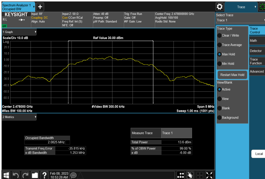
Plot 7-6. 6dB BW & 99% OBW Plot (Bluetooth (LE), 2Mbps – Ch. 38)
