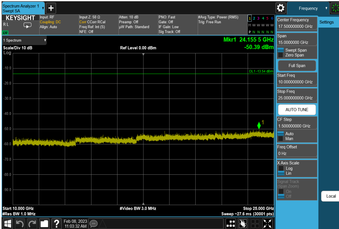
Plot 7-20. Conducted Spurious Plot (Bluetooth (LE), 1Mbps – Ch. 19)
