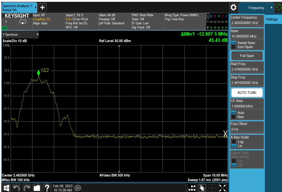
Plot 7-16. Band Edge Plot (Bluetooth (LE), 2Mbps – Ch. 38)
