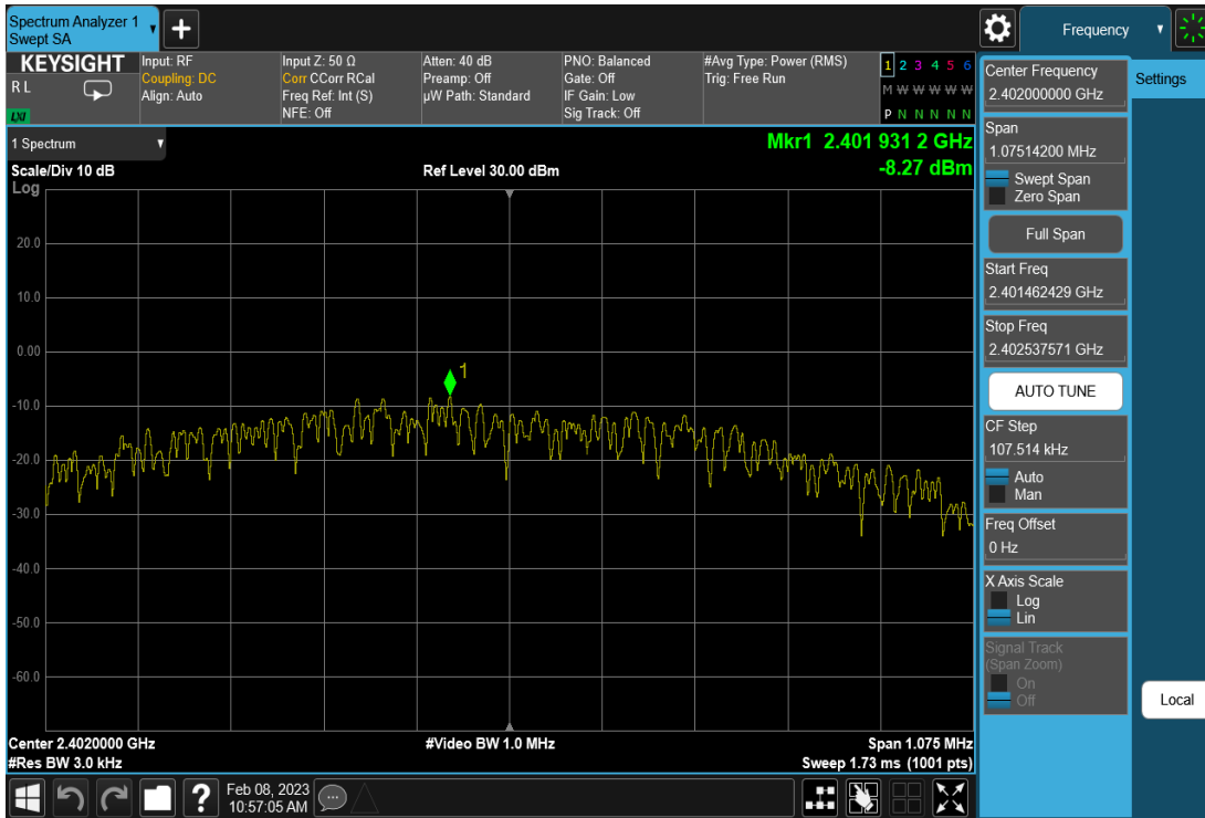
Plot 7-7. Power Spectral Density Plot (Bluetooth (LE), 1Mbps – Ch. 0)
