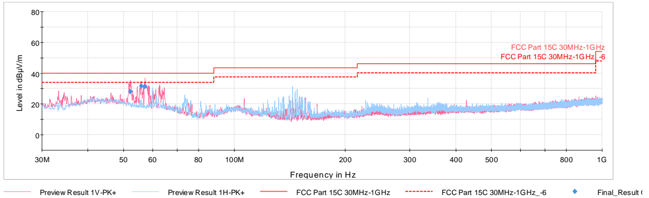
Plot 7-32. Radiated Spurious Emissions Below 1GHz (1Mbps – Ch39, Pol. H & V, with Laptop)
