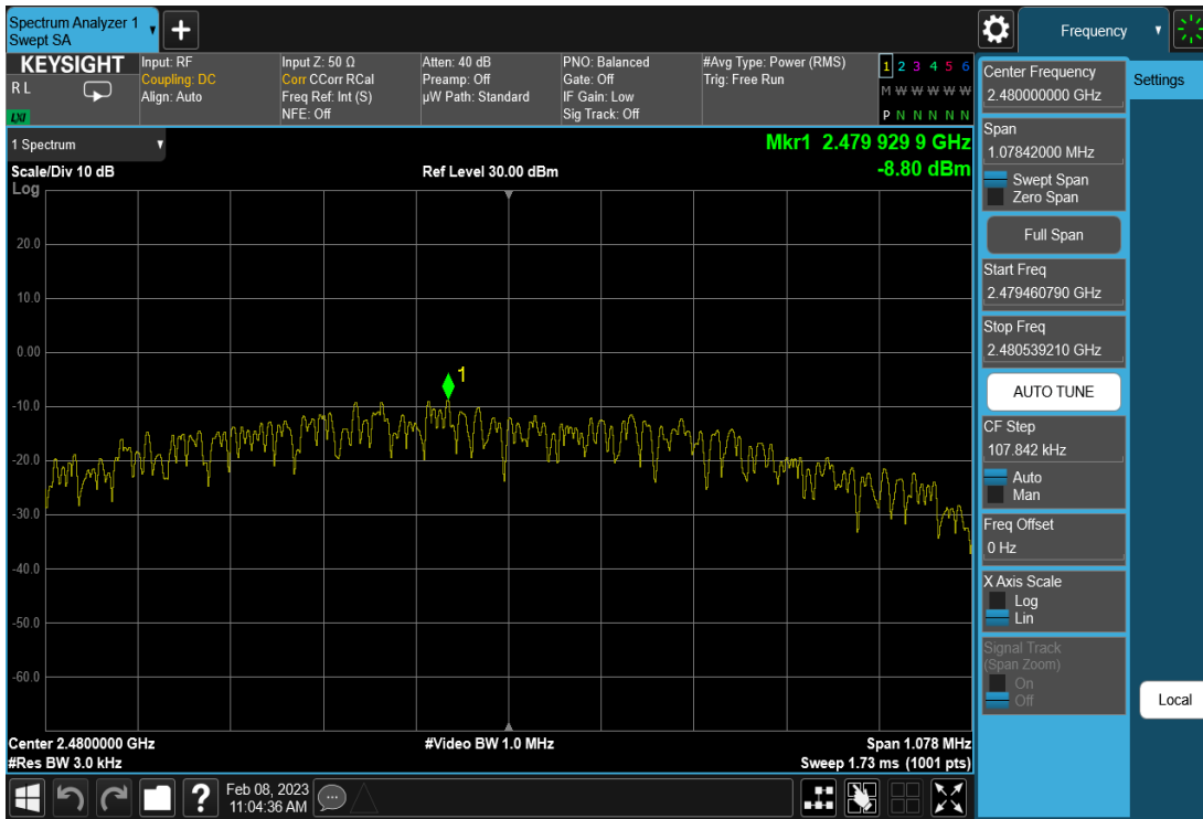
Plot 7-9. Power Spectral Density Plot (Bluetooth (LE), 1Mbps – Ch. 39)
