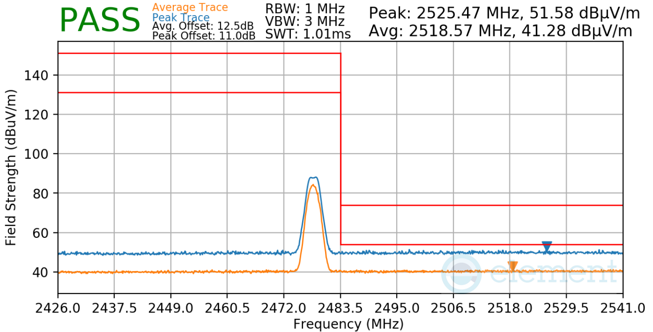
Plot 7-31. Radiated Restricted Upper Band Edge Measurement (Average & Peak)
