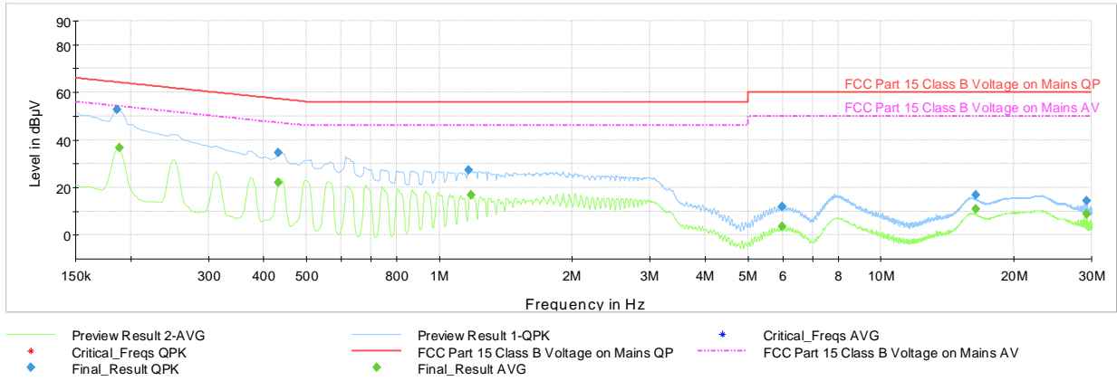
Plot 7-33. AC Line Conducted Plot with Bluetooth LE (L1, 1Mbps – Ch.39 with Laptop)
