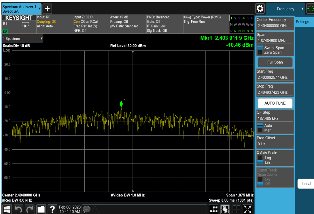
Plot 7-10. Power Spectral Density Plot (Bluetooth (LE), 2Mbps – Ch. 1)
