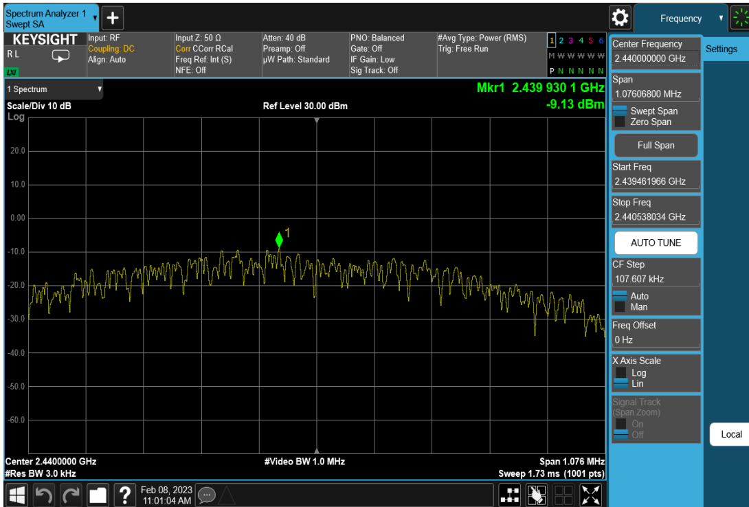
Plot 7-8. Power Spectral Density Plot (Bluetooth (LE), 1Mbps – Ch. 19)
