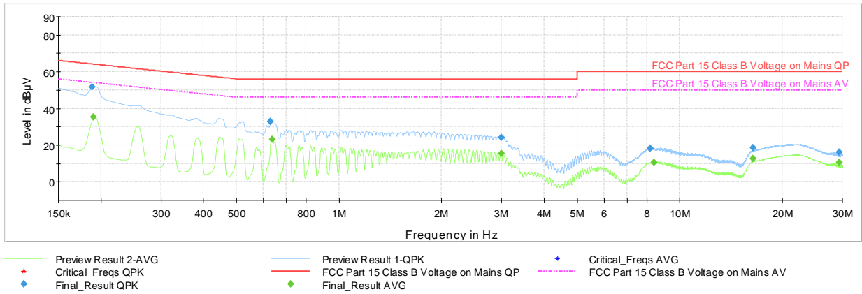
Plot 7-34. AC Line Conducted Plot with Bluetooth LE (N, 1Mbps – Ch.39, with Laptop)
