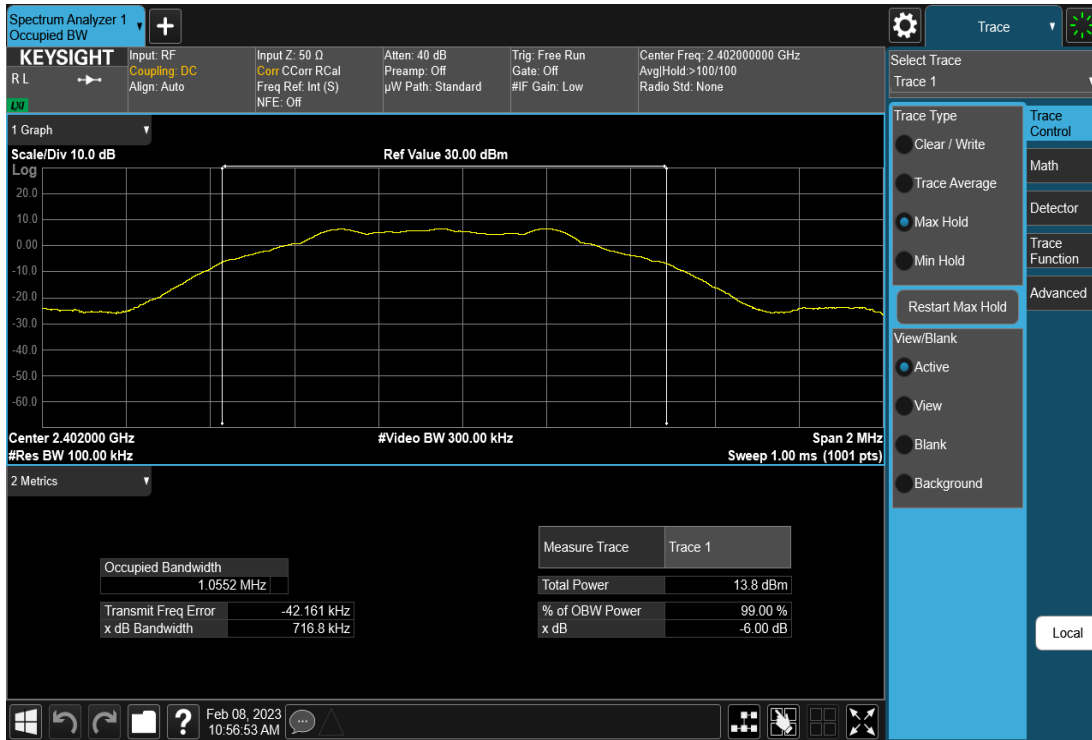
Plot 7-1. 6dB BW & 99% OBW Plot (Bluetooth (LE), 1Mbps – Ch. 0)
