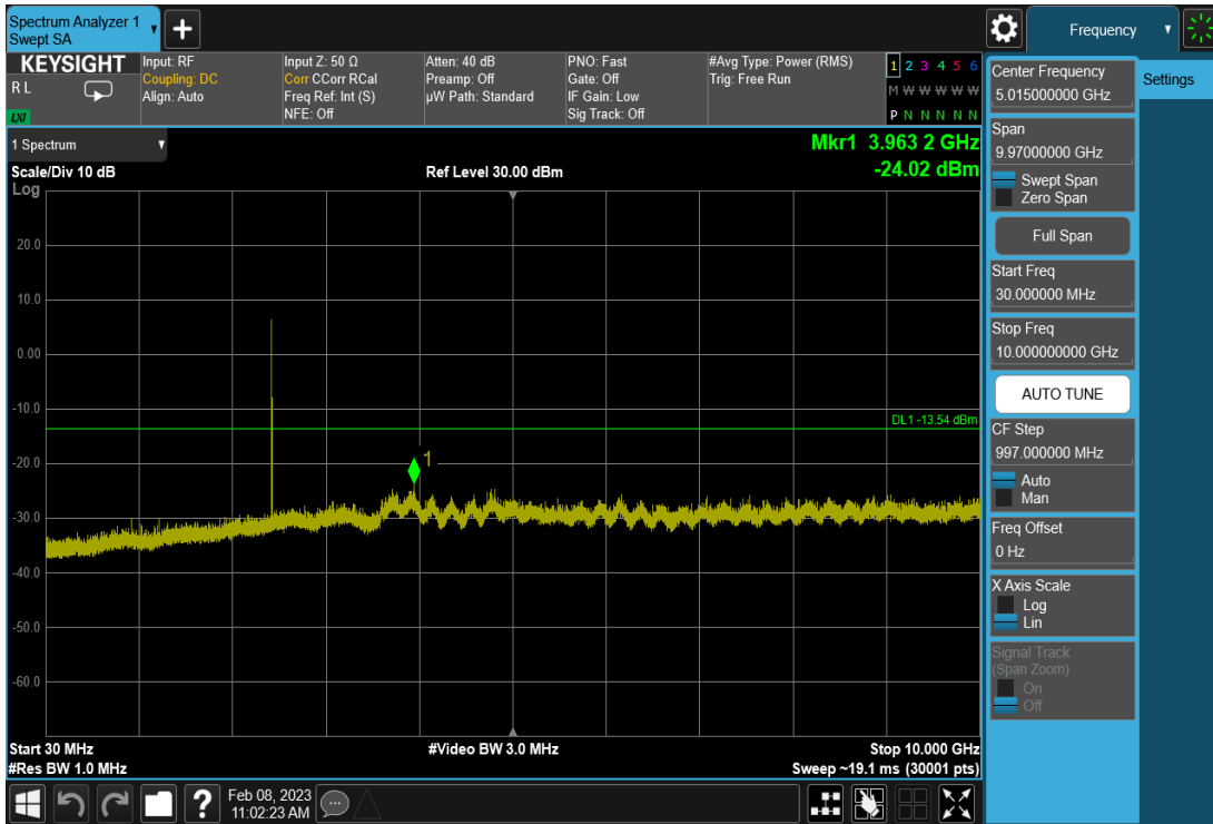
Plot 7-19. Conducted Spurious Plot (Bluetooth (LE), 1Mbps – Ch. 19)
