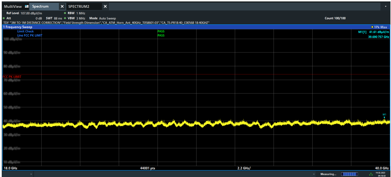
Plot 7-32. Radiated Spurious Emissions above 18GHz (BT GFSK – Ch. 78, Pol H)
