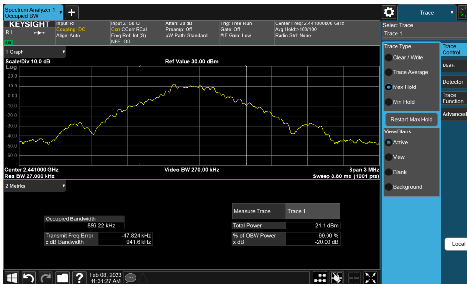
Plot 7-2. 20dB BW and 99% OBW Plot (Bluetooth, GFSK – Ch. 39)
