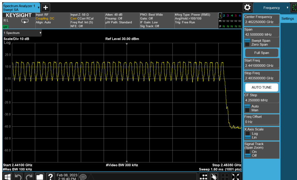
Plot 7-20. High End Spectrum Channel Hopping Plot (Bluetooth, GFSK)
