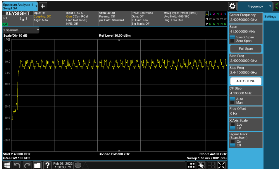
Plot 7-21. Low End Spectrum Channel Hopping Plot (Bluetooth, 8DPSK)
