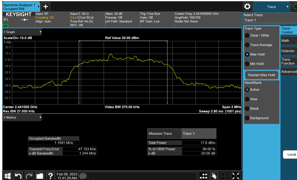
Plot 7-5. 20dB BW and 99% OBW Plot (Bluetooth, 8DPSK – Ch. 39)
