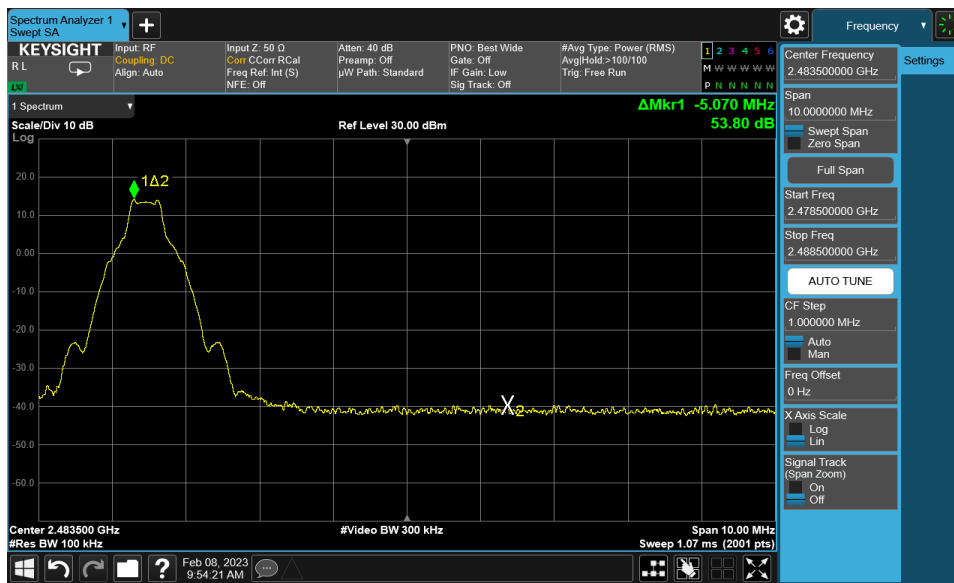
Plot 7-8. Band Edge Plot (Bluetooth with Hopping Disabled, GFSK – Ch. 78)
