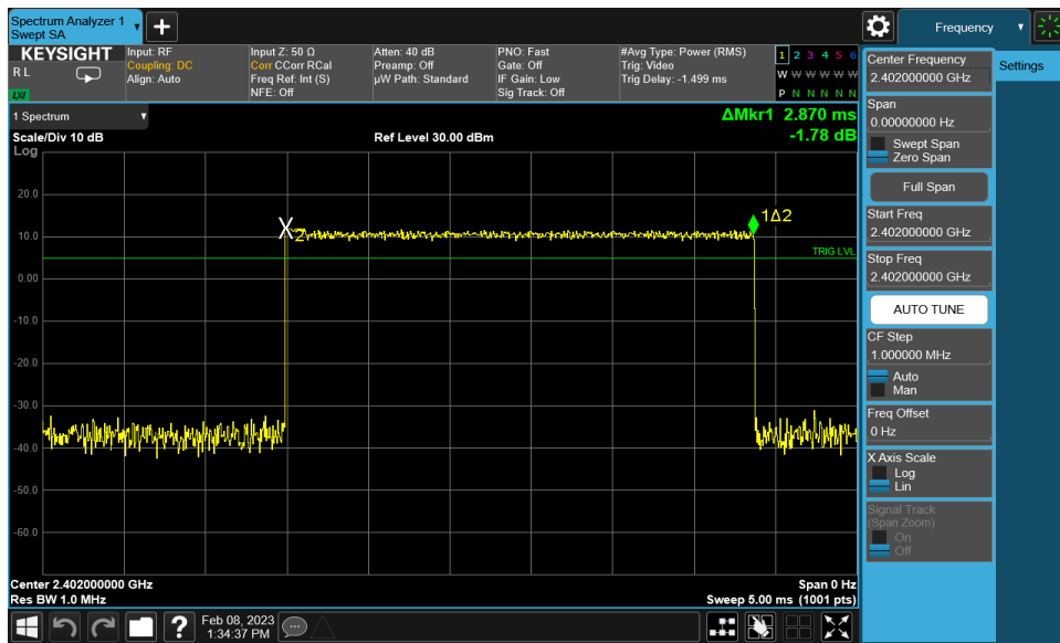
Plot 7-18. Time of Occupancy Plot (Bluetooth, 8DPSK)
