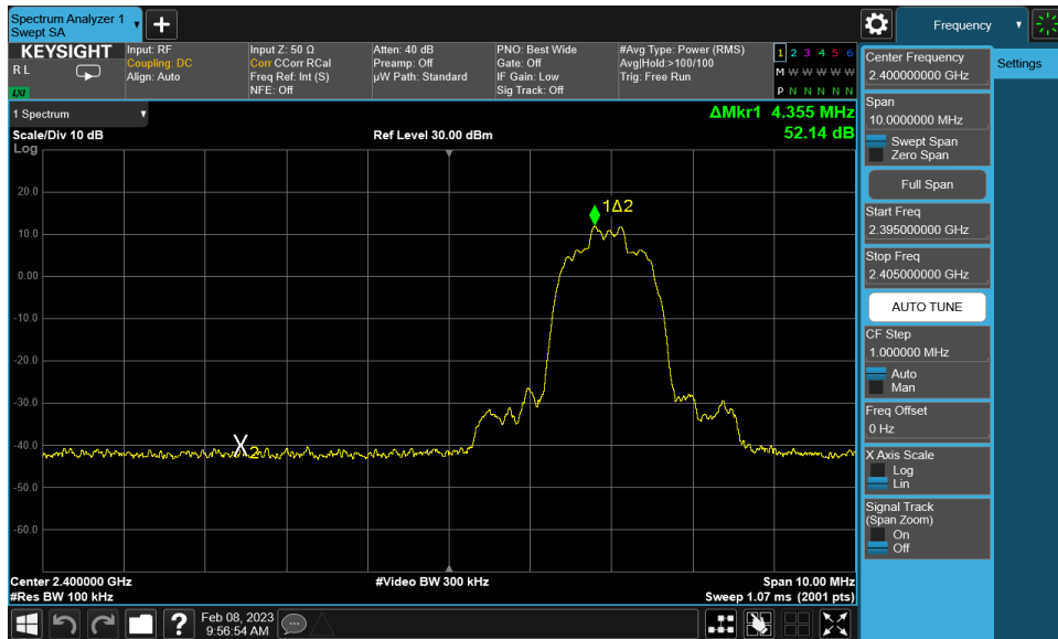
Plot 7-11. Band Edge Plot (Bluetooth with Hopping Disabled, 8DPSK, – Ch. 0)
