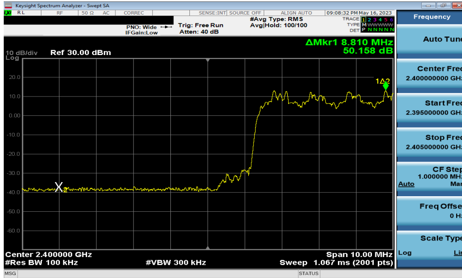
Plot 7-13. Band Edge Plot (Bluetooth with Hopping Enabled, 8DPSK)
