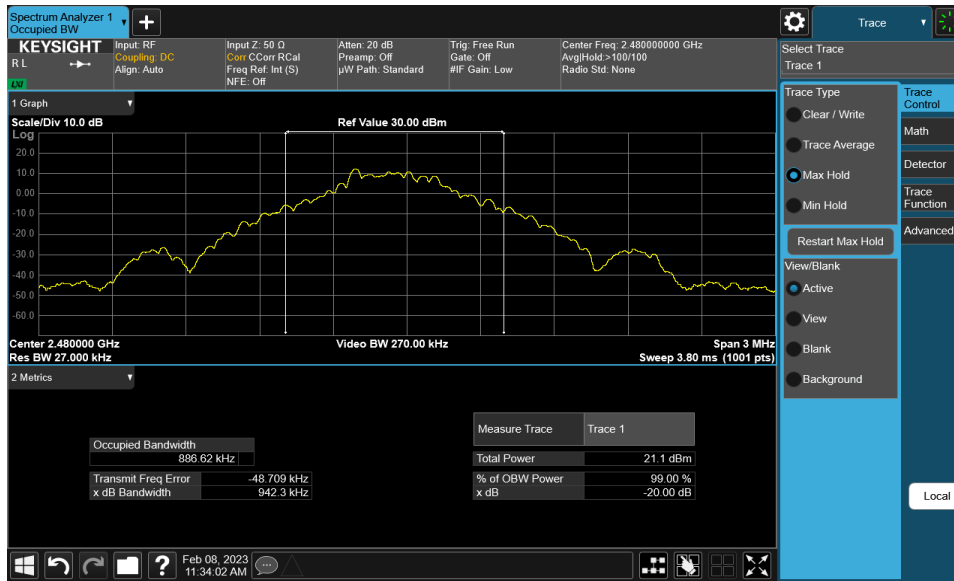
Plot 7-3. 20dB BW and 99% OBW Plot (Bluetooth, GFSK – Ch. 78)
