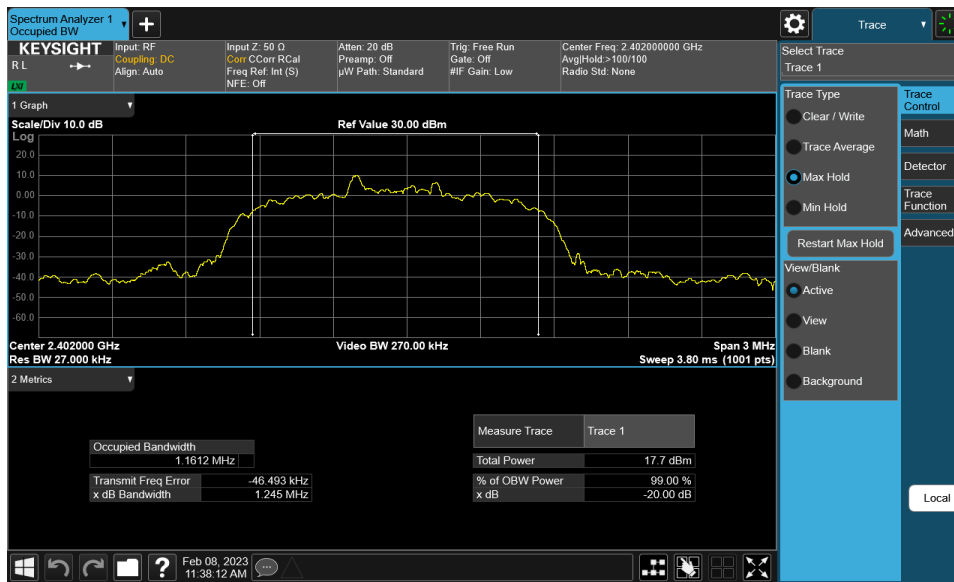
Plot 7-4. 20dB BW and 99% OBW Plot (Bluetooth, 8DPSK – Ch. 0)
