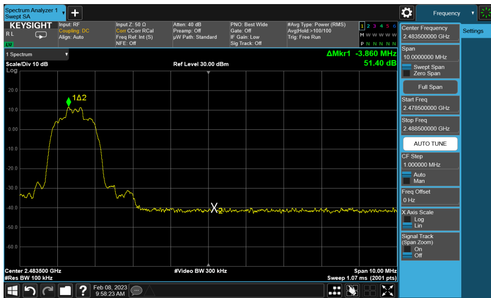
Plot 7-12. Band Edge Plot (Bluetooth with Hopping Disabled, 8DPSK – Ch. 78)
