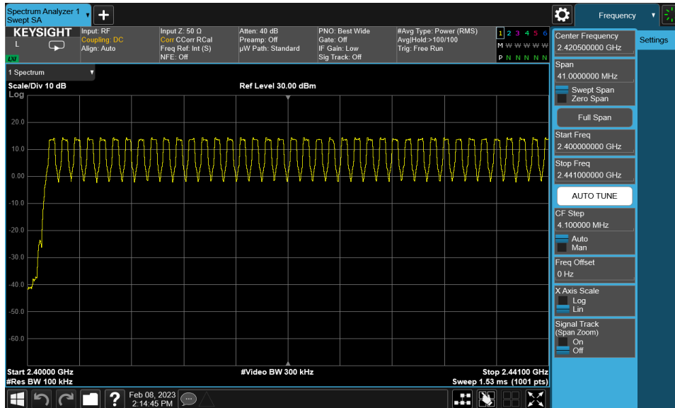
Plot 7-19. Low End Spectrum Channel Hopping Plot (Bluetooth, GFSK)
