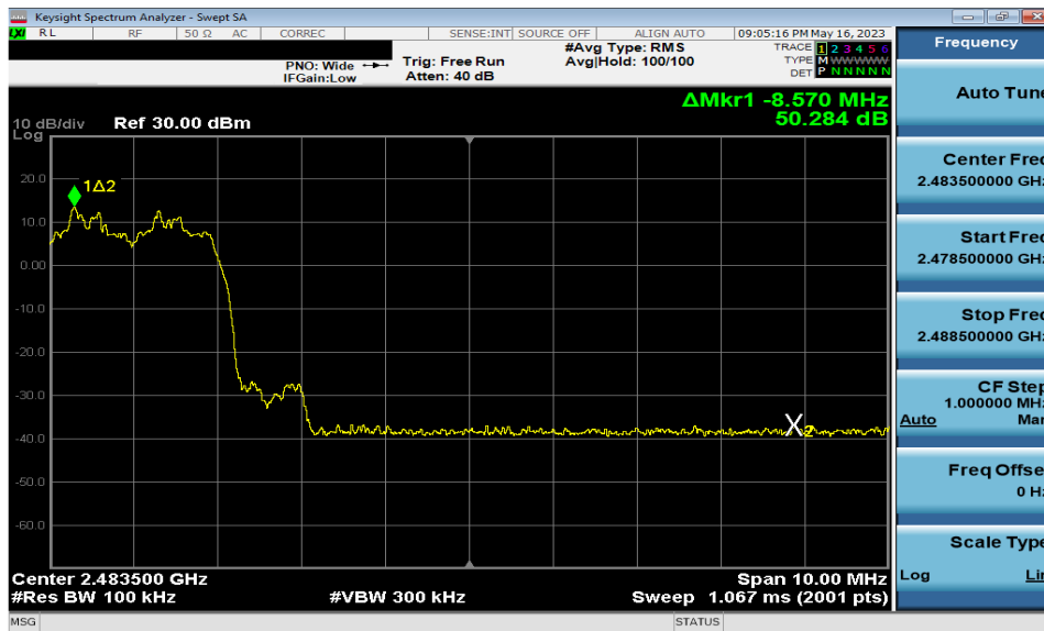
Plot 7-14. Band Edge Plot (Bluetooth with Hopping Enabled, 8DPSK)
