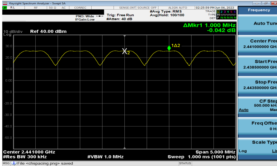
Plot 7-15. Channel Spacing Plot (Bluetooth, GFSK)
