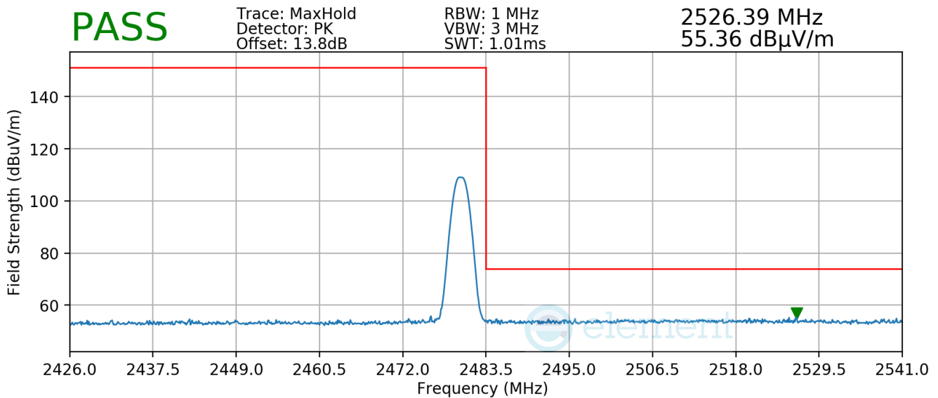
Plot 7-36. Radiated Restricted Upper Band Edge Measurement
