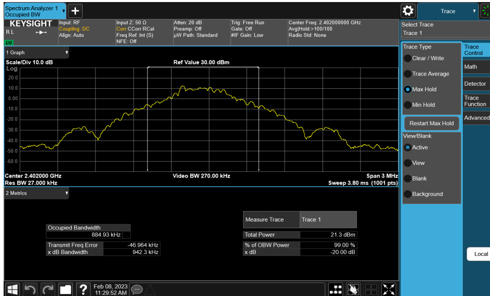
Plot 7-1. 20dB BW and 99% OBW Plot (Bluetooth, GFSK, – Ch. 0)
