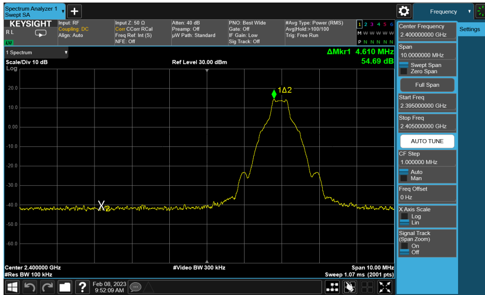
Plot 7-7. Band Edge Plot (Bluetooth with Hopping Disabled, GFSK – Ch. 0)
