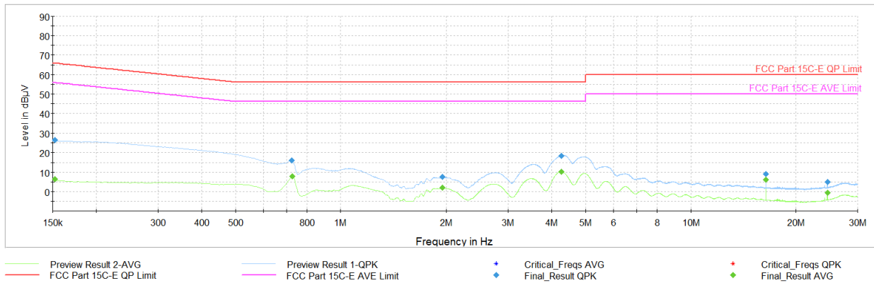
Plot 7-40. AC Line-Conducted Test Plot (N, GFSK – Ch.78, with AC/DC Adapter)
