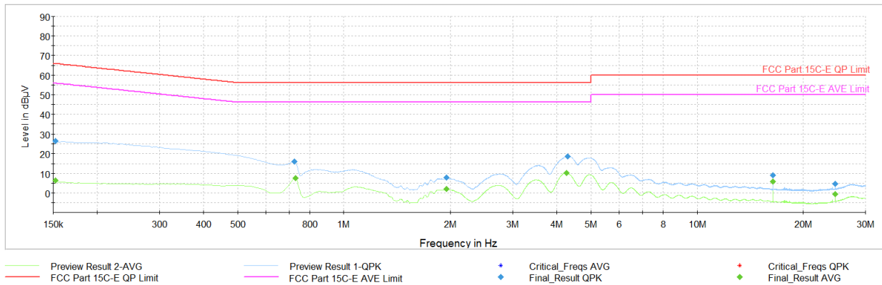
Plot 7-39. AC Line-Conducted Test Plot (L1, GFSK – Ch.78, with AC/DC Adapter)
