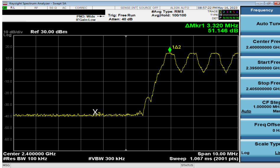
Plot 7-9. Band Edge Plot (Bluetooth with Hopping Enabled, GFSK)
