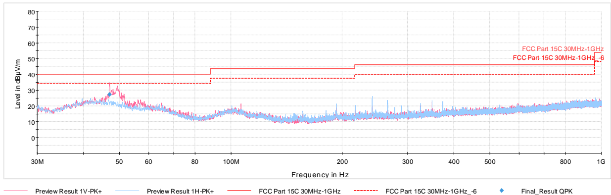
Plot 7-38. Radiated Spurious Emissions Below 1GHz (GFSK – Ch.78, with AC/DC Adapter)
