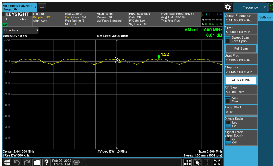
Plot 7-16. Channel Spacing Plot (Bluetooth, 8DPSK)
