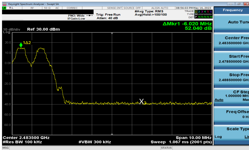
Plot 7-10. Band Edge Plot (Bluetooth with Hopping Enabled, GFSK)
