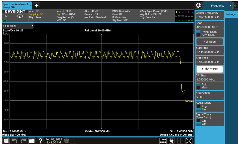
Plot 7-22. High End Spectrum Channel Hopping Plot (Bluetooth, 8DPSK)
