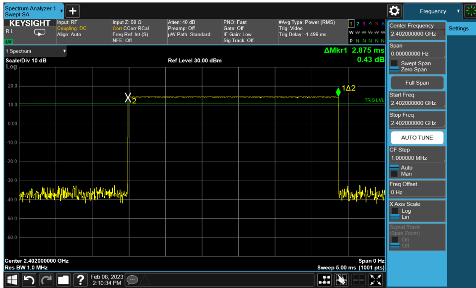
Plot 7-17. Time of Occupancy Plot (Bluetooth, GFSK)
