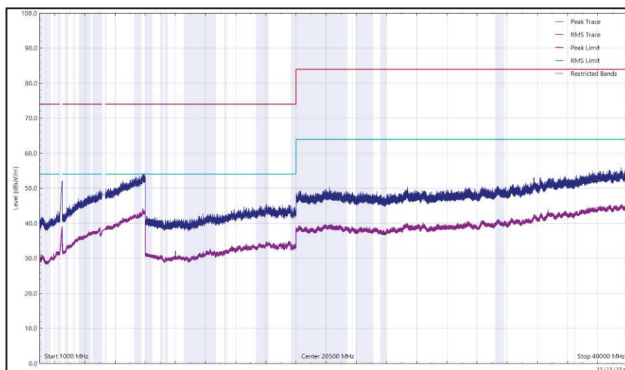
Figure 25 - 2437 MHz (CH6), HT20, Core 0 and 5204 MHz, HDR8, Core 1, ePA, 1 GHz to 40 GHz, Vertical
