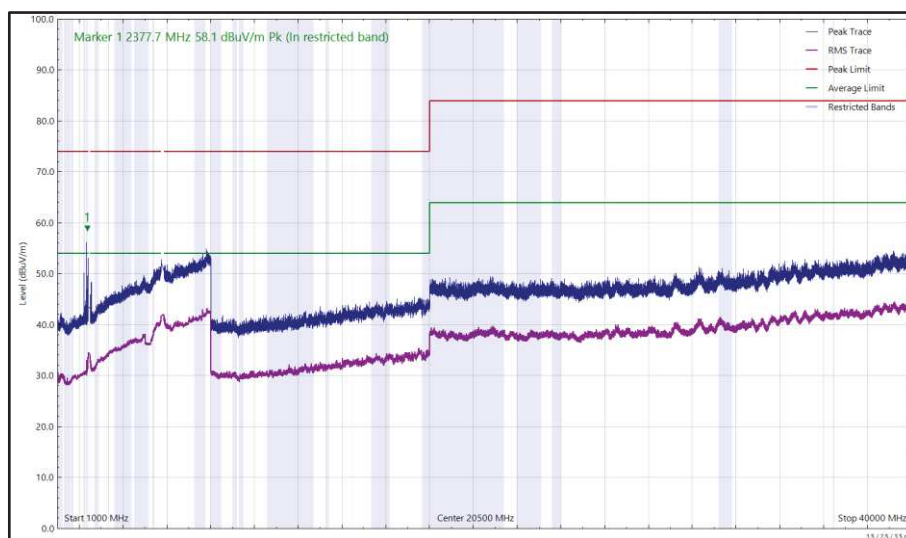
Figure 43 - 2440 MHz (CH18), Thread, ePA, Core 1 and U-NII-3 - 5785 MHz (CH157), VHT20, CDD, Core 0 + Core 1, 1 GHz to 40 GHz, Horizontal
