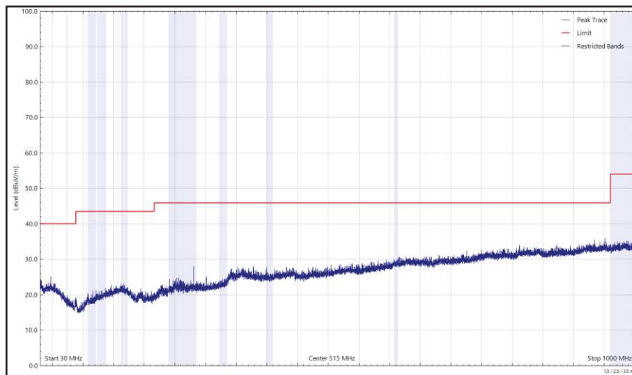
Figure 26 - 2437 MHz (CH6), HT20, Core 0 and 5788 MHz, HDR4, Core 1, ePA, 30 MHz to 1 GHz, Horizontal (Peak)
