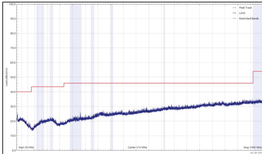
Figure 62 - 2440 MHz (CH18), Thread, ePA, Core 0 and U-NII-2C - 5640 (CH128), VHT20, CDD, Core 0 + Core 1, 30 MHz to 1 GHz, Horizontal (Peak)
