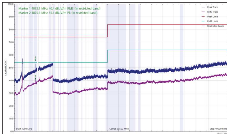
Figure 23 - 2437 MHz (CH6), HT20, Core 0 and 5204 MHz, HDR8, Core 1, ePA, 1 GHz to 40 GHz, Horizontal
