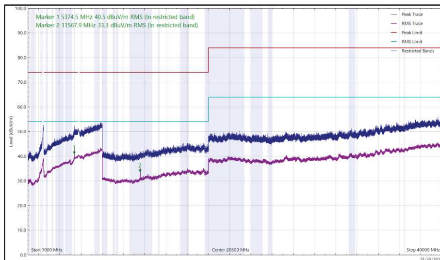
Figure 27 - 2437 MHz (CH6), HT20, Core 0 and 5788 MHz, HDR4, Core 1, ePA, 1 GHz to 40 GHz, Horizontal
