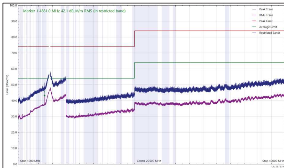
Figure 73 - 2440 MHz (CH18), Thread, ePA, Core 2 and U-NII-2C - 5640 (CH128), VHT20, CDD, Core 0 + Core 1, 1 GHz to 40 GHz, Vertical
