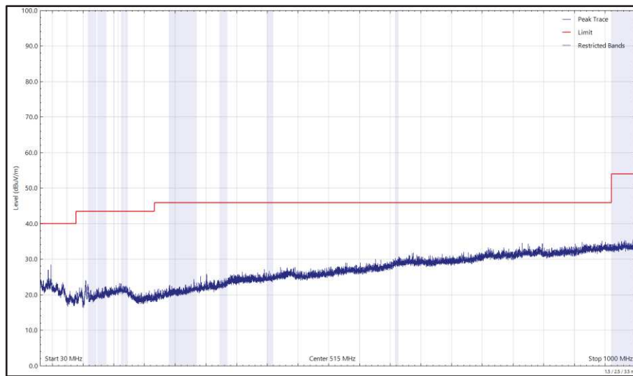
Figure 32 - 2437 MHz (CH6), HT20, Core 1 and 5204 MHz, HDR8, Core 0, ePA, 30 MHz to 1 GHz, Vertical (Peak)
