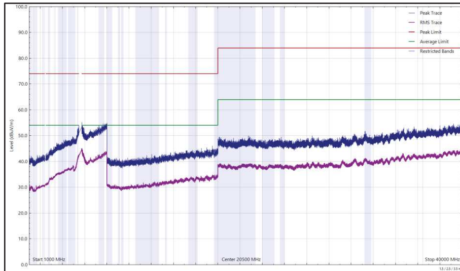
Figure 71 - 2440 MHz (CH18), Thread, ePA, Core 2 and U-NII-2C - 5640 (CH128), VHT20, CDD, Core 0 + Core 1, 1 GHz to 40 GHz, Horizontal
