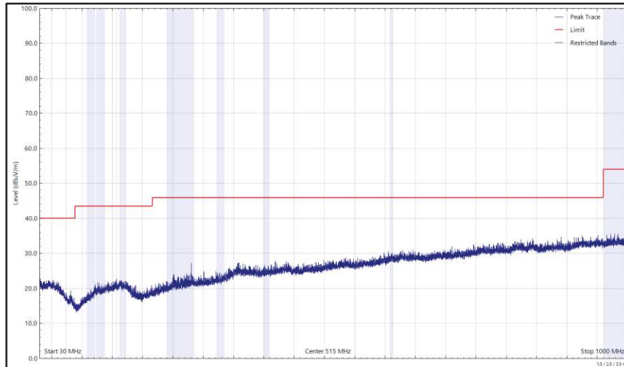
Figure 54 - 2440 MHz (CH18), Thread, ePA, Core 1 and U-NII-1 - 5240 MHz (CH48), VHT20, CDD, Core 0 + Core 1, 30 MHz to 1 GHz, Horizontal (Peak)
