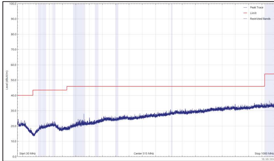
Figure 46 - 2440 MHz (CH18), Thread, ePA, Core 2 and U-NII-3 - 5785 MHz (CH157), VHT20, CDD, Core 0 + Core 1, 30 MHz to 1 GHz, Horizontal (Peak)
