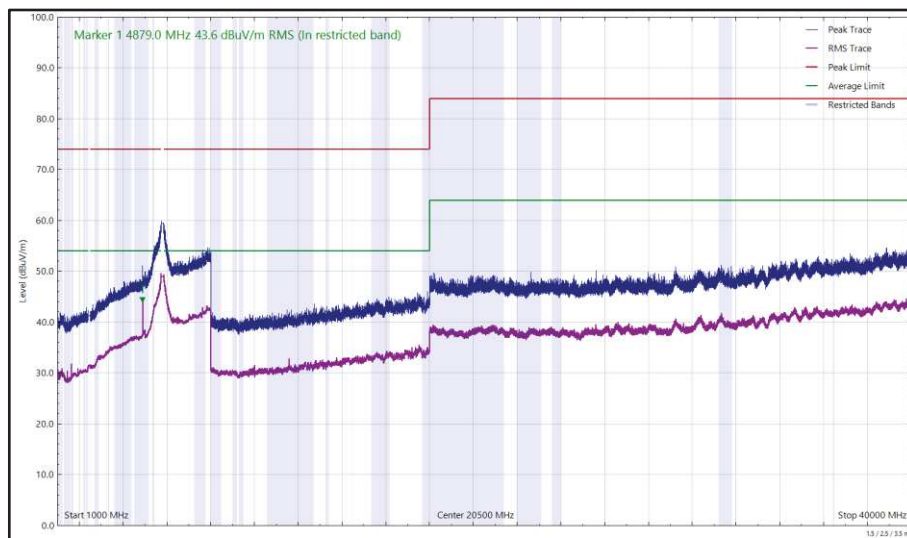
Figure 49 - 2440 MHz (CH18), Thread, ePA, Core 2 and U-NII-3 - 5785 MHz (CH157), VHT20, CDD, Core 0 + Core 1, 1 GHz to 40 GHz, Vertical
