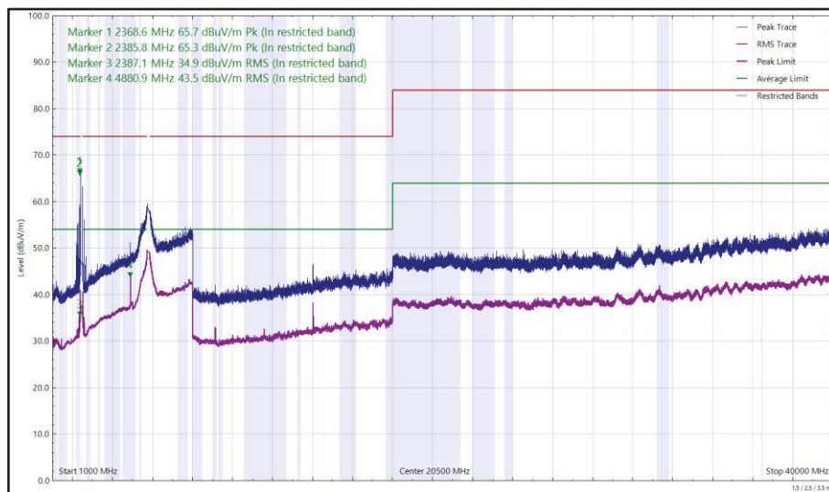
Figure 45 - 2440 MHz (CH18), Thread, ePA, Core 1 and U-NII-3 - 5785 MHz (CH157), VHT20, CDD, Core 0 + Core 1, 1 GHz to 40 GHz, Vertical
