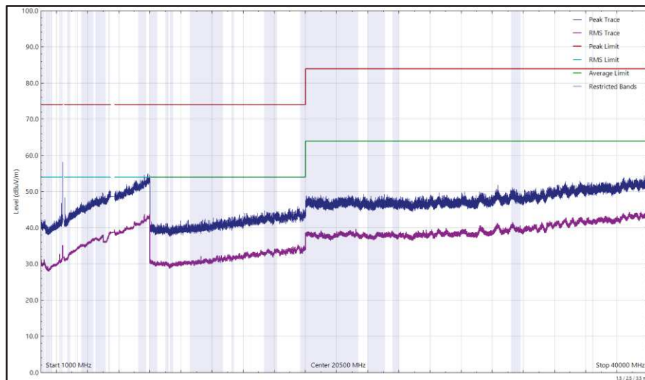
Figure 63 - 2440 MHz (CH18), Thread, ePA, Core 0 and U-NII-2C - 5640 (CH128), VHT20, CDD, Core 0 + Core 1, 1 GHz to 40 GHz, Horizontal
