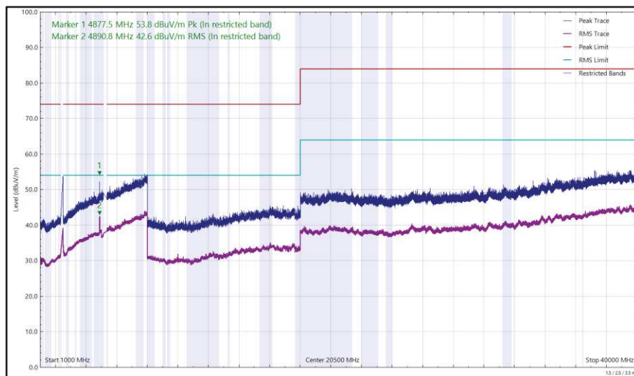
Figure 33 - 2437 MHz (CH6), HT20, Core 1 and 5204 MHz, HDR8, Core 0, ePA, 1 GHz to 40 GHz, Vertical
