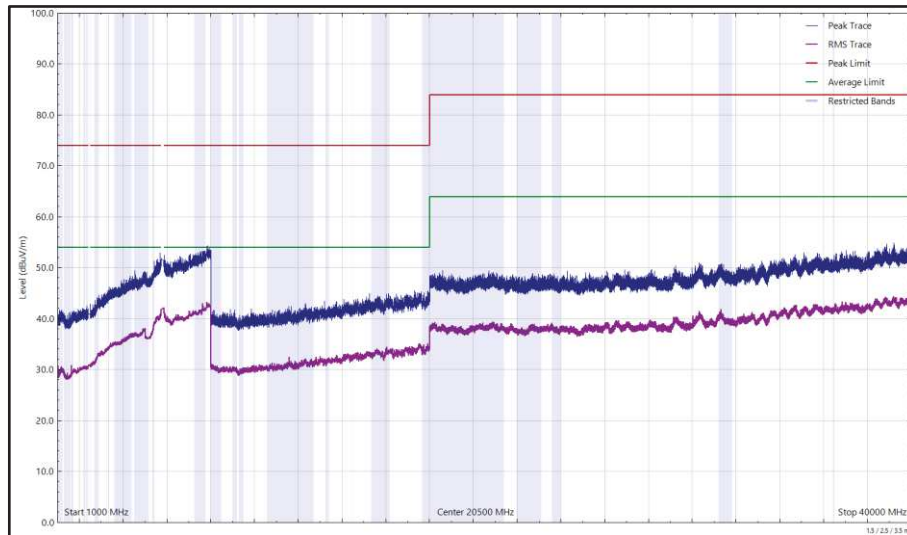
Figure 47 - 2440 MHz (CH18), Thread, ePA, Core 2 and U-NII-3 - 5785 MHz (CH157), VHT20, CDD, Core 0 + Core 1, 1 GHz to 40 GHz, Horizontal
