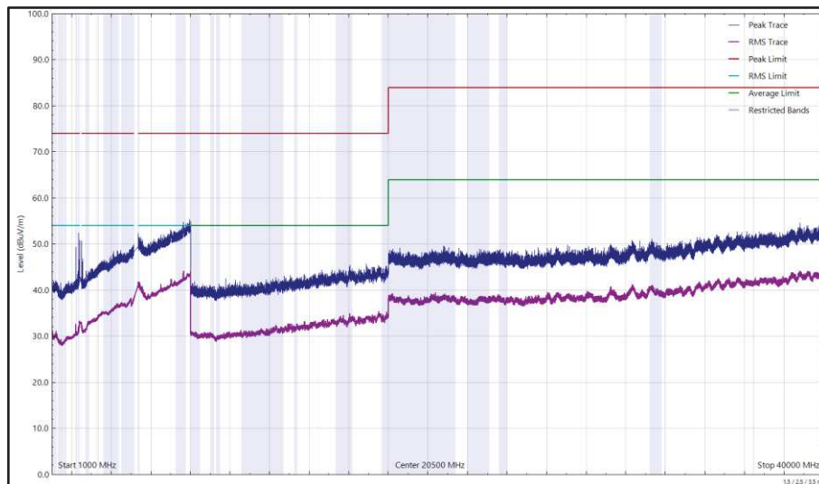
Figure 55 - 2440 MHz (CH18), Thread, ePA, Core 1 and U-NII-1 - 5240 MHz (CH48), VHT20, CDD, Core 0 + Core 1, 1 GHz to 40 GHz, Horizontal
