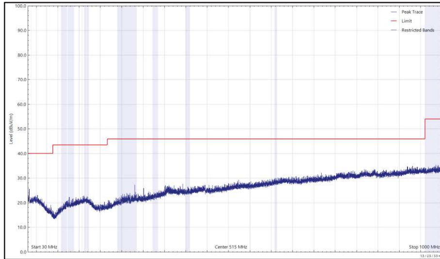
Figure 70 - 2440 MHz (CH18), Thread, ePA, Core 2 and U-NII-2C - 5640 (CH128), VHT20, CDD, Core 0 + Core 1, 30 MHz to 1 GHz, Horizontal (Peak)
