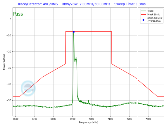
Plot 7-1530. LPI In-Band Emission Plot SDM Diversity Antenna 1b (160MHz 802.11ax RU26 (UNII Band 8) – Ch. 207)
