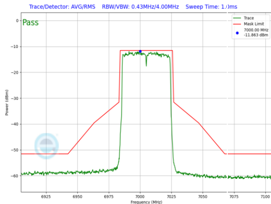
Plot 7-1519. LPI In-Band Emission Plot SDM Diversity Antenna 3c (40MHz 802.11ax RU484 (UNII Band 8) – Ch. 211)
