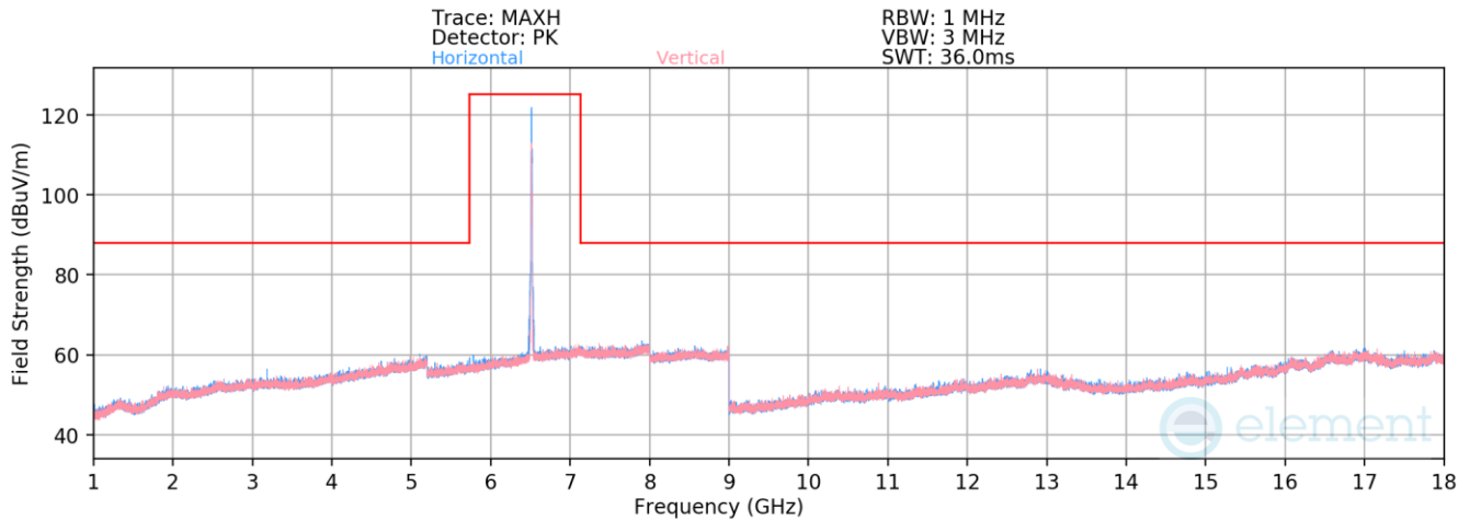
Plot 7-1578. Radiated Spurious Emissions above 1GHz Antenna 3c (802.11ax – Ch. 113 – RU26)
