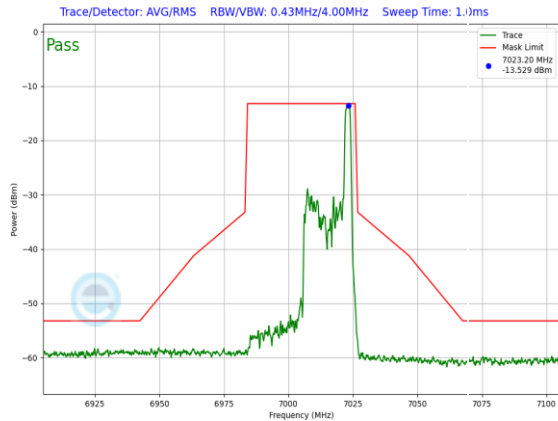
Plot 7-1517. LPI In-Band Emission Plot SDM Diversity Antenna 3c (40MHz 802.11ax RU26 (UNII Band 8) – Ch. 211)
