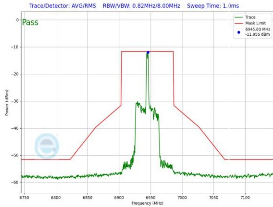
Plot 7-1523. LPI In-Band Emission Plot SDM Diversity Antenna 3c (80MHz 802.11ax RU26 (UNII Band 8) – Ch. 199)
