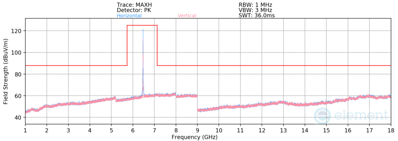
Plot 7-1577. Radiated Spurious Emissions above 1GHz Antenna 3c (802.11ax – Ch. 105 – RU26)
