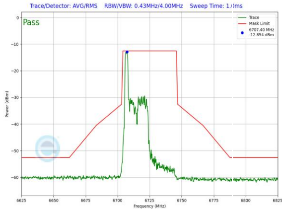
Plot 7-1481. LPI In-Band Emission Plot SDM Diversity Antenna 3c (40MHz 802.11ax RU26 (UNII Band 7) – Ch. 155)
