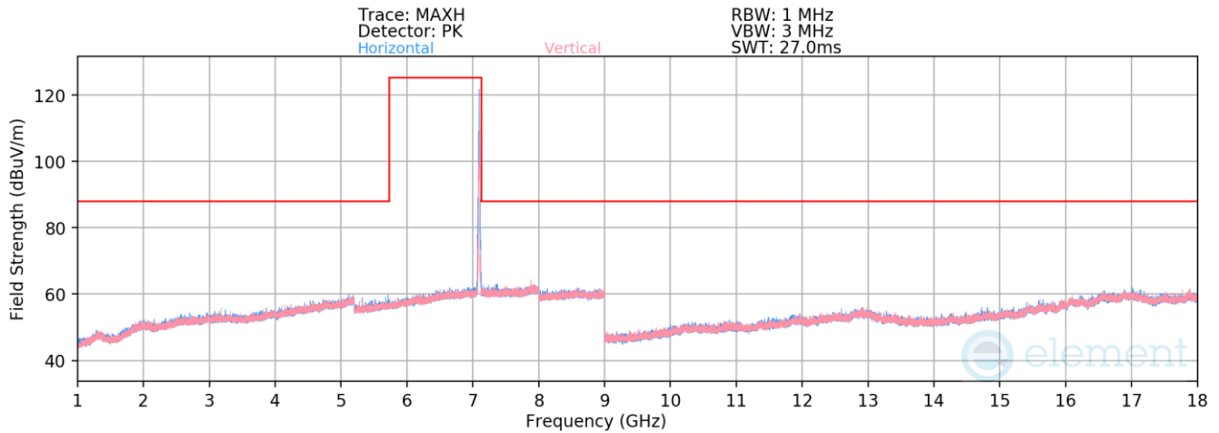
Plot 7-1584. Radiated Spurious Emissions above 1GHz Antenna 3c (802.11ax – Ch. 229 – RU26)
