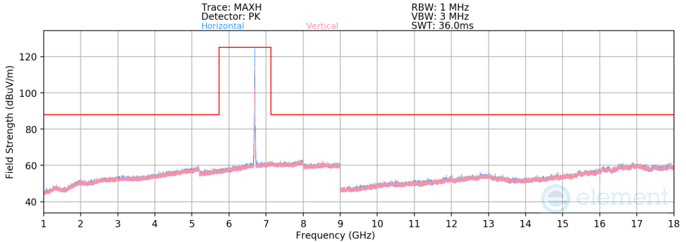
Plot 7-1580. Radiated Spurious Emissions above 1GHz Antenna 3c (802.11ax – Ch. 149 – RU26)
