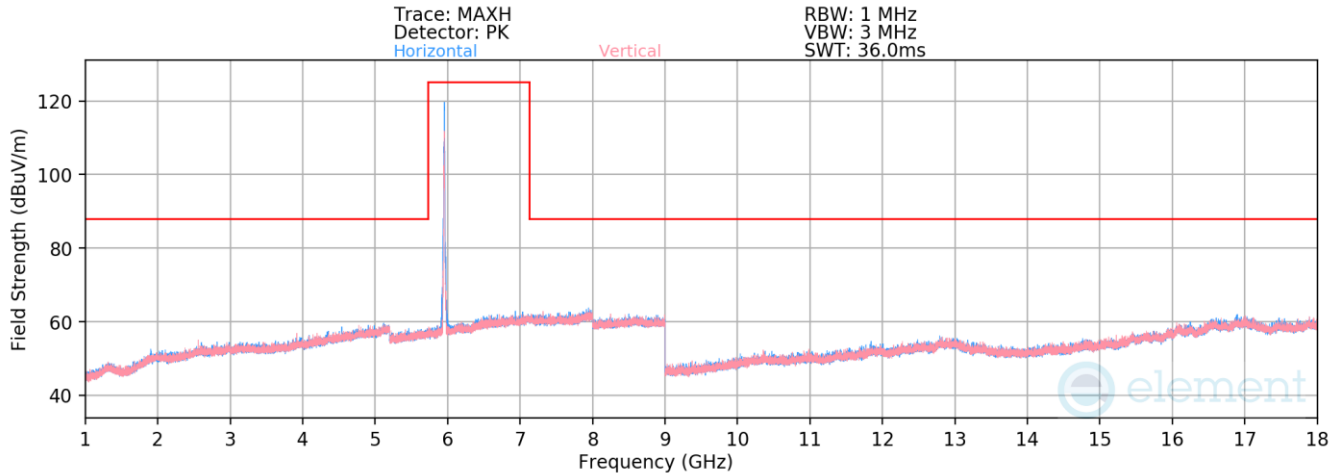
Plot 7-1573. Radiated Spurious Emissions above 1GHz Antenna 3c (802.11ax – Ch. 1 – RU26)
