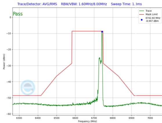
Plot 7-1501. LPI In-Band Emission Plot SDM Diversity Antenna 3c (160MHz 802.11ax RU26 (UNII Band 7) – Ch. 143)
