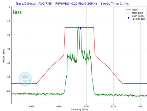
Plot 7-1507. LPI In-Band Emission Plot SDM Diversity Antenna 3c (20MHz 802.11ax RU26 (UNII Band 8) – Ch. 209)
