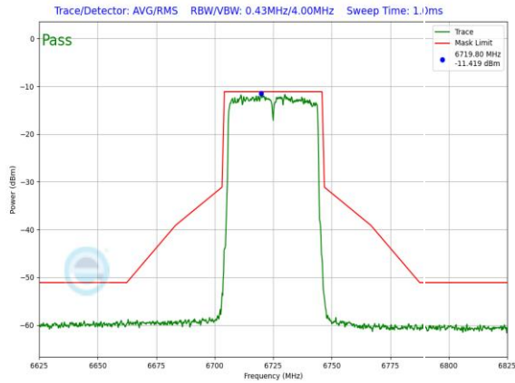
Plot 7-1487. LPI In-Band Emission Plot SDM Diversity Antenna 3c (40MHz 802.11ax RU484 (UNII Band 7) – Ch. 155)
