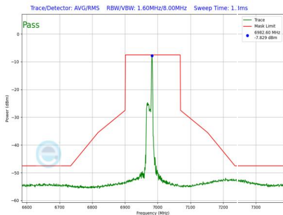
Plot 7-1531. LPI In-Band Emission Plot SDM Diversity Antenna 3c (160MHz 802.11ax RU26 (UNII Band 8) – Ch. 207)
