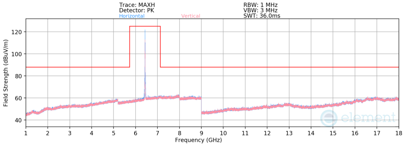
Plot 7-1576. Radiated Spurious Emissions above 1GHz Antenna 3c (802.11ax – Ch. 97 – RU26)
