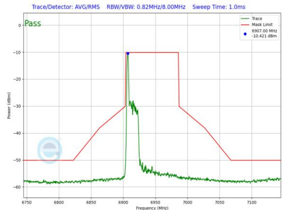
Plot 7-1521. LPI In-Band Emission Plot SDM Diversity Antenna 3c (80MHz 802.11ax RU26 (UNII Band 8) – Ch. 199)
