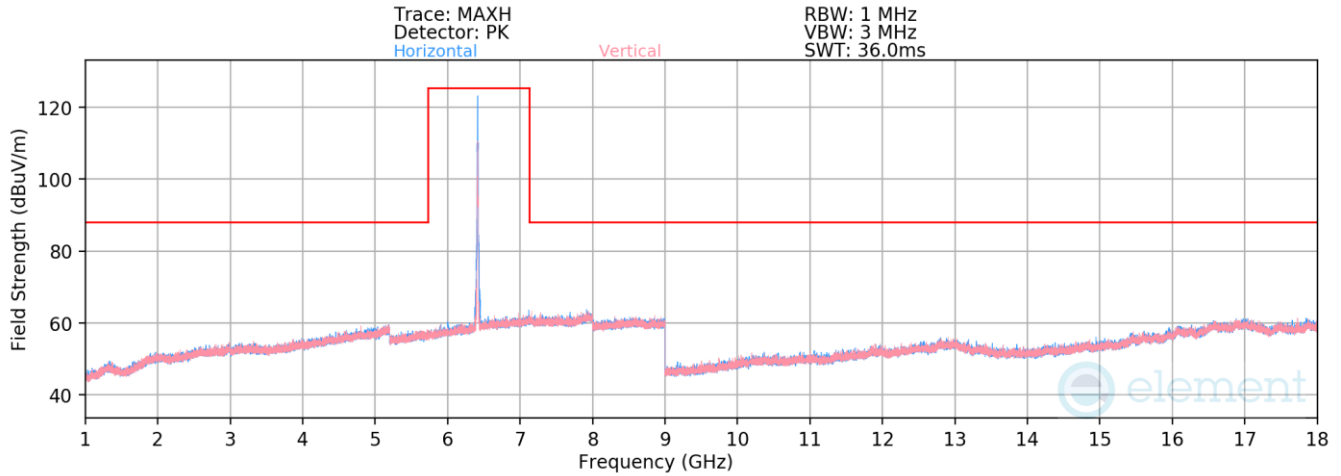
Plot 7-1575. Radiated Spurious Emissions above 1GHz Antenna 3c (802.11ax – Ch. 93 – RU26)
