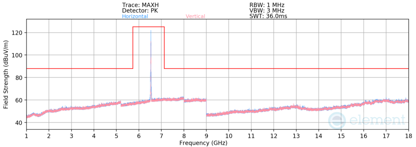
Plot 7-1579. Radiated Spurious Emissions above 1GHz Antenna 3c (802.11ax – Ch. 117 – RU26)
