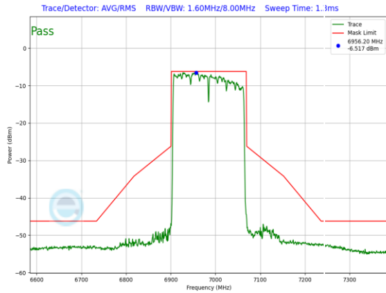
Plot 7-1535. LPI In-Band Emission Plot SDM Diversity Antenna 3c (160MHz 802.11ax RU996x2 (UNII Band 8) – Ch. 207)
