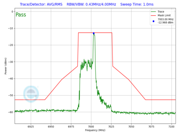
Plot 7-1515. LPI In-Band Emission Plot SDM Diversity Antenna 3c (40MHz 802.11ax RU26 (UNII Band 8) – Ch. 211)
