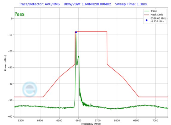
Plot 7-1497. LPI In-Band Emission Plot SDM Diversity Antenna 3c (160MHz) 802.11ax RU26 (UNII Band 7) – Ch. 143
