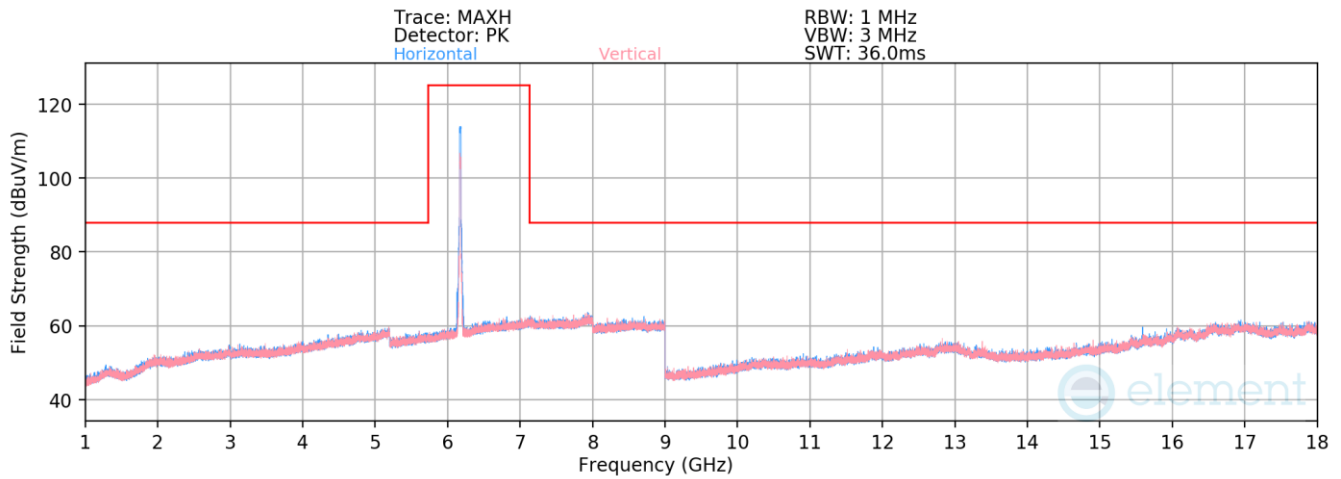
Plot 7-1586. Radiated Spurious Emissions above 1GHz Antenna 3c (802.11ax – Ch. 45 – RU242)
