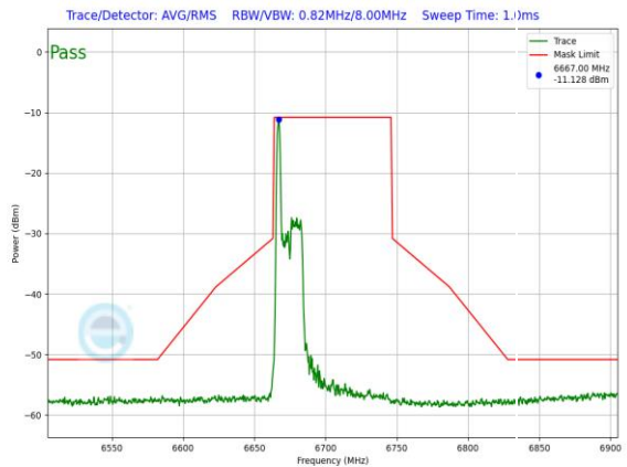
Plot 7-1489. LPI In-Band Emission Plot SDM Diversity Antenna 3c (80MHz 802.11ax RU26 (UNII Band 7) – Ch. 151)
