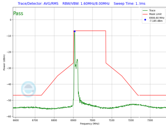
Plot 7-1529. LPI In-Band Emission Plot SDM Diversity Antenna 3c (160MHz 802.11ax RU26 (UNII Band 8) – Ch. 207)
