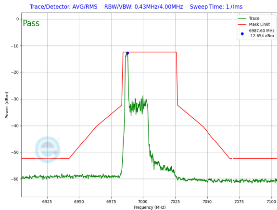
Plot 7-1513. LPI In-Band Emission Plot SDM Diversity Antenna 3c (40MHz 802.11ax RU26 (UNII Band 8) – Ch. 211)
