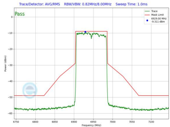
Plot 7-1527. LPI In-Band Emission Plot SDM Diversity Antenna 3c (80MHz 802.11ax RU996 (UNII Band 8) – Ch. 199)
