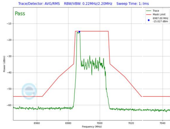
Plot 7-1505. LPI In-Band Emission Plot SDM Diversity Antenna 3c (20MHz 802.11ax RU26 (UNII Band 8) – Ch. 209)
