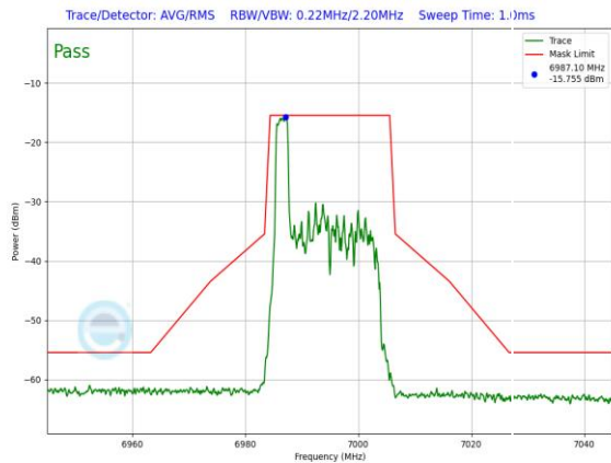
Plot 7-1506. LPI In-Band Emission Plot SDM Diversity Antenna 1b (20MHz 802.11ax RU26 (UNII Band 8) – Ch. 209)
