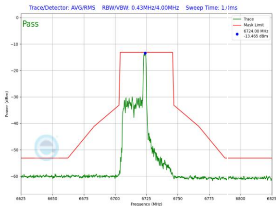
Plot 7-1483. LPI In-Band Emission Plot SDM Diversity Antenna 3c (40MHz 802.11ax RU26 (UNII Band 7) – Ch. 155)
