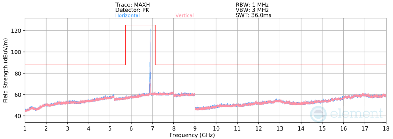
Plot 7-1582. Radiated Spurious Emissions above 1GHz Antenna 3c (802.11ax – Ch. 189 – RU26)
