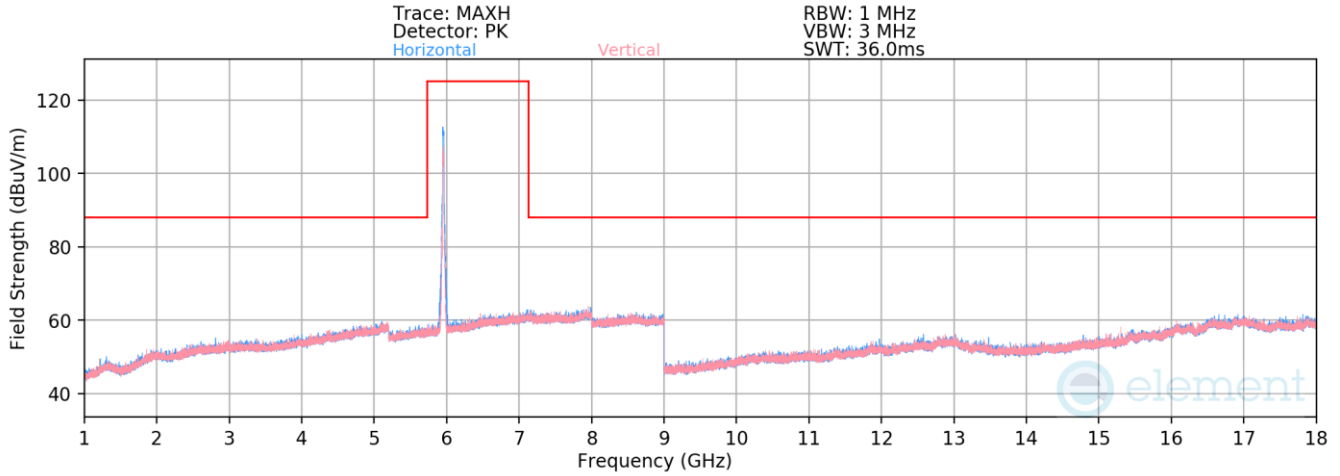
Plot 7-1585. Radiated Spurious Emissions above 1GHz Antenna 3c (802.11ax – Ch. 1 – RU242)
