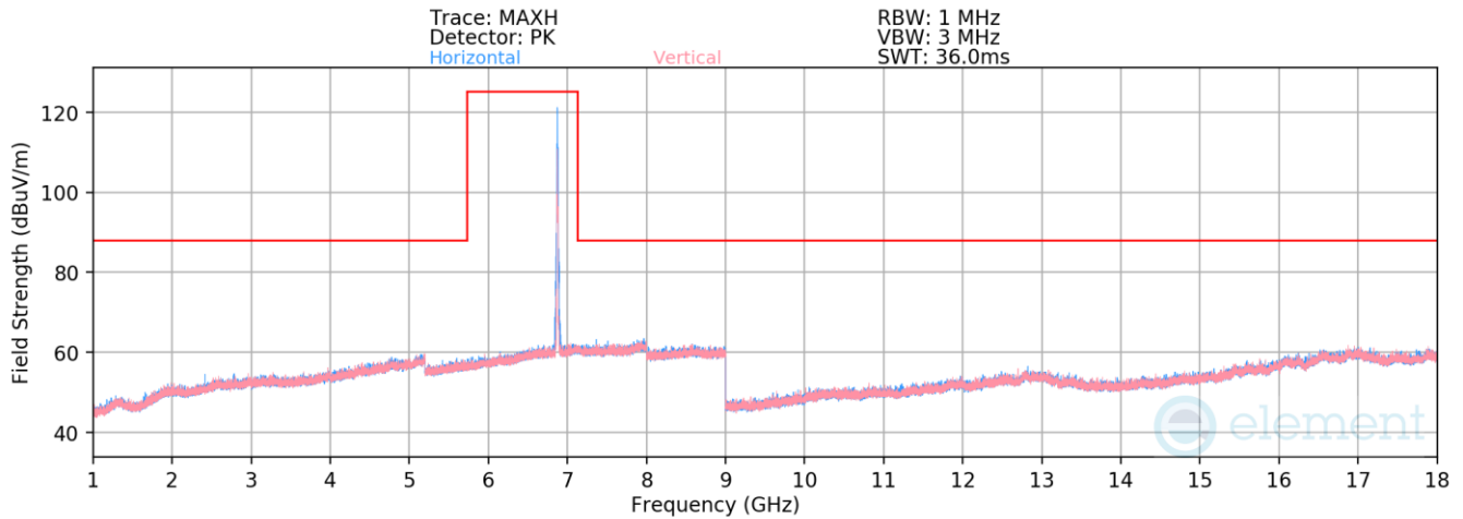
Plot 7-1581. Radiated Spurious Emissions above 1GHz Antenna 3c (802.11ax – Ch. 185 – RU26)
