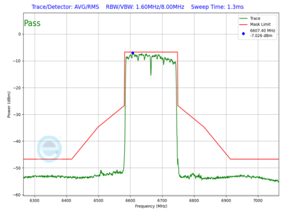
Plot 7-1503. LPI In-Band Emission Plot SDM Diversity Antenna 3c (160MHz 802.11ax RU996x2 (UNII Band 7) – Ch. 143)
