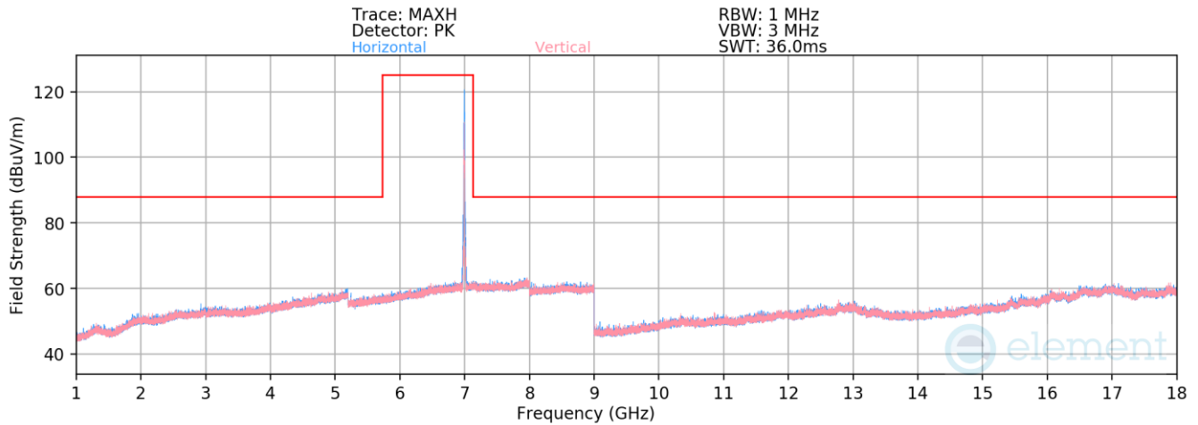
Plot 7-1583. Radiated Spurious Emissions above 1GHz Antenna 3c (802.11ax – Ch. 209 – RU26)
