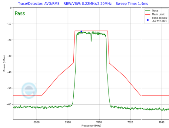
Plot 7-1511. LPI In-Band Emission Plot SDM Diversity Antenna 3c (20MHz 802.11ax RU242 (UNII Band 8) – Ch. 209)
