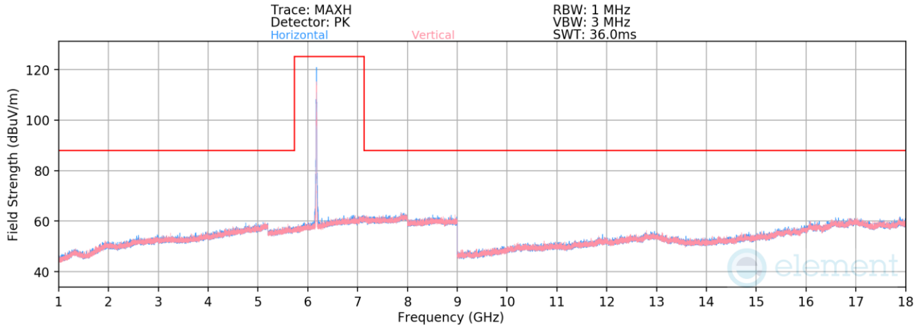
Plot 7-1574. Radiated Spurious Emissions above 1GHz Antenna 3c (802.11ax – Ch. 45 – RU26)
