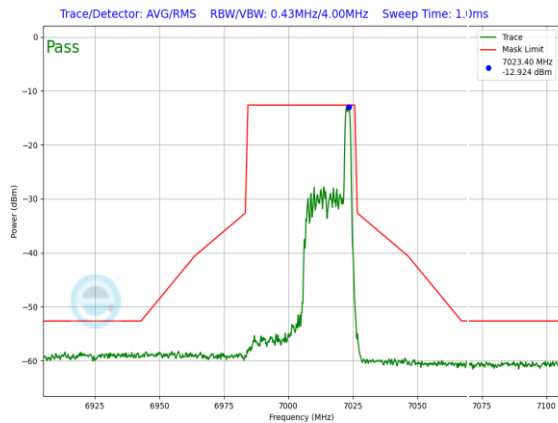
Plot 7-1390. LPI In-Band Emission Plot SDM Primary Antenna 3a (40MHz 802.11ax RU26 (UNII Band 8) – Ch. 211)
