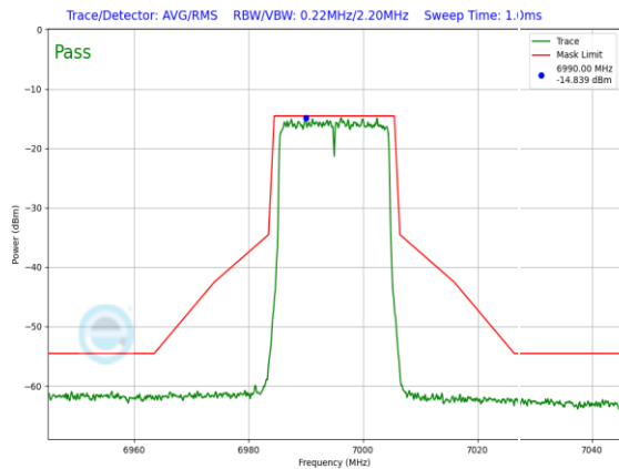
Plot 7-1384. LPI In-Band Emission Plot SDM Primary Antenna 3a (20MHz) 802.11ax RU242 (UNII Band 8) – Ch. 209)
