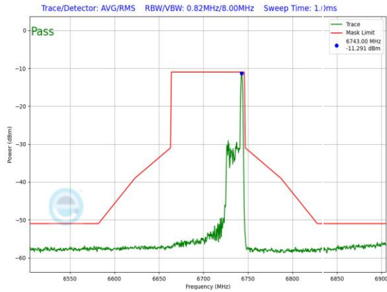
Plot 7-1365. LPI In-Band Emission Plot SDM Primary Antenna 3c (80MHz 802.11ax RU26 (UNII Band 7) – Ch. 151)
