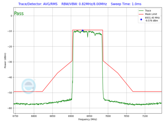
Plot 7-1400. LPI In-Band Emission Plot SDM Primary Antenna 3a (80MHz 802.11ax RU996 (UNII Band 8) – Ch. 199)
