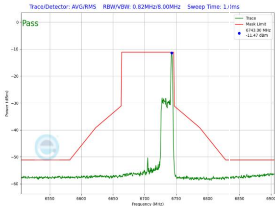
Plot 7-1366. LPI In-Band Emission Plot SDM Primary Antenna 3a (80MHz 802.11ax RU26 (UNII Band 7) – Ch. 151)
