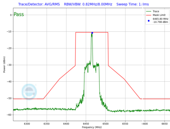
Plot 7-1459. LPI In-Band Emission Plot SDM Diversity Antenna 3c (80MHz 802.11ax RU26 (UNII Band 6) – Ch. 103)
