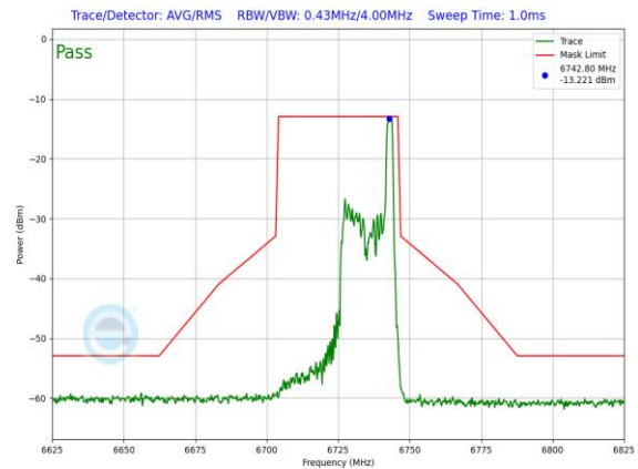
Plot 7-1357. LPI In-Band Emission Plot SDM Primary Antenna 3c (40MHz 802.11ax RU26 (UNII Band 7) – Ch. 155)
