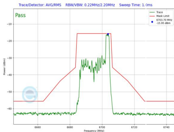
Plot 7-1349. LPI In-Band Emission Plot SDM Primary Antenna 3c (20MHz 802.11ax RU26 (UNII Band 7) – Ch. 149)
