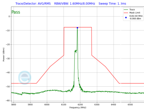
Plot 7-1435. LPI In-Band Emission Plot SDM Diversity Antenna 3c (160MHz 802.11ax RU26 (UNII Band 5) – Ch. 47)
