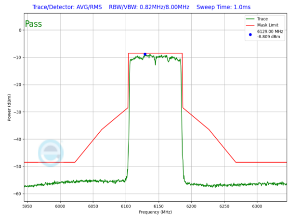
Plot 7-1431. LPI In-Band Emission Plot SDM Diversity Antenna 3c (80MHz 802.11ax RU996 (UNII Band 5) – Ch. 39)
