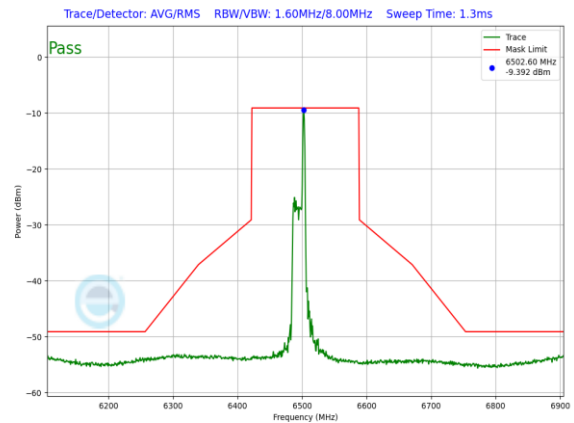
Plot 7-1340. LPI In-Band Emission Plot SDM Primary Antenna 3a (160MHz) 802.11ax RU26 (UNII Band 6) – Ch. 111
