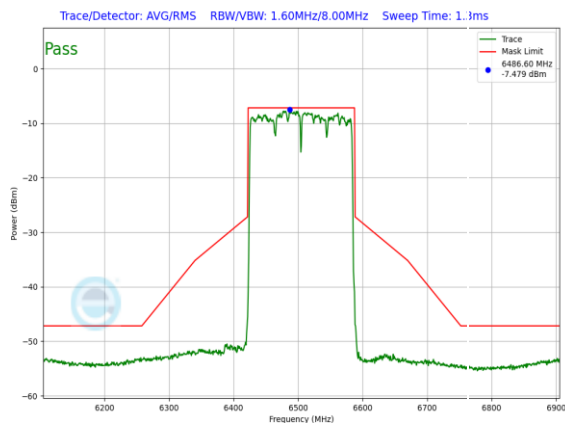
Plot 7-1471. LPI In-Band Emission Plot SDM Diversity Antenna 3c (160MHz 802.11ax RU996x2 (UNII Band 6) – Ch. 111)
