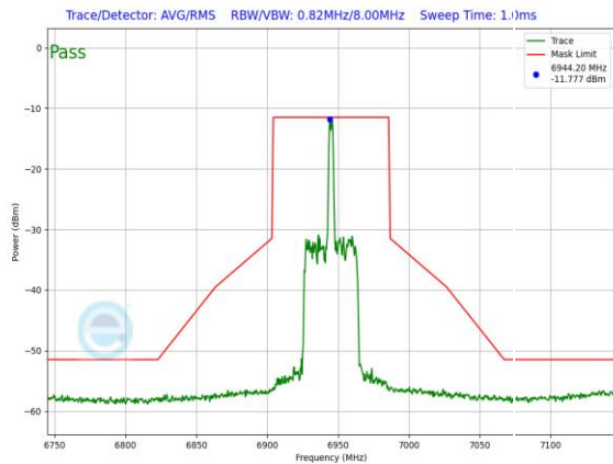
Plot 7-1396. LPI In-Band Emission Plot SDM Primary Antenna 3a (80MHz 802.11ax RU26 (UNII Band 8) – Ch. 199)
