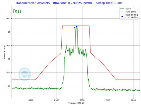
Plot 7-1380. LPI In-Band Emission Plot SDM Primary Antenna 3a (20MHz 802.11ax RU26 (UNII Band 8) – Ch. 209)
