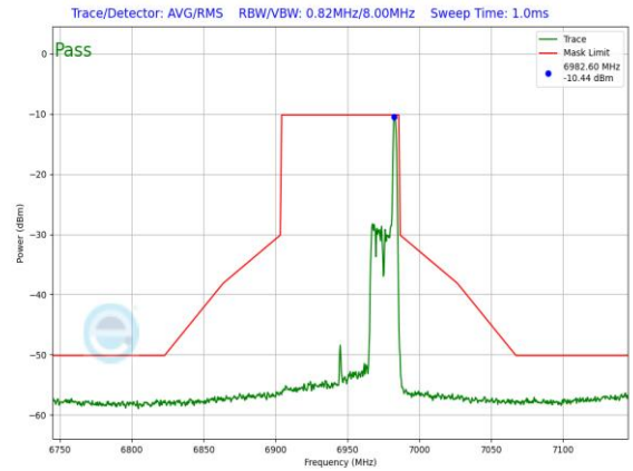
Plot 7-1398. LPI In-Band Emission Plot SDM Primary Antenna 3a (80MHz 802.11ax RU26 (UNII Band 8) – Ch. 199)
