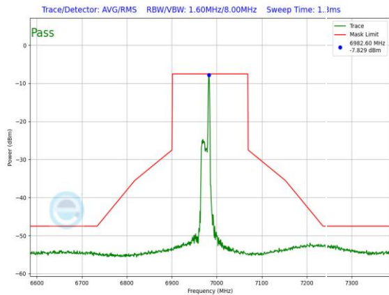
Plot 7-1403. LPI In-Band Emission Plot SDM Primary Antenna 3c (160MHz 802.11ax RU26 (UNII Band 8) – Ch. 207)
