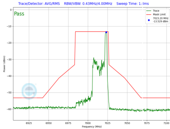
Plot 7-1389. LPI In-Band Emission Plot SDM Primary Antenna 3c (40MHz 802.11ax RU26 (UNII Band 8) – Ch. 211)
