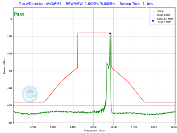
Plot 7-1469. LPI In-Band Emission Plot SDM Diversity Antenna 3c (160MHz 802.11ax RU26 (UNII Band 6) – Ch. 111)
