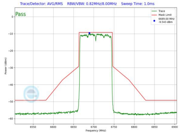
Plot 7-1368. LPI In-Band Emission Plot SDM Primary Antenna 3a (80MHz 802.11ax RU996 (UNII Band 7) – Ch. 151)
