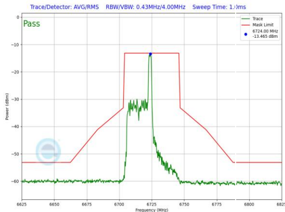
Plot 7-1355. LPI In-Band Emission Plot SDM Primary Antenna 3c (40MHz 802.11ax RU26 (UNII Band 7) – Ch. 155)
