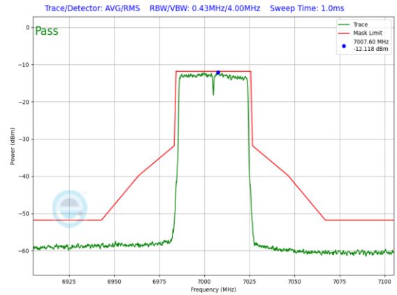
Plot 7-1392. LPI In-Band Emission Plot SDM Primary Antenna 3a (40MHz 802.11ax RU484 (UNII Band 8) – Ch. 211)
