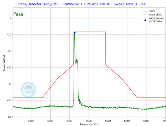
Plot 7-1337. LPI In-Band Emission Plot SDM Primary Antenna 3c (160MHz) 802.11ax RU26 (UNII Band 6) – Ch. 111
