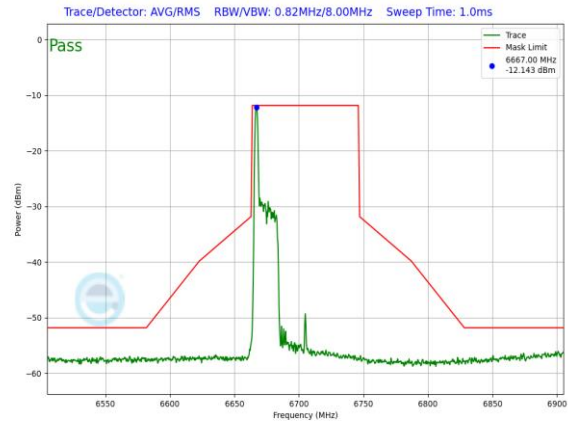
Plot 7-1362. LPI In-Band Emission Plot SDM Primary Antenna 3a (80MHz 802.11ax RU26 (UNII Band 7) – Ch. 151)
