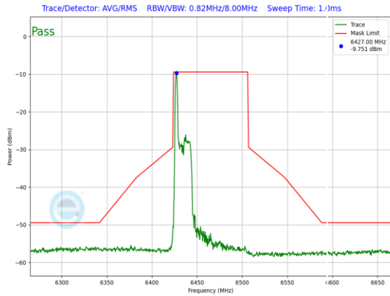
Plot 7-1457. LPI In-Band Emission Plot SDM Diversity Antenna 3c (80MHz 802.11ax RU26 (UNII Band 6) – Ch. 103)
