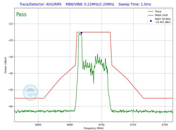
Plot 7-1473. LPI In-Band Emission Plot SDM Diversity Antenna 3c (20MHz 802.11ax RU26 (UNII Band 7) – Ch. 149)
