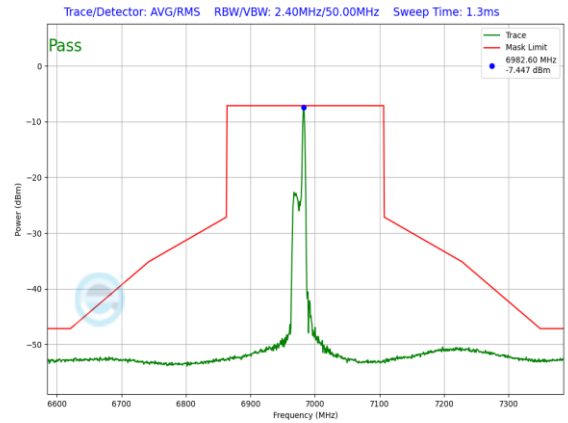
Plot 7-1404. LPI In-Band Emission Plot SDM Primary Antenna 3a (160MHz 802.11ax RU26 (UNII Band 8) – Ch. 207)
