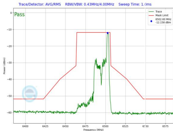
Plot 7-1453. LPI In-Band Emission Plot SDM Diversity Antenna 3c (40MHz 802.11ax RU26 (UNII Band 6) – Ch. 107)
