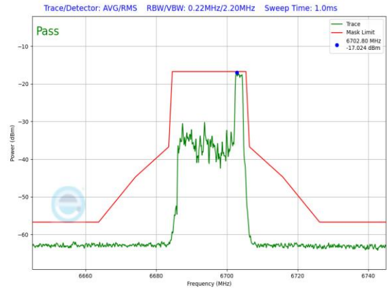
Plot 7-1350. LPI In-Band Emission Plot SDM Primary Antenna 3a (20MHz 802.11ax RU26 (UNII Band 7) – Ch. 149)
