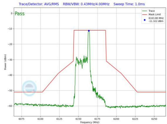
Plot 7-1419. LPI In-Band Emission Plot SDM Diversity Antenna 3c (40MHz 802.11ax RU26 (UNII Band 5) – Ch. 43)
