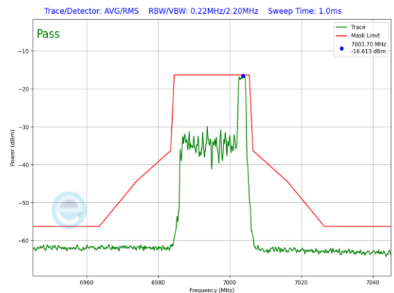
Plot 7-1382. LPI In-Band Emission Plot SDM Primary Antenna 3a (20MHz 802.11ax RU26 (UNII Band 8) – Ch. 209)
