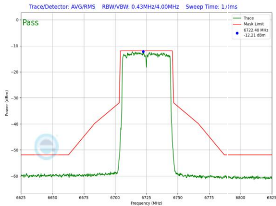
Plot 7-1360. LPI In-Band Emission Plot SDM Primary Antenna 3a (40MHz 802.11ax RU484 (UNII Band 7) – Ch. 155)
