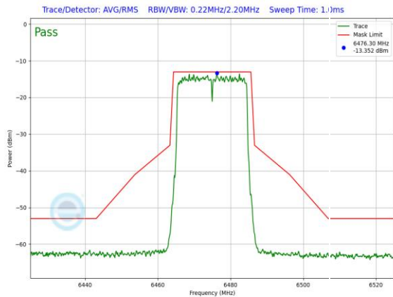
Plot 7-1447. LPI In-Band Emission Plot SDM Diversity Antenna 3c (20MHz 802.11ax RU242 (UNII Band 6) – Ch. 105)
