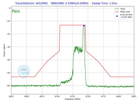
Plot 7-1358. LPI In-Band Emission Plot SDM Primary Antenna 3a (40MHz 802.11ax RU26 (UNII Band 7) – Ch. 155)
