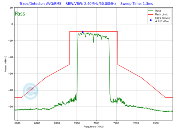
Plot 7-1408. LPI In-Band Emission Plot SDM Primary Antenna 3a (160MHz 802.11ax RU996x2 (UNII Band 8) – Ch. 207)
