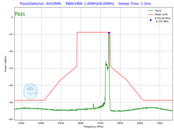
Plot 7-1374. LPI In-Band Emission Plot SDM Primary Antenna 3a (160MHz 802.11ax RU26 (UNII Band 7) – Ch. 143)
