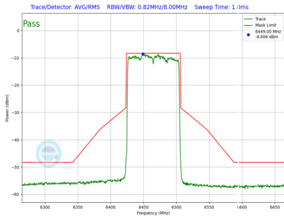
Plot 7-1336. LPI In-Band Emission Plot SDM Primary Antenna 3a (80MHz) 802.11ax RU996 (UNII Band 6) – Ch. 103
