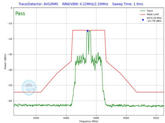
Plot 7-1443. LPI In-Band Emission Plot SDM Diversity Antenna 3c (20MHz 802.11ax RU26 (UNII Band 6) – Ch. 105)
