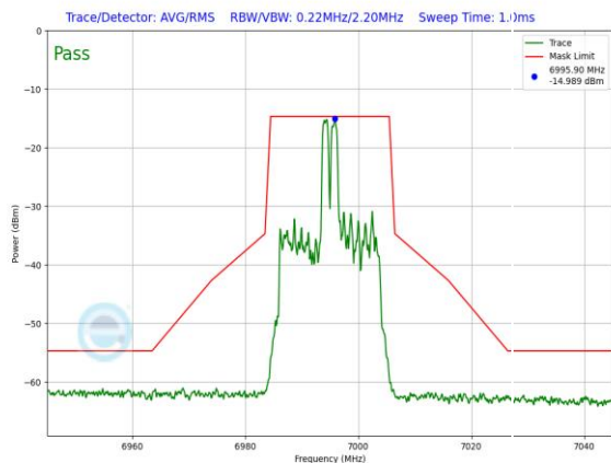
Plot 7-1379. LPI In-Band Emission Plot SDM Primary Antenna 3c (20MHz 802.11ax RU26 (UNII Band 8) – Ch. 209)
