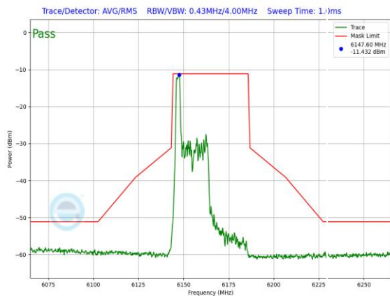
Plot 7-1417. LPI In-Band Emission Plot SDM Diversity Antenna 3c (40MHz 802.11ax RU26 (UNII Band 5) – Ch. 43)
