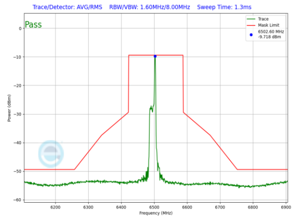
Plot 7-1339. LPI In-Band Emission Plot SDM Primary Antenna 3c (160MHz) 802.11ax RU26 (UNII Band 6) – Ch. 111
