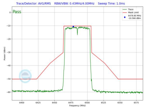
Plot 7-1455. LPI In-Band Emission Plot SDM Diversity Antenna 3c (40MHz 802.11ax RU484 (UNII Band 6) – Ch. 107)
