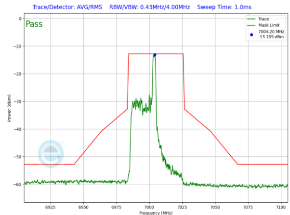
Plot 7-1388. LPI In-Band Emission Plot SDM Primary Antenna 3a (40MHz) 802.11ax RU26 (UNII Band 8) – Ch. 211)
