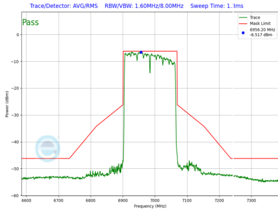
Plot 7-1407. LPI In-Band Emission Plot SDM Primary Antenna 3c (160MHz 802.11ax RU996x2 (UNII Band 8) – Ch. 207)
