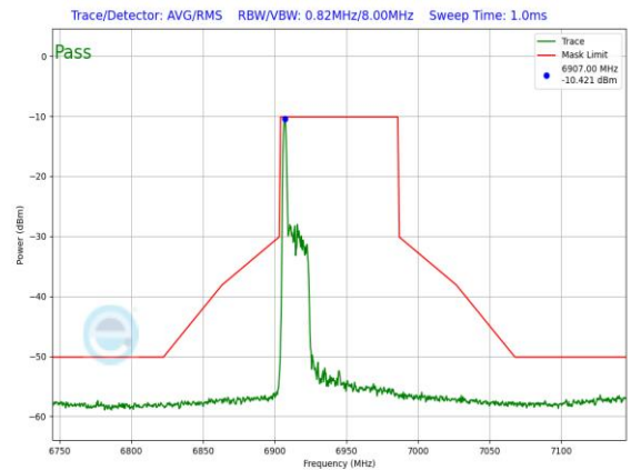
Plot 7-1393. LPI In-Band Emission Plot SDM Primary Antenna 3c (80MHz 802.11ax RU26 (UNII Band 8) – Ch. 199)
