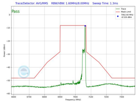
Plot 7-1405. LPI In-Band Emission Plot SDM Primary Antenna 3c (160MHz 802.11ax RU26 (UNII Band 8) – Ch. 207)
