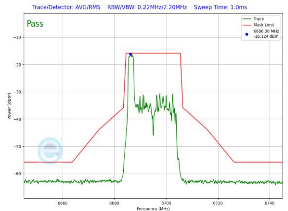
Plot 7-1346. LPI In-Band Emission Plot SDM Primary Antenna 3a (20MHz 802.11ax RU26 (UNII Band 7) – Ch. 149)
