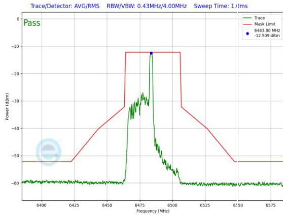
Plot 7-1451. LPI In-Band Emission Plot SDM Diversity Antenna 3c (40MHz 802.11ax RU26 (UNII Band 6) – Ch. 107)
