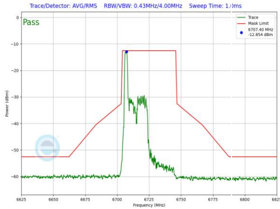
Plot 7-1353. LPI In-Band Emission Plot SDM Primary Antenna 3c (40MHz 802.11ax RU26 (UNII Band 7) – Ch. 155)
