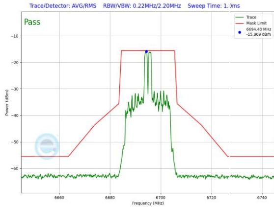
Plot 7-1475. LPI In-Band Emission Plot SDM Diversity Antenna 3c (20MHz 802.11ax RU26 (UNII Band 7) – Ch. 149)
