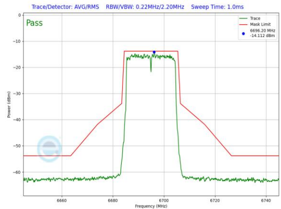
Plot 7-1351. LPI In-Band Emission Plot SDM Primary Antenna 3c (20MHz 802.11ax RU242 (UNII Band 7) – Ch. 149)
