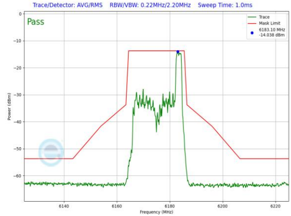
Plot 7-1413. LPI In-Band Emission Plot SDM Diversity Antenna 3c (20MHz 802.11ax RU26 (UNII Band 5) – Ch. 45)
