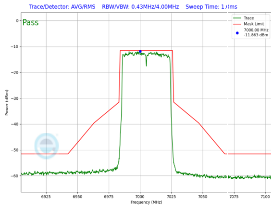
Plot 7-1391. LPI In-Band Emission Plot SDM Primary Antenna 3c (40MHz 802.11ax RU484 (UNII Band 8) – Ch. 211)
