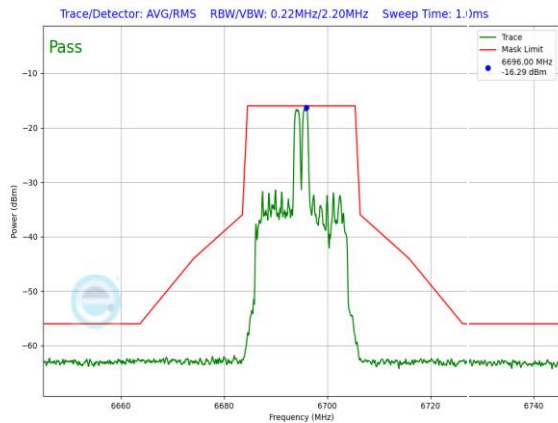
Plot 7-1348. LPI In-Band Emission Plot SDM Primary Antenna 3a (20MHz 802.11ax RU26 (UNII Band 7) – Ch. 149)
