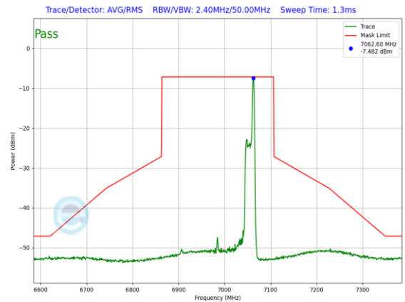
Plot 7-1406. LPI In-Band Emission Plot SDM Primary Antenna 3a (160MHz 802.11ax RU26 (UNII Band 8) – Ch. 207)
