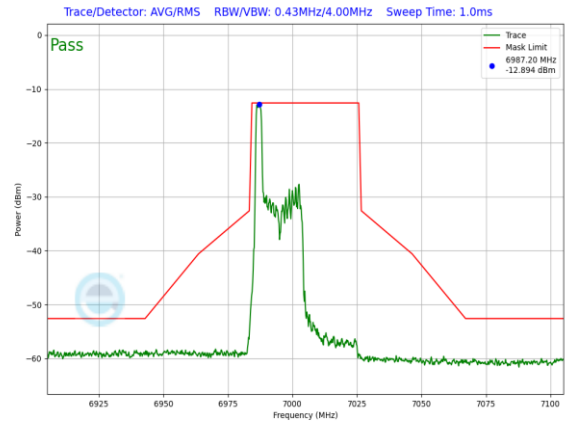
Plot 7-1386. LPI In-Band Emission Plot SDM Primary Antenna 3a (40MHz) 802.11ax RU26 (UNII Band 8) – Ch. 211)
