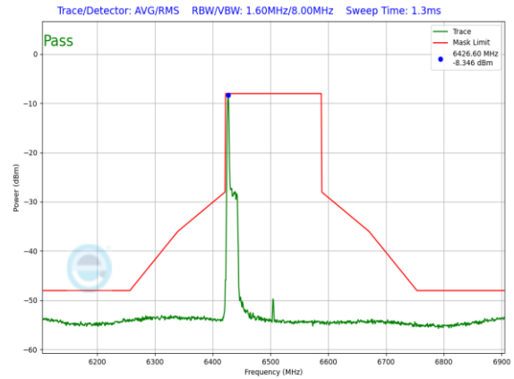
Plot 7-1338. LPI In-Band Emission Plot SDM Primary Antenna 3a (160MHz) 802.11ax RU26 (UNII Band 6) – Ch. 111
