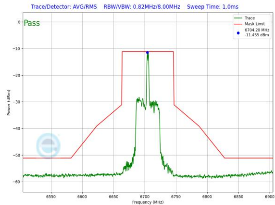
Plot 7-1363. LPI In-Band Emission Plot SDM Primary Antenna 3c (80MHz 802.11ax RU26 (UNII Band 7) – Ch. 151)
