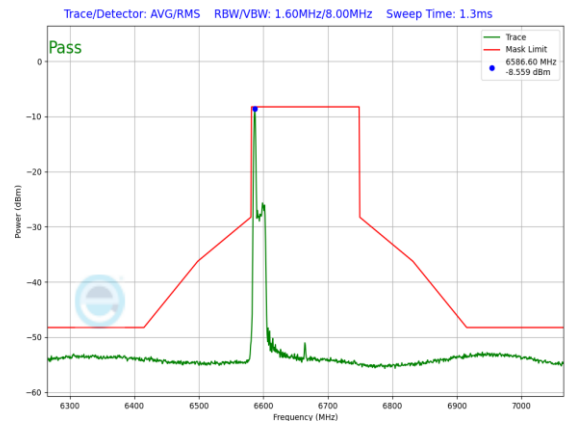
Plot 7-1370. LPI In-Band Emission Plot SDM Primary Antenna 3a (160MHz 802.11ax RU26 (UNII Band 7) – Ch. 143)
