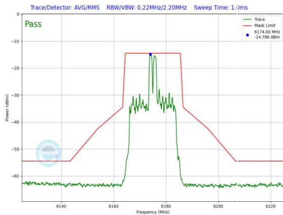
Plot 7-1411. LPI In-Band Emission Plot SDM Diversity Antenna 3c (20MHz 802.11ax RU26 (UNII Band 5) – Ch. 45)
