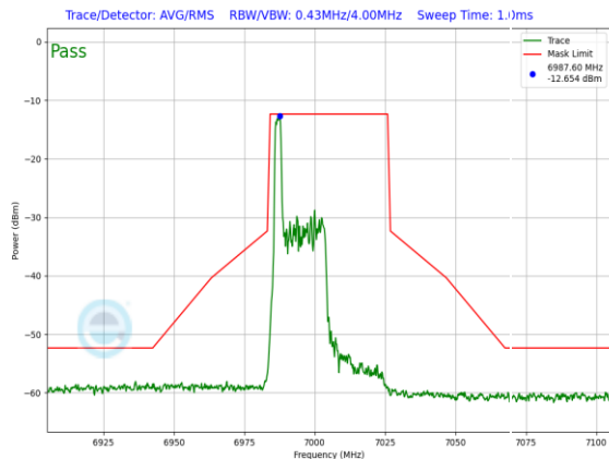
Plot 7-1385. LPI In-Band Emission Plot SDM Primary Antenna 3c (40MHz) 802.11ax RU26 (UNII Band 8) – Ch. 211)
