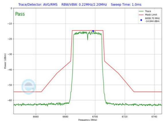
Plot 7-1352. LPI In-Band Emission Plot SDM Primary Antenna 3a (20MHz 802.11ax RU242 (UNII Band 7) – Ch. 149)
