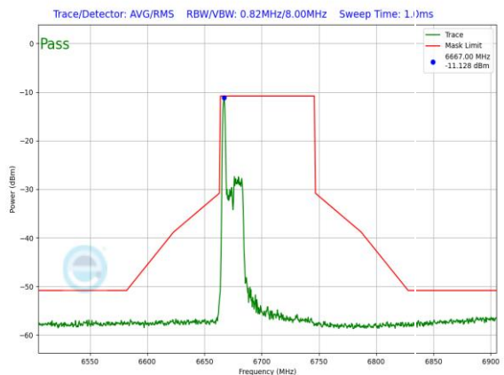
Plot 7-1361. LPI In-Band Emission Plot SDM Primary Antenna 3c (80MHz 802.11ax RU26 (UNII Band 7) – Ch. 151)
