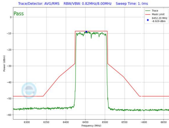
Plot 7-1335. LPI In-Band Emission Plot SDM Primary Antenna 3c (80MHz) 802.11ax RU996 (UNII Band 6) – Ch. 103
