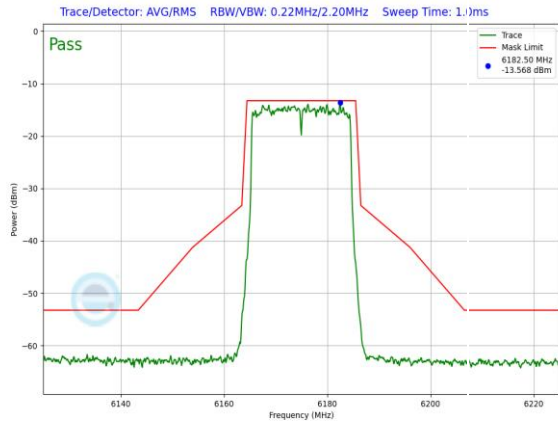
Plot 7-1415. LPI In-Band Emission Plot SDM Diversity Antenna 3c (20MHz 802.11ax RU242 (UNII Band 5) – Ch. 45)
