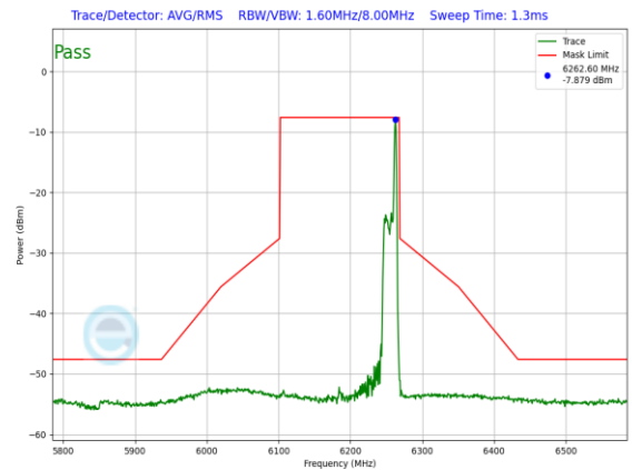
Plot 7-1437. LPI In-Band Emission Plot SDM Diversity Antenna 3c (160MHz 802.11ax RU26 (UNII Band 5) – Ch. 47)
