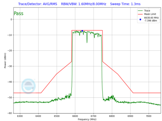
Plot 7-1376. LPI In-Band Emission Plot SDM Primary Antenna 3a (160MHz 802.11ax RU996x2 (UNII Band 7) – Ch. 143)
