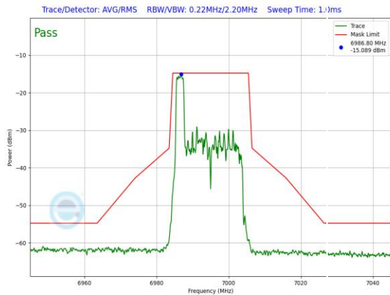
Plot 7-1378. LPI In-Band Emission Plot SDM Primary Antenna 3a (20MHz 802.11ax RU26 (UNII Band 8) – Ch. 209)
