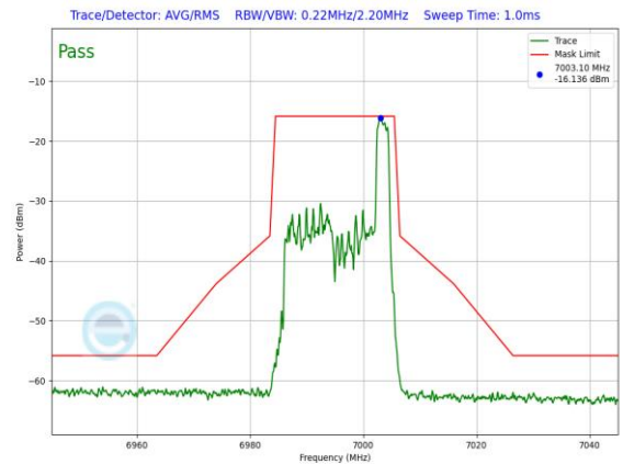
Plot 7-1381. LPI In-Band Emission Plot SDM Primary Antenna 3c (20MHz 802.11ax RU26 (UNII Band 8) – Ch. 209)
