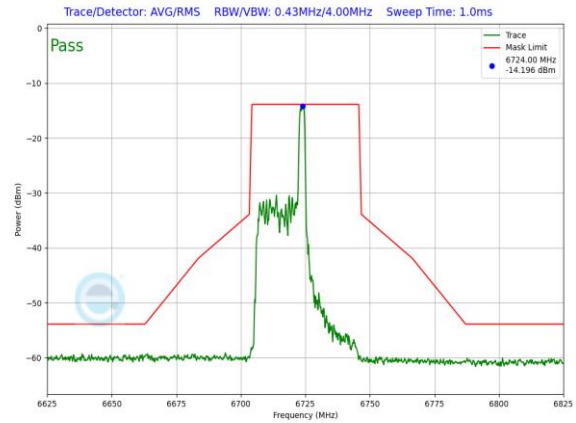
Plot 7-1356. LPI In-Band Emission Plot SDM Primary Antenna 3a (40MHz 802.11ax RU26 (UNII Band 7) – Ch. 155)
