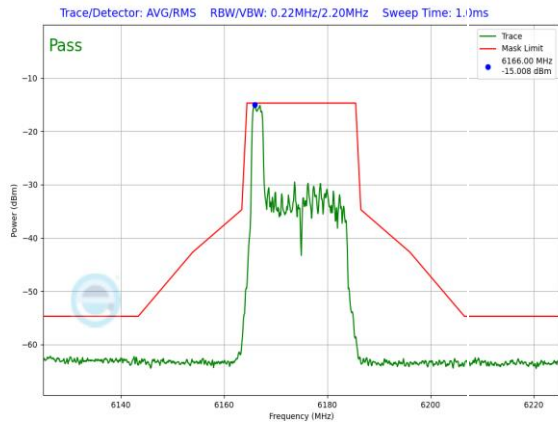
Plot 7-1409. LPI In-Band Emission Plot SDM Diversity Antenna 3c (20MHz 802.11ax RU26 (UNII Band 5) – Ch. 45)
