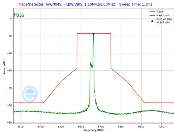
Plot 7-1372. LPI In-Band Emission Plot SDM Primary Antenna 3a (160MHz 802.11ax RU26 (UNII Band 7) – Ch. 143)
