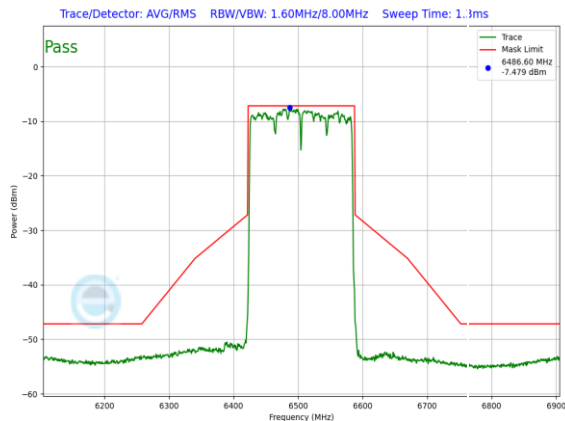
Plot 7-1343. LPI In-Band Emission Plot SDM Primary Antenna 3c (160MHz 802.11ax RU996x2 (UNII Band 6) – Ch. 111)
