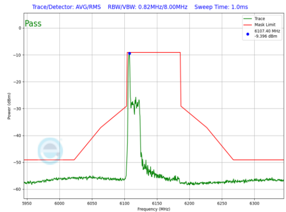
Plot 7-1425. LPI In-Band Emission Plot SDM Diversity Antenna 3c (80MHz 802.11ax RU26 (UNII Band 5) – Ch. 39)
