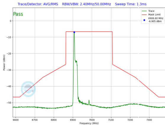
Plot 7-1402. LPI In-Band Emission Plot SDM Primary Antenna 3a (160MHz 802.11ax RU26 (UNII Band 8) – Ch. 207)
