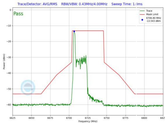
Plot 7-1354. LPI In-Band Emission Plot SDM Primary Antenna 3a (40MHz 802.11ax RU26 (UNII Band 7) – Ch. 155)
