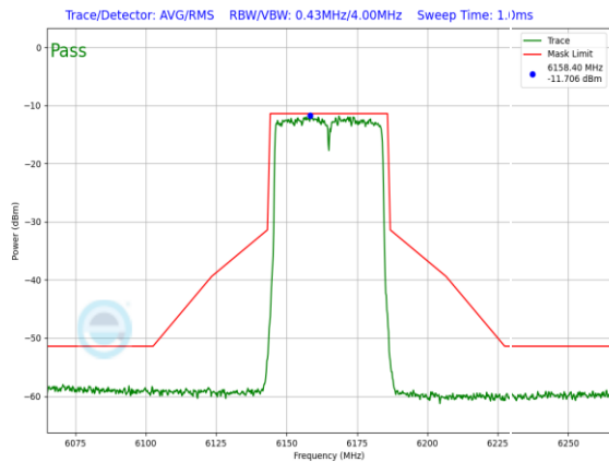
Plot 7-1423. LPI In-Band Emission Plot SDM Diversity Antenna 3c (40MHz 802.11ax RU484 (UNII Band 5) – Ch. 43)
