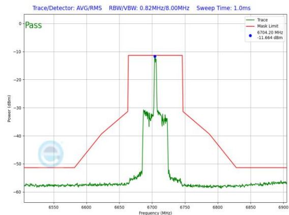
Plot 7-1364. LPI In-Band Emission Plot SDM Primary Antenna 3a (80MHz 802.11ax RU26 (UNII Band 7) – Ch. 151)
