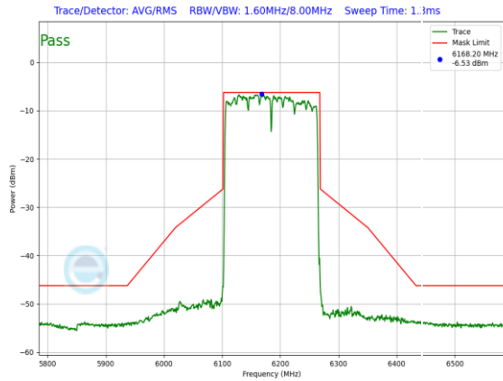
Plot 7-1439. LPI In-Band Emission Plot SDM Diversity Antenna 3c (160MHz 802.11ax RU996x2 (UNII Band 5) – Ch. 47)
