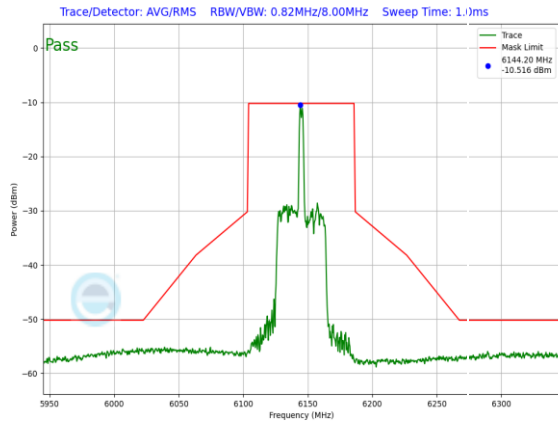
Plot 7-1427. LPI In-Band Emission Plot SDM Diversity Antenna 3c (80MHz 802.11ax RU26 (UNII Band 5) – Ch. 39)
