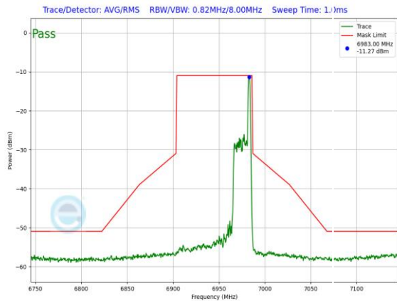
Plot 7-1397. LPI In-Band Emission Plot SDM Primary Antenna 3c (80MHz 802.11ax RU26 (UNII Band 8) – Ch. 199)
