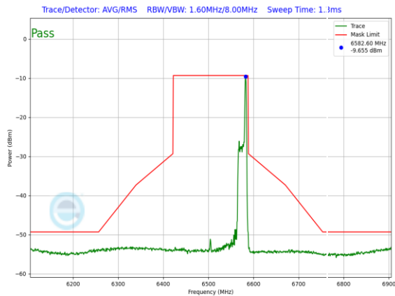
Plot 7-1342. LPI In-Band Emission Plot SDM Primary Antenna 3a (160MHz 802.11ax RU26 (UNII Band 6) – Ch. 111)
