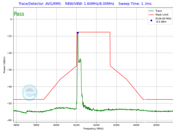
Plot 7-1433. LPI In-Band Emission Plot SDM Diversity Antenna 3c (160MHz 802.11ax RU26 (UNII Band 5) – Ch. 47)
