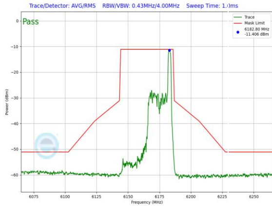
Plot 7-1421. LPI In-Band Emission Plot SDM Diversity Antenna 3c (40MHz 802.11ax RU26 (UNII Band 5) – Ch. 43)
