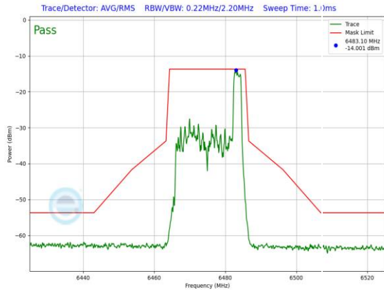
Plot 7-1445. LPI In-Band Emission Plot SDM Diversity Antenna 3c (20MHz 802.11ax RU26 (UNII Band 6) – Ch. 105)
