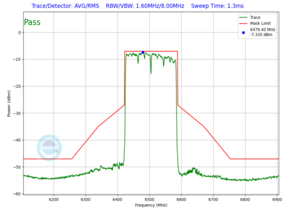
Plot 7-1344. LPI In-Band Emission Plot SDM Primary Antenna 3a (160MHz 802.11ax RU996x2 (UNII Band 6) – Ch. 111)
