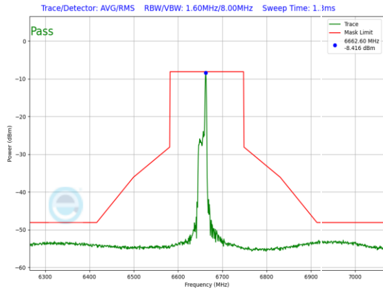
Plot 7-1371. LPI In-Band Emission Plot SDM Primary Antenna 3c (160MHz 802.11ax RU26 (UNII Band 7) – Ch. 143)
