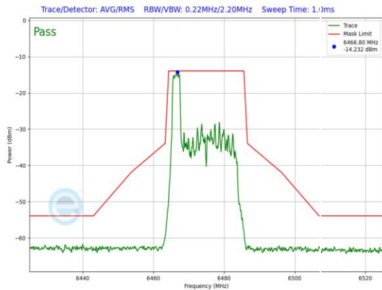
Plot 7-1441. LPI In-Band Emission Plot SDM Diversity Antenna 3c (20MHz 802.11ax RU26 (UNII Band 6) – Ch. 105)
