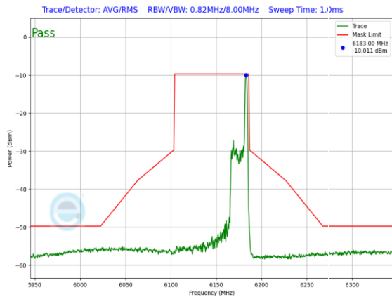
Plot 7-1429. LPI In-Band Emission Plot SDM Diversity Antenna 3c (80MHz 802.11ax RU26 (UNII Band 5) – Ch. 39)
