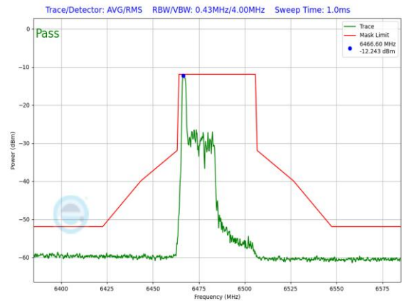
Plot 7-1449. LPI In-Band Emission Plot SDM Diversity Antenna 3c (40MHz 802.11ax RU26 (UNII Band 6) – Ch. 107)
