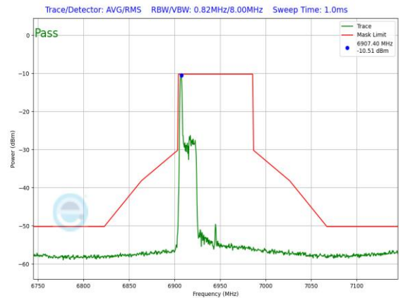
Plot 7-1394. LPI In-Band Emission Plot SDM Primary Antenna 3a (80MHz 802.11ax RU26 (UNII Band 8) – Ch. 199)
