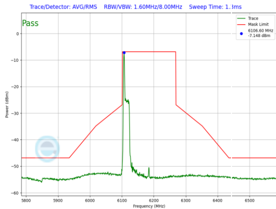
Plot 7-1306. LPI In-Band Emission Plot SDM Primary Antenna 3a (160MHz 802.11ax RU26 (UNII Band 5) – Ch. 47)
