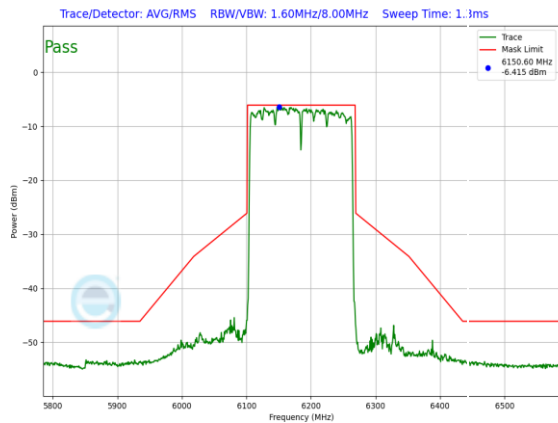
Plot 7-1312. LPI In-Band Emission Plot SDM Primary Antenna 3a (160MHz 802.11ax RU996x2 (UNII Band 5) – Ch. 47)
