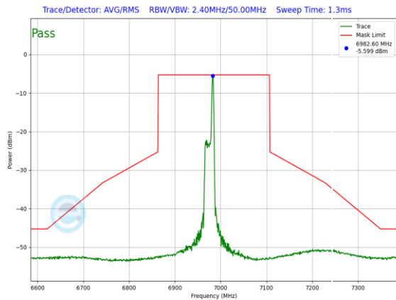
Plot 7-1214. LPI In-Band Emission Plot Antenna 3a (160MHz 802.11ax RU26 (UNII Band 8) – Ch. 207)
