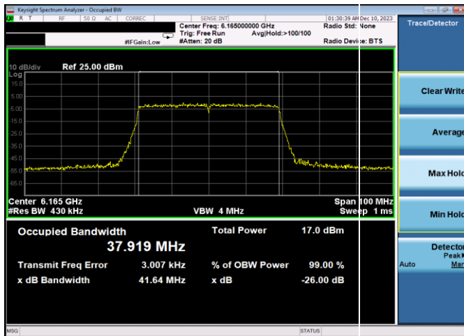
Plot 7-8. 26dB & 99% Bandwidth Plot Antenna 3c (40MHz 802.11ax RU484 (UNII Band 5) – Ch. 43)
