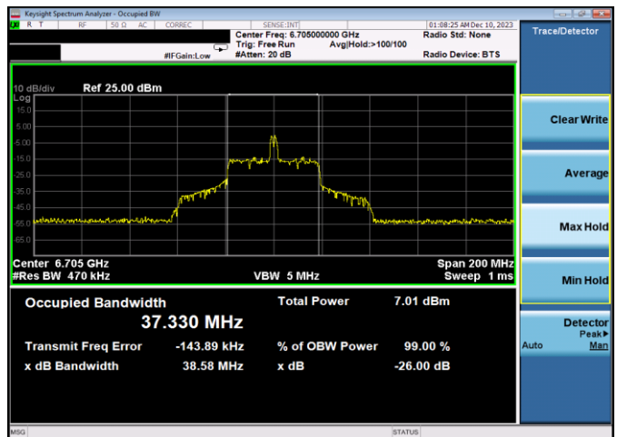
Plot 7-42. 26dB & 99% Bandwidth Plot Antenna 3c (80MHz 802.11ax RU2 (UNII Band 7) – Ch. 151)
