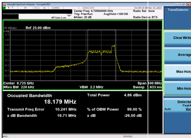
Plot 7-39. 26dB & 99% Bandwidth Plot Antenna 3c (40MHz 802.11ax RU26 (UNII Band 7) – Ch. 155)
