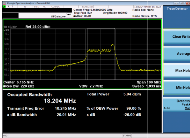
Plot 7-7. 26dB & 99% Bandwidth Plot Antenna 3c (40MHz 802.11ax RU26 (UNII Band 5) – Ch. 43)
