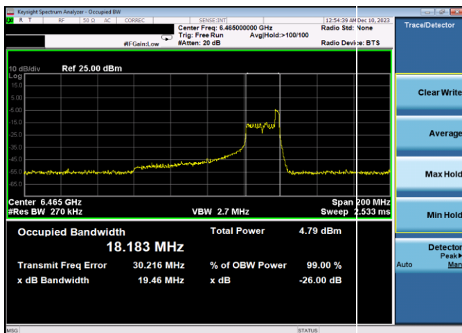
Plot 7-27. 26dB & 99% Bandwidth Plot Antenna 3c (80MHz 802.11ax RU26 (UNII Band 6) – Ch. 103)
