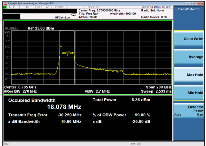
Plot 7-41. 26dB & 99% Bandwidth Plot Antenna 3c (80MHz 802.11ax RU2 (UNII Band 7) – Ch. 151)
