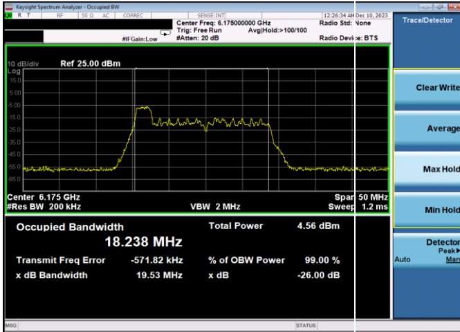
Plot 7-1. 26dB & 99% Bandwidth Plot Antenna 3c (20MHz 802.11ax RU26 (UNII Band 5) – Ch. 45)
