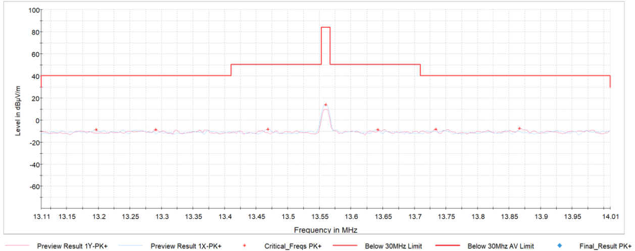
Plot 7-1. In Band Radiated Spurious Emissions (Charging Rate 2.6C, with AC/DC Adapter)
