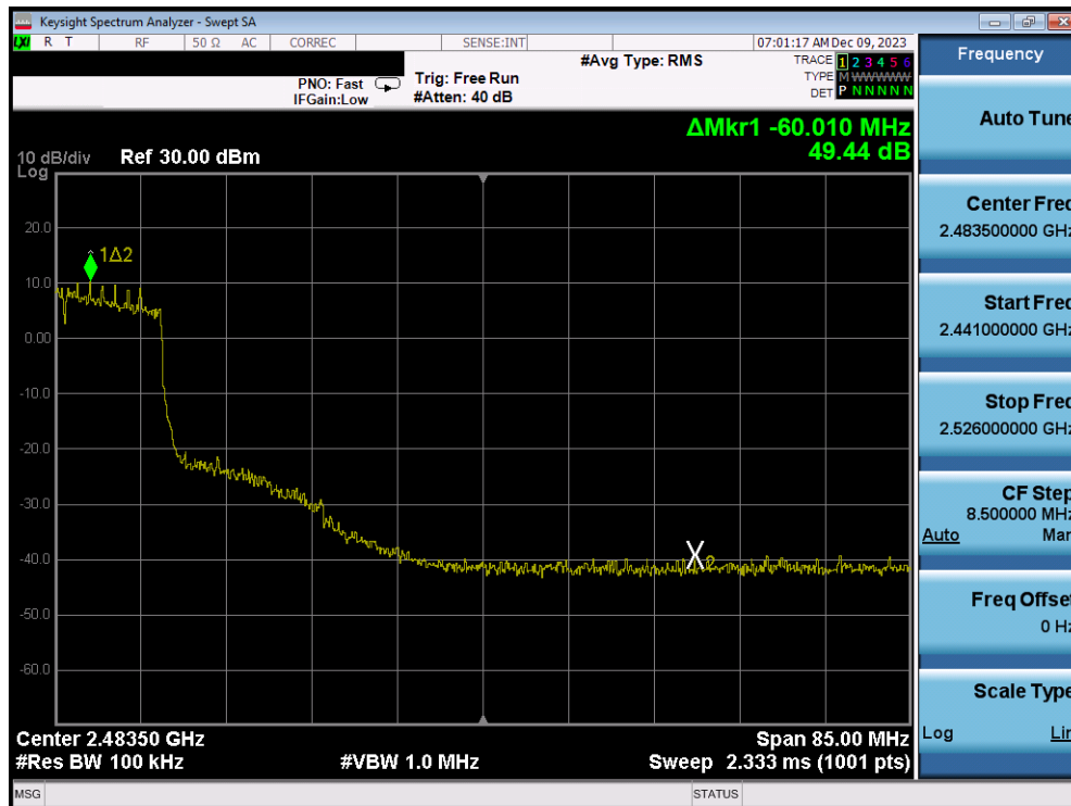
Plot 7-334. Band Edge Plot Antenna 1a (802.11ax (SU - 2.4GHz) – Ch. 7) – MCS2
