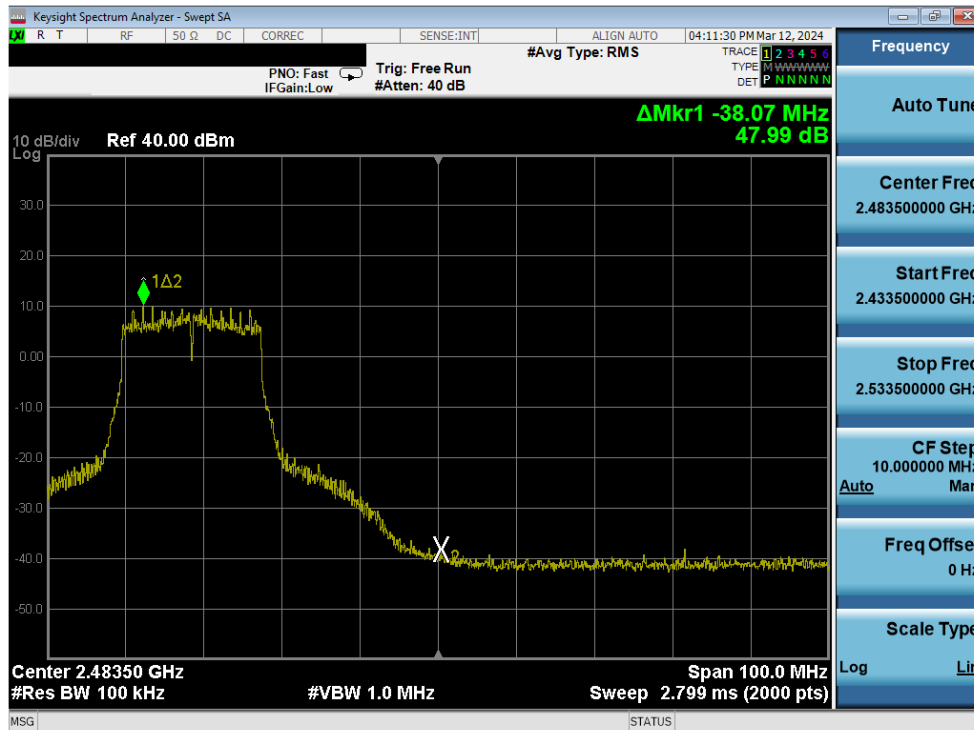
Plot 7-363. Band Edge Plot Antenna 1a (802.11n (2.4GHz) – Ch. 9) – MCS4
