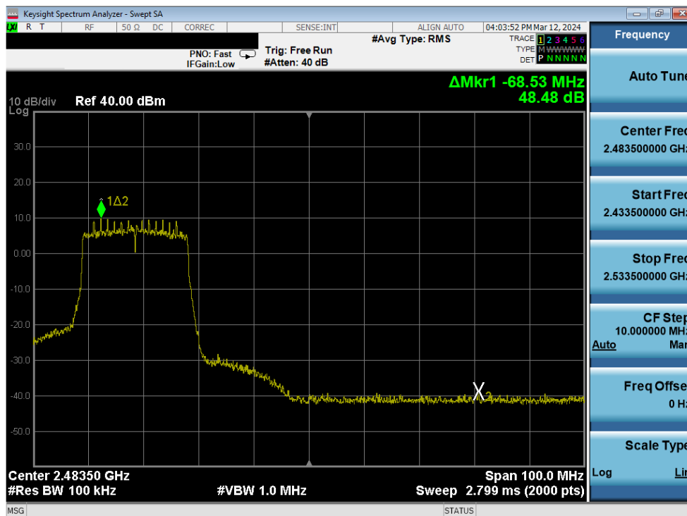
Plot 7-336. Band Edge Plot Antenna 1a (802.11ax (SU - 2.4GHz) – Ch. 9) – MCS2
