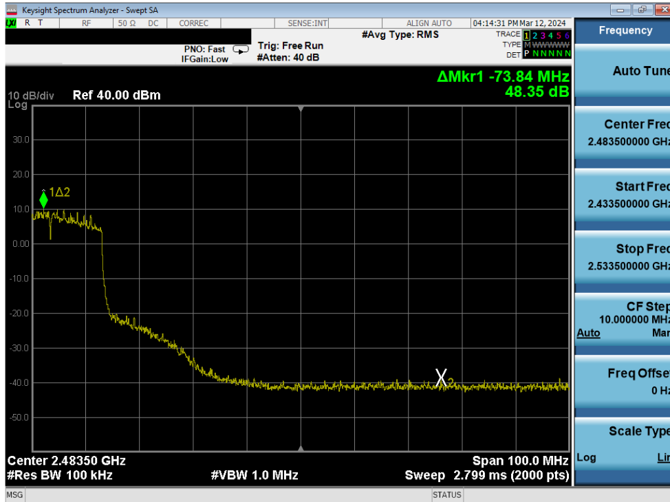
Plot 7-374. Band Edge Plot Antenna 1a (802.11ax (SU - 2.4GHz) – Ch. 6 (high)) – MCS4
