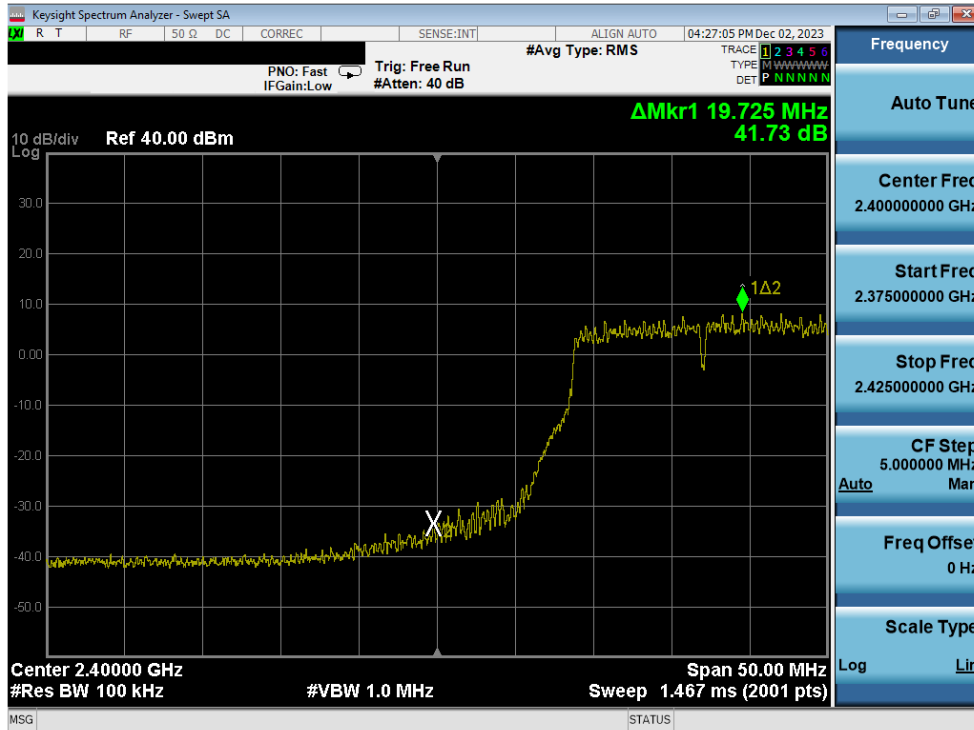
Plot 7-261. Band Edge Plot Antenna 3a (802.11g – Ch. 2) – 54Mbps
