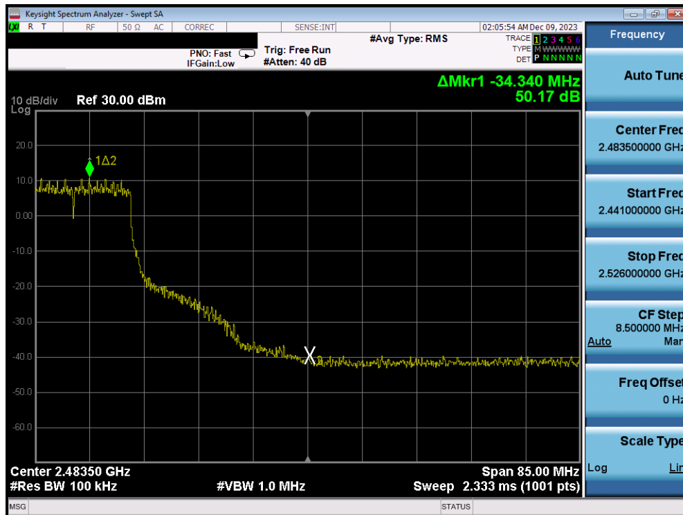
Plot 7-282. Band Edge Plot Antenna 3a (802.11n (2.4GHz) – Ch. 8) – MCS7
