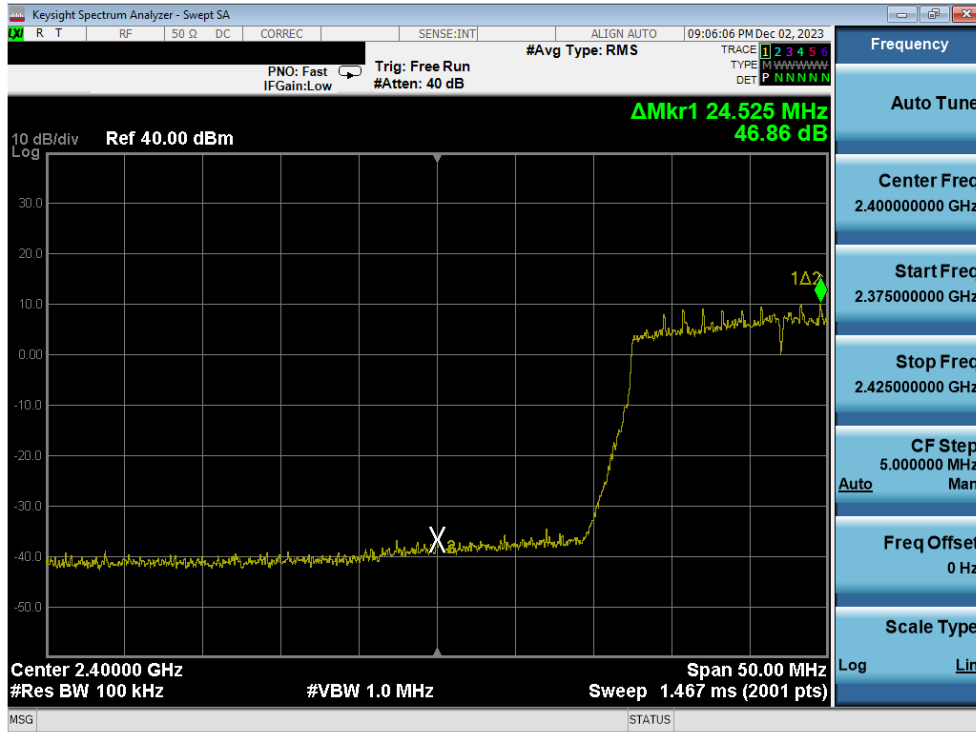
Plot 7-329. Band Edge Plot Antenna 1a (802.11ax (SU - 2.4GHz) – Ch. 3) – MCS2
