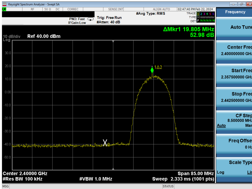
Plot 7-256. Band Edge Plot Antenna 3a (802.11b – Ch. 2) – 11Mbps
