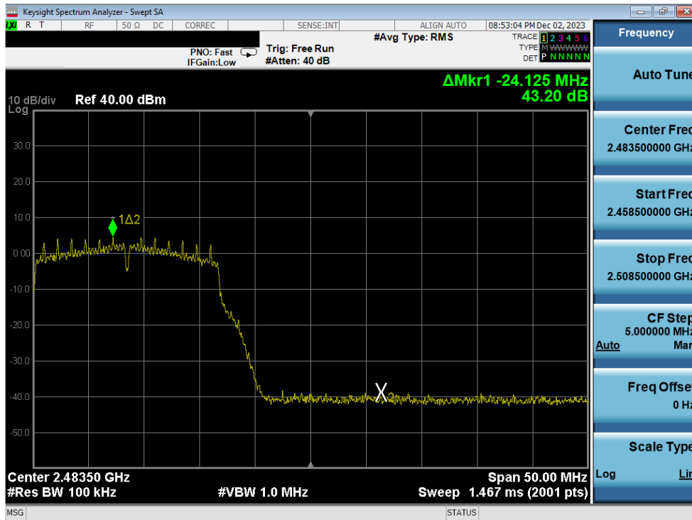
Plot 7-312. Band Edge Plot Antenna 1a (802.11g – Ch. 12) – 12Mbps
