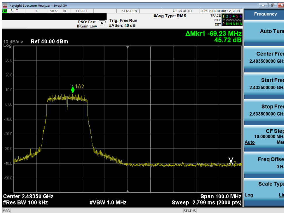
Plot 7-284. Band Edge Plot Antenna 3a (802.11n (2.4GHz) – Ch. 10) – MCS7
