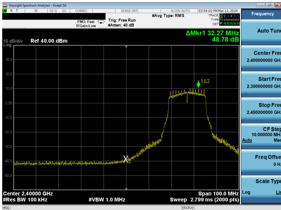
Plot 7-304. Band Edge Plot Antenna 1a (802.11g - Ch. 4) - 12Mbps
