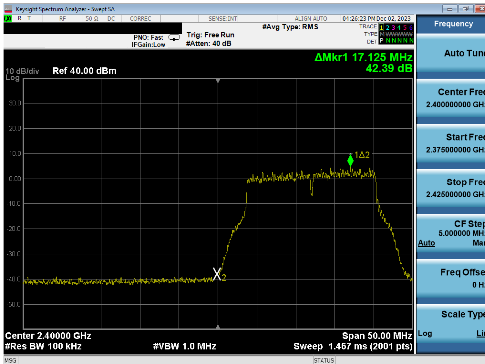
Plot 7-260. Band Edge Plot Antenna 3a (802.11g – Ch. 1) – 54Mbps
