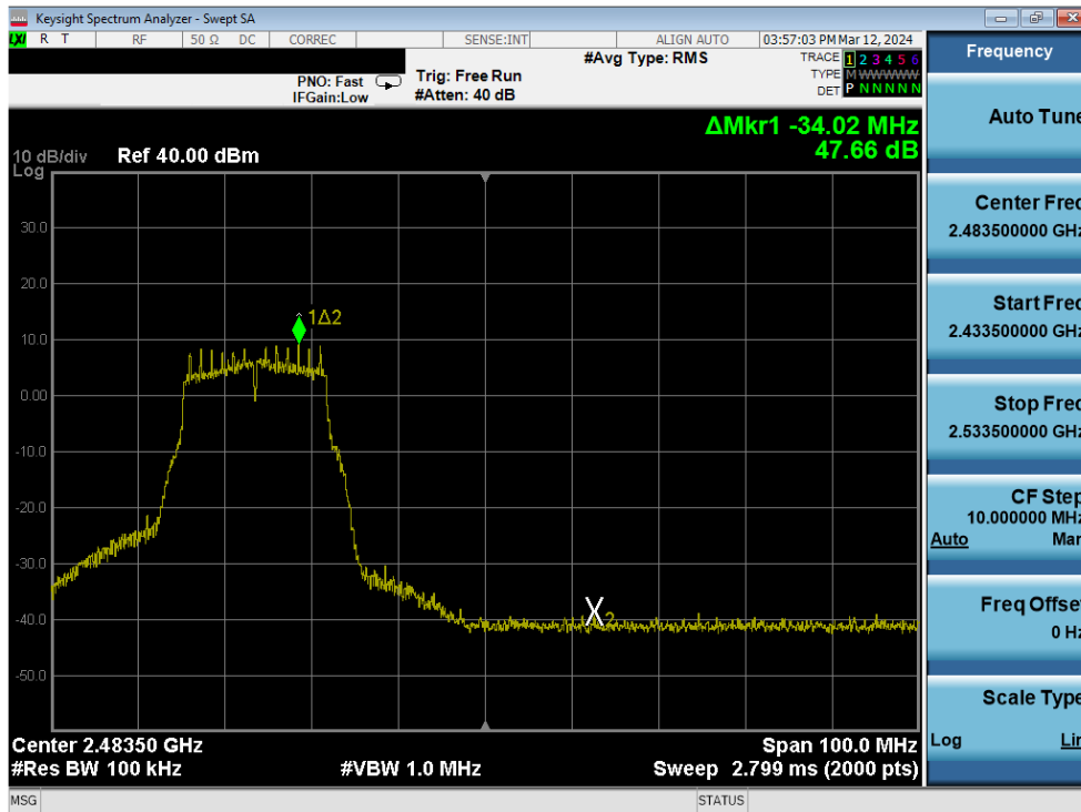
Plot 7-310. Band Edge Plot Antenna 1a (802.11g – Ch. 10) – 12Mbps
