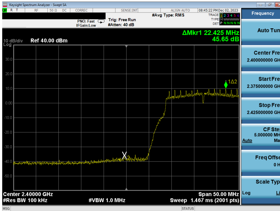
Plot 7-302. Band Edge Plot Antenna 1a (802.11g – Ch. 2) – 12Mbps
