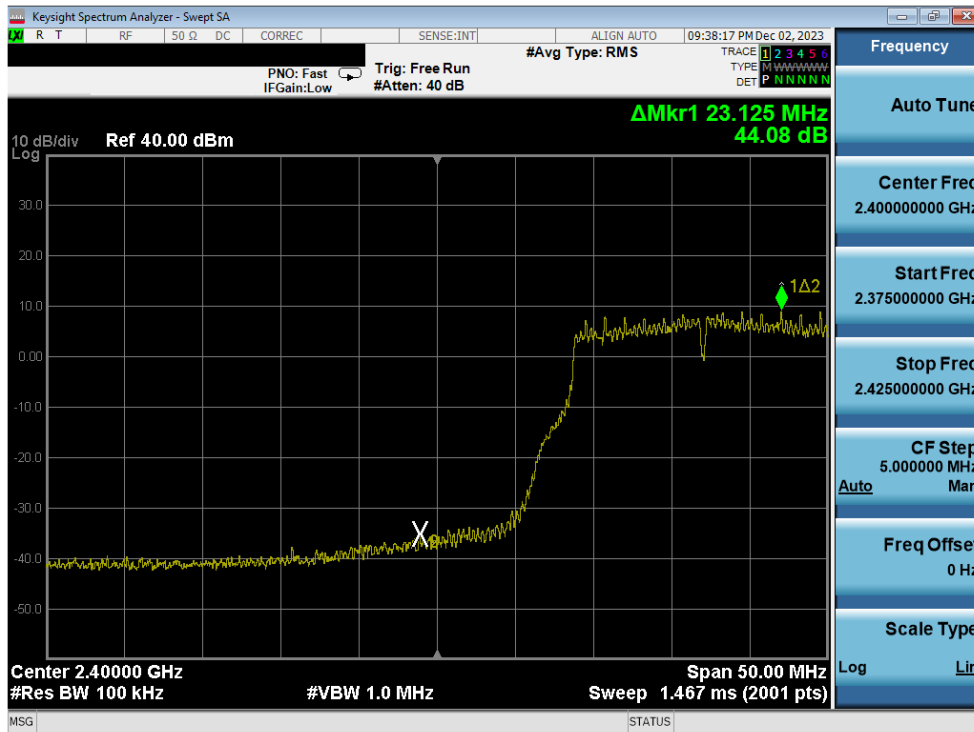
Plot 7-341. Band Edge Plot Antenna 1a (802.11g – Ch. 2) – 24Mbps
