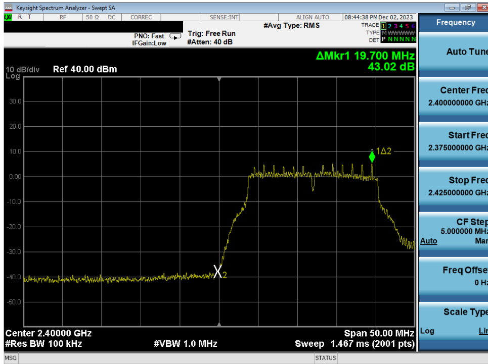
Plot 7-301. Band Edge Plot Antenna 1a (802.11g – Ch. 1) – 12Mbps
