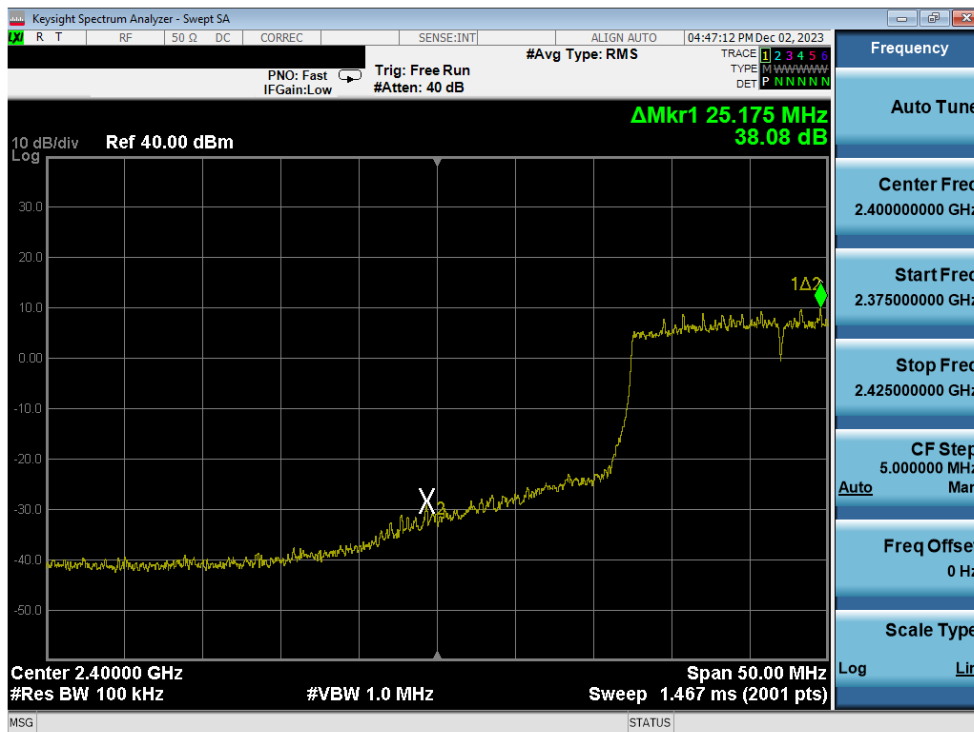
Plot 7-290. Band Edge Plot Antenna 3a (802.11ax (SU - 2.4GHz) – Ch. 3) – MCS9
