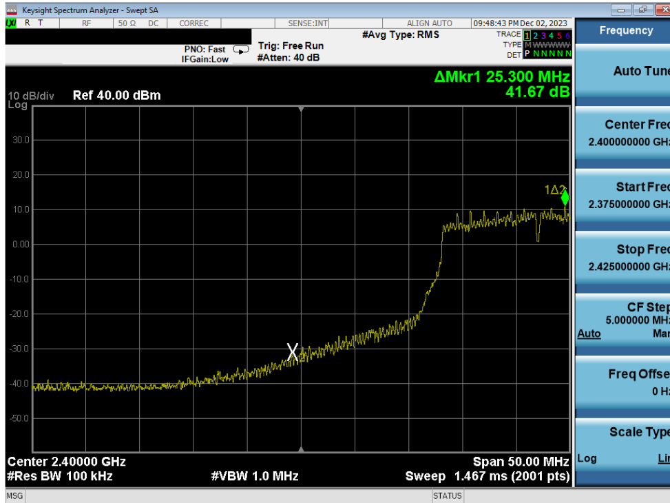
Plot 7-356. Band Edge Plot Antenna 1a (802.11n (2.4GHz) – Ch. 3) – MCS4
