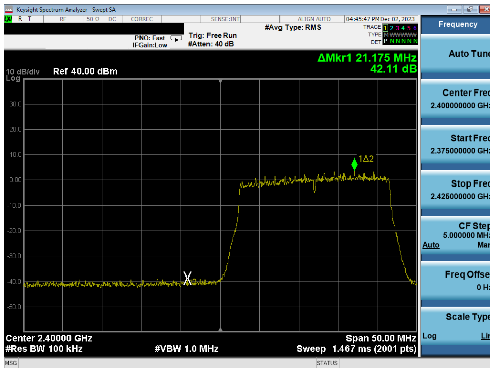
Plot 7-288. Band Edge Plot Antenna 3a (802.11ax (SU - 2.4GHz) – Ch. 1) – MCS9
