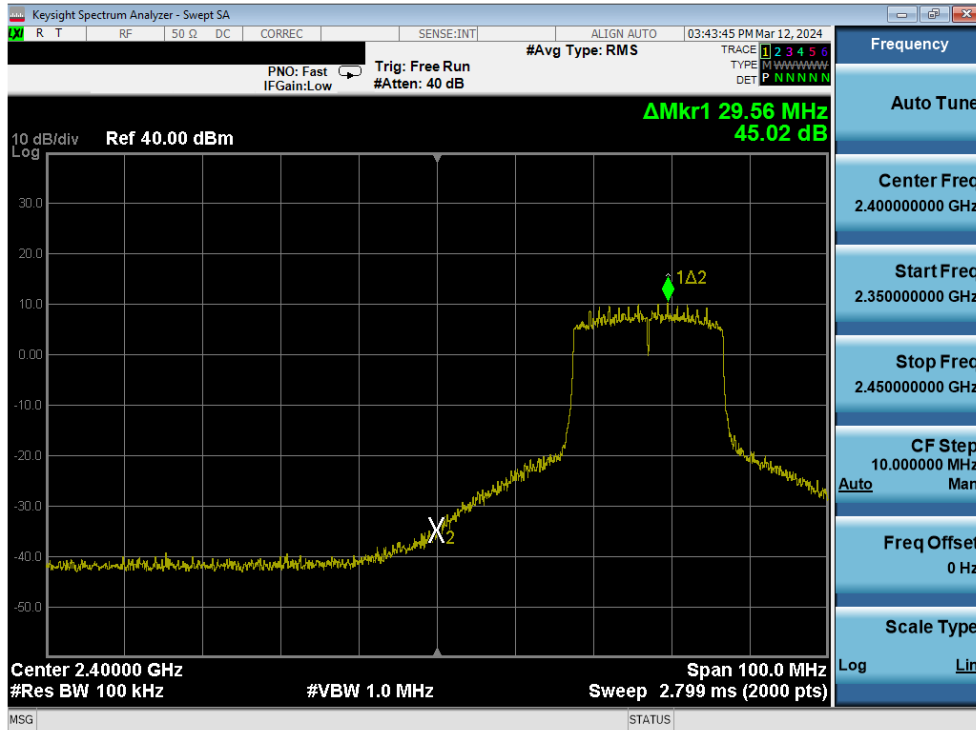
Plot 7-291. Band Edge Plot Antenna 3a (802.11ax (SU - 2.4GHz) – Ch. 4) – MCS9
