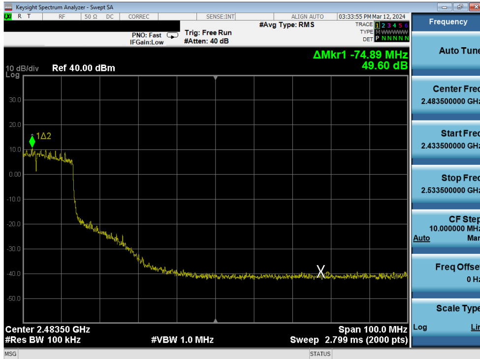
Plot 7-248. Band Edge Plot Antenna 3a (802.11ax (SU - 2.4GHz) – Ch. 6 (high)) – MCS4
