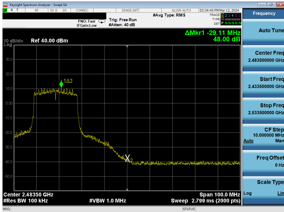
Plot 7-251. Band Edge Plot Antenna 3a (802.11ax (SU - 2.4GHz) – Ch. 9) – MCS4
