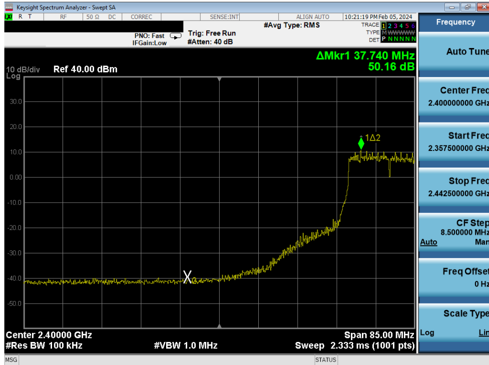
Plot 7-279. Band Edge Plot Antenna 3a (802.11n (2.4GHz) – Ch. 6(low)) – MCS7
