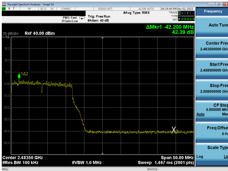
Plot 7-272. Band Edge Plot Antenna 3a (802.11g – Ch. 12) – 54Mbps
