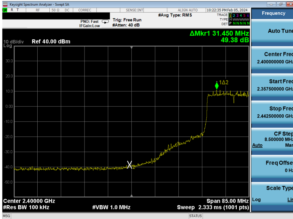
Plot 7-293. Band Edge Plot Antenna 3a (802.11ax (SU - 2.4GHz) – Ch. 6 (low)) – MCS9
