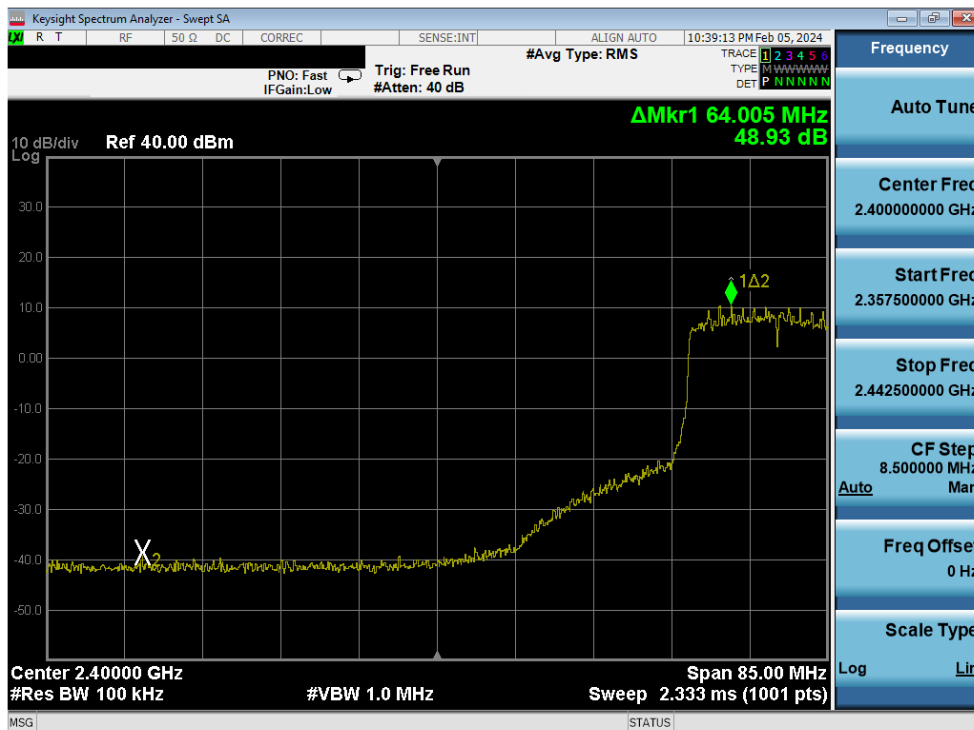
Plot 7-332. Band Edge Plot Antenna 1a (802.11ax (SU - 2.4GHz) – Ch. 6 (low)) – MCS2
