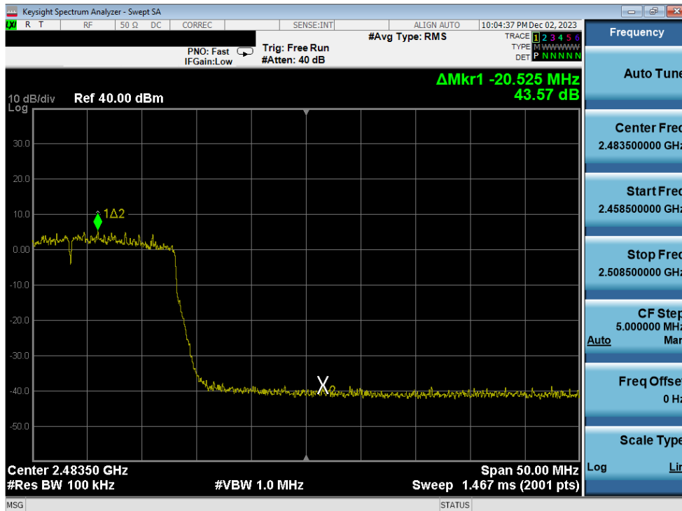
Plot 7-379. Band Edge Plot Antenna 1a (802.11ax (SU - 2.4GHz) – Ch. 11) – MCS4
