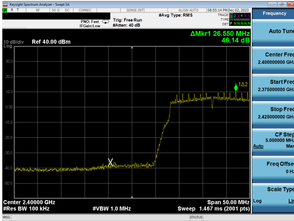
Plot 7-315. Band Edge Plot Antenna 1a (802.11n (2.4GHz) – Ch. 2) – MCS2
