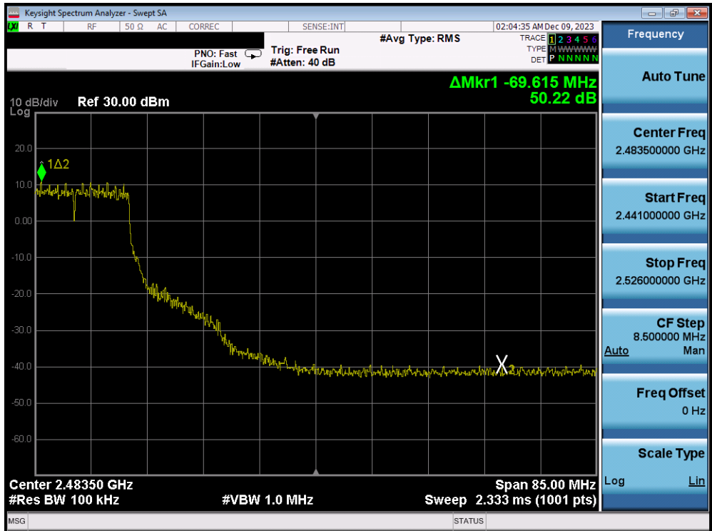
Plot 7-268. Band Edge Plot Antenna 3a (802.11g – Ch. 8) – 54Mbps
