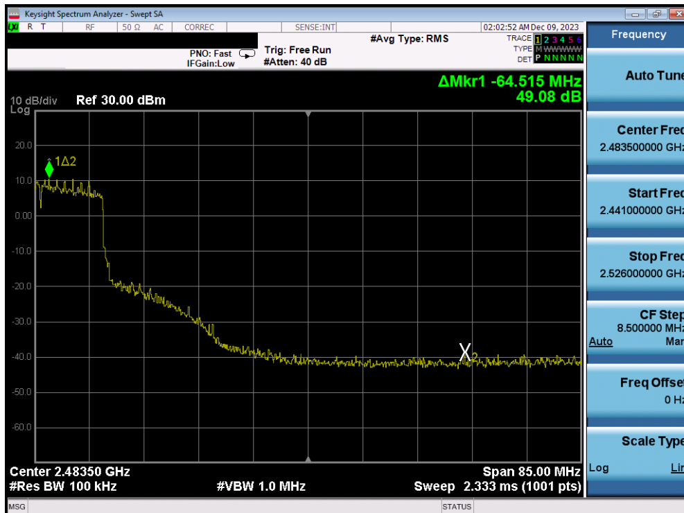
Plot 7-249. Band Edge Plot Antenna 3a (802.11ax (SU - 2.4GHz) – Ch. 7) – MCS4
