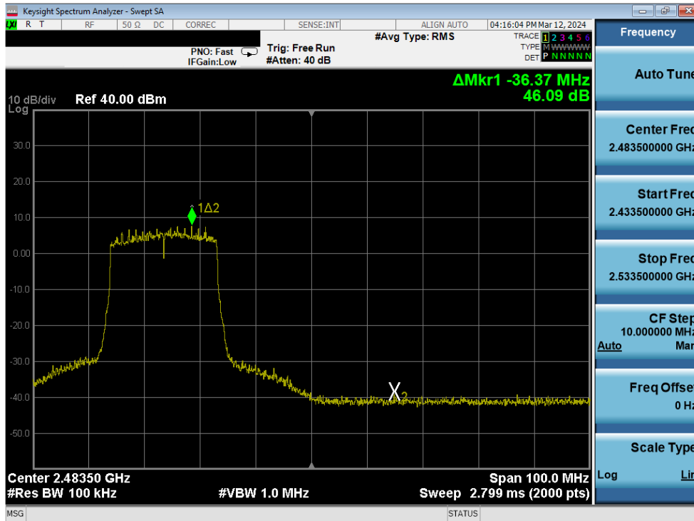
Plot 7-378. Band Edge Plot Antenna 1a (802.11ax (SU - 2.4GHz) – Ch. 10) – MCS4
