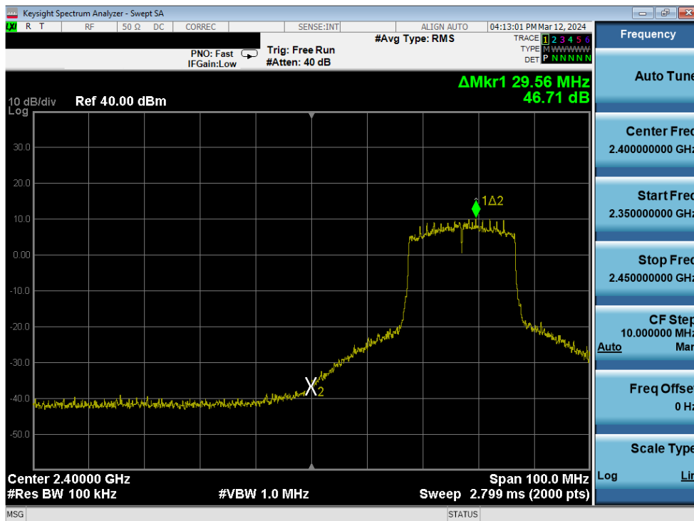
Plot 7-371. Band Edge Plot Antenna 1a (802.11ax (SU - 2.4GHz) – Ch. 4) – MCS4
