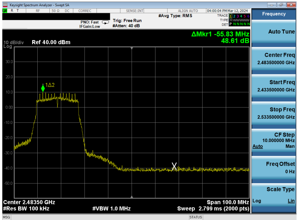
Plot 7-322. Band Edge Plot Antenna 1a (802.11n (2.4GHz) – Ch. 9) – MCS2
