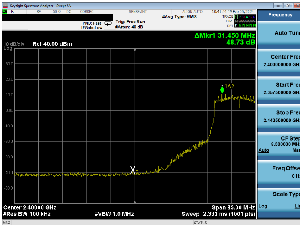
Plot 7-359. Band Edge Plot Antenna 1a (802.11n (2.4GHz) – Ch. 6(low)) – MCS4
