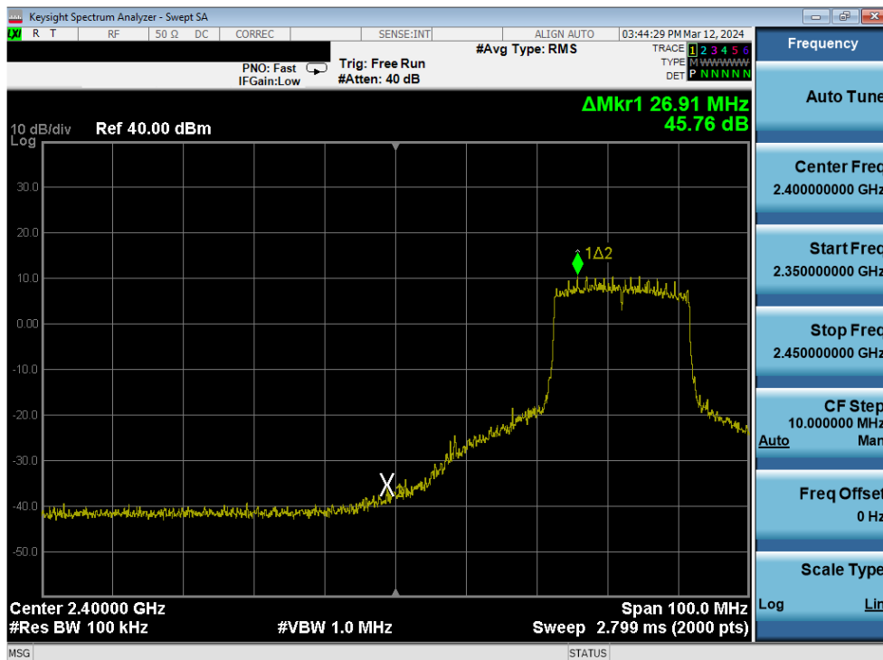
Plot 7-292. Band Edge Plot Antenna 3a (802.11ax (SU - 2.4GHz) – Ch. 5) – MCS9
