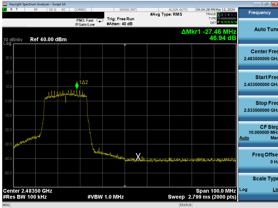
Plot 7-337. Band Edge Plot Antenna 1a (802.11ax (SU - 2.4GHz) – Ch. 10) – MCS2
