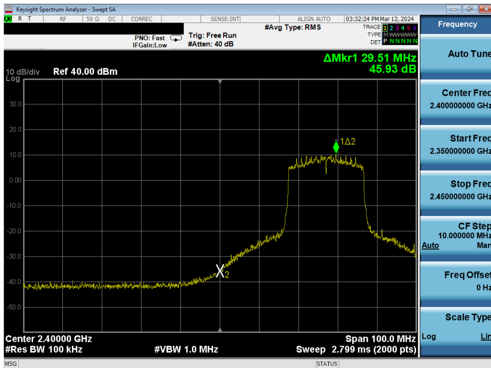
Plot 7-245. Band Edge Plot Antenna 3a (802.11ax (SU - 2.4GHz) – Ch. 4) – MCS4
