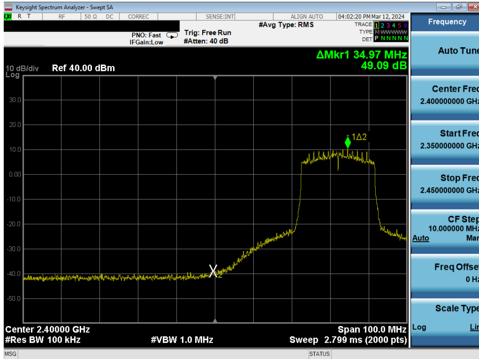
Plot 7-331. Band Edge Plot Antenna 1a (802.11ax (SU - 2.4GHz) – Ch. 5) – MCS2
