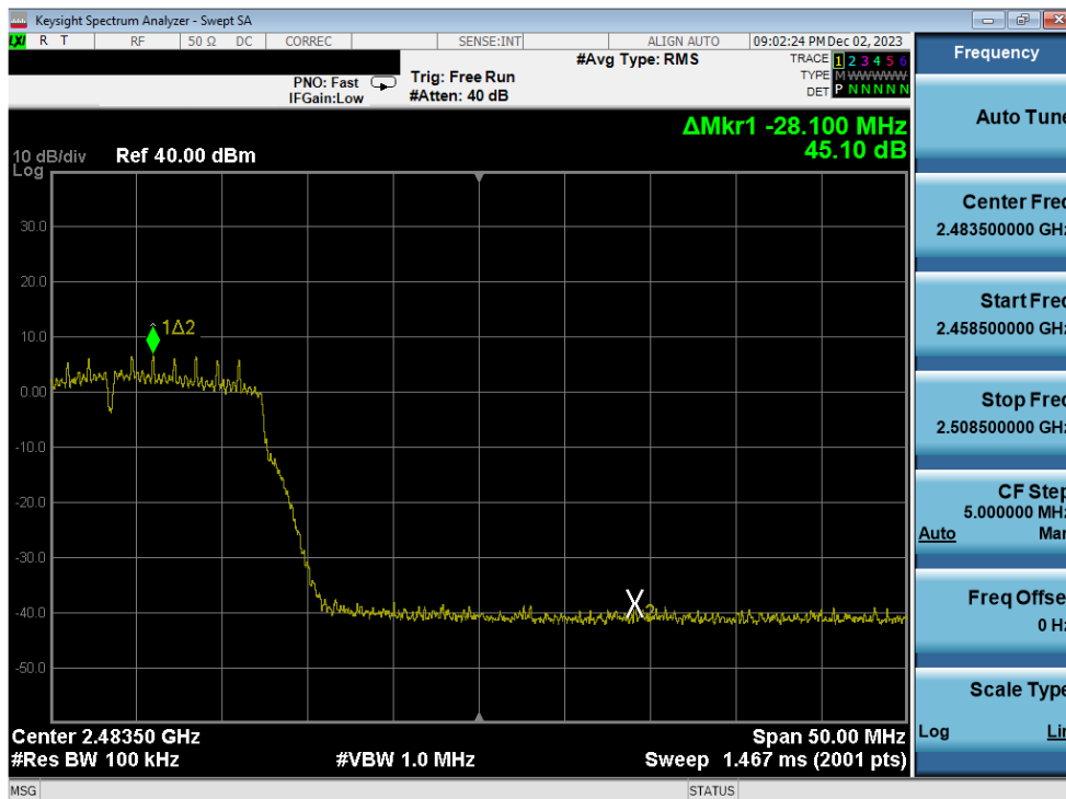
Plot 7-324. Band Edge Plot Antenna 1a (802.11n (2.4GHz) – Ch. 11) – MCS2
