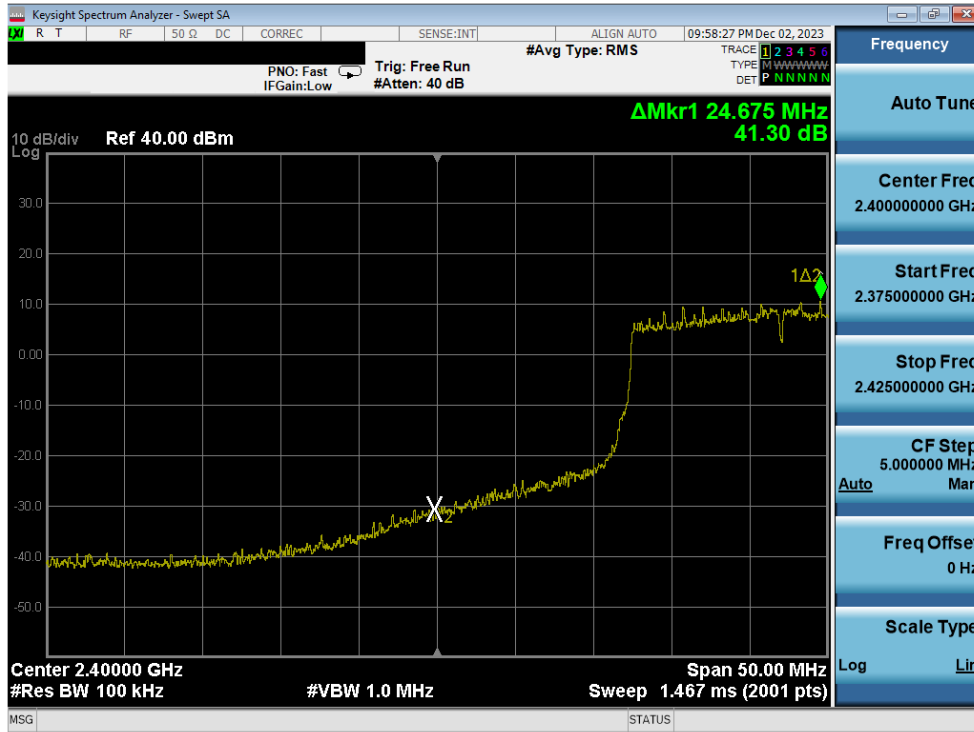
Plot 7-370. Band Edge Plot Antenna 1a (802.11ax (SU - 2.4GHz) – Ch. 3) – MCS4
