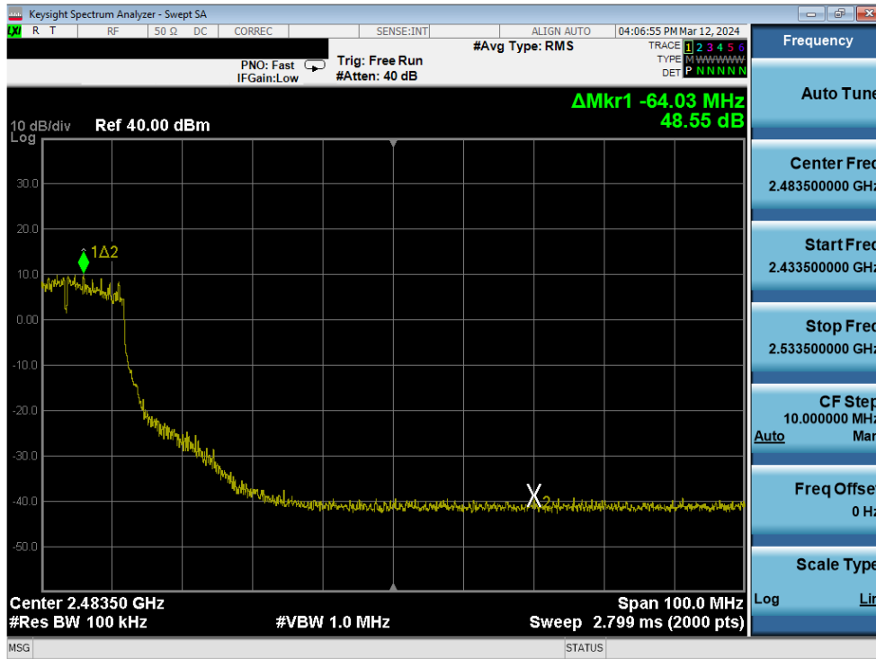
Plot 7-346. Band Edge Plot Antenna 1a (802.11g – Ch. 6 (high)) – 24Mbps
