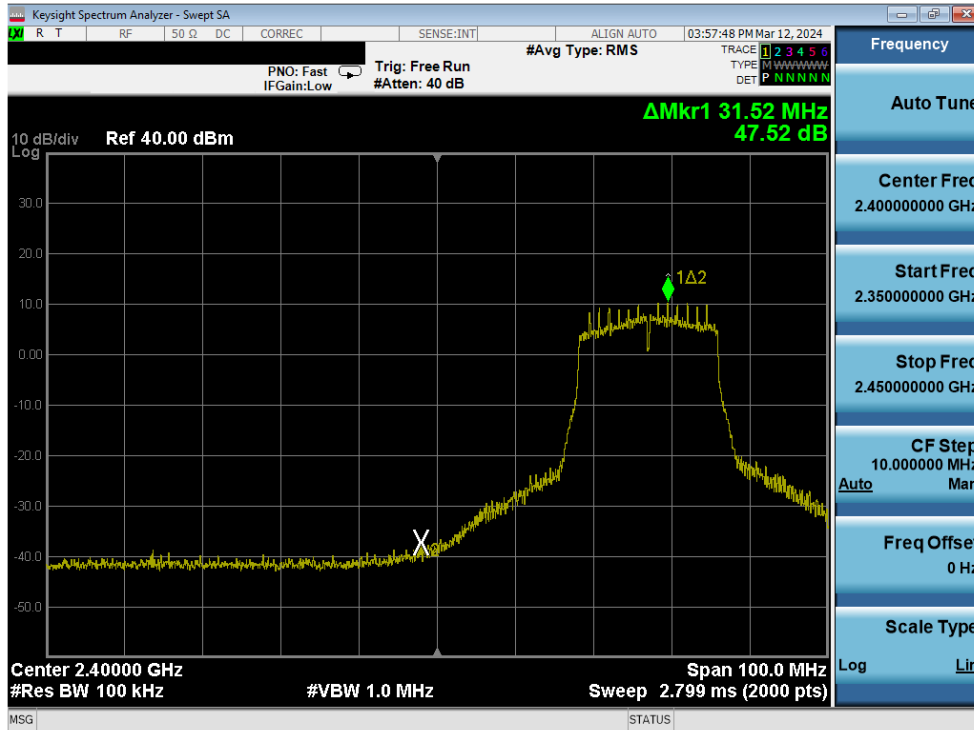
Plot 7-317. Band Edge Plot Antenna 1a (802.11n (2.4GHz) – Ch. 4) – MCS2
