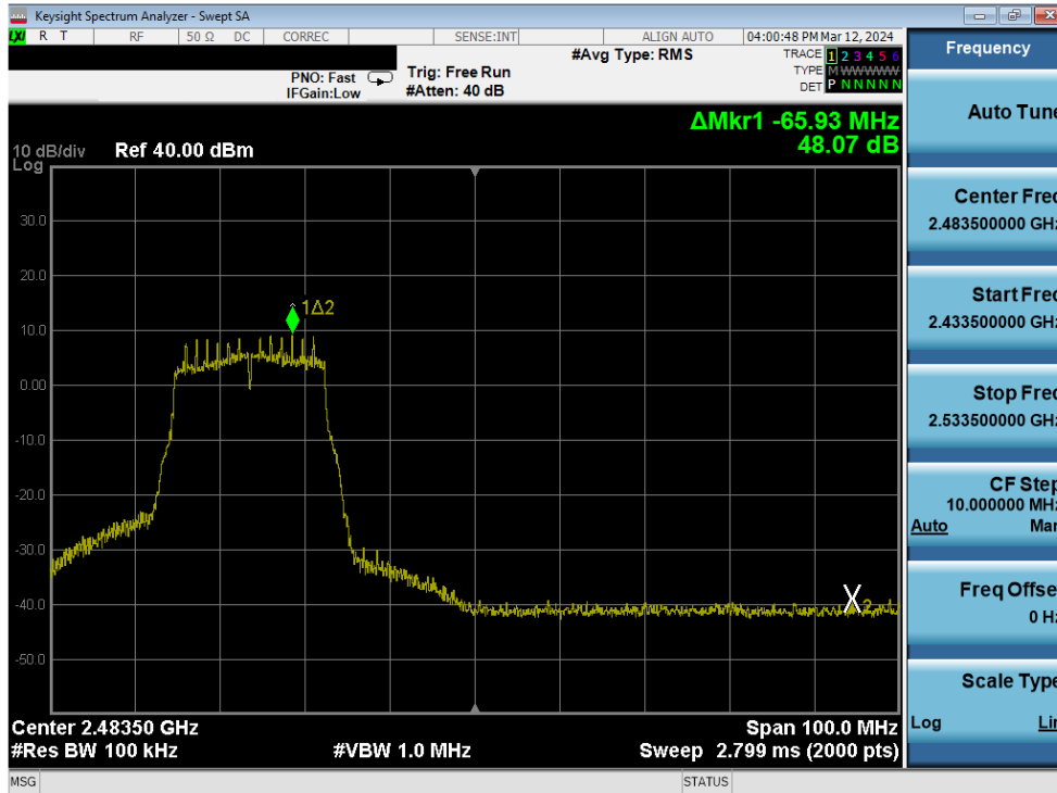
Plot 7-323. Band Edge Plot Antenna 1a (802.11n (2.4GHz) – Ch. 10) – MCS2
