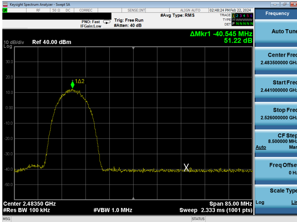
Plot 7-257. Band Edge Plot Antenna 3a (802.11b – Ch. 11) – 11Mbps
