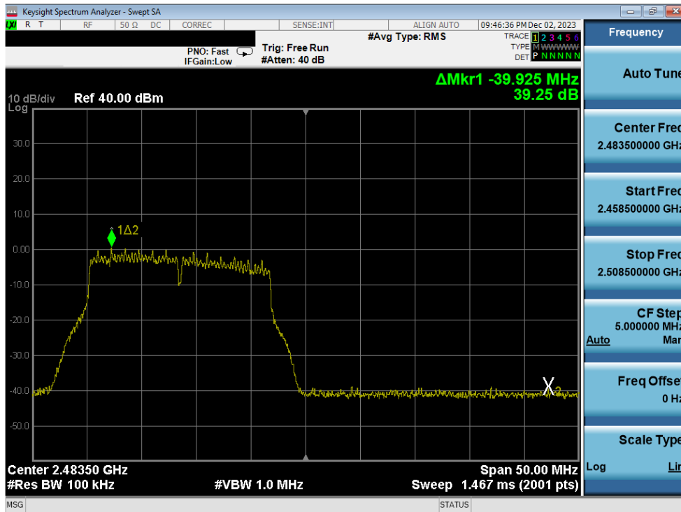
Plot 7-353. Band Edge Plot Antenna 1a (802.11g – Ch. 13) – 24Mbps
