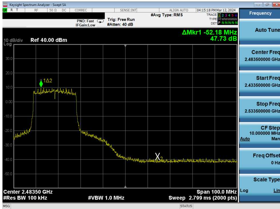
Plot 7-377. Band Edge Plot Antenna 1a (802.11ax (SU - 2.4GHz) – Ch. 9) – MCS4
