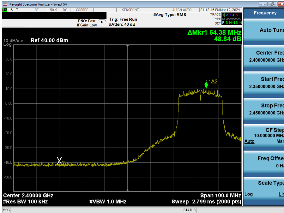
Plot 7-372. Band Edge Plot Antenna 1a (802.11ax (SU - 2.4GHz) – Ch. 5) – MCS4
