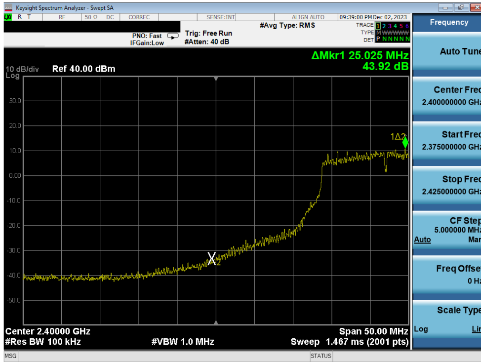
Plot 7-342. Band Edge Plot Antenna 1a (802.11g – Ch. 3) – 24Mbps
