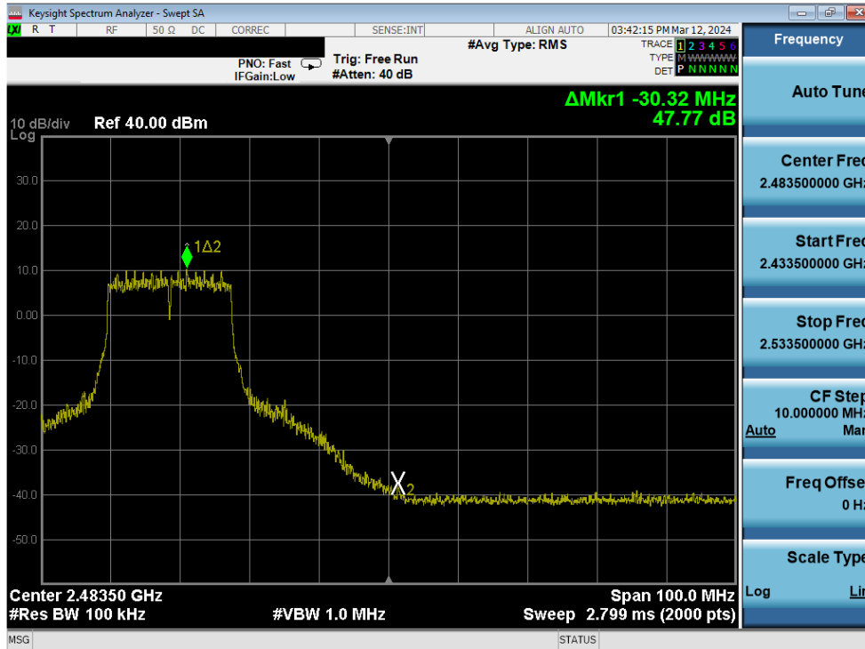
Plot 7-283. Band Edge Plot Antenna 3a (802.11n (2.4GHz) – Ch. 9) – MCS7
