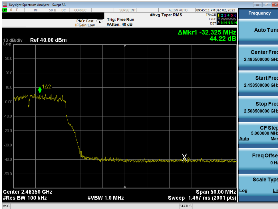
Plot 7-351. Band Edge Plot Antenna 1a (802.11g – Ch. 11) – 24Mbps
