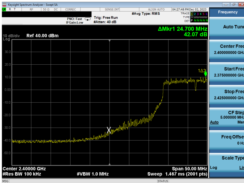
Plot 7-262. Band Edge Plot Antenna 3a (802.11g – Ch. 3) – 54Mbps
