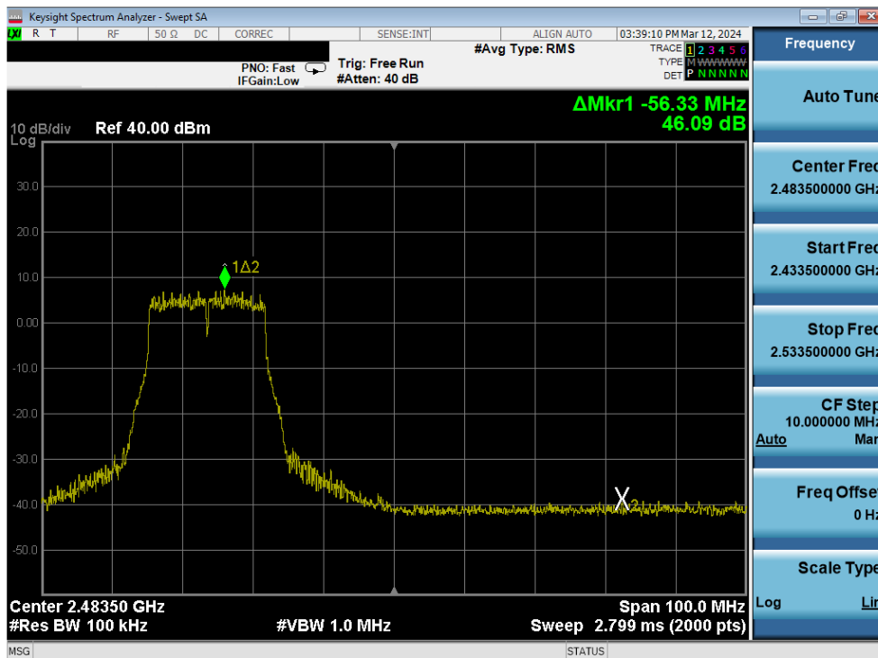
Plot 7-270. Band Edge Plot Antenna 3a (802.11g – Ch. 10) – 54Mbps
