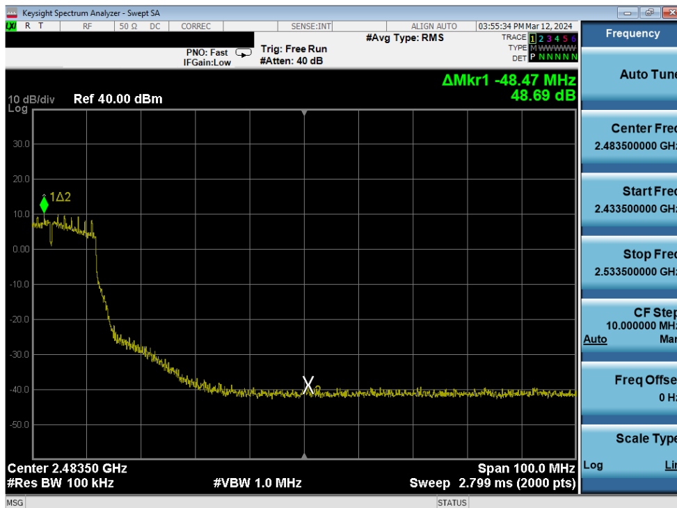
Plot 7-306. Band Edge Plot Antenna 1a (802.11g – Ch. 6 (high)) – 12Mbps
