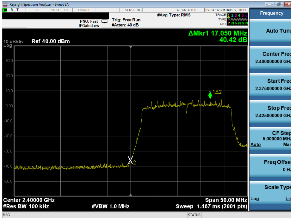
Plot 7-327. Band Edge Plot Antenna 1a (802.11ax (SU - 2.4GHz) – Ch. 1) – MCS2
