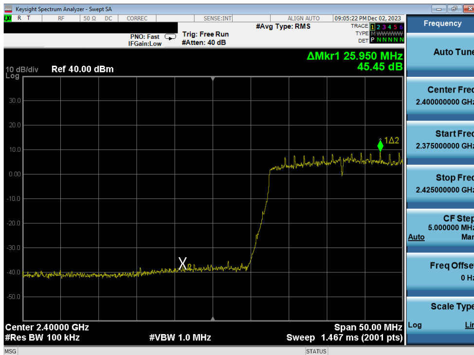
Plot 7-328. Band Edge Plot Antenna 1a (802.11ax (SU - 2.4GHz) – Ch. 2) – MCS2
