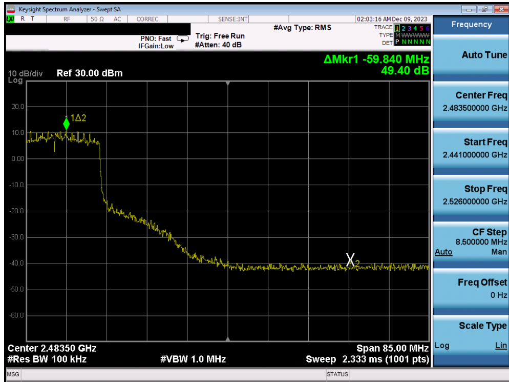
Plot 7-250. Band Edge Plot Antenna 3a (802.11ax (SU - 2.4GHz) – Ch. 8) – MCS4
