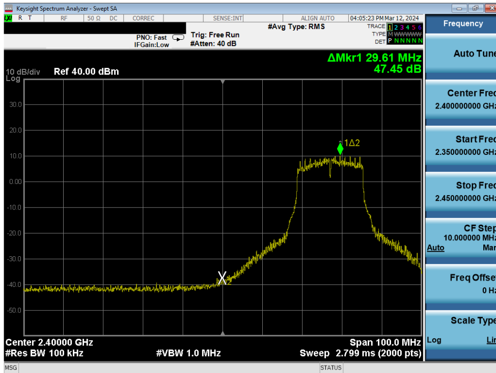
Plot 7-343. Band Edge Plot Antenna 1a (802.11g – Ch. 4) – 24Mbps
