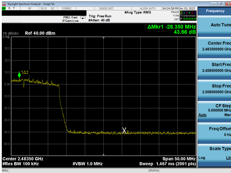
Plot 7-253. Band Edge Plot Antenna 3a (802.11ax (SU - 2.4GHz) – Ch. 11) – MCS4
