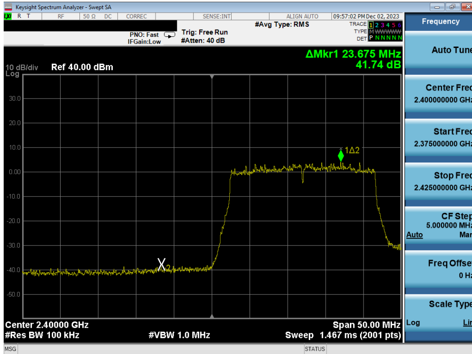
Plot 7-368. Band Edge Plot Antenna 1a (802.11ax (SU - 2.4GHz) – Ch. 1) – MCS4
