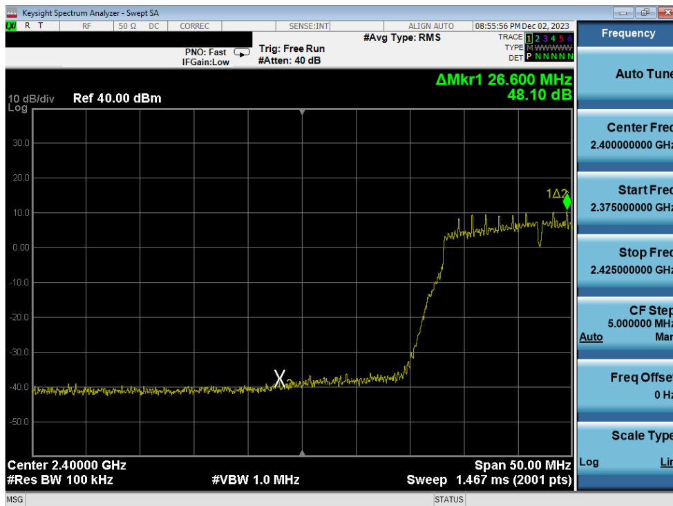
Plot 7-316. Band Edge Plot Antenna 1a (802.11n (2.4GHz) – Ch. 3) – MCS2
