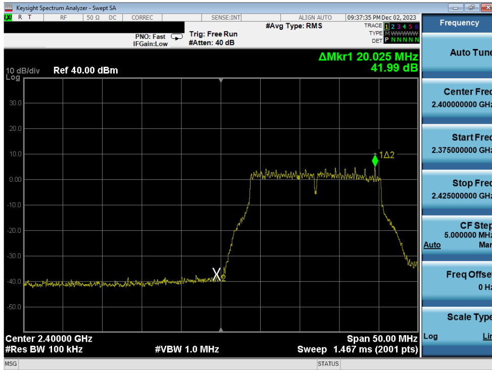
Plot 7-340. Band Edge Plot Antenna 1a (802.11g – Ch. 1) – 24Mbps
