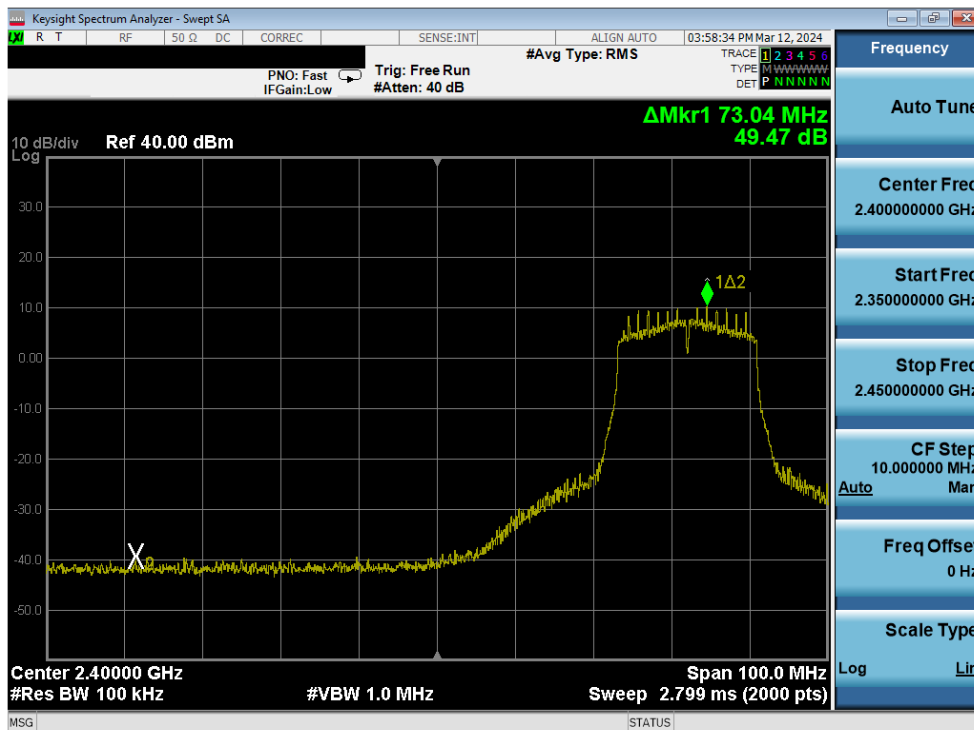
Plot 7-318. Band Edge Plot Antenna 1a (802.11n (2.4GHz) – Ch. 5) – MCS2
