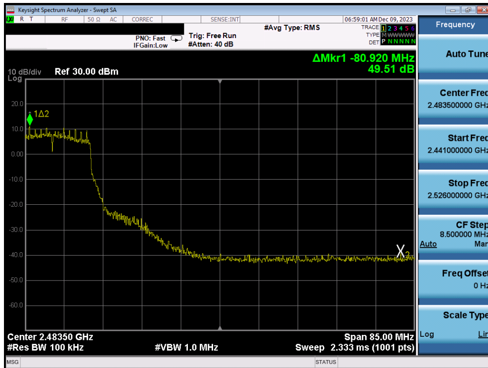
Plot 7-308. Band Edge Plot Antenna 1a (802.11g - Ch. 8) - 12Mbps
