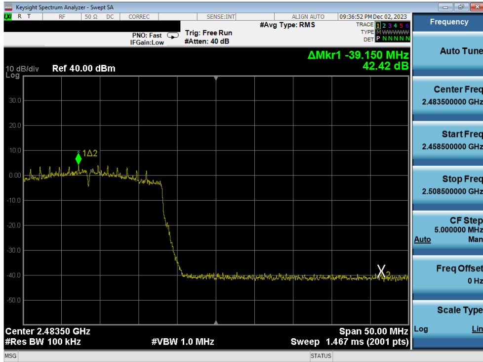
Plot 7-339. Band Edge Plot Antenna 1a (802.11ax (SU - 2.4GHz) – Ch. 12) – MCS2
