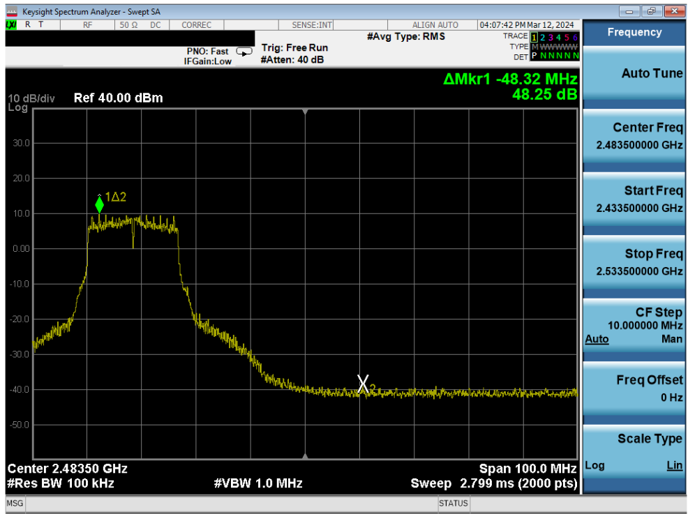
Plot 7-349. Band Edge Plot Antenna 1a (802.11g – Ch. 9) – 24Mbps
