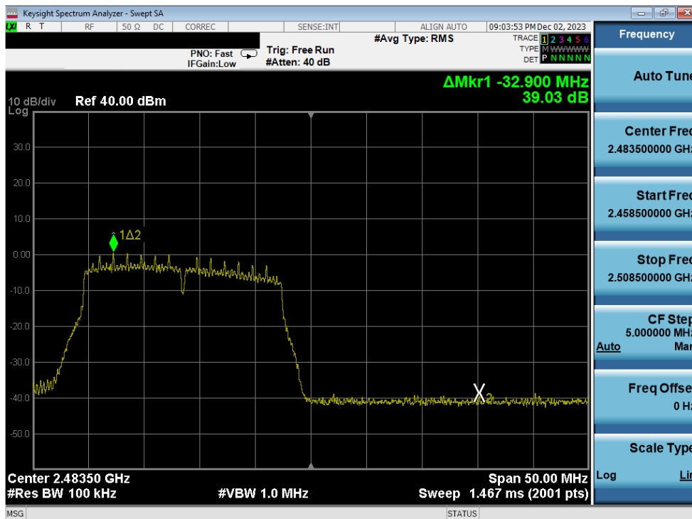
Plot 7-326. Band Edge Plot Antenna 1a (802.11n (2.4GHz) – Ch. 13) – MCS2
