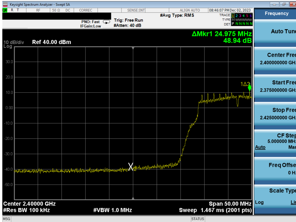
Plot 7-303. Band Edge Plot Antenna 1a (802.11g - Ch. 3) - 12Mbps
