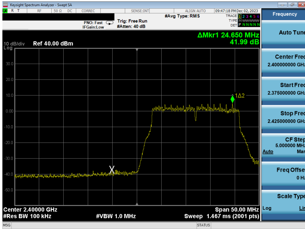
Plot 7-354. Band Edge Plot Antenna 1a (802.11n (2.4GHz) – Ch. 1) – MCS4
