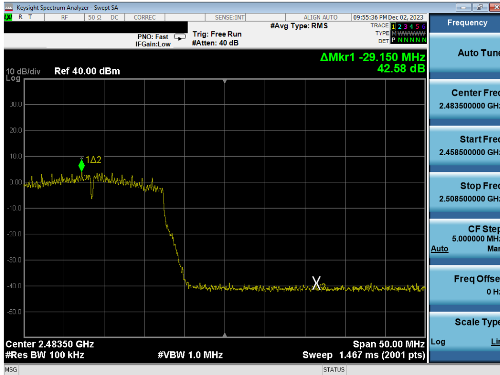
Plot 7-366. Band Edge Plot Antenna 1a (802.11n (2.4GHz) – Ch. 12) – MCS4
