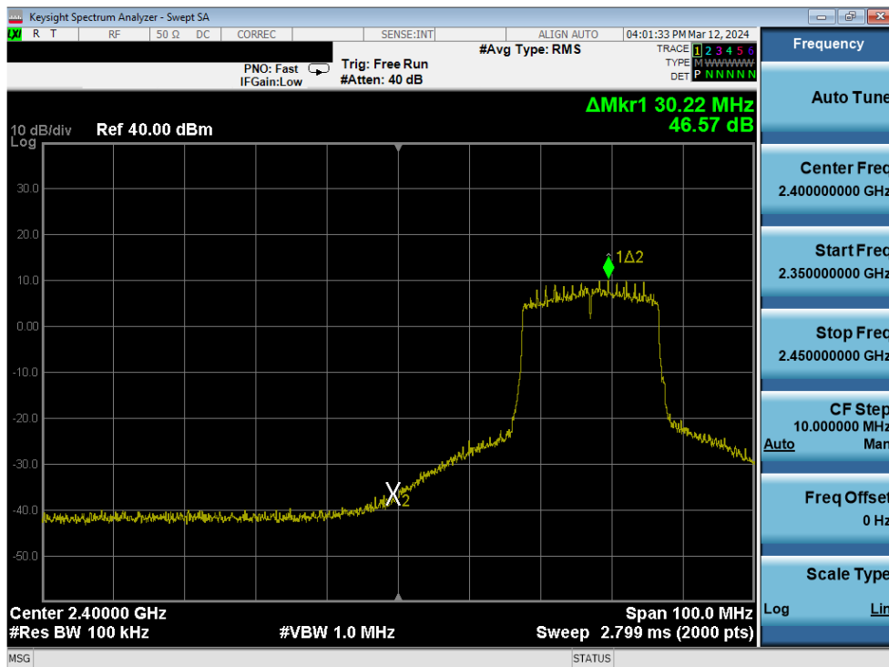
Plot 7-330. Band Edge Plot Antenna 1a (802.11ax (SU - 2.4GHz) – Ch. 4) – MCS2
