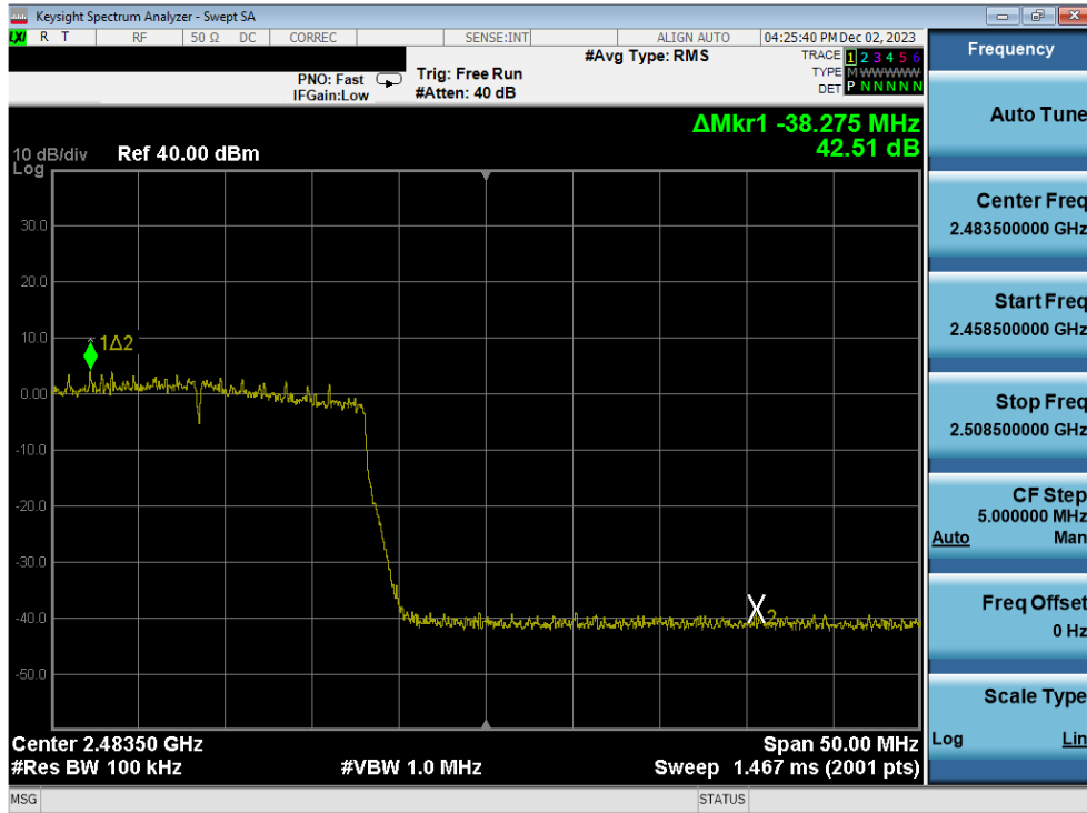
Plot 7-254. Band Edge Plot Antenna 3a (802.11ax (SU - 2.4GHz) – Ch. 12) – MCS4
