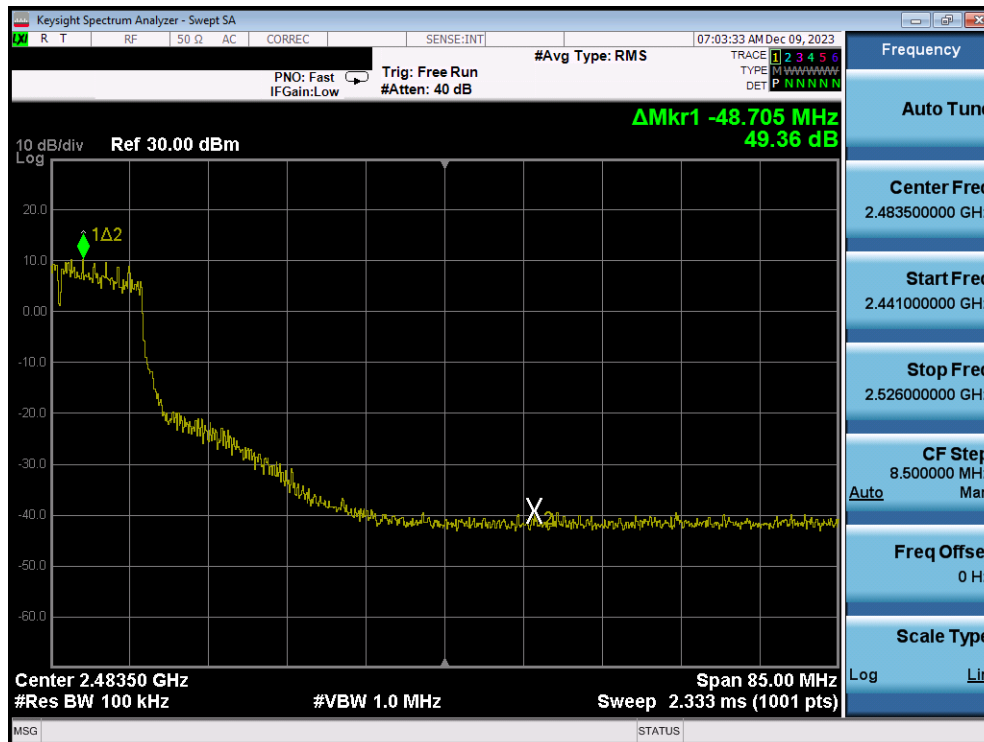
Plot 7-361. Band Edge Plot Antenna 1a (802.11n (2.4GHz) – Ch. 7) – MCS4
