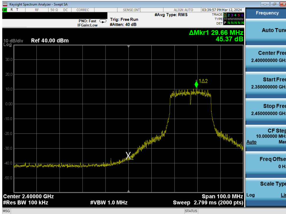
Plot 7-277. Band Edge Plot Antenna 3a (802.11n (2.4GHz) – Ch. 4) – MCS7
