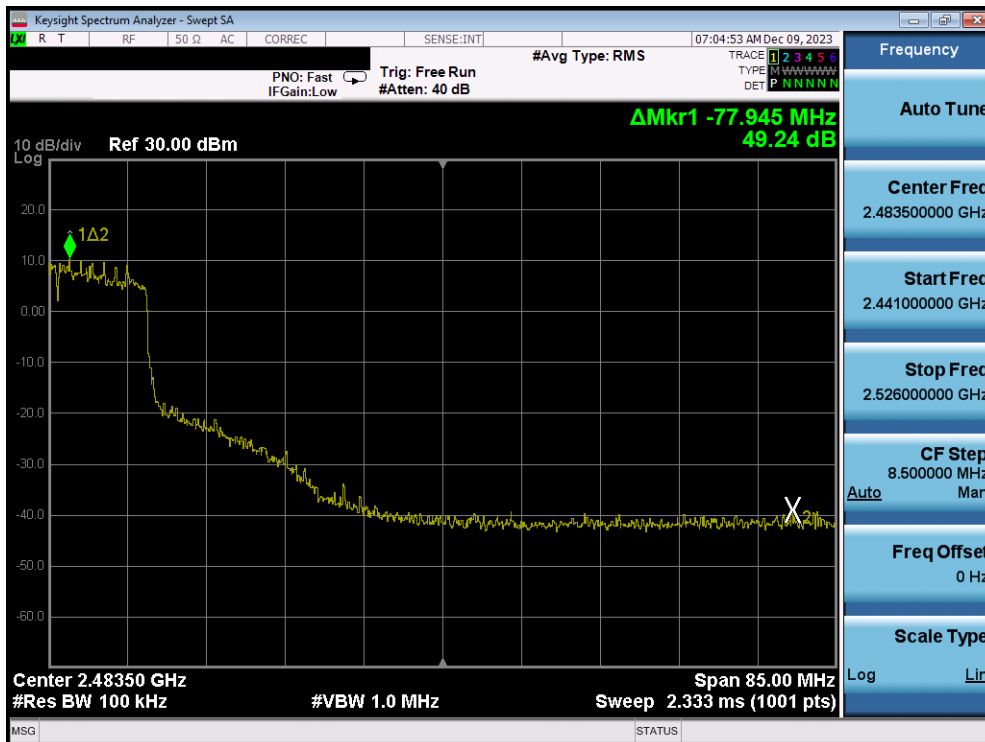
Plot 7-375. Band Edge Plot Antenna 1a (802.11ax (SU - 2.4GHz) – Ch. 7) – MCS4
