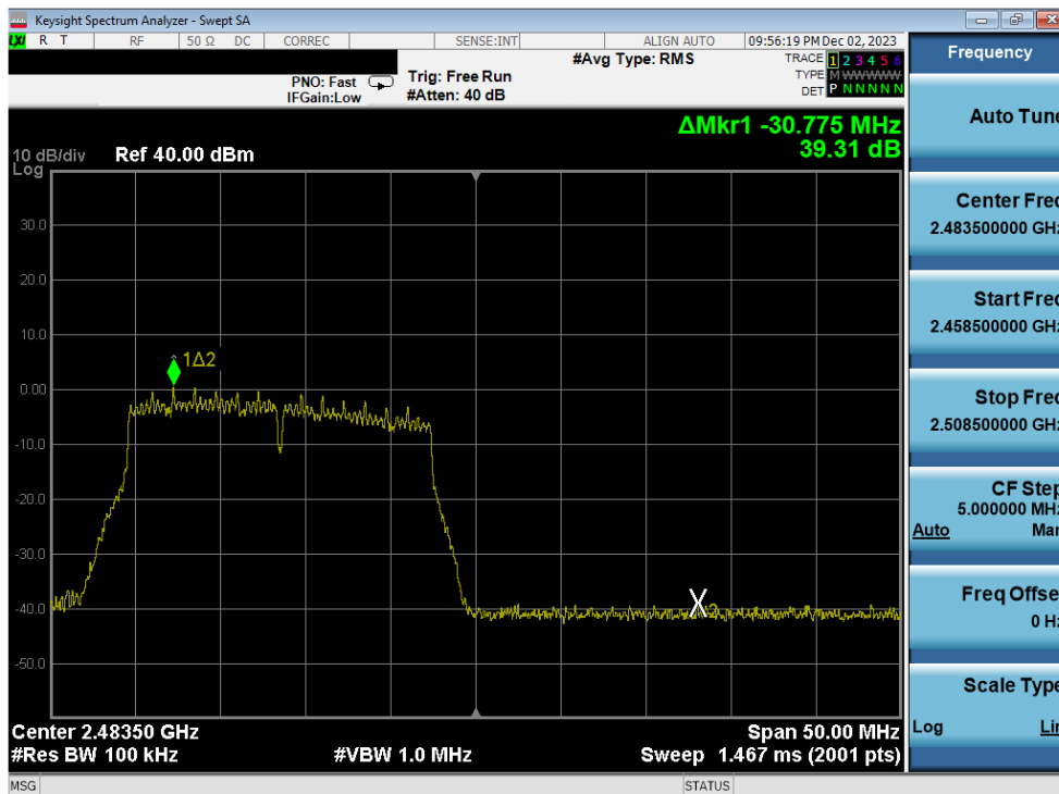
Plot 7-367. Band Edge Plot Antenna 1a (802.11n (2.4GHz) – Ch. 13) – MCS4
