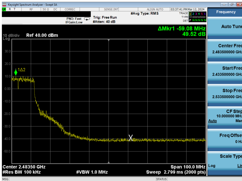
Plot 7-266. Band Edge Plot Antenna 3a (802.11g – Ch. 6 (high)) – 54Mbps
