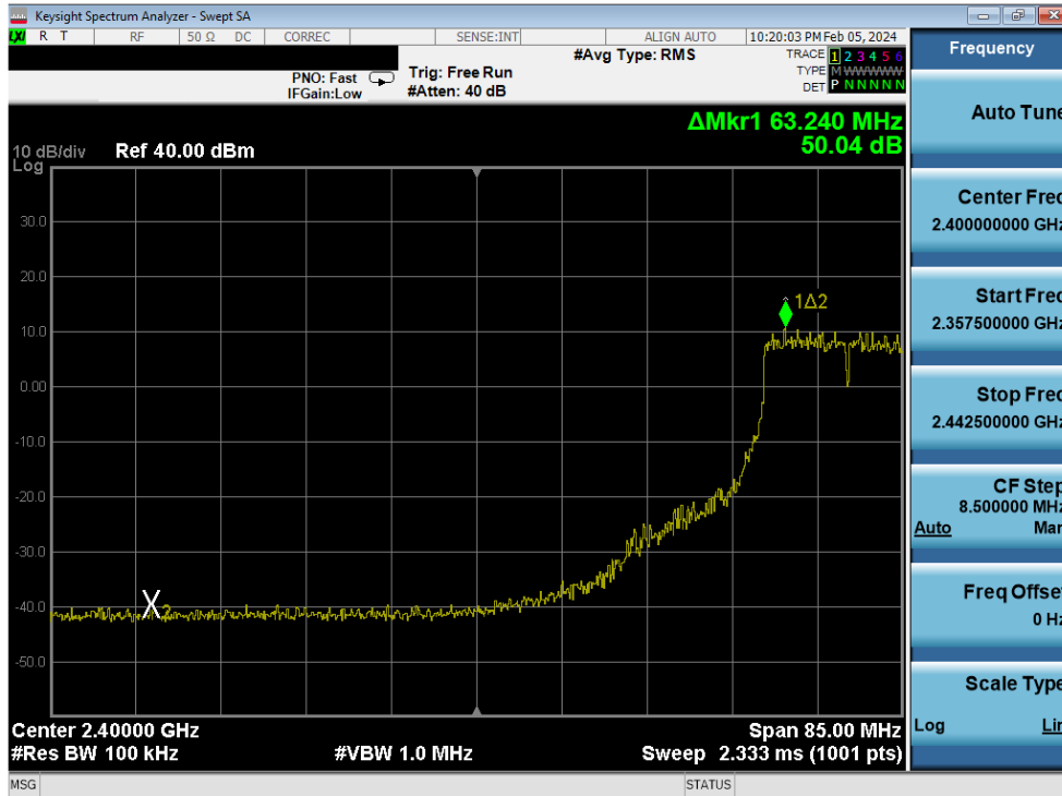
Plot 7-265. Band Edge Plot Antenna 3a (802.11g – Ch. 6 (low)) – 54Mbps
