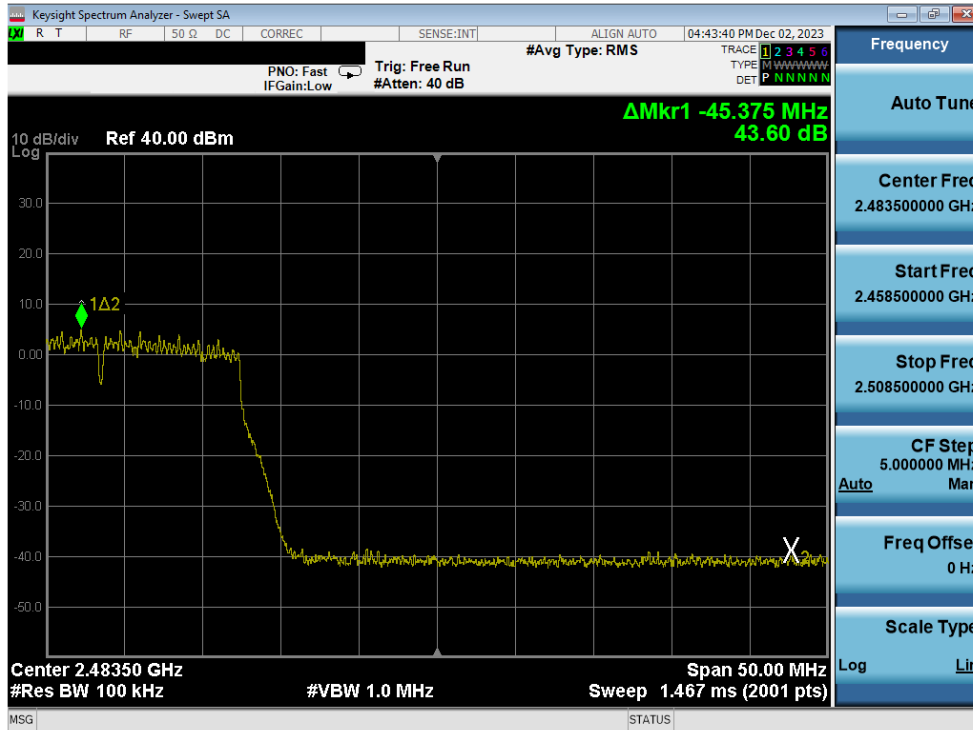
Plot 7-285. Band Edge Plot Antenna 3a (802.11n (2.4GHz) - Ch. 11) - MCS7
