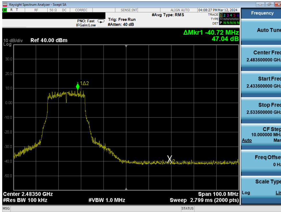
Plot 7-350. Band Edge Plot Antenna 1a (802.11g – Ch. 10) – 24Mbps
