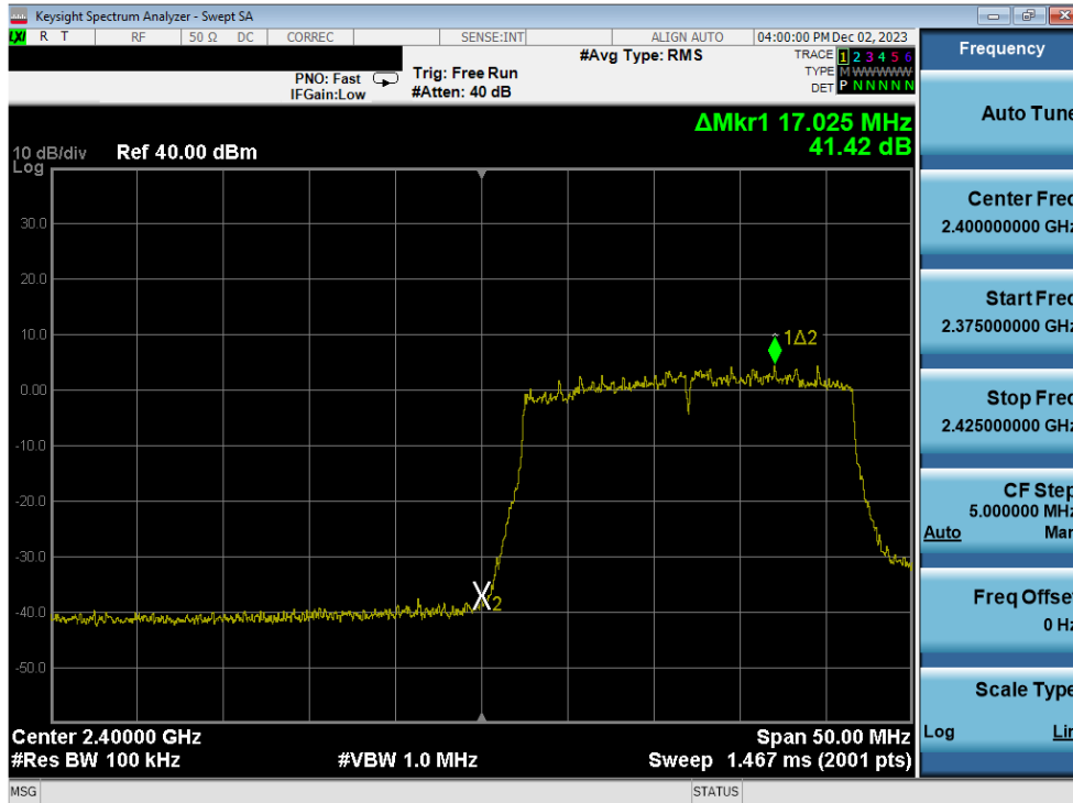
Plot 7-242. Band Edge Plot Antenna 3a (802.11ax (SU - 2.4GHz) – Ch. 1) – MCS4
