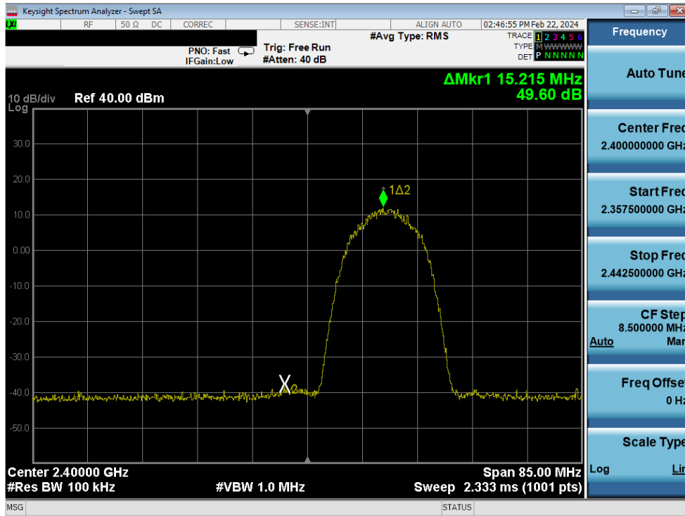
Plot 7-255. Band Edge Plot Antenna 3a (802.11b – Ch. 1) – 11Mbps
