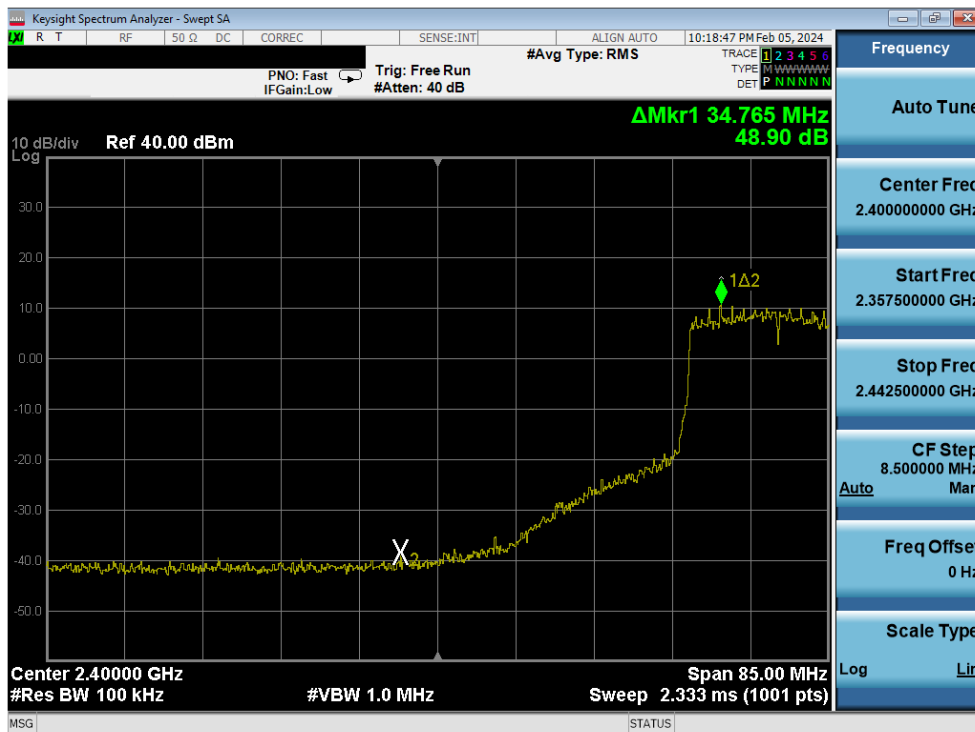
Plot 7-247. Band Edge Plot Antenna 3a (802.11ax (SU - 2.4GHz) – Ch. 6 (low)) – MCS4
