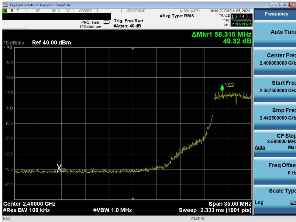
Plot 7-345. Band Edge Plot Antenna 1a (802.11g – Ch. 6 (low)) – 24Mbps
