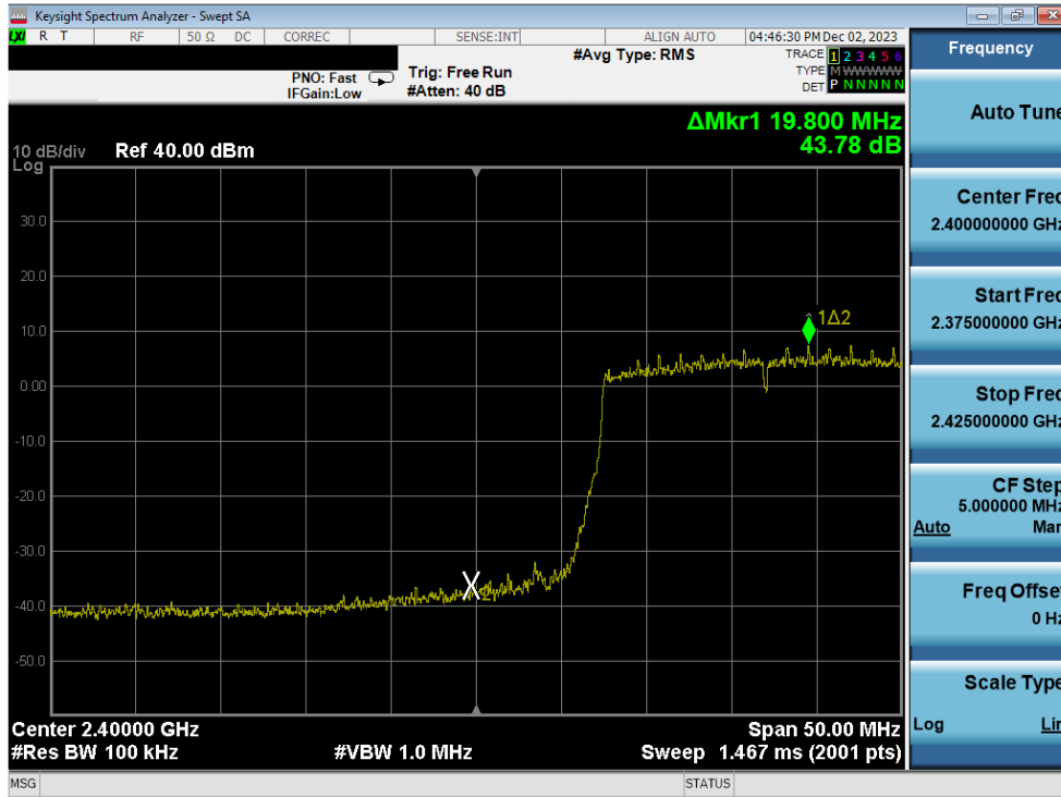
Plot 7-289. Band Edge Plot Antenna 3a (802.11ax (SU - 2.4GHz) – Ch. 2) – MCS9
