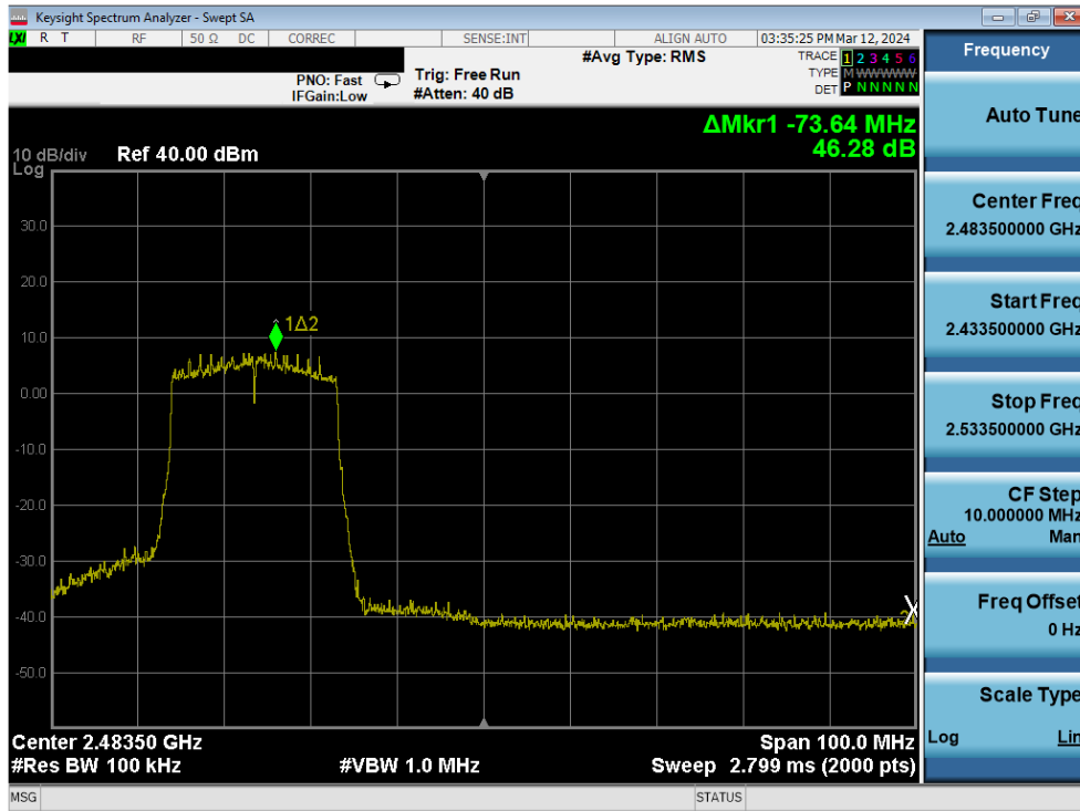
Plot 7-252. Band Edge Plot Antenna 3a (802.11ax (SU - 2.4GHz) – Ch. 10) – MCS4
