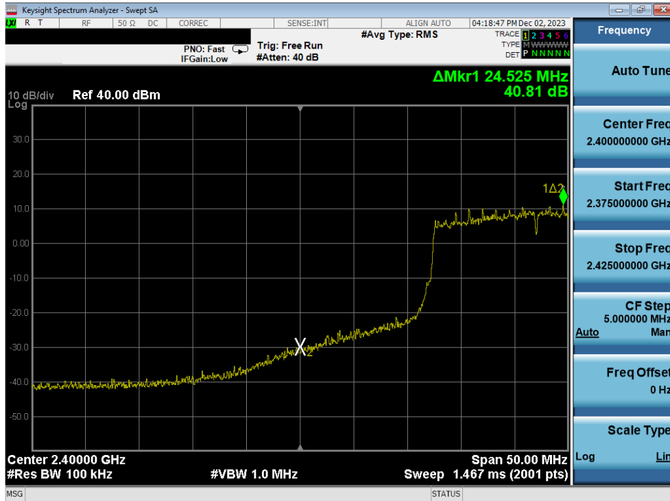
Plot 7-244. Band Edge Plot Antenna 3a (802.11ax (SU - 2.4GHz) – Ch. 3) – MCS4
