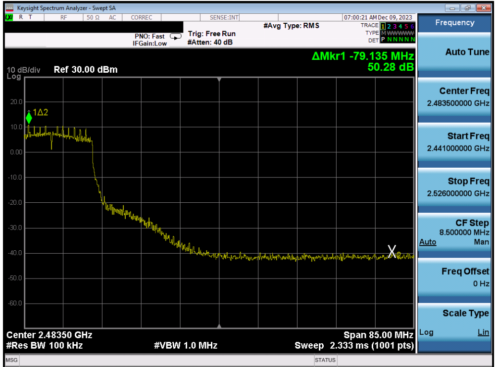
Plot 7-321. Band Edge Plot Antenna 1a (802.11n (2.4GHz) – Ch. 8) – MCS2
