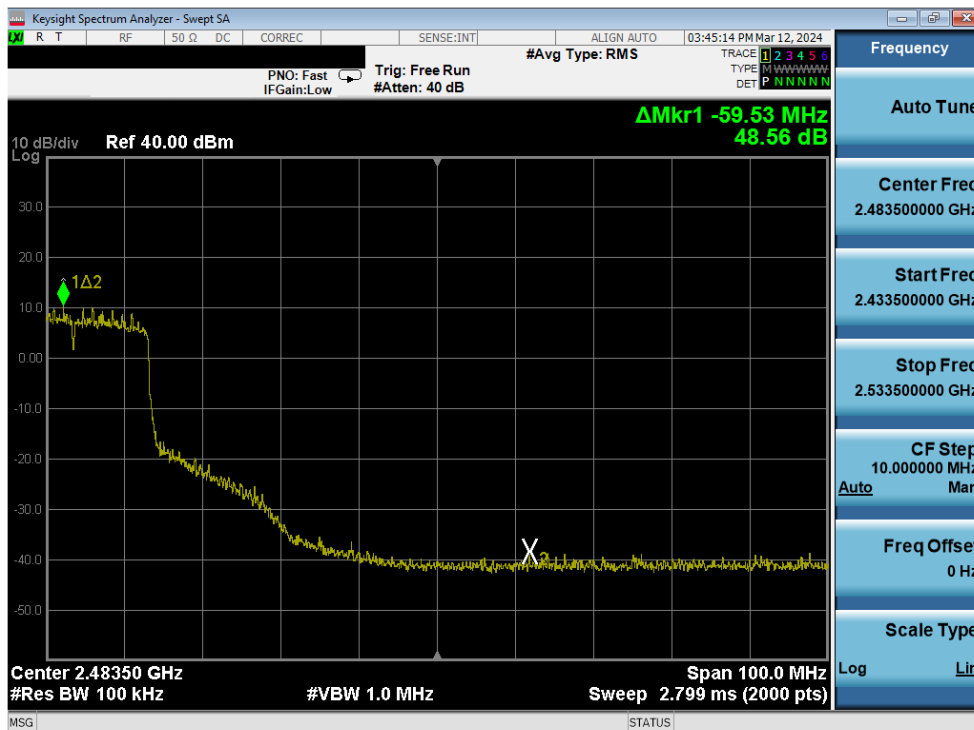
Plot 7-294. Band Edge Plot Antenna 3a (802.11ax (SU - 2.4GHz) – Ch. 6 (high)) – MCS9
