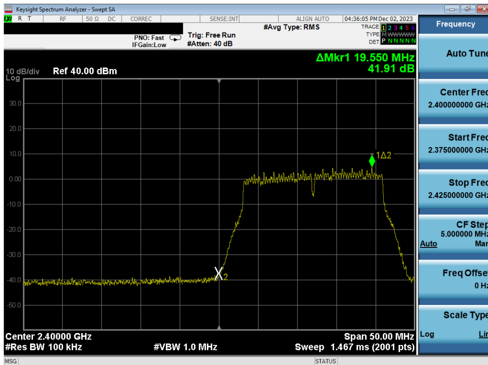
Plot 7-274. Band Edge Plot Antenna 3a (802.11n (2.4GHz) – Ch. 1) – MCS7
