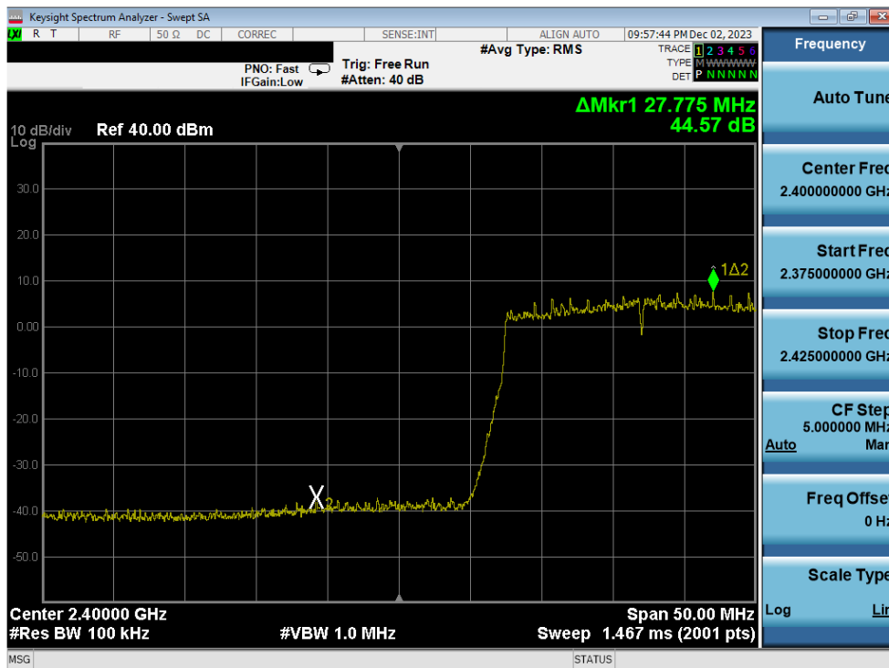
Plot 7-369. Band Edge Plot Antenna 1a (802.11ax (SU - 2.4GHz) – Ch. 2) – MCS4
