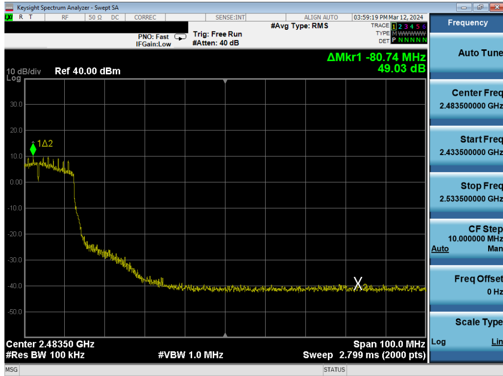
Plot 7-319. Band Edge Plot Antenna 1a (802.11n (2.4GHz) – Ch. 6 (high)) – MCS2
