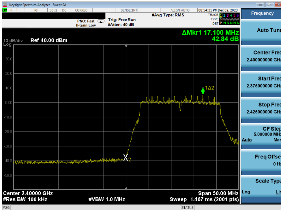
Plot 7-314. Band Edge Plot Antenna 1a (802.11n (2.4GHz) – Ch. 1) – MCS2
