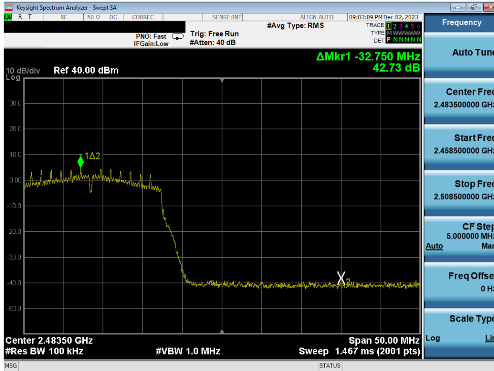
Plot 7-325. Band Edge Plot Antenna 1a (802.11n (2.4GHz) – Ch. 12) – MCS2
