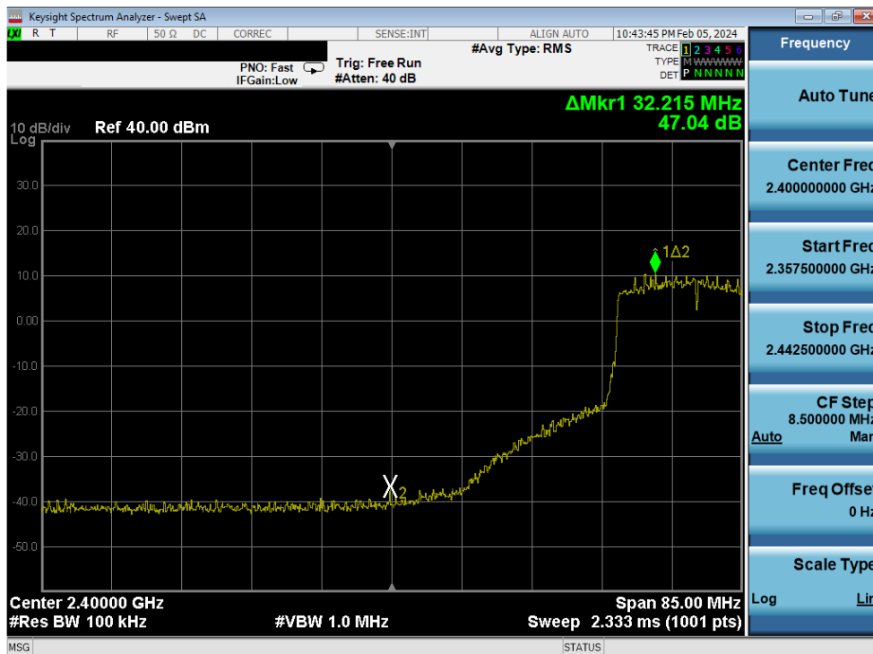
Plot 7-373. Band Edge Plot Antenna 1a (802.11ax (SU - 2.4GHz) – Ch. 6 (low)) – MCS4
