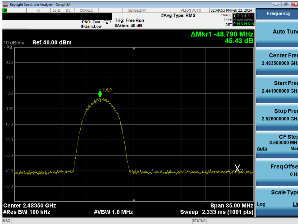
Plot 7-259. Band Edge Plot Antenna 3a (802.11b – Ch. 13) – 11Mbps
