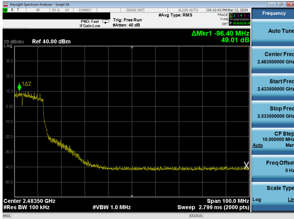
Plot 7-360. Band Edge Plot Antenna 1a (802.11n (2.4GHz) – Ch. 6 (high)) – MCS4
