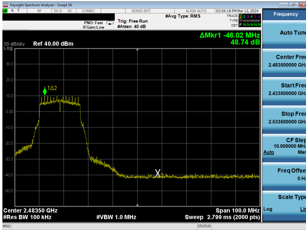
Plot 7-309. Band Edge Plot Antenna 1a (802.11g – Ch. 9) – 12Mbps
