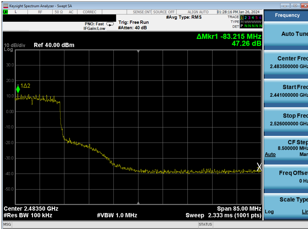
Plot 7-335. Band Edge Plot Antenna 1a (802.11ax (SU - 2.4GHz) – Ch. 8) – MCS2
