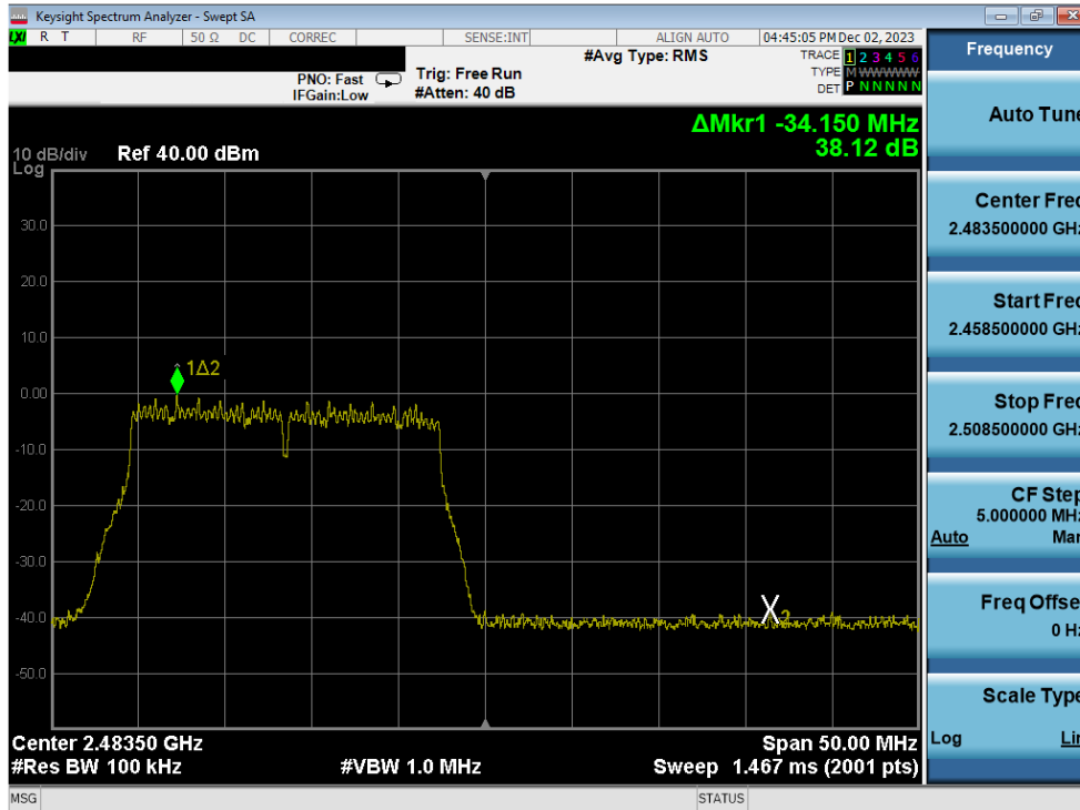
Plot 7-287. Band Edge Plot Antenna 3a (802.11n (2.4GHz) – Ch. 13) – MCS7
