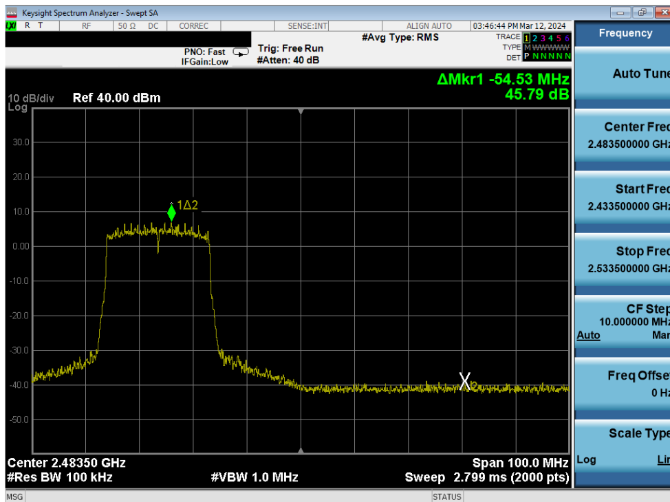
Plot 7-298. Band Edge Plot Antenna 3a (802.11ax (SU - 2.4GHz) – Ch. 10) – MCS9
