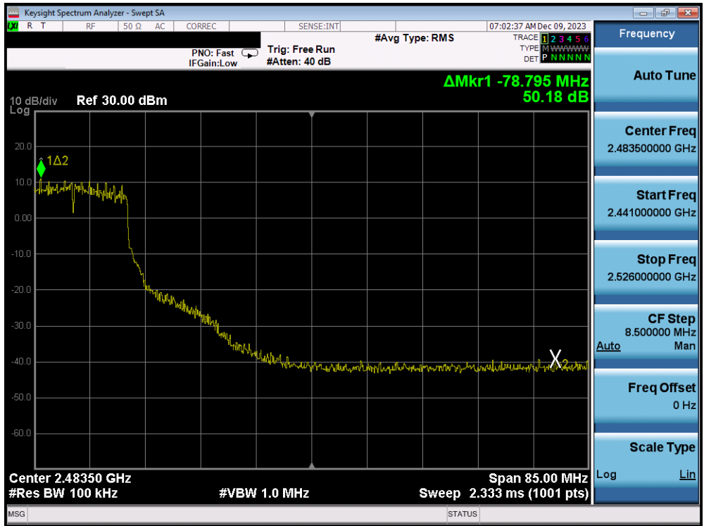
Plot 7-348. Band Edge Plot Antenna 1a (802.11g – Ch. 8) – 24Mbps
