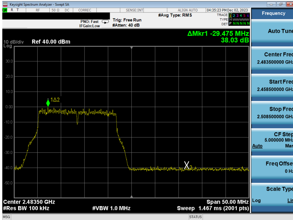
Plot 7-273. Band Edge Plot Antenna 3a (802.11g – Ch. 13) – 54Mbps
