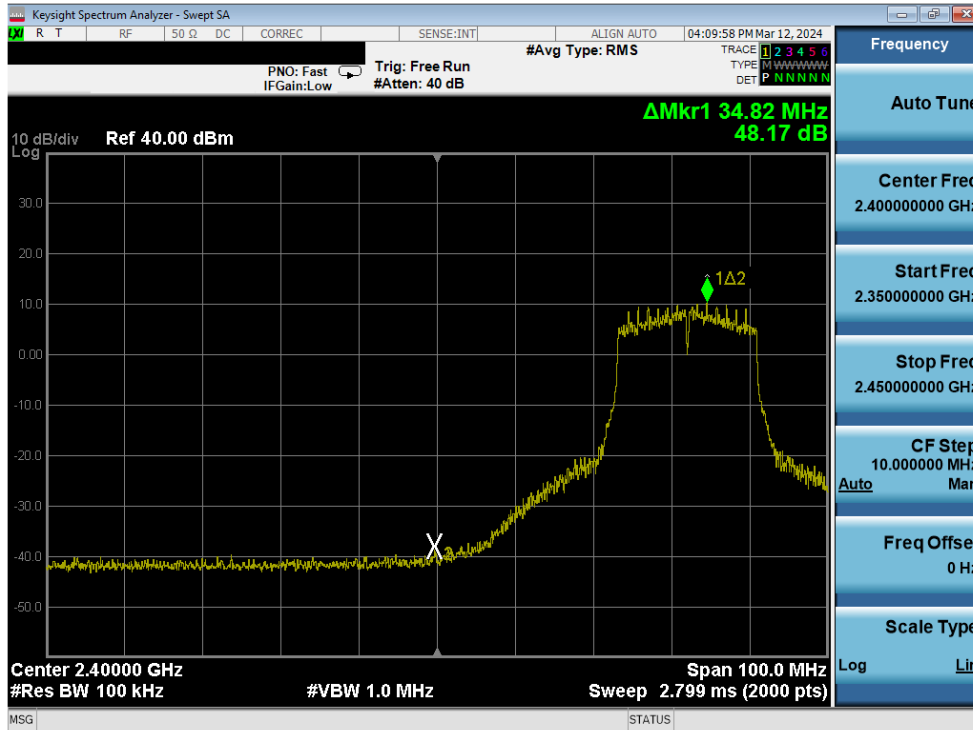
Plot 7-358. Band Edge Plot Antenna 1a (802.11n (2.4GHz) – Ch. 5) – MCS4
