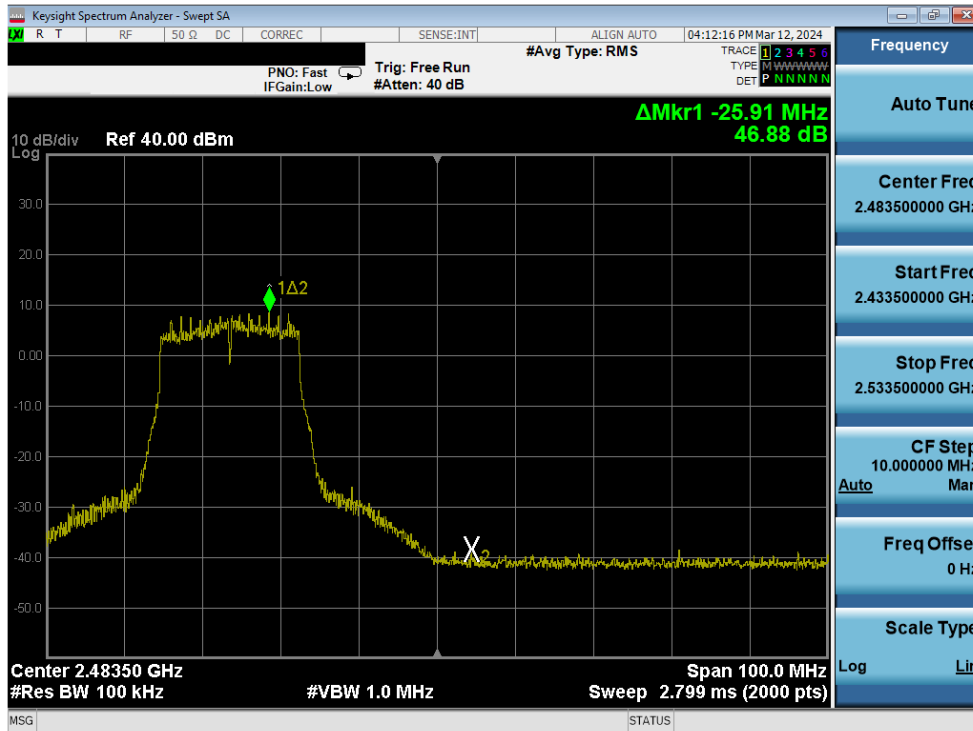
Plot 7-364. Band Edge Plot Antenna 1a (802.11n (2.4GHz) – Ch. 10) – MCS4
