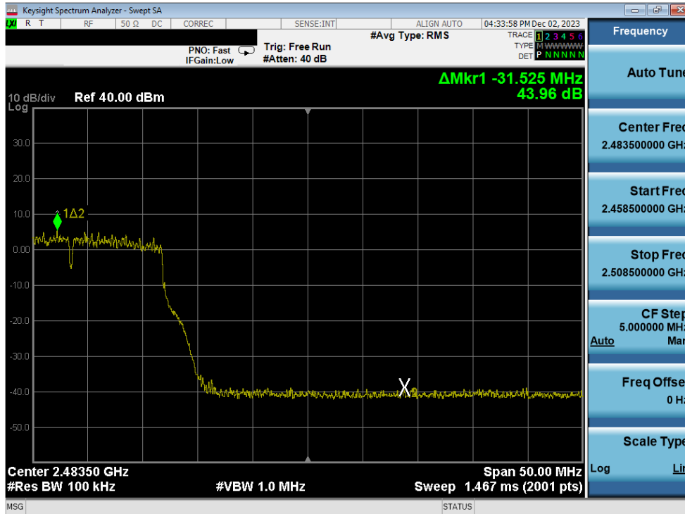
Plot 7-271. Band Edge Plot Antenna 3a (802.11g – Ch. 11) – 54Mbps
