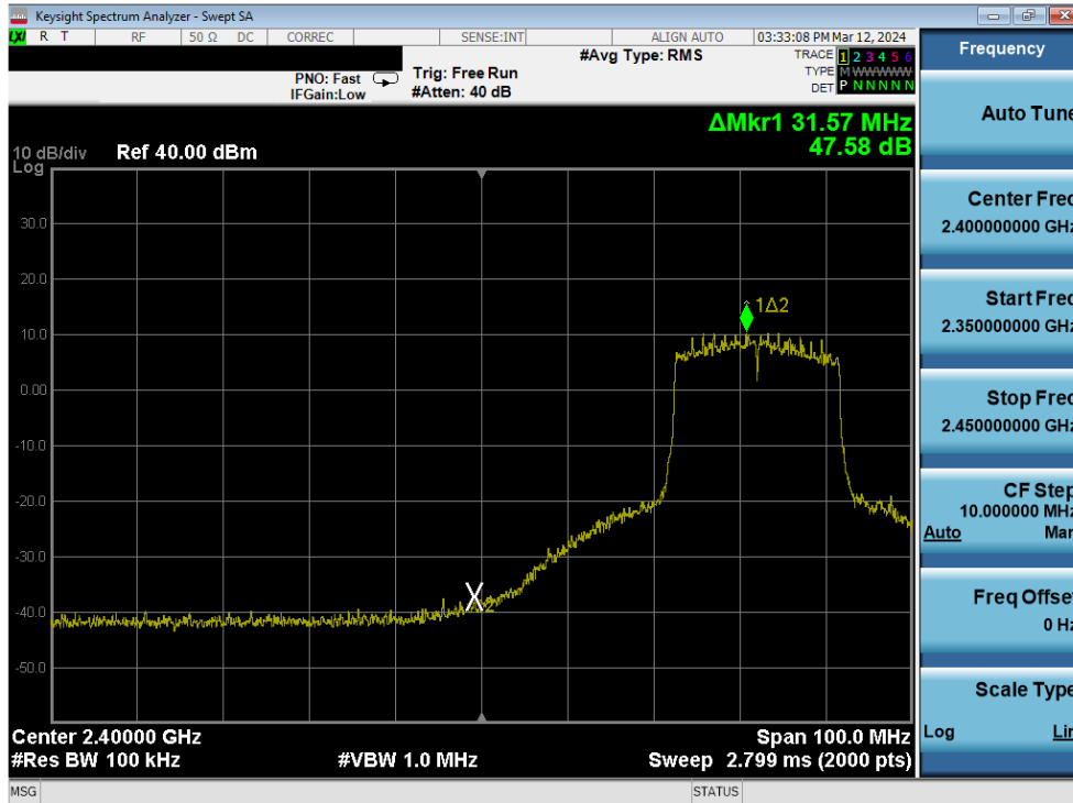
Plot 7-246. Band Edge Plot Antenna 3a (802.11ax (SU - 2.4GHz) – Ch. 5) – MCS4
