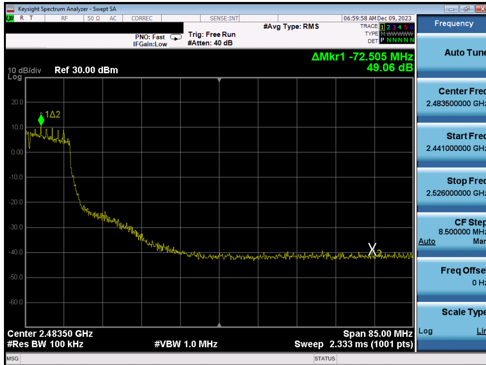
Plot 7-320. Band Edge Plot Antenna 1a (802.11n (2.4GHz) – Ch. 7) – MCS2
