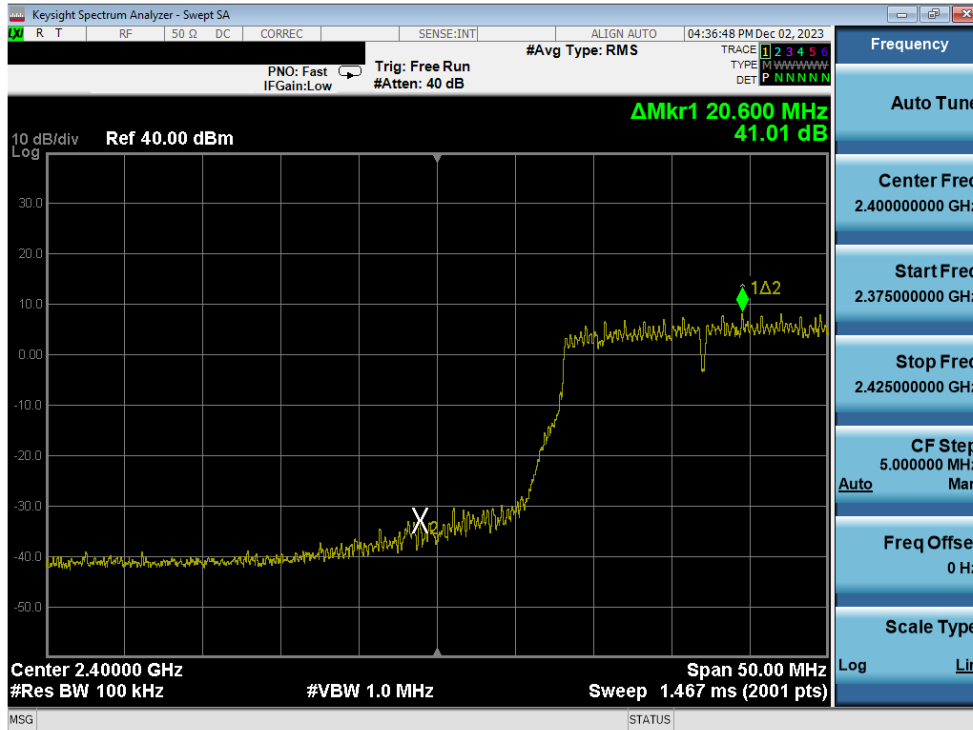
Plot 7-275. Band Edge Plot Antenna 3a (802.11n (2.4GHz) – Ch. 2) – MCS7
