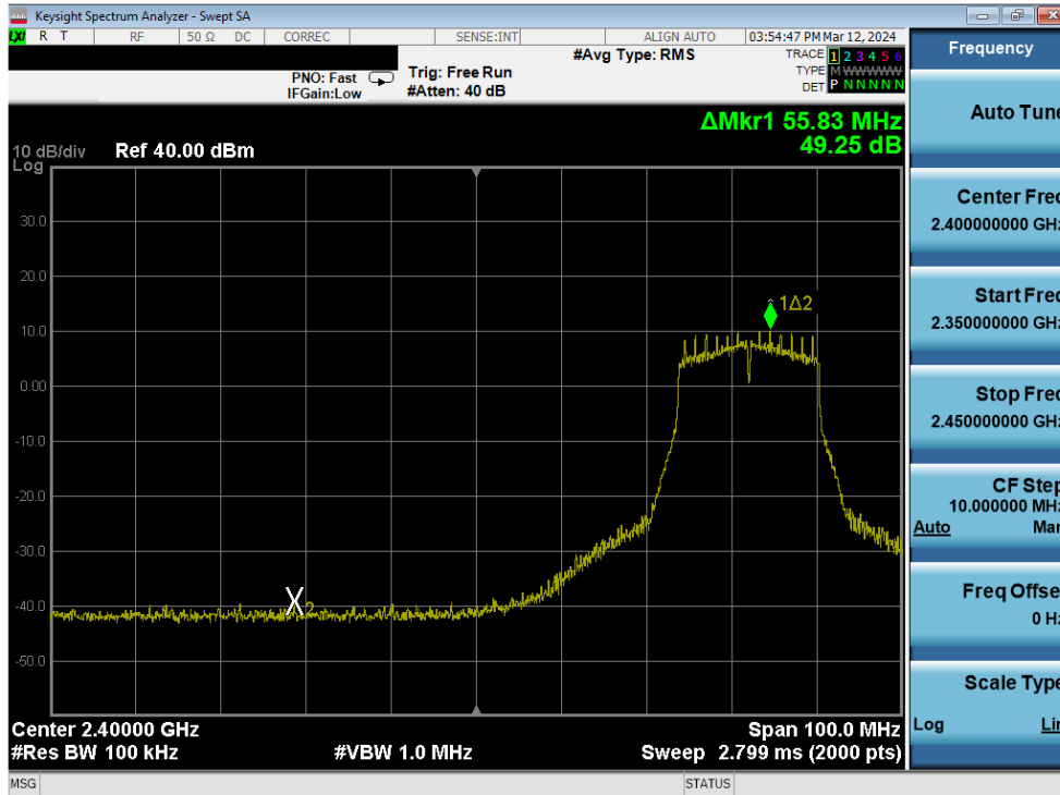
Plot 7-305. Band Edge Plot Antenna 1a (802.11g – Ch. 5) – 12Mbps
