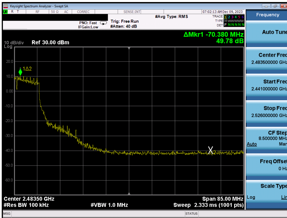
Plot 7-347. Band Edge Plot Antenna 1a (802.11g – Ch. 7) – 24Mbps
