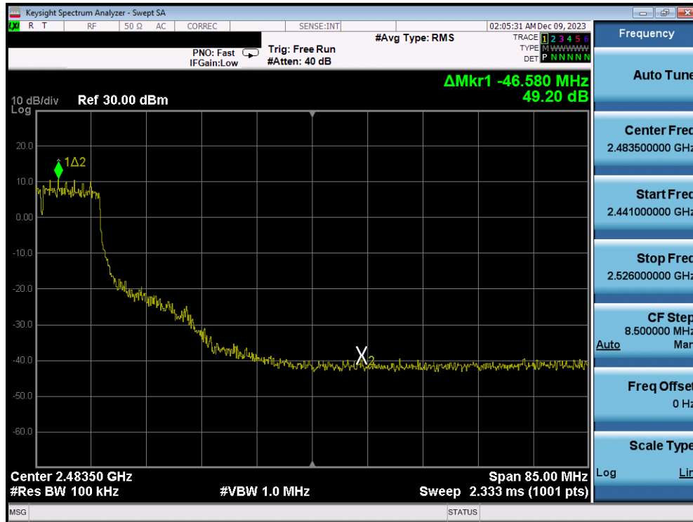
Plot 7-281. Band Edge Plot Antenna 3a (802.11n (2.4GHz) – Ch. 7) – MCS7
