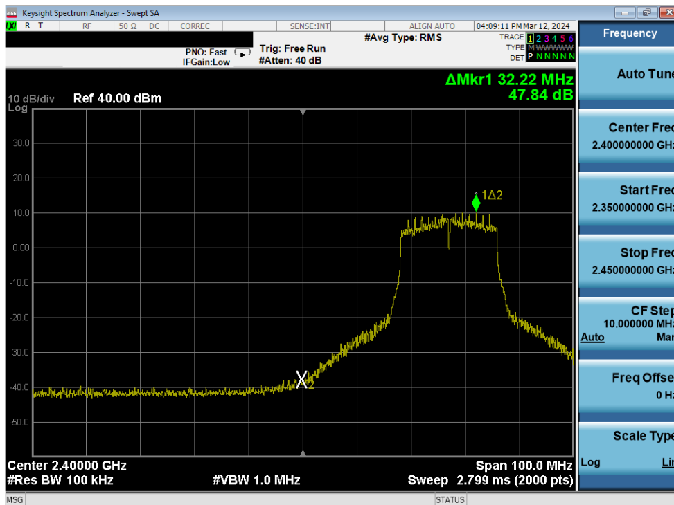
Plot 7-357. Band Edge Plot Antenna 1a (802.11n (2.4GHz) – Ch. 4) – MCS4
