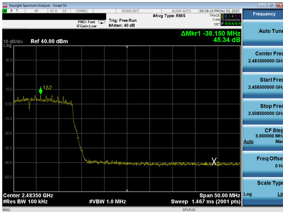
Plot 7-338. Band Edge Plot Antenna 1a (802.11ax (SU - 2.4GHz) – Ch. 11) – MCS2
