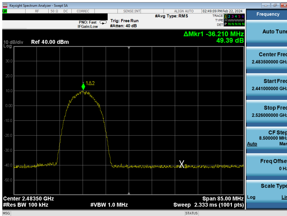
Plot 7-258. Band Edge Plot Antenna 3a (802.11b – Ch. 12) – 11Mbps
