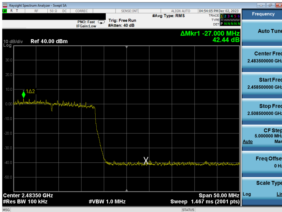
Plot 7-300. Band Edge Plot Antenna 3a (802.11ax (SU - 2.4GHz) – Ch. 12) – MCS9
