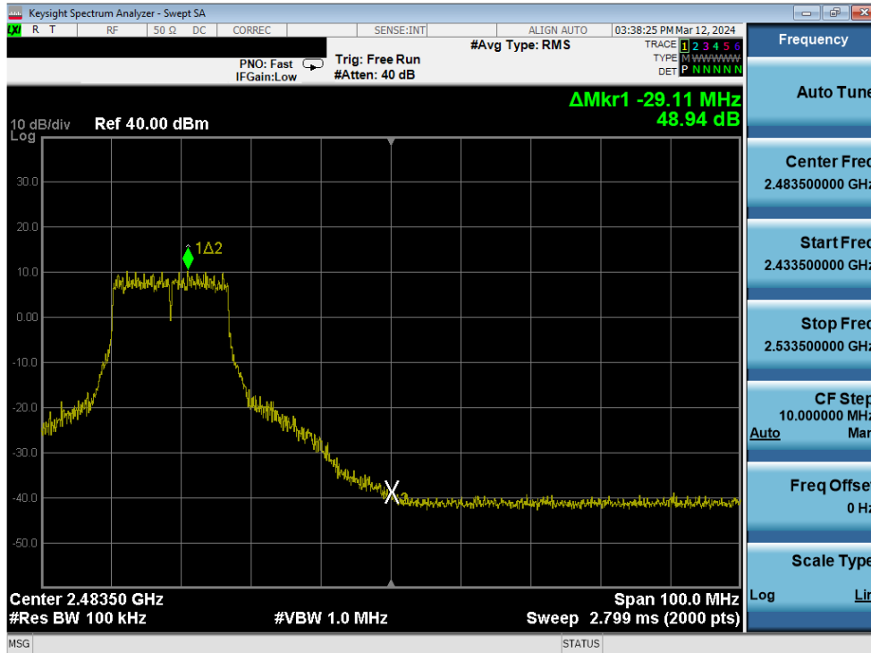
Plot 7-269. Band Edge Plot Antenna 3a (802.11g – Ch. 9) – 54Mbps
