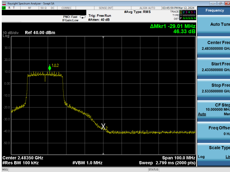
Plot 7-297. Band Edge Plot Antenna 3a (802.11ax (SU - 2.4GHz) – Ch. 9) – MCS9
