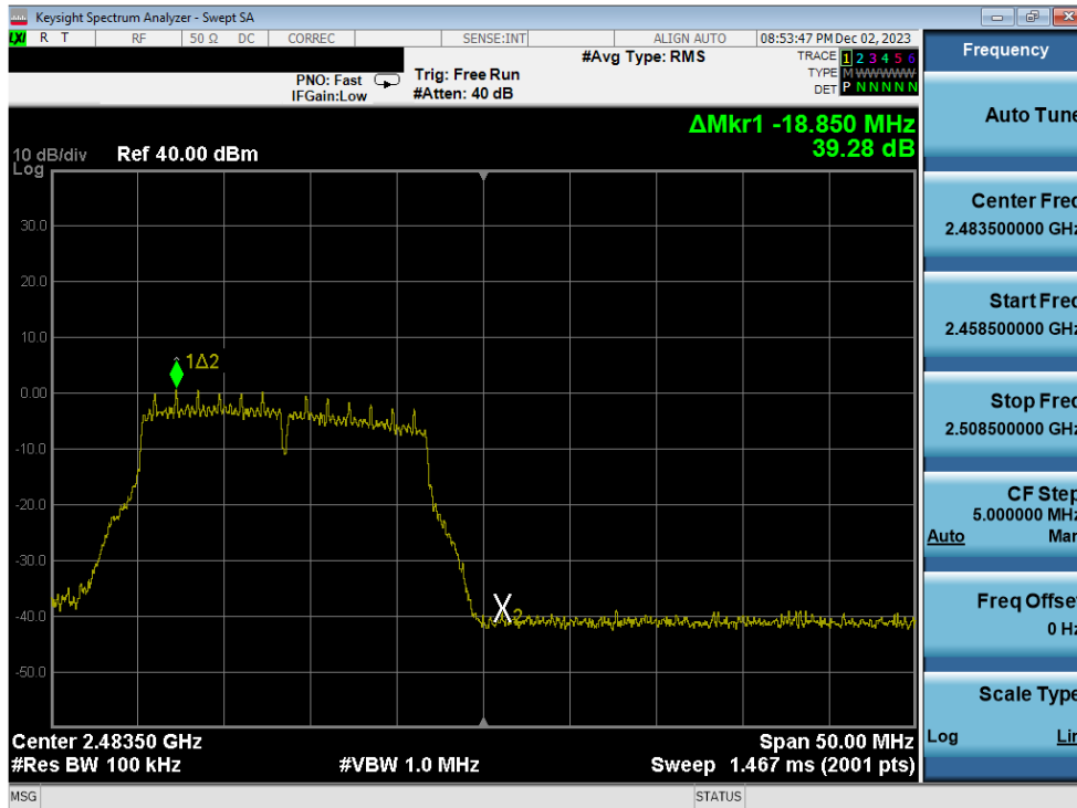
Plot 7-313. Band Edge Plot Antenna 1a (802.11g – Ch. 13) – 12Mbps
