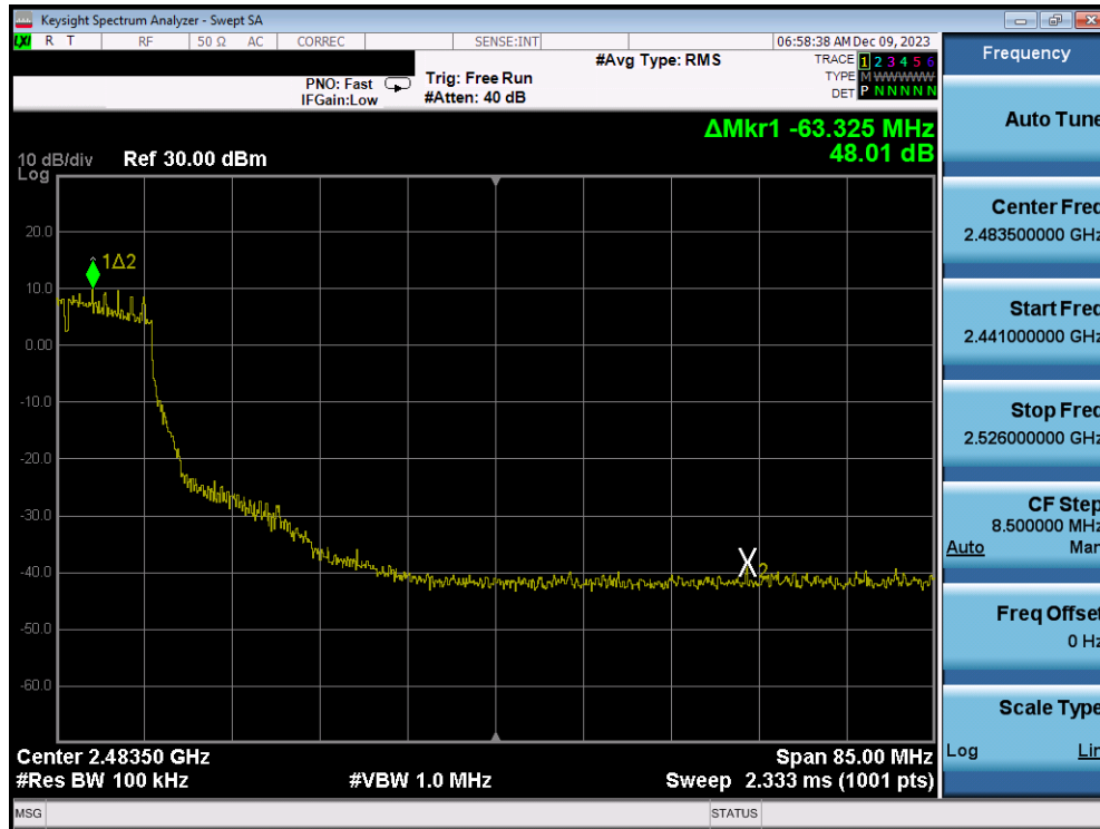
Plot 7-307. Band Edge Plot Antenna 1a (802.11g - Ch. 7) - 12Mbps
