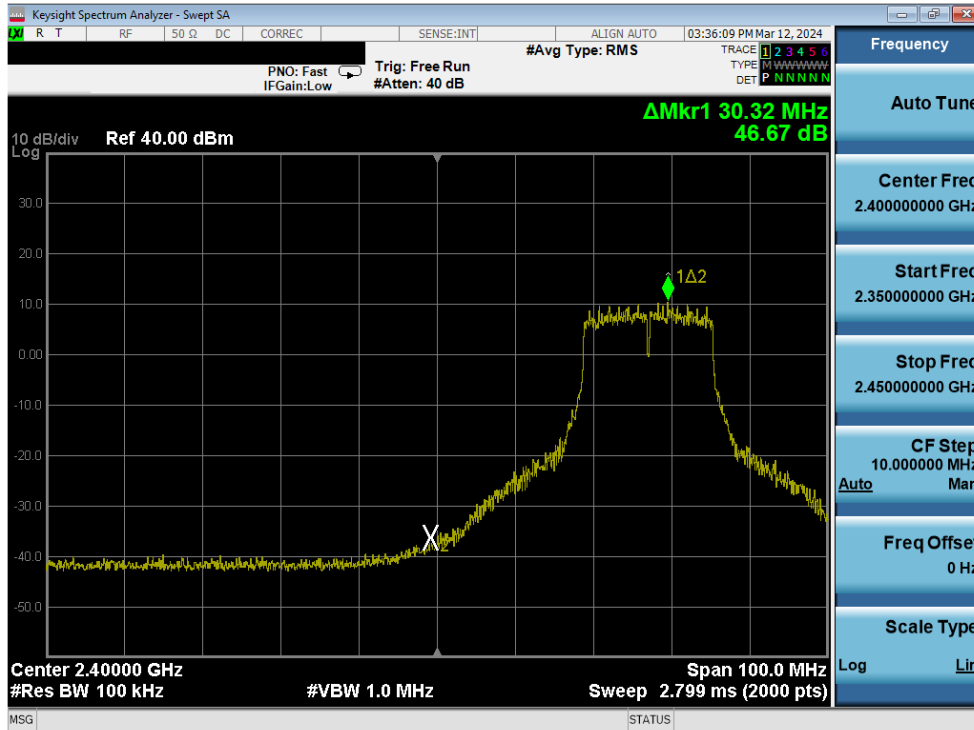
Plot 7-263. Band Edge Plot Antenna 3a (802.11g – Ch. 4) – 54Mbps
