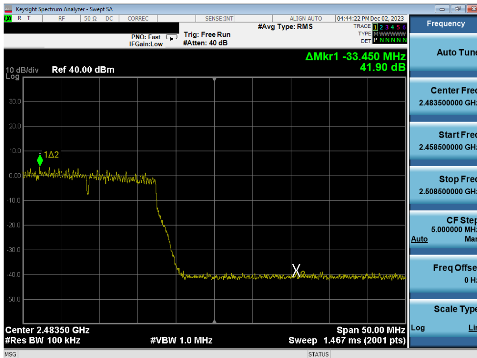
Plot 7-286. Band Edge Plot Antenna 3a (802.11n (2.4GHz) - Ch. 12) - MCS7
