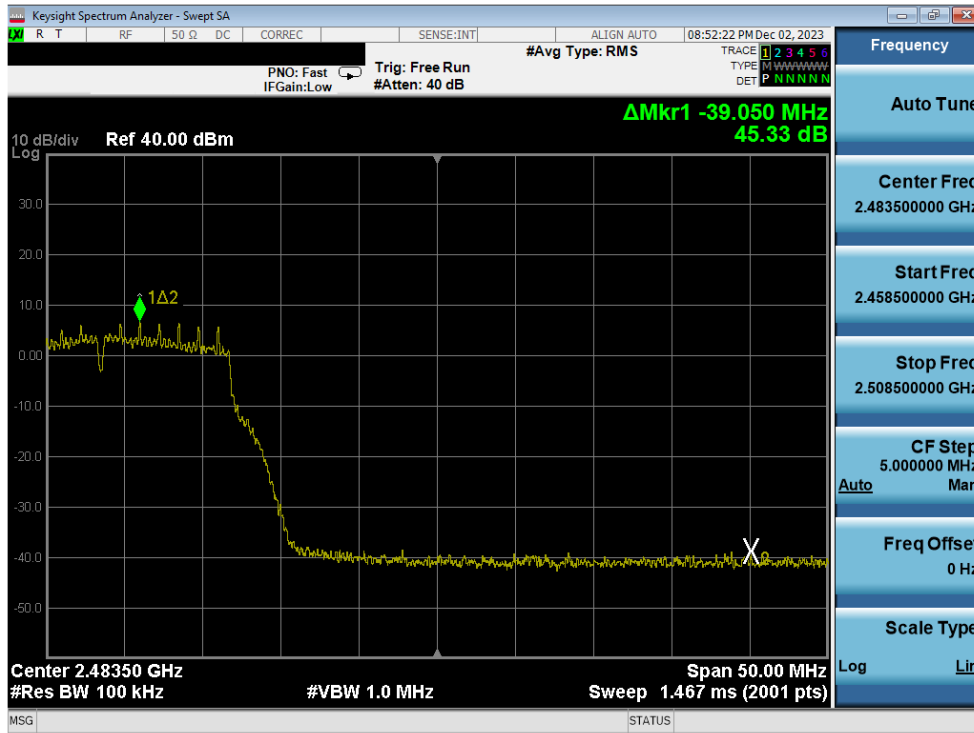
Plot 7-311. Band Edge Plot Antenna 1a (802.11g – Ch. 11) – 12Mbps
