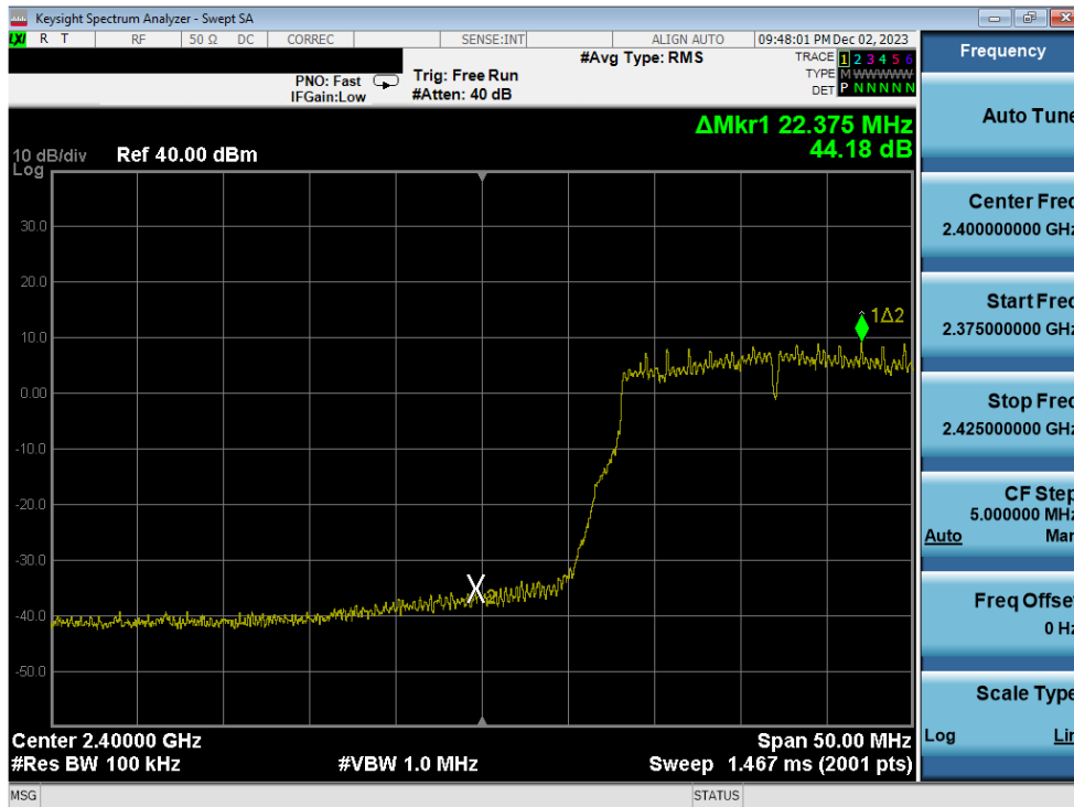
Plot 7-355. Band Edge Plot Antenna 1a (802.11n (2.4GHz) – Ch. 2) – MCS4
