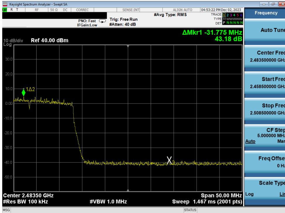
Plot 7-299. Band Edge Plot Antenna 3a (802.11ax (SU - 2.4GHz) – Ch. 11) – MCS9
