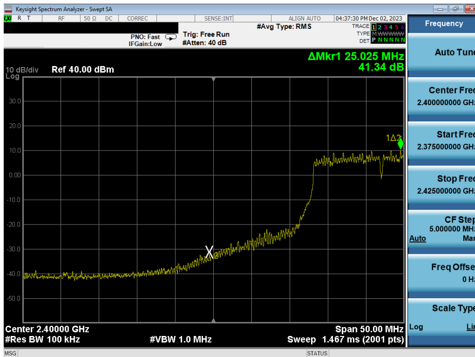
Plot 7-276. Band Edge Plot Antenna 3a (802.11n (2.4GHz) – Ch. 3) – MCS7
