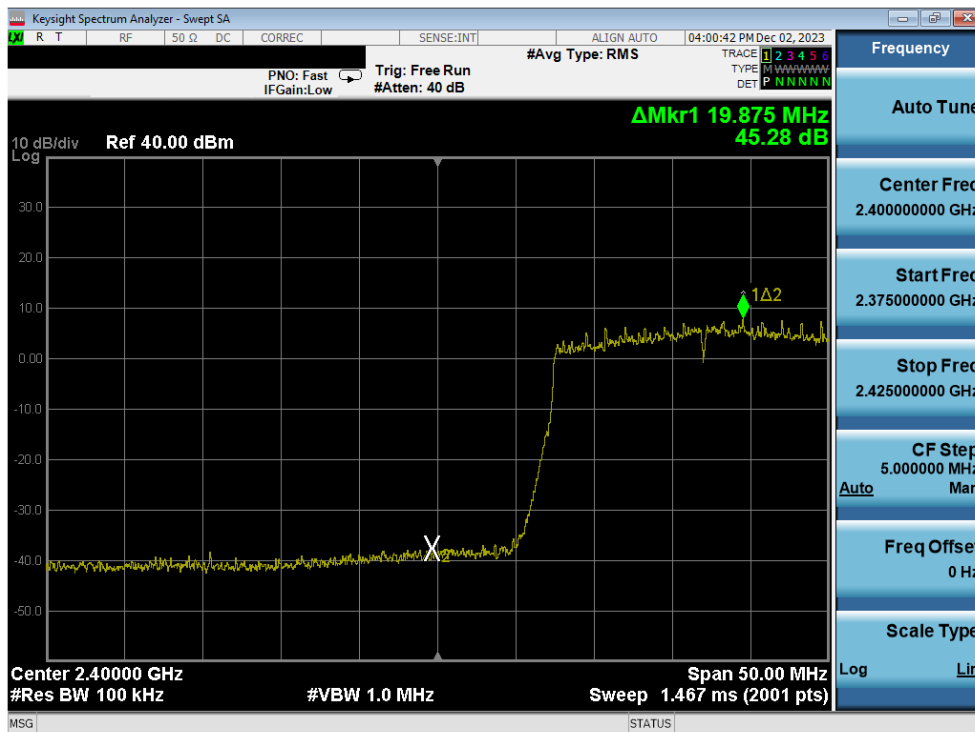
Plot 7-243. Band Edge Plot Antenna 3a (802.11ax (SU - 2.4GHz) – Ch. 2) – MCS4
