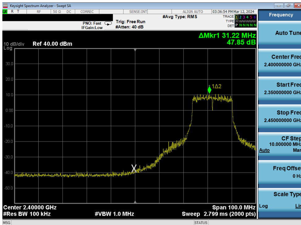
Plot 7-264. Band Edge Plot Antenna 3a (802.11g – Ch. 5) – 54Mbps
