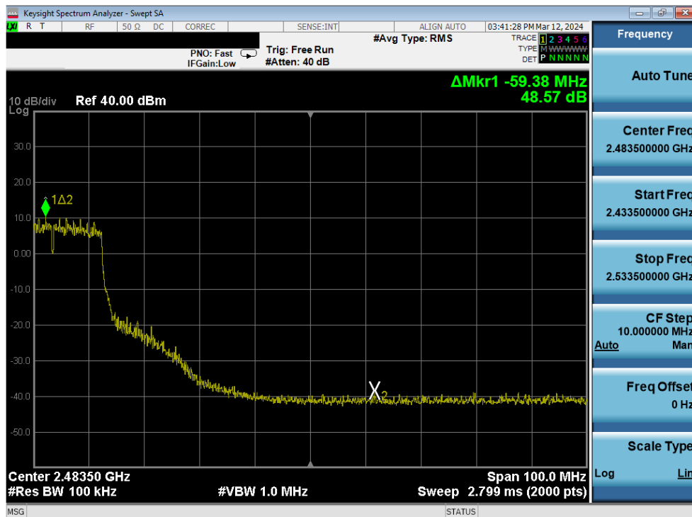
Plot 7-280. Band Edge Plot Antenna 3a (802.11n (2.4GHz) – Ch. 6 (high)) – MCS7
