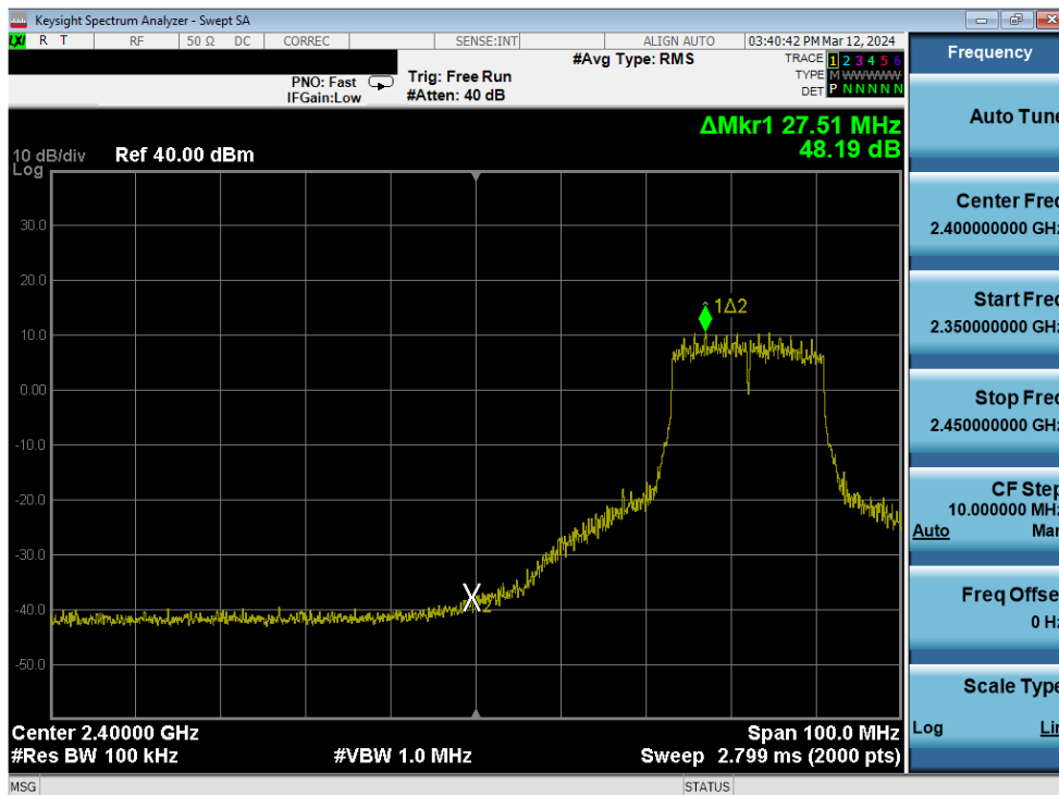
Plot 7-278. Band Edge Plot Antenna 3a (802.11n (2.4GHz) – Ch. 5) – MCS7
