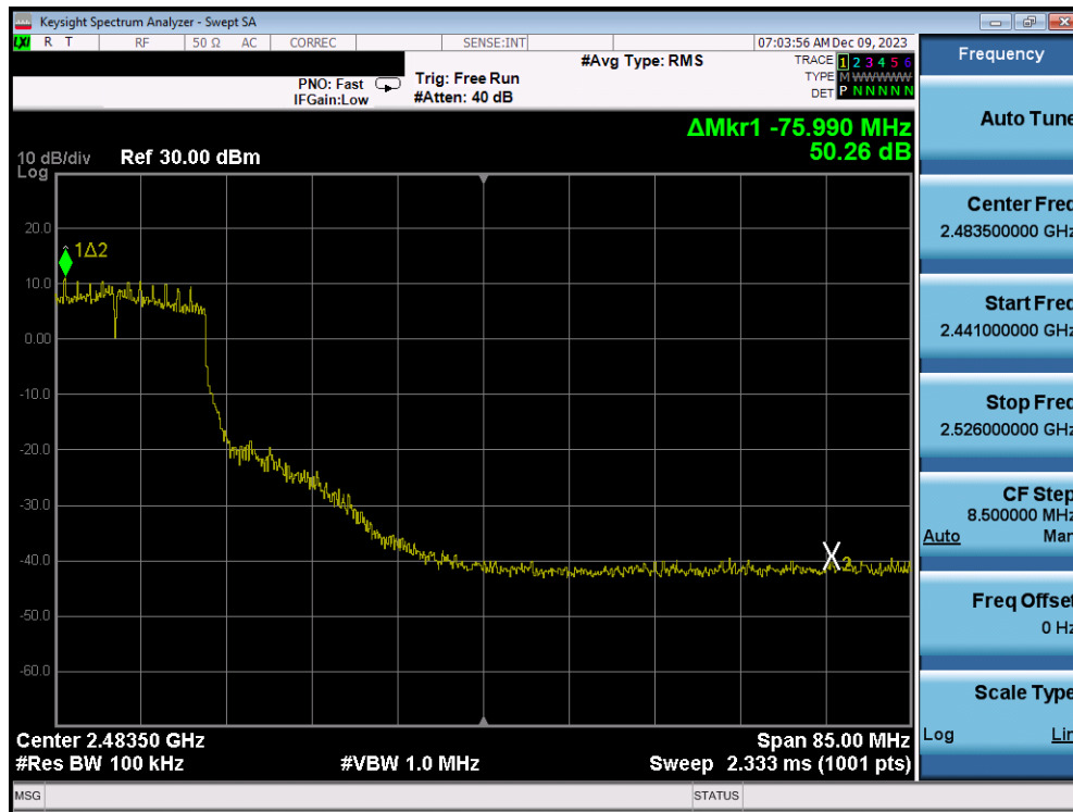
Plot 7-362. Band Edge Plot Antenna 1a (802.11n (2.4GHz) – Ch. 8) – MCS4
