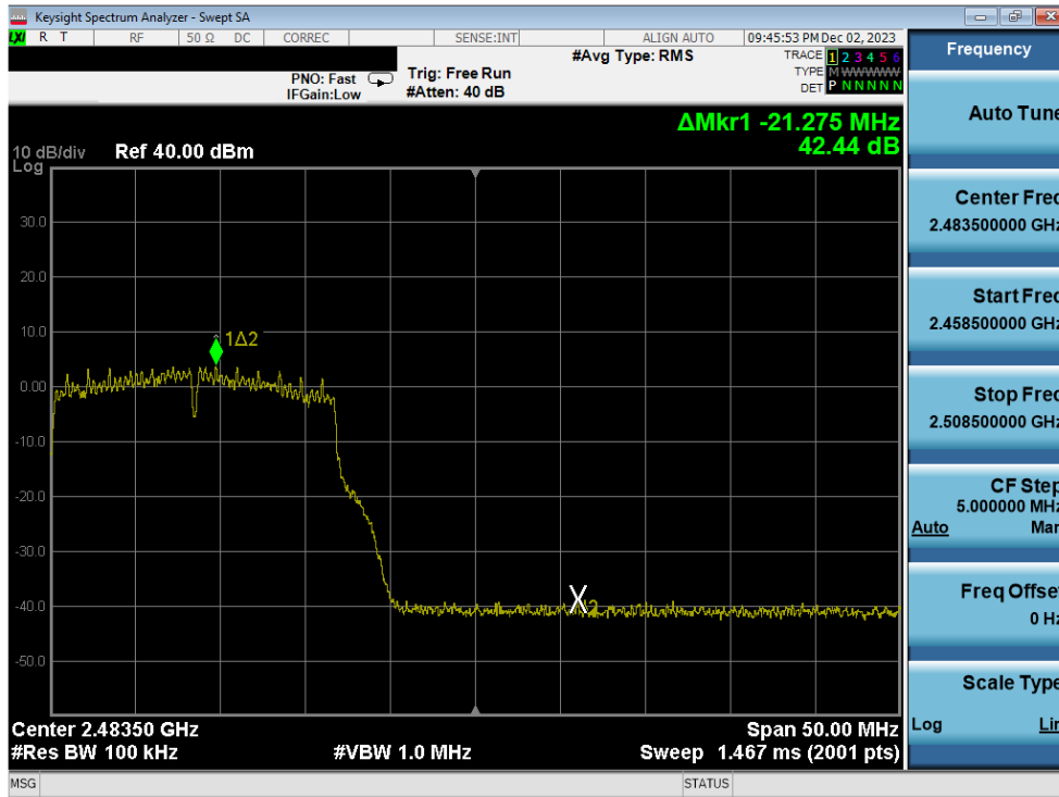
Plot 7-352. Band Edge Plot Antenna 1a (802.11g – Ch. 12) – 24Mbps
