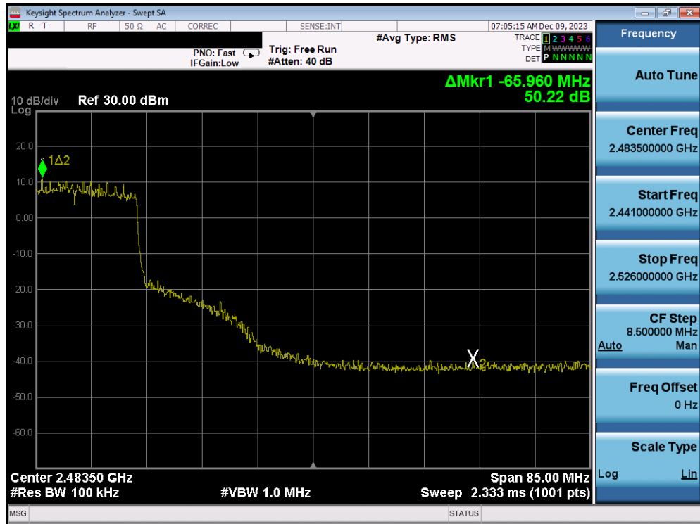
Plot 7-376. Band Edge Plot Antenna 1a (802.11ax (SU - 2.4GHz) – Ch. 8) – MCS4
