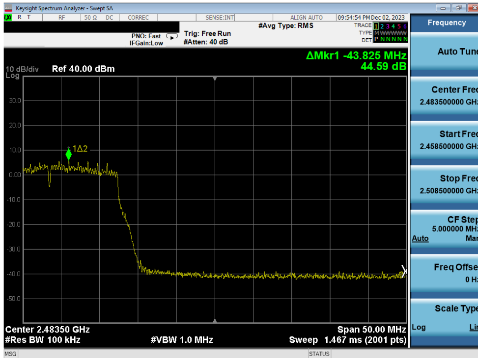
Plot 7-365. Band Edge Plot Antenna 1a (802.11n (2.4GHz) – Ch. 11) – MCS4
