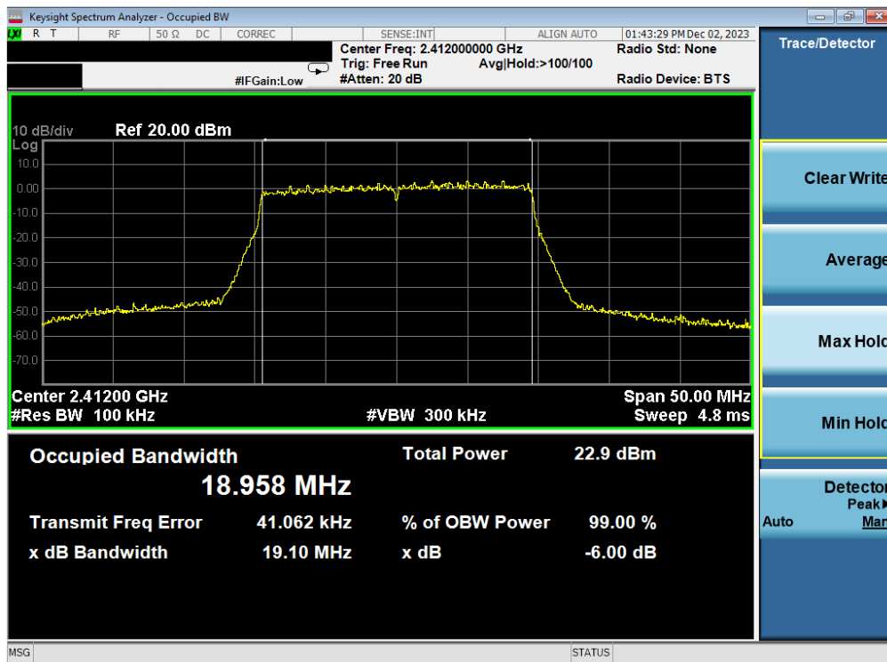
Plot 7-28. 6 dB BW and 99% OBW Plot Antenna 3a (802.11ax (SU - 2.4GHz) – Ch. 1) – MCS9
