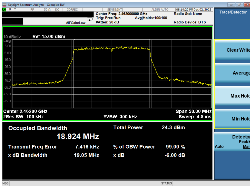
Plot 7-60. 6 dB BW and 99% OBW Plot Antenna 1a (802.11ax (SU - 2.4GHz) – Ch. 11) – MCS9
