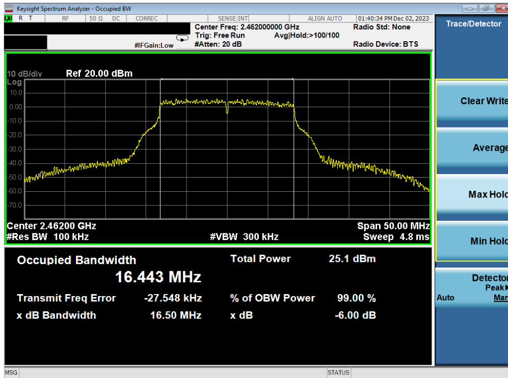
Plot 7-24. 6 dB BW and 99% OBW Plot Antenna 3a (802.11g – Ch. 11) – 54Mbps
