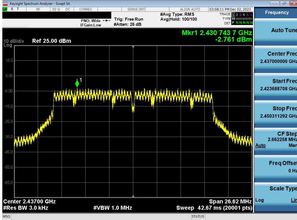
Plot 7-86. Power Spectral Density Plot Antenna 3a (802.11n (2.4GHz) – Ch. 6) – MCS7
