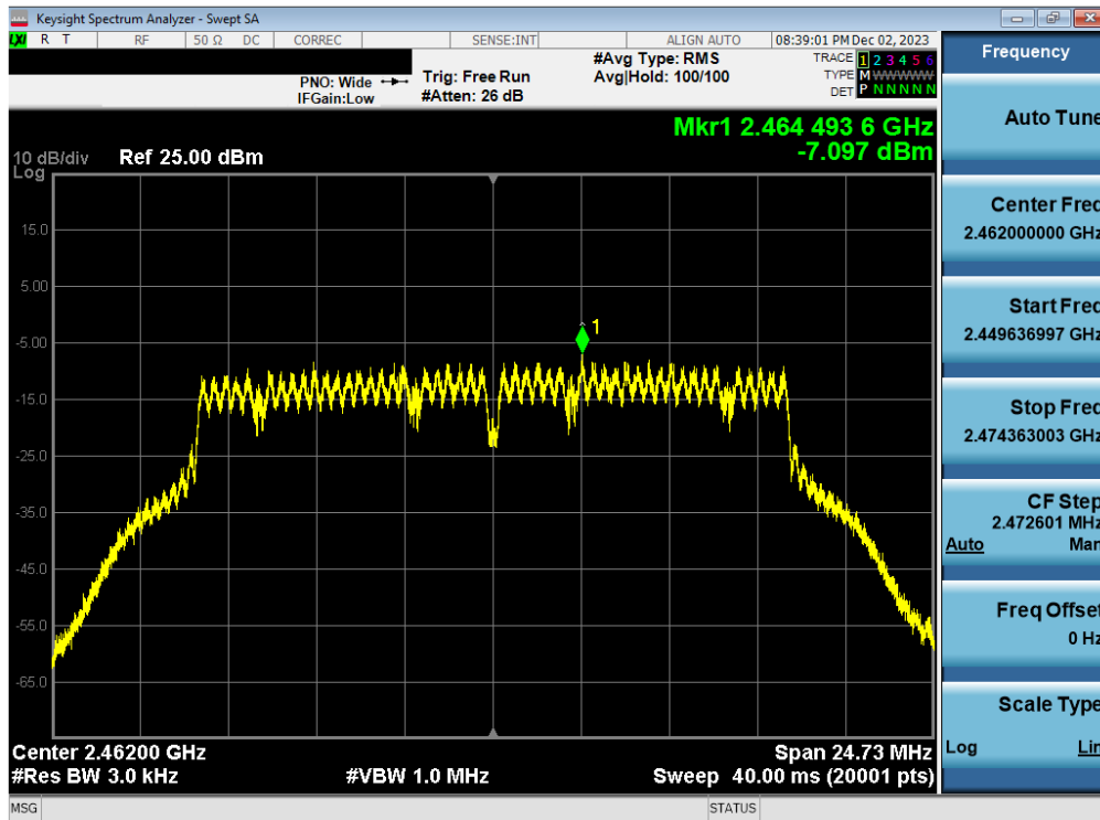
Plot 7-114. Power Spectral Density Plot Antenna 1a (802.11g – Ch. 11) – 54Mbps
