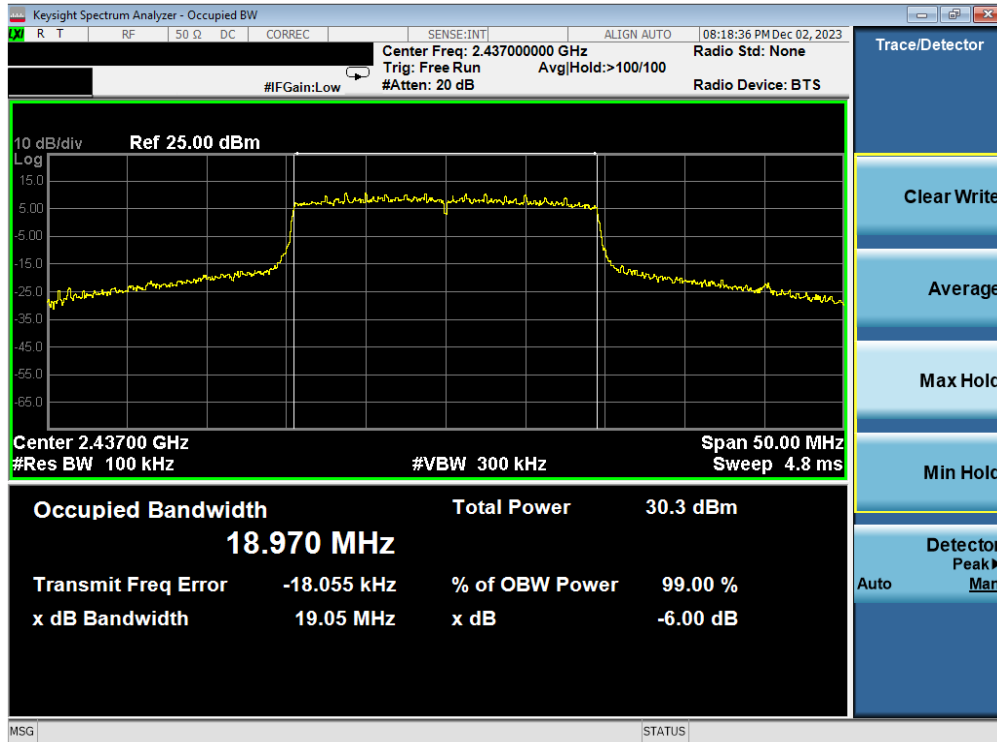
Plot 7-59. 6 dB BW and 99% OBW Plot Antenna 1a (802.11ax (SU - 2.4GHz) – Ch. 6) – MCS9
