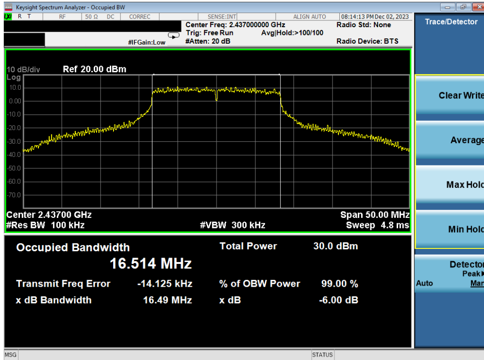
Plot 7-53. 6 dB BW and 99% OBW Plot Antenna 1a (802.11g – Ch. 6) – 54Mbps
