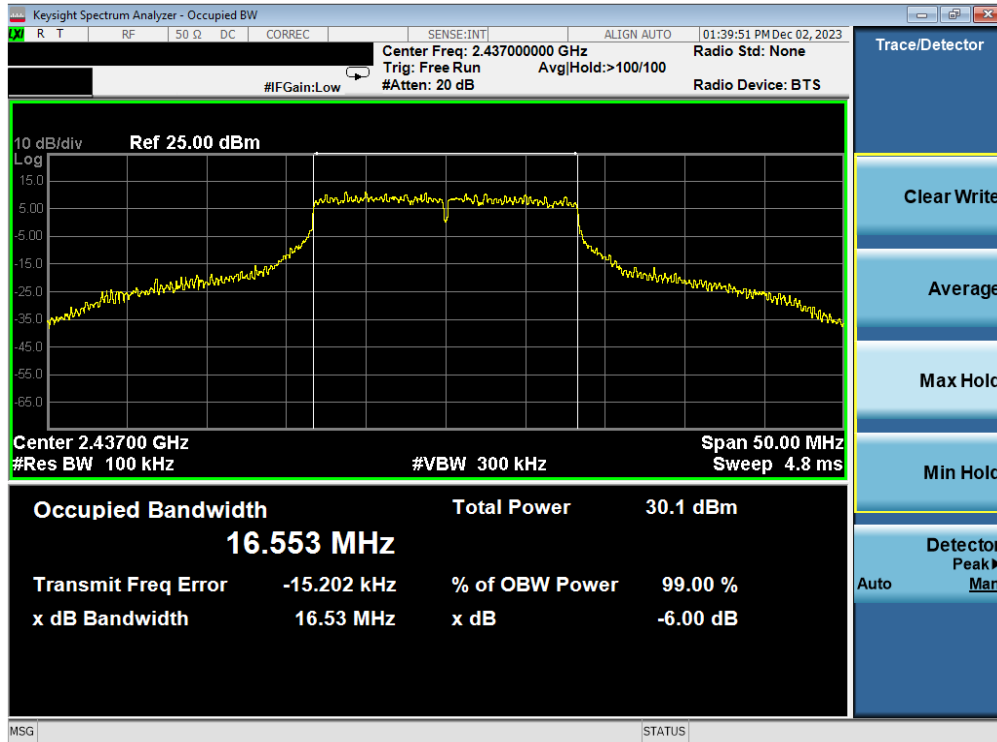
Plot 7-23. 6 dB BW and 99% OBW Plot Antenna 3a (802.11g – Ch. 6) – 54Mbps
