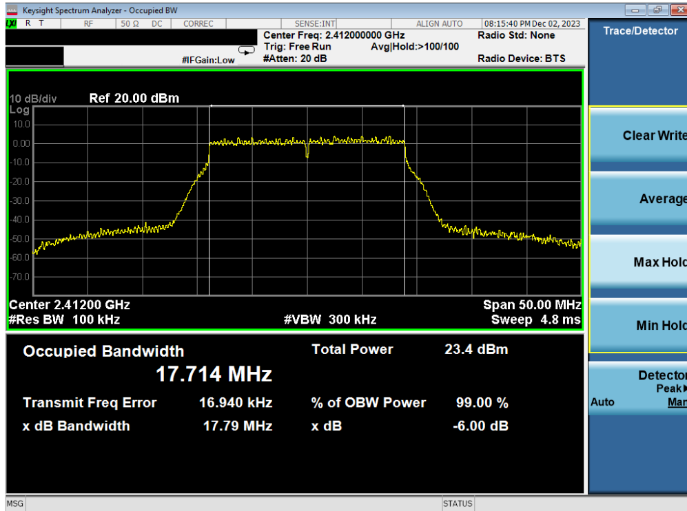
Plot 7-55. 6 dB BW and 99% OBW Plot Antenna 1a (802.11n (2.4GHz) – Ch. 1) – MCS7
