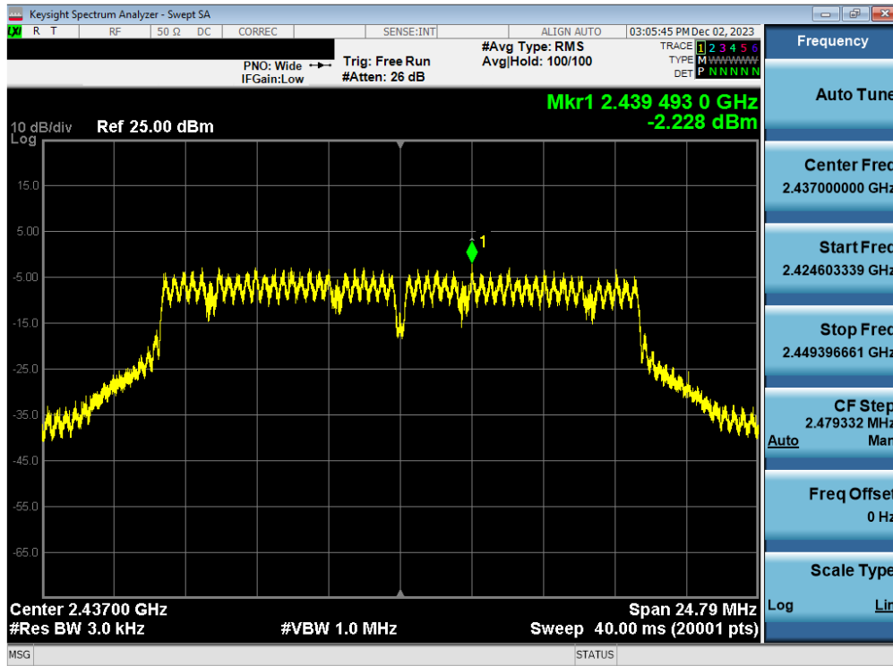
Plot 7-83. Power Spectral Density Plot Antenna 3a (802.11g – Ch. 6) – 54Mbps
