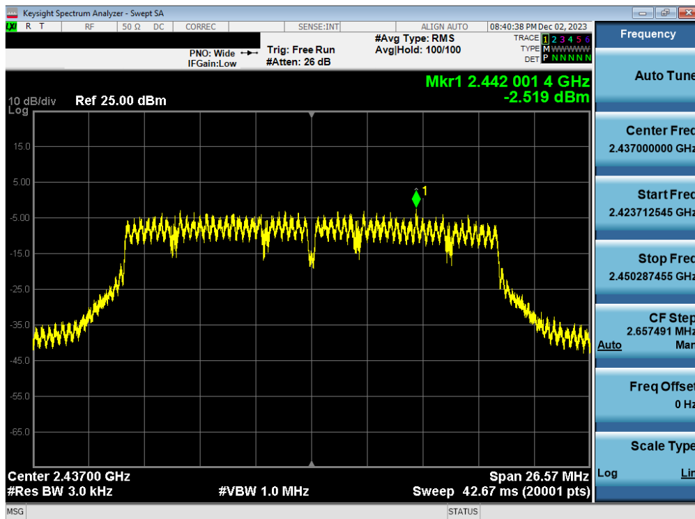
Plot 7-116. Power Spectral Density Plot Antenna 1a (802.11n (2.4GHz) – Ch. 6) – MCS7
