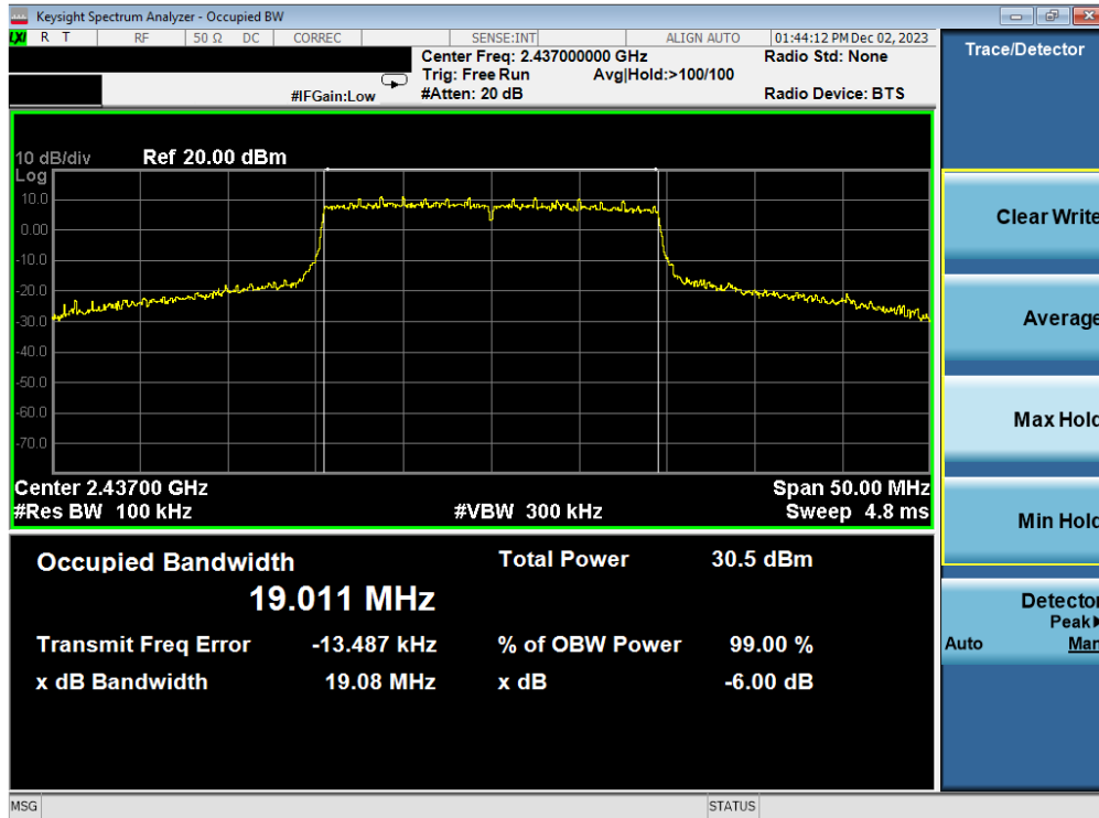
Plot 7-29. 6 dB BW and 99% OBW Plot Antenna 3a (802.11ax (SU - 2.4GHz) – Ch. 6) – MCS9
