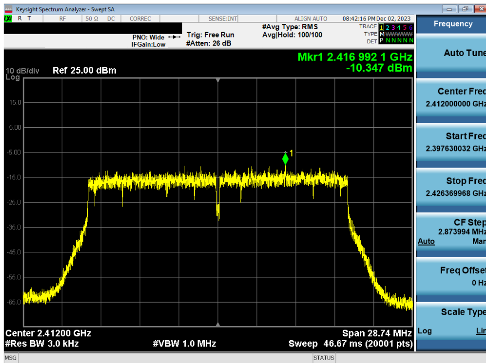
Plot 7-118. Power Spectral Density Plot Antenna 1a (802.11ax (SU - 2.4GHz) – Ch. 1) – MCS9
