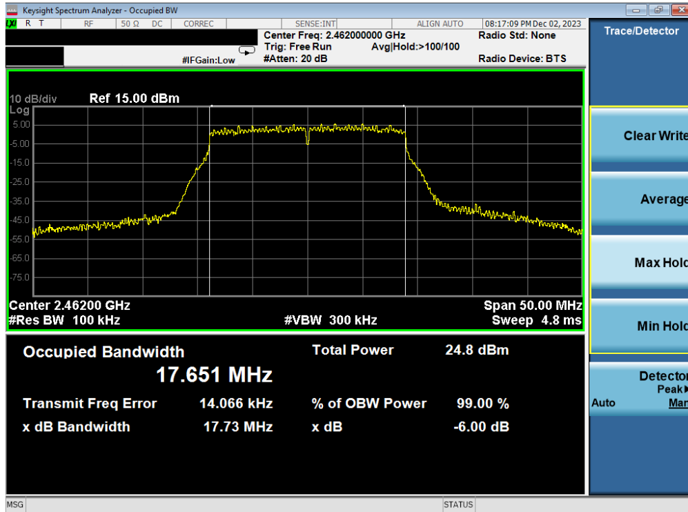
Plot 7-57. 6 dB BW and 99% OBW Plot Antenna 1a (802.11n (2.4GHz) – Ch. 11) – MCS7
