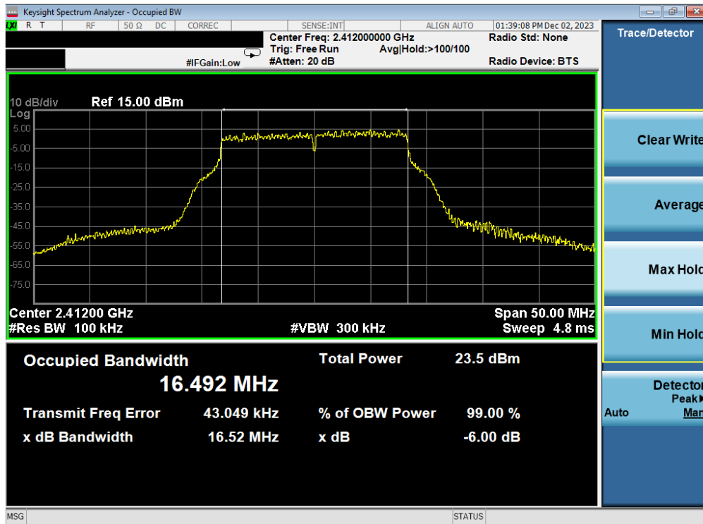
Plot 7-22. 6 dB BW and 99% OBW Plot Antenna 3a (802.11g – Ch. 1) – 54Mbps
