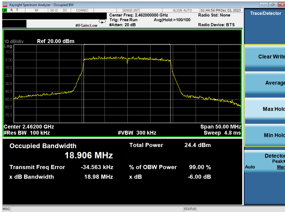
Plot 7-30. 6 dB BW and 99% OBW Plot Antenna 3a (802.11ax (SU - 2.4GHz) – Ch. 11) – MCS9
