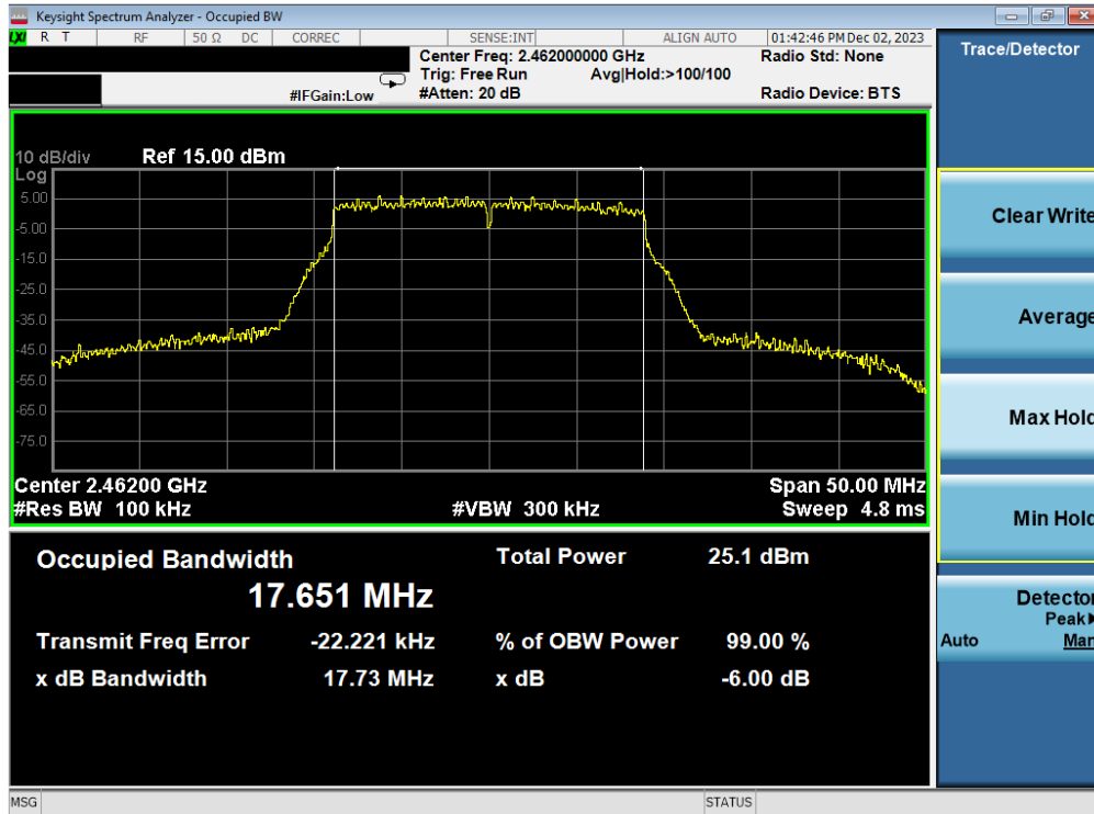
Plot 7-27. 6 dB BW and 99% OBW Plot Antenna 3a (802.11n (2.4GHz) – Ch. 11) – MCS7
