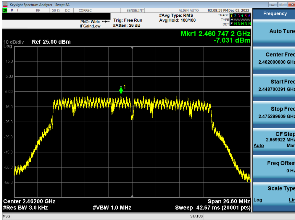
Plot 7-87. Power Spectral Density Plot Antenna 3a (802.11n (2.4GHz) – Ch. 11) – MCS7
