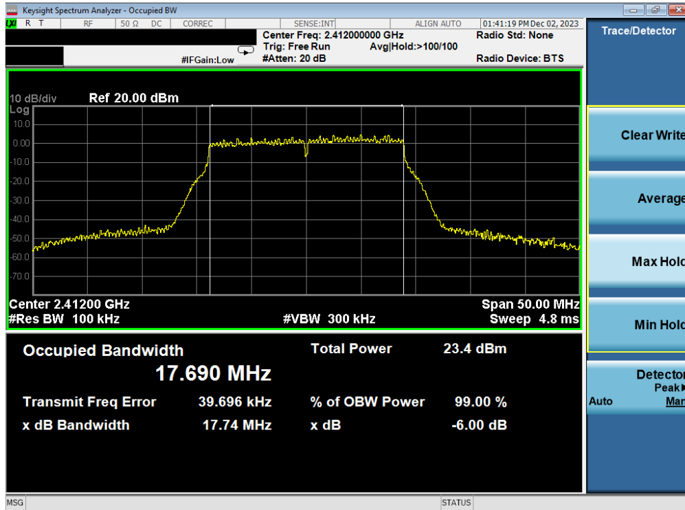
Plot 7-25. 6 dB BW and 99% OBW Plot Antenna 3a (802.11n (2.4GHz) – Ch. 1) – MCS7
