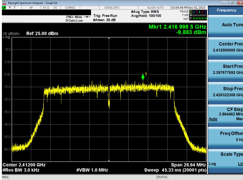
Plot 7-88. Power Spectral Density Plot Antenna 3a (802.11ax (SU - 2.4GHz) – Ch. 1) – MCS9
