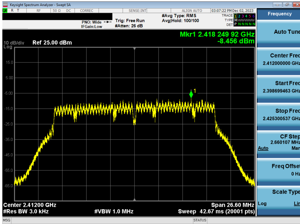
Plot 7-85. Power Spectral Density Plot Antenna 3a (802.11n (2.4GHz) – Ch. 1) – MCS7
