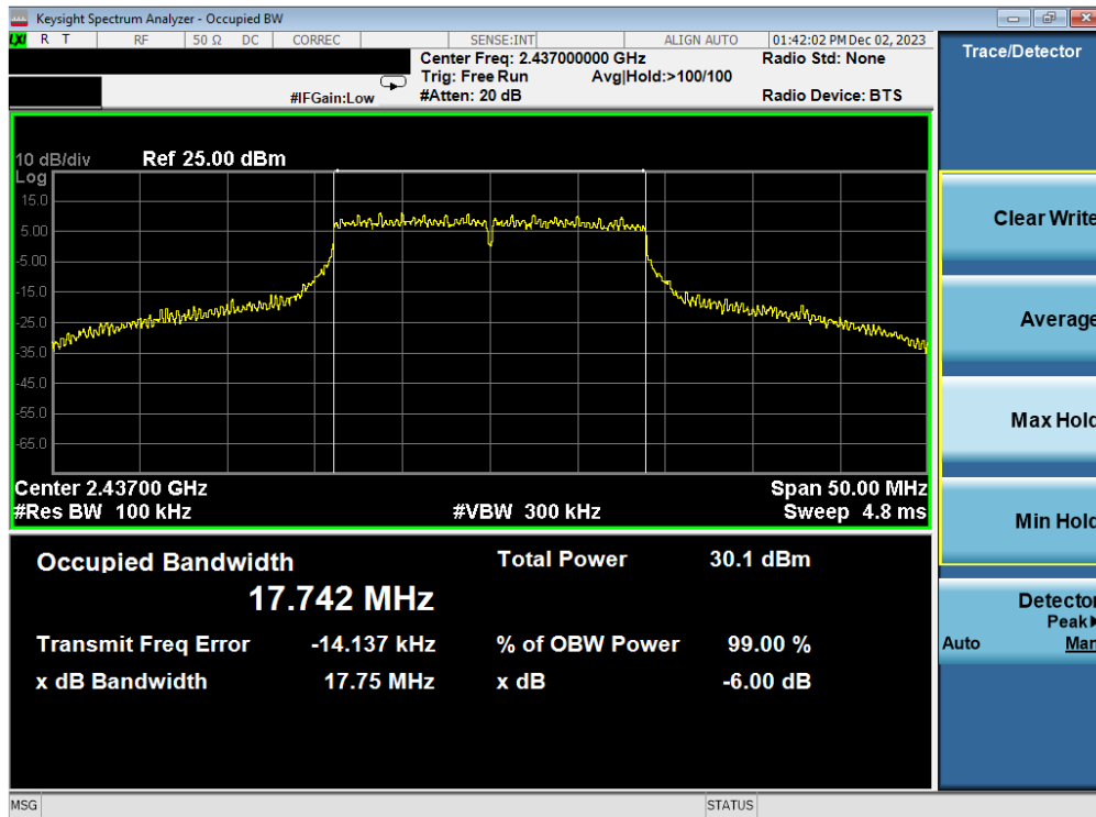
Plot 7-26. 6 dB BW and 99% OBW Plot Antenna 3a (802.11n (2.4GHz) – Ch. 6) – MCS7
