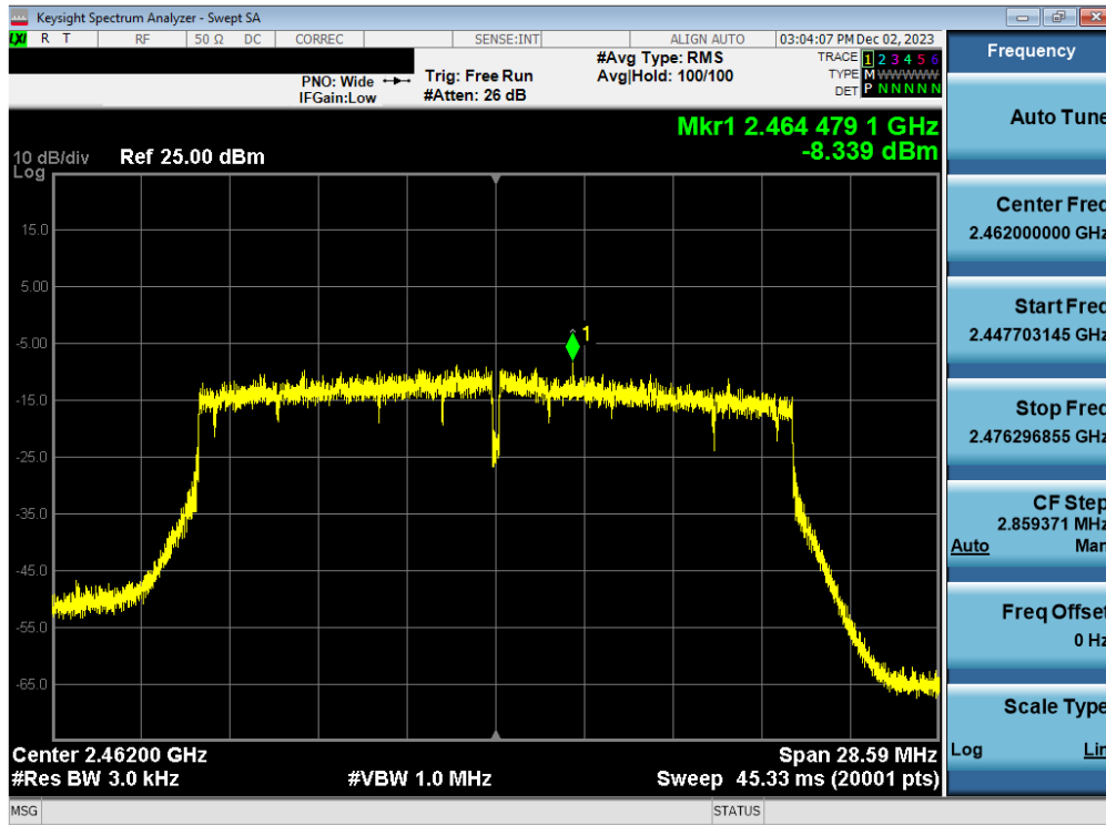
Plot 7-78. Power Spectral Density Plot Antenna 3a (802.11ax (SU - 2.4GHz) – Ch. 11) – MCS4
