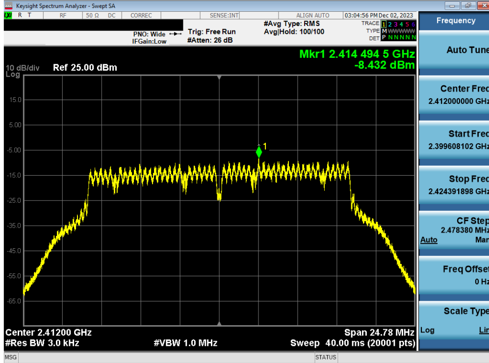
Plot 7-82. Power Spectral Density Plot Antenna 3a (802.11g – Ch. 1) – 54Mbps
