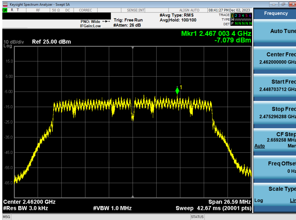
Plot 7-117. Power Spectral Density Plot Antenna 1a (802.11n (2.4GHz) – Ch. 11) – MCS7
