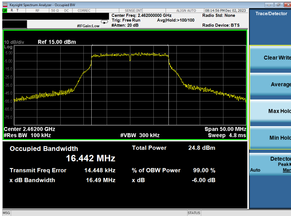
Plot 7-54. 6 dB BW and 99% OBW Plot Antenna 1a (802.11g – Ch. 11) – 54Mbps
