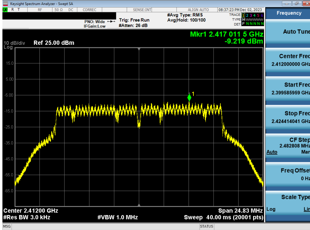
Plot 7-112. Power Spectral Density Plot Antenna 1a (802.11g – Ch. 1) – 54Mbps
