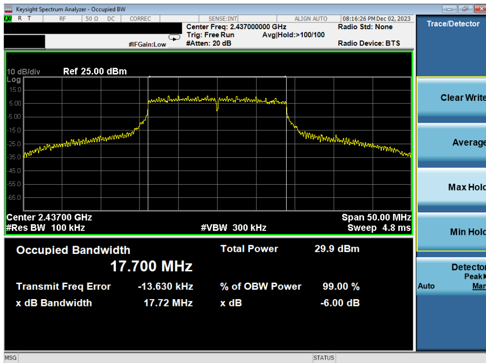
Plot 7-56. 6 dB BW and 99% OBW Plot Antenna 1a (802.11n (2.4GHz) – Ch. 6) – MCS7
