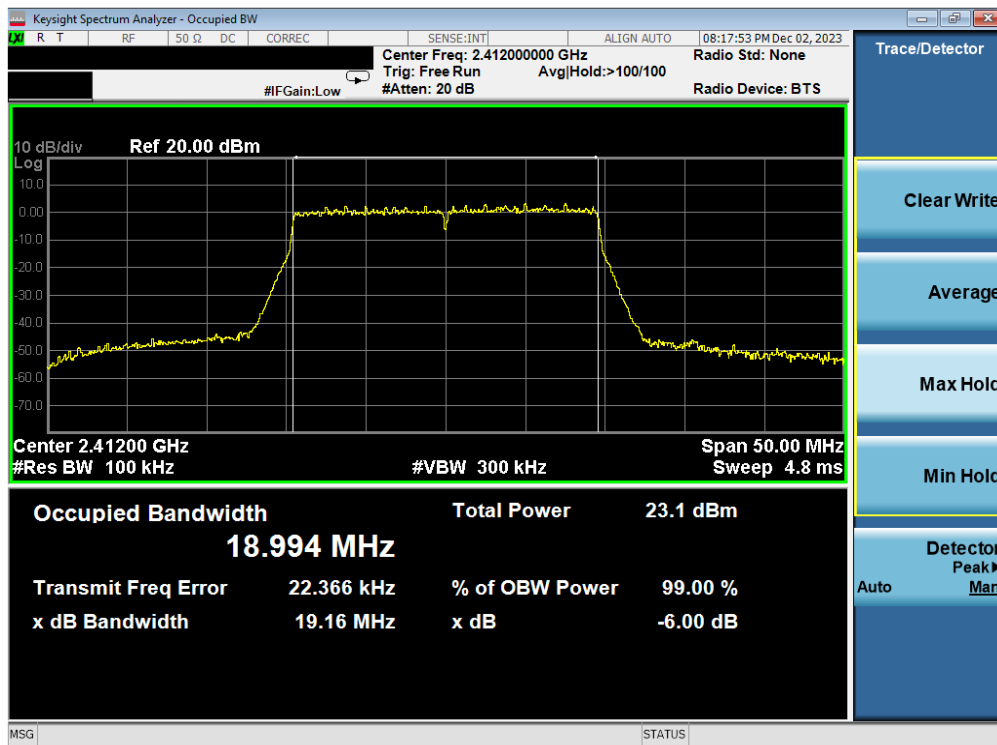
Plot 7-58. 6 dB BW and 99% OBW Plot Antenna 1a (802.11ax (SU - 2.4GHz) – Ch. 1) – MCS9
