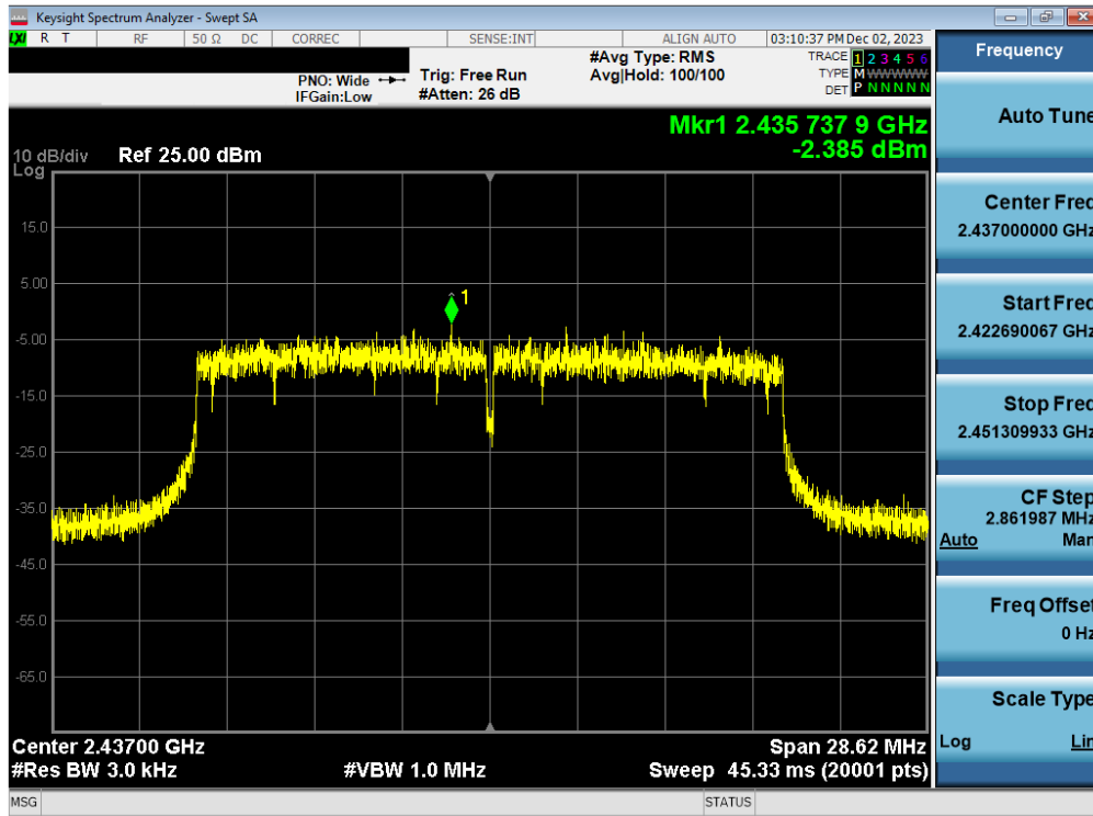
Plot 7-89. Power Spectral Density Plot Antenna 3a (802.11ax (SU - 2.4GHz) – Ch. 6) – MCS9
