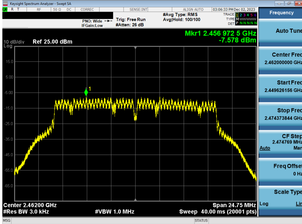
Plot 7-84. Power Spectral Density Plot Antenna 3a (802.11g – Ch. 11) – 54Mbps
