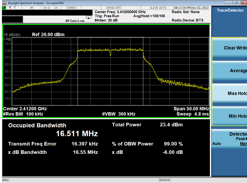
Plot 7-52. 6 dB BW and 99% OBW Plot Antenna 1a (802.11g – Ch. 1) – 54Mbps
