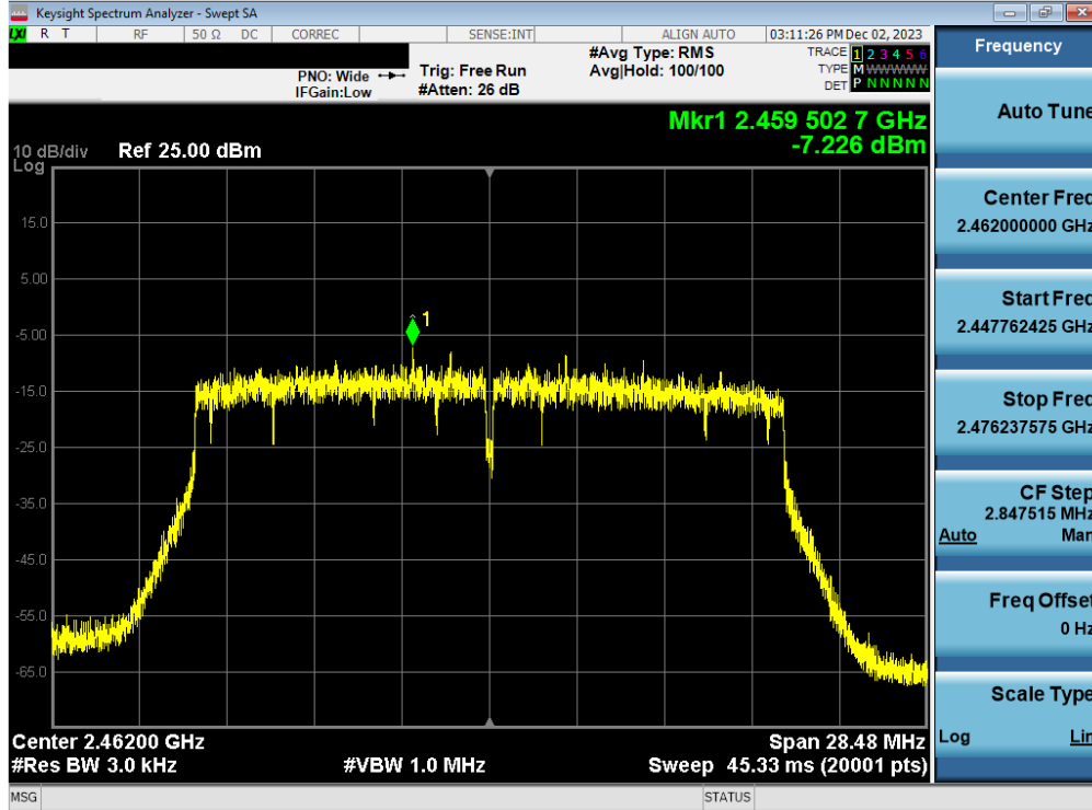
Plot 7-90. Power Spectral Density Plot Antenna 3a (802.11ax (SU - 2.4GHz) – Ch. 11) – MCS9
