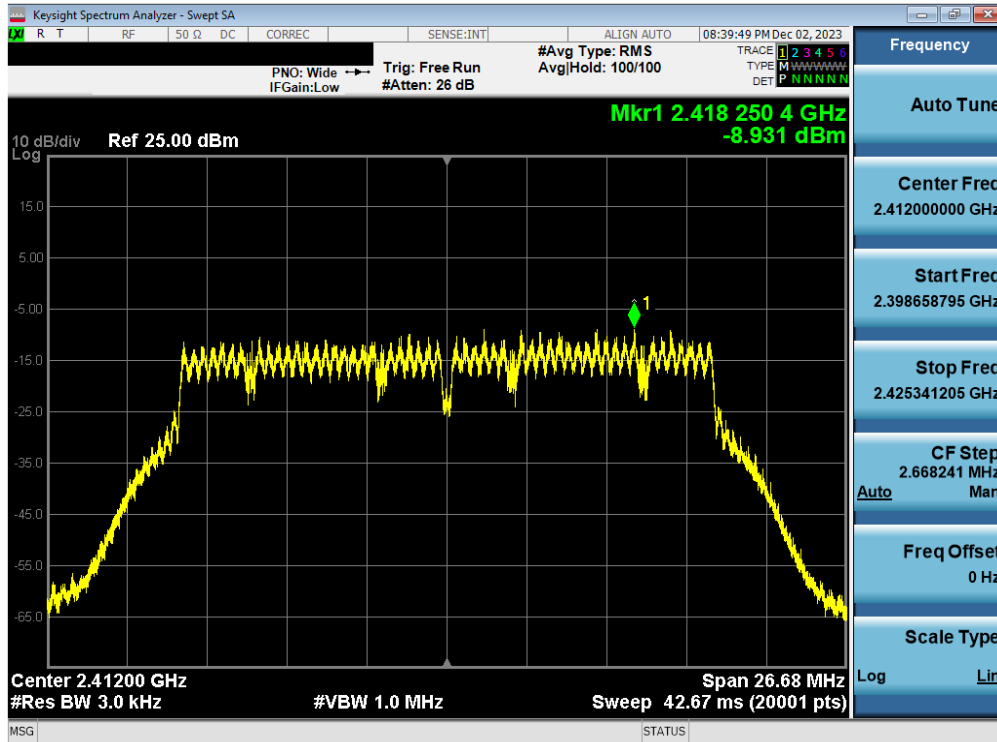
Plot 7-115. Power Spectral Density Plot Antenna 1a (802.11n (2.4GHz) – Ch. 1) – MCS7
