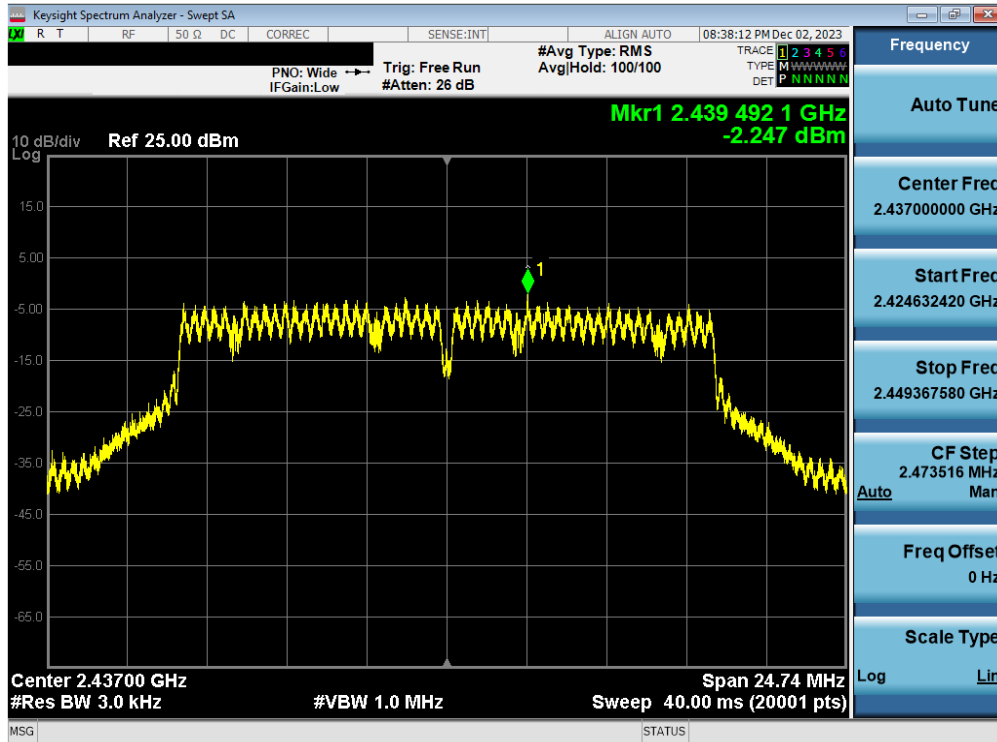
Plot 7-113. Power Spectral Density Plot Antenna 1a (802.11g – Ch. 6) – 54Mbps
