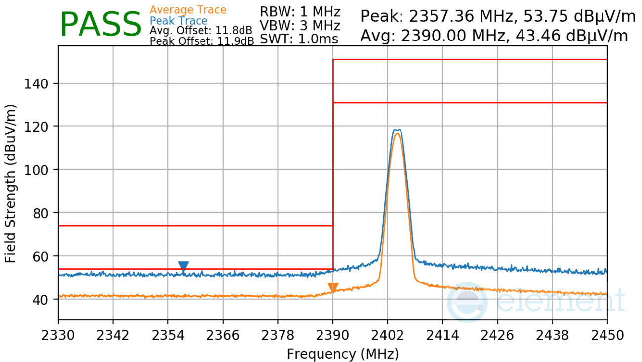
Plot 7-97. Radiated Restricted Lower Band Edge Measurement Antenna 1a (Average & Peak)
