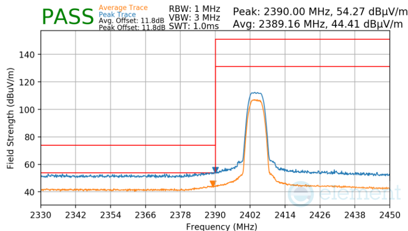
Plot 7-92. Radiated Restricted Lower Band Edge Measurement Antenna 3a
