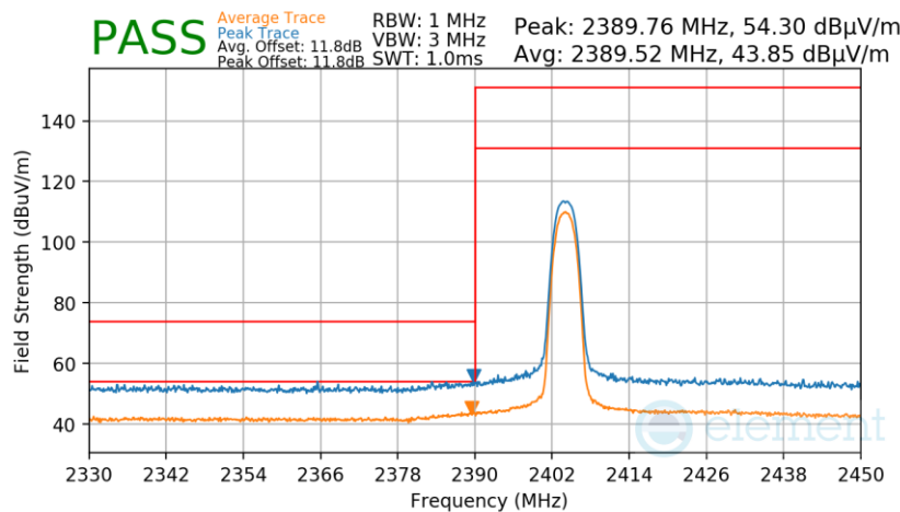
Plot 7-91. Radiated Restricted Lower Band Edge Measurement Antenna 3a
