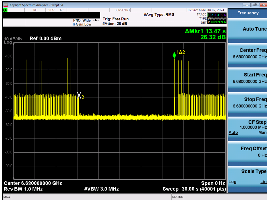
Plot 7-1322. Contention Based Protocol Timing Plot – UNII 7 – 160MHz Channel 143 – Low
