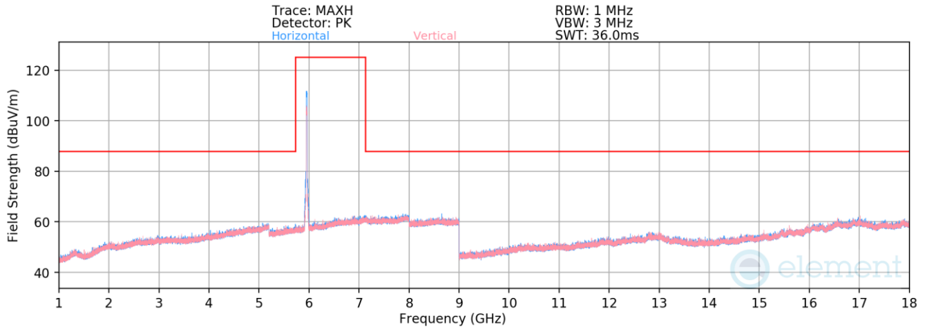
Plot 7-1333. Radiated Spurious Emissions above 1GHz Antenna 3c (802.11ax – Ch. 1)
