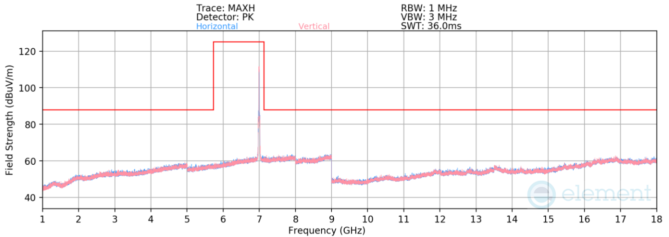
Plot 7-1355. Radiated Spurious Emissions above 1GHz Antenna 3a (802.11ax – Ch. 209, MCS0)
