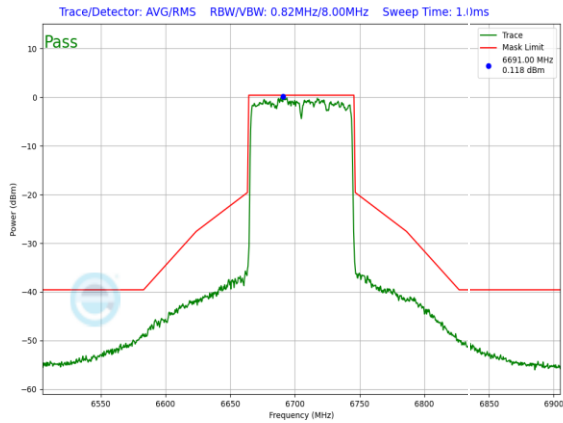
Plot 7-1293. SP In-Band Emission Plot SDM Diversity Antenna 3c (80MHz 802.11ax (UNII Band 7) – Ch. 151, MCS11)
