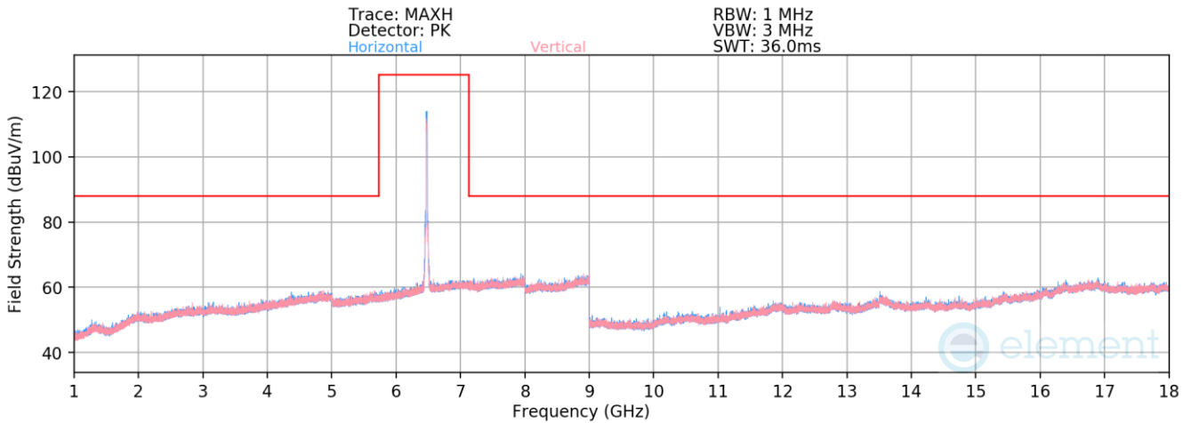
Plot 7-1349. Radiated Spurious Emissions above 1GHz Antenna 3a (802.11ax – Ch. 105, MCS0)
