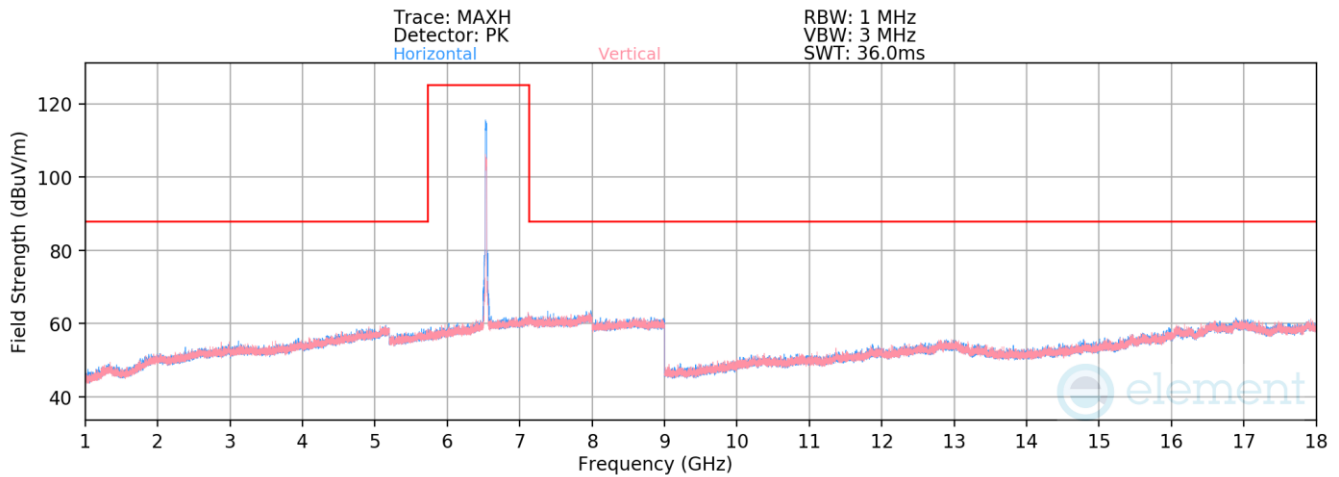
Plot 7-1339. Radiated Spurious Emissions above 1GHz Antenna 3c (802.11ax – Ch. 117)
