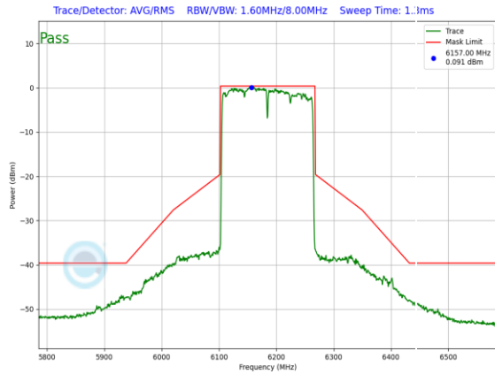
Plot 7-1271. SP In-Band Emission Plot SDM Diversity Antenna 3c (160MHz 802.11ax (UNII Band 5) – Ch. 47, MCS4)
