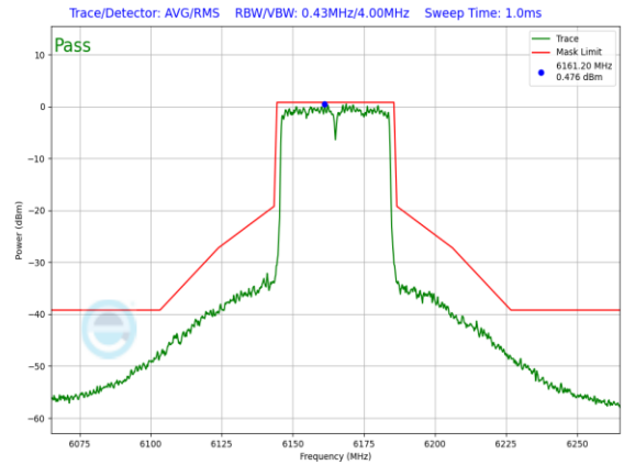
Plot 7-1284. SP In-Band Emission Plot SDM Diversity Antenna 3a (40MHz 802.11ax (UNII Band 5) – Ch. 43, MCS11)
