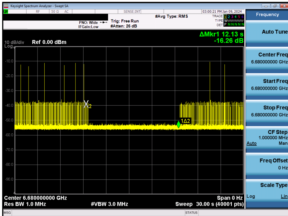
Plot 7-1324. Contention Based Protocol Timing Plot – UNII 7 – 160MHz Channel 143 – High
