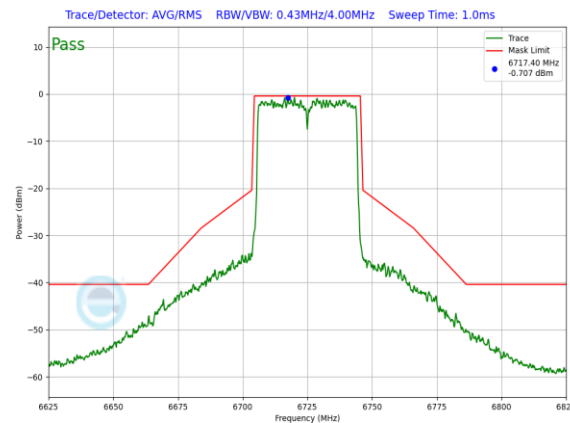
Plot 7-1292. SP In-Band Emission Plot SDM Diversity Antenna 3a (40MHz 802.11ax (UNII Band 7) – Ch. 155, MCS11)
