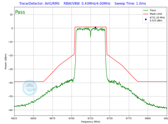
Plot 7-1291. SP In-Band Emission Plot SDM Diversity Antenna 3c (40MHz 802.11ax (UNII Band 7) – Ch. 155, MCS11)
