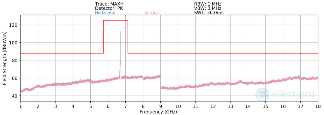
Plot 7-1352. Radiated Spurious Emissions above 1GHz Antenna 3a (802.11ax – Ch. 149, MCS0)
