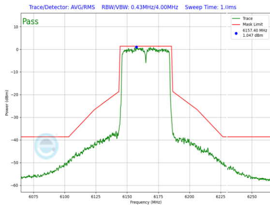
Plot 7-1283. SP In-Band Emission Plot SDM Diversity Antenna 3c (40MHz 802.11ax (UNII Band 5) – Ch. 43, MCS11)
