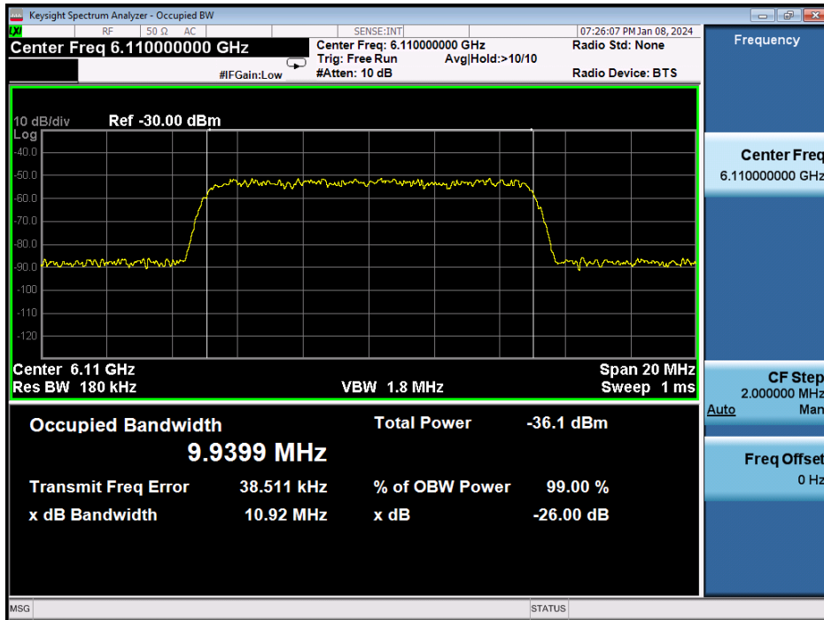
Plot 7-1298. AWGN Signal – UNII 5 – 160MHz - Low
