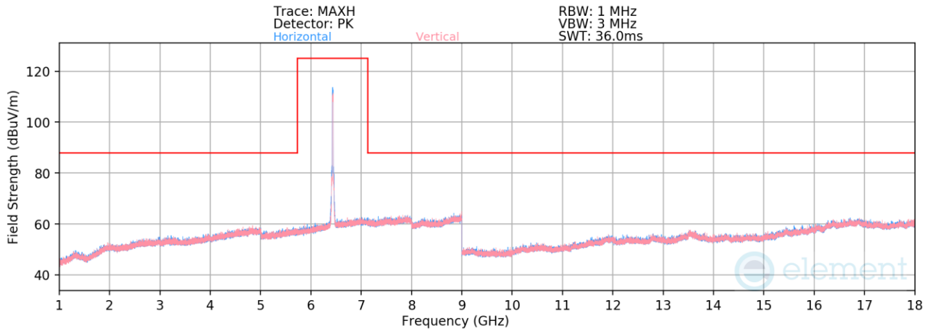
Plot 7-1348. Radiated Spurious Emissions above 1GHz Antenna 3a (802.11ax – Ch. 97)
