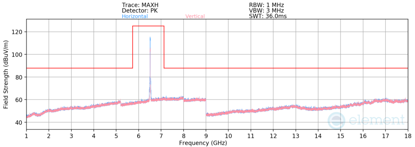
Plot 7-1338. Radiated Spurious Emissions above 1GHz Antenna 3c (802.11ax – Ch. 113)
