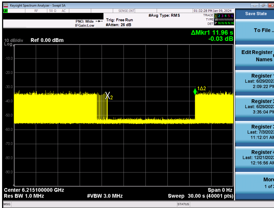
Plot 7-1313. Contention Based Protocol Timing Plot – UNII 5 – 20MHz Channel 53
