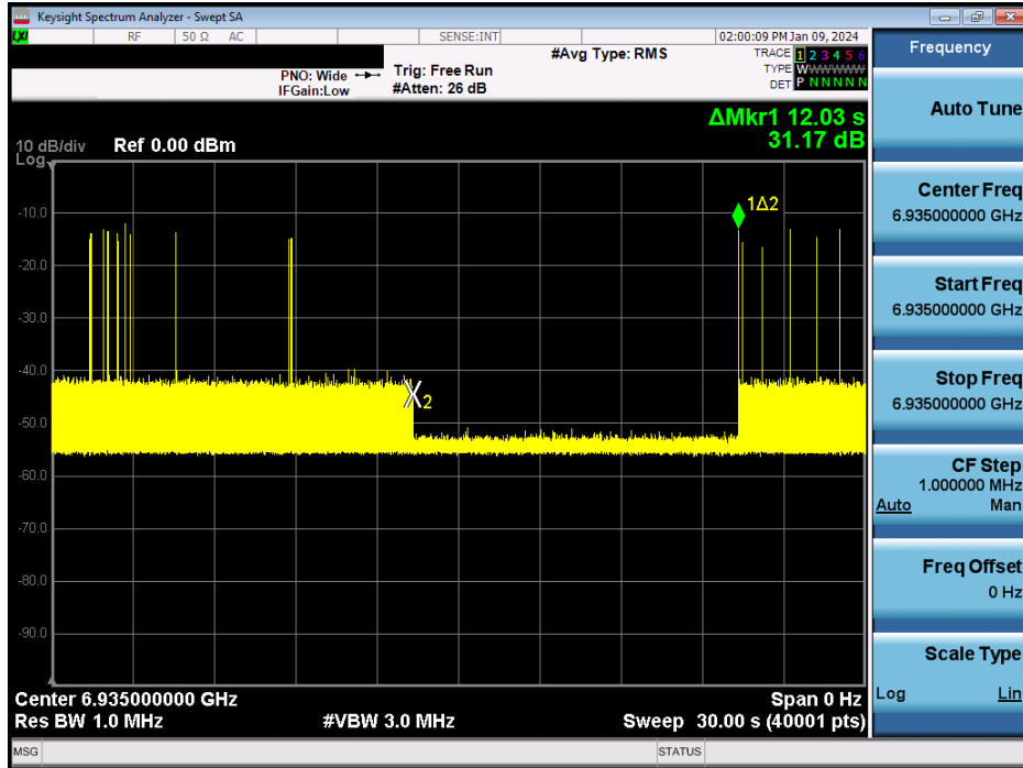
Plot 7-1325. Contention Based Protocol Timing Plot – UNII 8 – 20MHz Channel 197
