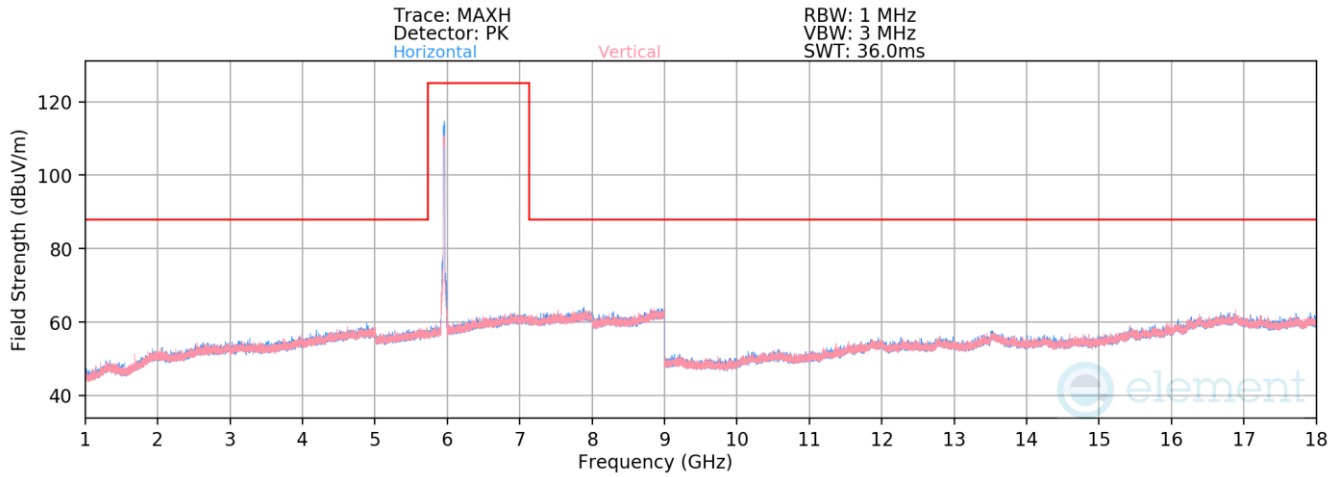
Plot 7-1345. Radiated Spurious Emissions above 1GHz Antenna 3a (802.11ax – Ch. 1)
