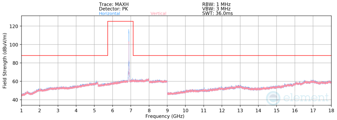
Plot 7-1342. Radiated Spurious Emissions above 1GHz Antenna 3c (802.11ax – Ch. 189)
