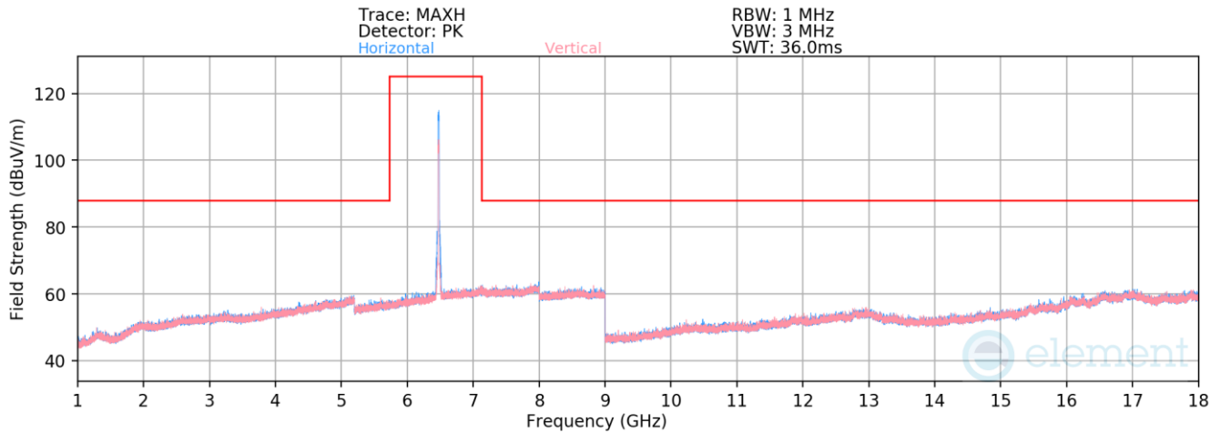
Plot 7-1337. Radiated Spurious Emissions above 1GHz Antenna 3c (802.11ax – Ch. 105, MCS0)
