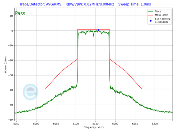
Plot 7-1285. SP In-Band Emission Plot SDM Diversity Antenna 3c (80MHz 802.11ax (UNII Band 5) – Ch. 39, MCS11)
