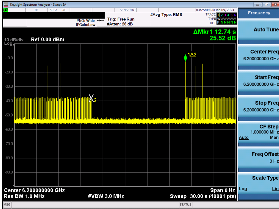
Plot 7-1315. Contention Based Protocol Timing Plot – UNII 5 – 160MHz Channel 47 – Mid
