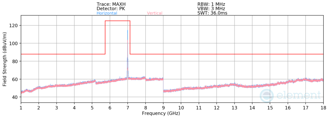
Plot 7-1343. Radiated Spurious Emissions above 1GHz Antenna 3c (802.11ax – Ch. 209, MCS0)
