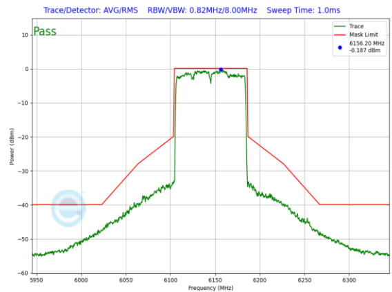
Plot 7-1286. SP In-Band Emission Plot SDM Diversity Antenna 3a (80MHz 802.11ax (UNII Band 5) – Ch. 39, MCS11)
