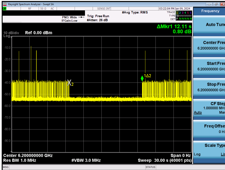
Plot 7-1314. Contention Based Protocol Timing Plot – UNII 5 – 160MHz Channel 47 – Low
