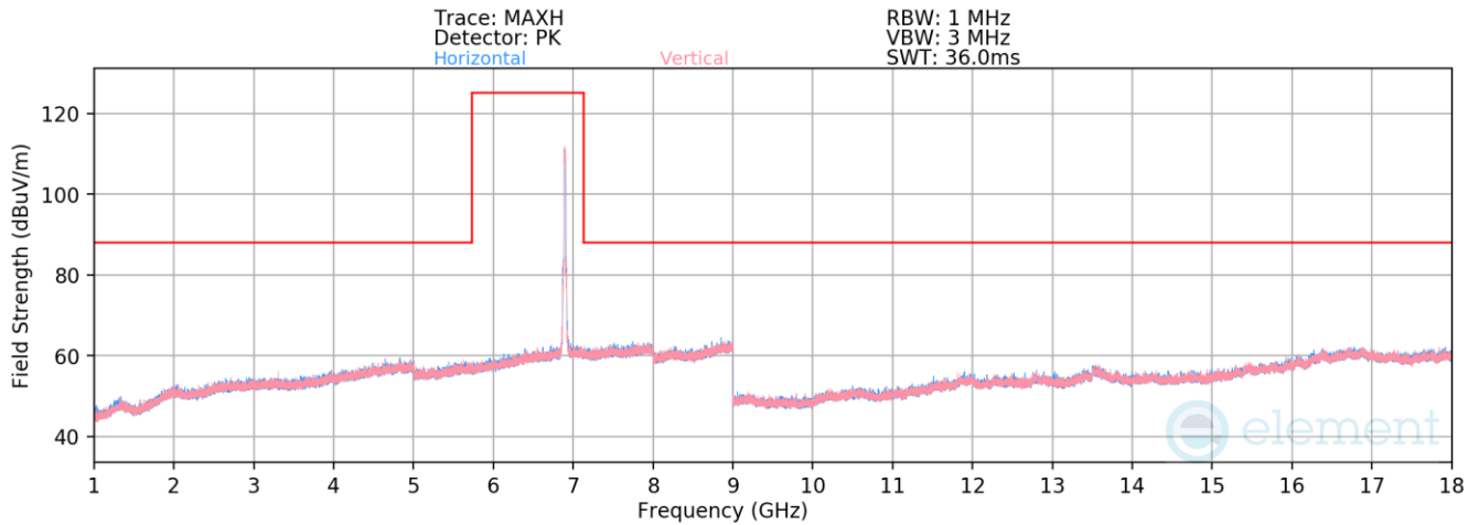
Plot 7-1354. Radiated Spurious Emissions above 1GHz Antenna 3a (802.11ax – Ch. 189)
