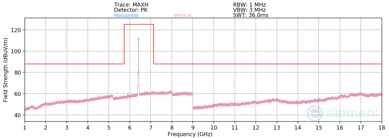
Plot 7-1359. Radiated Spurious Emissions above 1GHz Antenna 1b (802.11ax – Ch. 93)
