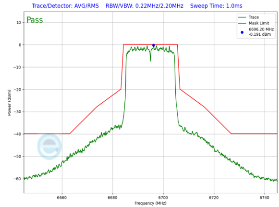
Plot 7-1290. SP In-Band Emission Plot SDM Diversity Antenna 3a (20MHz 802.11ax (UNII Band 7) – Ch. 149, MCS11)
