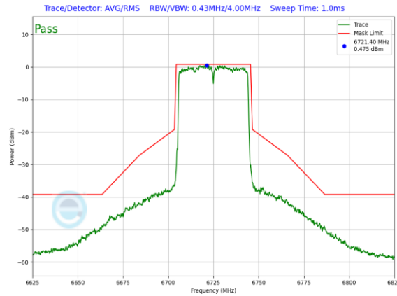
Plot 7-1275. SP In-Band Emission Plot SDM Diversity Antenna 3c (40MHz 802.11ax (UNII Band 7) – Ch. 155, MCS4)
