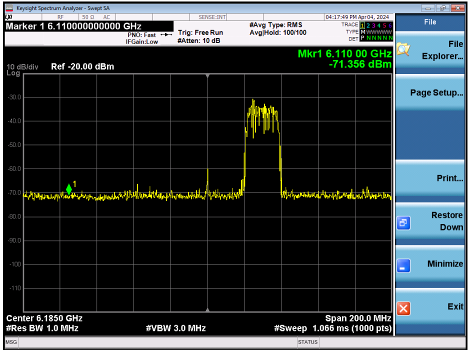
Plot 7-1330. 160MHz Bandwidth – AWGN Signal Injected at Low End – Channel 47
