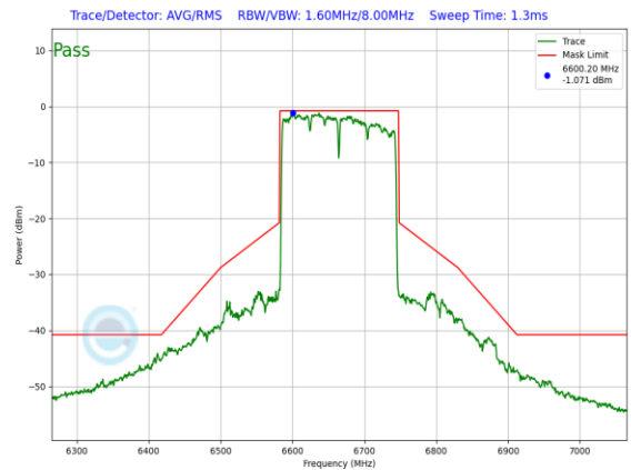
Plot 7-1296. SP In-Band Emission Plot SDM Diversity Antenna 3a (160MHz 802.11ax (UNII Band 7) – Ch. 143, MCS11)
