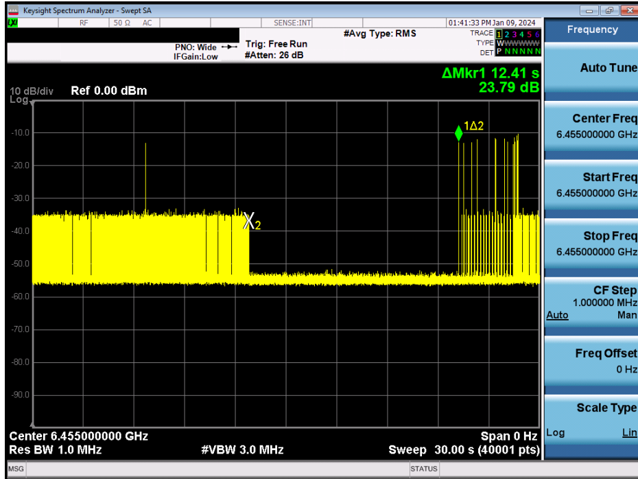
Plot 7-1317. Contention Based Protocol Timing Plot – UNII 6 – 20MHz Channel 101
