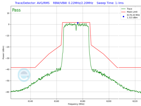
Plot 7-1281. SP In-Band Emission Plot SDM Diversity Antenna 3c (20MHz 802.11ax (UNII Band 5) – Ch. 45, MCS11)
