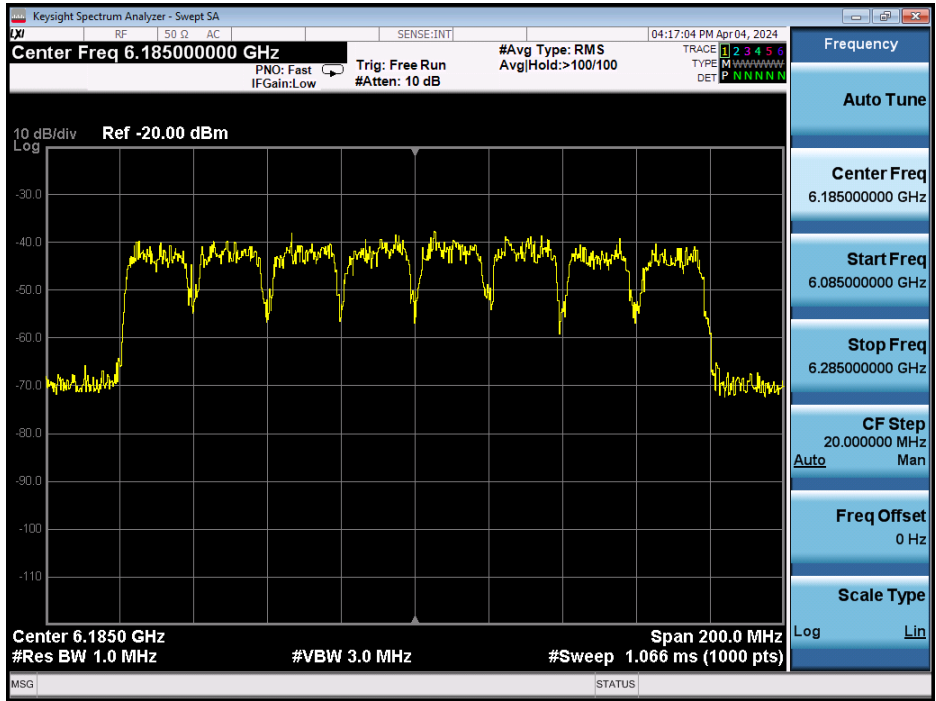
Plot 7-1329. 160MHz Bandwidth – Before AWGN Signal Injected – Channel 47
