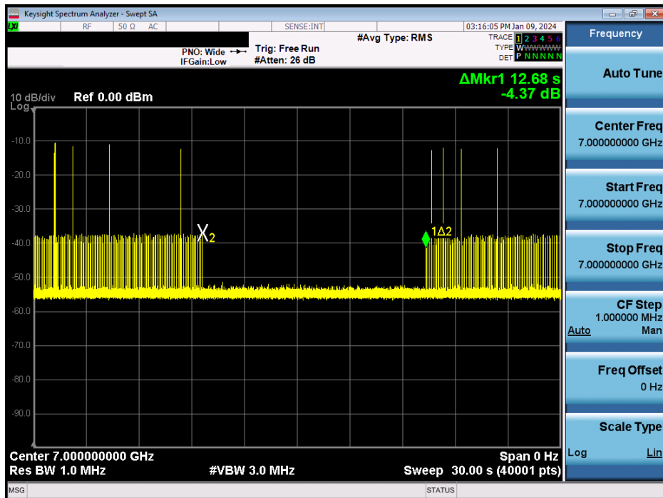
Plot 7-1328. Contention Based Protocol Timing Plot – UNII 8 – 160MHz Channel 207 – High
