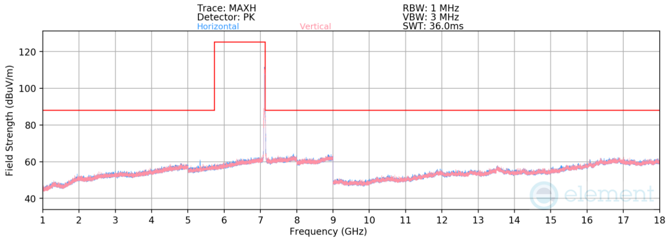
Plot 7-1356. Radiated Spurious Emissions above 1GHz Antenna 3a (802.11ax – Ch. 233)
