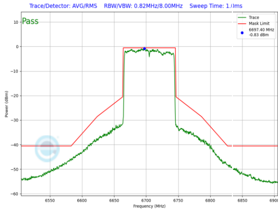
Plot 7-1278. SP In-Band Emission Plot SDM Diversity Antenna 3a (80MHz 802.11ax (UNII Band 7) – Ch. 151, MCS4)
