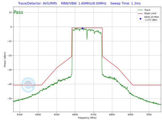
Plot 7-1280. SP In-Band Emission Plot SDM Diversity Antenna 3a (160MHz 802.11ax (UNII Band 7) – Ch. 143, MCS4)
