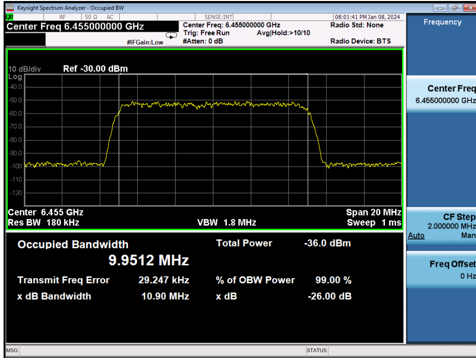
Plot 7-1301. AWGN Signal – UNII 6 – 20MHz
