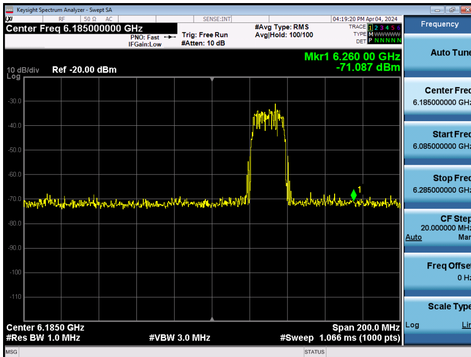
Plot 7-1332. 160MHz Bandwidth – AWGN Signal Injected at High End – Channel 47
