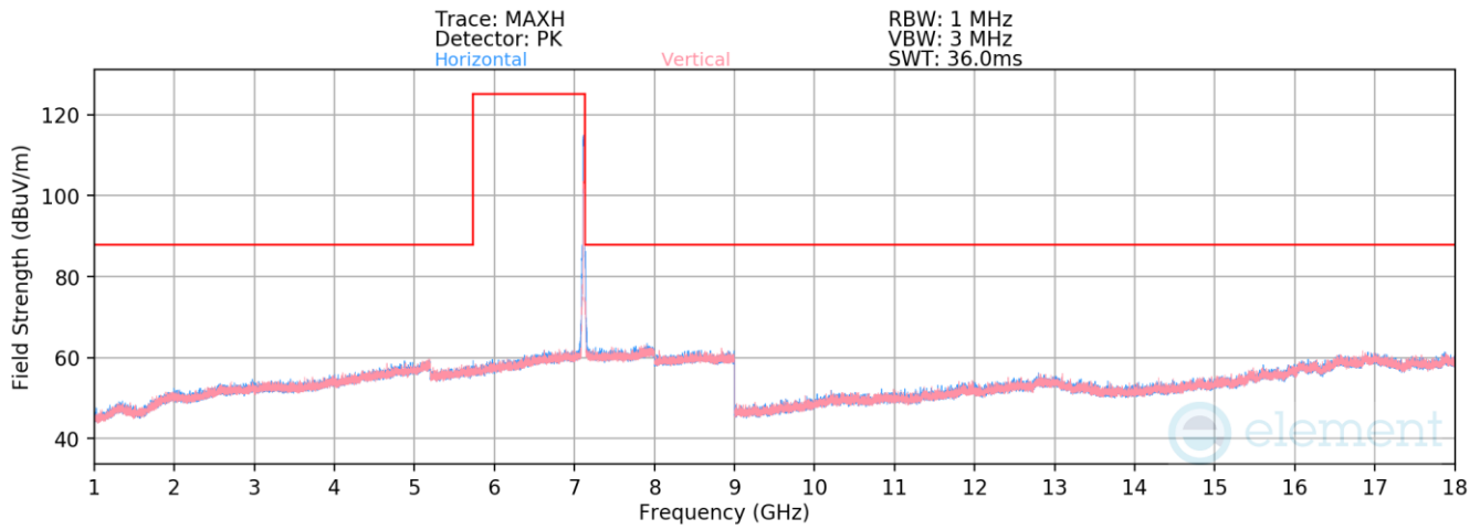
Plot 7-1344. Radiated Spurious Emissions above 1GHz Antenna 3c (802.11ax – Ch. 233)
