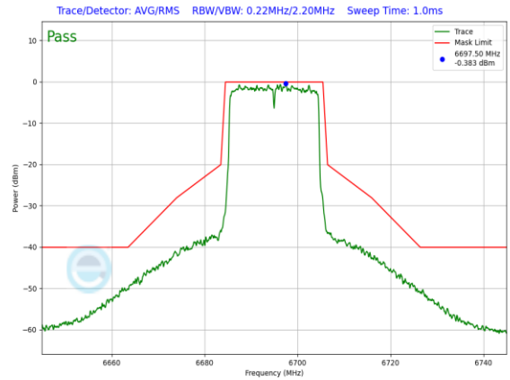
Plot 7-1274. SP In-Band Emission Plot SDM Diversity Antenna 3a (20MHz 802.11ax (UNII Band 7) – Ch. 149, MCS4)
