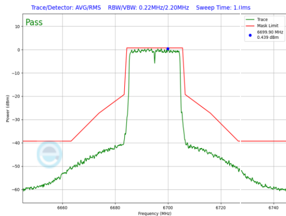
Plot 7-1273. SP In-Band Emission Plot SDM Diversity Antenna 3c (20MHz 802.11ax (UNII Band 7) – Ch. 149, MCS4)
