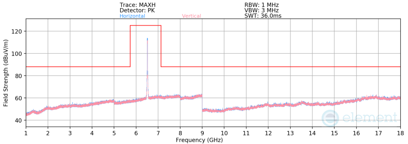
Plot 7-1350. Radiated Spurious Emissions above 1GHz Antenna 3a (802.11ax – Ch. 113)
