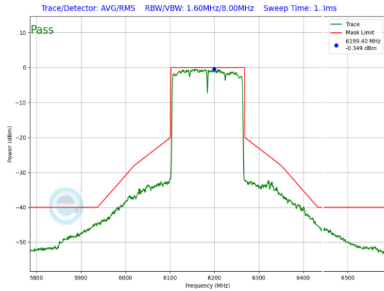
Plot 7-1272. SP In-Band Emission Plot SDM Diversity Antenna 3a (160MHz 802.11ax (UNII Band 5) – Ch. 47, MCS4)
