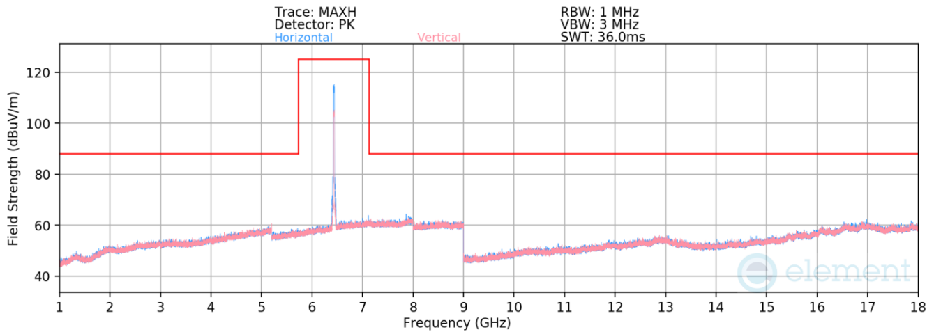
Plot 7-1336. Radiated Spurious Emissions above 1GHz Antenna 3c (802.11ax – Ch. 97)
