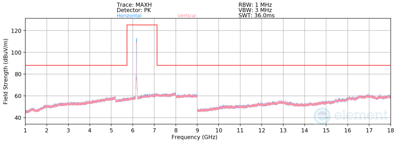
Plot 7-1358. Radiated Spurious Emissions above 1GHz Antenna 1b (802.11ax – Ch. 45, MCS0)
