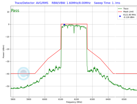
Plot 7-1287. SP In-Band Emission Plot SDM Diversity Antenna 3c (160MHz 802.11ax (UNII Band 5) – Ch. 47, MCS11)
