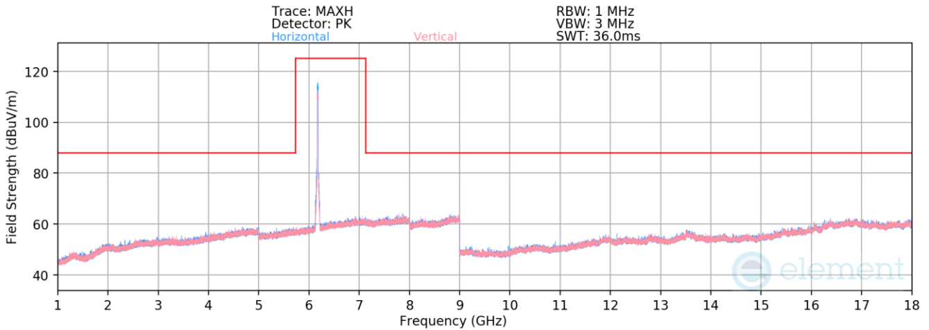
Plot 7-1346. Radiated Spurious Emissions above 1GHz Antenna 3a (802.11ax – Ch. 45, MCS0)
