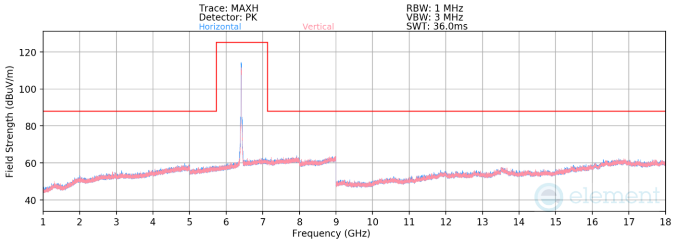
Plot 7-1347. Radiated Spurious Emissions above 1GHz Antenna 3a (802.11ax – Ch. 93)
