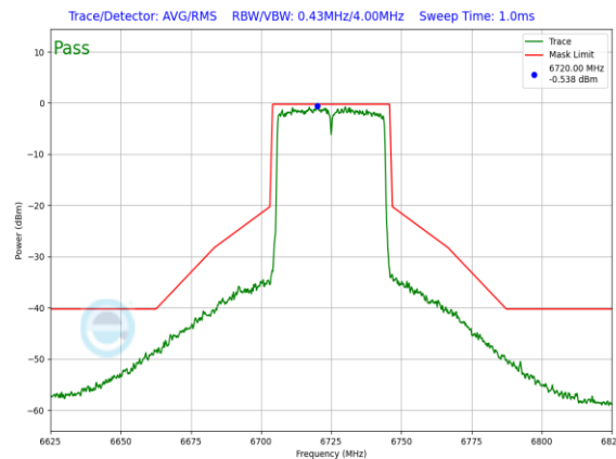
Plot 7-1276. SP In-Band Emission Plot SDM Diversity Antenna 3a (40MHz 802.11ax (UNII Band 7) – Ch. 155, MCS4)
