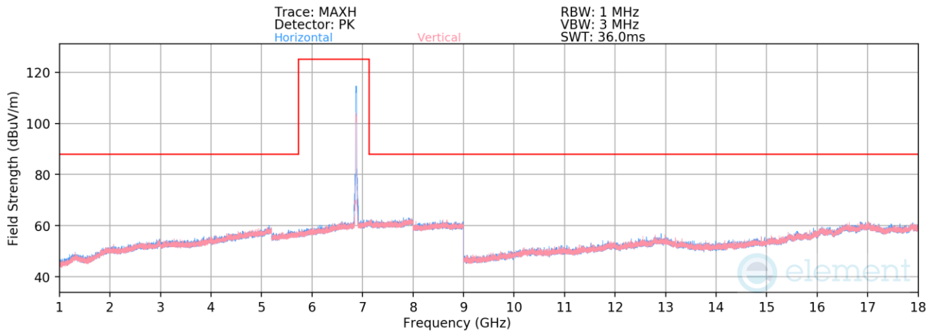
Plot 7-1341. Radiated Spurious Emissions above 1GHz Antenna 3c (802.11ax – Ch. 185)
