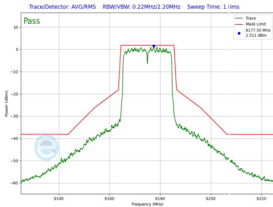
Plot 7-1282. SP In-Band Emission Plot SDM Diversity Antenna 3a (20MHz 802.11ax (UNII Band 5) – Ch. 45, MCS11)
