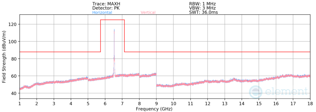
Plot 7-1351. Radiated Spurious Emissions above 1GHz Antenna 3a (802.11ax – Ch. 117)
