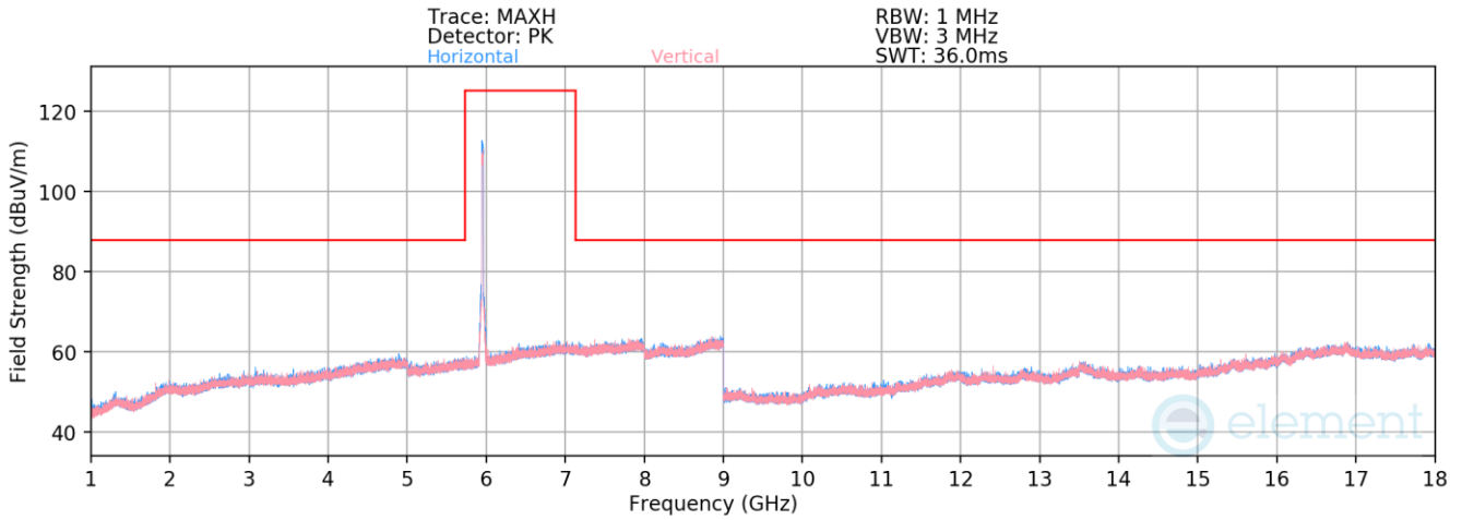
Plot 7-1357. Radiated Spurious Emissions above 1GHz Antenna 1b (802.11ax – Ch. 1)
