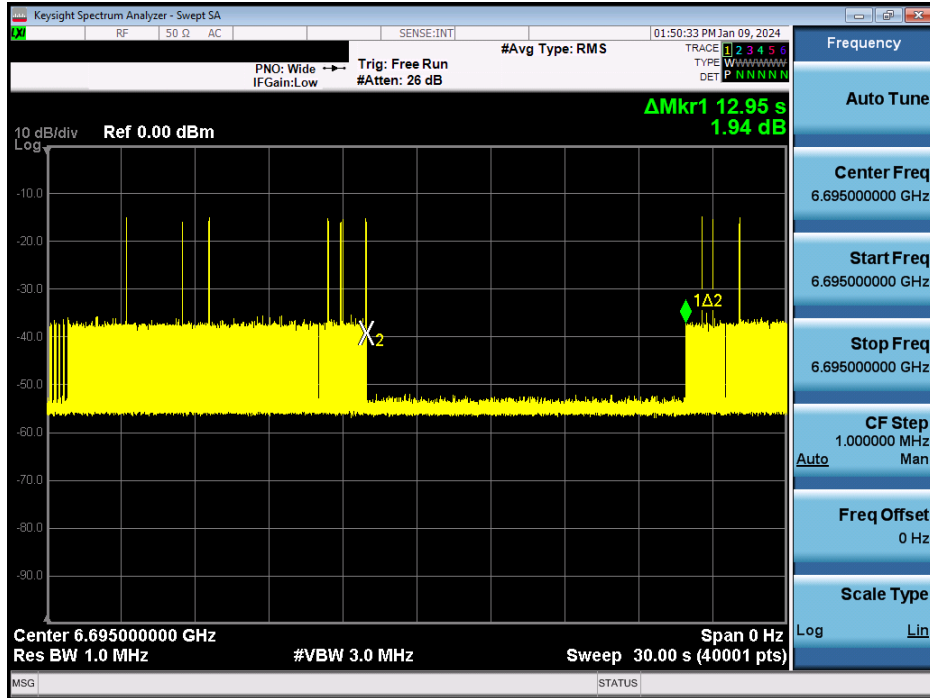
Plot 7-1321. Contention Based Protocol Timing Plot – UNII 7 – 20MHz Channel 149
