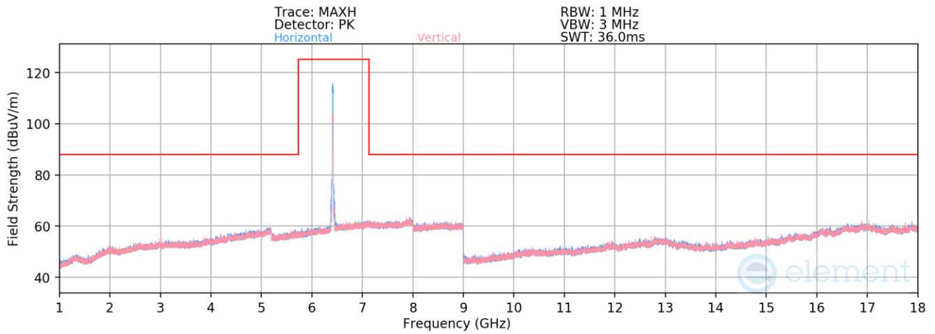
Plot 7-1335. Radiated Spurious Emissions above 1GHz Antenna 3c (802.11ax – Ch. 93)
