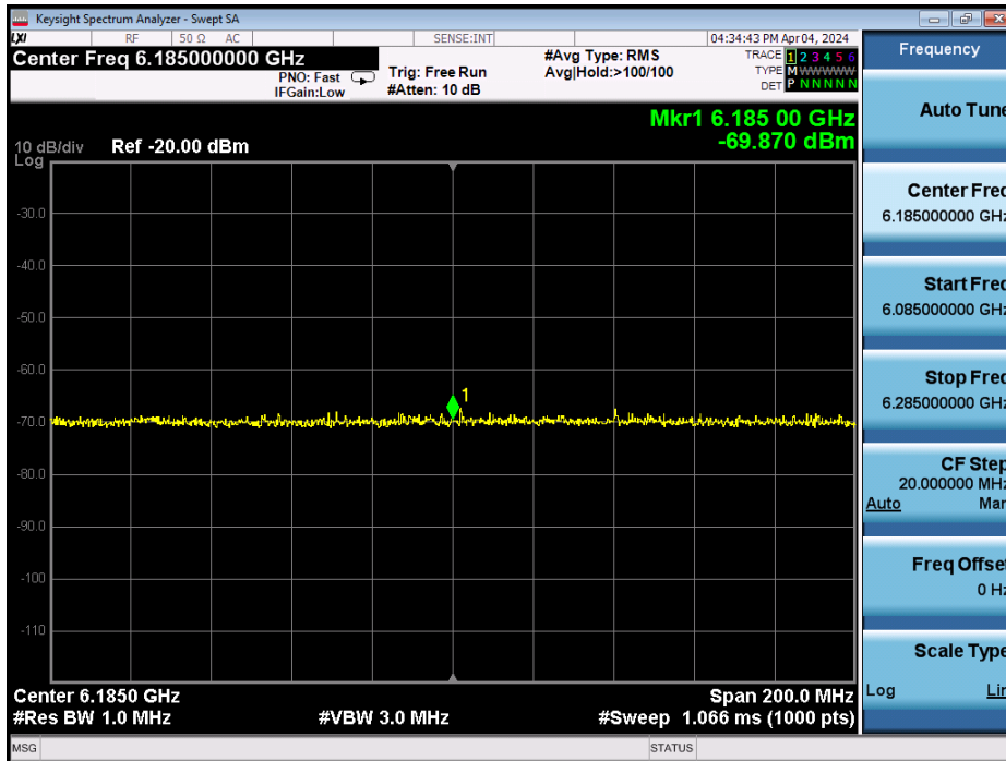
Plot 7-1331. 160MHz Bandwidth – AWGN Signal Injected at Center – Channel 47
