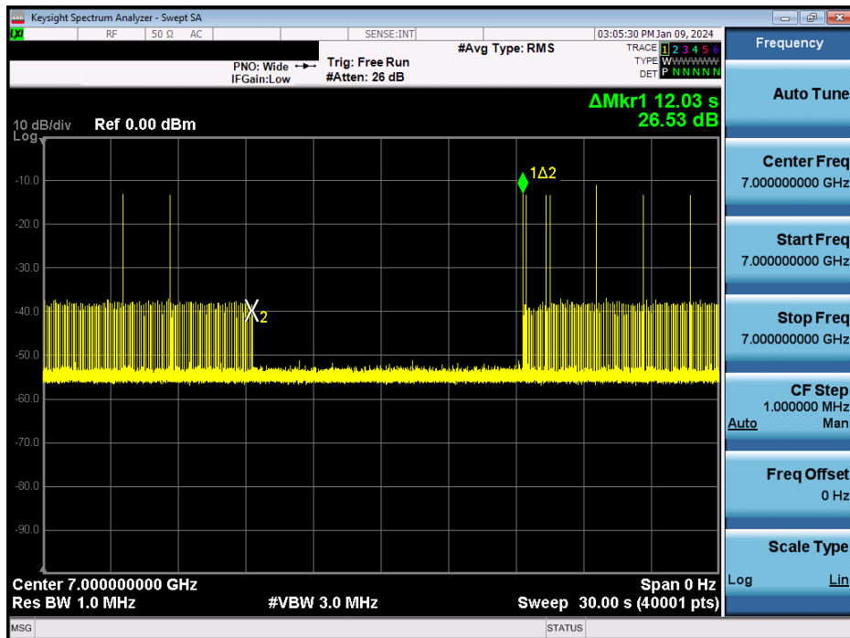
Plot 7-1326. Contention Based Protocol Timing Plot – UNII 8 – 160MHz Channel 207 – Low
