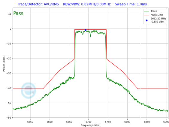
Plot 7-1294. SP In-Band Emission Plot SDM Diversity Antenna 3a (80MHz 802.11ax (UNII Band 7) – Ch. 151, MCS11)
