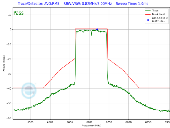
Plot 7-1277. SP In-Band Emission Plot SDM Diversity Antenna 3c (80MHz 802.11ax (UNII Band 7) – Ch. 151, MCS4)
