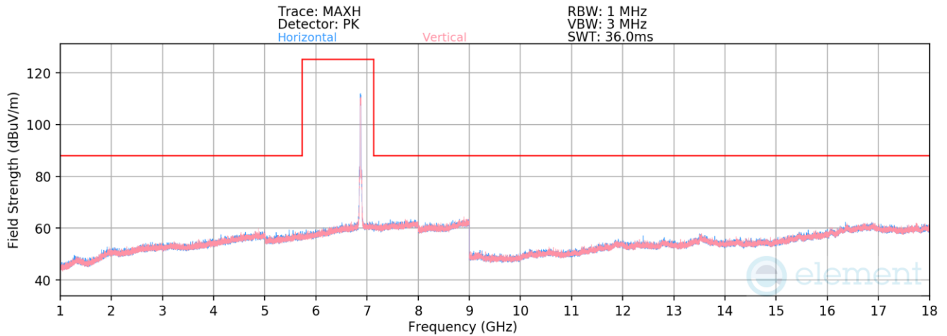
Plot 7-1353. Radiated Spurious Emissions above 1GHz Antenna 3a (802.11ax – Ch. 185)
