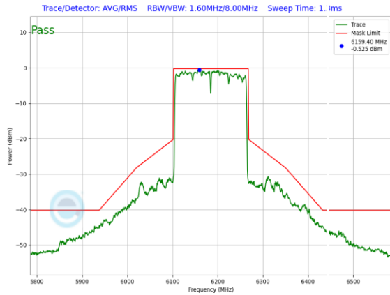
Plot 7-1288. SP In-Band Emission Plot SDM Diversity Antenna 3a (160MHz 802.11ax (UNII Band 5) – Ch. 47, MCS11)
