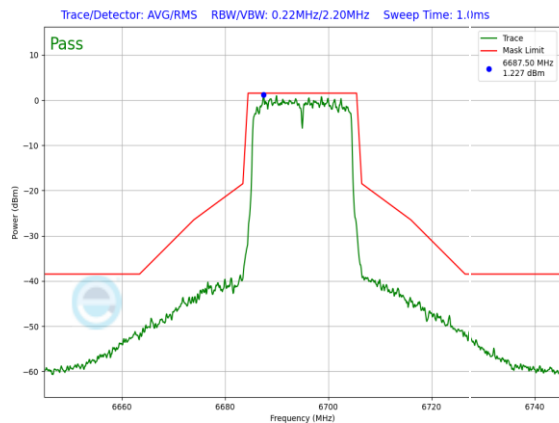
Plot 7-1289. SP In-Band Emission Plot SDM Diversity Antenna 3c (20MHz 802.11ax (UNII Band 7) – Ch. 149, MCS11)
