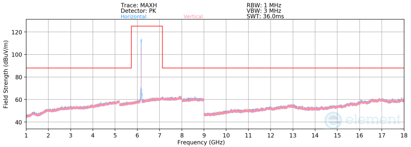
Plot 7-1334. Radiated Spurious Emissions above 1GHz Antenna 3c (802.11ax – Ch. 45, MCS0)
