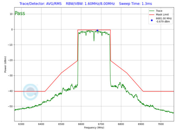
Plot 7-1295. SP In-Band Emission Plot SDM Diversity Antenna 3c (160MHz 802.11ax (UNII Band 7) – Ch. 143, MCS11)
