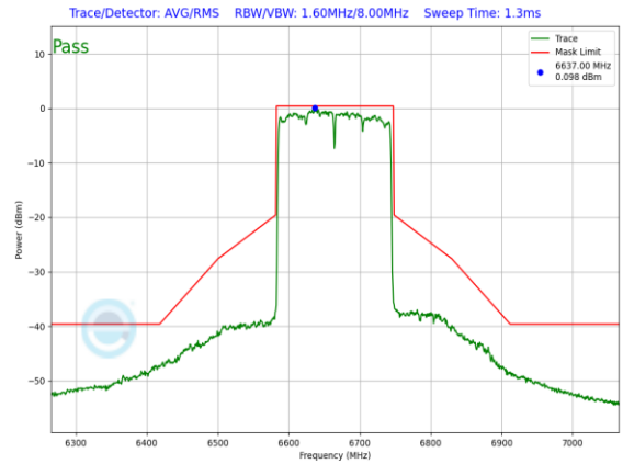
Plot 7-1279. SP In-Band Emission Plot SDM Diversity Antenna 3c (160MHz 802.11ax (UNII Band 7) – Ch. 143, MCS4)
