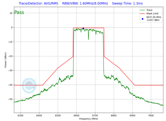
Plot 7-918. SP In-Band Emission Plot Antenna 3a (160MHz 802.11ax (UNII Band 7) – Ch. 143, MCS11)
