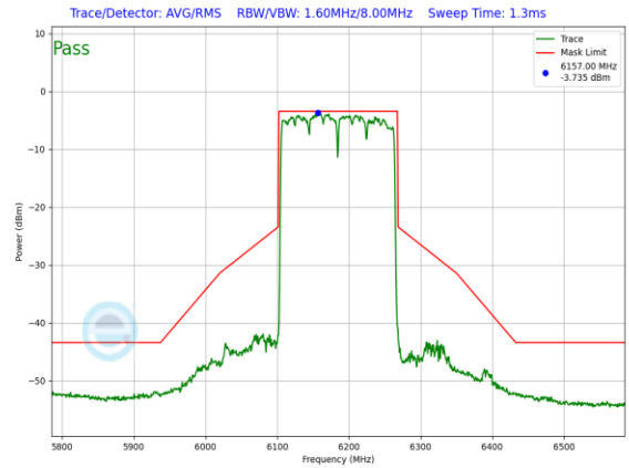
Plot 7-959. LPI In-Band Emission Plot Antenna 1b (160MHz 802.11ax (UNII Band 5) – Ch. 47, MCS11)
