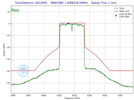
Plot 7-893. SP In-Band Emission Plot Antenna 3a (160MHz 802.11ax (UNII Band 5) – Ch. 47, MCS2)
