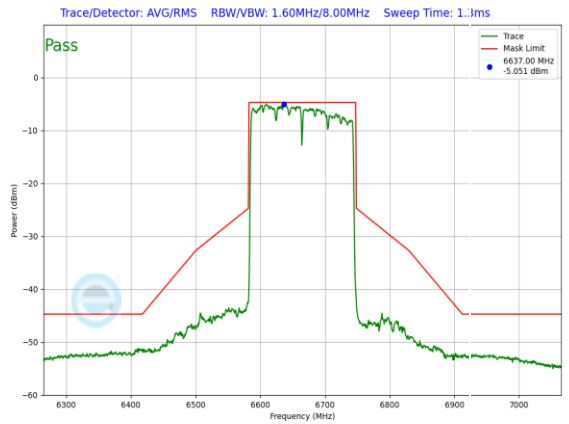
Plot 7-969. LPI In-Band Emission Plot Antenna 1b (160MHz) 802.11ax (UNII Band 7) – Ch. 143, MCS11)
