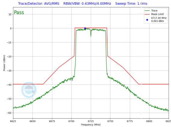
Plot 7-906. SP In-Band Emission Plot Antenna 3a (40MHz 802.11ax (UNII Band 7) – Ch. 155, MCS4)
