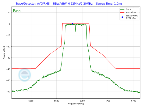
Plot 7-894. SP In-Band Emission Plot Antenna 3a (20MHz 802.11a (UNII Band 7) – Ch. 149, 12Mbps)
