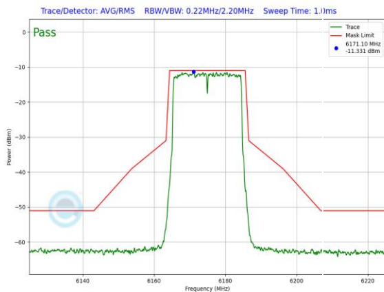
Plot 7-920. LPI In-Band Emission Plot Antenna 1b (20MHz 802.11ax (UNII Band 5) – Ch. 45, MCS2)
