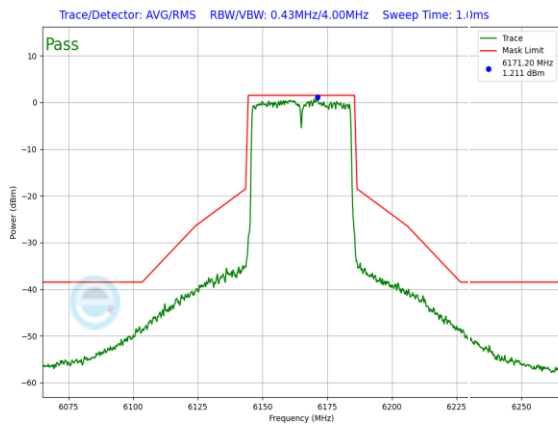
Plot 7-901. SP In-Band Emission Plot Antenna 3a (40MHz 802.11ax (UNII Band 5) – Ch. 43, MCS4)
