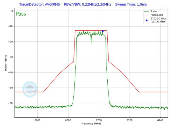
Plot 7-876. LPI In-Band Emission Plot Antenna 3a (20MHz 802.11ax (UNII Band 7) – Ch. 149, MCS11)
