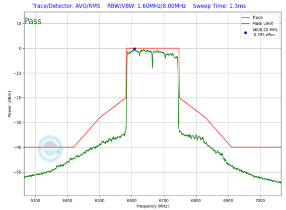
Plot 7-908. SP In-Band Emission Plot Antenna 3a (160MHz 802.11ax (UNII Band 7) – Ch. 143, MCS4)
