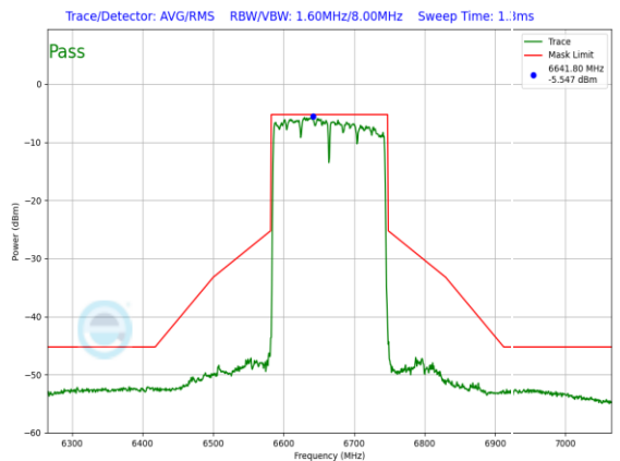
Plot 7-879. LPI In-Band Emission Plot Antenna 3a (160MHz 802.11ax (UNII Band 7) – Ch. 143, MCS11)
