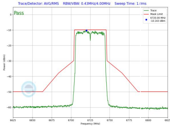
Plot 7-877. LPI In-Band Emission Plot Antenna 3a (40MHz 802.11ax (UNII Band 7) – Ch. 155, MCS11)
