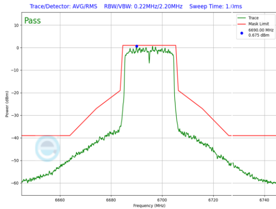
Plot 7-915. SP In-Band Emission Plot Antenna 3a (20MHz 802.11ax (UNII Band 7) – Ch. 149, MCS11)
