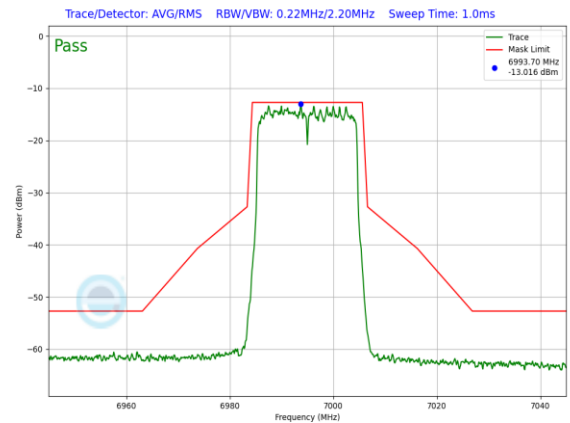
Plot 7-881. LPI In-Band Emission Plot Antenna 3a (20MHz 802.11ax (UNII Band 8) – Ch. 209, MCS11)
