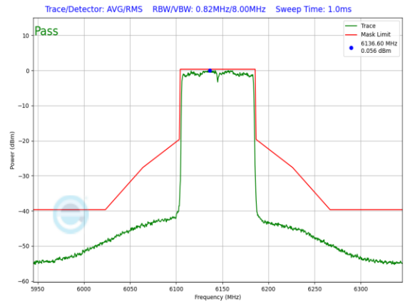
Plot 7-892. SP In-Band Emission Plot Antenna 3a (80MHz 802.11ax (UNII Band 5) – Ch. 39, MCS2)
