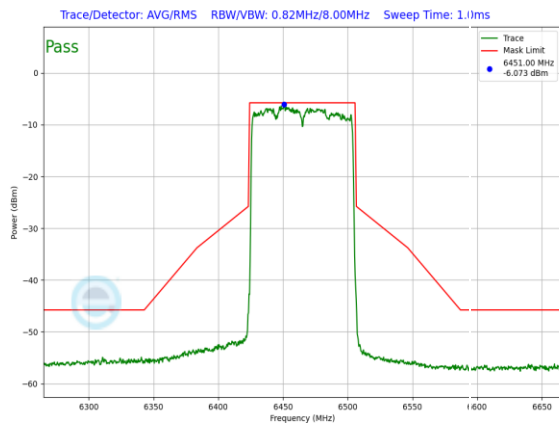
Plot 7-873. LPI In-Band Emission Plot Antenna 3a (80MHz 802.11ax (UNII Band 6) – Ch. 103, MCS11)
