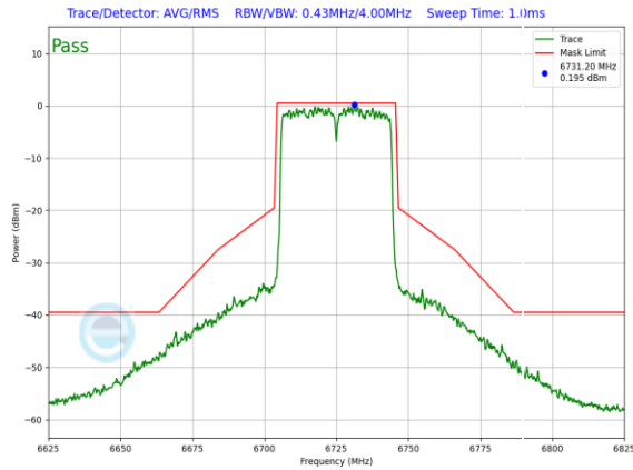
Plot 7-916. SP In-Band Emission Plot Antenna 3a (40MHz 802.11ax (UNII Band 7) – Ch. 155, MCS11)
