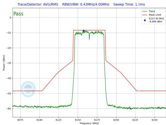
Plot 7-957. LPI In-Band Emission Plot Antenna 1b (40MHz 802.11ax (UNII Band 5) – Ch. 43, MCS11)
