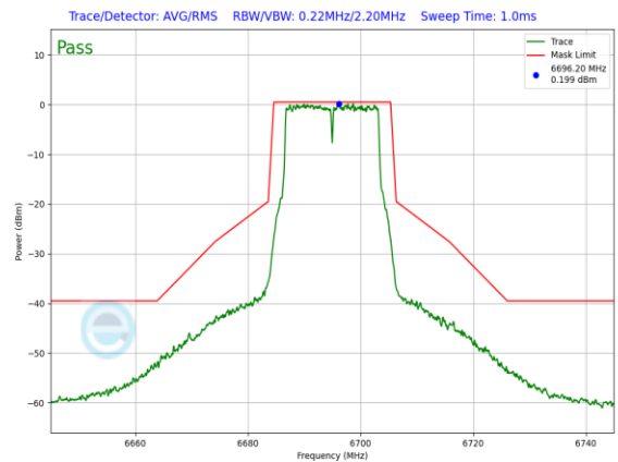
Plot 7-904. SP In-Band Emission Plot Antenna 3a (20MHz 802.11a (UNII Band 7) – Ch. 149, 24Mbps)
