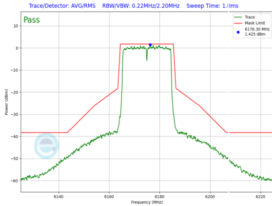
Plot 7-900. SP In-Band Emission Plot Antenna 3a (20MHz 802.11ax (UNII Band 5) – Ch. 45, MCS4)
