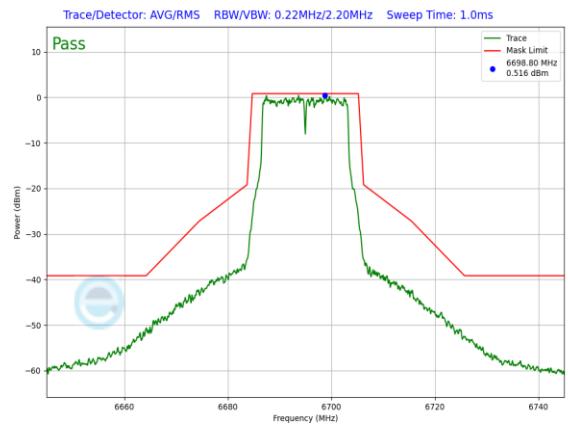
Plot 7-914. SP In-Band Emission Plot Antenna 3a (20MHz 802.11a (UNII Band 7) – Ch. 149, 54Mbps)
