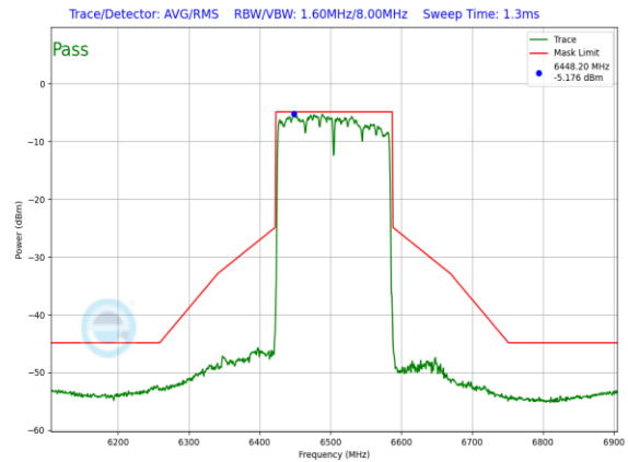
Plot 7-964. LPI In-Band Emission Plot Antenna 1b (160MHz) 802.11ax (UNII Band 6) – Ch. 111, MCS11)
