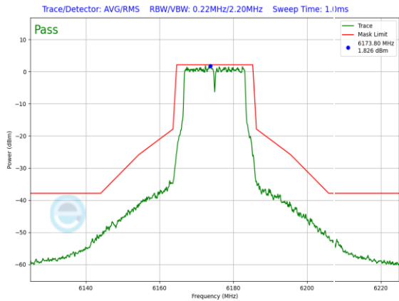
Plot 7-909. SP In-Band Emission Plot Antenna 3a (20MHz 802.11a (UNII Band 5) – Ch. 45, 54Mbps)
