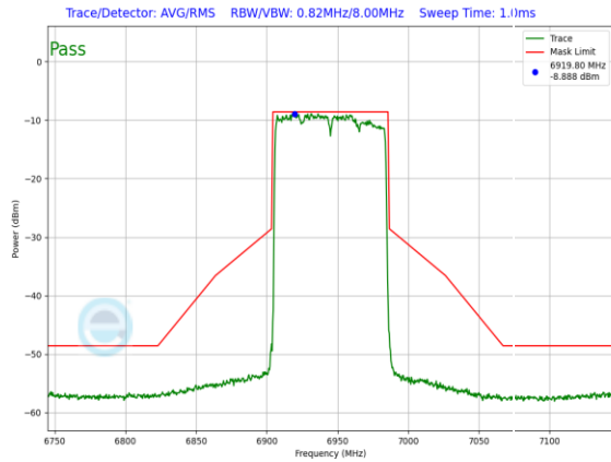
Plot 7-973. LPI In-Band Emission Plot Antenna 1b (80MHz) 802.11ax (UNII Band 8) – Ch. 199, MCS11)
