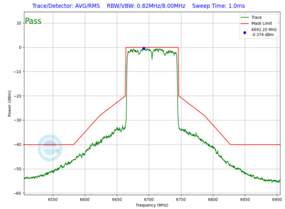
Plot 7-917. SP In-Band Emission Plot Antenna 3a (80MHz 802.11ax (UNII Band 7) – Ch. 151, MCS11)
