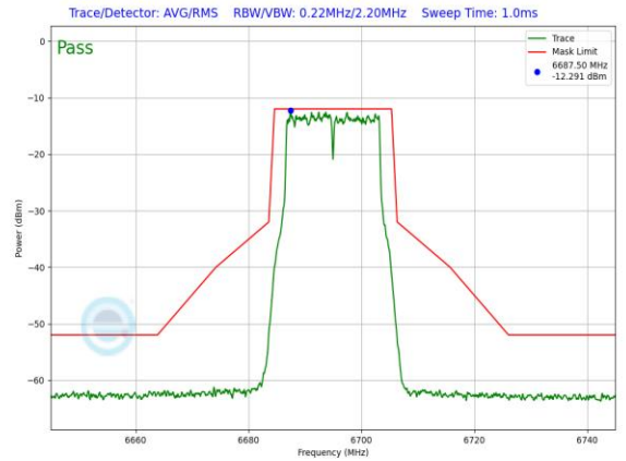
Plot 7-965. LPI In-Band Emission Plot Antenna 1b (20MHz) 802.11a (UNII Band 7) – Ch. 149, 54Mbps)
