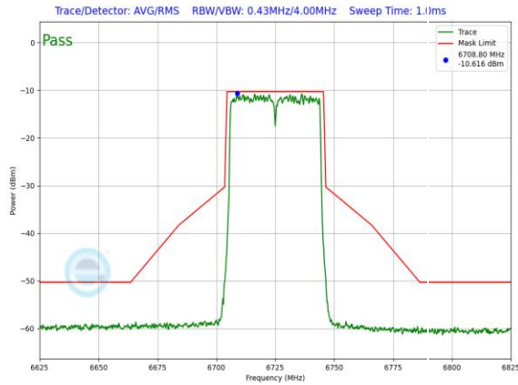
Plot 7-967. LPI In-Band Emission Plot Antenna 1b (40MHz) 802.11ax (UNII Band 7) – Ch. 155, MCS11)
