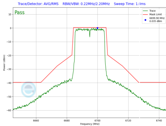
Plot 7-905. SP In-Band Emission Plot Antenna 3a (20MHz 802.11ax (UNII Band 7) – Ch. 149, MCS4)
