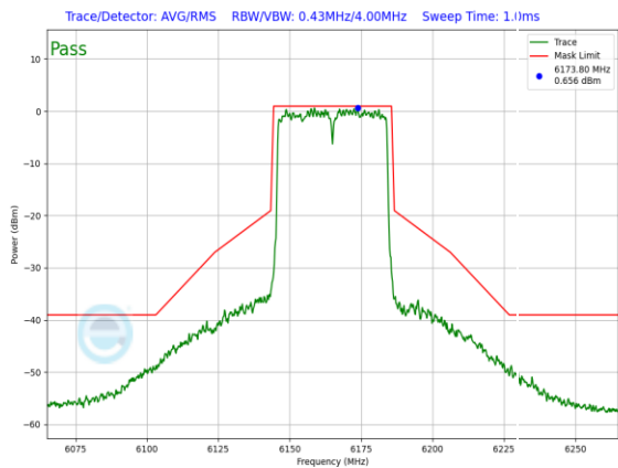
Plot 7-911. SP In-Band Emission Plot Antenna 3a (40MHz 802.11ax (UNII Band 5) – Ch. 43, MCS11)
