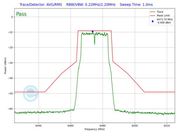
Plot 7-960. LPI In-Band Emission Plot Antenna 1b (20MHz 802.11a (UNII Band 6) – Ch. 105, 54Mbps)
