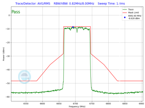
Plot 7-878. LPI In-Band Emission Plot Antenna 3a (80MHz 802.11ax (UNII Band 7) – Ch. 151, MCS11)
