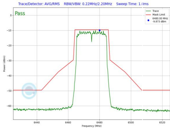
Plot 7-961. LPI In-Band Emission Plot Antenna 1b (20MHz) 802.11ax (UNII Band 6) – Ch. 105, MCS11)
