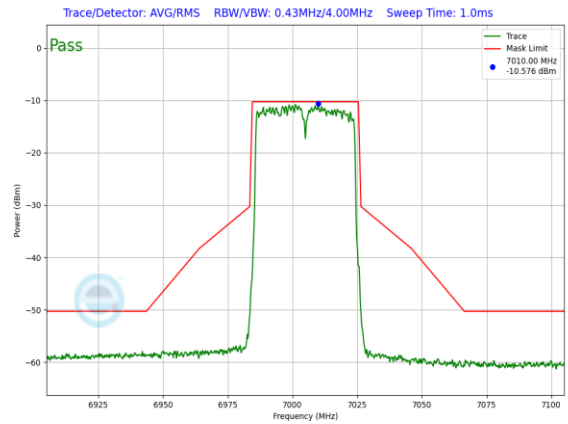
Plot 7-972. LPI In-Band Emission Plot Antenna 1b (40MHz) 802.11ax (UNII Band 8) – Ch. 211, MCS11)
