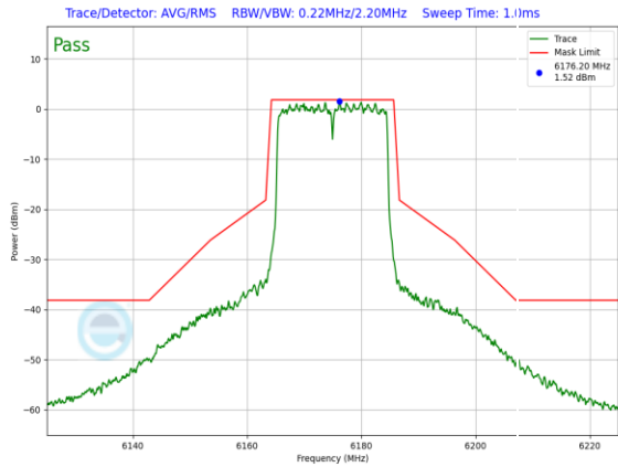
Plot 7-910. SP In-Band Emission Plot Antenna 3a (20MHz 802.11ax (UNII Band 5) – Ch. 45, MCS11)
