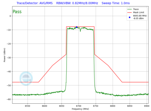
Plot 7-932. LPI In-Band Emission Plot Antenna 1b (80MHz 802.11a (UNII Band 7) – Ch. 151, MCS2)
