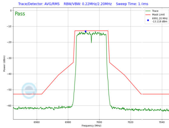
Plot 7-885. LPI In-Band Emission Plot Antenna 3a (20MHz) 802.11ax (UNII Band 8) – Ch. 209, MCS11)
