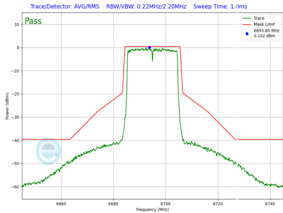
Plot 7-895. SP In-Band Emission Plot Antenna 3a (20MHz 802.11ax (UNII Band 7) – Ch. 149, MCS2)
