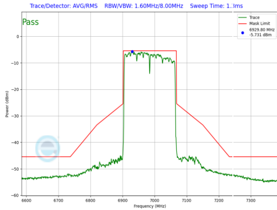
Plot 7-974. LPI In-Band Emission Plot Antenna 1b (160MHz) 802.11ax (UNII Band 8) – Ch. 207, MCS11)
