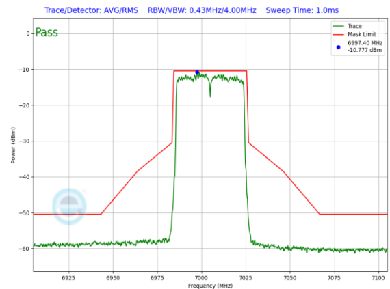
Plot 7-882. LPI In-Band Emission Plot Antenna 3a (40MHz 802.11ax (UNII Band 8) – Ch. 211, MCS11)
