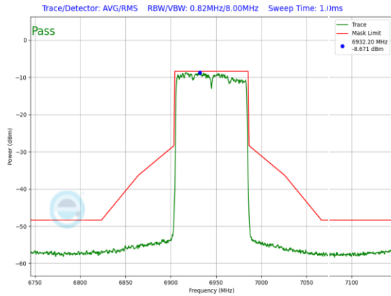
Plot 7-883. LPI In-Band Emission Plot Antenna 3a (80MHz) 802.11ax (UNII Band 8) – Ch. 199, MCS11)
