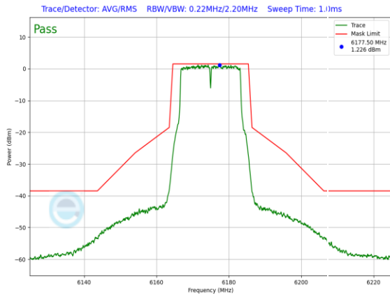
Plot 7-889. SP In-Band Emission Plot Antenna 3a (20MHz 802.11a (UNII Band 5) – Ch. 45, 12Mbps)
