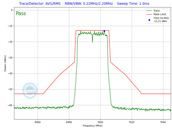
Plot 7-971. LPI In-Band Emission Plot Antenna 1b (20MHz) 802.11ax (UNII Band 8) – Ch. 209, MCS11)
