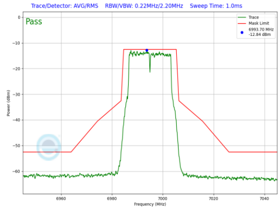
Plot 7-970. LPI In-Band Emission Plot Antenna 1b (20MHz) 802.11a (UNII Band 8) – Ch. 209, 54Mbps)
