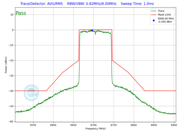
Plot 7-897. SP In-Band Emission Plot Antenna 3a (80MHz 802.11ax (UNII Band 7) – Ch. 151, MCS2)
