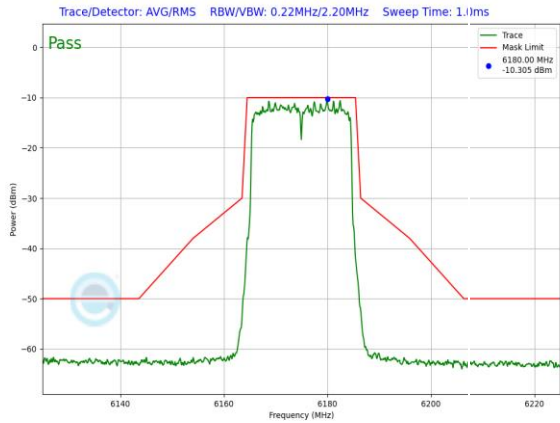
Plot 7-956. LPI In-Band Emission Plot Antenna 1b (20MHz 802.11ax (UNII Band 5) – Ch. 45, MCS11)
