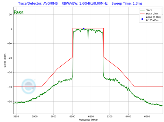
Plot 7-903. SP In-Band Emission Plot Antenna 3a (160MHz 802.11ax (UNII Band 5) – Ch. 47, MCS4)
