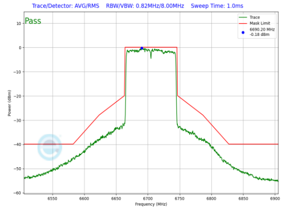
Plot 7-907. SP In-Band Emission Plot Antenna 3a (80MHz 802.11ax (UNII Band 7) – Ch. 151, MCS4)
