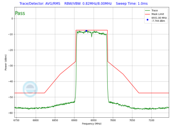
Plot 7-887. LPI In-Band Emission Plot Antenna 3a (80MHz) 802.11ax (UNII Band 8) – Ch. 199, MCS11)
