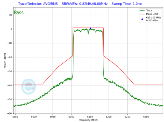
Plot 7-912. SP In-Band Emission Plot Antenna 3a (80MHz 802.11ax (UNII Band 5) – Ch. 39, MCS11)
