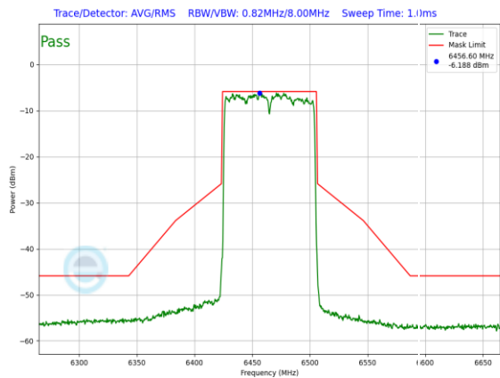
Plot 7-963. LPI In-Band Emission Plot Antenna 1b (80MHz) 802.11ax (UNII Band 6) – Ch. 103, MCS11)
