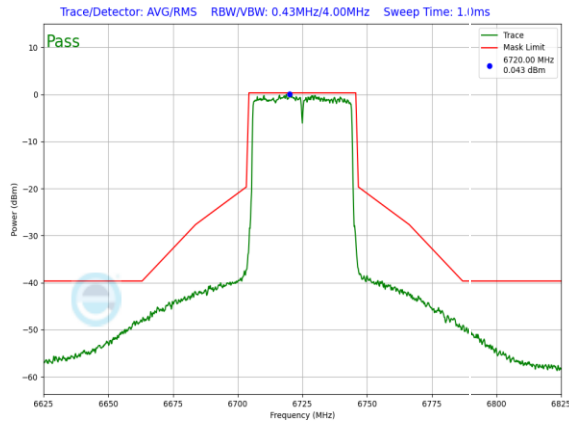
Plot 7-896. SP In-Band Emission Plot Antenna 3a (40MHz 802.11ax (UNII Band 7) – Ch. 155, MCS2)
