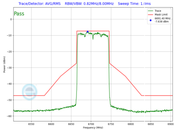
Plot 7-968. LPI In-Band Emission Plot Antenna 1b (80MHz) 802.11ax (UNII Band 7) – Ch. 151, MCS11)
