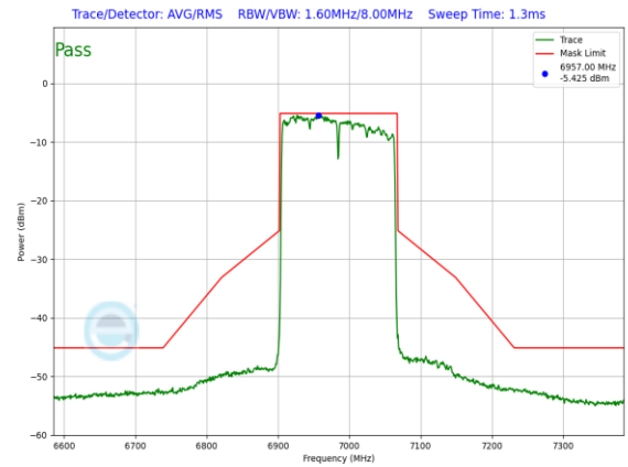
Plot 7-888. LPI In-Band Emission Plot Antenna 3a (160MHz) 802.11ax (UNII Band 8) – Ch. 207, MCS11)
