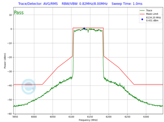
Plot 7-902. SP In-Band Emission Plot Antenna 3a (80MHz 802.11ax (UNII Band 5) – Ch. 39, MCS4)
