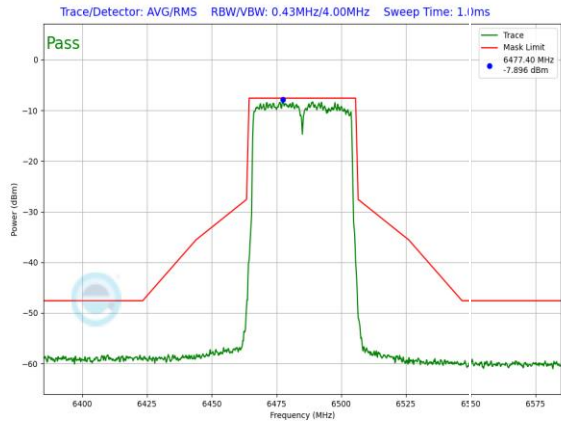
Plot 7-962. LPI In-Band Emission Plot Antenna 1b (40MHz) 802.11ax (UNII Band 6) – Ch. 107, MCS11)
