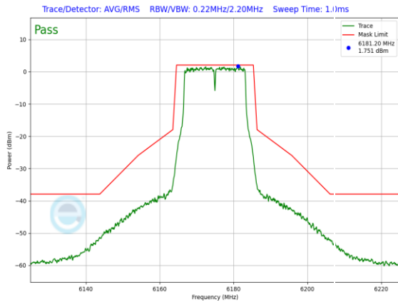
Plot 7-899. SP In-Band Emission Plot Antenna 3a (20MHz 802.11a (UNII Band 5) – Ch. 45, 24Mbps)
