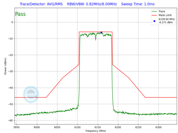
Plot 7-958. LPI In-Band Emission Plot Antenna 1b (80MHz 802.11ax (UNII Band 5) – Ch. 39, MCS11)
