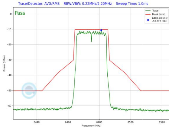
Plot 7-871. LPI In-Band Emission Plot Antenna 3a (20MHz 802.11ax (UNII Band 6) – Ch. 105, MCS11)
