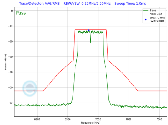
Plot 7-880. LPI In-Band Emission Plot Antenna 3a (20MHz 802.11a (UNII Band 8) – Ch. 209, 54Mbps)
