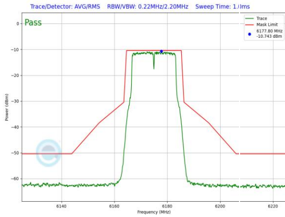
Plot 7-919. LPI In-Band Emission Plot Antenna 1b (20MHz 802.11a (UNII Band 5) – Ch. 45, 12Mbps)
