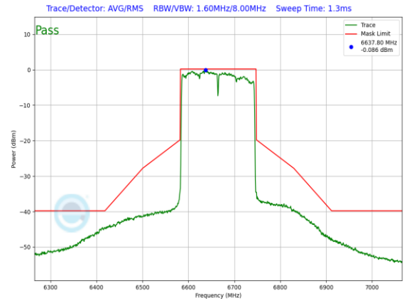
Plot 7-898. SP In-Band Emission Plot Antenna 3a (160MHz 802.11ax (UNII Band 7) – Ch. 143, MCS2)
