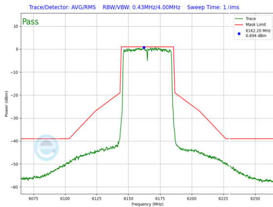
Plot 7-891. SP In-Band Emission Plot Antenna 3a (40MHz 802.11ax (UNII Band 5) – Ch. 43, MCS2)
