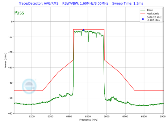
Plot 7-874. LPI In-Band Emission Plot Antenna 3a (160MHz 802.11ax (UNII Band 6) – Ch. 111, MCS11)
