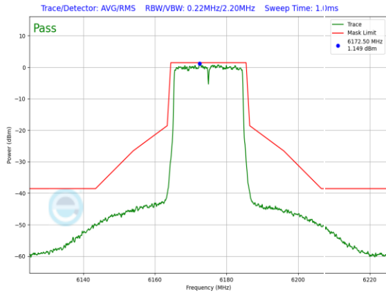
Plot 7-890. SP In-Band Emission Plot Antenna 3a (20MHz 802.11ax (UNII Band 5) – Ch. 45, MCS2)
