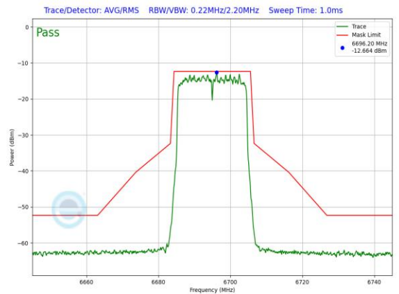
Plot 7-966. LPI In-Band Emission Plot Antenna 1b (20MHz) 802.11ax (UNII Band 7) – Ch. 149, MCS11)
