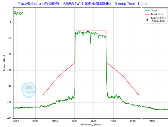
Plot 7-884. LPI In-Band Emission Plot Antenna 3a (160MHz) 802.11ax (UNII Band 8) – Ch. 207, MCS11)
