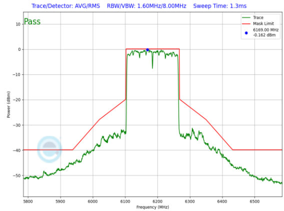
Plot 7-913. SP In-Band Emission Plot Antenna 3a (160MHz 802.11ax (UNII Band 5) – Ch. 47, MCS11)
