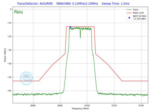
Plot 7-875. LPI In-Band Emission Plot Antenna 3a (20MHz 802.11a (UNII Band 7) – Ch. 149, 54Mbps)
