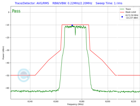
Plot 7-955. LPI In-Band Emission Plot Antenna 1b (20MHz 802.11a (UNII Band 5) – Ch. 45, 54Mbps)
