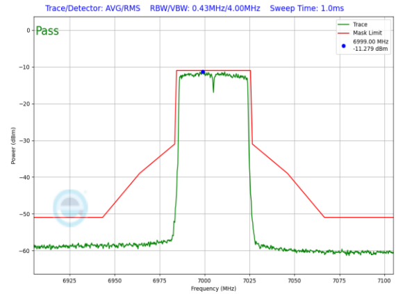
Plot 7-886. LPI In-Band Emission Plot Antenna 3a (40MHz) 802.11ax (UNII Band 8) – Ch. 211, MCS11)
