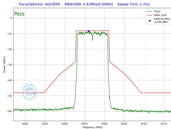
Plot 7-872. LPI In-Band Emission Plot Antenna 3a (40MHz 802.11ax (UNII Band 6) – Ch. 107, MCS11)
