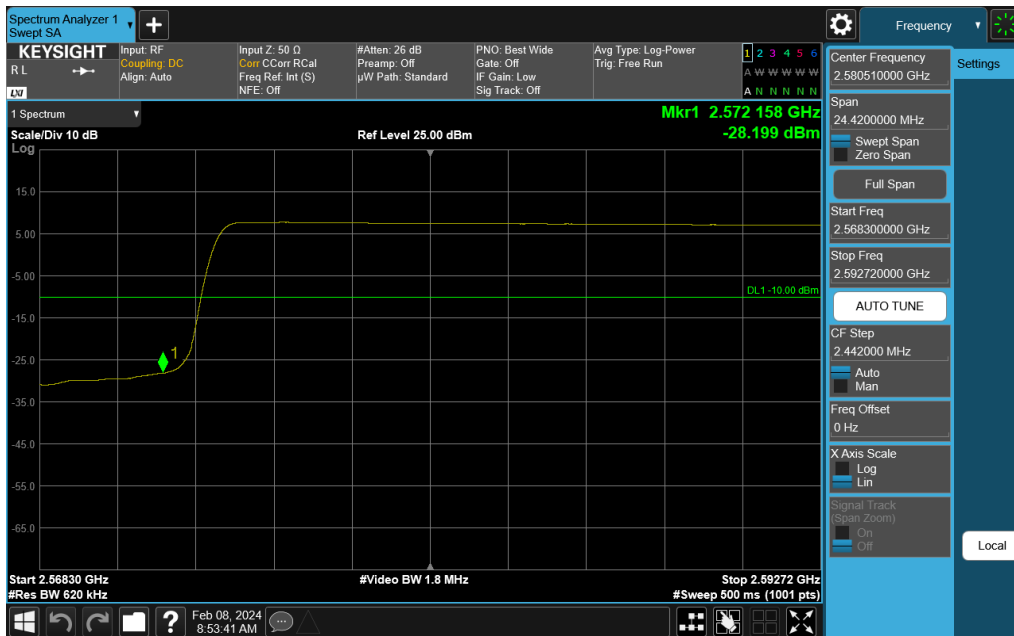
Plot 7-750. Middle Band Edge Plot (NR Band n41 - 40MHz DFT-s-OFDM QPSK – Full RB)
