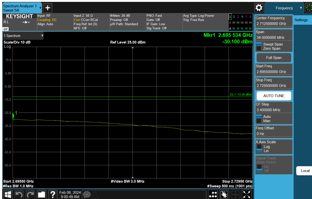
Plot 7-764. Upper Band Edge Plot (NR Band n41 - 40MHz DFT-s-OFDM QPSK – Full RB)
