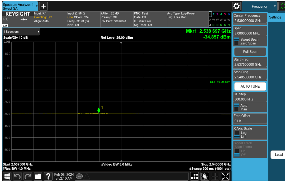
Plot 7-747. Lower Band Edge Plot (NR Band n41 - 40MHz DFT-s-OFDM QPSK – Full RB)
