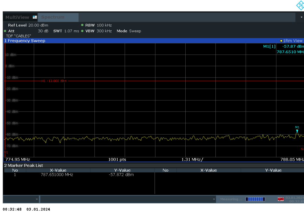
Plot 7-68. Conducted Spurious Plot (LTE Band 14 - 5MHz QPSK - RB Size 1, RB Offset 0 - High Channel)
