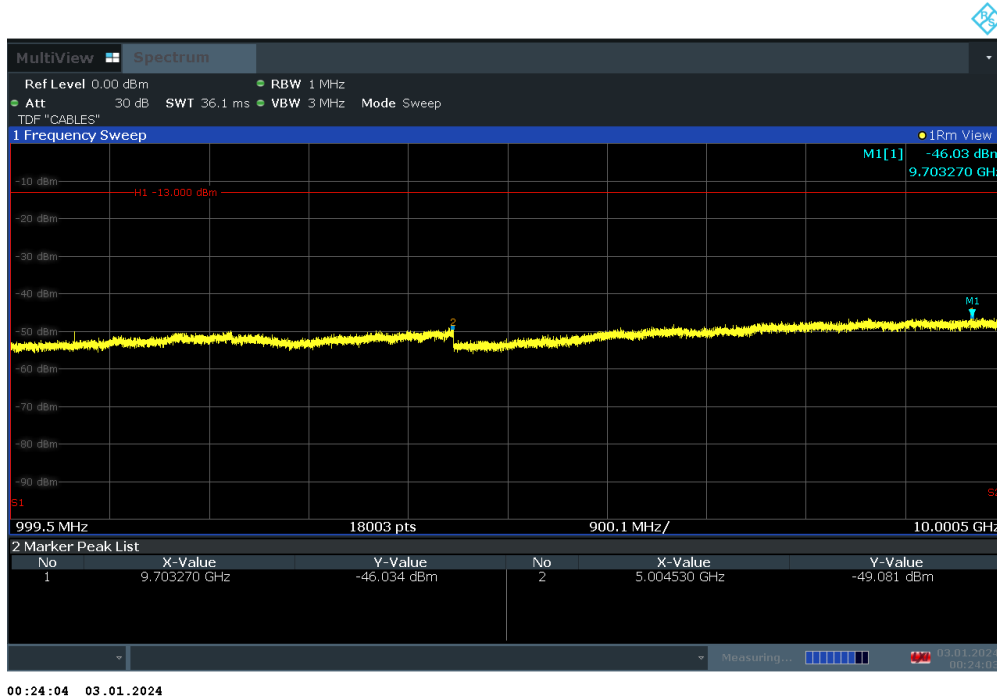
Plot 7-59. Conducted Spurious Plot (LTE Band 14 - 5MHz QPSK - RB Size 1, RB Offset 0 - Low Channel)
