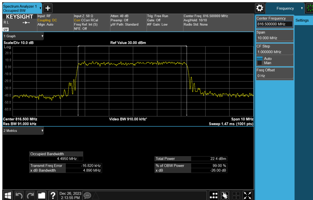
Plot 7-38. Occupied Bandwidth Plot (NR Band 26 - 5MHz DFT-s-OFDM 64-QAM - Full RB)
