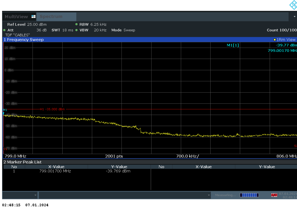
Plot 7-101. Upper Emission Mask Plot (LTE Band 14 - 5MHz QPSK – RB Size 25)
