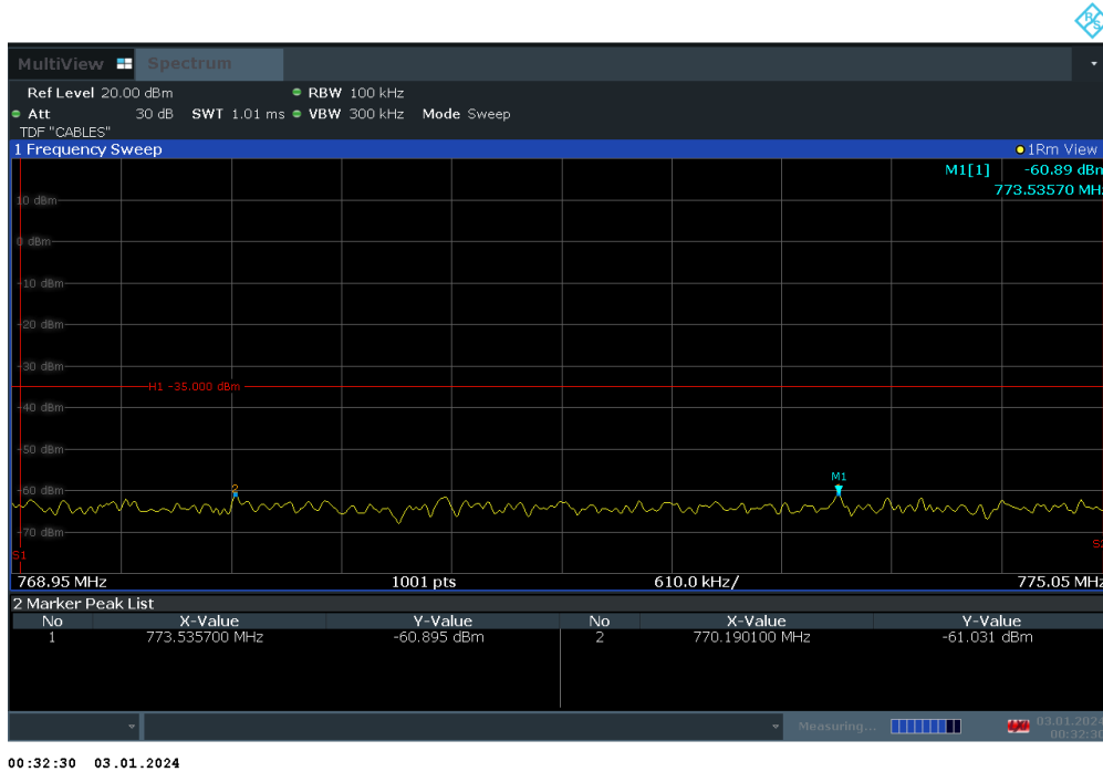
Plot 7-67. Conducted Spurious Plot (LTE Band 14 - 5MHz QPSK - RB Size 1, RB Offset 0 - High Channel)
