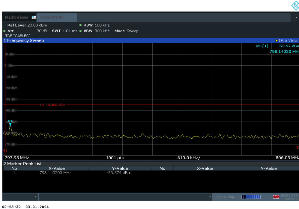
Plot 7-57. Conducted Spurious Plot (LTE Band 14 - 5MHz QPSK - RB Size 1, RB Offset 0 - Low Channel)
