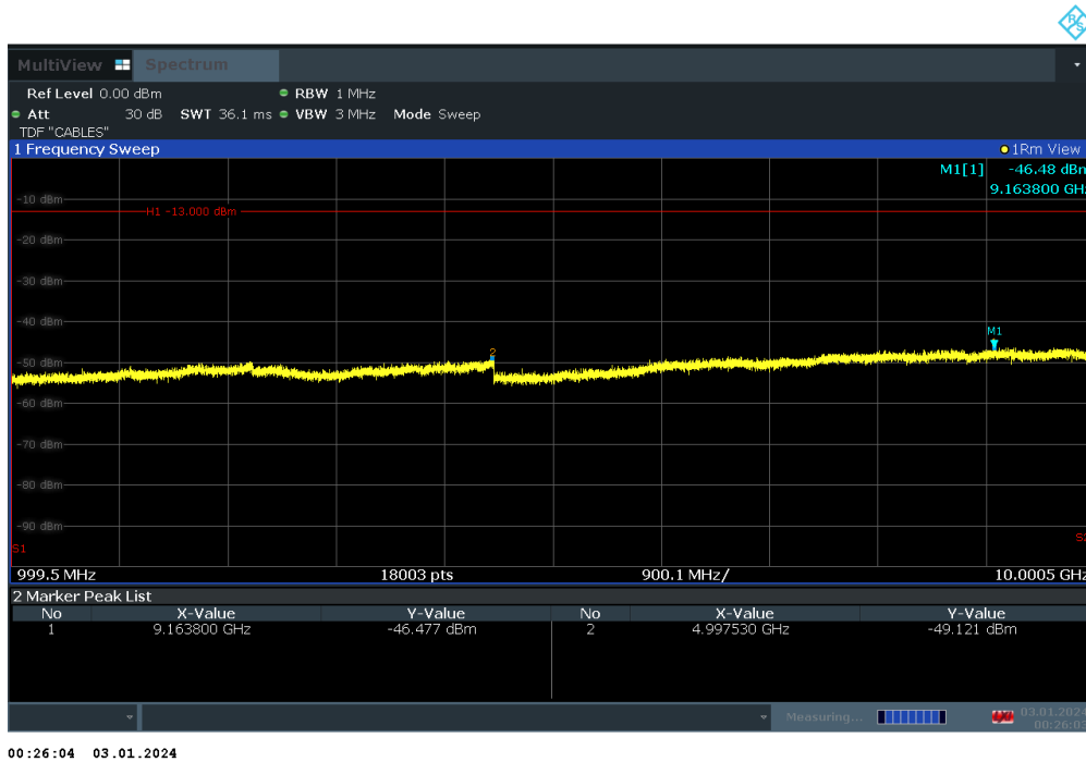
Plot 7-65. Conducted Spurious Plot (LTE Band 14 - 10MHz QPSK - RB Size 1, RB Offset 0 - Mid Channel)
