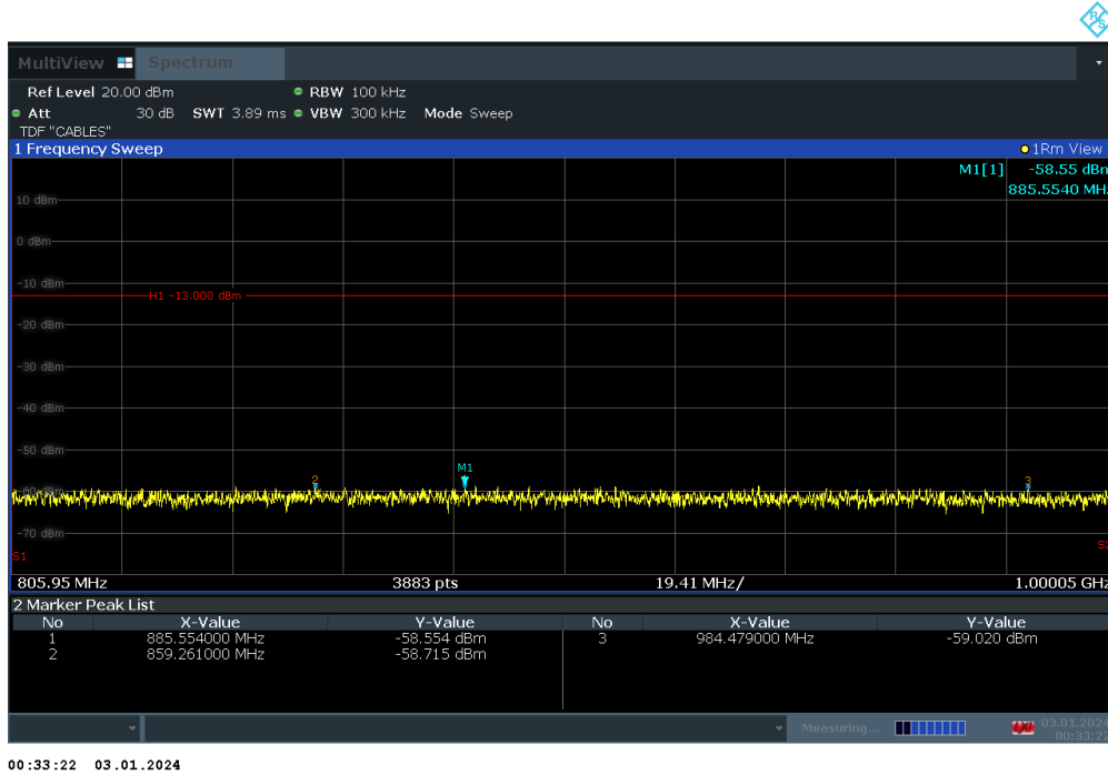
Plot 7-70. Conducted Spurious Plot (LTE Band 14 - 5MHz QPSK - RB Size 1, RB Offset 0 - High Channel)
