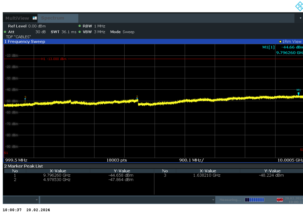
Plot 7-50. Conducted Spurious Plot (LTE Band 26 - 10MHz QPSK - RB Size 1, RB Offset 0 - Mid Channel)
