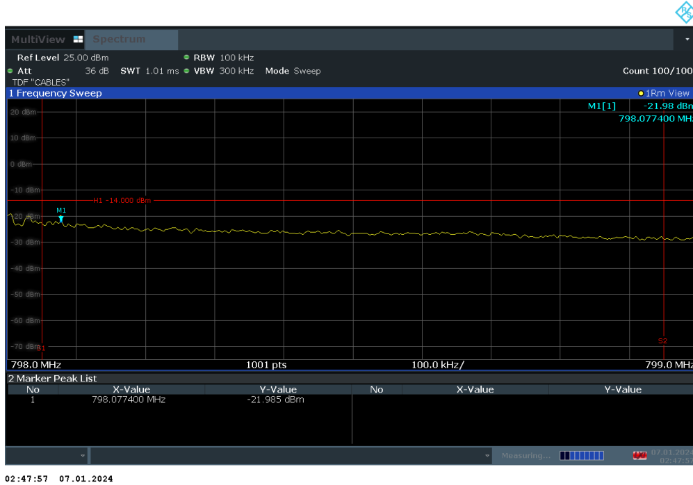
Plot 7-100. Upper Band Edge Plot (LTE Band 14 - 5MHz QPSK – RB Size 25)
