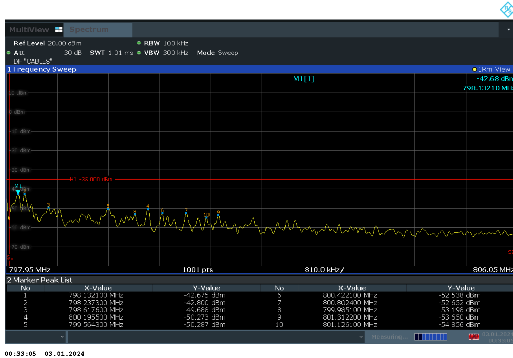
Plot 7-69. Conducted Spurious Plot (LTE Band 14 - 5MHz QPSK - RB Size 1, RB Offset 0 - High Channel)
