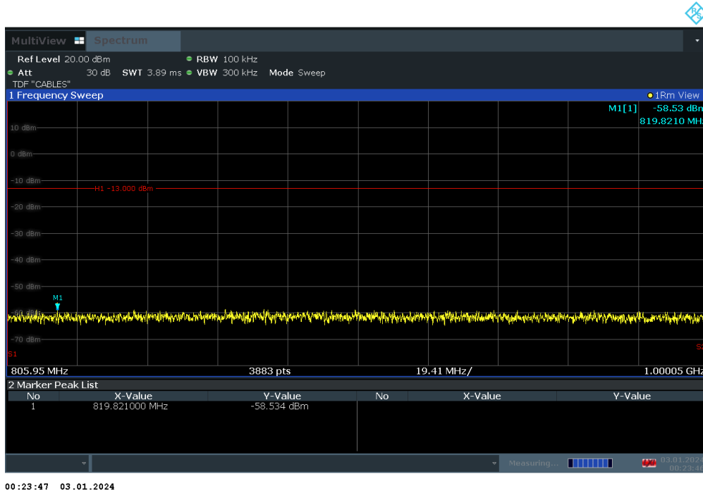
Plot 7-58. Conducted Spurious Plot (LTE Band 14 - 5MHz QPSK - RB Size 1, RB Offset 0 - Low Channel)
