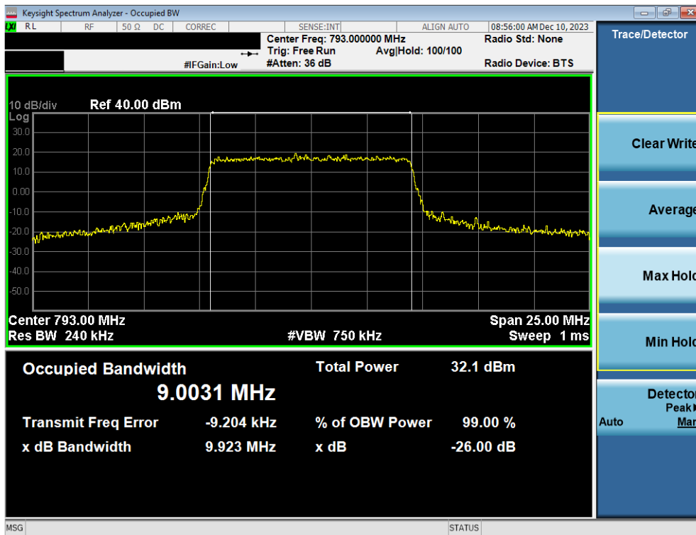
Plot 7-22. Occupied Bandwidth Plot (LTE Band 14 - 10MHz 16-QAM - Full RB)
