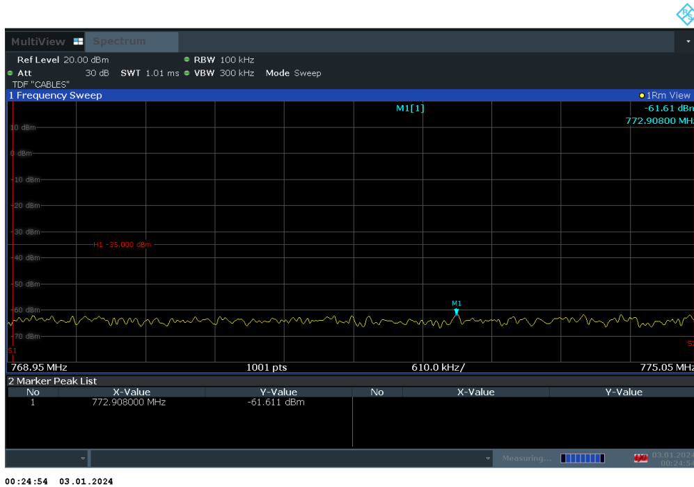
Plot 7-61. Conducted Spurious Plot (LTE Band 14 - 10MHz QPSK - RB Size 1, RB Offset 0 - Mid Channel)
