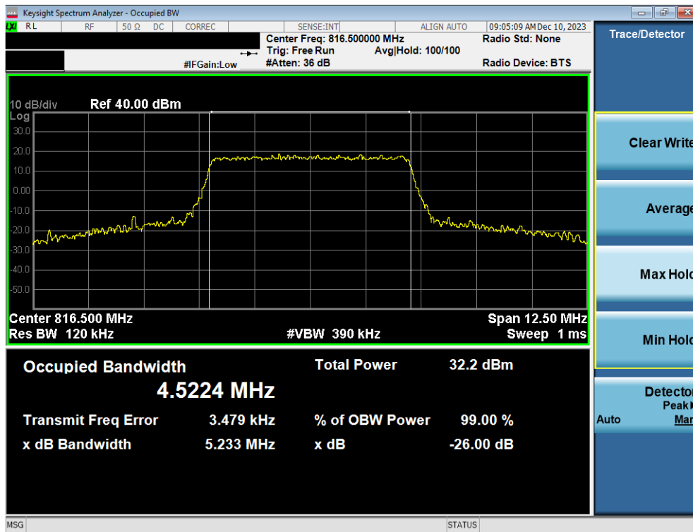
Plot 7-10. Occupied Bandwidth Plot (LTE Band 26 - 5MHz 16-QAM - Full RB)
