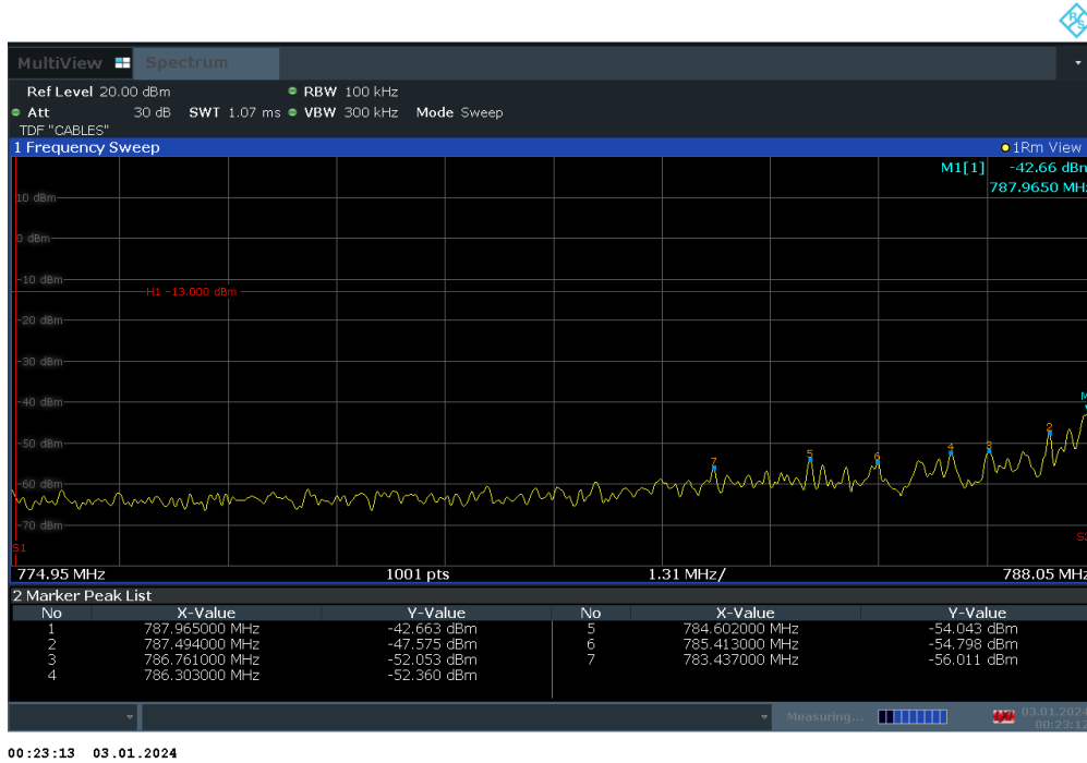
Plot 7-56. Conducted Spurious Plot (LTE Band 14 - 5MHz QPSK - RB Size 1, RB Offset 0 - Low Channel)
