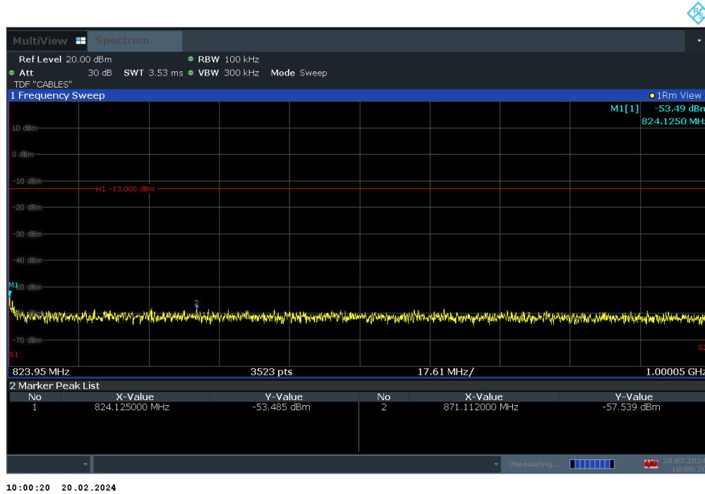
Plot 7-49. Conducted Spurious Plot (LTE Band 26 - 10MHz QPSK - RB Size 1, RB Offset 0 - Mid Channel)
