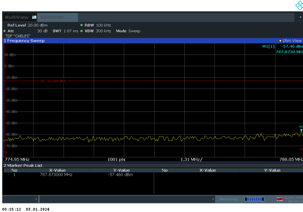
Plot 7-62. Conducted Spurious Plot (LTE Band 14 - 10MHz QPSK - RB Size 1, RB Offset 0 - Mid Channel)
