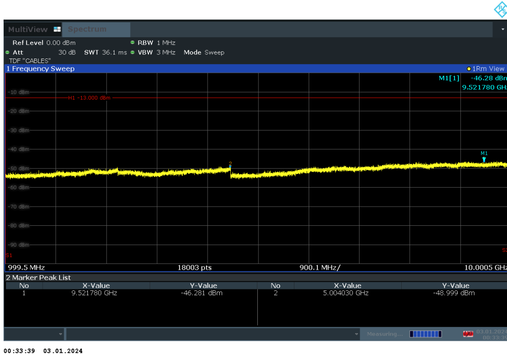
Plot 7-71. Conducted Spurious Plot (LTE Band 14 - 5MHz QPSK - RB Size 1, RB Offset 0 - High Channel)
