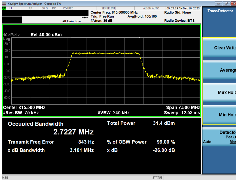
Plot 7-7. Occupied Bandwidth Plot (LTE Band 26 - 3MHz 64-QAM - Full RB)
