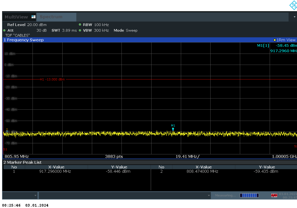
Plot 7-64. Conducted Spurious Plot (LTE Band 14 - 10MHz QPSK - RB Size 1, RB Offset 0 - Mid Channel)
