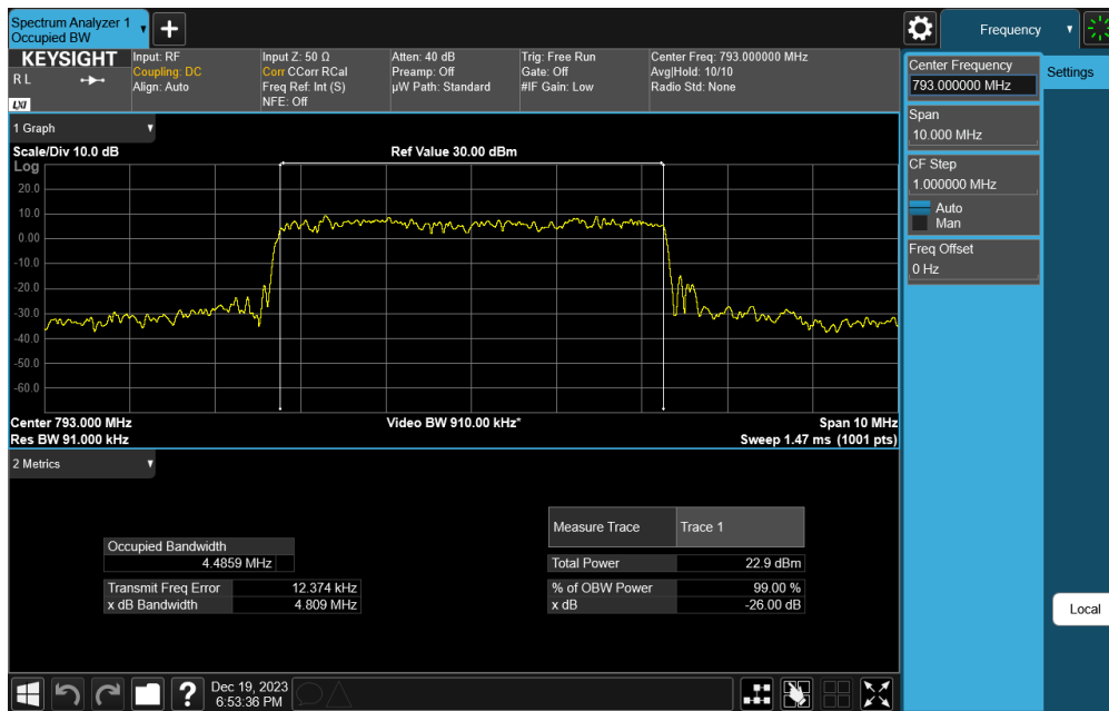
Plot 7-28. Occupied Bandwidth Plot (NR Band 14 - 5MHz DFT-s-OFDM 64-QAM - Full RB)
