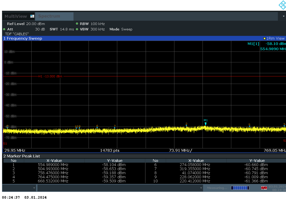
Plot 7-60. Conducted Spurious Plot (LTE Band 14 - 10MHz QPSK - RB Size 1, RB Offset 0 - Mid Channel)
