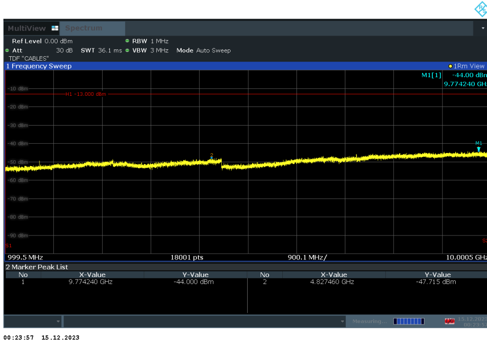
Plot 7-47. Conducted Spurious Plot (LTE Band 26 - 5MHz QPSK - RB Size 1, RB Offset 0 - Low Channel)
