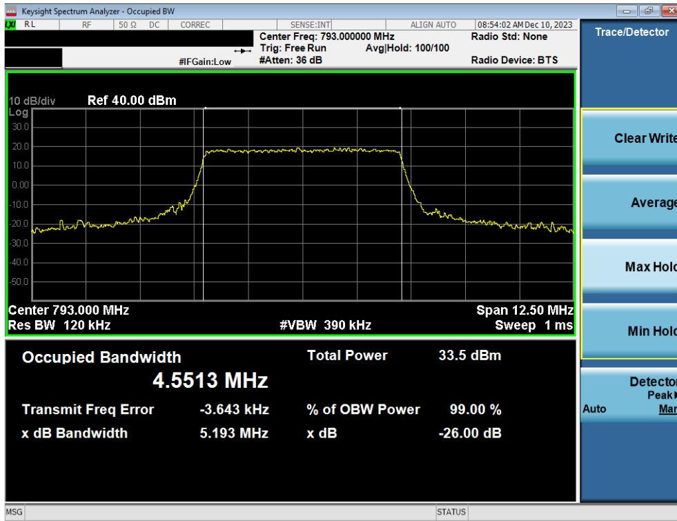
Plot 7-17. Occupied Bandwidth Plot (LTE Band 14 - 5MHz QPSK - Full RB)
