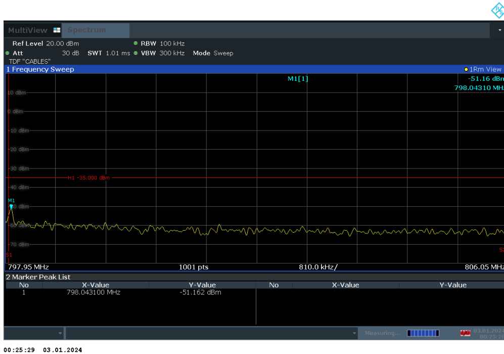
Plot 7-63. Conducted Spurious Plot (LTE Band 14 - 10MHz QPSK - RB Size 1, RB Offset 0 - Mid Channel)
