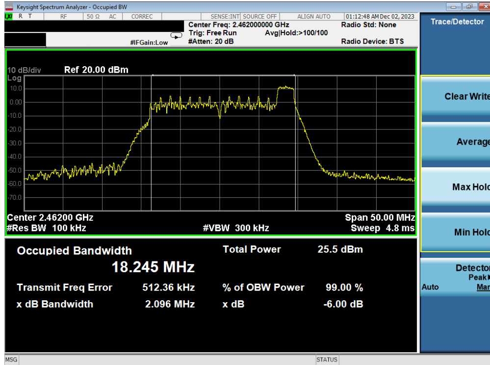
Plot 7-21. 6dB BW & 99% OBW Plot Antenna WF7b (802.11ax OFDMA – RU26 Index 8 – Ch. 11)
