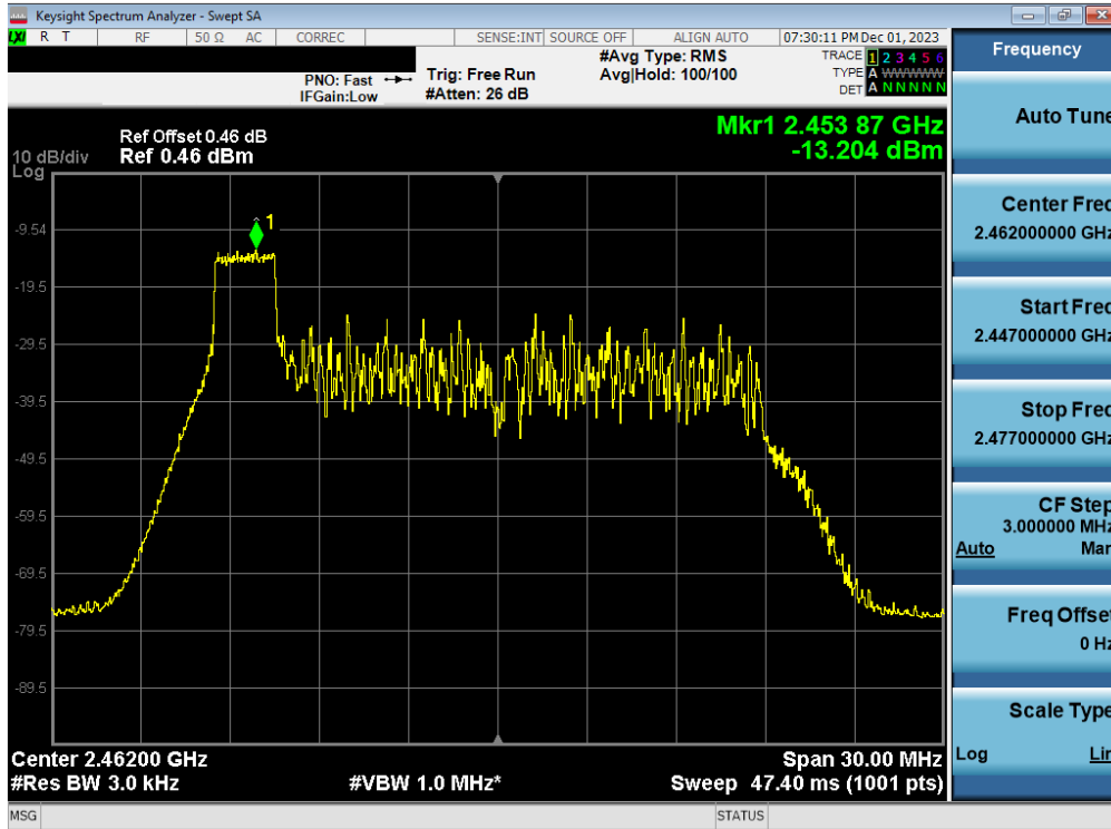
Plot 7-61. Power Spectral Density Plot Antenna WF8 (802.11ax OFDMA – RU26 Index 0 – Ch. 11)
