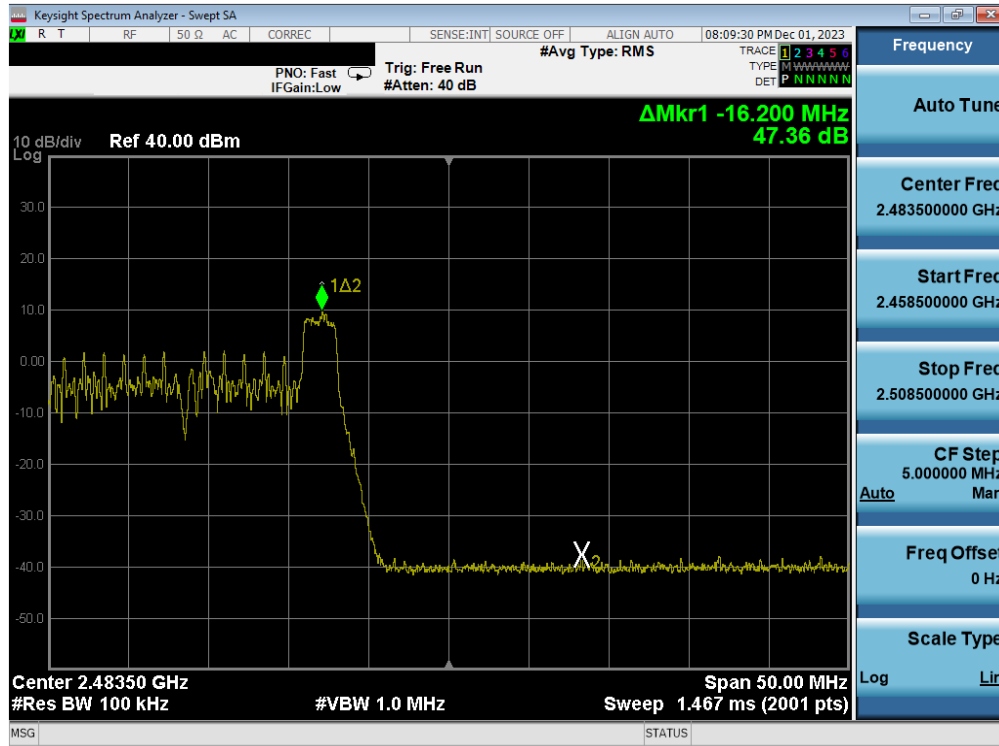
Plot 7-75. Band Edge Antenna WF8 (802.11ax OFDMA – RU26 Index 8 – Ch. 12)
