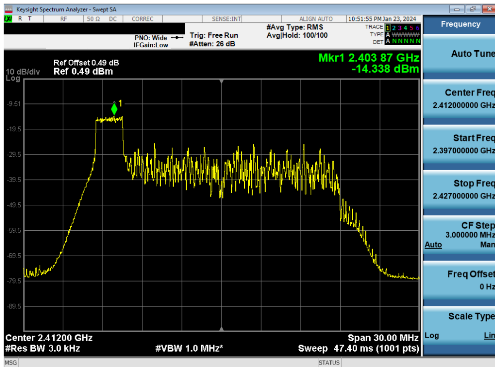
Plot 7-50. Power Spectral Density Plot Antenna WF7b (802.11ax OFDMA – RU26 Index 0 – Ch. 1)
