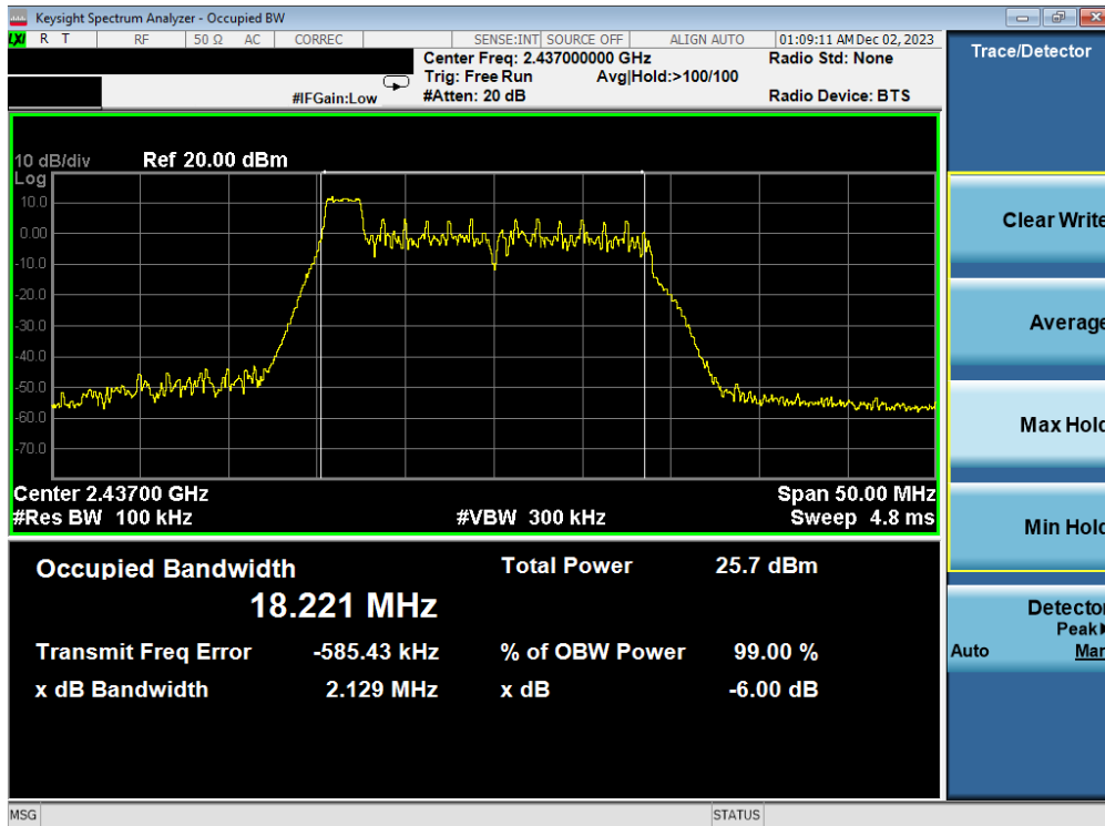
Plot 7-16. 6dB BW & 99% OBW Plot Antenna WF7b (802.11ax OFDMA – RU26 Index 0 – Ch. 6)
