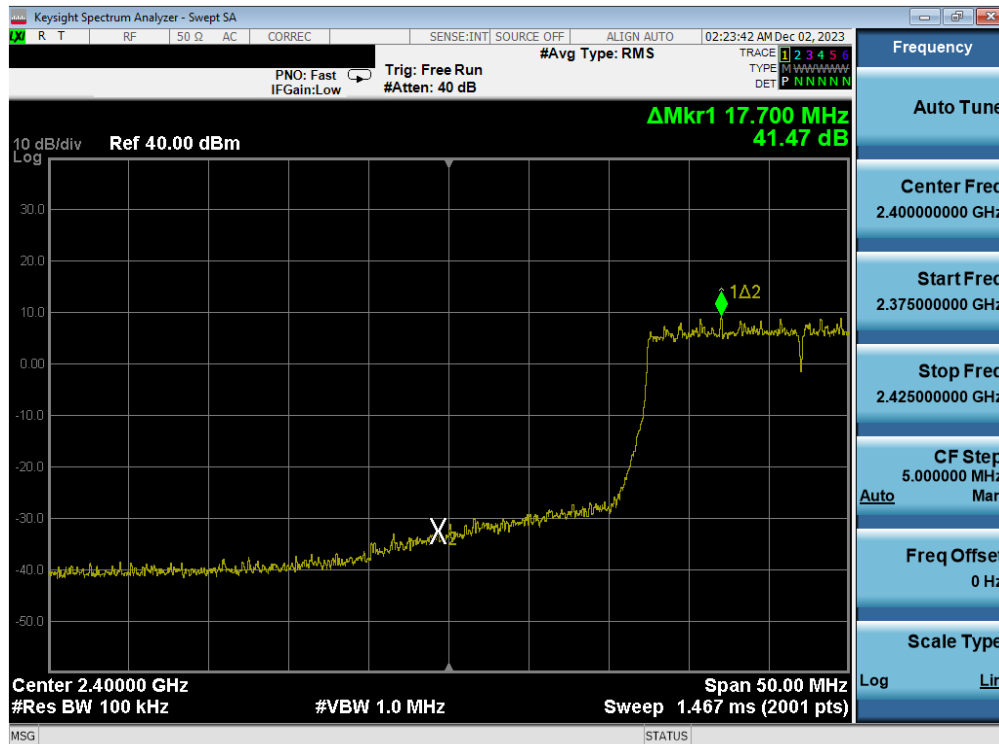
Plot 7-94. Band Edge Antenna WF7b (802.11ax OFDMA – RU242 – Ch. 3)
