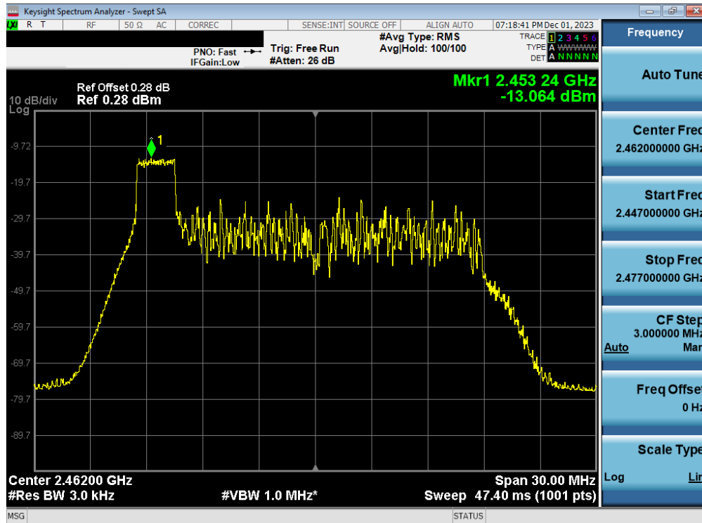
Plot 7-31. Power Spectral Density Plot Antenna WF8 (802.11ax OFDMA – RU26 Index 0 – Ch. 11)
