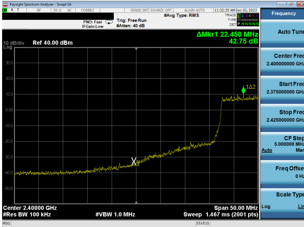
Plot 7-79. Band Edge Antenna WF8 (802.11ax OFDMA – RU242 – Ch. 4)
