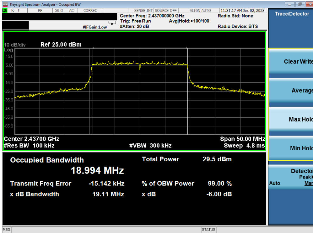
Plot 7-11. 6dB BW & 99% OBW Plot Antenna WF8 (802.11ax OFDMA – RU242 – Ch. 6)
