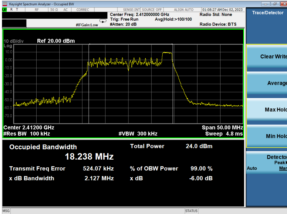
Plot 7-15. 6dB BW & 99% OBW Plot Antenna WF7b (802.11ax OFDMA – RU26 Index 8 – Ch. 1)
