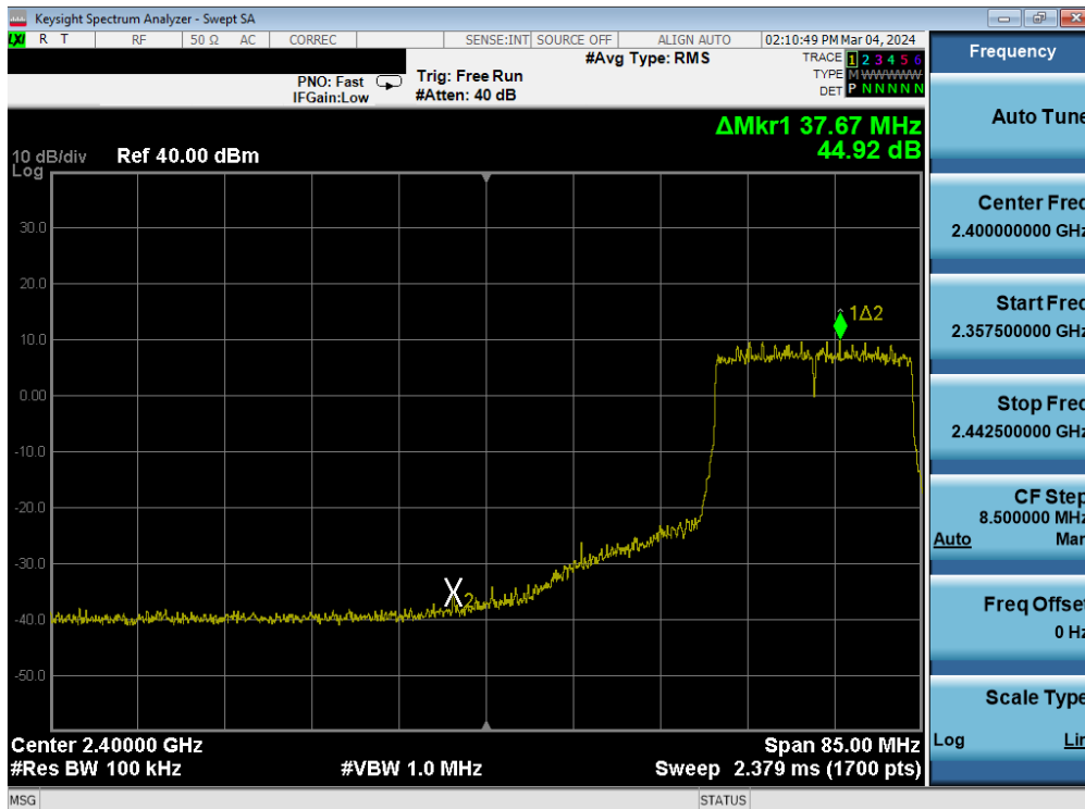
Plot 7-96. Band Edge Antenna WF7b (802.11ax OFDMA – RU242 – Ch. 5)
