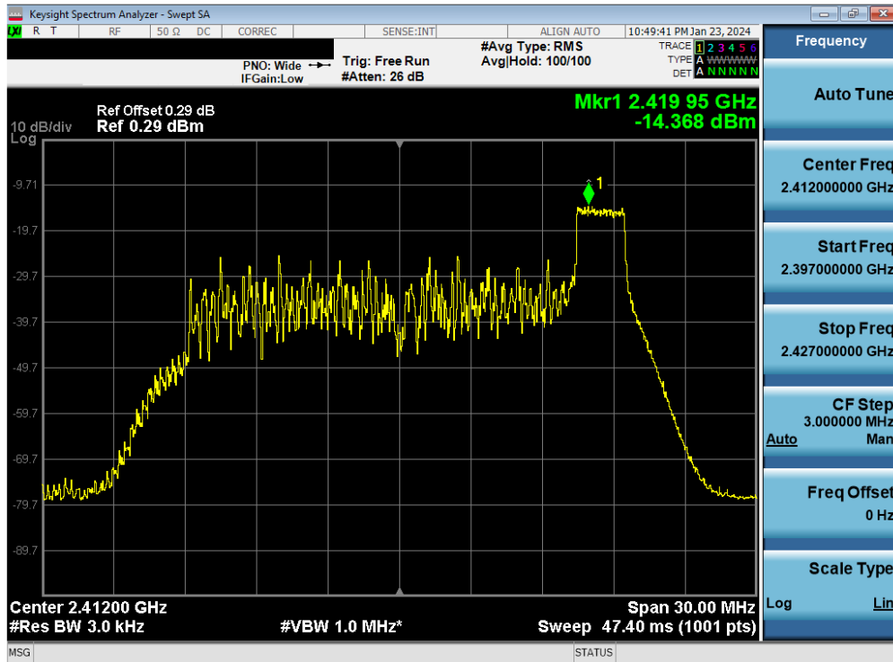
Plot 7-39. Power Spectral Density Plot Antenna WF7b (802.11ax OFDMA – RU26 Index 8 – Ch. 1)
