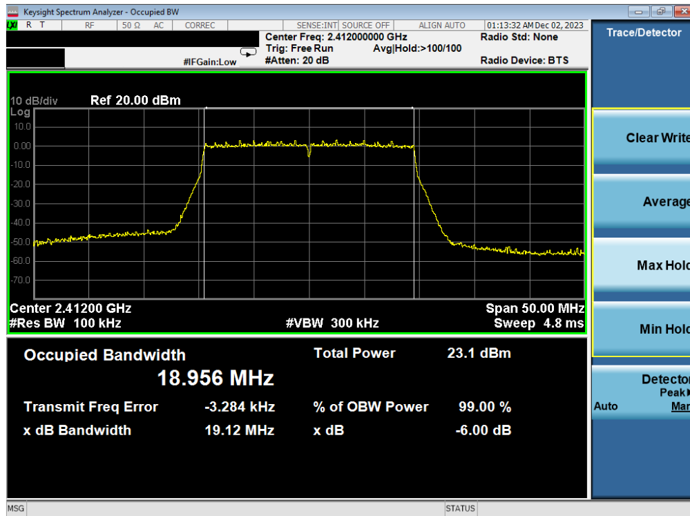
Plot 7-22. 6dB BW & 99% OBW Plot Antenna WF7b (802.11ax OFDMA – RU242 – Ch. 1)
