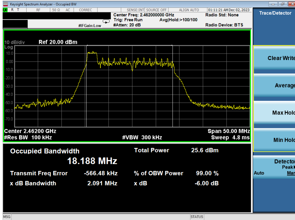
Plot 7-19. 6dB BW & 99% OBW Antenna WF7b (802.11ax OFDMA – RU26 Index 0 – Ch. 11)
