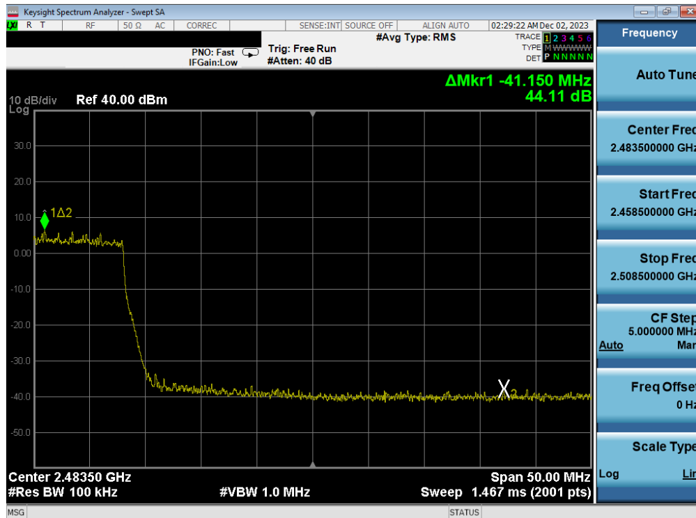
Plot 7-102. Band Edge Antenna WF7b (802.11ax OFDMA – RU242 – Ch. 10)
