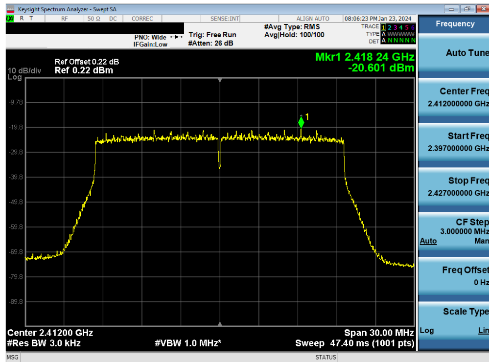
Plot 7-34. Power Spectral Density Plot Antenna WF8 (802.11ax OFDMA – RU242 – Ch. 1)
