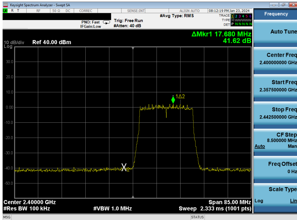
Plot 7-76. Band Edge Antenna WF8 (802.11ax OFDMA – RU242 – Ch. 1)
