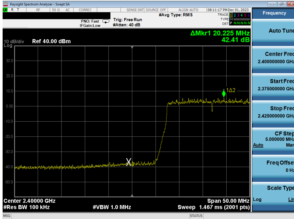
Plot 7-77. Band Edge Antenna WF8 (802.11ax OFDMA – RU242 – Ch. 2)
