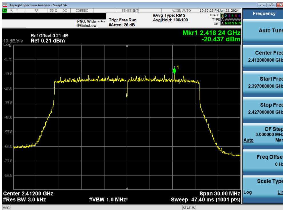
Plot 7-46. Power Spectral Density Plot Antenna WF7b (802.11ax OFDMA – RU242 – Ch. 1)
