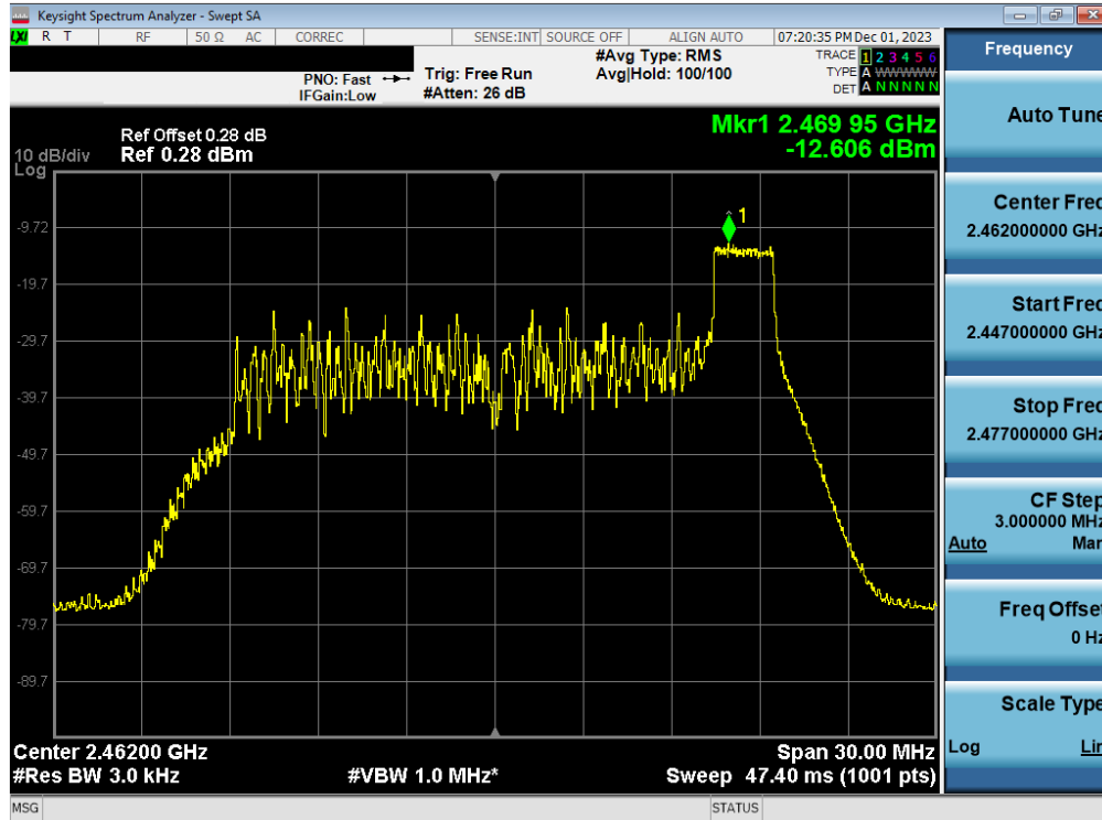
Plot 7-33. Power Spectral Density Plot Antenna WF8 (802.11ax OFDMA – RU26 Index 8 – Ch. 11)
