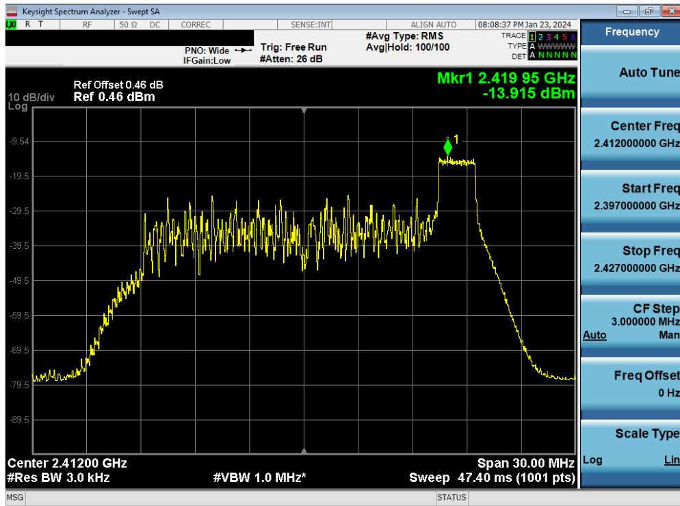
Plot 7-53. Power Spectral Density Plot Antenna WF8 (802.11ax OFDMA – RU26 Index 8 – Ch. 1)
