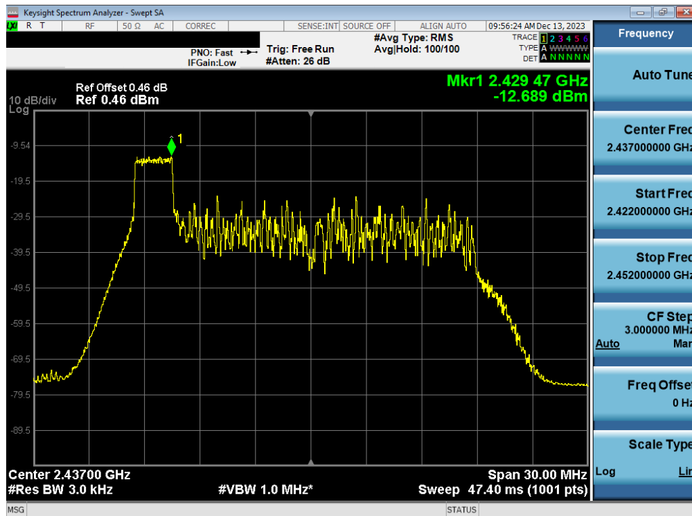
Plot 7-56. Power Spectral Density Plot Antenna WF7b (802.11ax OFDMA – RU26 Index 0 – Ch. 6)
