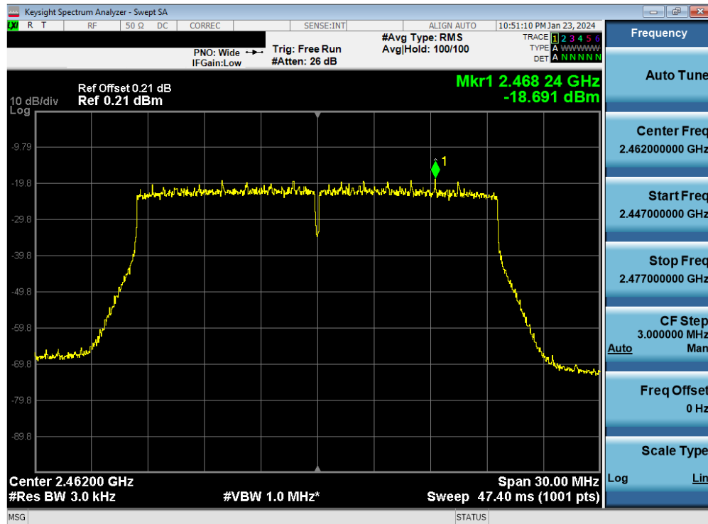
Plot 7-48. Power Spectral Density Plot Antenna WF7b (802.11ax OFDMA – RU242 – Ch. 11)
