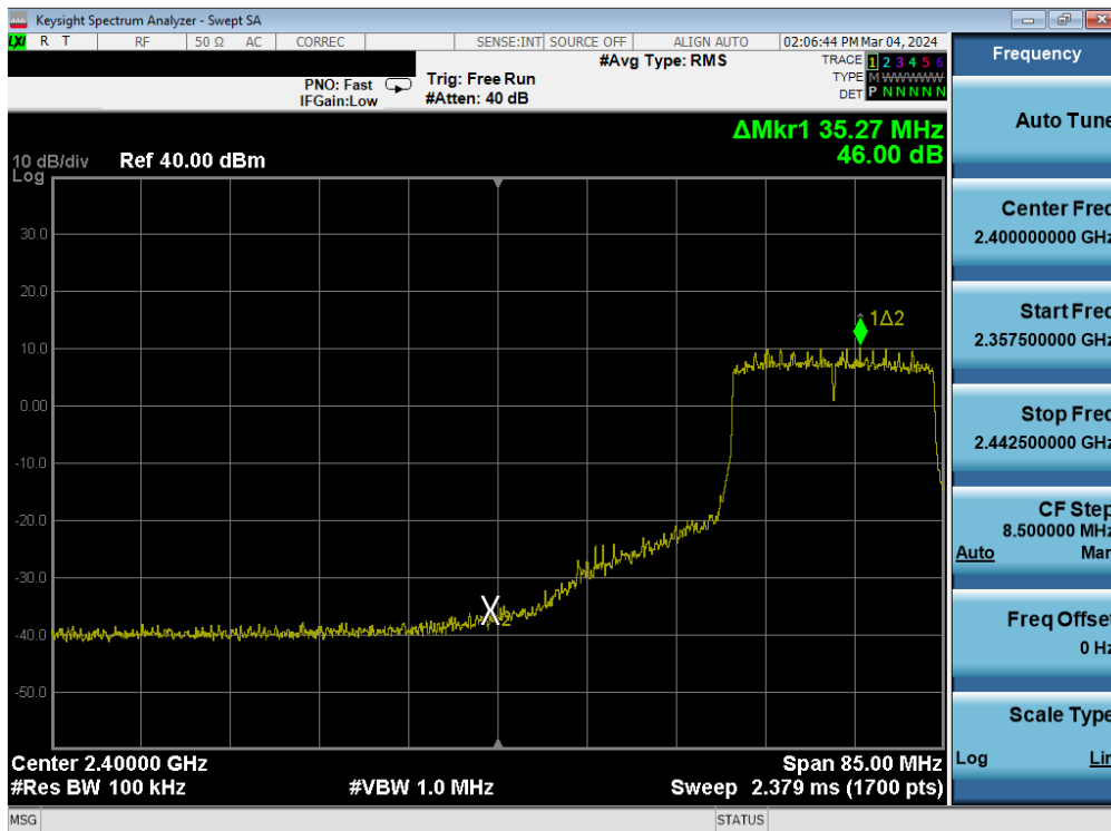
Plot 7-80. Band Edge Antenna WF8 (802.11ax OFDMA – RU242 – Ch. 5)
