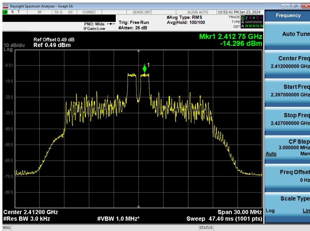
Plot 7-52. Power Spectral Density Plot Antenna WF7b (802.11ax OFDMA – RU26 Index 4 – Ch. 1)
