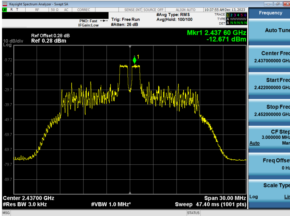
Plot 7-41. Power Spectral Density Plot Antenna WF7b (802.11ax OFDMA – RU26 Index 4 – Ch. 6)
