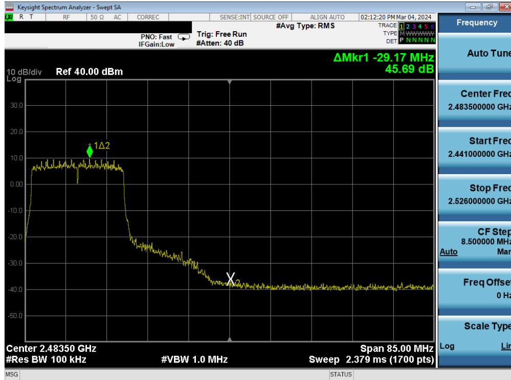
Plot 7-101. Band Edge Antenna WF7b (802.11ax OFDMA – RU242 – Ch. 9)
