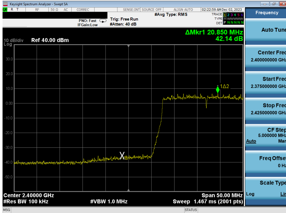
Plot 7-93. Band Edge Antenna WF7b (802.11ax OFDMA – RU242 – Ch. 2)
