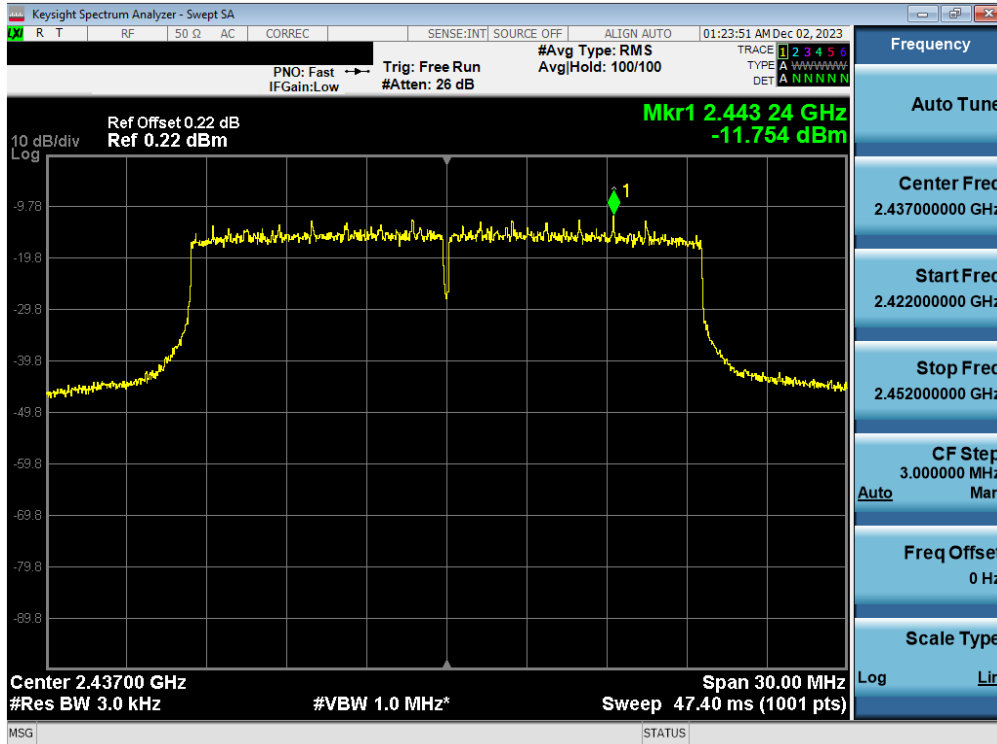
Plot 7-47. Power Spectral Density Plot Antenna WF7b (802.11ax OFDMA – RU242 – Ch. 6)
