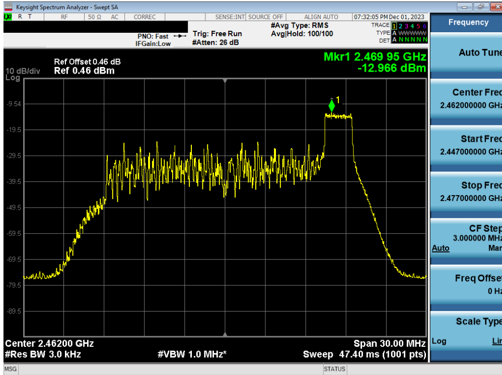
Plot 7-65. Power Spectral Density Plot Antenna WF8 (802.11ax OFDMA – RU26 Index 8 – Ch. 11)
