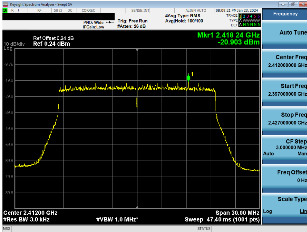
Plot 7-67. Power Spectral Density Plot Antenna WF8 (802.11ax OFDMA – RU242 – Ch. 1)
