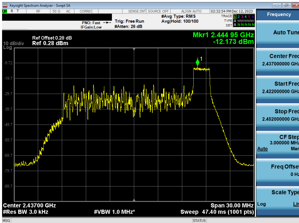
Plot 7-30. Power Spectral Density Plot Antenna WF8 (802.11ax OFDMA – RU26 Index 8 – Ch. 6)
