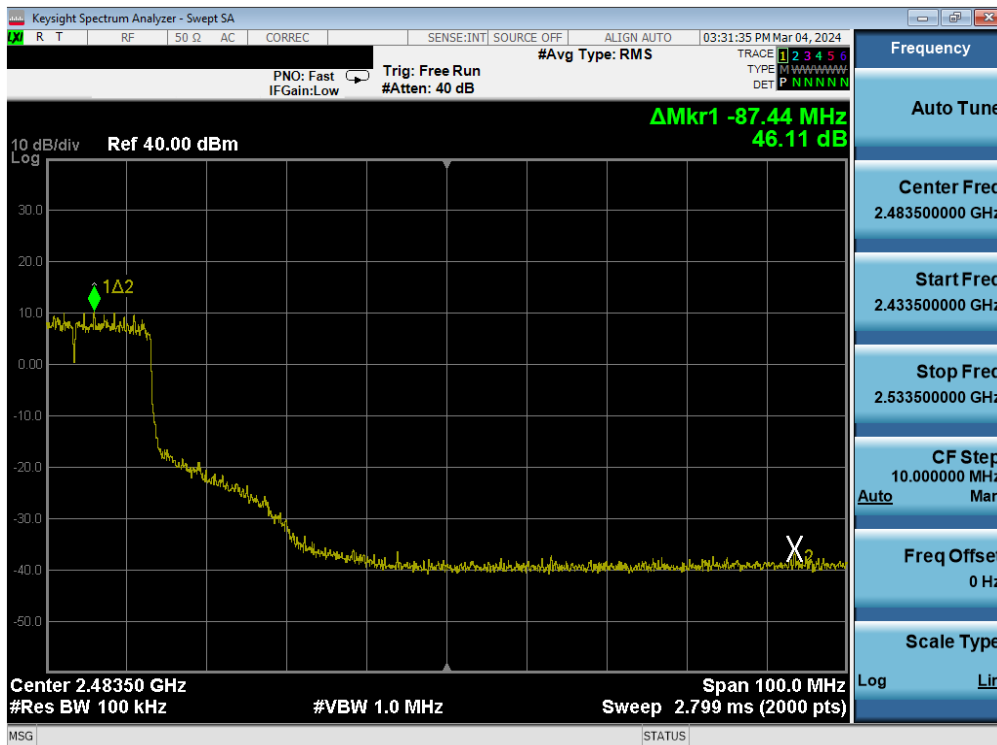
Plot 7-82. Band Edge Antenna WF8 (802.11ax OFDMA – RU242 – Ch. 6(high))
