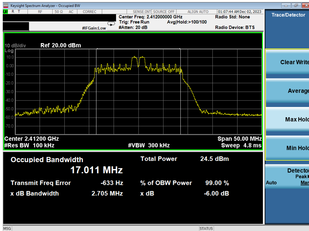
Plot 7-14. 6dB BW & 99% OBW Plot Antenna WF7b (802.11ax OFDMA – RU26 Index 4 – Ch. 1)
