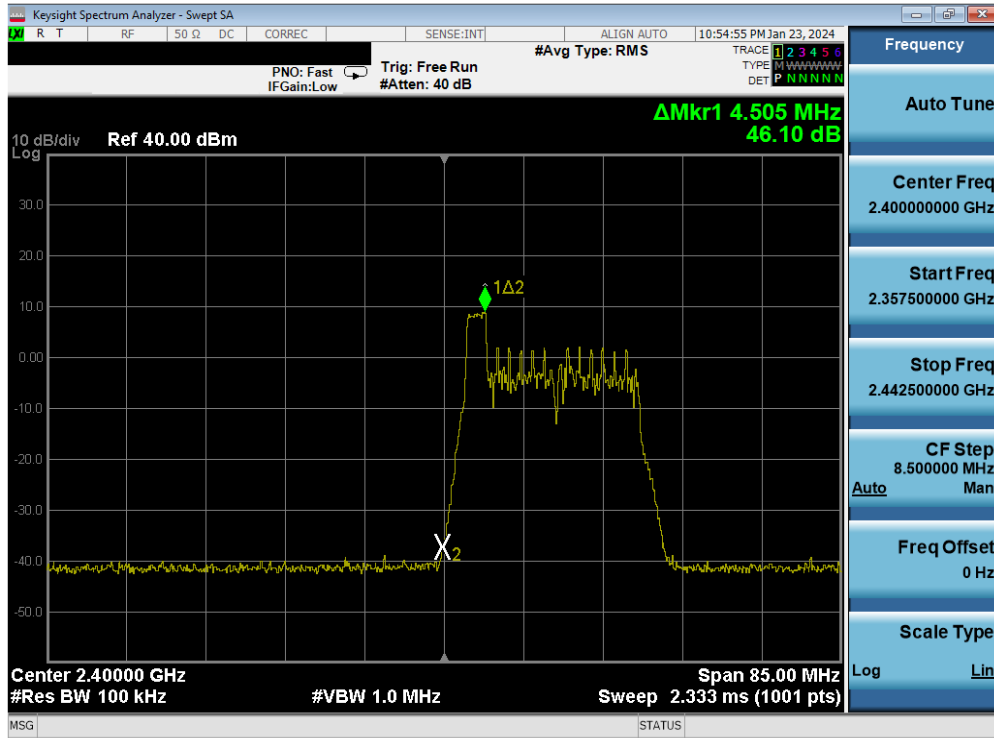
Plot 7-89. Band Edge Antenna WF7b (802.11ax OFDMA – RU26 Index 0 – Ch. 1)
