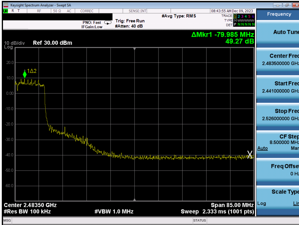
Plot 7-99. Band Edge Antenna WF7b (802.11ax OFDMA – RU242 – Ch. 7)
