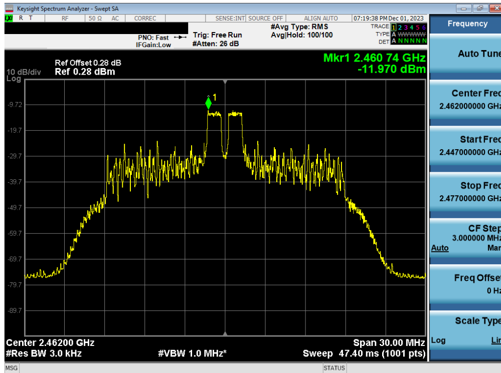
Plot 7-32. Power Spectral Density Plot Antenna WF8 (802.11ax OFDMA – RU26 Index 4 – Ch. 11)
