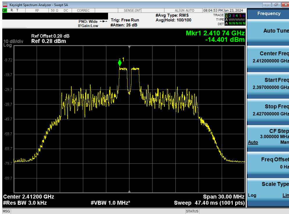
Plot 7-26. Power Spectral Density Plot Antenna WF8 (802.11ax OFDMA – RU26 Index 4 – Ch. 1)
