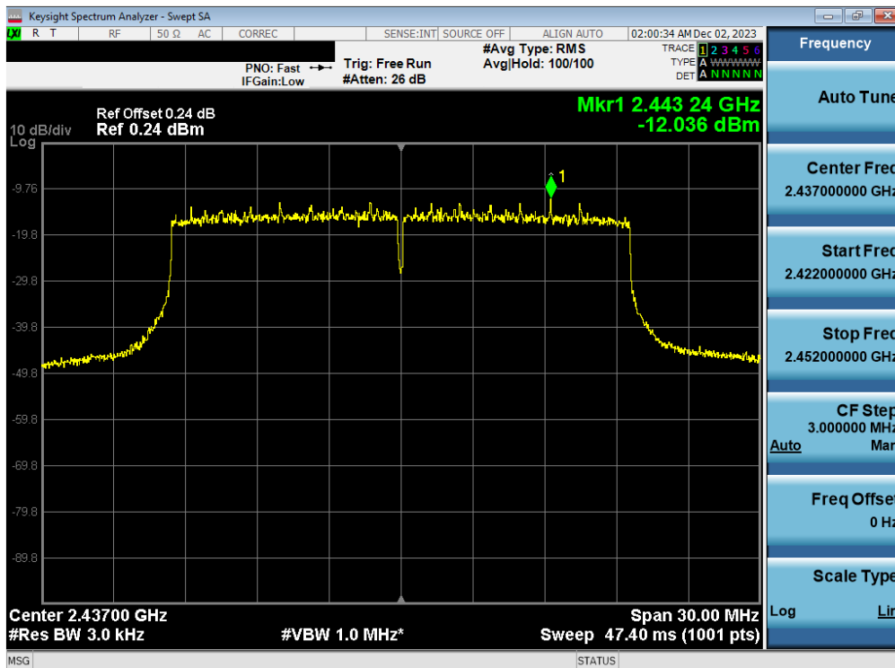
Plot 7-70. Power Spectral Density Plot Antenna WF7b (802.11ax OFDMA – RU242 – Ch. 6)
