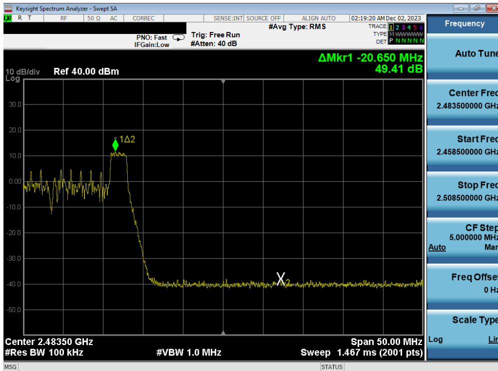
Plot 7-90. Band Edge Antenna WF7b (802.11ax OFDMA – RU26 Index 8 – Ch. 11)
