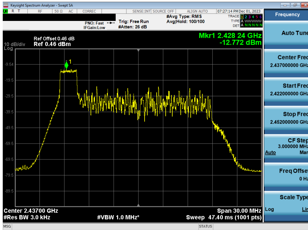
Plot 7-55. Power Spectral Density Plot Antenna WF8 (802.11ax OFDMA – RU26 Index 0 – Ch. 6)
