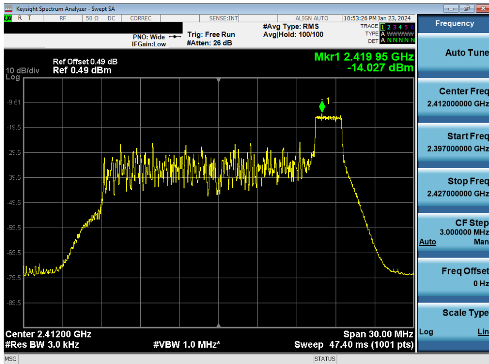
Plot 7-54. Power Spectral Density Plot Antenna WF7b (802.11ax OFDMA – RU26 Index 8 – Ch. 1)
