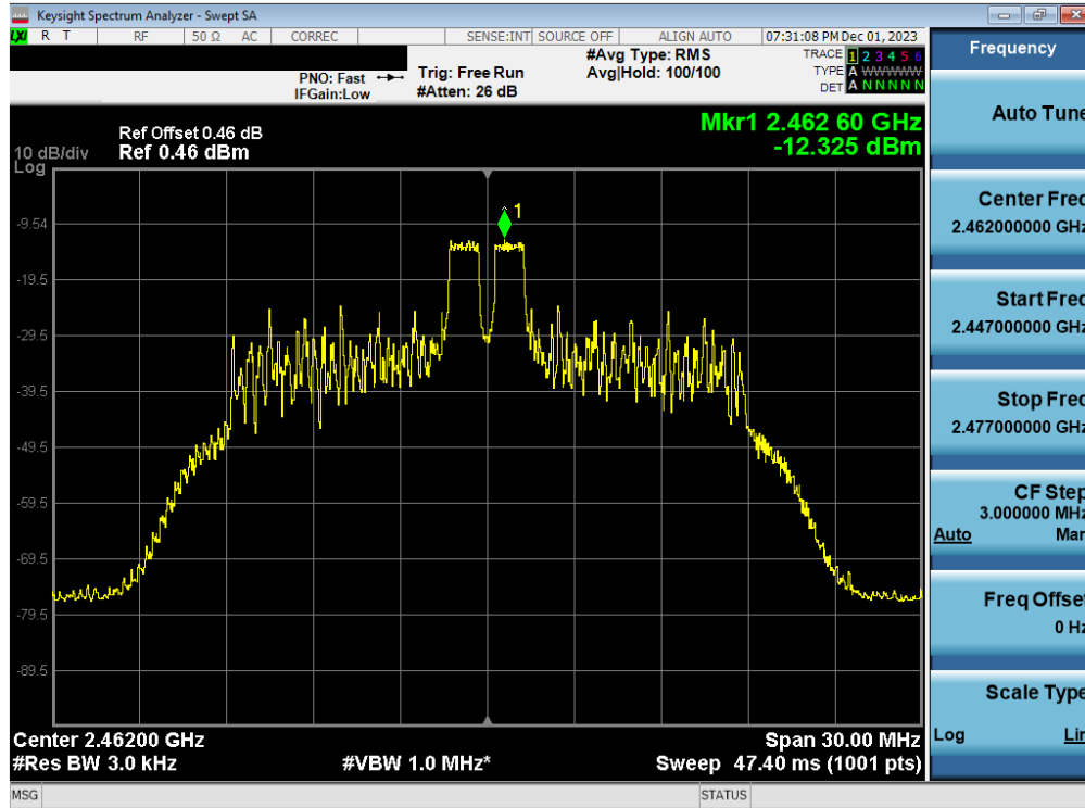
Plot 7-63. Power Spectral Density Plot Antenna WF8 (802.11ax OFDMA – RU26 Index 4 – Ch. 11)
