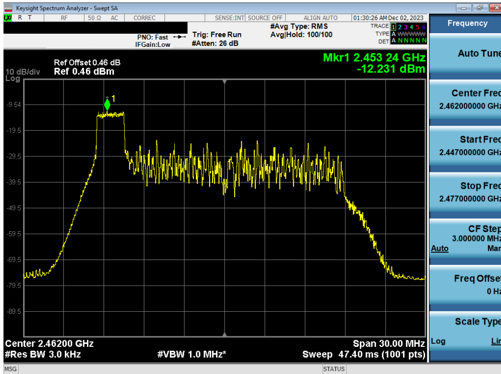
Plot 7-62. Power Spectral Density Plot Antenna WF7b (802.11ax OFDMA – RU26 Index 0 – Ch. 11)
