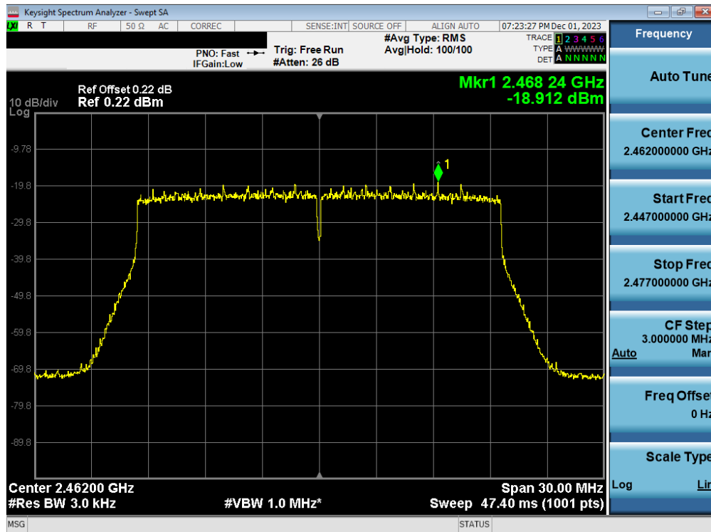
Plot 7-36. Power Spectral Density Plot Antenna WF8 (802.11ax OFDMA – RU242 – Ch. 11)
