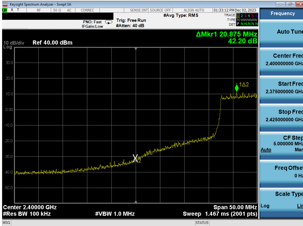
Plot 7-95. Band Edge Antenna WF7b (802.11ax OFDMA – RU242 – Ch. 4)
