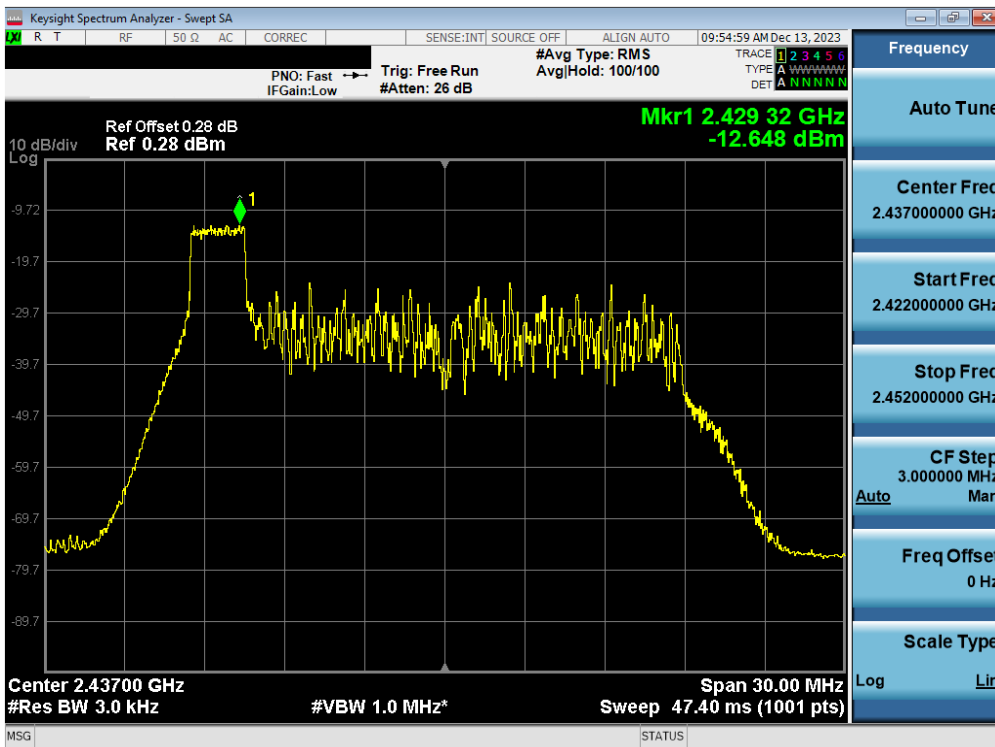
Plot 7-40. Power Spectral Density Plot Antenna WF7b (802.11ax OFDMA – RU26 Index 0 – Ch. 6)
