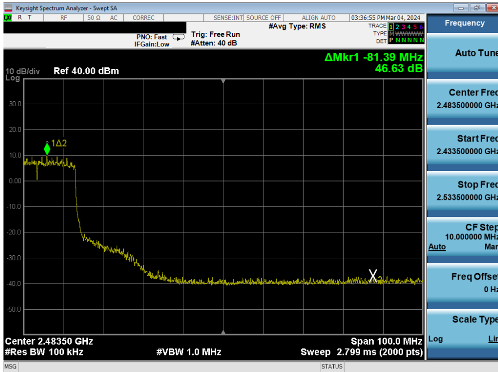
Plot 7-98. Band Edge Antenna WF7b (802.11ax OFDMA – RU242 – Ch. 6(high))
