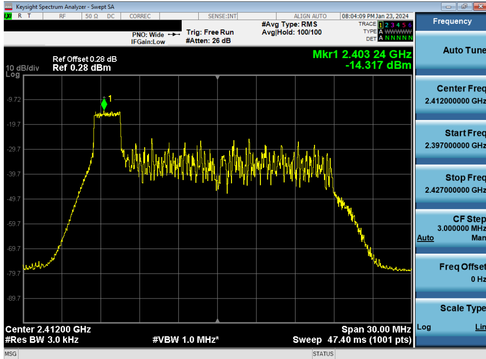
Plot 7-25. Power Spectral Density Plot Antenna WF8 (802.11ax OFDMA – RU26 Index 0 – Ch. 1)
