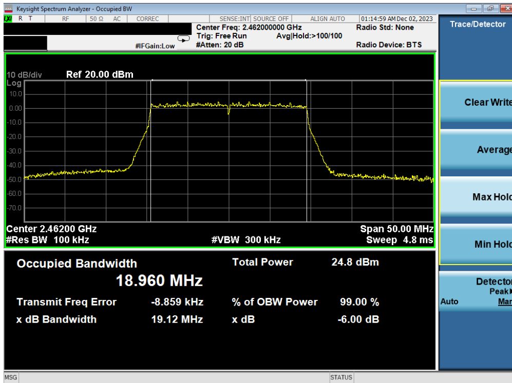
Plot 7-24. 6dB BW & 99% OBW Plot Antenna WF7b (802.11ax OFDMA – RU242 – Ch. 11)
