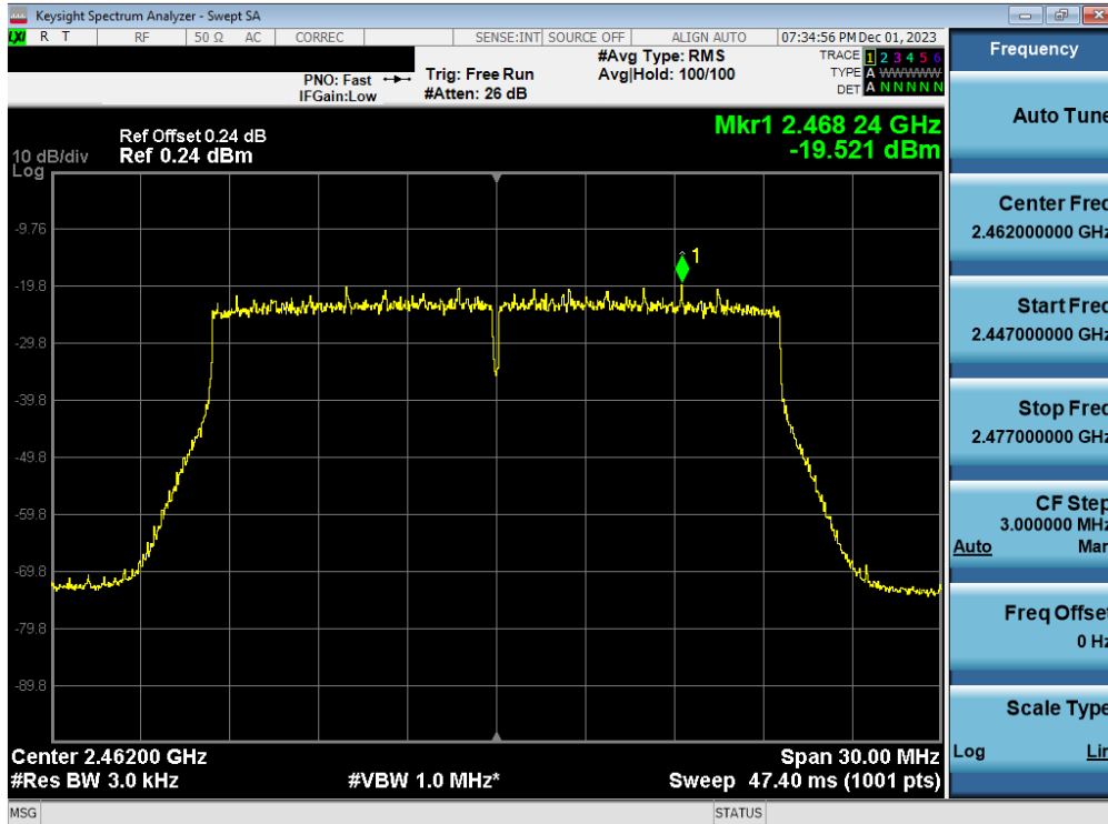
Plot 7-71. Power Spectral Density Plot Antenna WF8 (802.11ax OFDMA – RU242 – Ch. 11)
