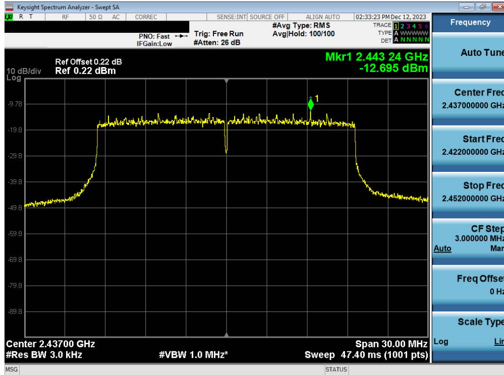
Plot 7-35. Power Spectral Density Plot Antenna WF8 (802.11ax OFDMA – RU242 – Ch. 6)
