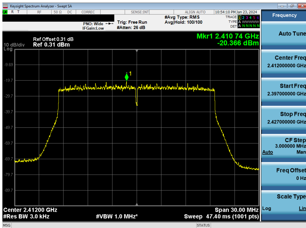
Plot 7-68. Power Spectral Density Plot Antenna WF7b (802.11ax OFDMA – RU242 – Ch. 1)
