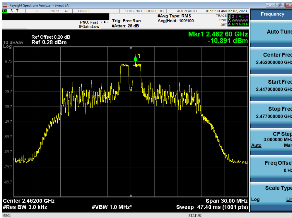
Plot 7-44. Power Spectral Density Plot Antenna WF7b (802.11ax OFDMA – RU26 Index 4 – Ch. 11)
