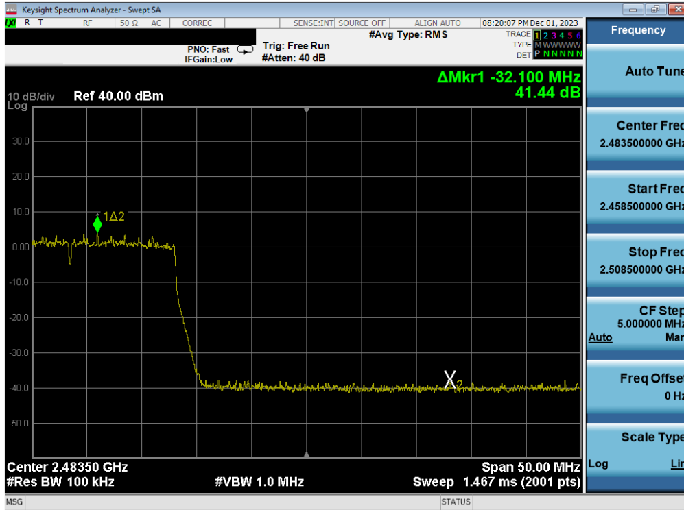
Plot 7-87. Band Edge Antenna WF8 (802.11ax OFDMA – RU242 – Ch. 11)
