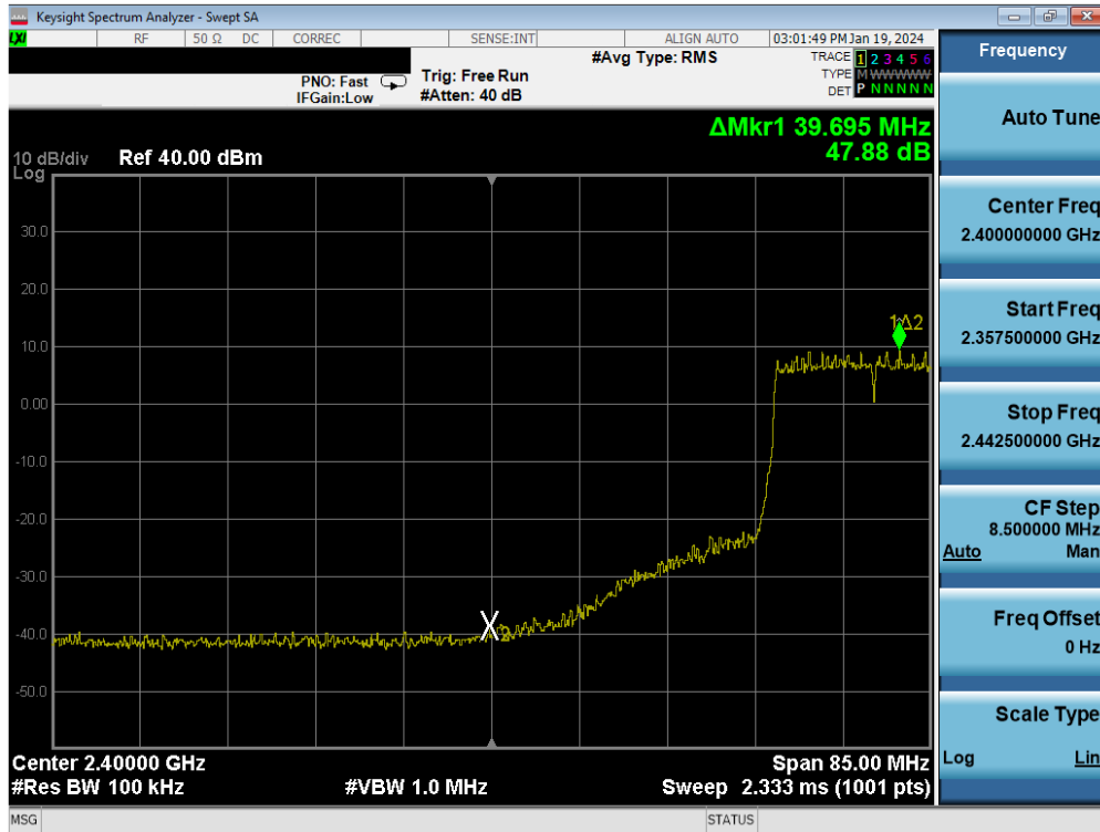
Plot 7-97. Band Edge Antenna WF7b (802.11ax OFDMA – RU242 – Ch. 6(low))
