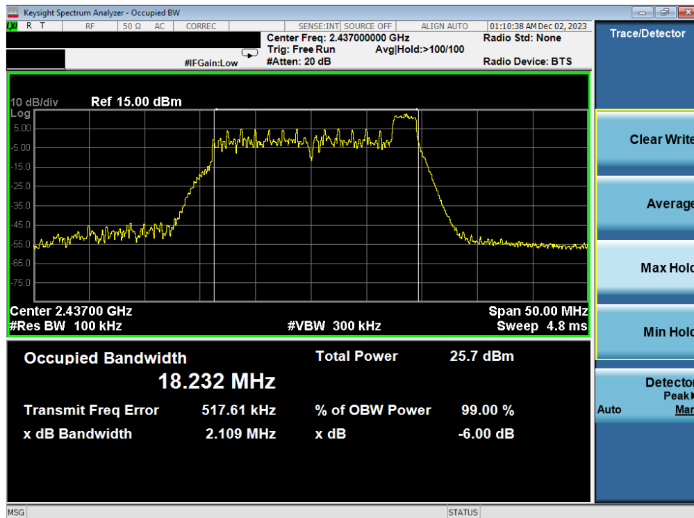
Plot 7-18. 6dB BW & 99% OBW Antenna WF7b (802.11ax OFDMA – RU26 Index 8 – Ch. 6)
