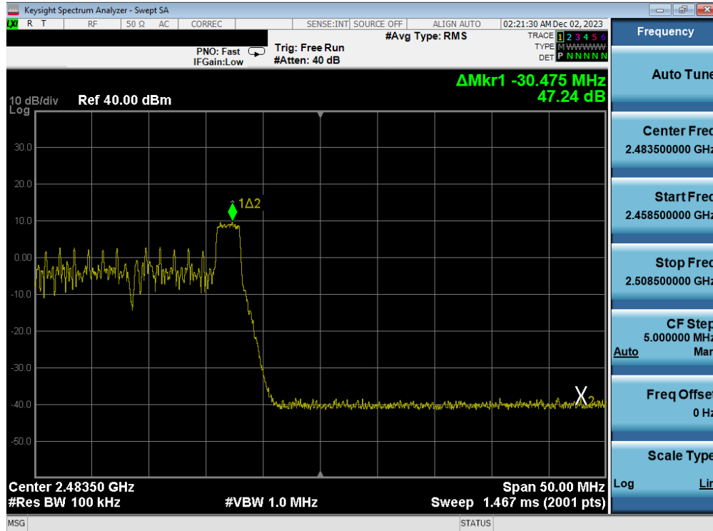
Plot 7-91. Band Edge Antenna WF7b (802.11ax OFDMA – RU26 Index 8 – Ch. 12)
