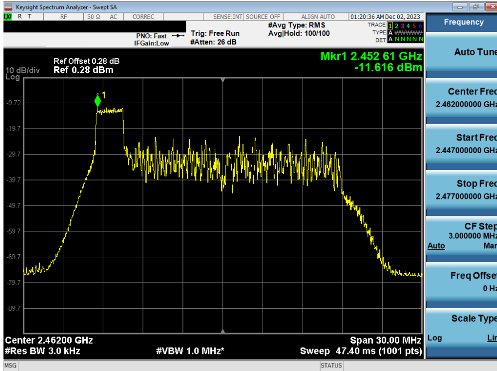
Plot 7-43. Power Spectral Density Plot Antenna WF7b (802.11ax OFDMA – RU26 Index 0 – Ch. 11)
