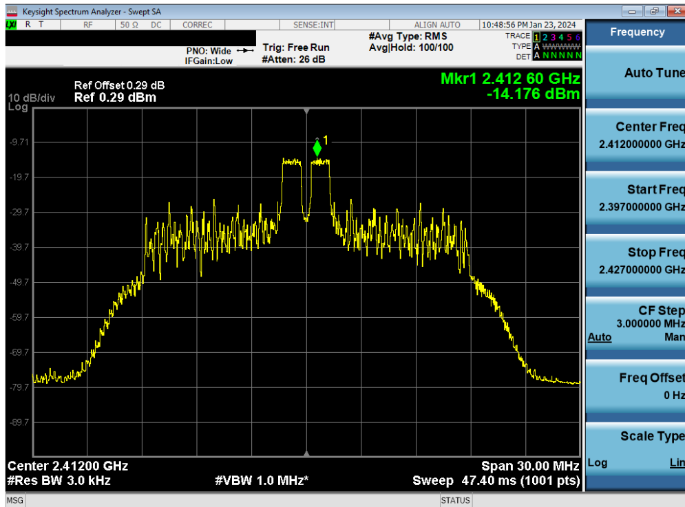
Plot 7-38. Power Spectral Density Plot Antenna WF7b (802.11ax OFDMA – RU26 Index 4 – Ch. 1)
