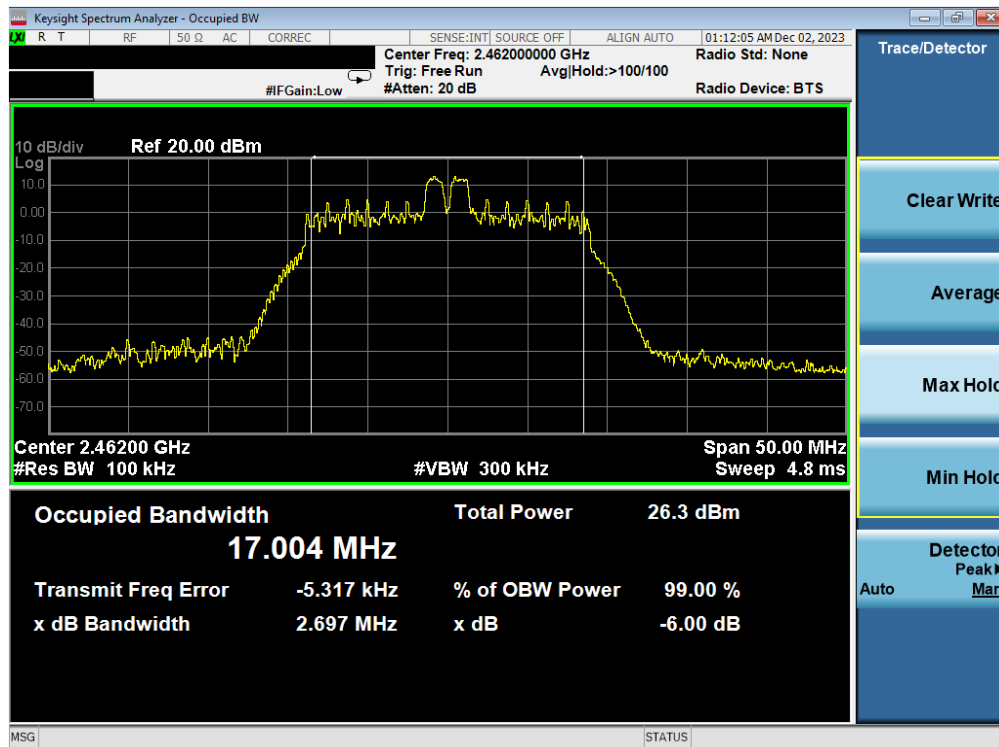
Plot 7-20. 6dB BW & 99% OBW Antenna WF7b (802.11ax OFDMA – RU26 Index 4 – Ch. 11)
