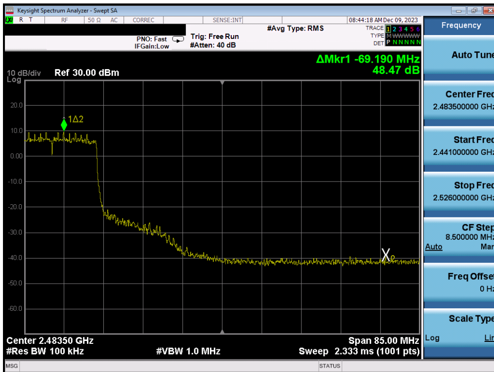
Plot 7-100. Band Edge Antenna WF7b (802.11ax OFDMA – RU242 – Ch. 8)
