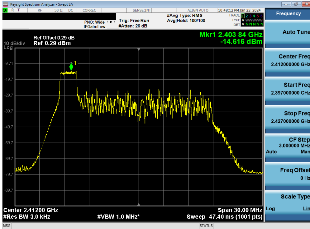
Plot 7-37. Power Spectral Density Plot Antenna WF7b (802.11ax OFDMA – RU26 Index 0 – Ch. 1)
