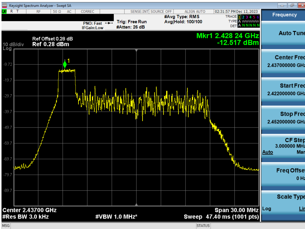
Plot 7-28. Power Spectral Density Plot Antenna WF8 (802.11ax OFDMA – RU26 Index 0 – Ch. 6)
