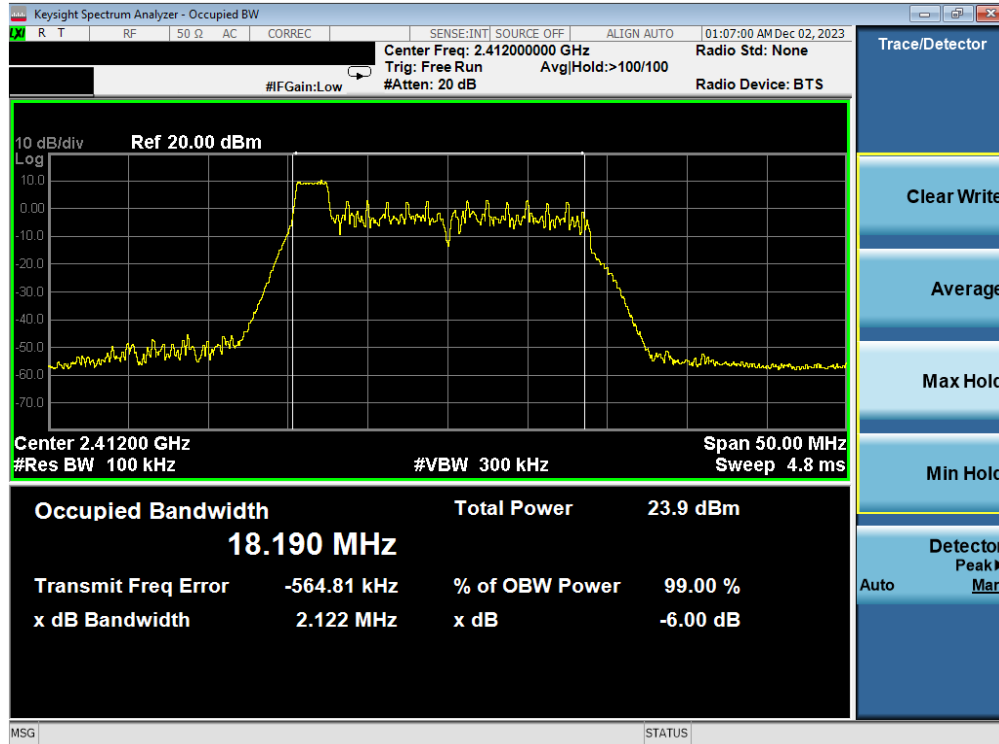
Plot 7-13. 6dB BW & 99% OBW Plot Antenna WF7b (802.11ax OFDMA – RU26 Index 0 – Ch. 1)
