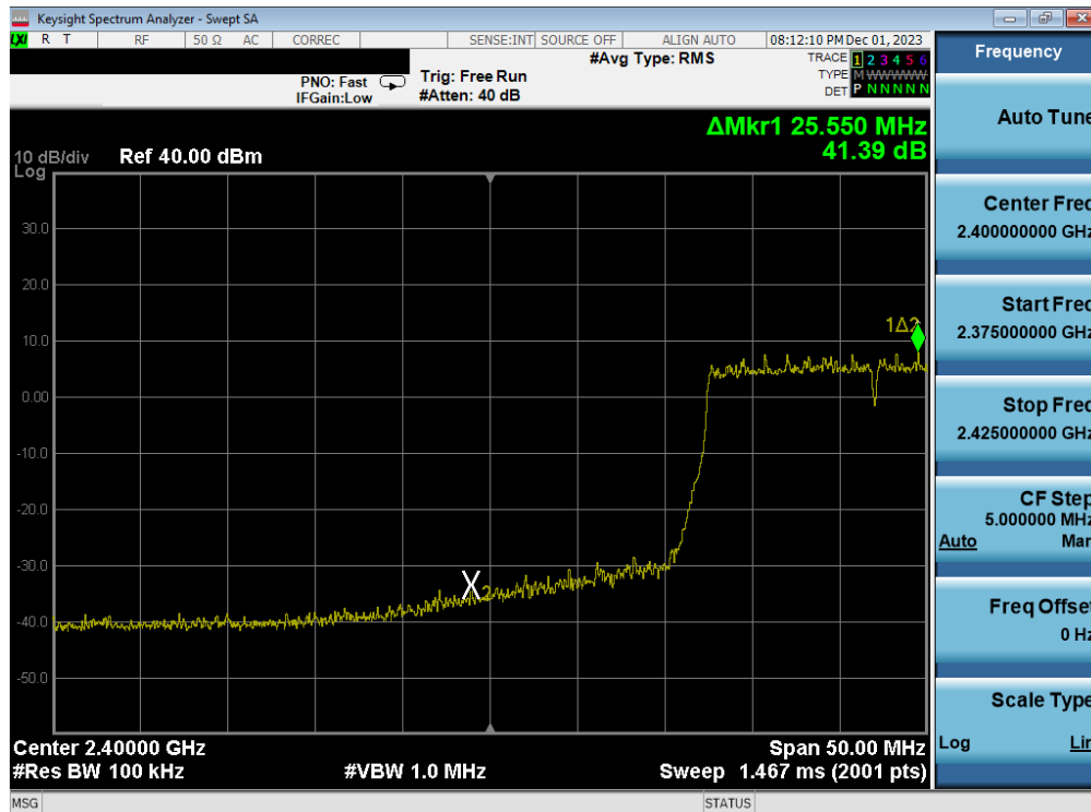
Plot 7-78. Band Edge Antenna WF8 (802.11ax OFDMA – RU242 – Ch. 3)
