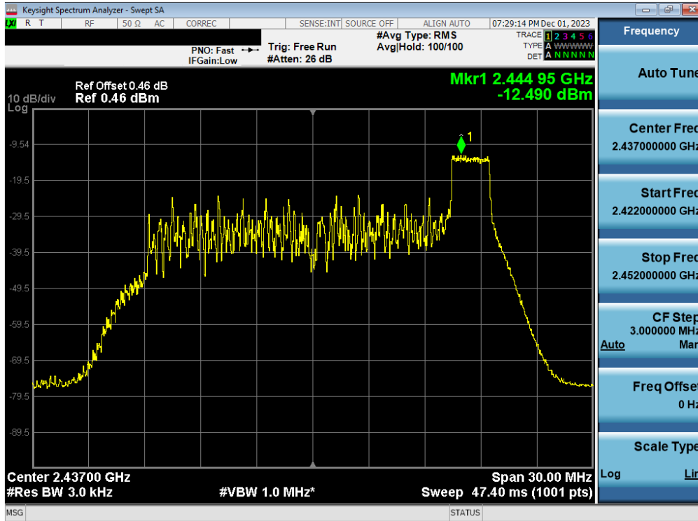
Plot 7-59. Power Spectral Density Plot Antenna WF8 (802.11ax OFDMA – RU26 Index 8 – Ch. 6)
