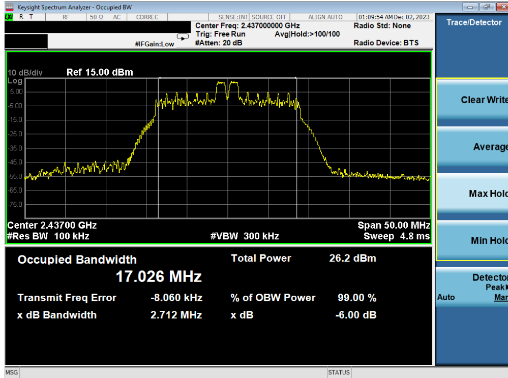
Plot 7-17. 6dB BW & 99% OBW Plot Antenna WF7b (802.11ax OFDMA – RU26 Index 4 – Ch. 6)
