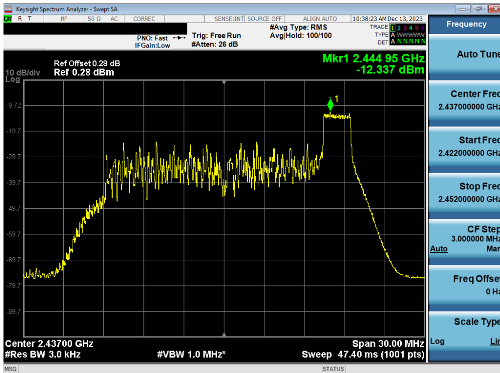
Plot 7-42. Power Spectral Density Plot Antenna WF7b (802.11ax OFDMA – RU26 Index 8 – Ch. 6)
