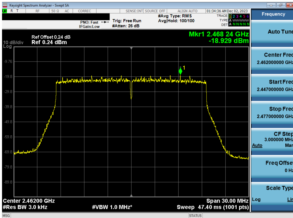
Plot 7-72. Power Spectral Density Plot Antenna WF7b (802.11ax OFDMA – RU242 – Ch. 11)
