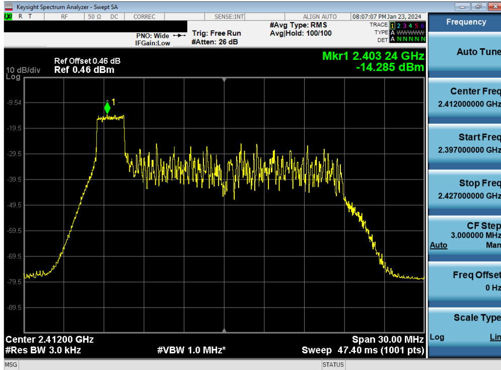
Plot 7-49. Power Spectral Density Plot Antenna WF8 (802.11ax OFDMA – RU26 Index 0 – Ch. 1)
