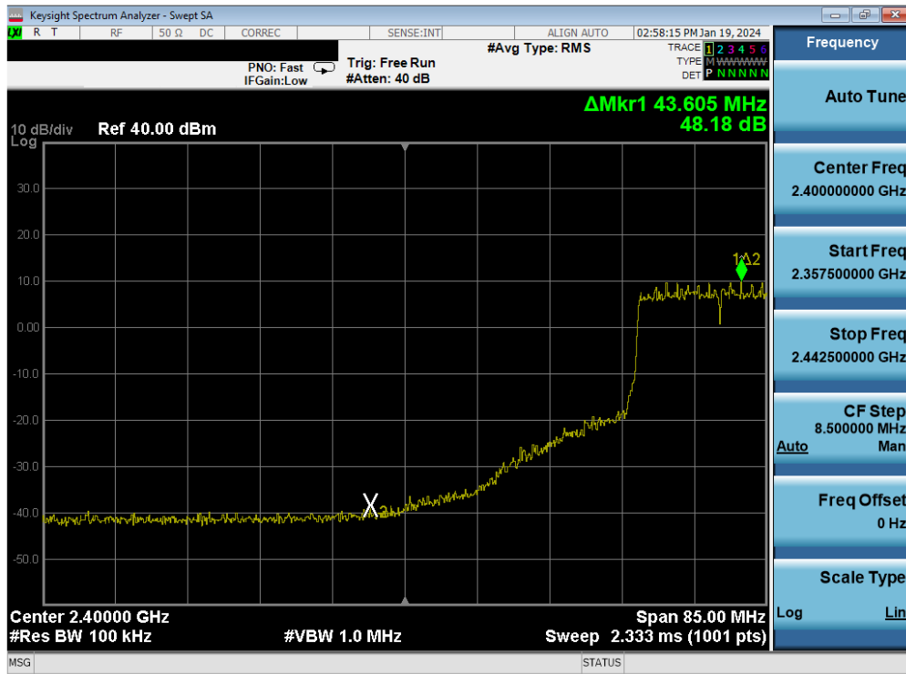
Plot 7-81. Band Edge Antenna WF8 (802.11ax OFDMA – RU242 – Ch. 6(low))
