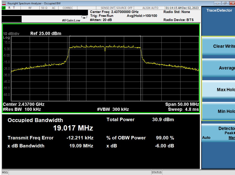
Plot 7-23. 6dB BW & 99% OBW Plot Antenna WF7b (802.11ax OFDMA – RU242 – Ch. 6)
