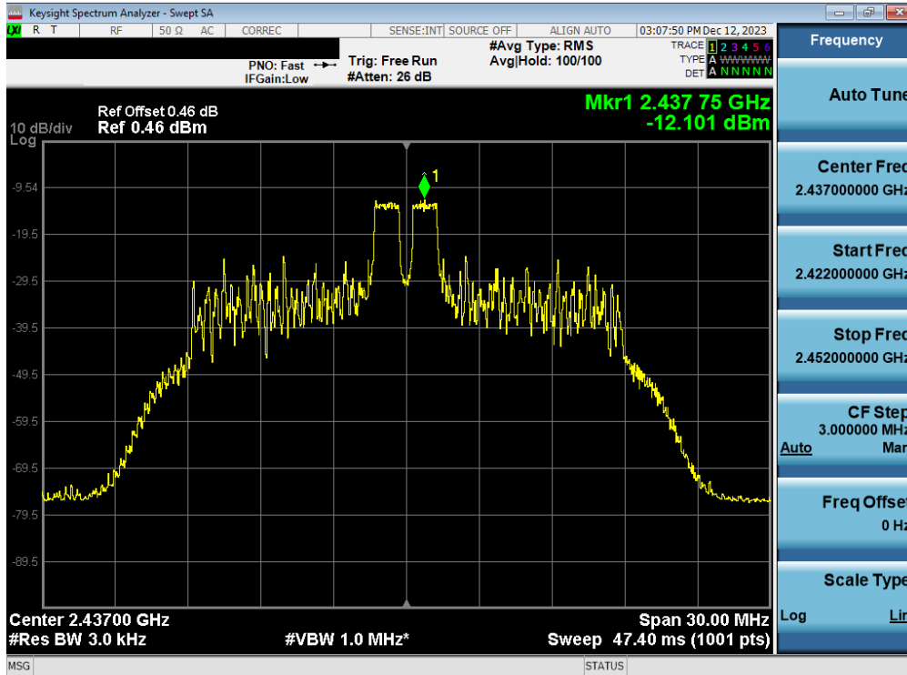
Plot 7-57. Power Spectral Density Plot Antenna WF8 (802.11ax OFDMA – RU26 Index 4 – Ch. 6)
