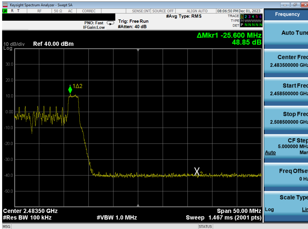
Plot 7-74. Band Edge Antenna WF8 (802.11ax OFDMA – RU26 Index 8 – Ch. 11)
