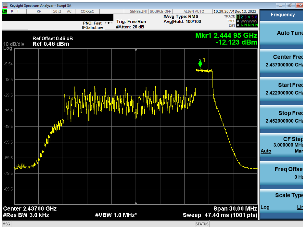
Plot 7-60. Power Spectral Density Plot Antenna WF7b (802.11ax OFDMA – RU26 Index 8 – Ch. 6)
