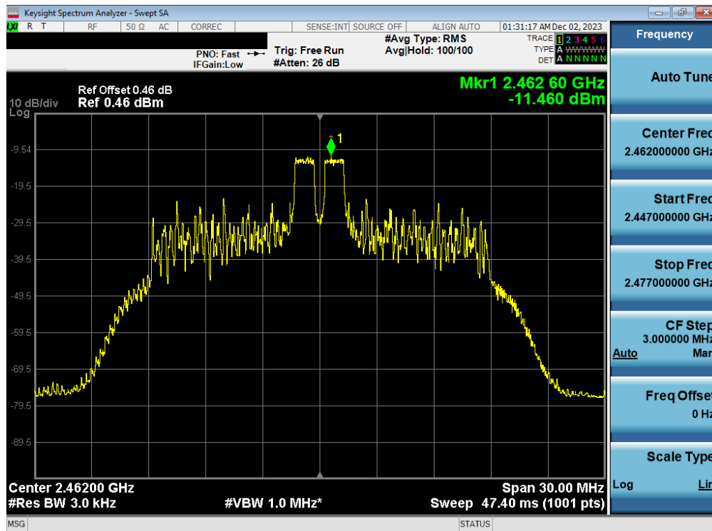
Plot 7-64. Power Spectral Density Plot Antenna WF7b (802.11ax OFDMA – RU26 Index 4 – Ch. 11)
