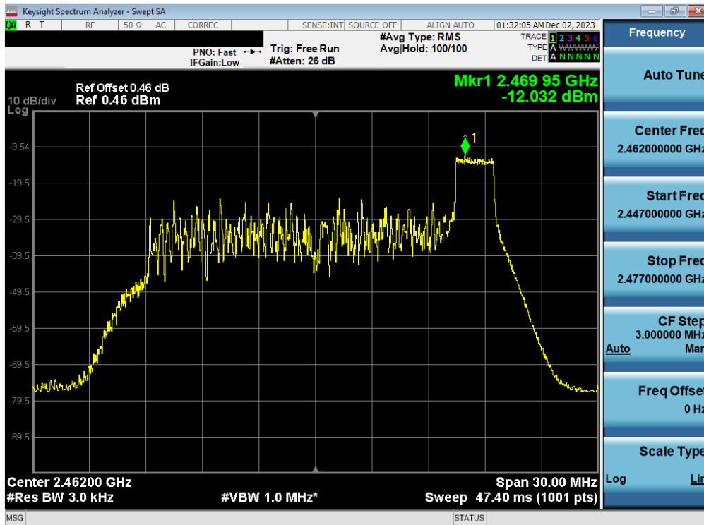
Plot 7-66. Power Spectral Density Plot Antenna WF7b (802.11ax OFDMA – RU26 Index 8 – Ch. 11)
