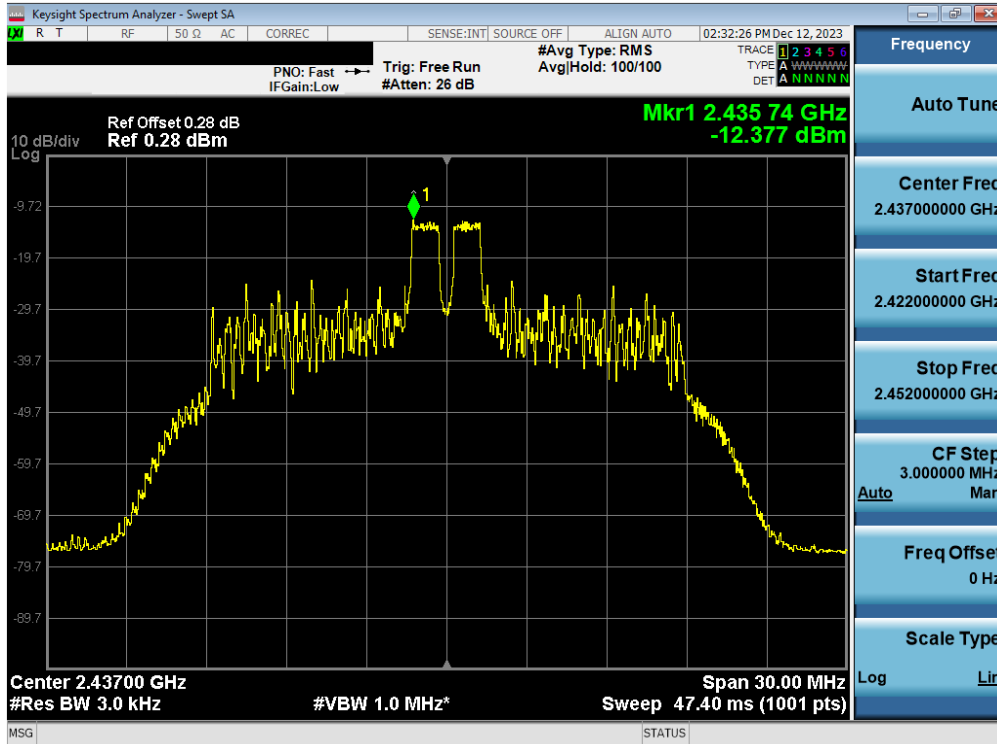
Plot 7-29. Power Spectral Density Plot Antenna WF8 (802.11ax OFDMA – RU26 Index 4 – Ch. 6)
