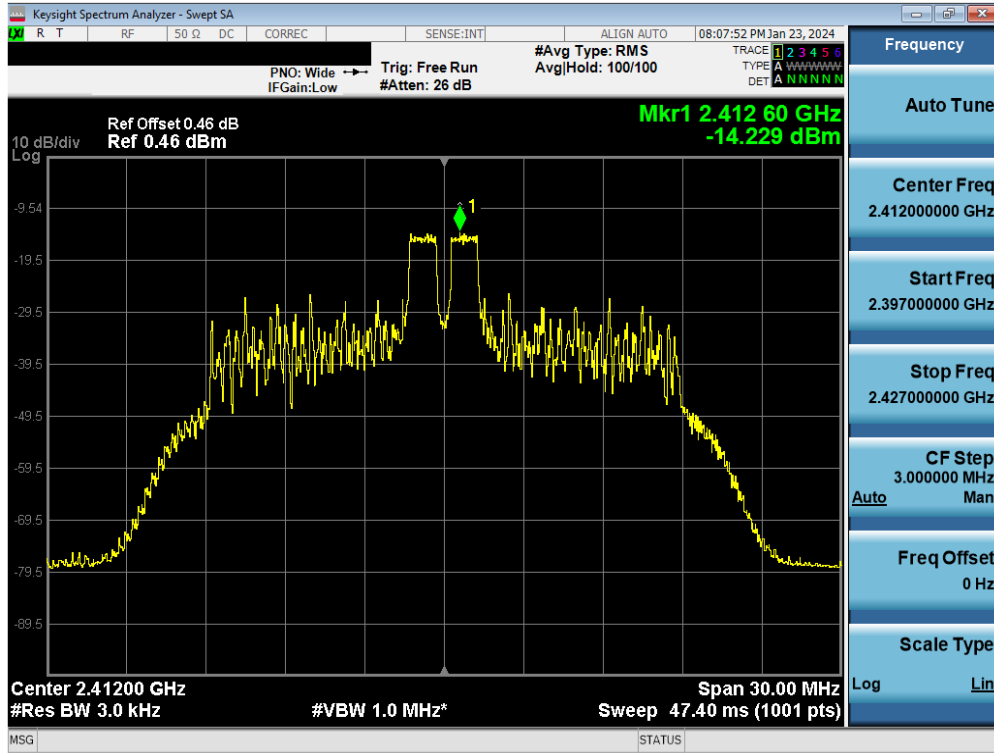
Plot 7-51. Power Spectral Density Plot Antenna WF8 (802.11ax OFDMA – RU26 Index 4 – Ch. 1)
