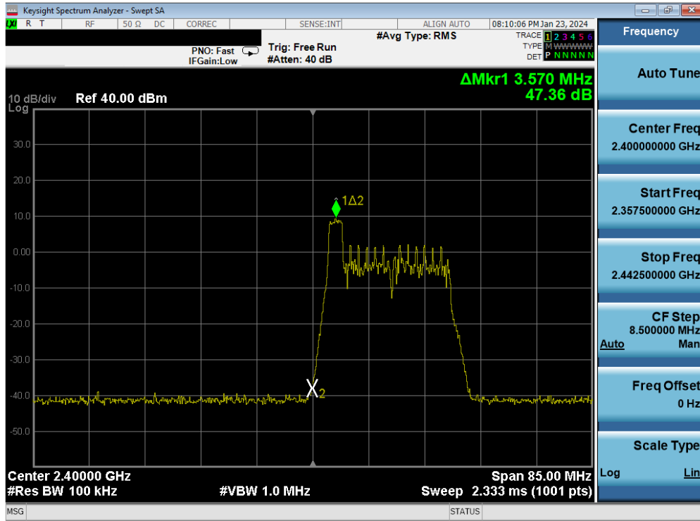
Plot 7-73. Band Edge Antenna WF8 (802.11ax OFDMA – RU26 Index 0 – Ch. 1)
