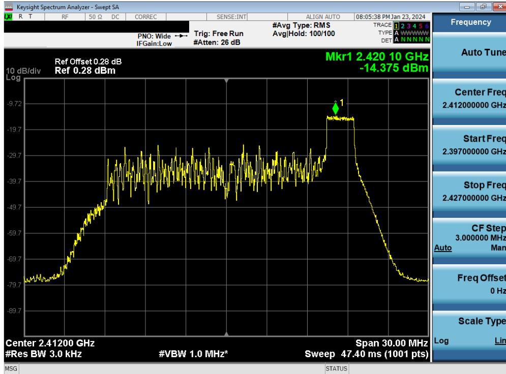
Plot 7-27. Power Spectral Density Plot Antenna WF8 (802.11ax OFDMA – RU26 Index 8 – Ch. 1)
