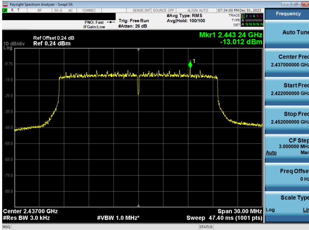
Plot 7-69. Power Spectral Density Plot Antenna WF8 (802.11ax OFDMA – RU242 – Ch. 6)
