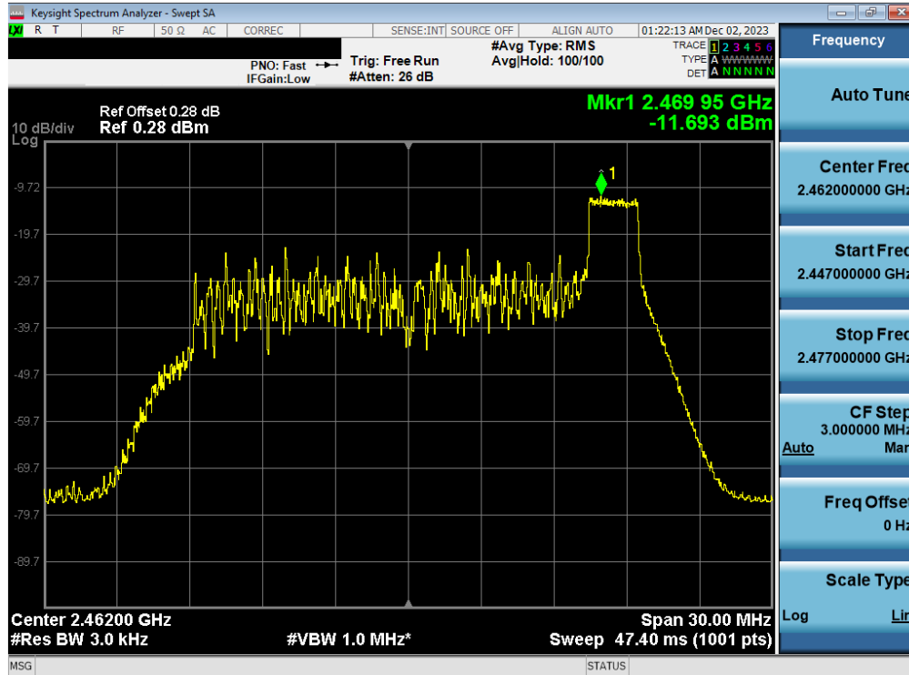
Plot 7-45. Power Spectral Density Plot Antenna WF7b (802.11ax OFDMA – RU26 Index 8 – Ch. 11)
