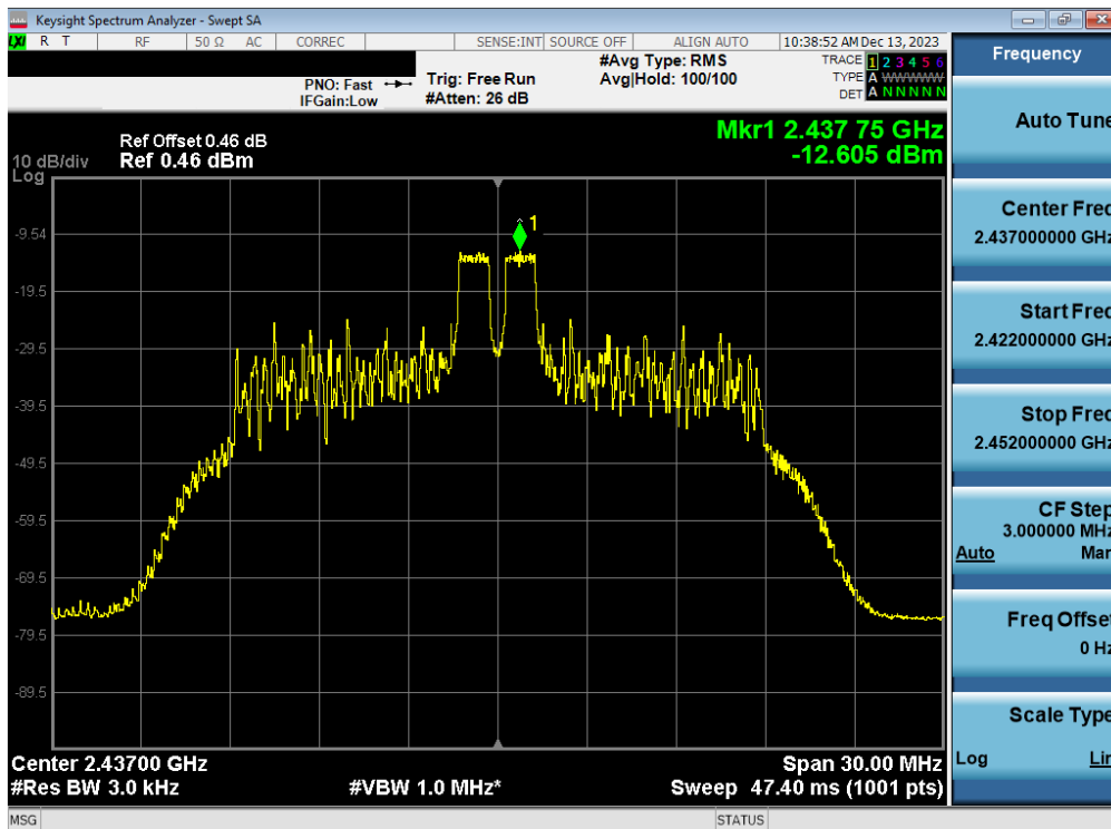
Plot 7-58. Power Spectral Density Plot Antenna WF7b (802.11ax OFDMA – RU26 Index 4 – Ch. 6)
