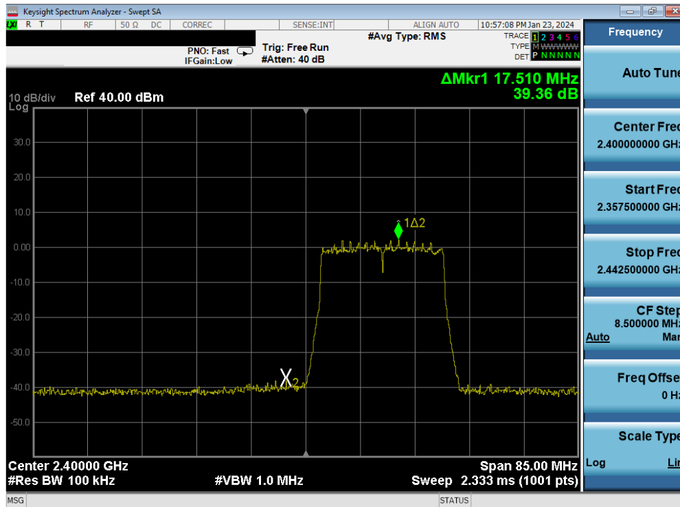
Plot 7-92. Band Edge Antenna WF7b (802.11ax OFDMA – RU242 – Ch. 1)
