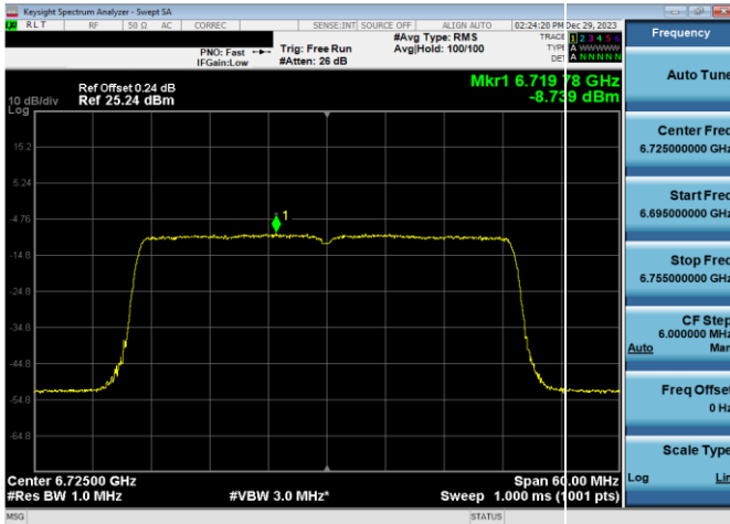
Plot 7-463. LPI Power Spectral Density Plot SDM Antenna WF8 (40MHz 802.11ax RU484 (UNII Band 7) – Ch. 155)
