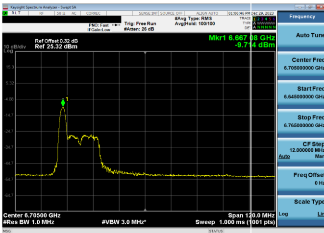
Plot 7-465. LPI Power Spectral Density Plot SDM Antenna WF8 (80MHz 802.11ax RU26 (UNII Band 7) – Ch. 151)
